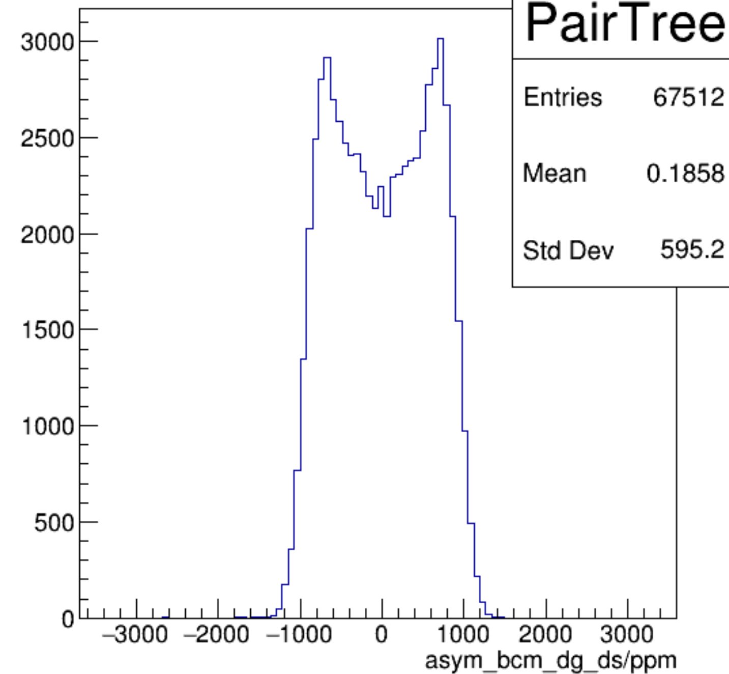
asym_bcm_dg_ds/ppm {ErrorFlag==0}
