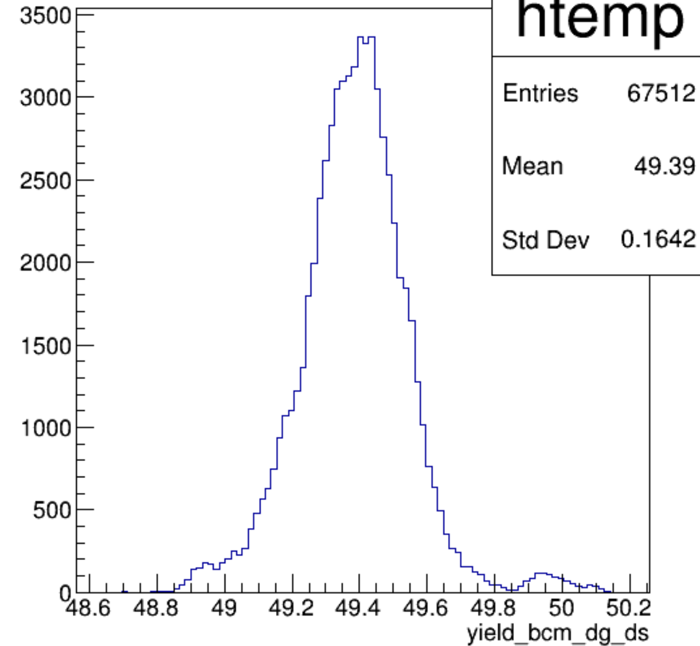
yield_bcm_dg_ds {ErrorFlag==0}
