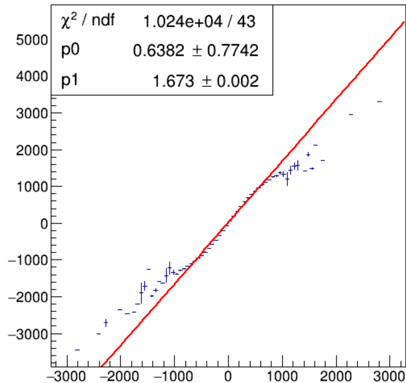
run3552_000_asym_bcm_dg_us_vs_asym_bcm_an_ds3_pr.png
