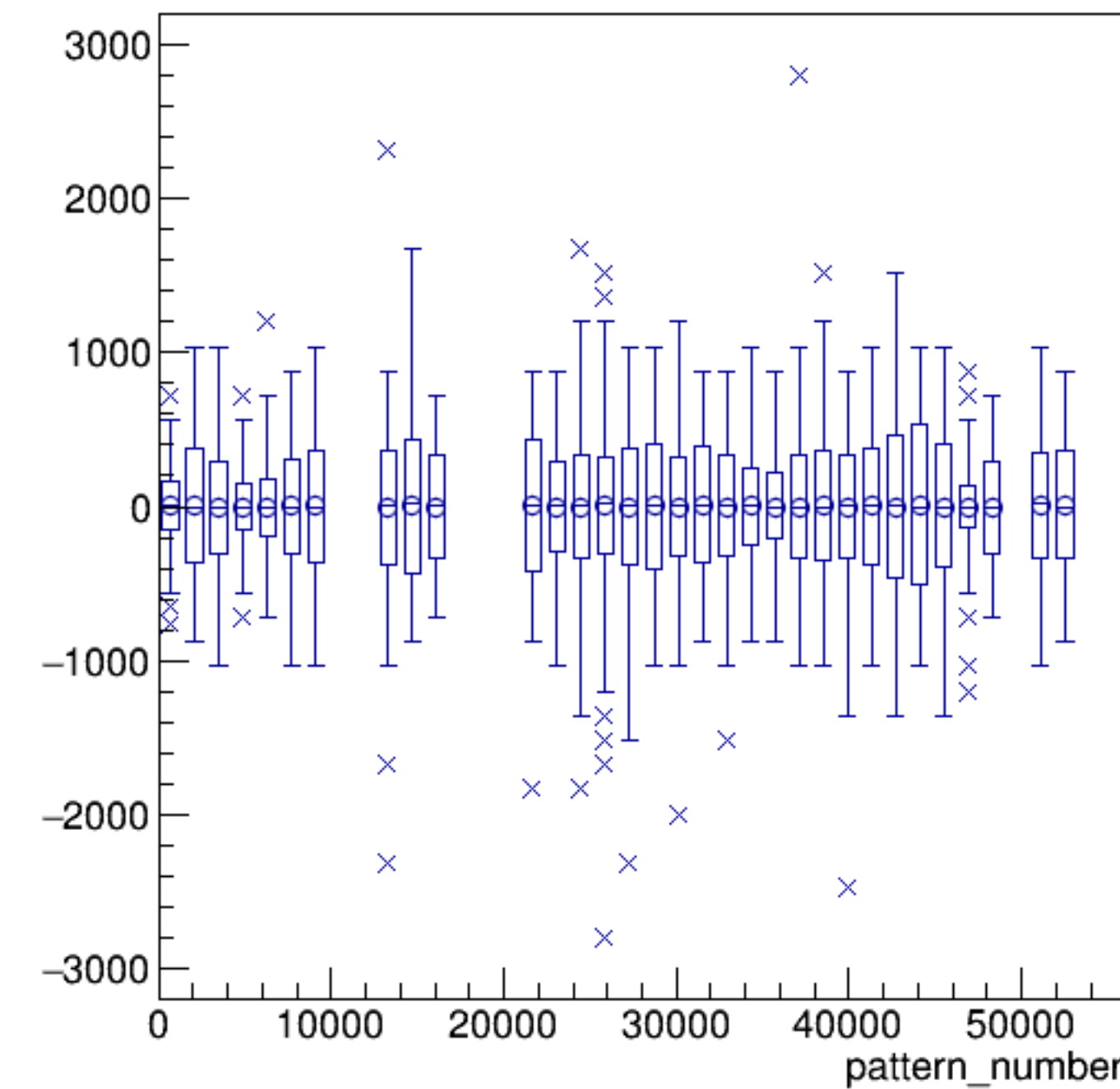
asym_bcm_an_ds3/ppm:pattern_number {ErrorFlag==0}
