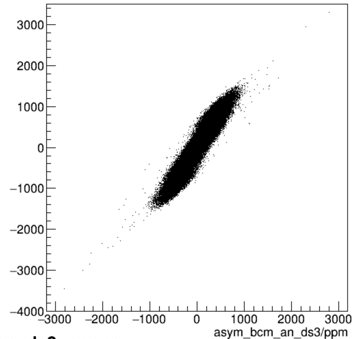
run3552_000_asym_bcm_dg_us_vs_asym_bcm_an_ds3_pr.png
