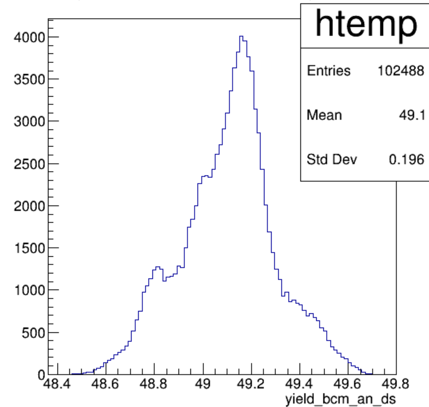
yield_bcm_an_ds {ErrorFlag==0}
