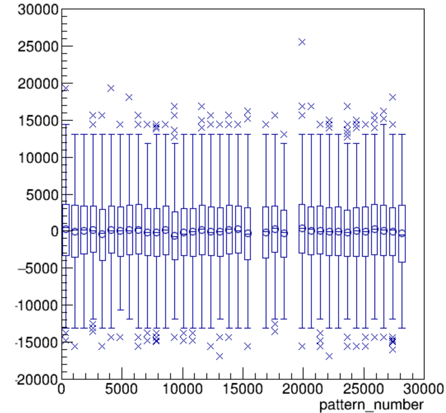
asym_sam3/ppm:pattern_number {ErrorFlag==0}
