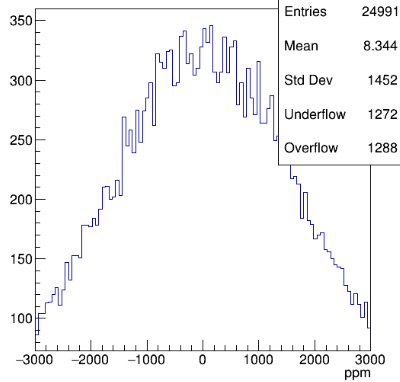
asym_sam8
