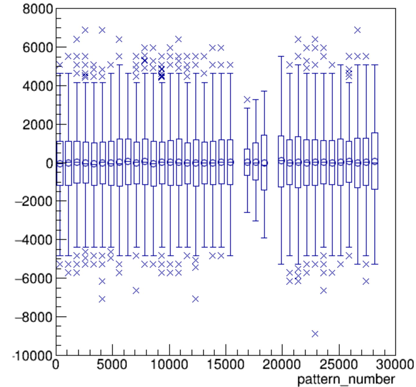
asym_sam1/ppm:pattern_number {ErrorFlag==0}
