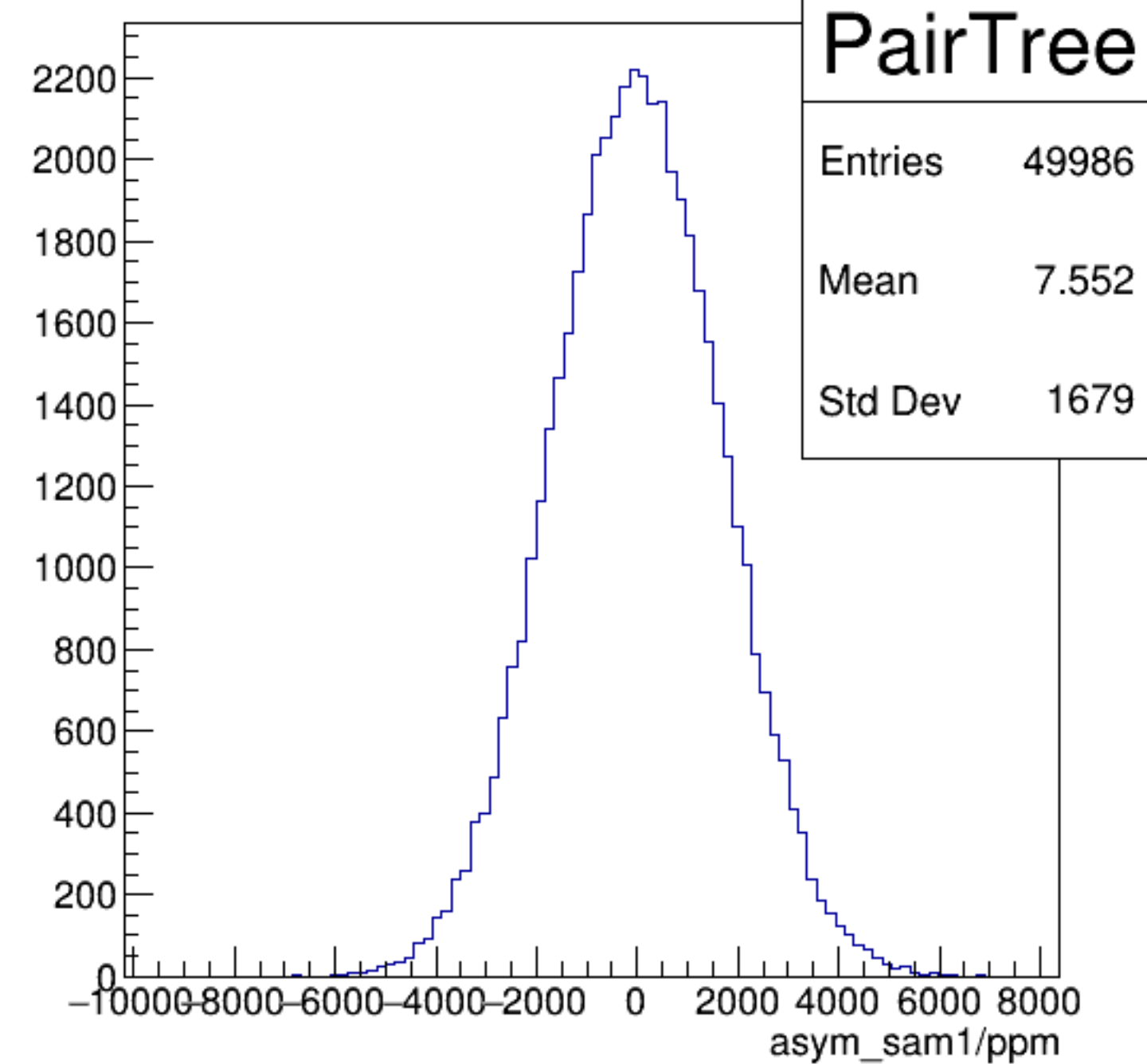
asym_sam1/ppm {ErrorFlag==0}
