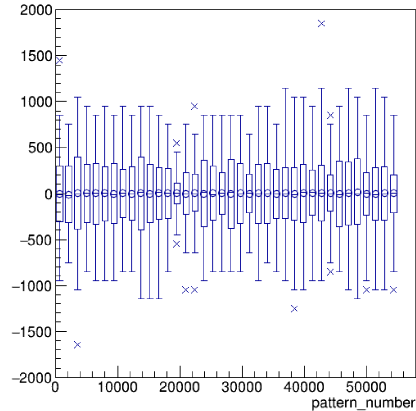
asym_bcm_an_us/ppm:pattern_number {ErrorFlag==0}
