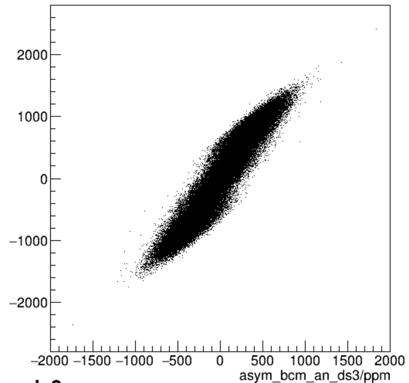
run3568_000_asym_bcm_dg_us_vs_asym_bcm_an_ds3_pr.png
