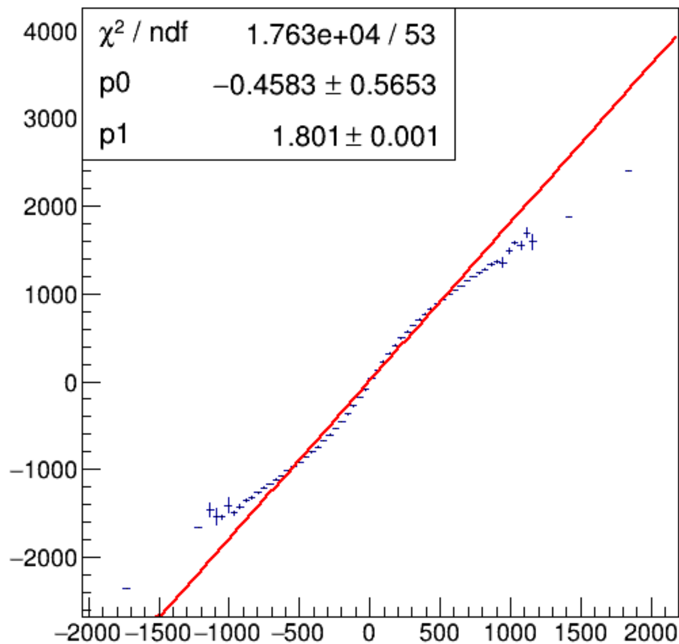
run3568_000_asym_bcm_dg_us_vs_asym_bcm_an_ds_pr.png
