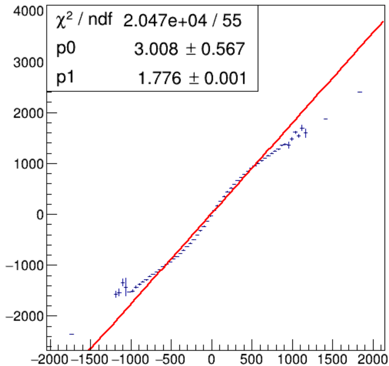
run3568_000_asym_bcm_dg_us_vs_asym_bcm_an_ds3_pr.png
