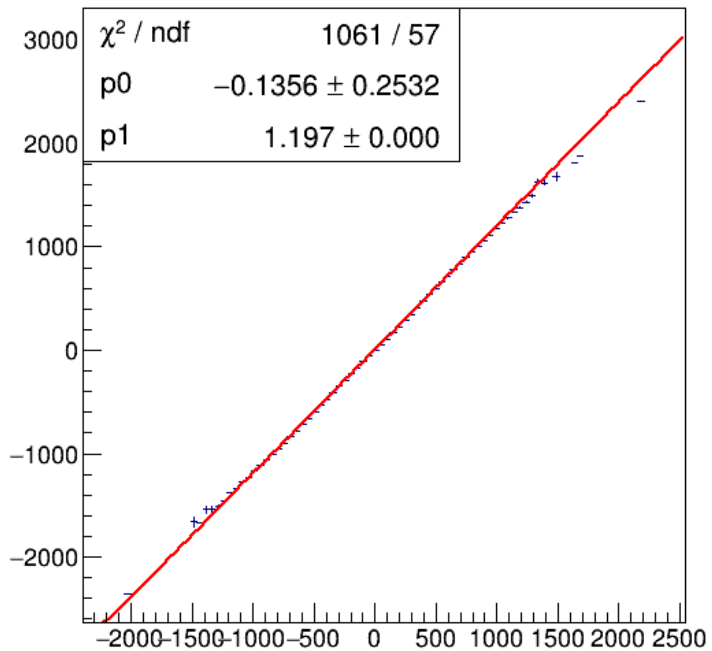
run3568_000_asym_bcm_dg_us_vs_asym_bcm_dg_ds_pr.png
