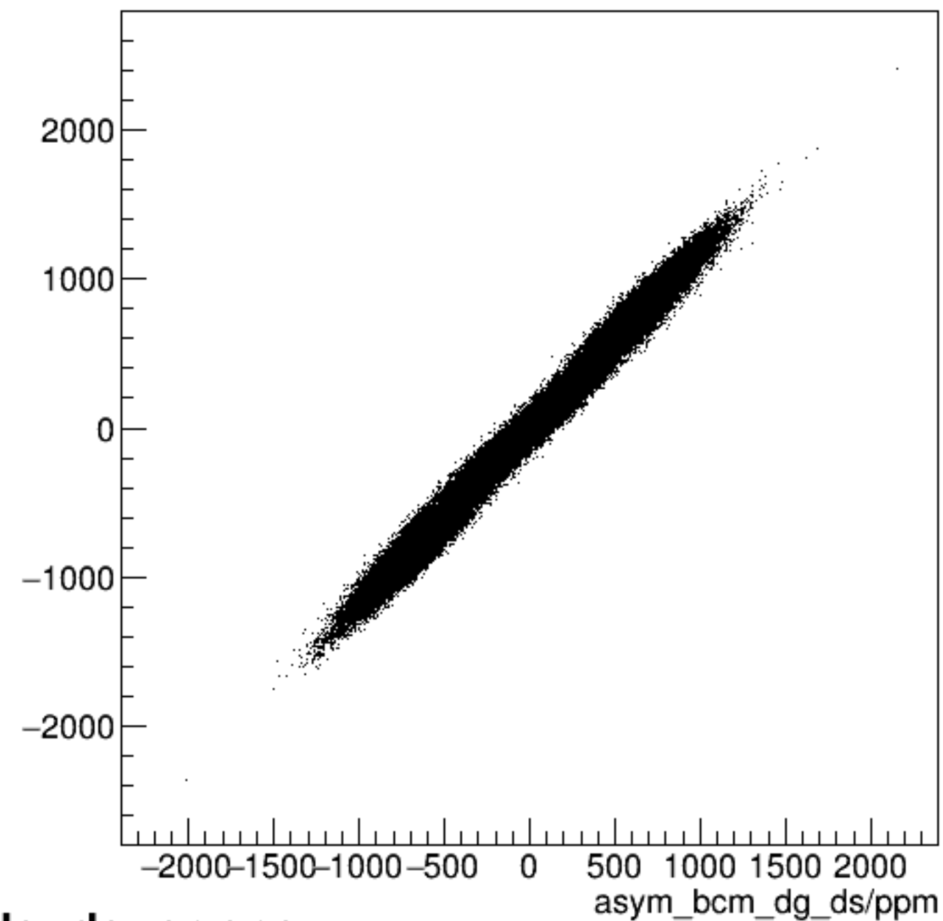
run3568_000_asym_bcm_dg_us_vs_asym_bcm_dg_ds_pr.png
