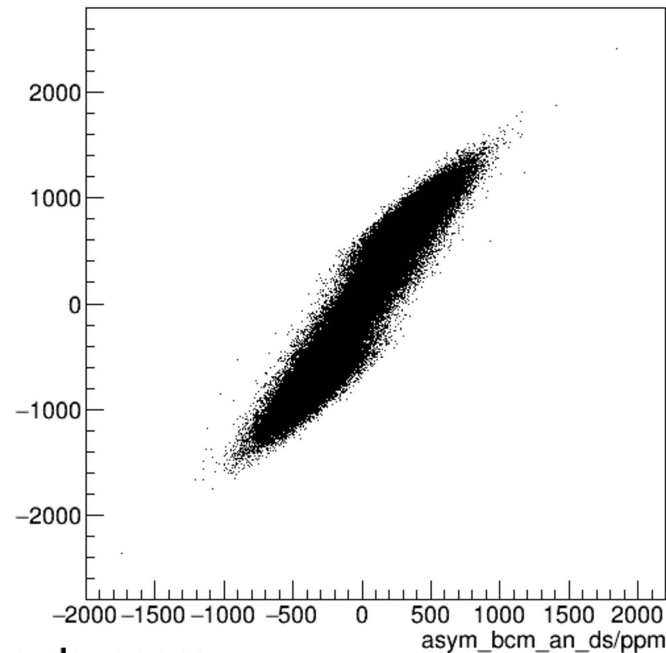
run3568_000_asym_bcm_dg_us_vs_asym_bcm_an_ds_pr.png
