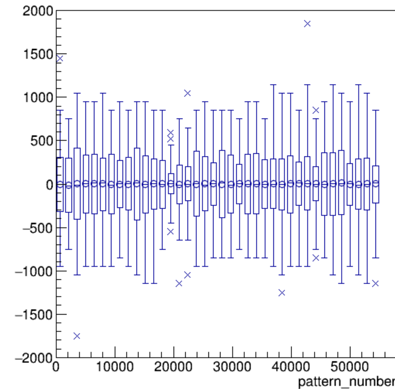
asym_bcm_an_ds3/ppm:pattern_number {ErrorFlag==0}
