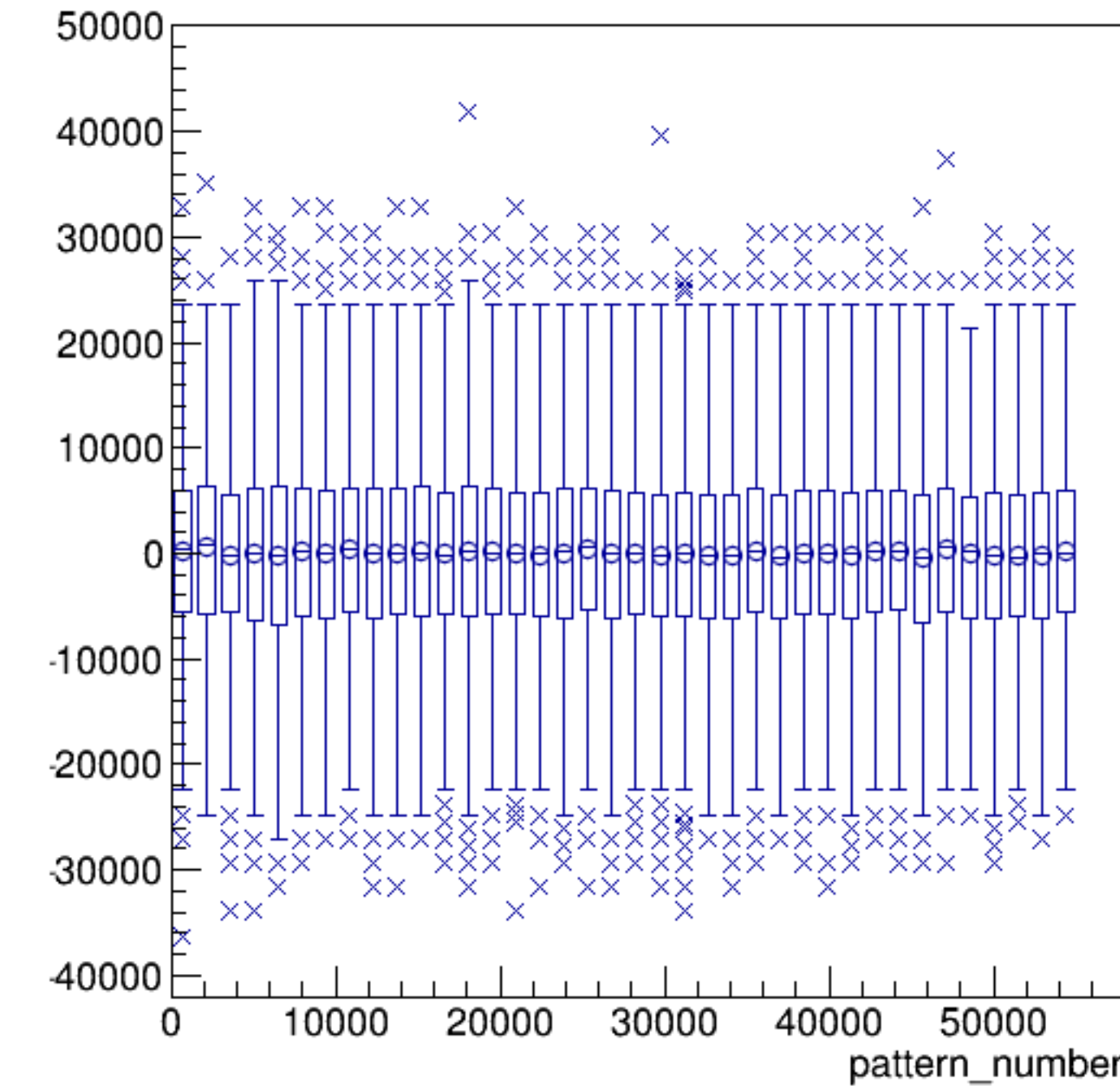
asym_sam2/ppm:pattern_number {ErrorFlag==0}
