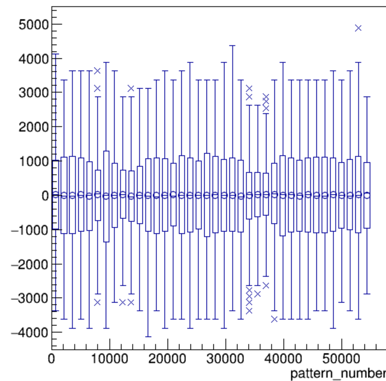
asym_usl/ppm:pattern_number {ErrorFlag==0}
