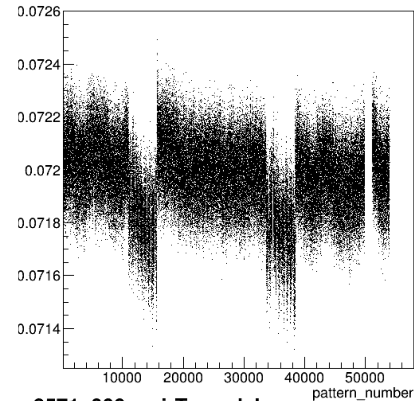
yield_dsl:pattern_number {ErrorFlag==0}
