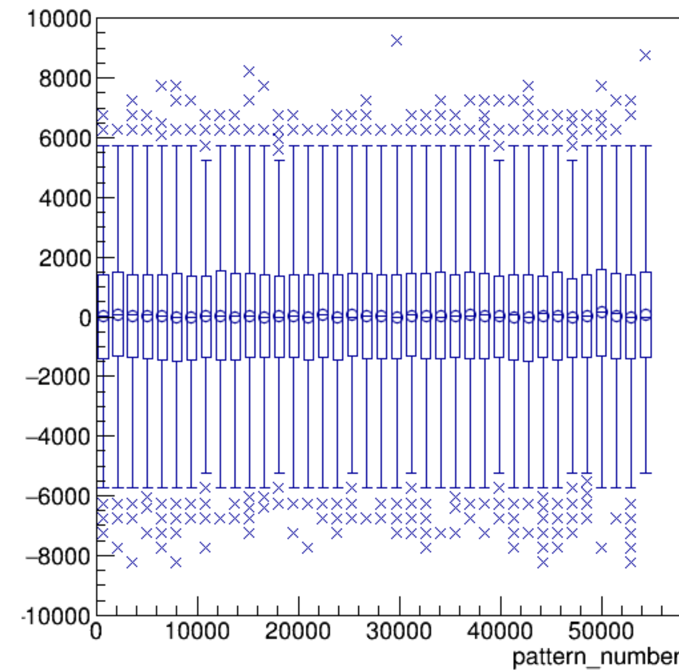
asym_usr/ppm:pattern_number {ErrorFlag==0}
