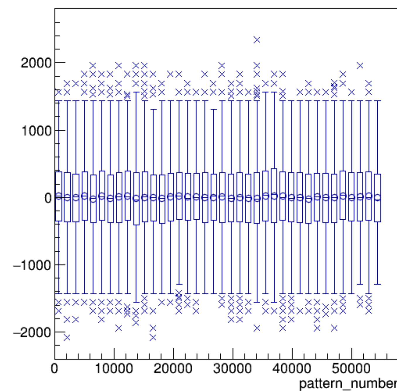
asym_usl/ppm:pattern_number {ErrorFlag==0}
