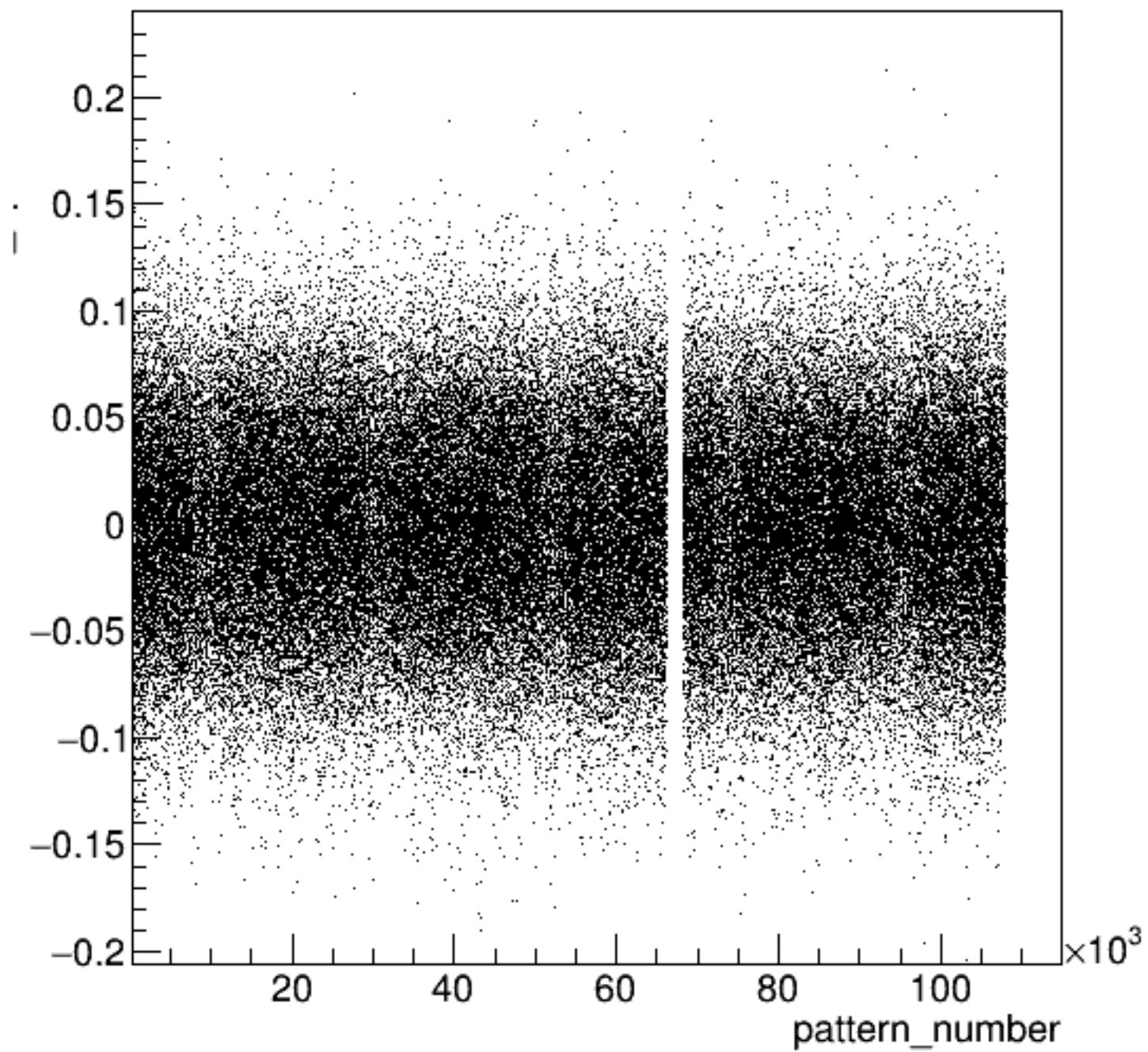
diff_bpm4acX/um:pattern_number {ErrorFlag==0}
