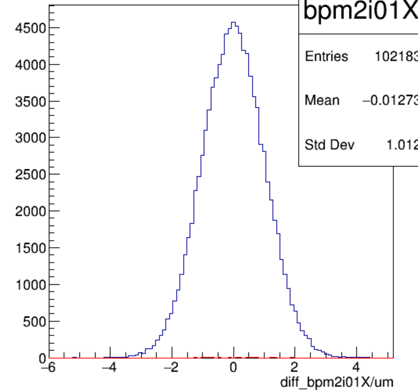
diff_bpm2i01X/um {ErrorFlag==0}
