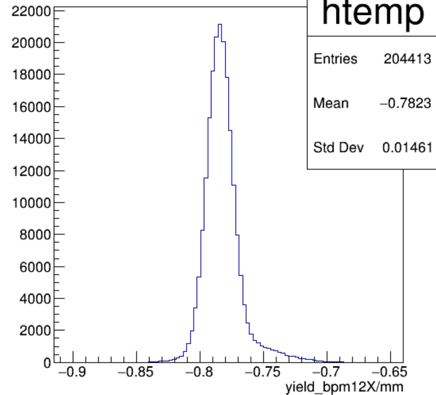
yield_bpm12X/mm {ErrorFlag==0}
