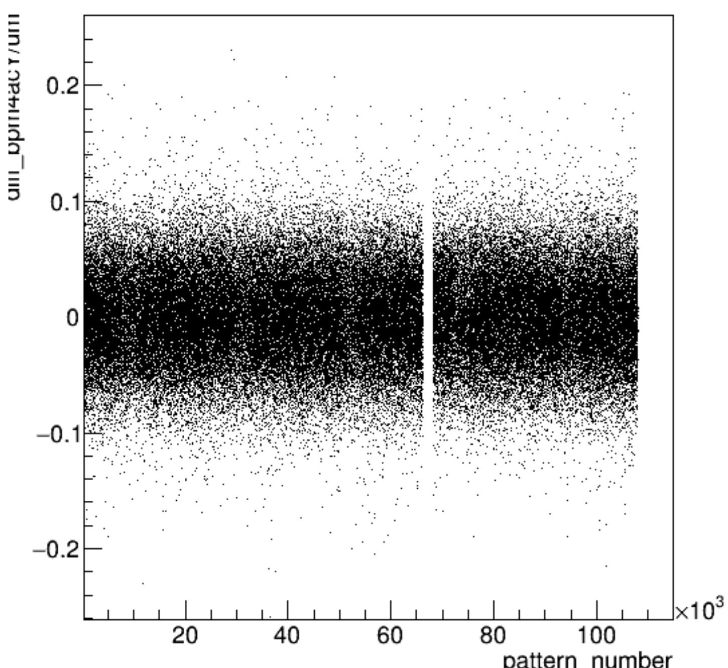
diff_bpm4acY/um:pattern_number {ErrorFlag==0}
