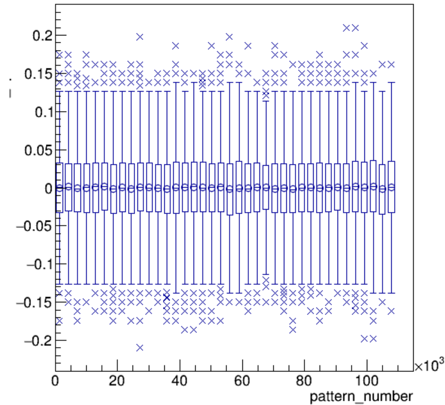
diff_bpm4acX/um:pattern_number {ErrorFlag==0}
