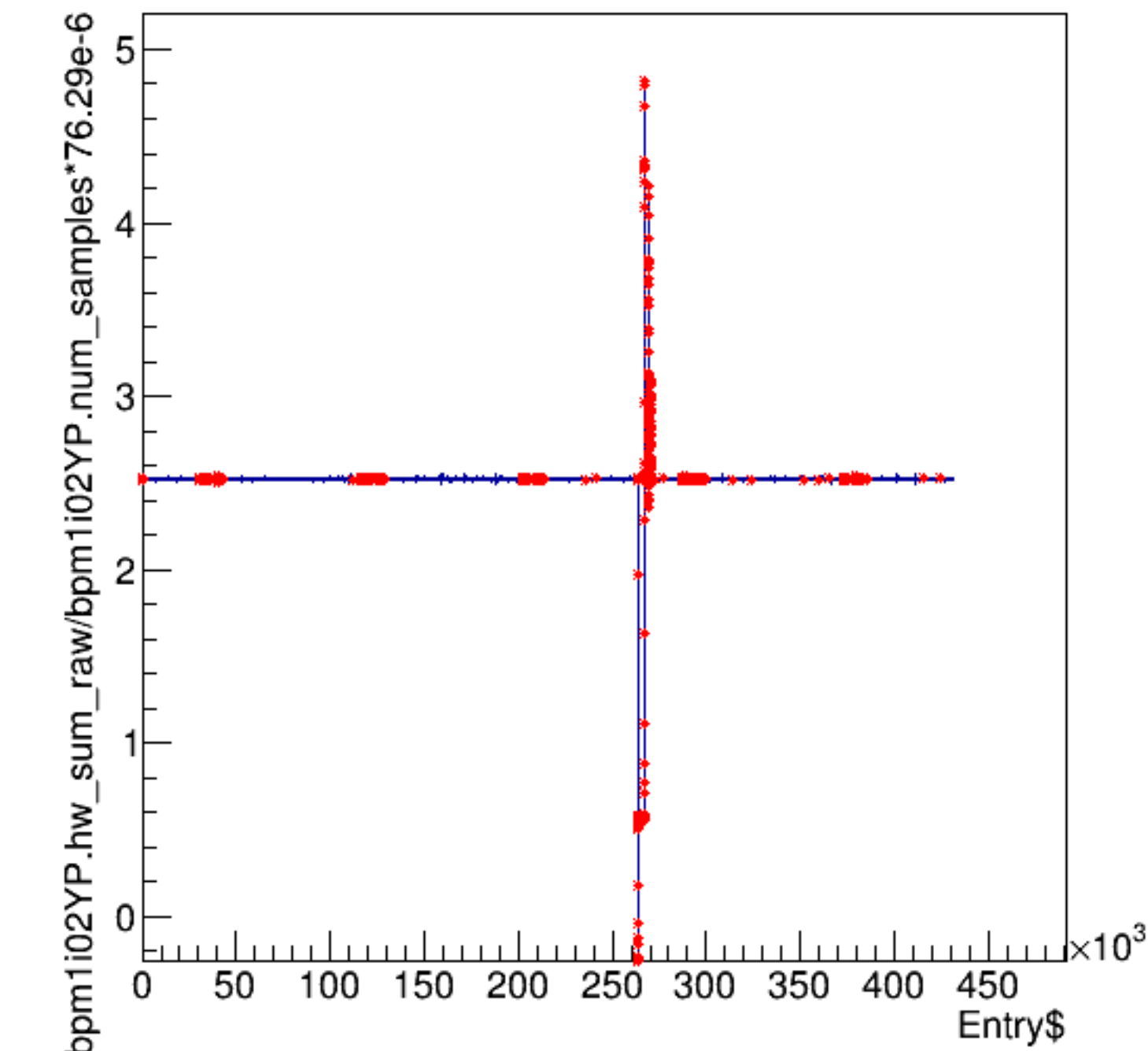
bpm1i02YP.hw_sum_raw/bpm1i02YP.num_samples*76.29e-6:Entry$
