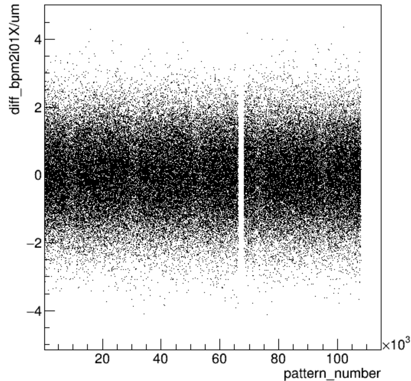
diff_bpm2i01X/um:pattern_number {ErrorFlag==0}
