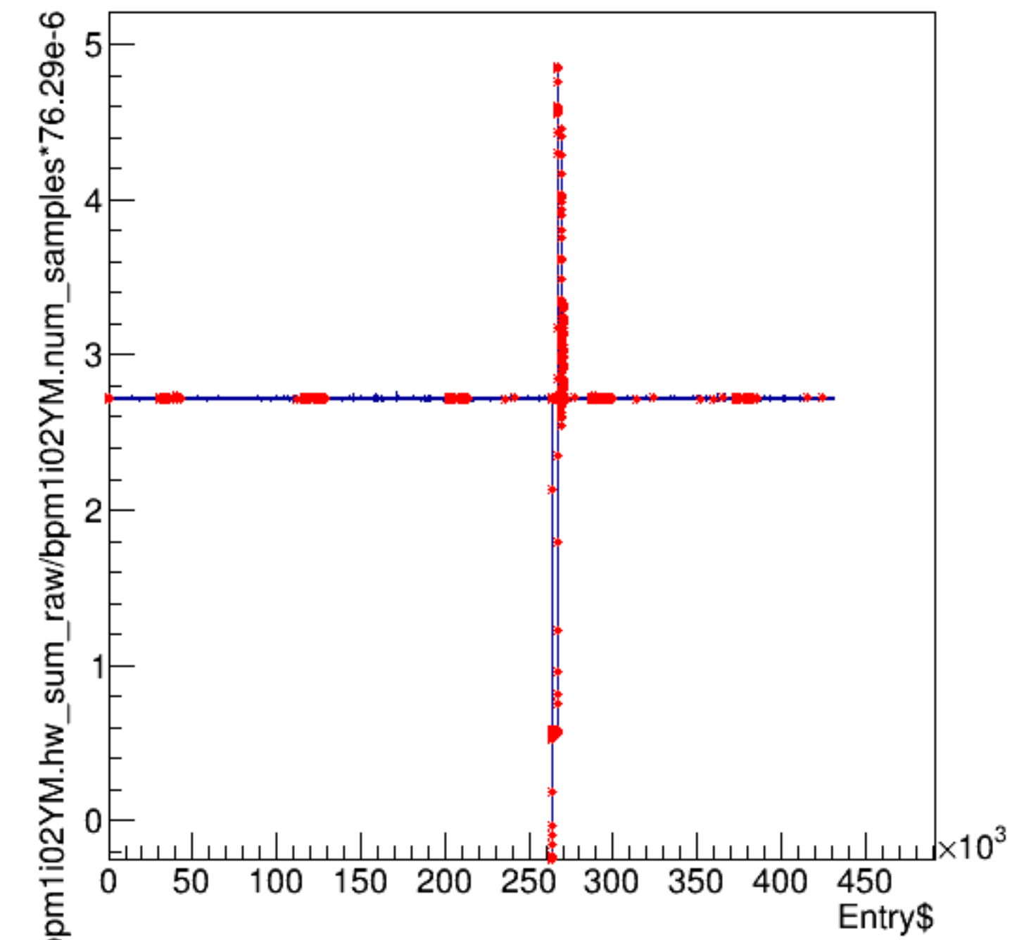
bpm1i02YM.hw_sum_raw/bpm1i02YM.num_samples*76.29e-6:Entry$
