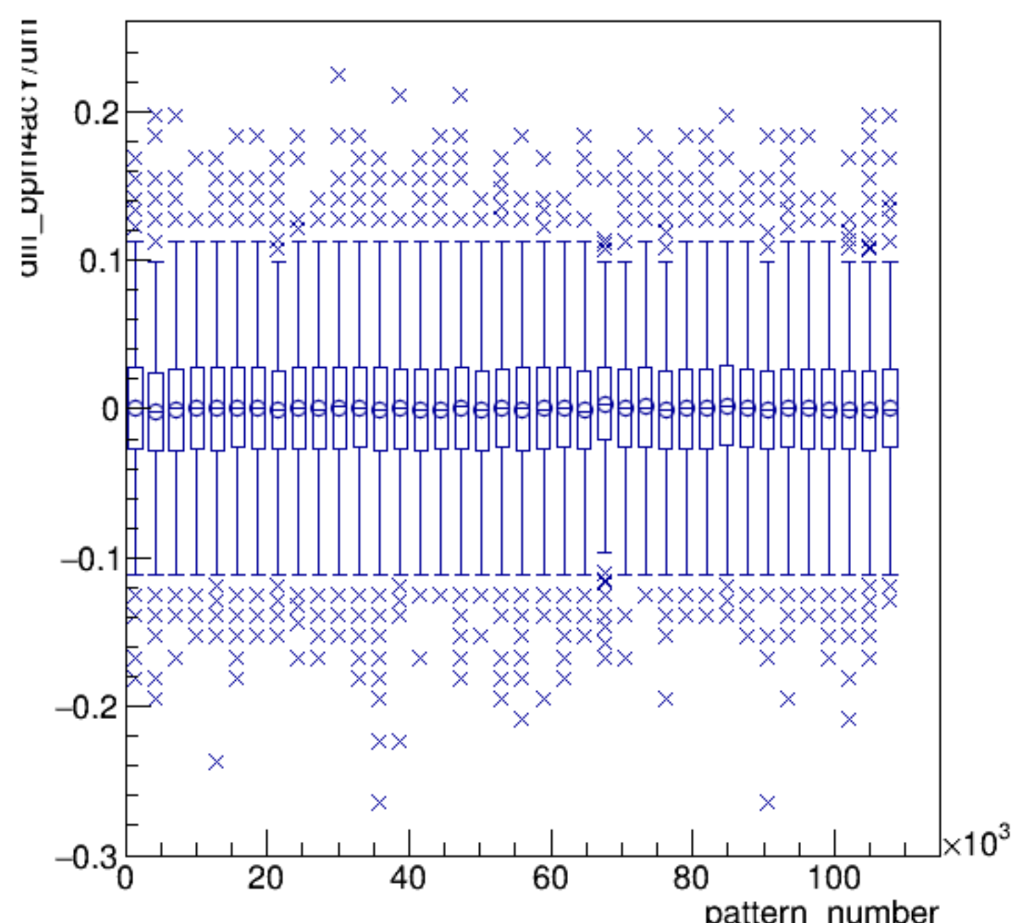
diff_bpm4acY/um:pattern_number {ErrorFlag==0}
