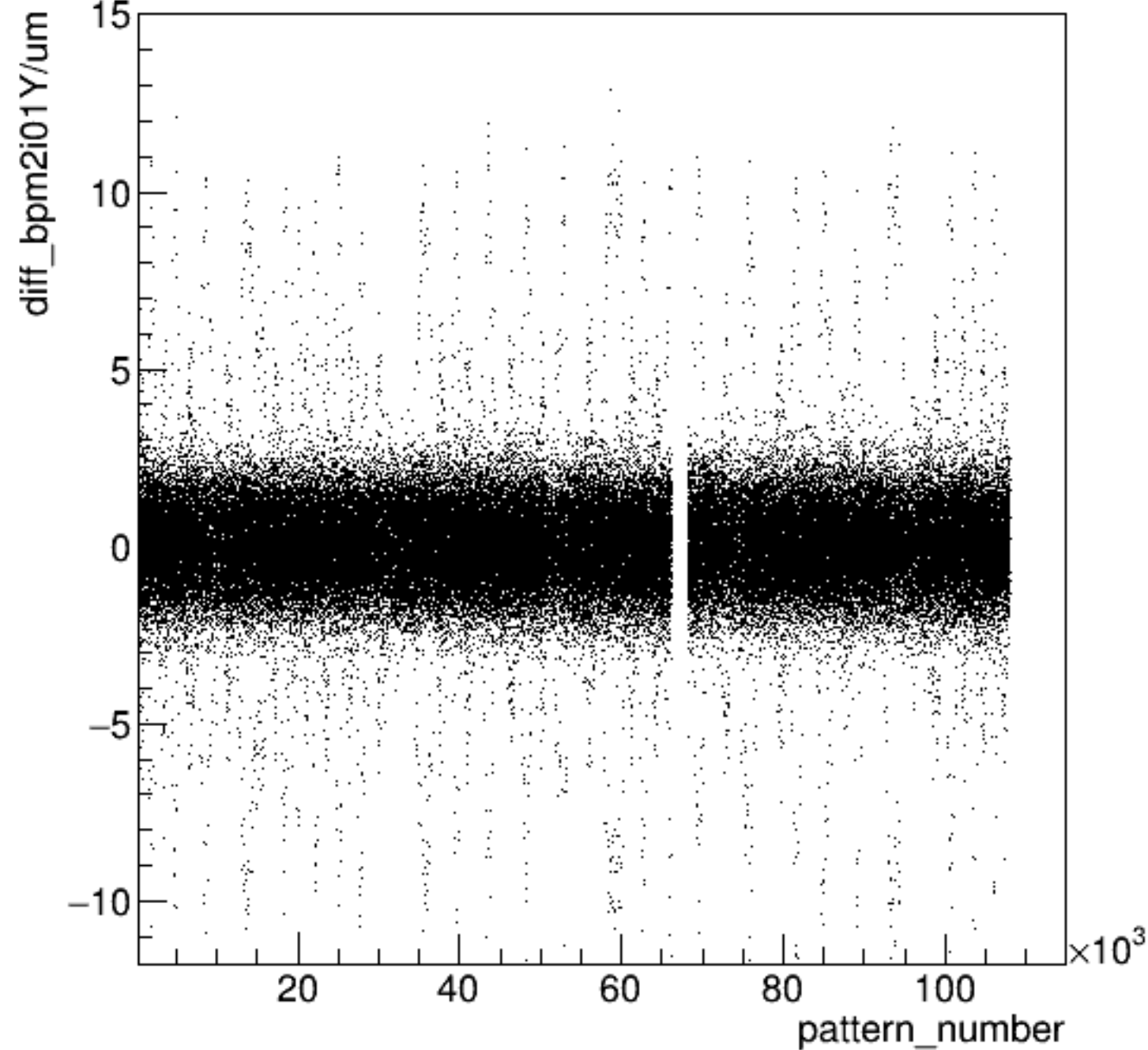
diff_bpm2i01Y/um:pattern_number {ErrorFlag==0}
