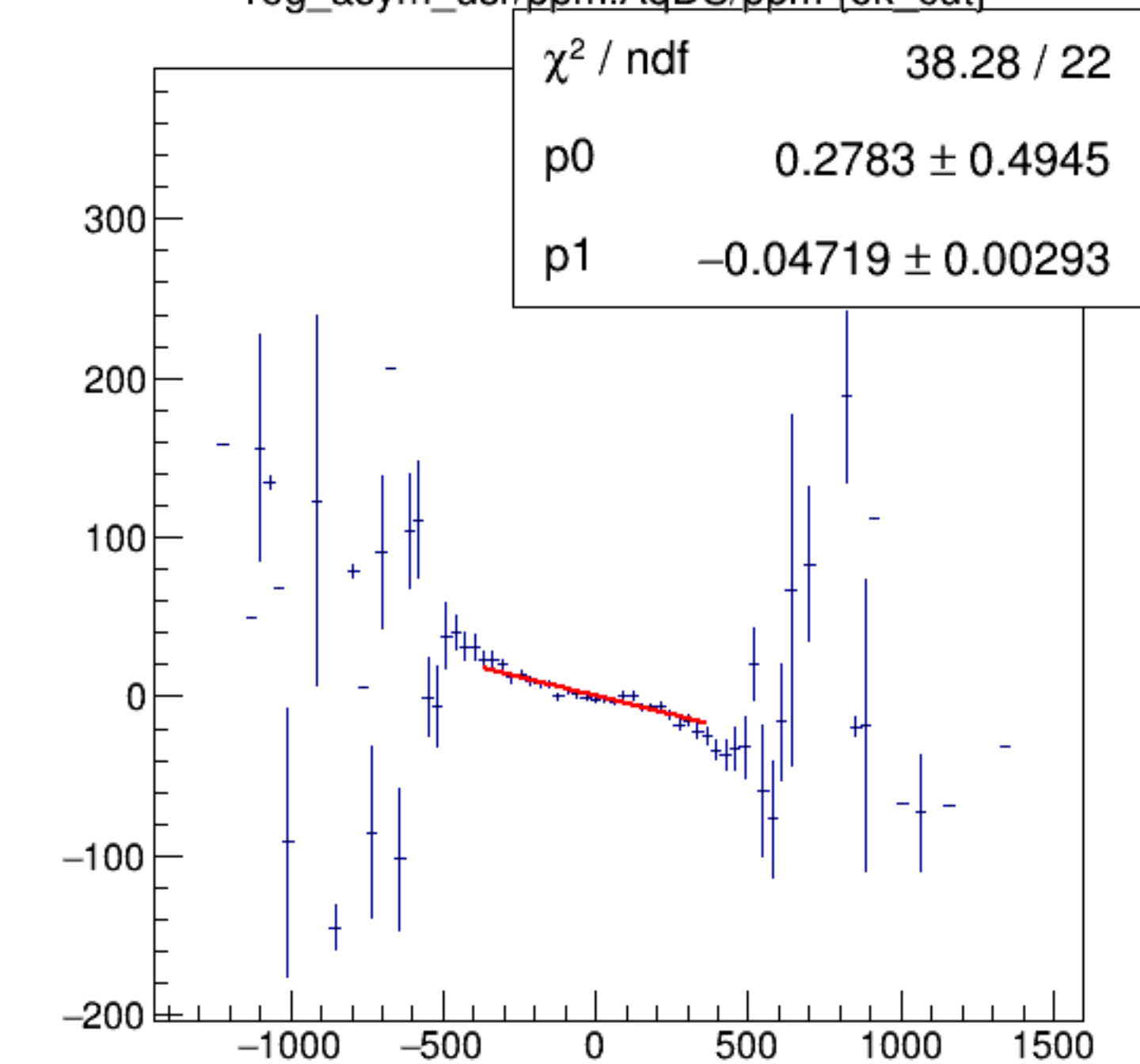
reg_asym_usr/ppm:AqDS/ppm {ok_cut}
