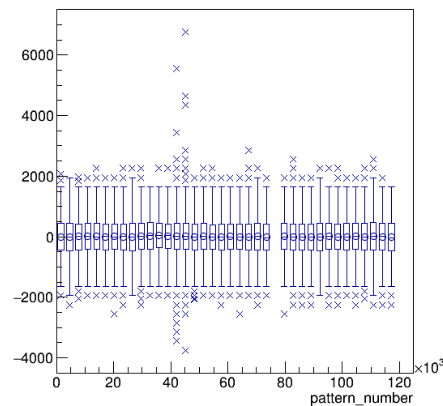
asym_usr/ppm:pattern_number {ErrorFlag==0}
