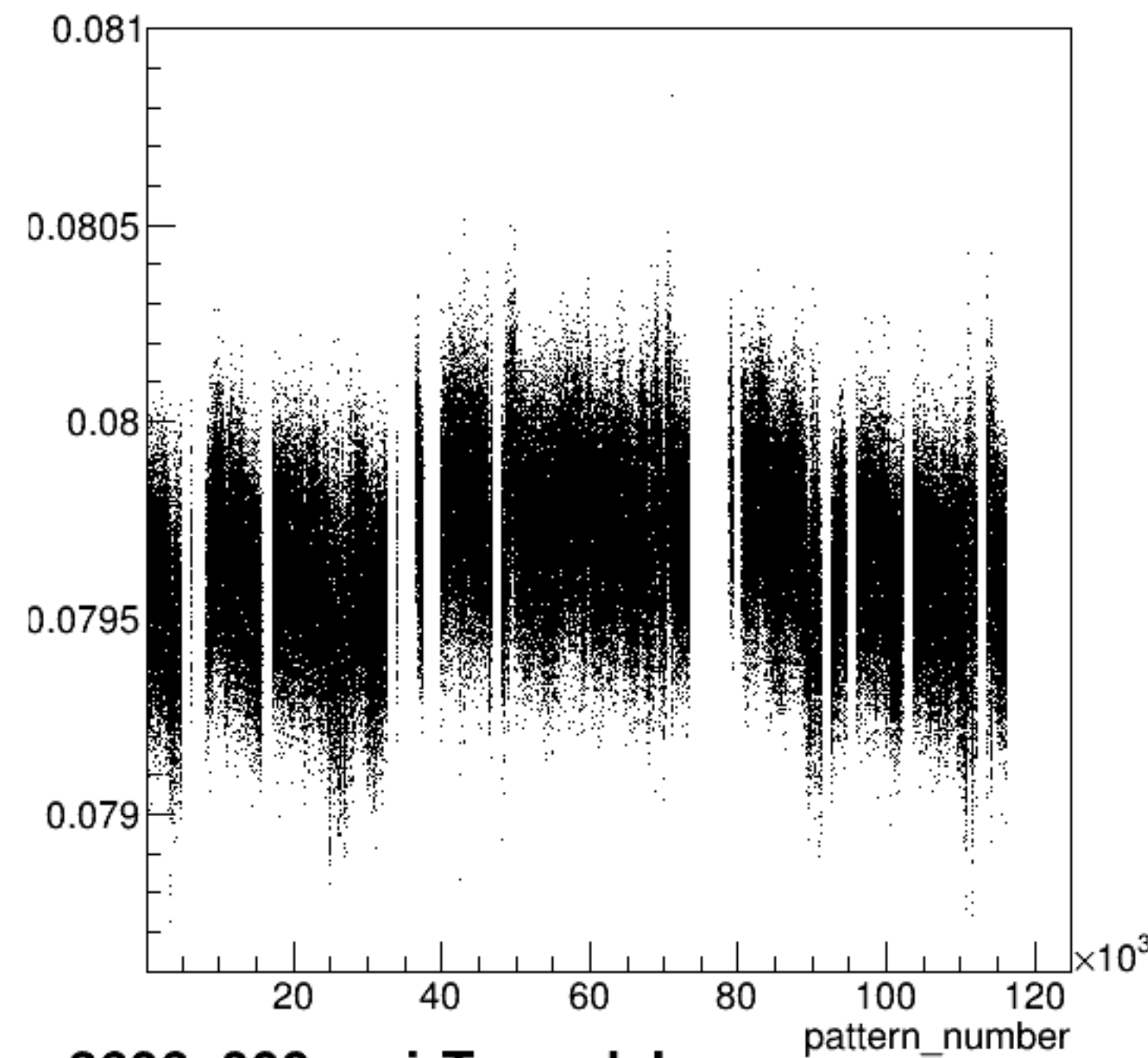
yield_dsl:pattern_number {ErrorFlag==0}
