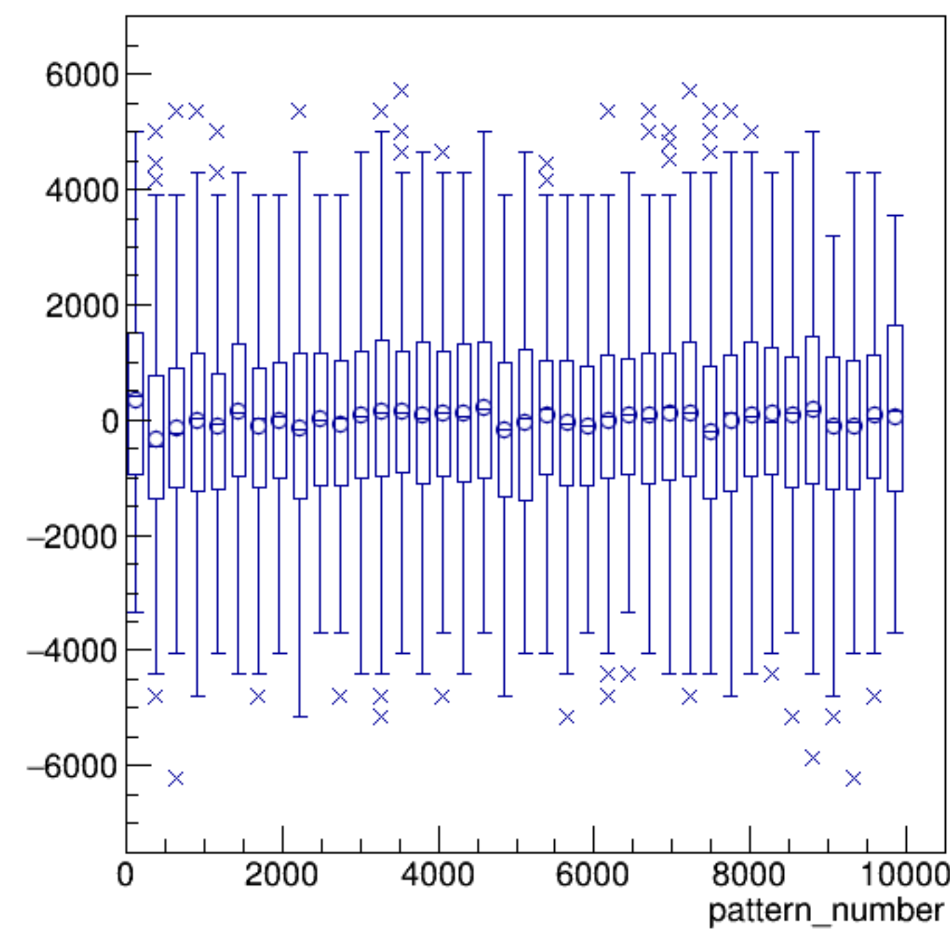
asym_sam5/ppm:pattern_number {ErrorFlag==0}
