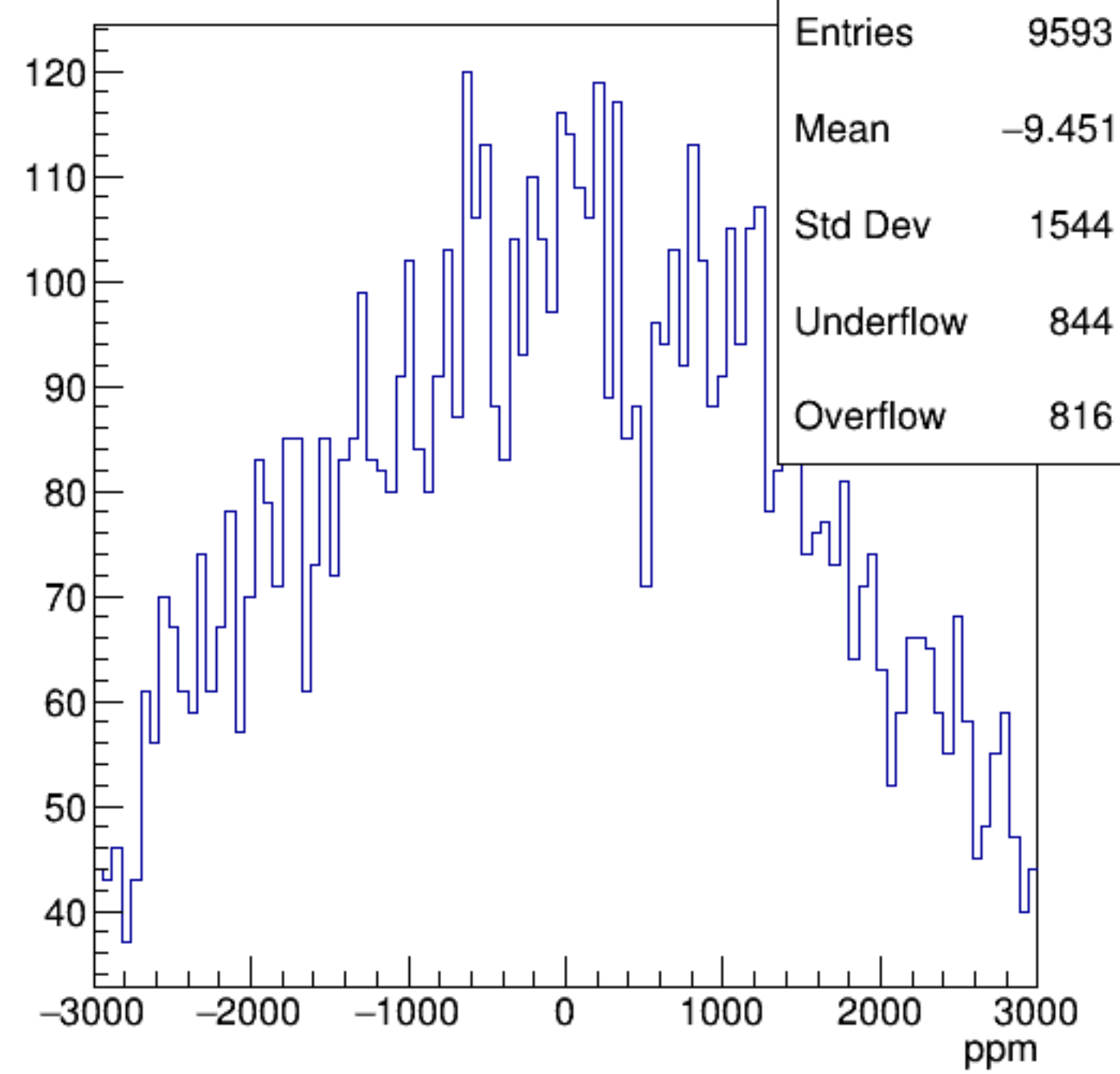
asym_sam8
