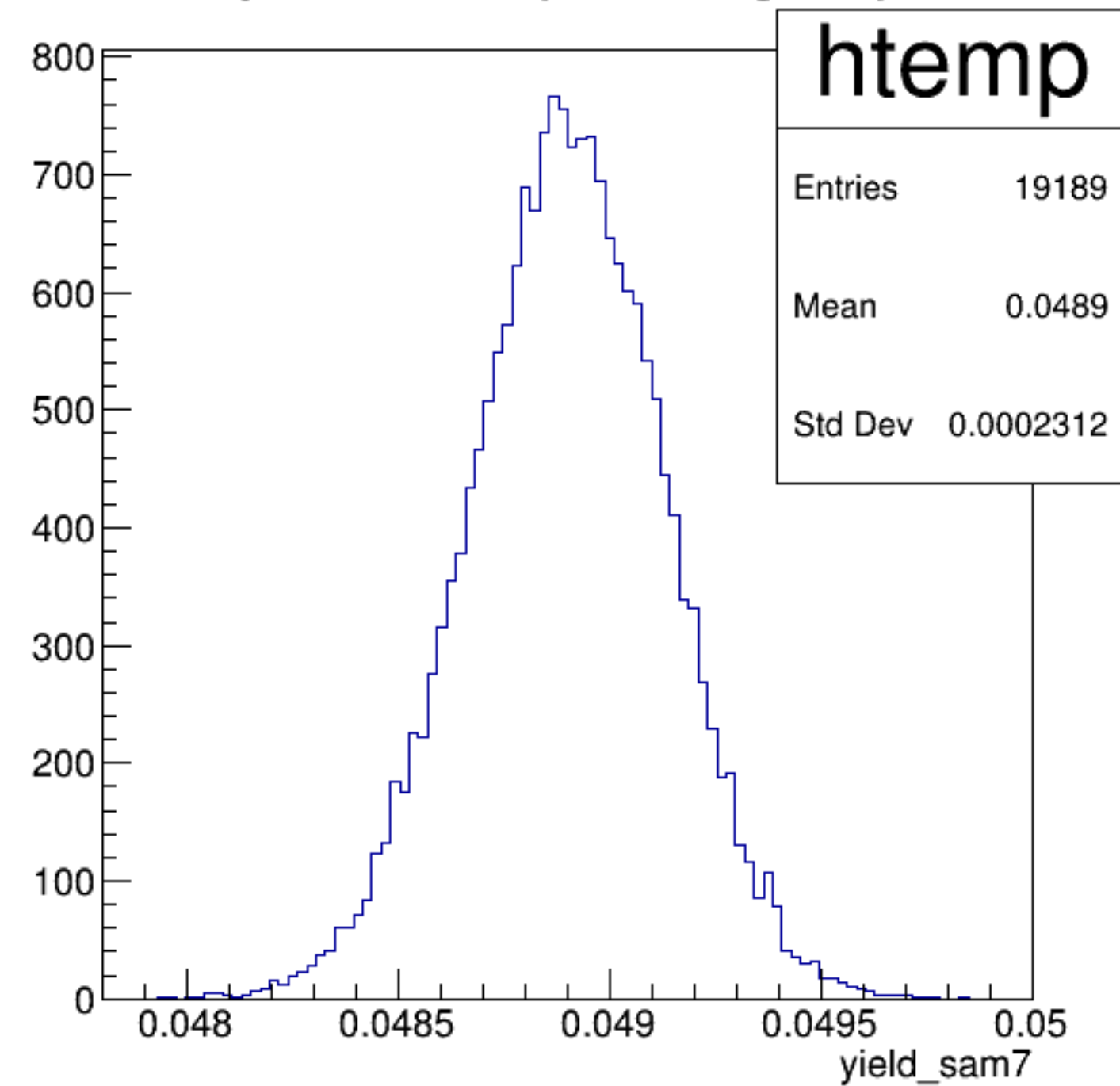
yield_sam7 {ErrorFlag==0}
