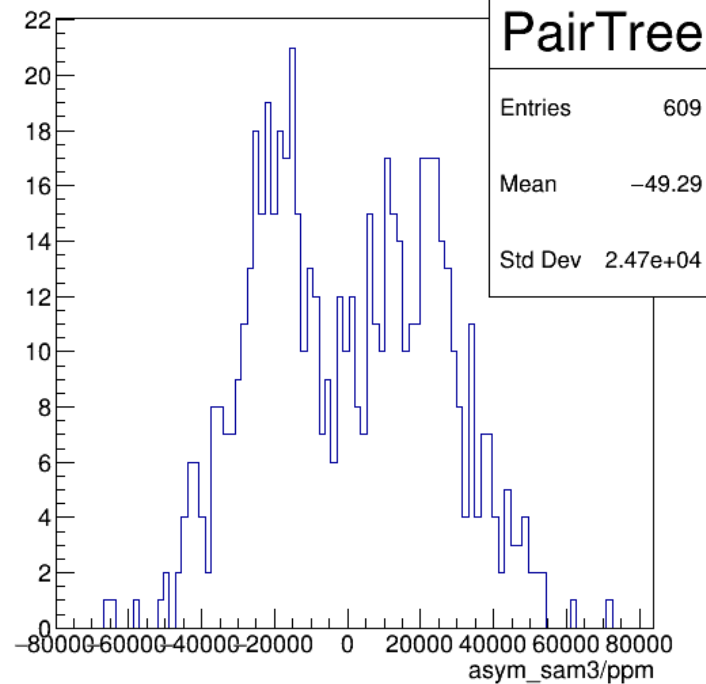
asym_sam3/ppm {ErrorFlag==0}
