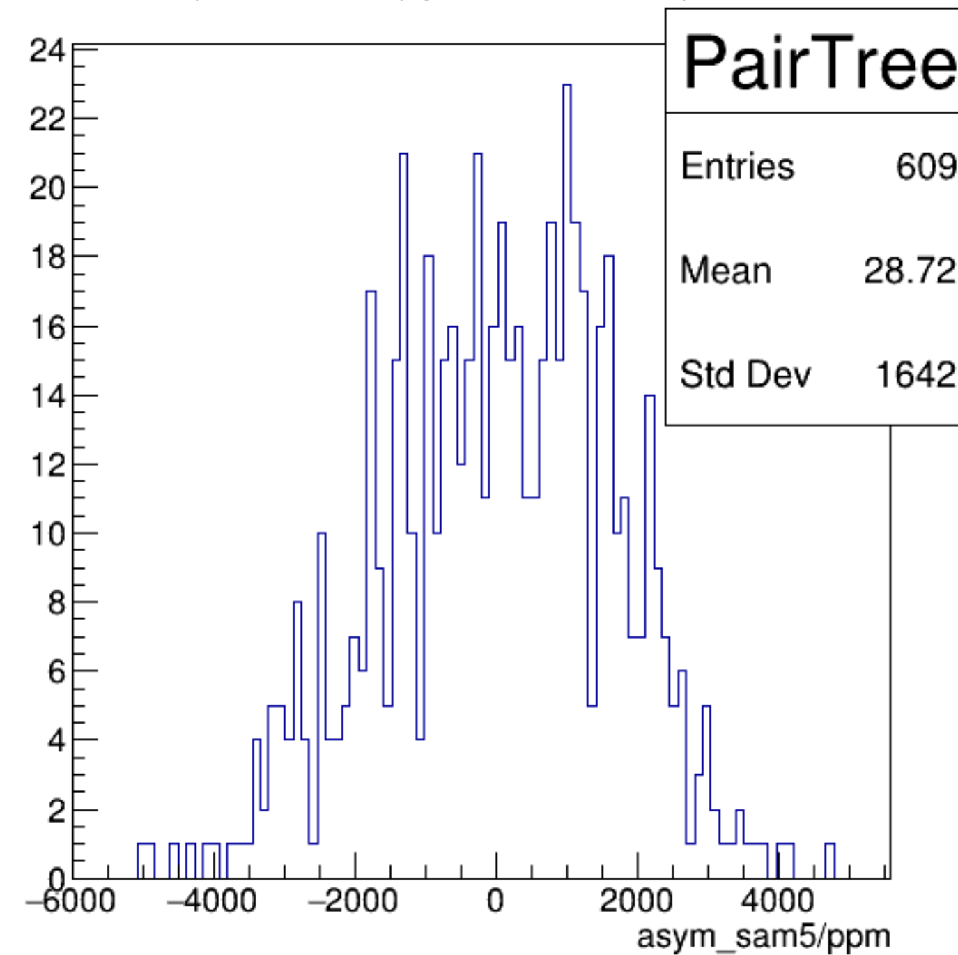
asym_sam5/ppm {ErrorFlag==0}
