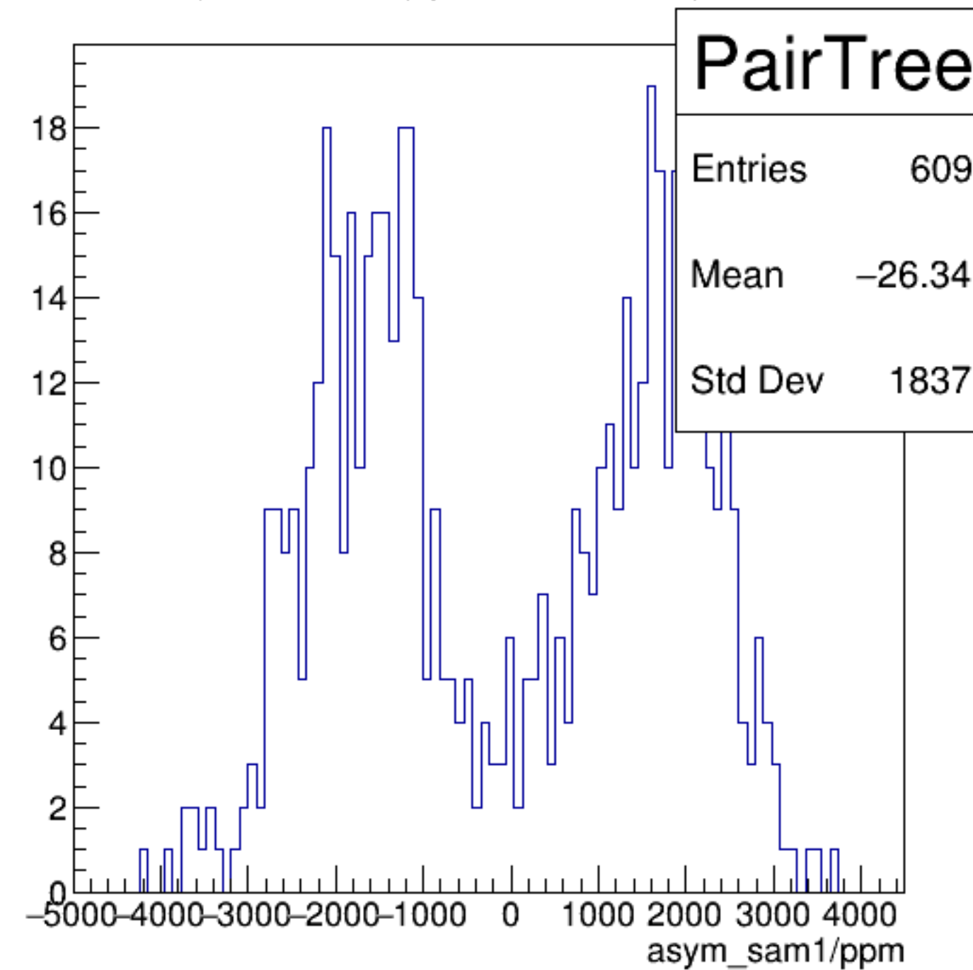
asym_sam1/ppm {ErrorFlag==0}
