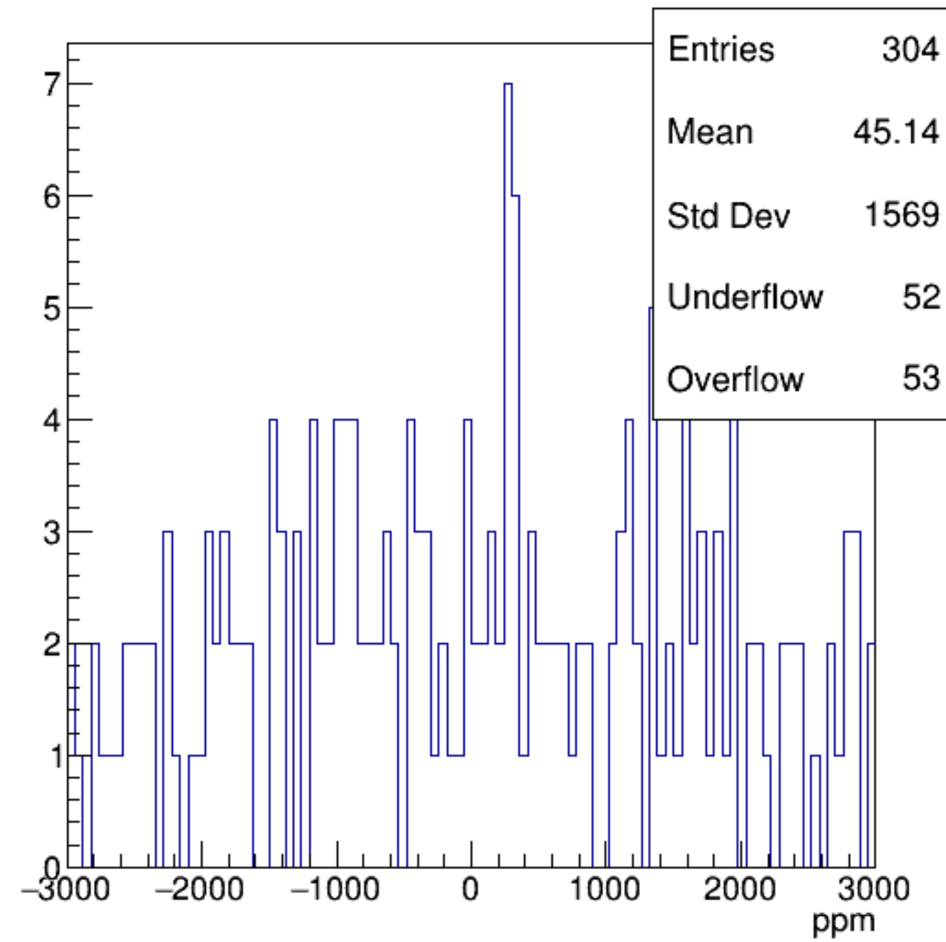
asym_sam7
