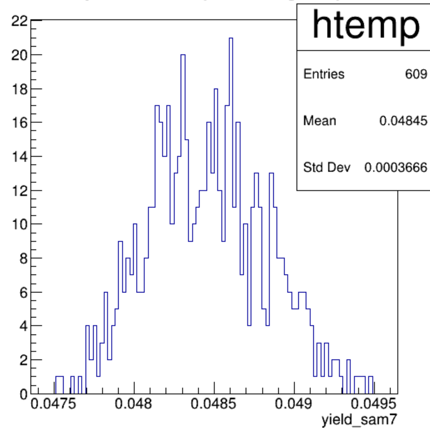
yield_sam7 {ErrorFlag==0}
