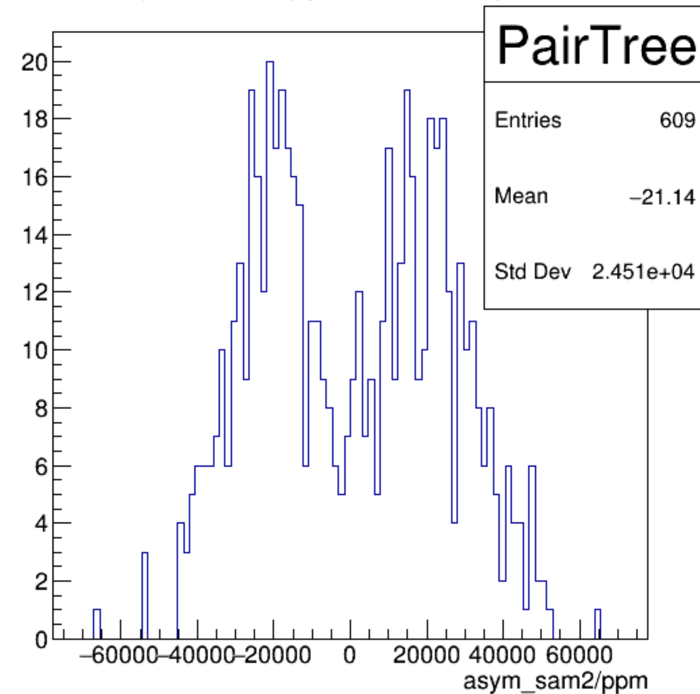
asym_sam2/ppm {ErrorFlag==0}
