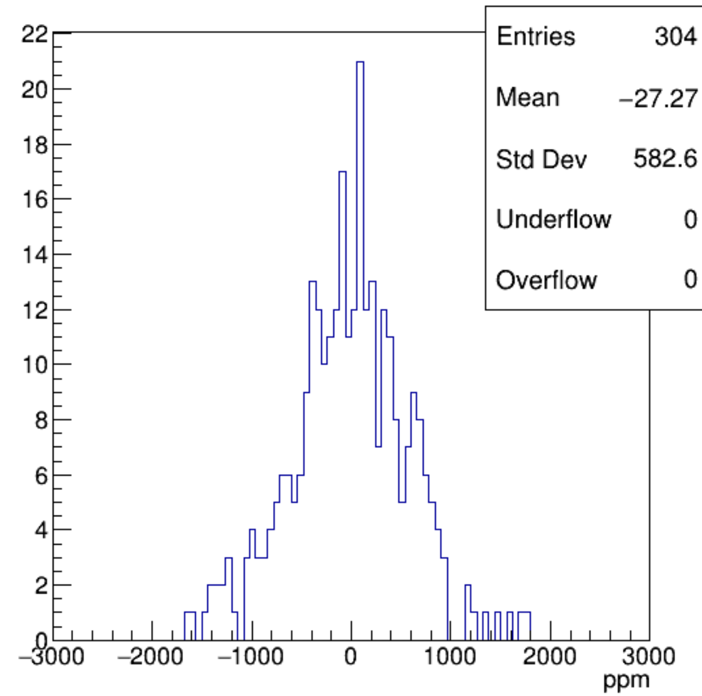
asym_sam1
