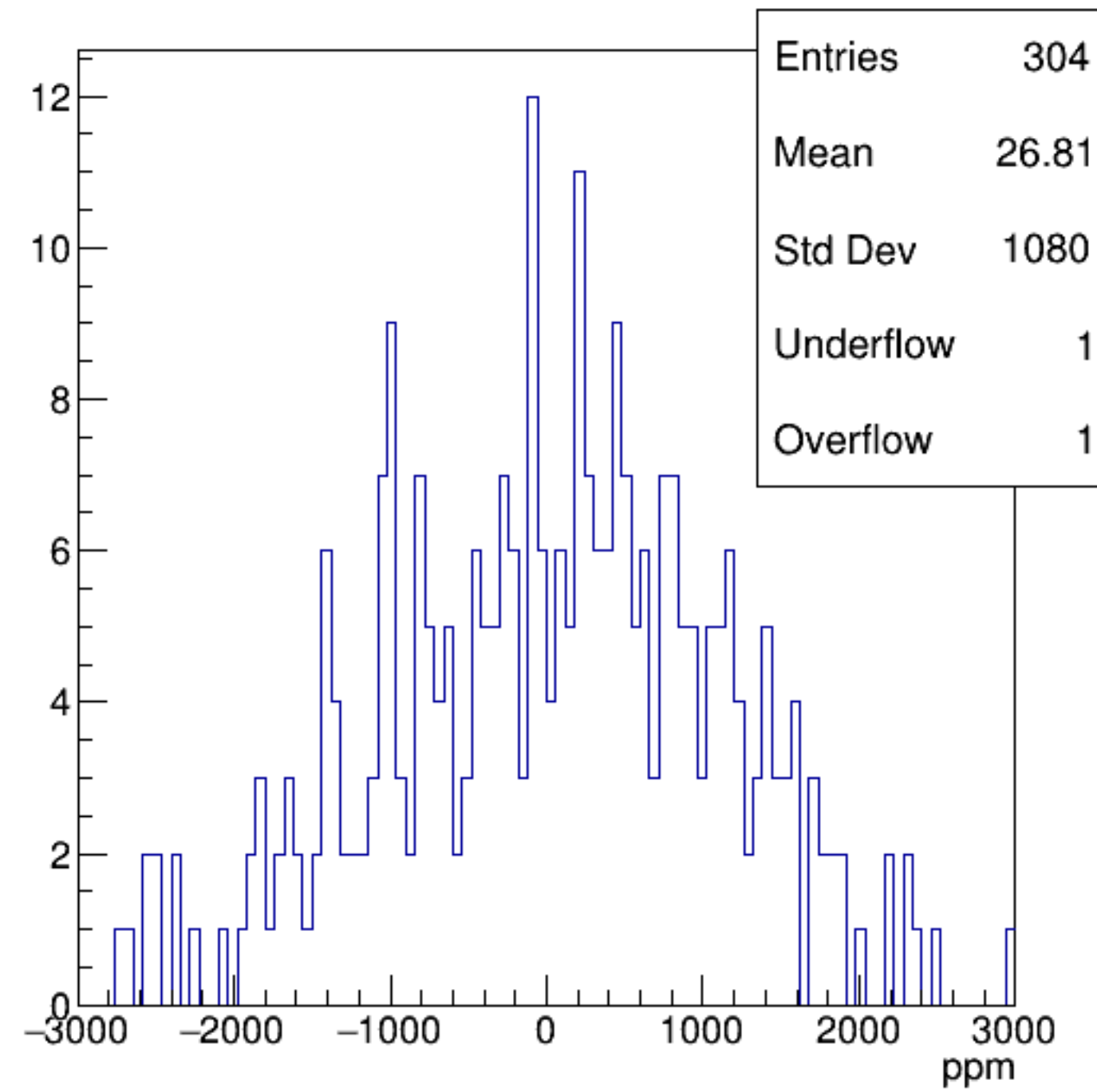
asym_sam5
