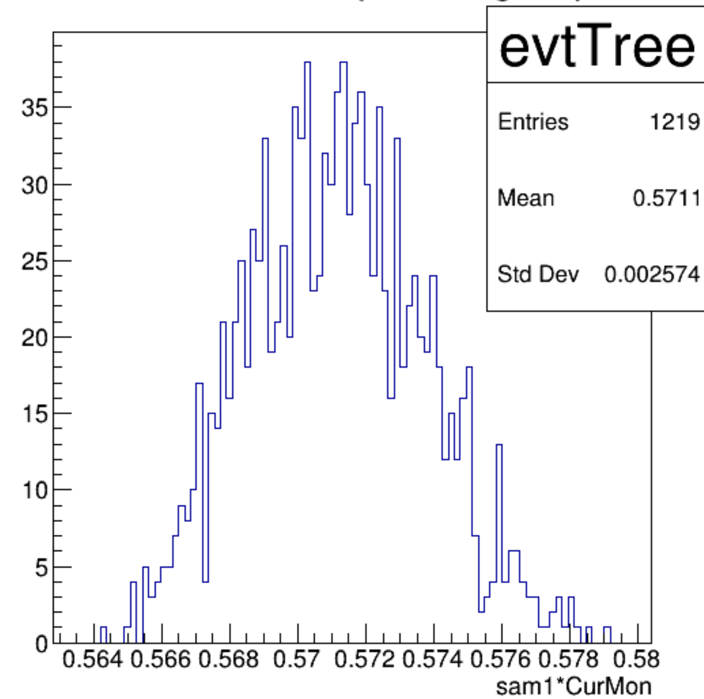
sam1*CurMon {ErrorFlag==0}
