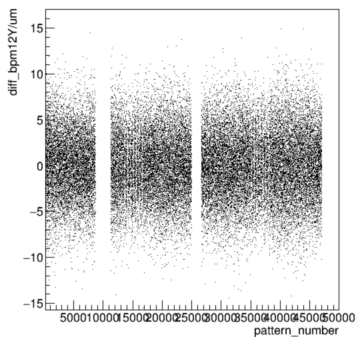
diff_bpm12Y/um:pattern_number {ErrorFlag==0}
