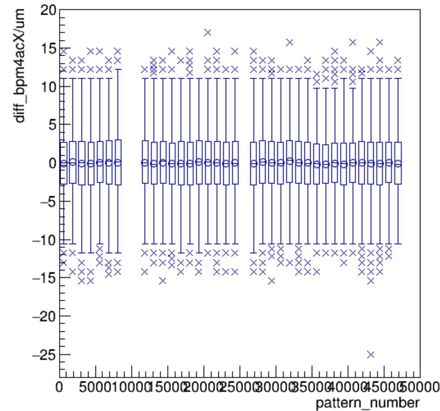
diff_bpm4acX/um:pattern_number {ErrorFlag==0}
