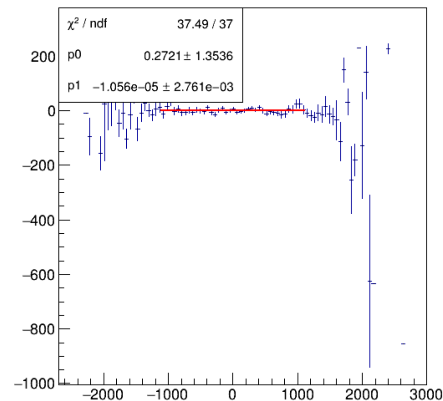
asym_bpm4eWS/ppm:Aq/ppm {ErrorFlag==0}
