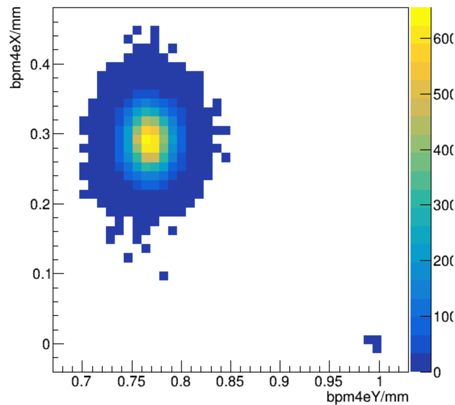
bpm4eX/mm:bpm4eY/mm {ErrorFlag==0}
