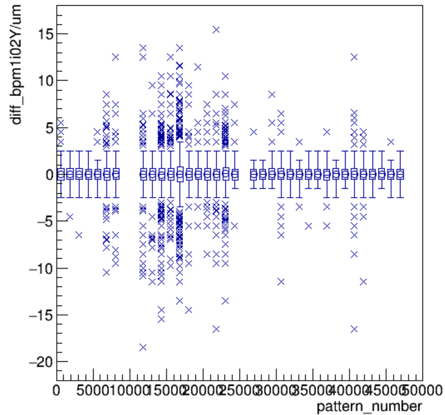
diff_bpm1i02Y/um:pattern_number {ErrorFlag==0}
