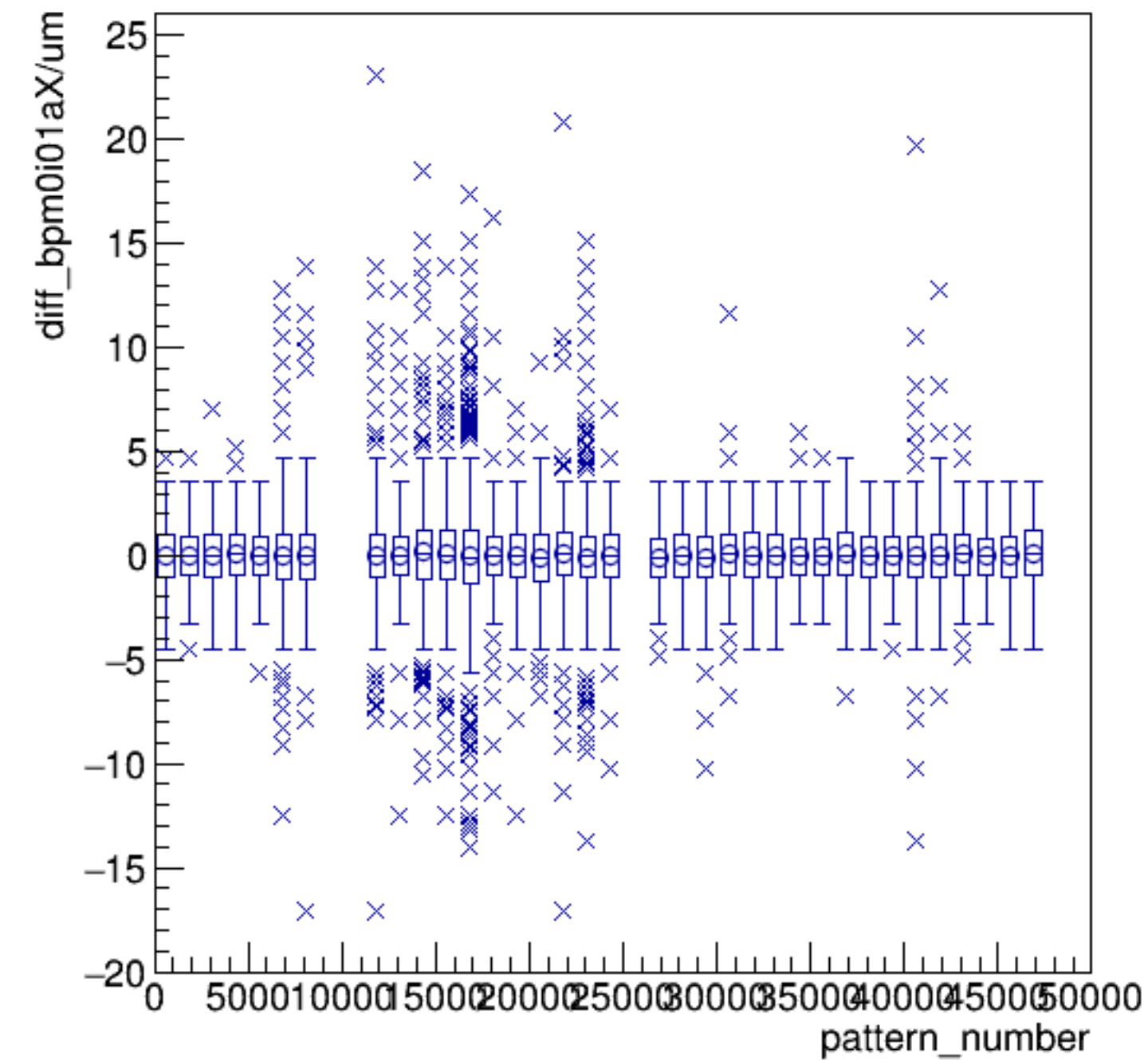
diff_bpm0i01aX/um:pattern_number {ErrorFlag==0}
