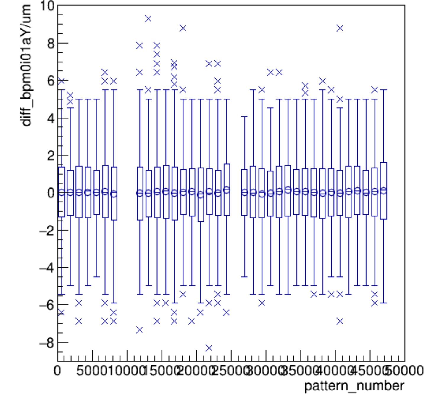
diff_bpm0i01aY/um:pattern_number {ErrorFlag==0}
