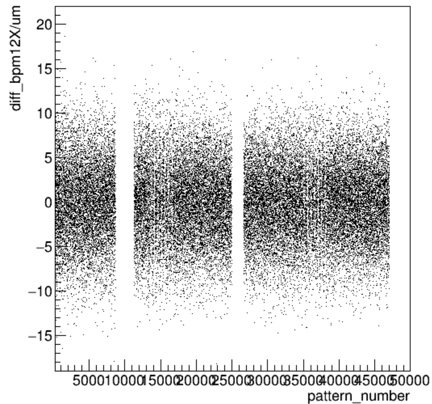
diff_bpm12X/um:pattern_number {ErrorFlag==0}
