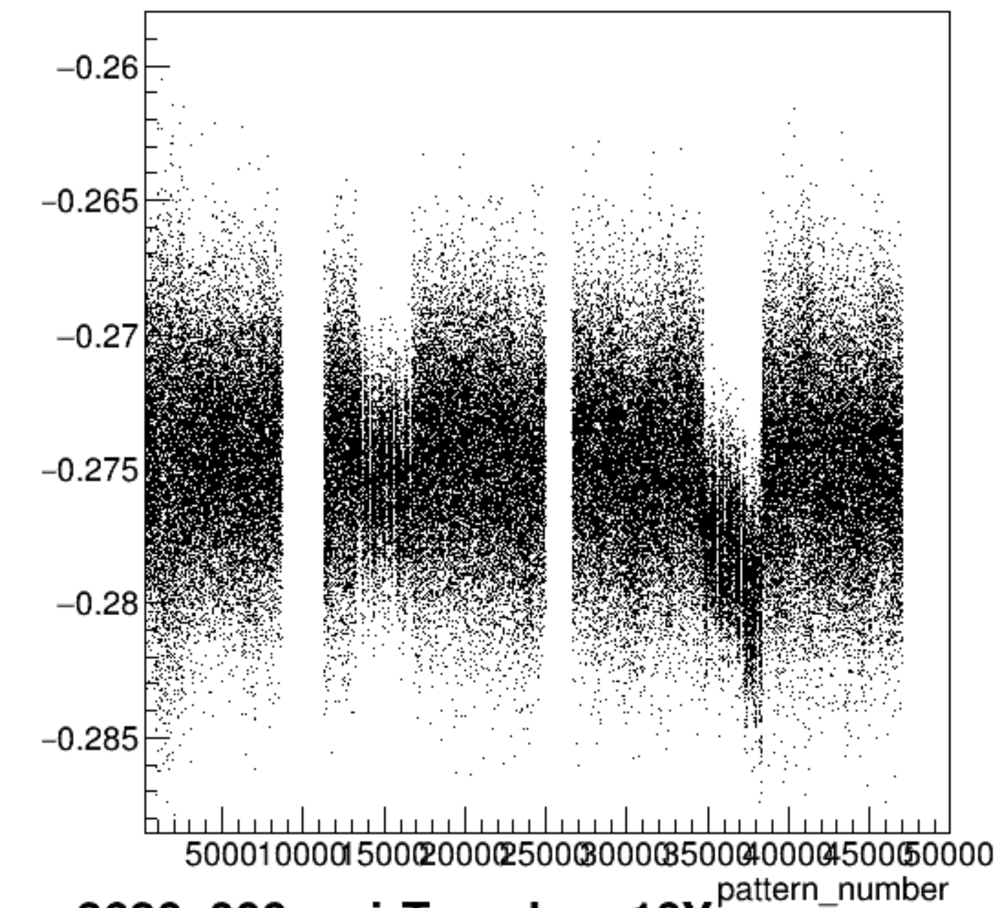
yield_bpm16Y/mm:pattern_number {ErrorFlag==0}
