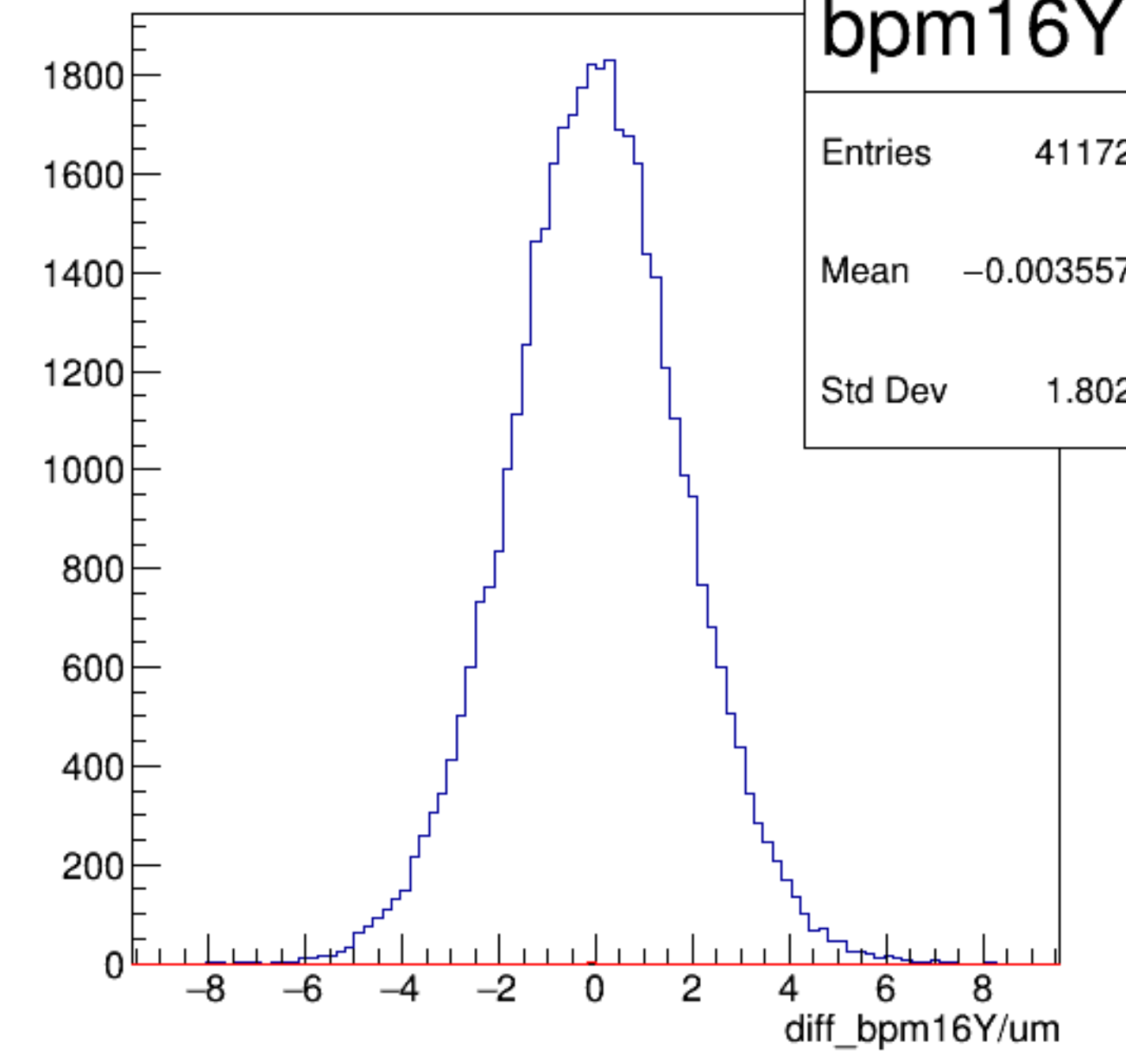
diff_bpm16Y/um {ErrorFlag==0}
