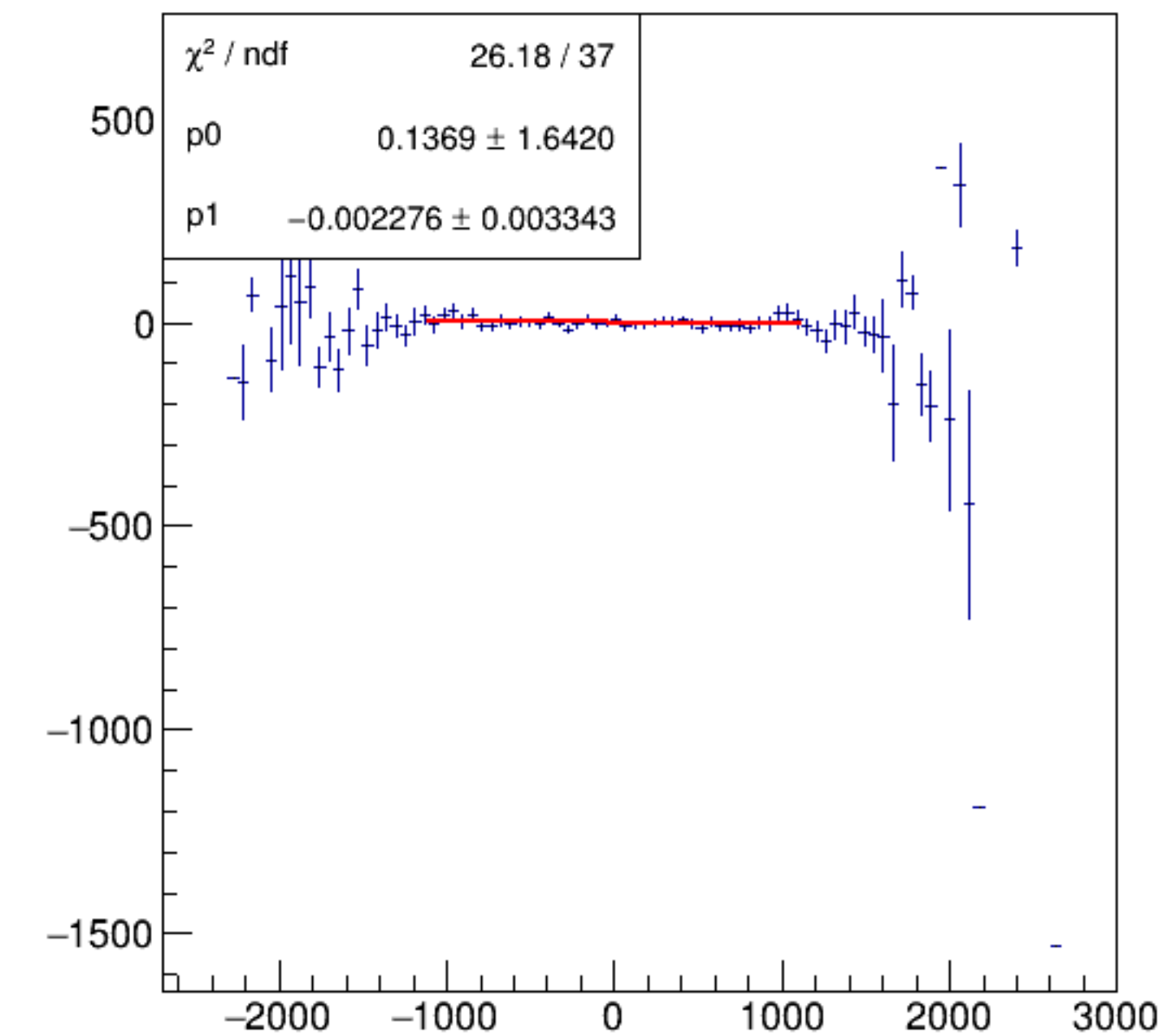
asym_bpm4aWS/ppm:Aq/ppm {ErrorFlag==0}
