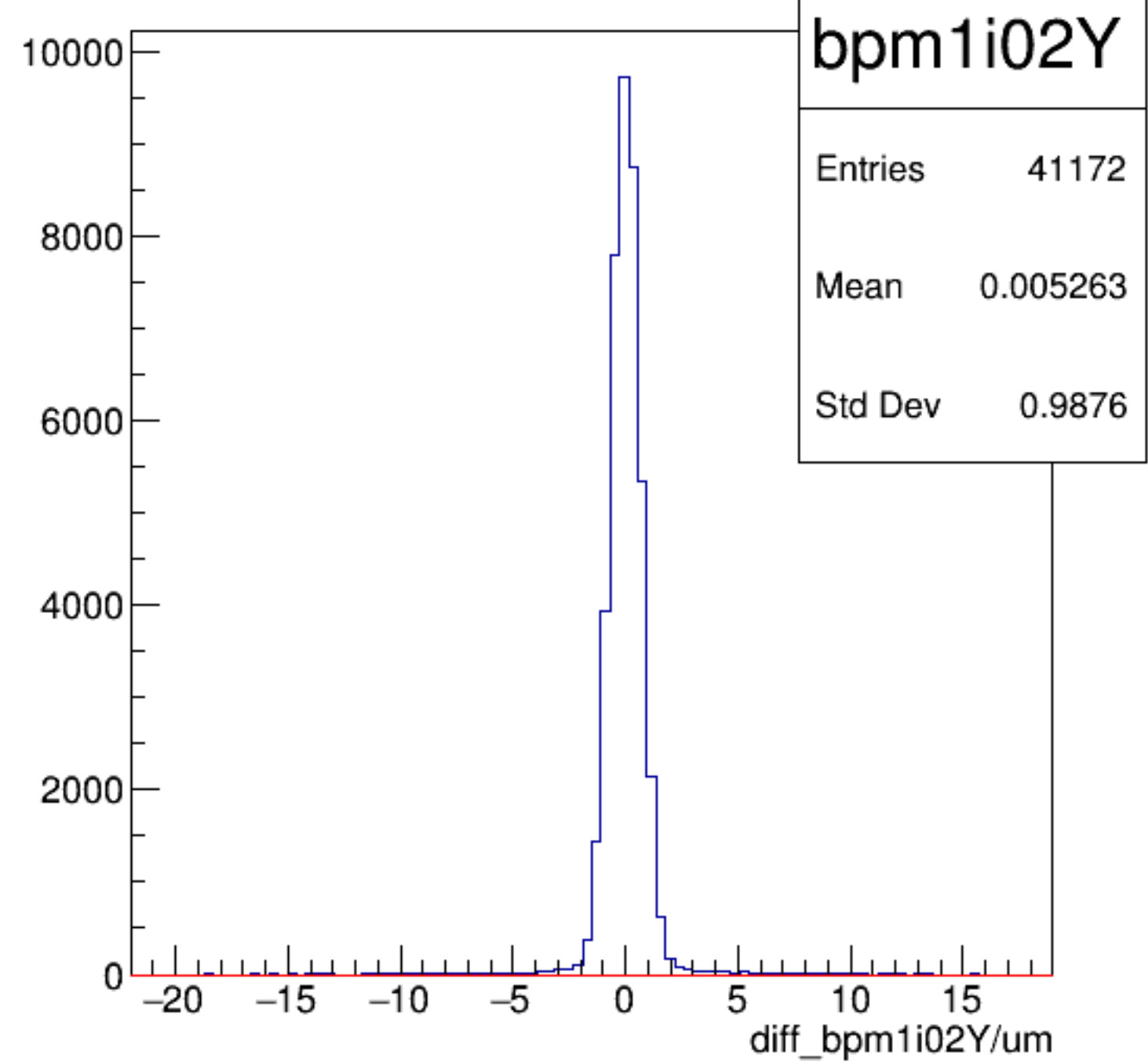
diff_bpm1i02Y/um {ErrorFlag==0}
