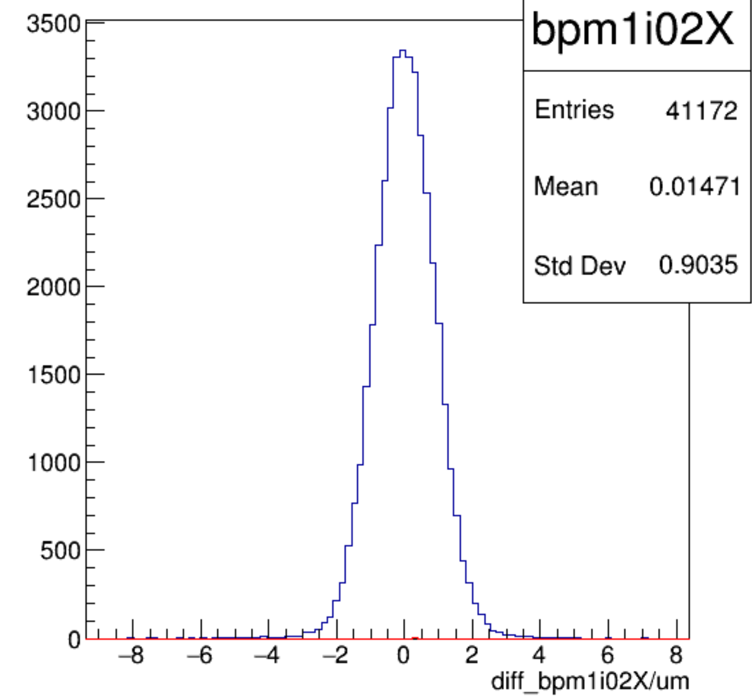
diff_bpm1i02X/um {ErrorFlag==0}
