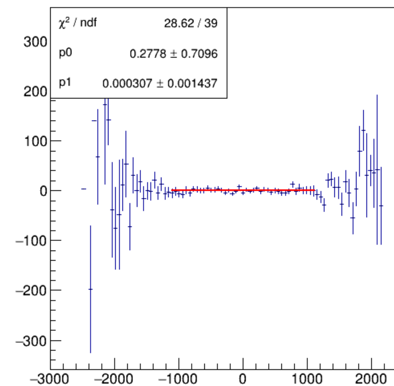
asym_bpm11WS/ppm:Aq/ppm {ErrorFlag==0}
