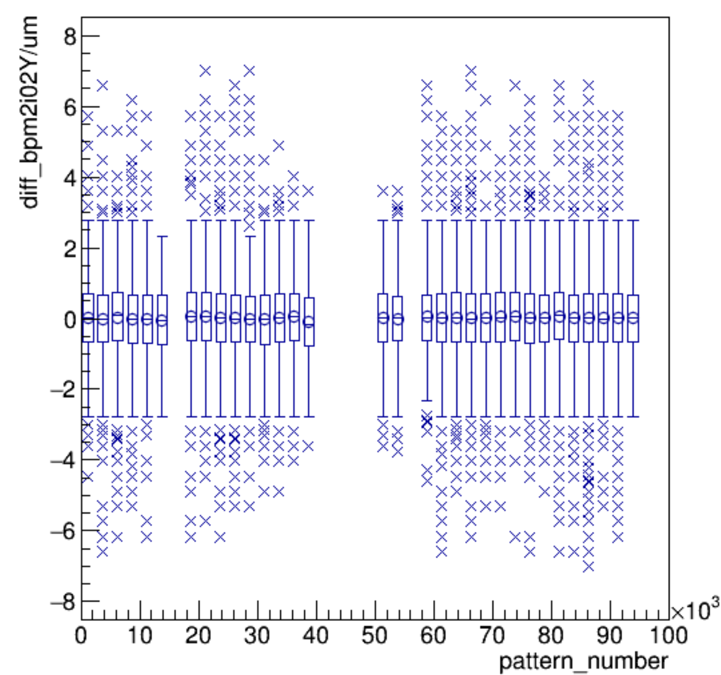
diff_bpm2i02Y/um:pattern_number {ErrorFlag==0}
