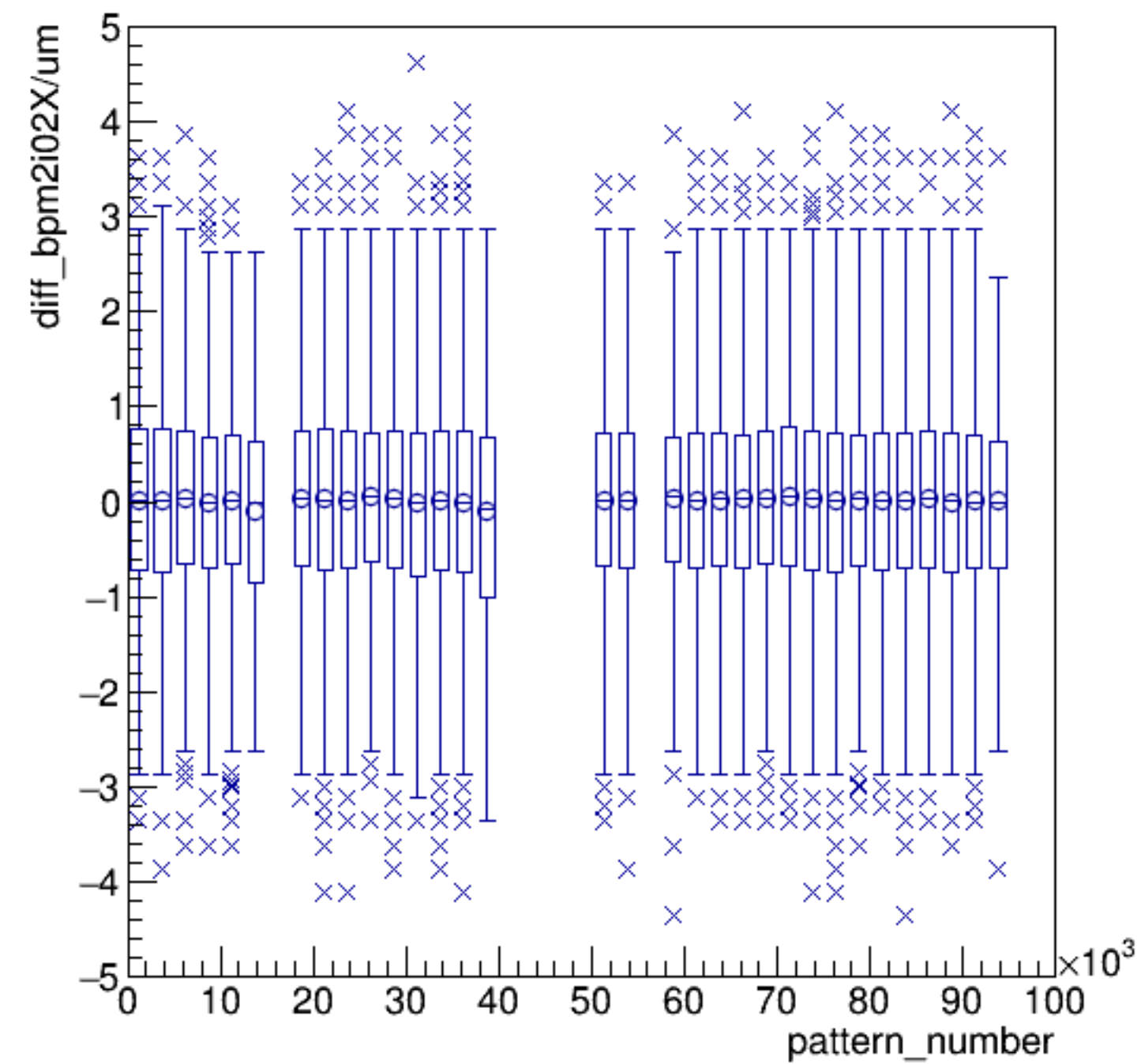
diff_bpm2i02X/um:pattern_number {ErrorFlag==0}
