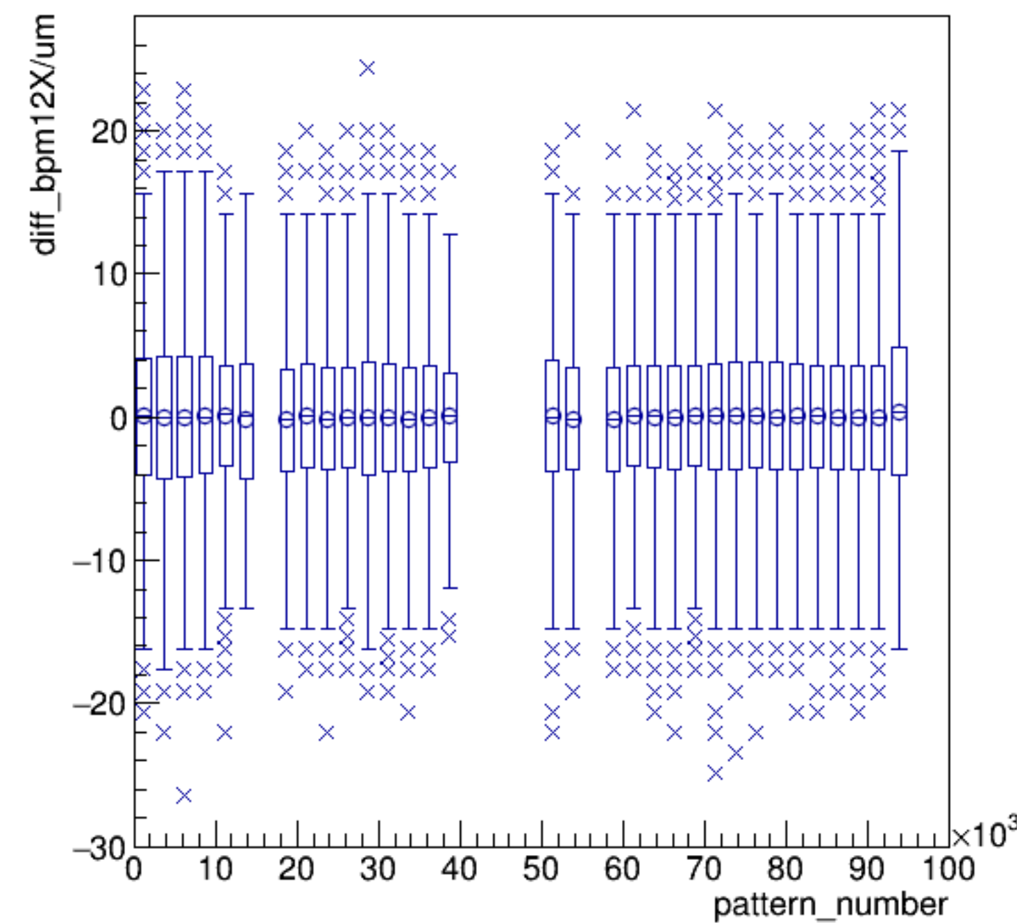
diff_bpm12X/um:pattern_number {ErrorFlag==0}
