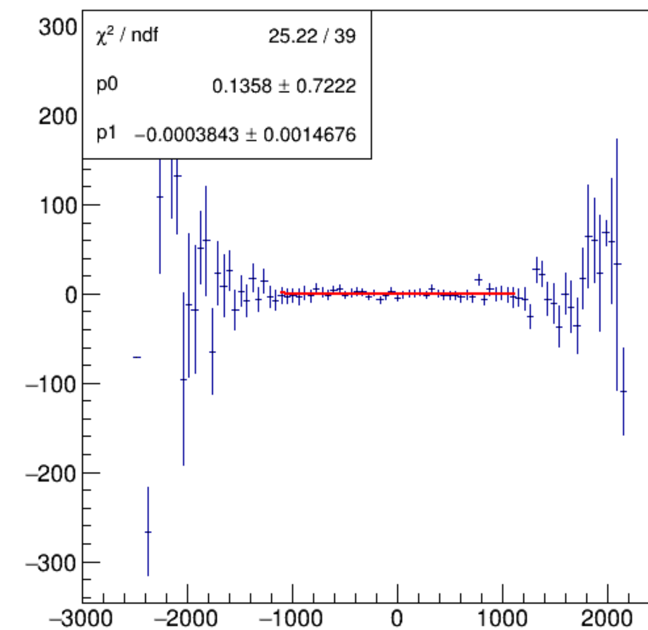
asym_bpm16WS/ppm:Aq/ppm {ErrorFlag==0}
