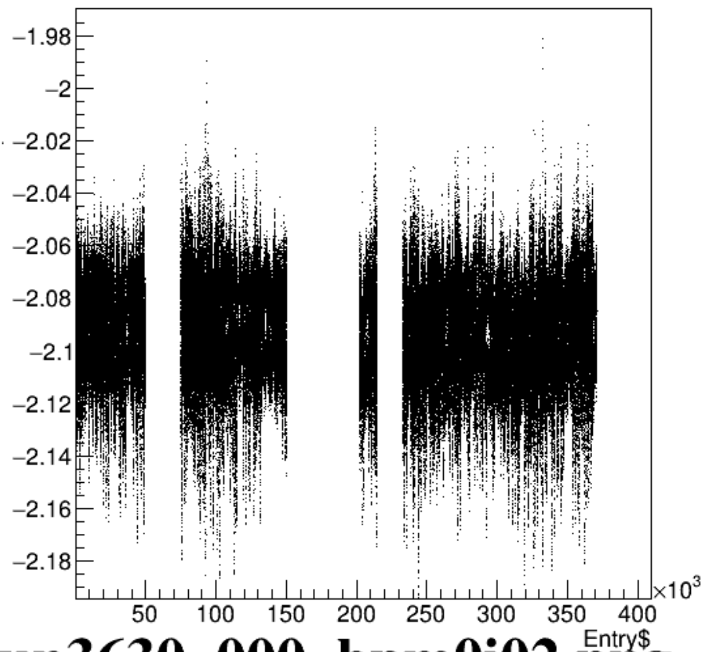
bpm0i02Y/mm:Entry$ {ErrorFlag==0}
