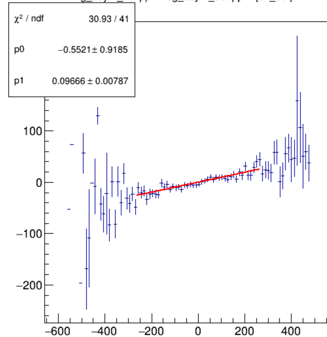
reg_asym_dsl/ppm:reg_asym_dsr/ppm {ok_cut}
