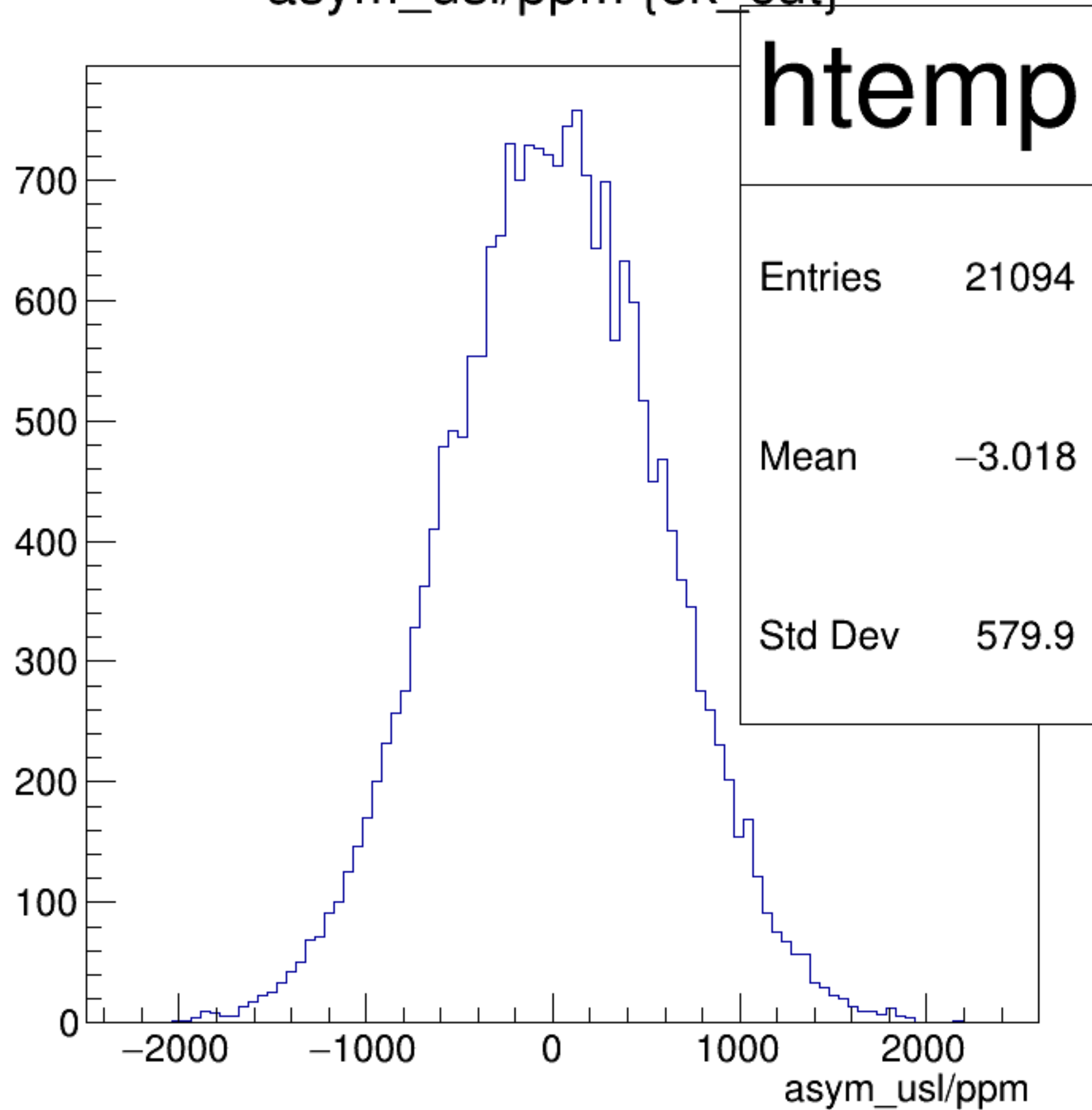
asym_usl/ppm {ok_cut}
