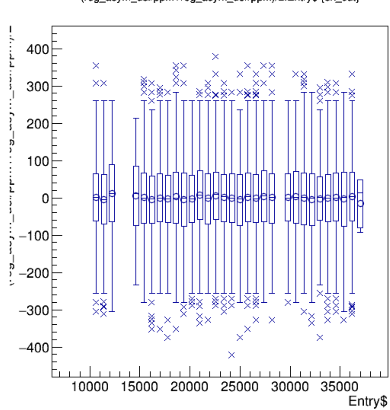
(reg_asym_usl/ppm+reg_asym_usr/ppm)/2:Entry$ {ok_cut}
