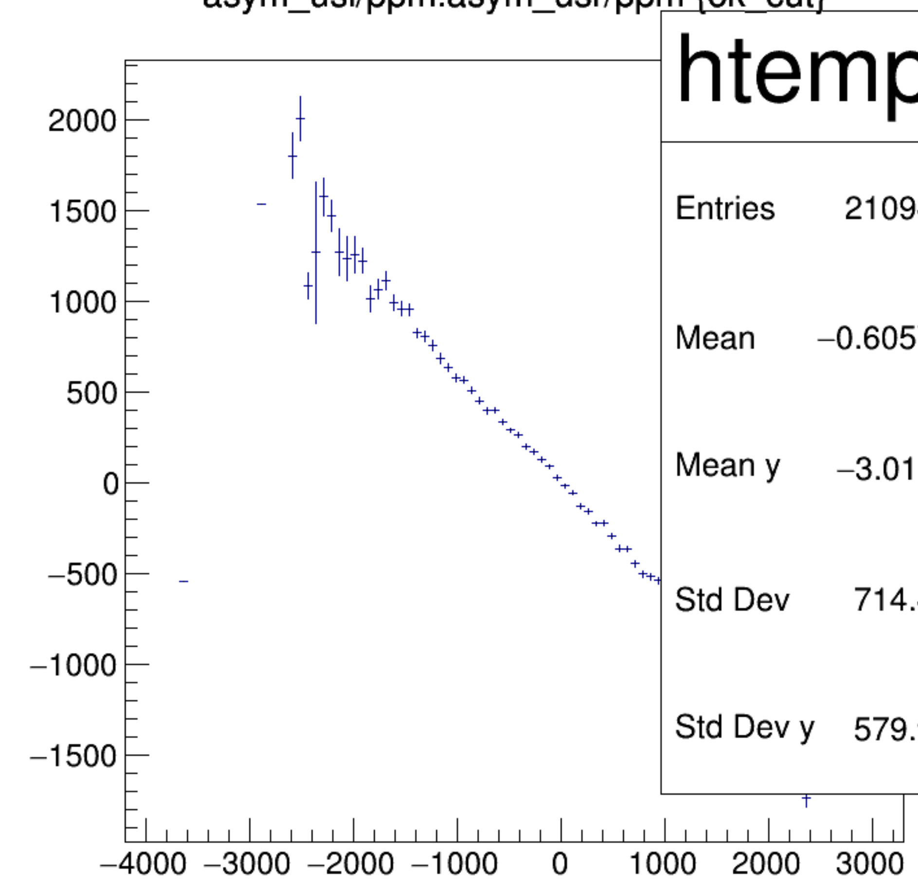
asym_usl/ppm:asym_usr/ppm {ok_cut}
