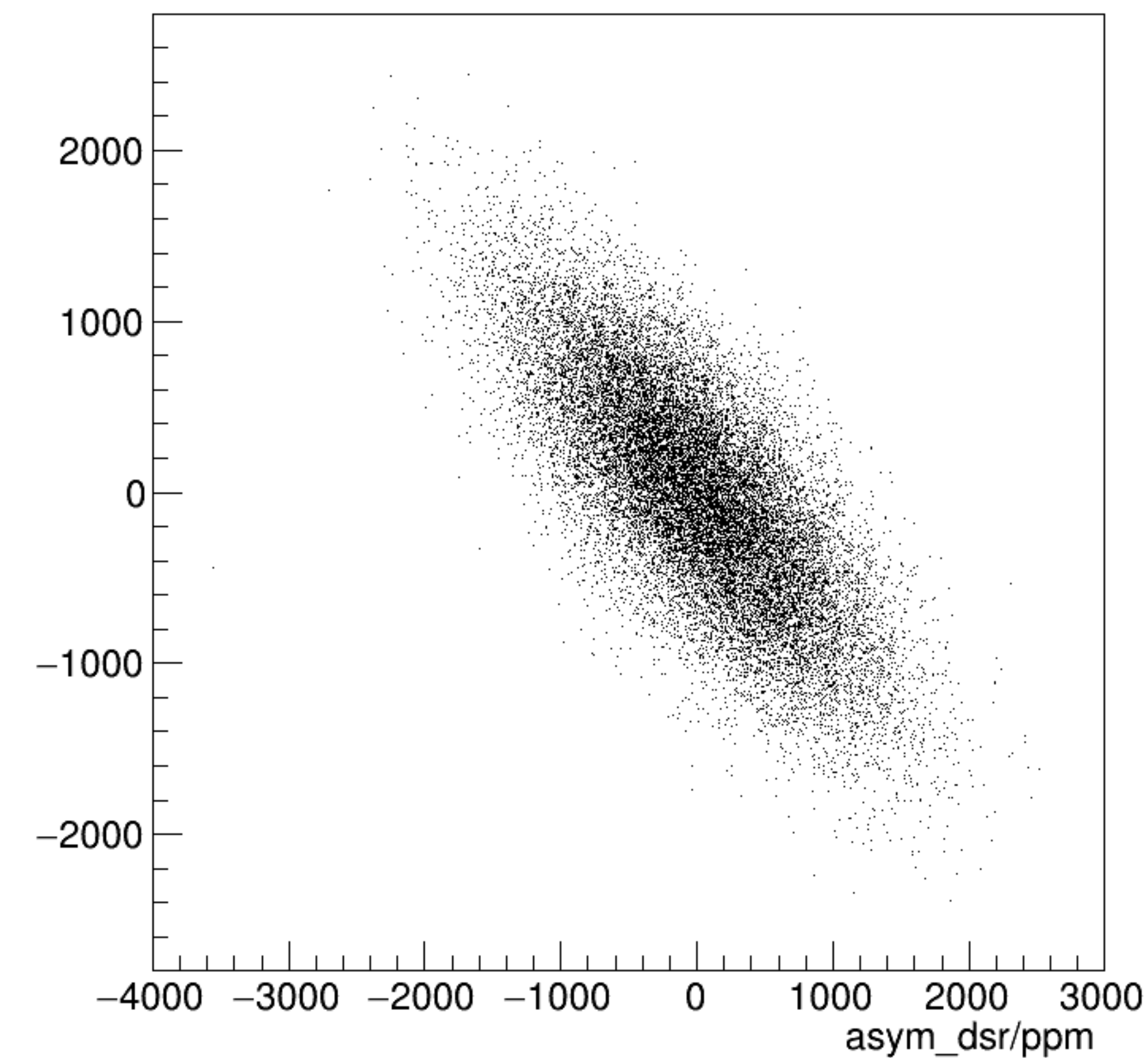
asym_dsl/ppm:asym_dsr/ppm {ok_cut}
