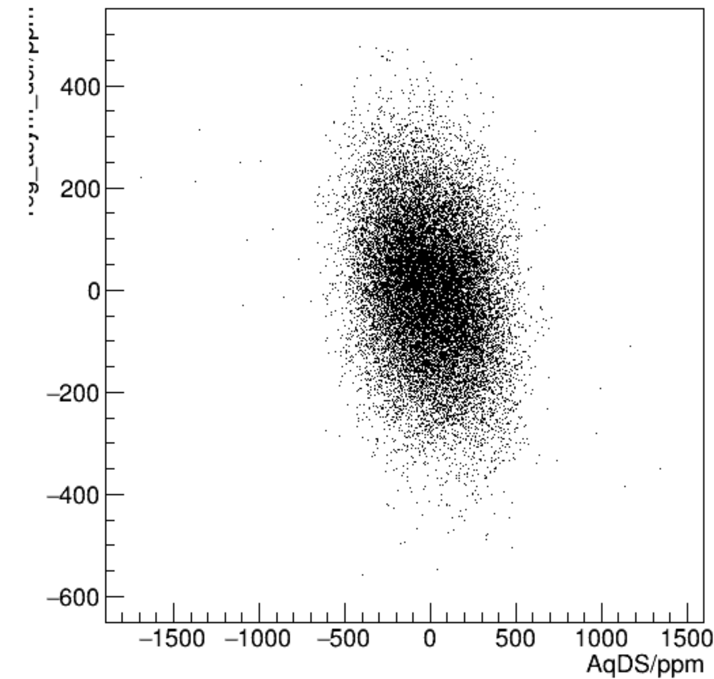
reg_asym_dsr/ppm:AqDS/ppm {ok_cut}
