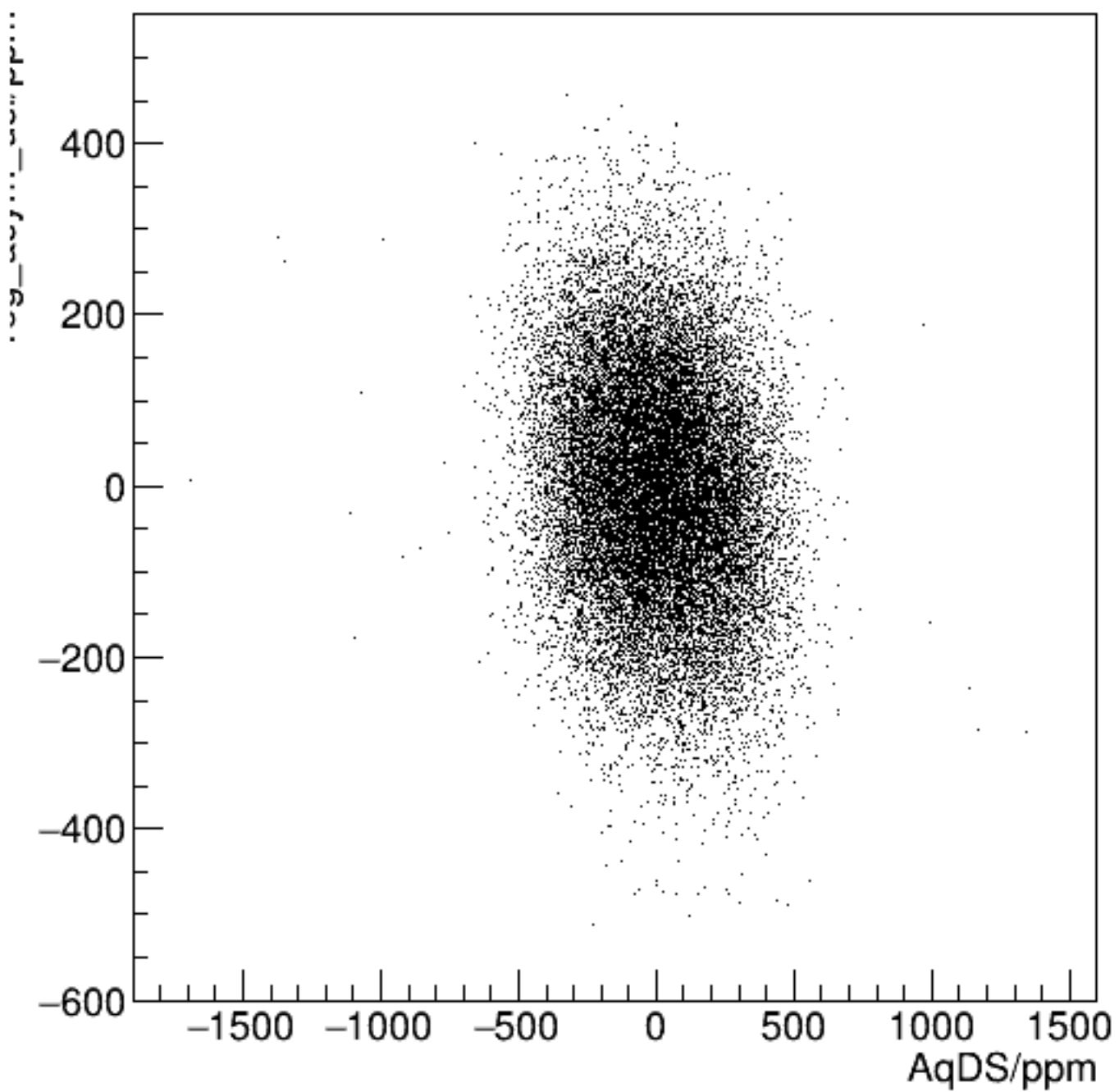
reg_asym_usl/ppm:AqDS/ppm {ok_cut}
