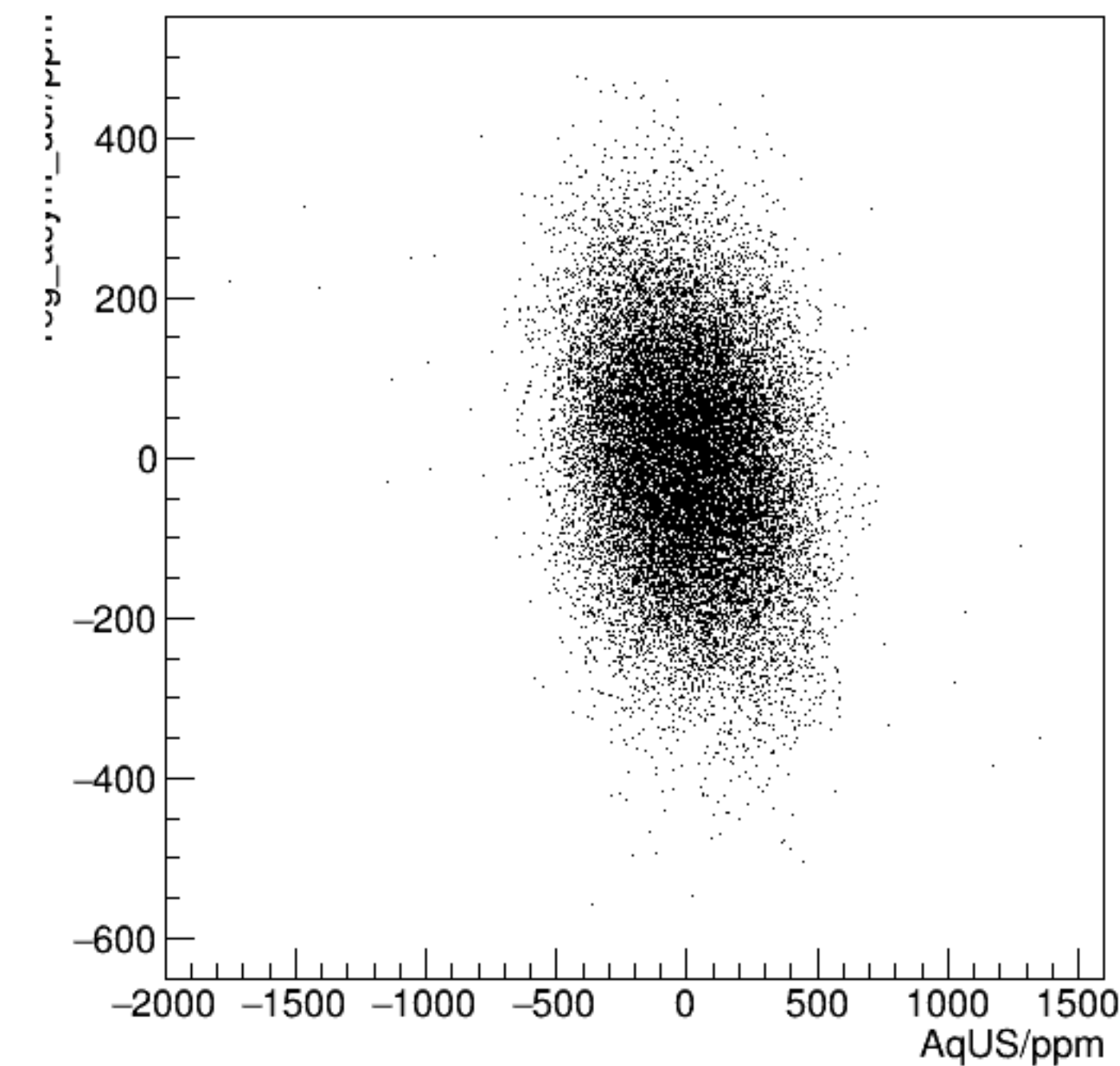
reg_asym_dsr/ppm:AqUS/ppm {ok_cut}
