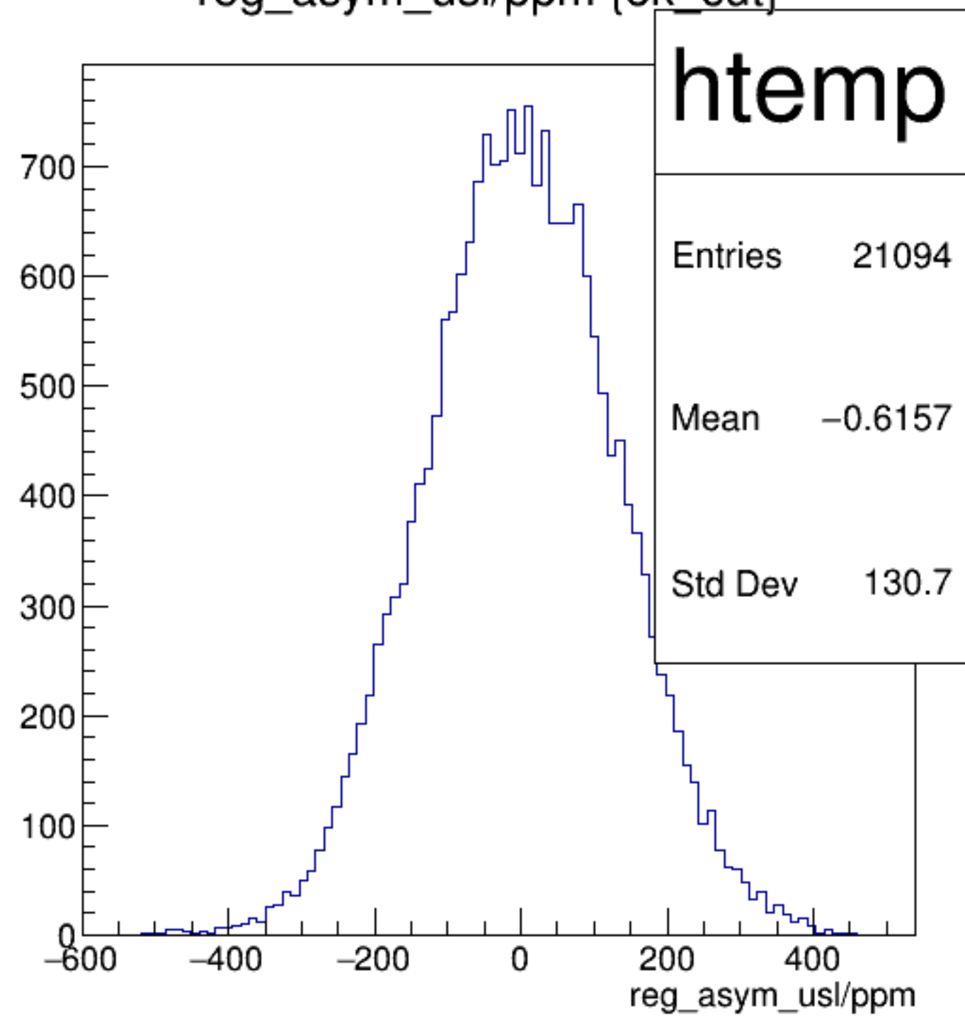
reg_asym_usl/ppm {ok_cut}
