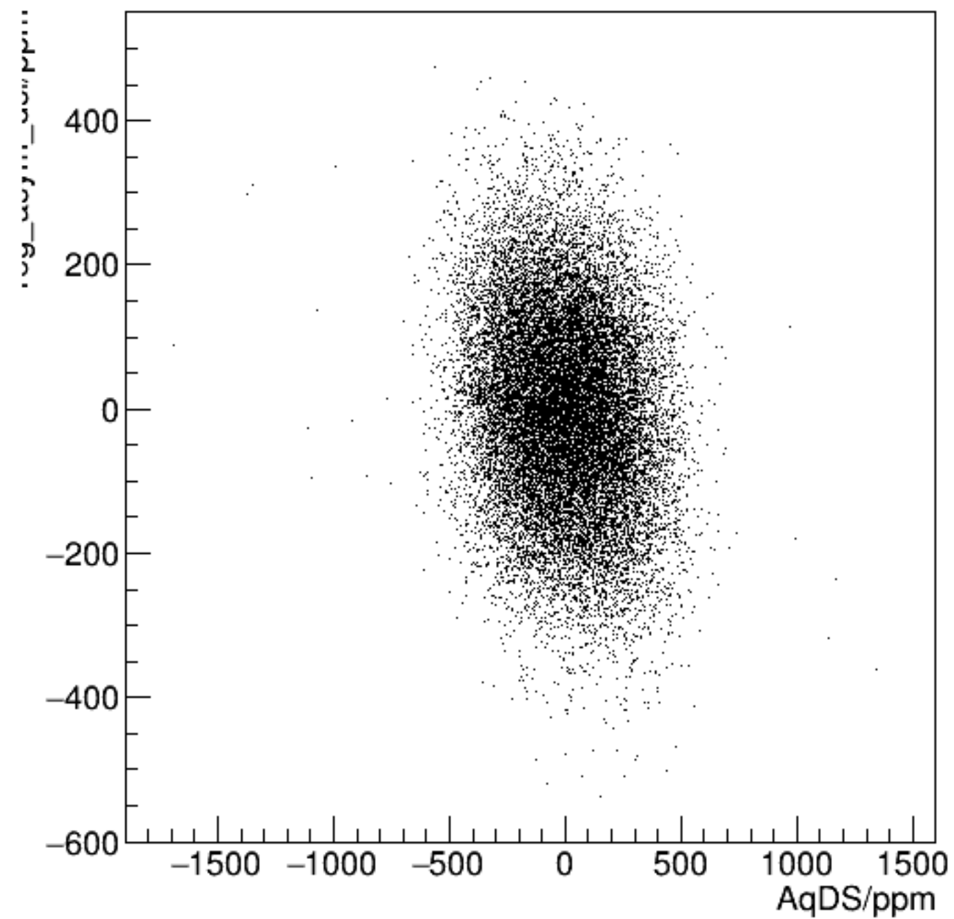
reg_asym_dsl/ppm:AqDS/ppm {ok_cut}
