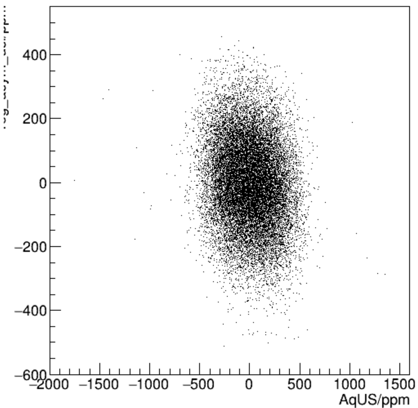
reg_asym_usl/ppm:AqUS/ppm {ok_cut}
