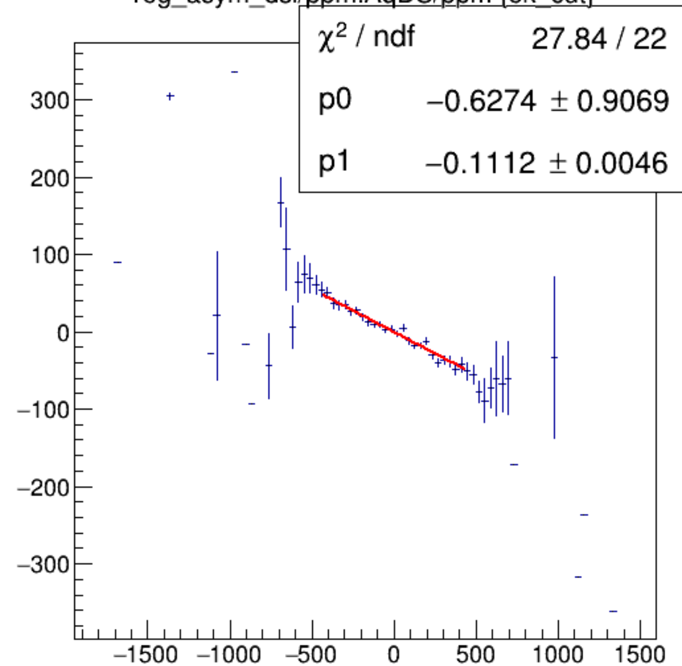
reg_asym_dsl/ppm:AqDS/ppm {ok_cut}
