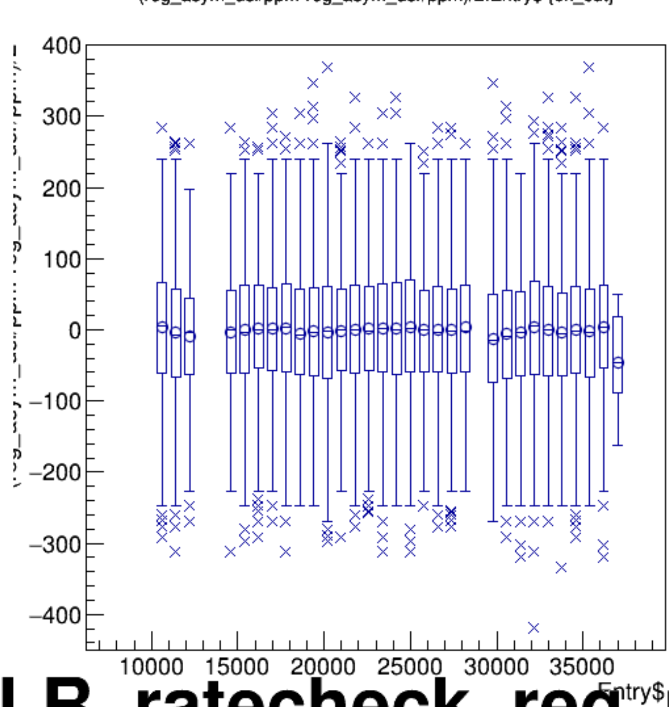
(reg_asym_usl/ppm-reg_asym_usr/ppm)/2:Entry$ {ok_cut}
