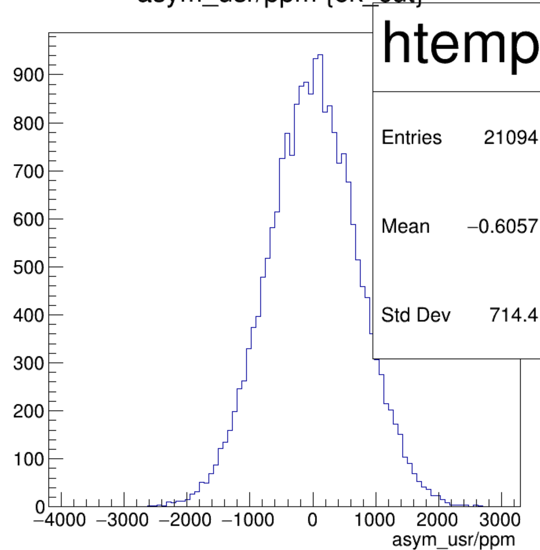
asym_usr/ppm {ok_cut}
