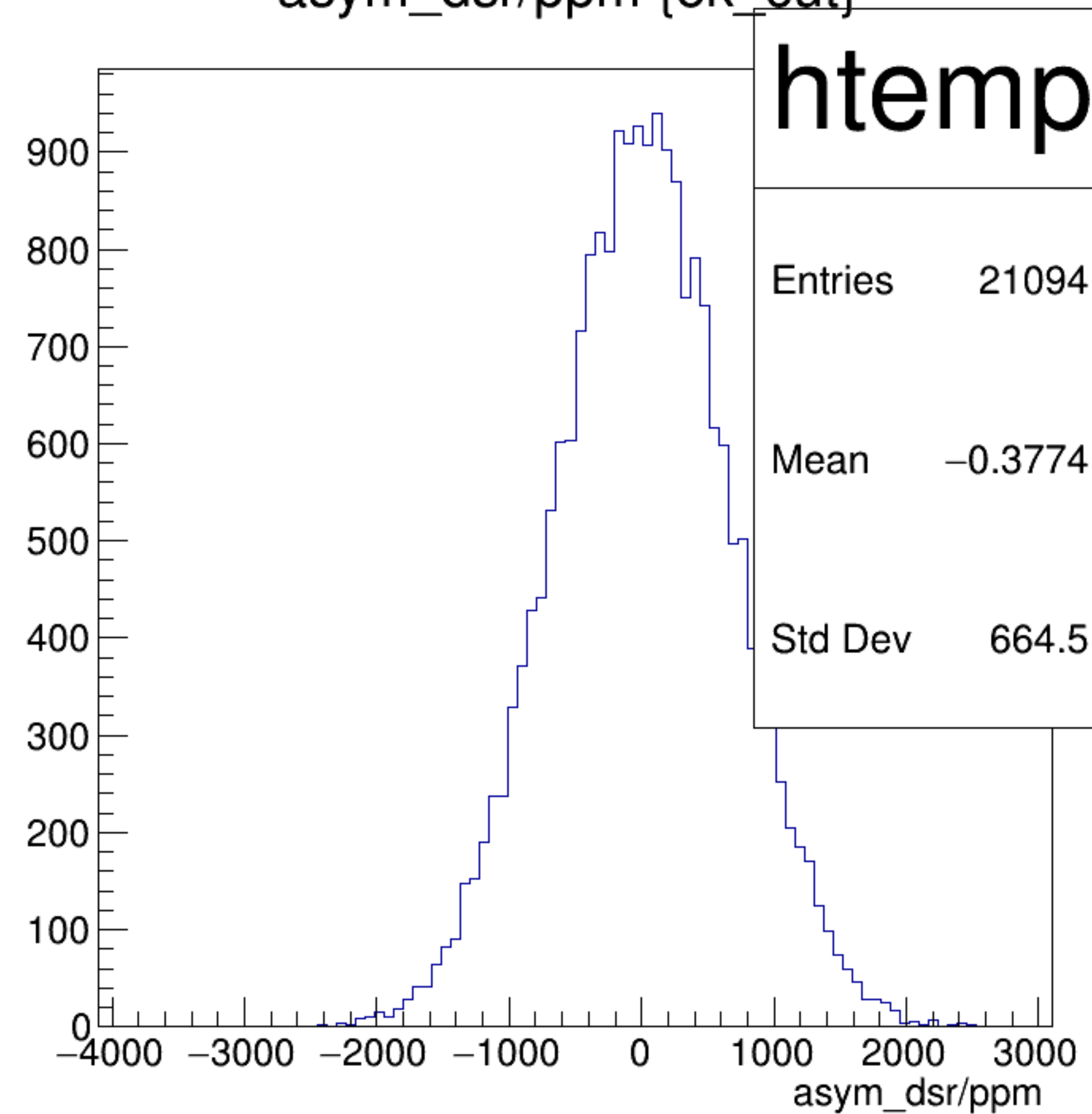
asym_dsr/ppm {ok_cut}
