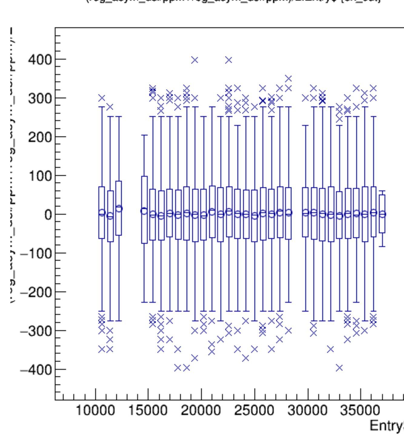
(reg_asym_dsl/ppm+reg_asym_dsr/ppm)/2:Entry$ {ok_cut}
