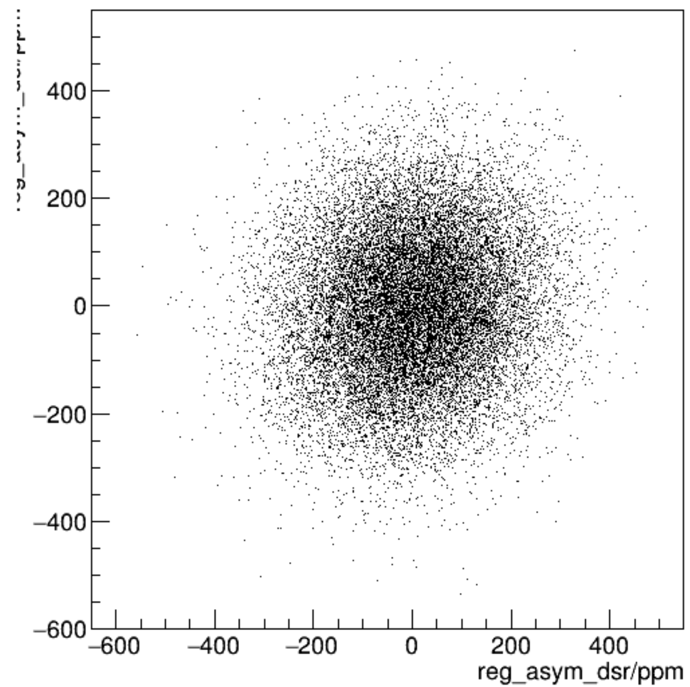
reg_asym_dsl/ppm:reg_asym_dsr/ppm {ok_cut}
