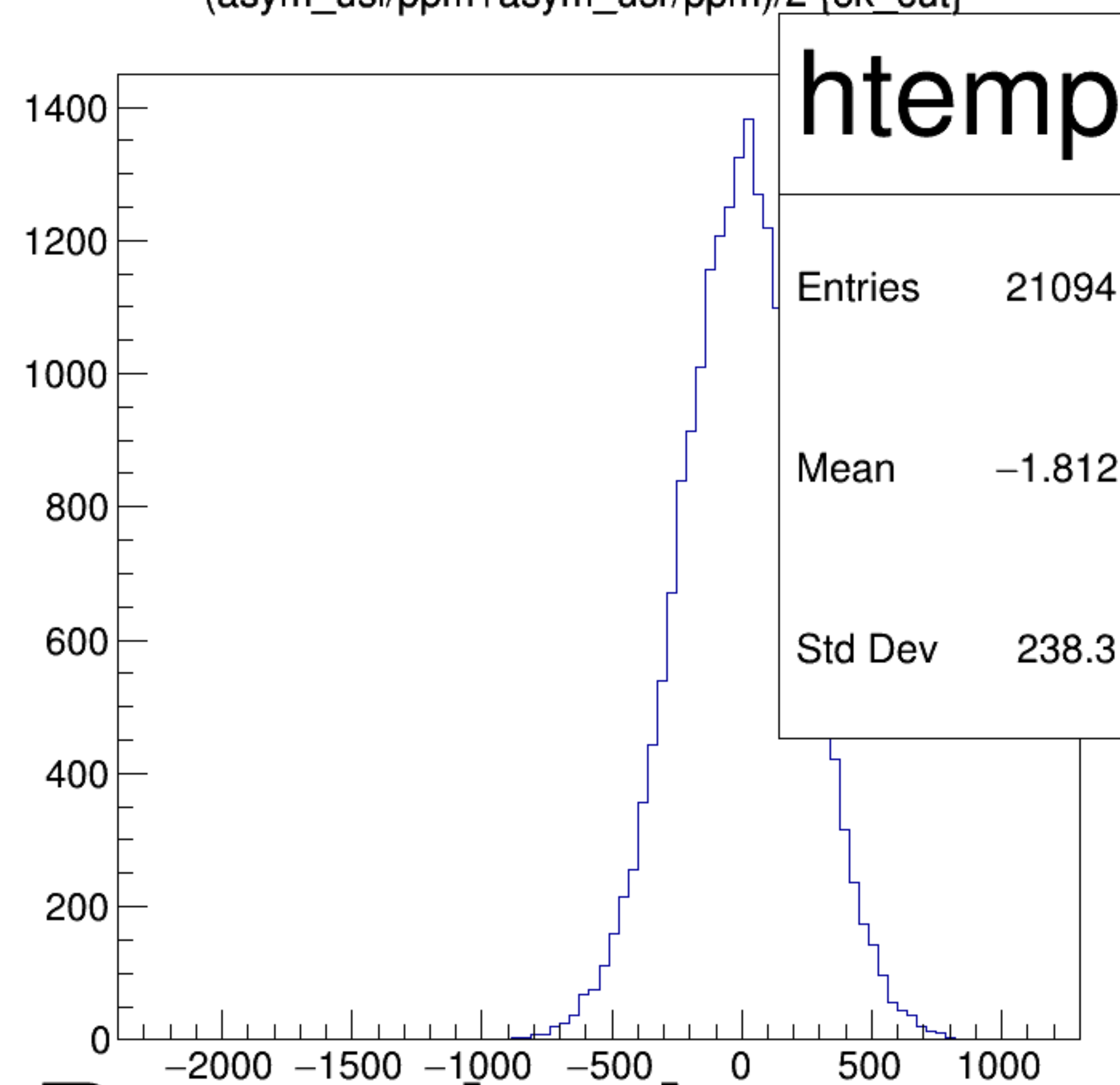
(asym_usl/ppm+asym_usr/ppm)/2 {ok_cut}
