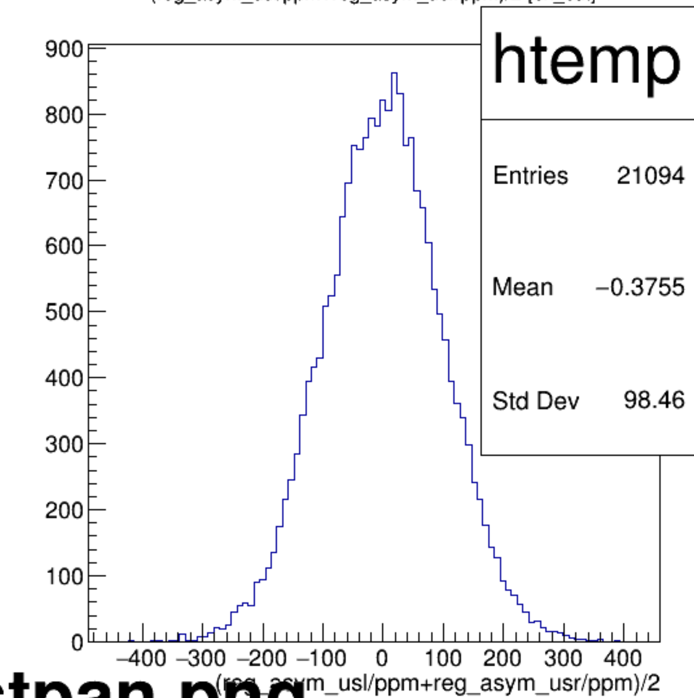
(reg_asym_usl/ppm+reg_asym_usr/ppm)/2 {ok_cut}
