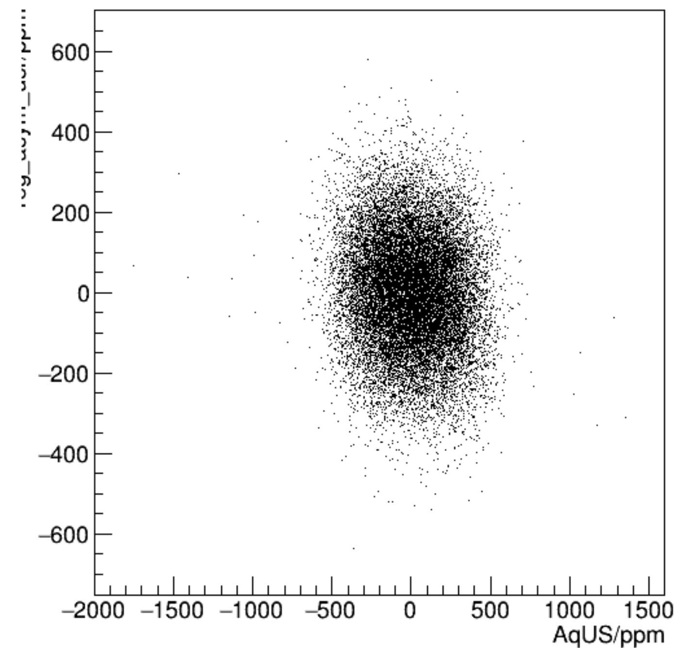
reg_asym_usr/ppm:AqUS/ppm {ok_cut}
