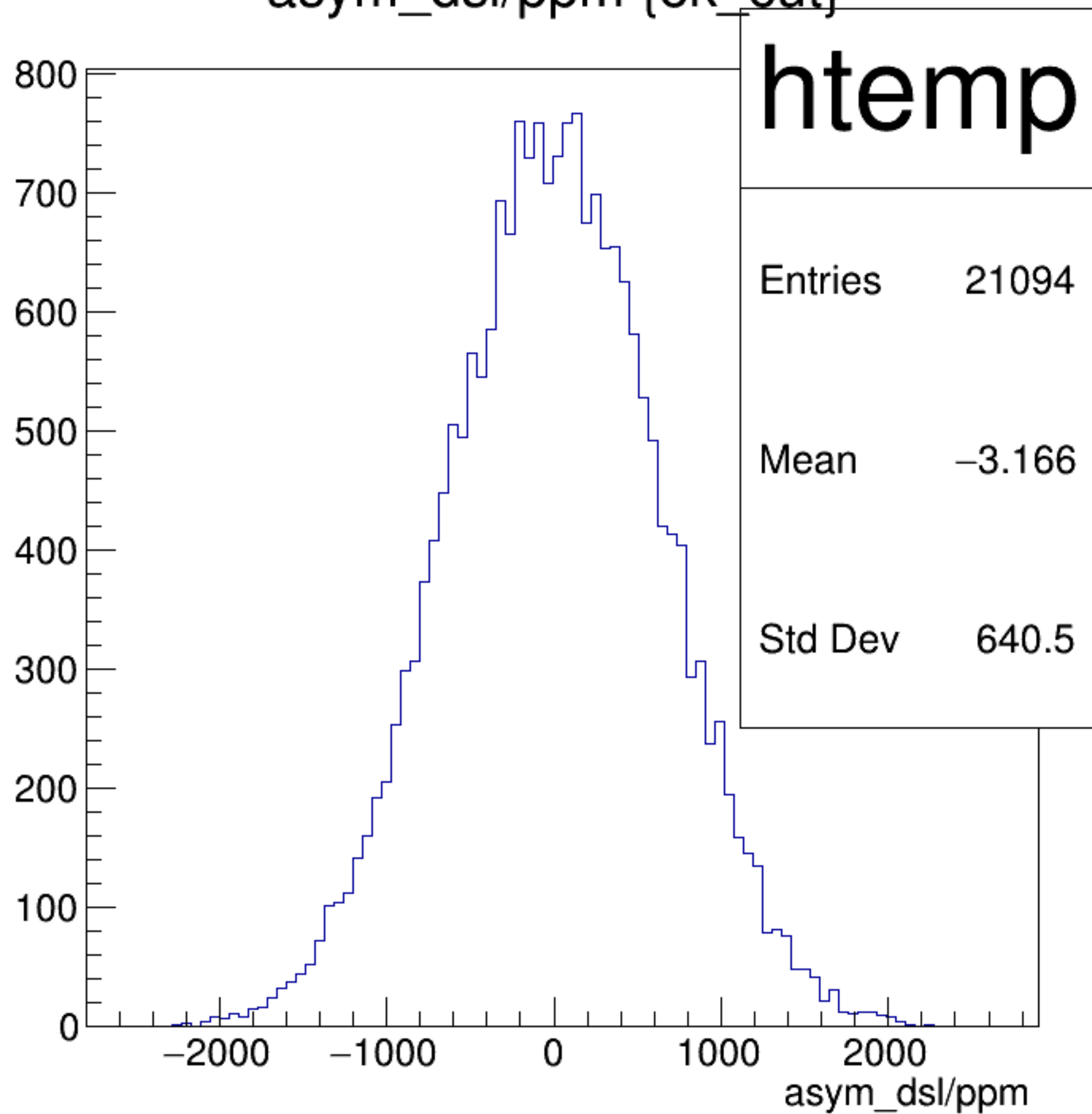
asym_dsl/ppm {ok_cut}
