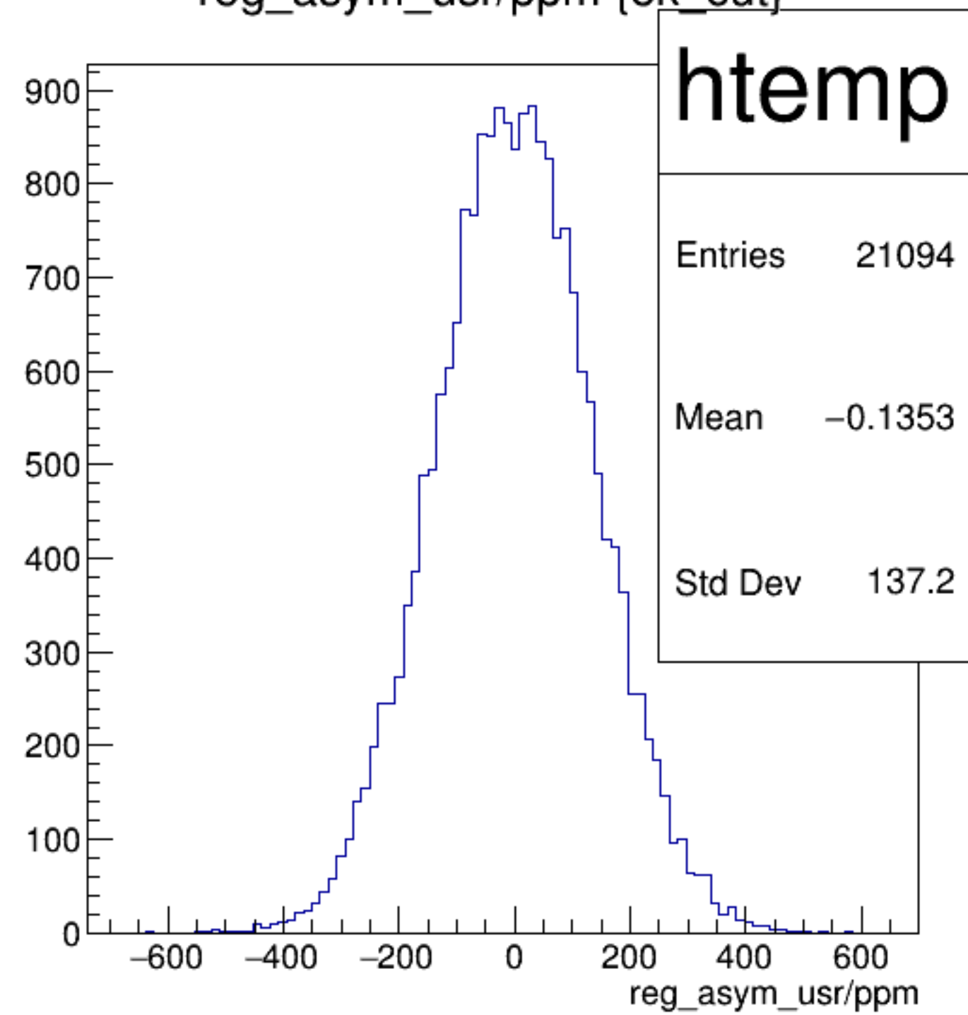
reg_asym_usr/ppm {ok_cut}
