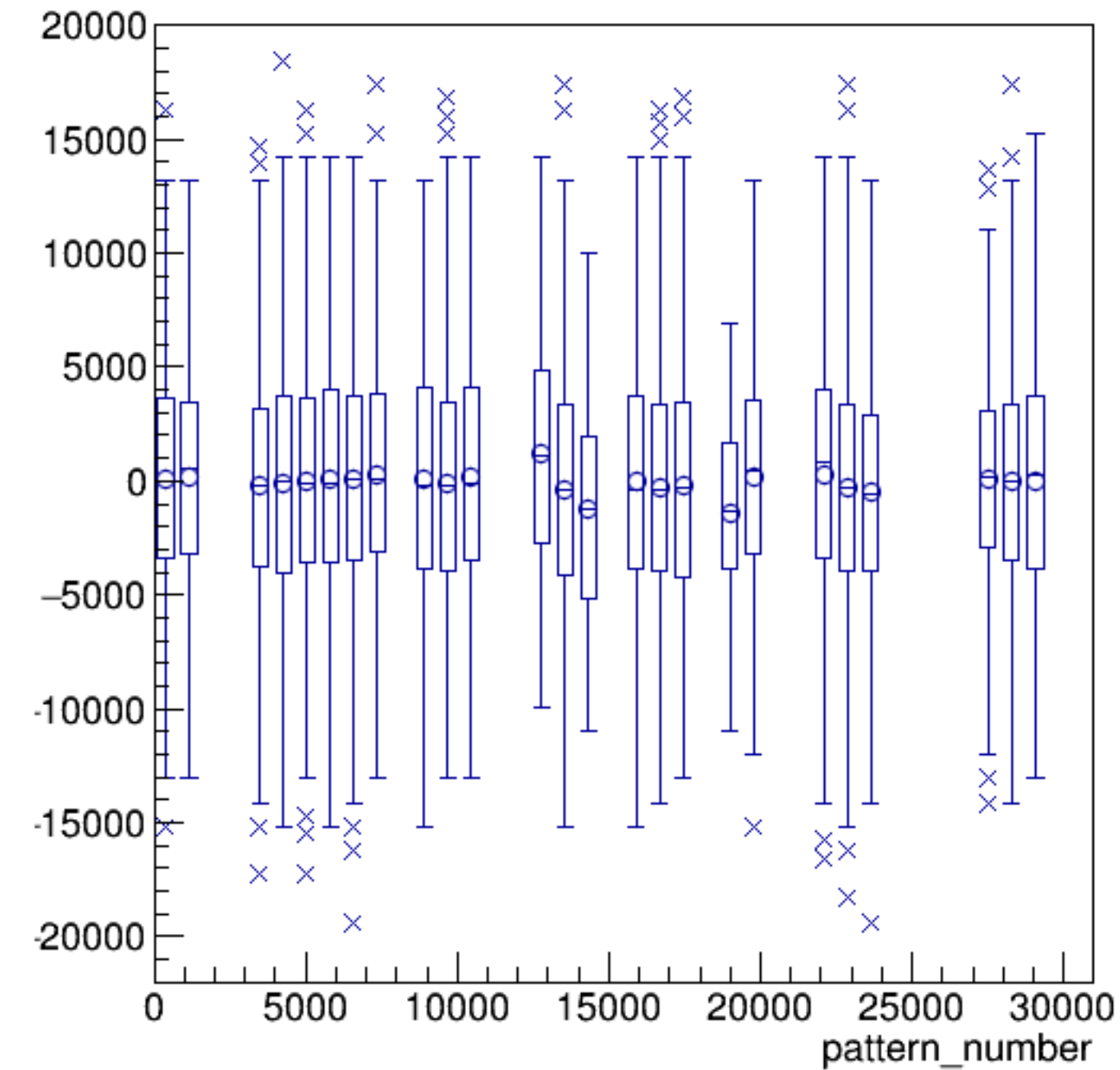
asym_sam7/ppm:pattern_number {ErrorFlag==0}
