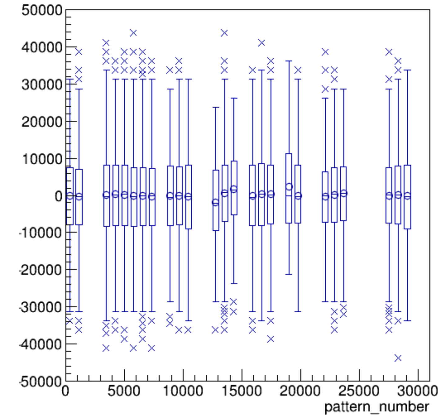
asym_sam2/ppm:pattern_number {ErrorFlag==0}
