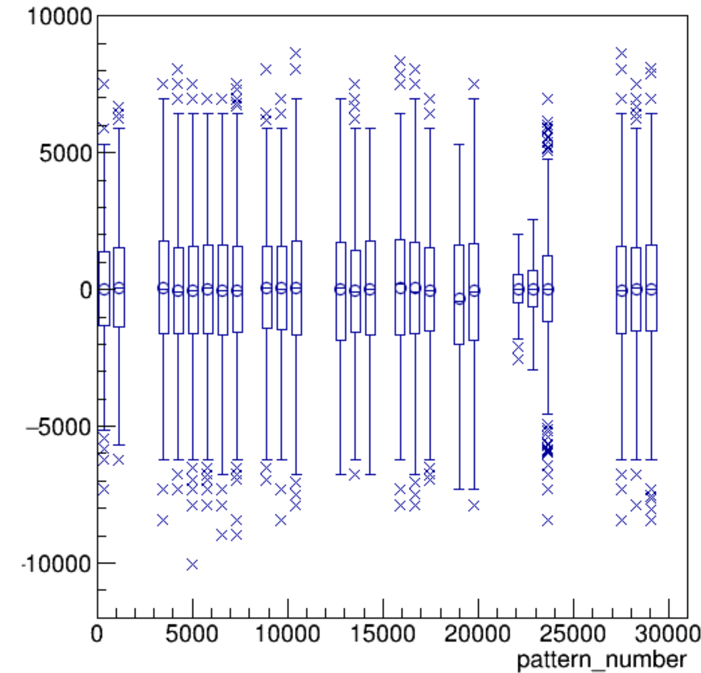
asym_sam5/ppm:pattern_number {ErrorFlag==0}
