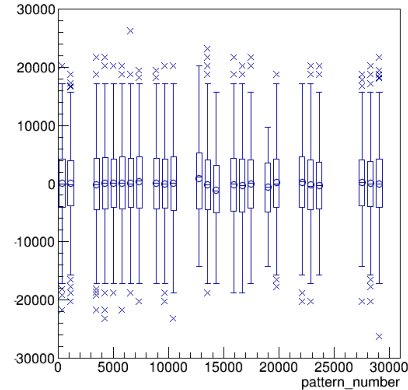
asym_sam8/ppm:pattern_number {ErrorFlag==0}
