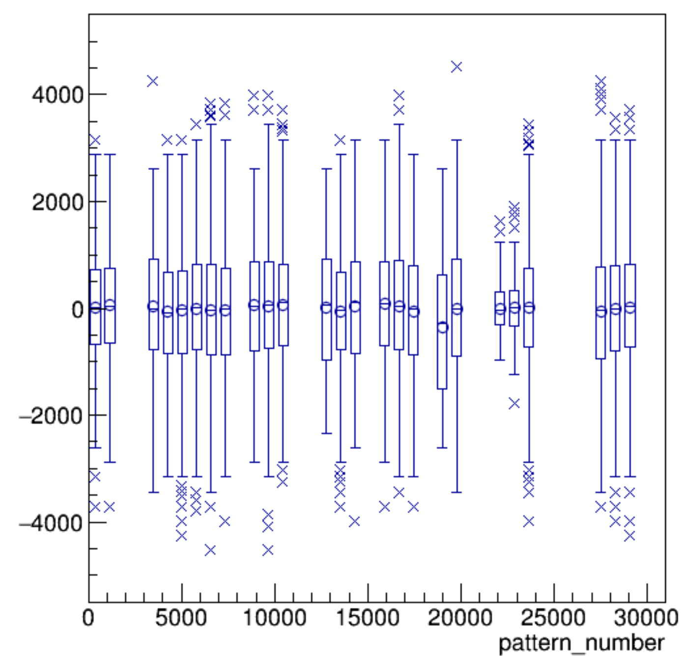
asym_sam5/ppm:pattern_number {ErrorFlag==0}
