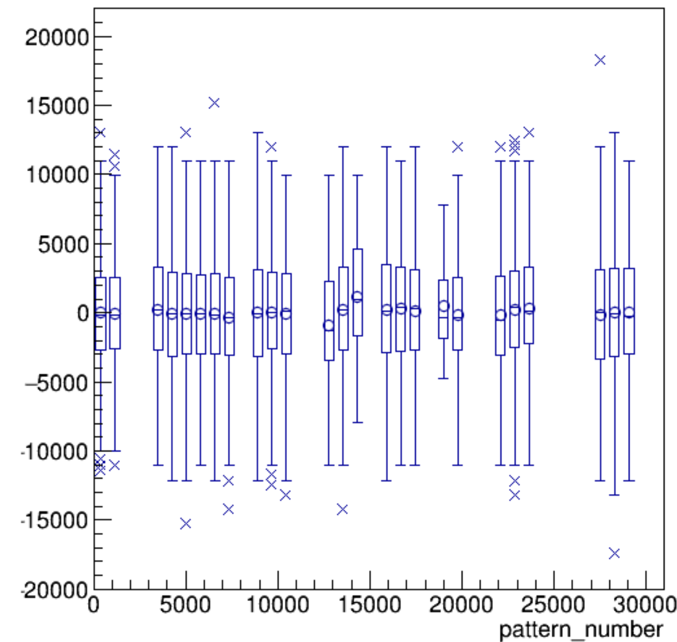
asym_sam4/ppm:pattern_number {ErrorFlag==0}
