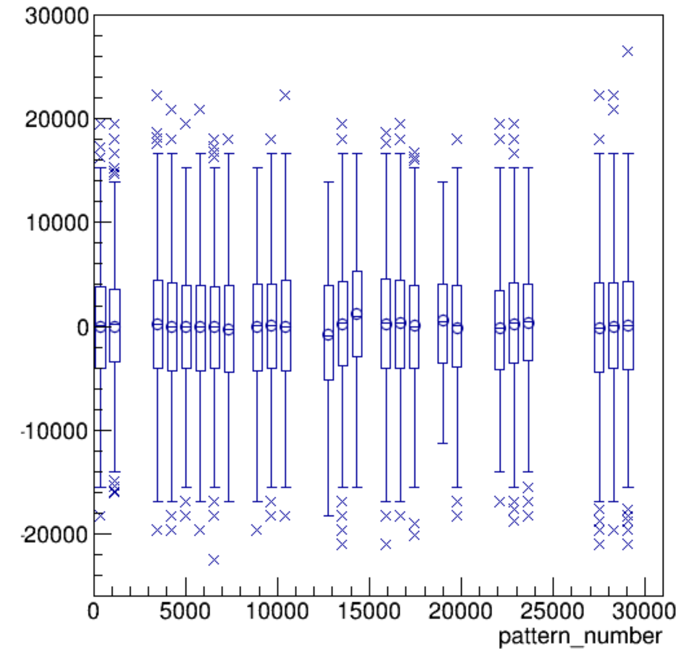
asym_sam4/ppm:pattern_number {ErrorFlag==0}
