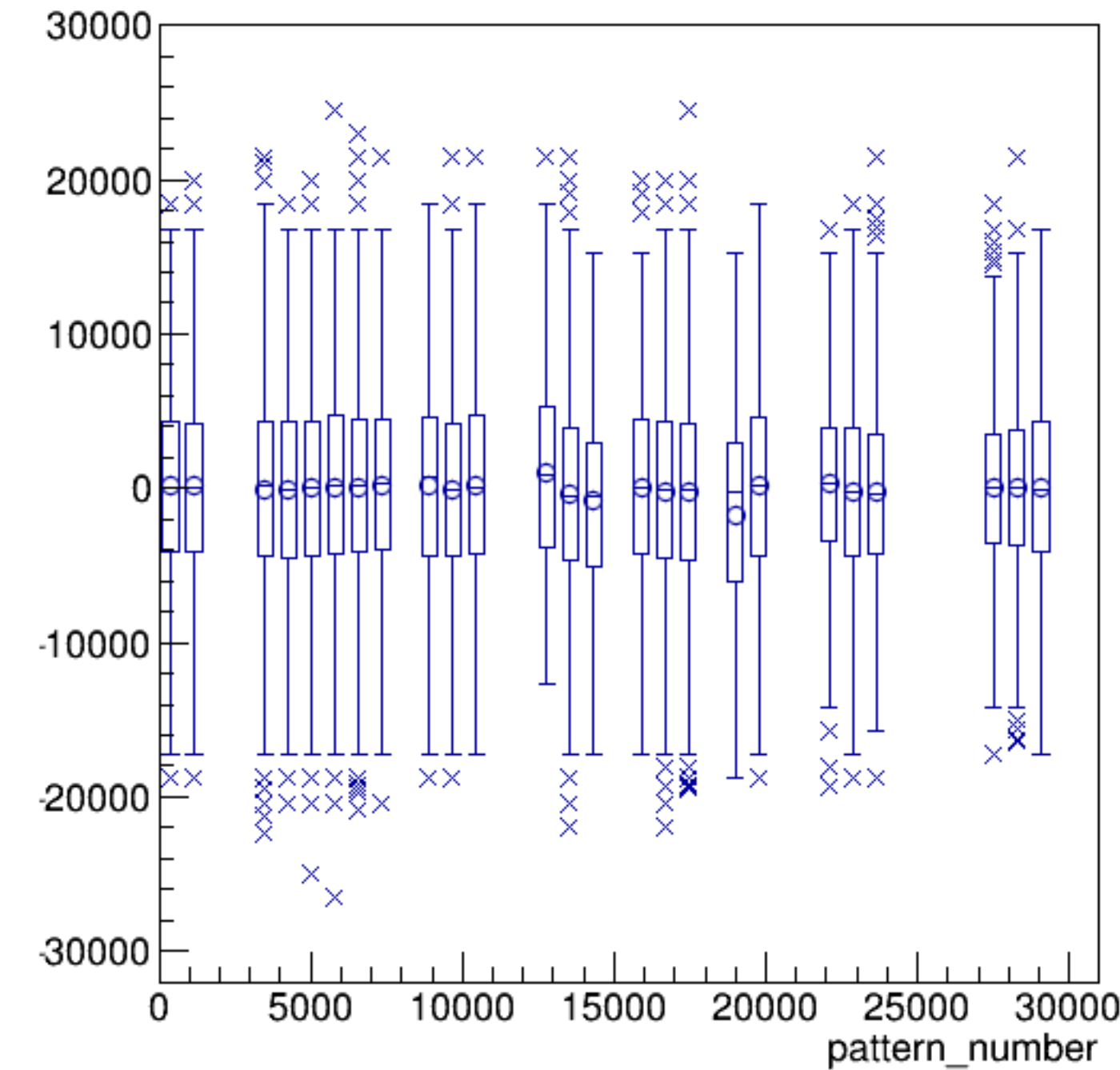
asym_sam6/ppm:pattern_number {ErrorFlag==0}
