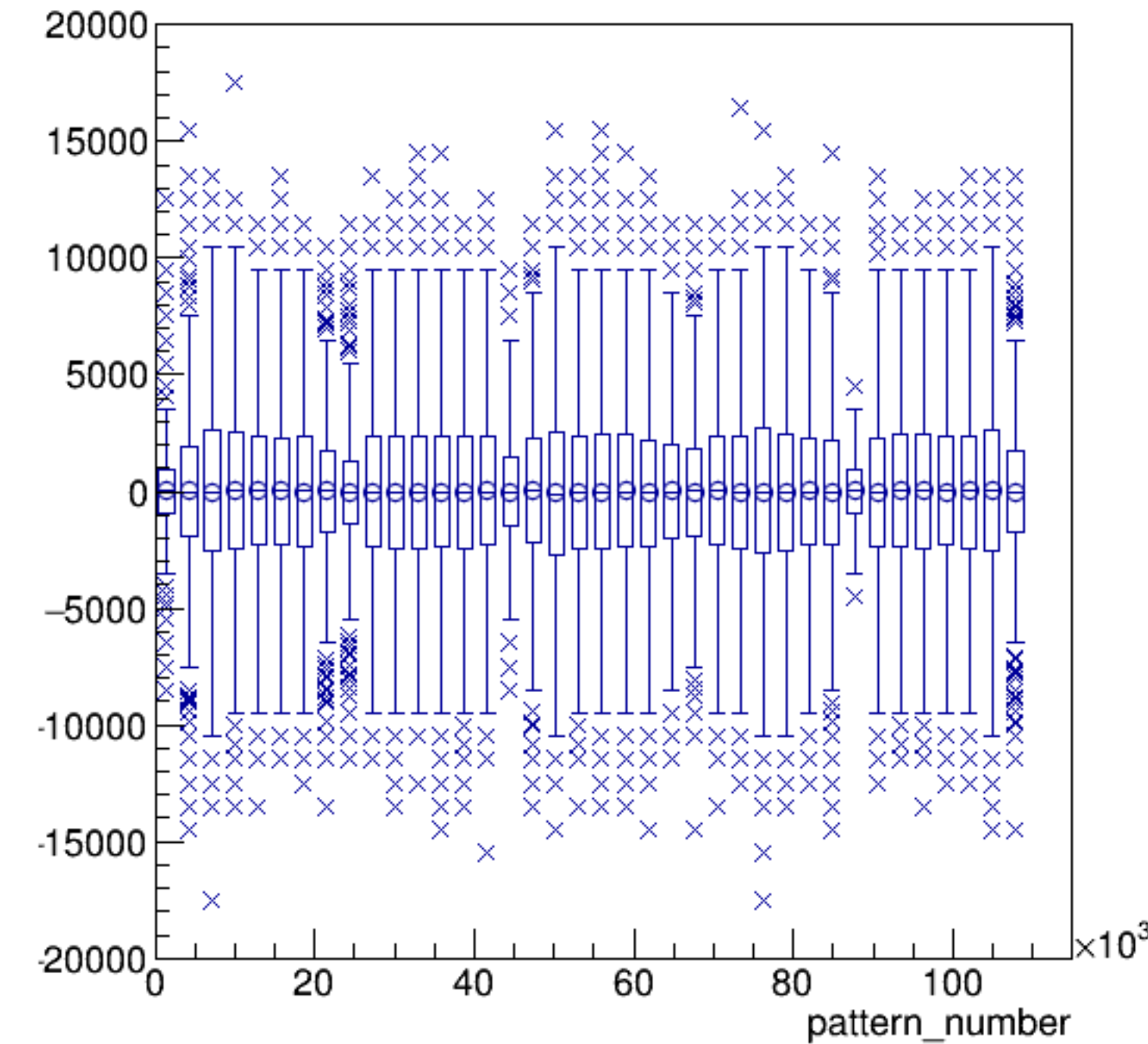
asym_sam1/ppm:pattern_number {ErrorFlag==0}
