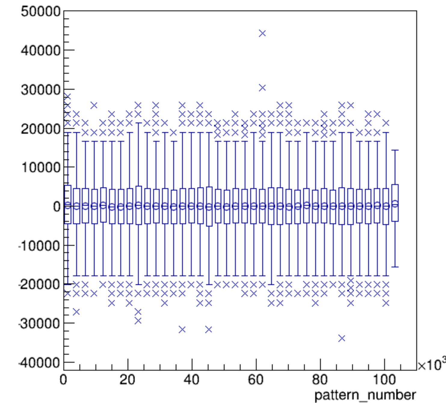
asym_sam7/ppm:pattern_number {ErrorFlag==0}
