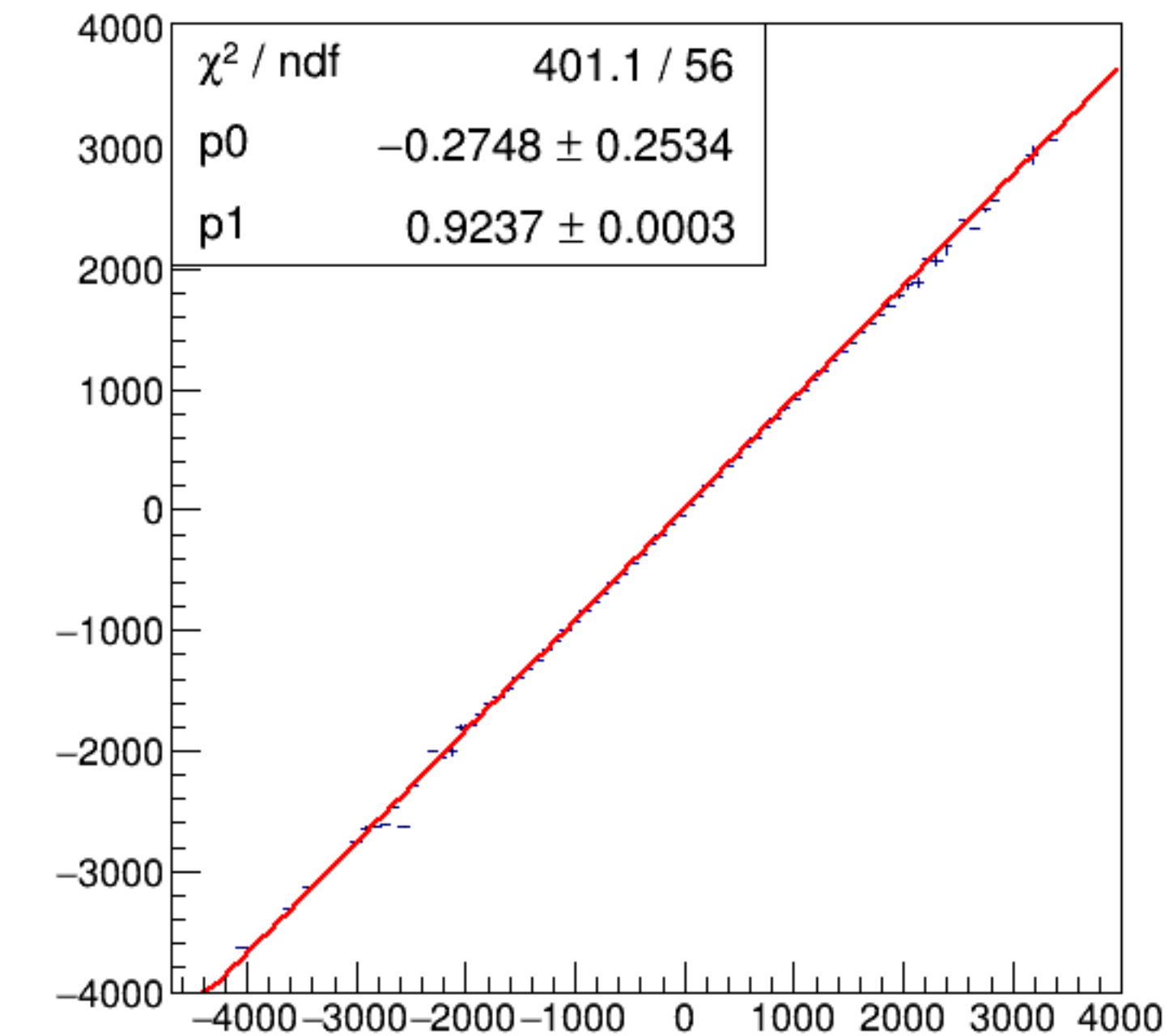
run3675_000_asym_bcm_dg_us_vs_asym_bcm_dg_ds_pr.png
