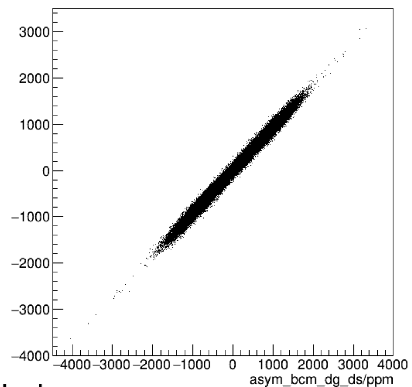
run3675_000_asym_bcm_dg_us_vs_asym_bcm_dg_ds_pr.png
