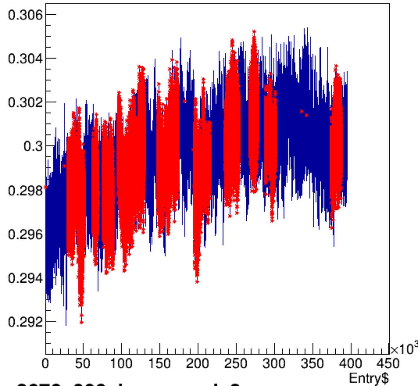
bcm_an_ds3:Entry$
