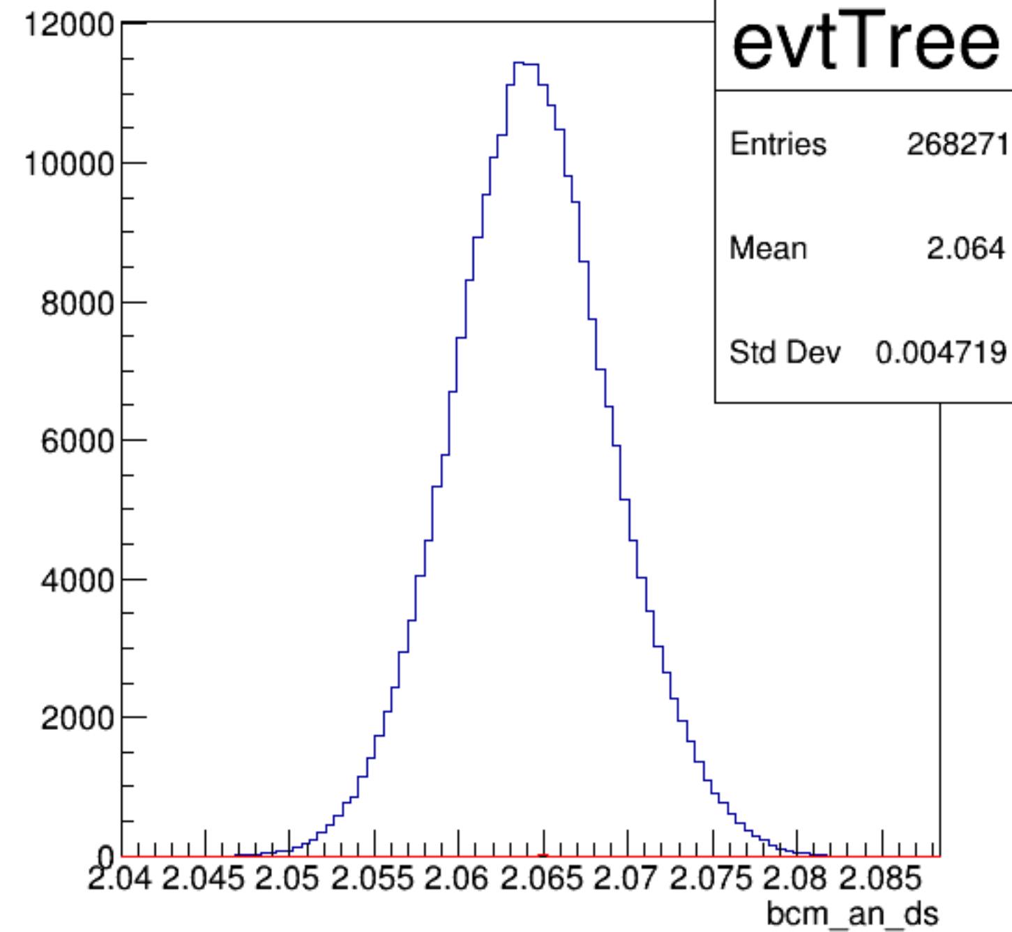
bcm_an_ds {ErrorFlag==0}
