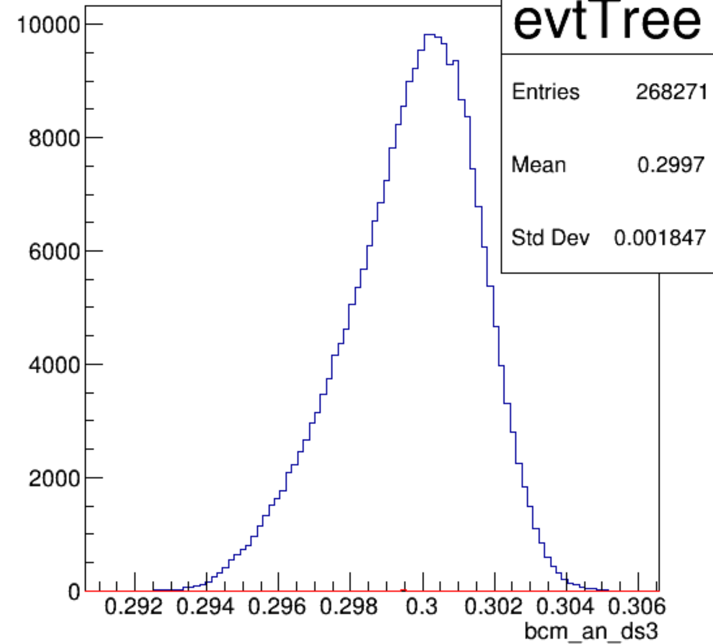
bcm_an_ds3 {ErrorFlag==0}
