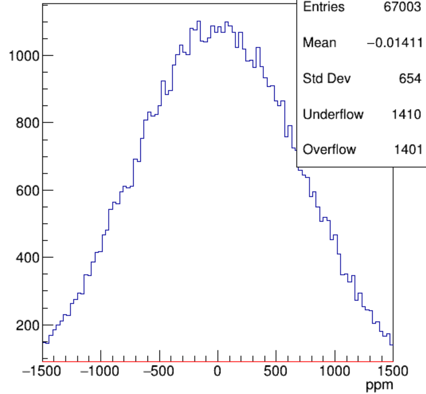
asym_bcm_an_ds3
