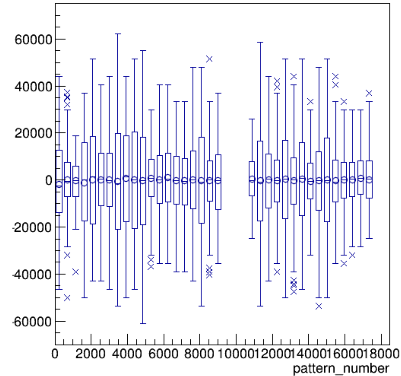
asym_sam4/ppm:pattern_number {ErrorFlag==0}
