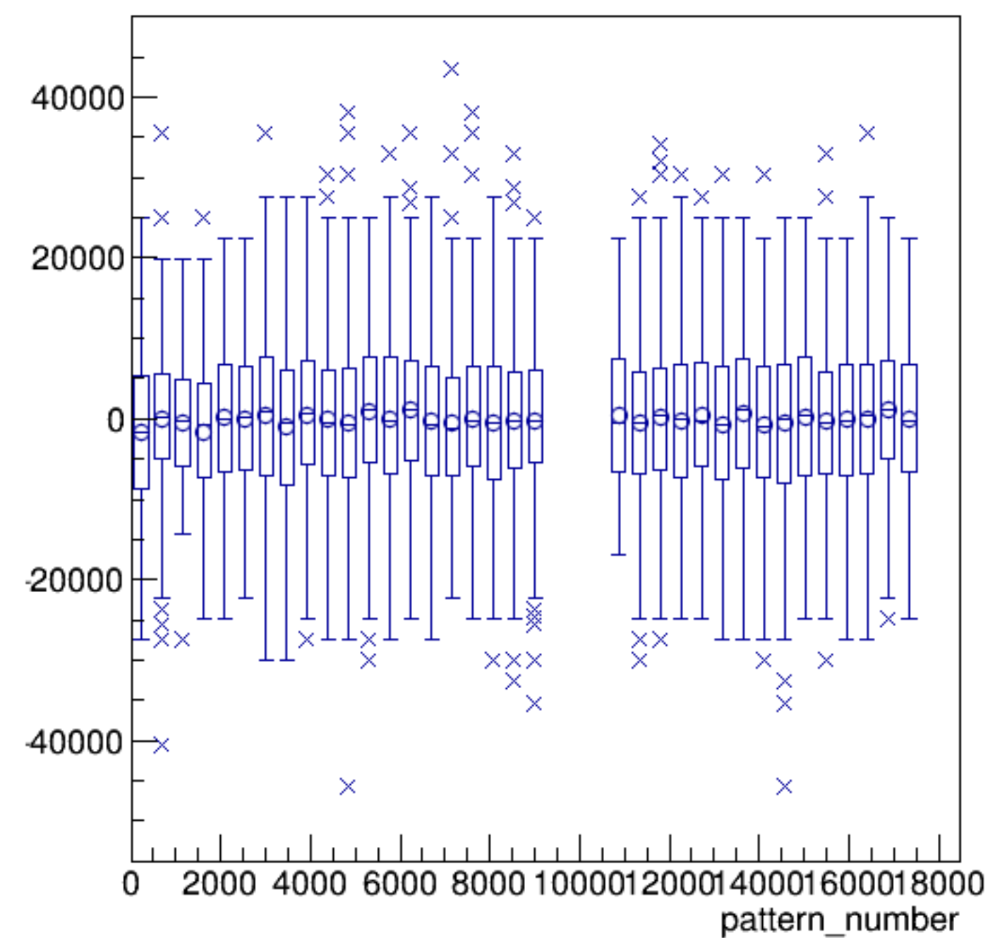
asym_sam2/ppm:pattern_number {ErrorFlag==0}
