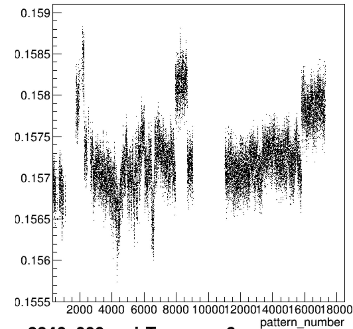
yield_sam8:pattern_number {ErrorFlag==0}
