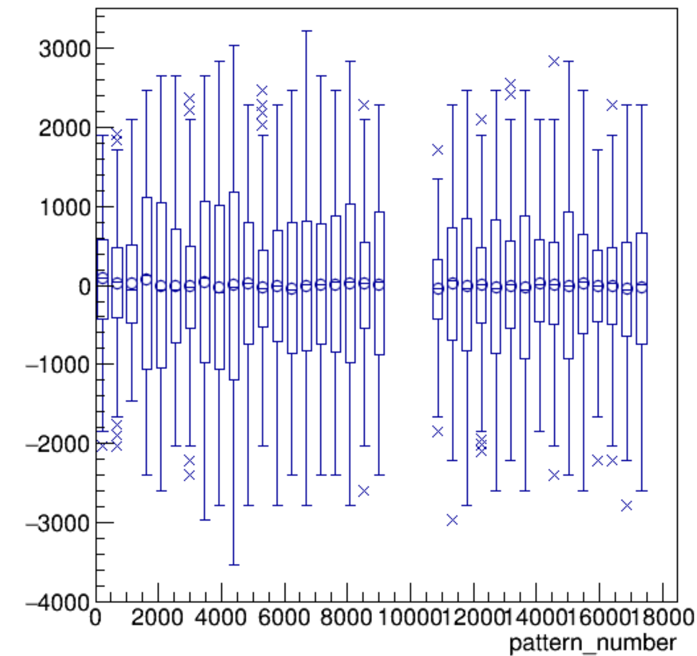
asym_sam8/ppm:pattern_number {ErrorFlag==0}
