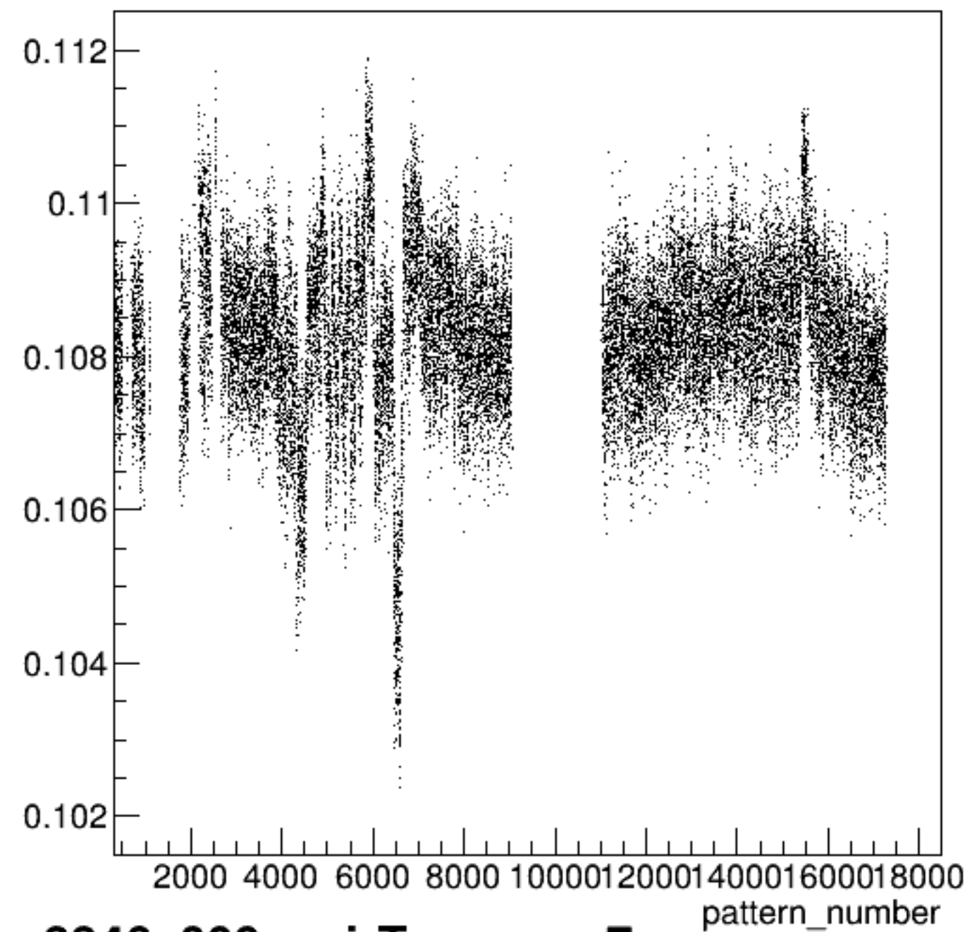
yield_sam7:pattern_number {ErrorFlag==0}
