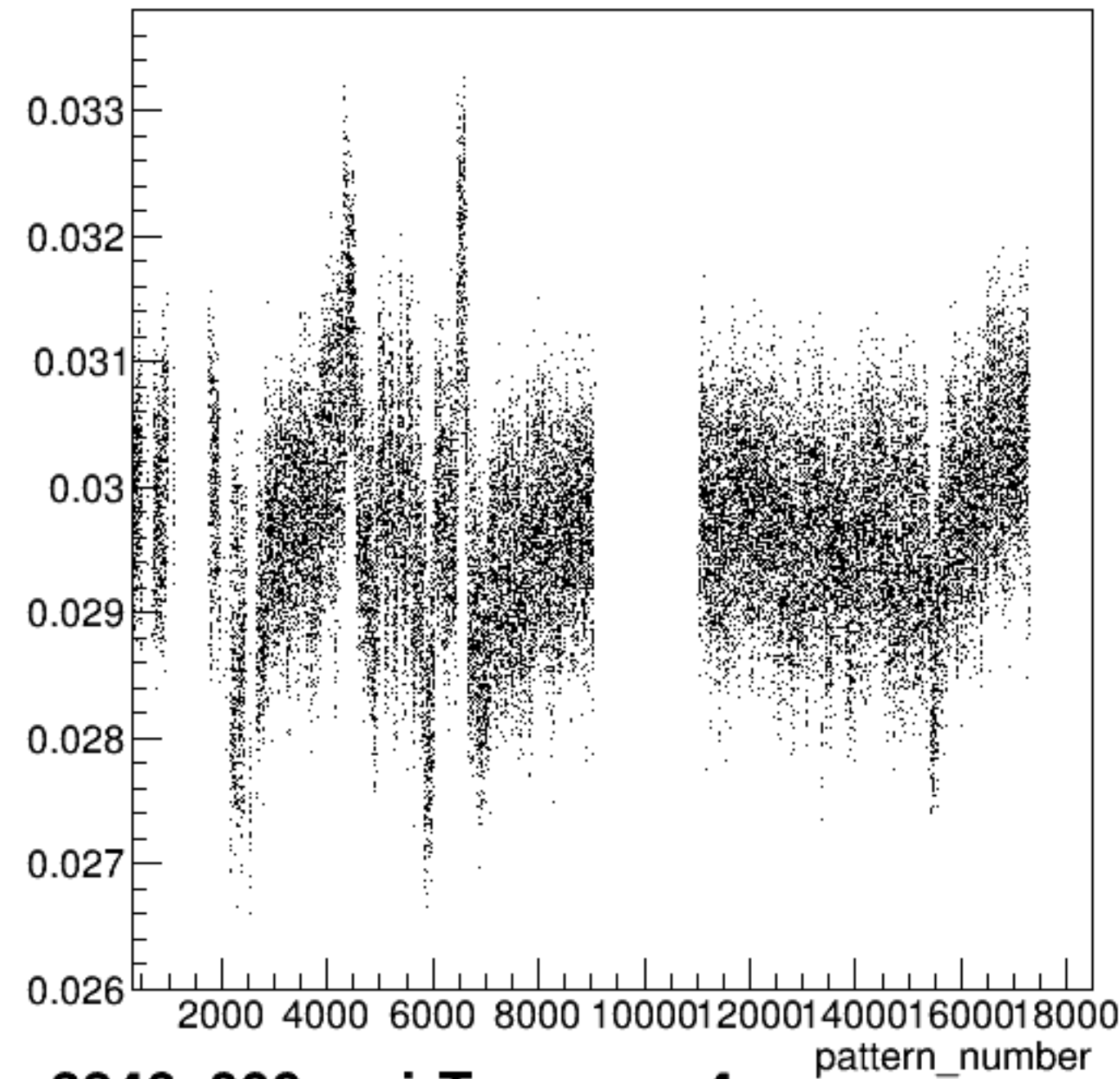
yield_sam4:pattern_number {ErrorFlag==0}
