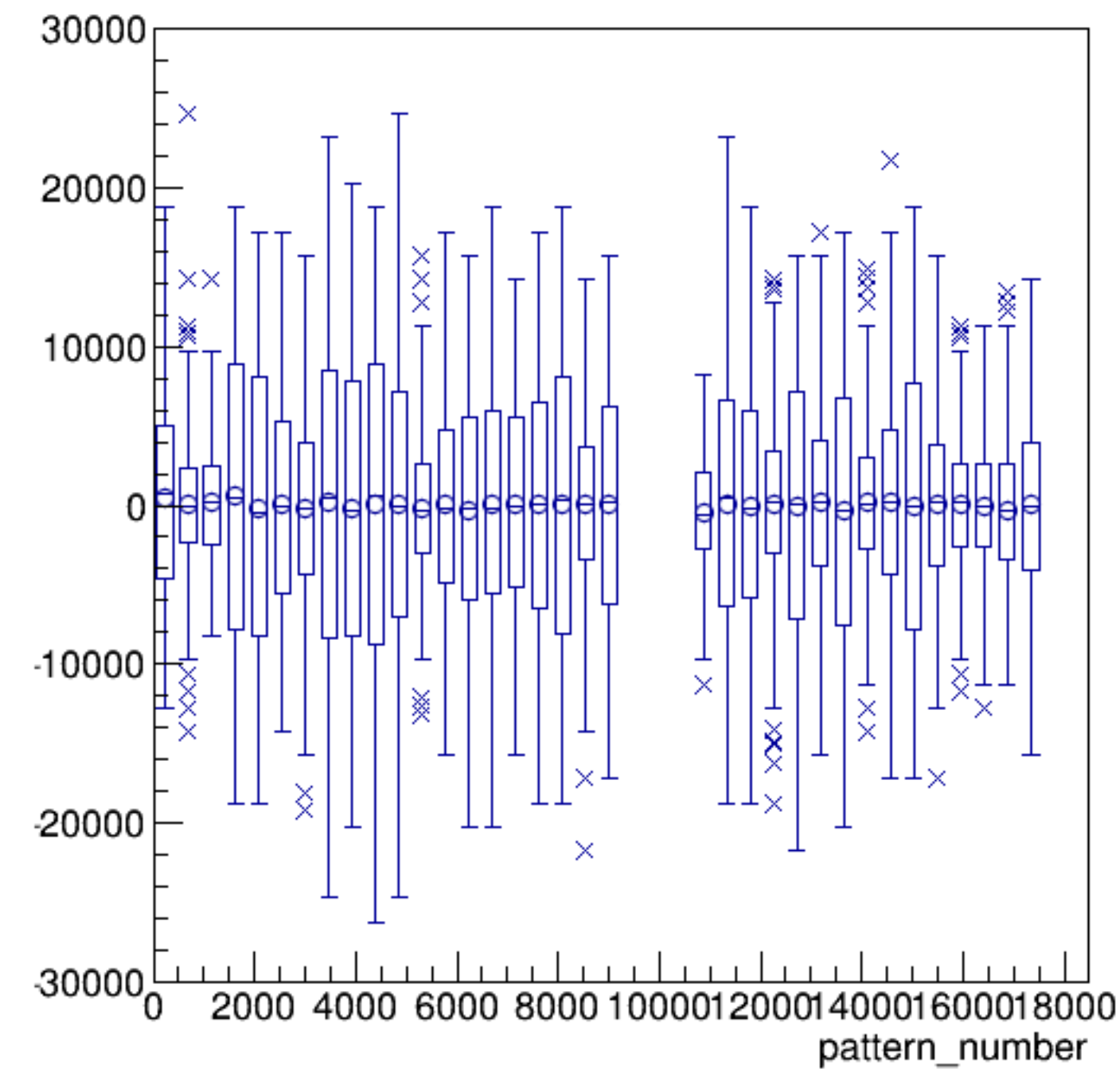
asym_sam6/ppm:pattern_number {ErrorFlag==0}
