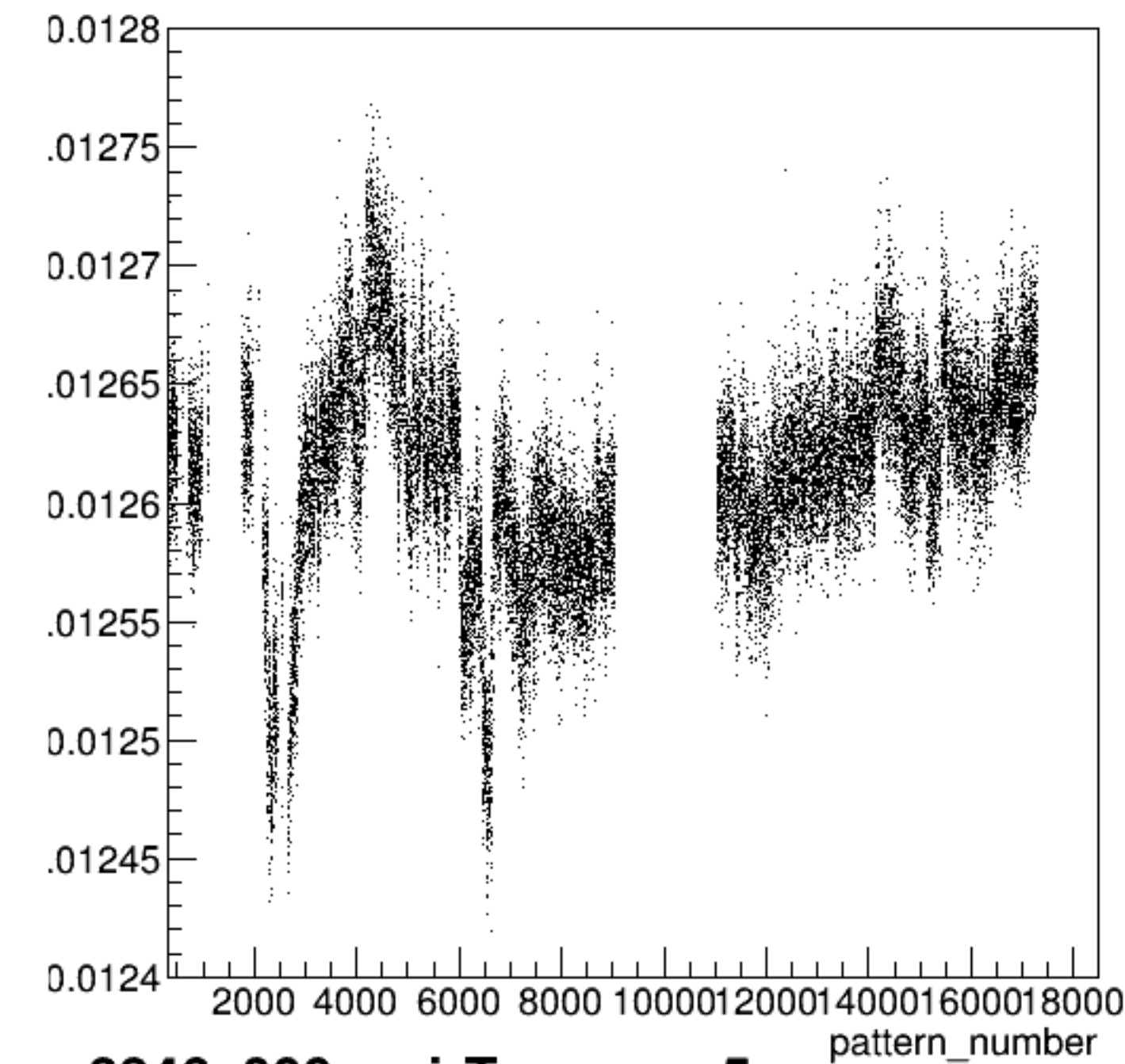
yield_sam5:pattern_number {ErrorFlag==0}
