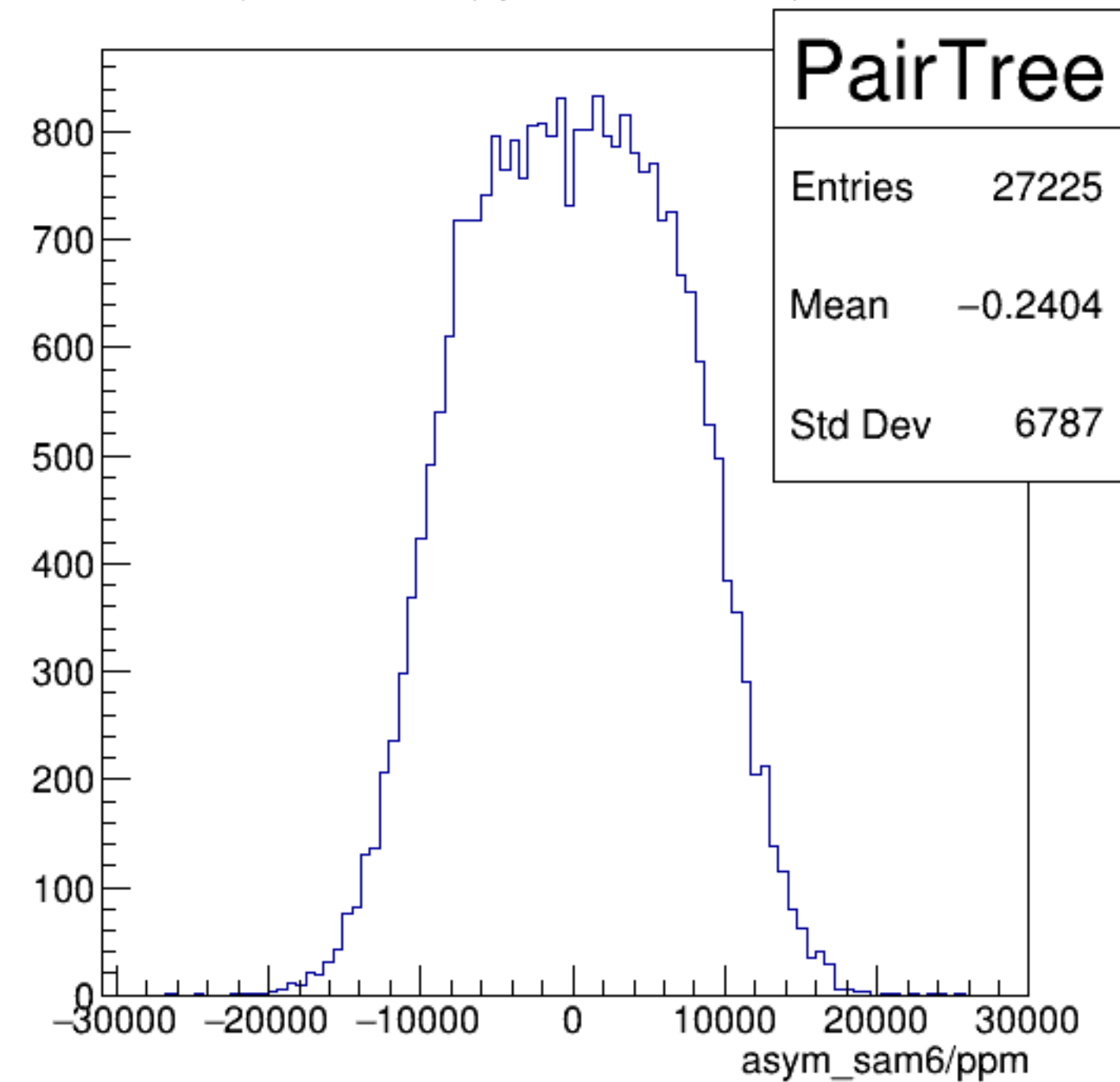
asym_sam6/ppm {ErrorFlag==0}
