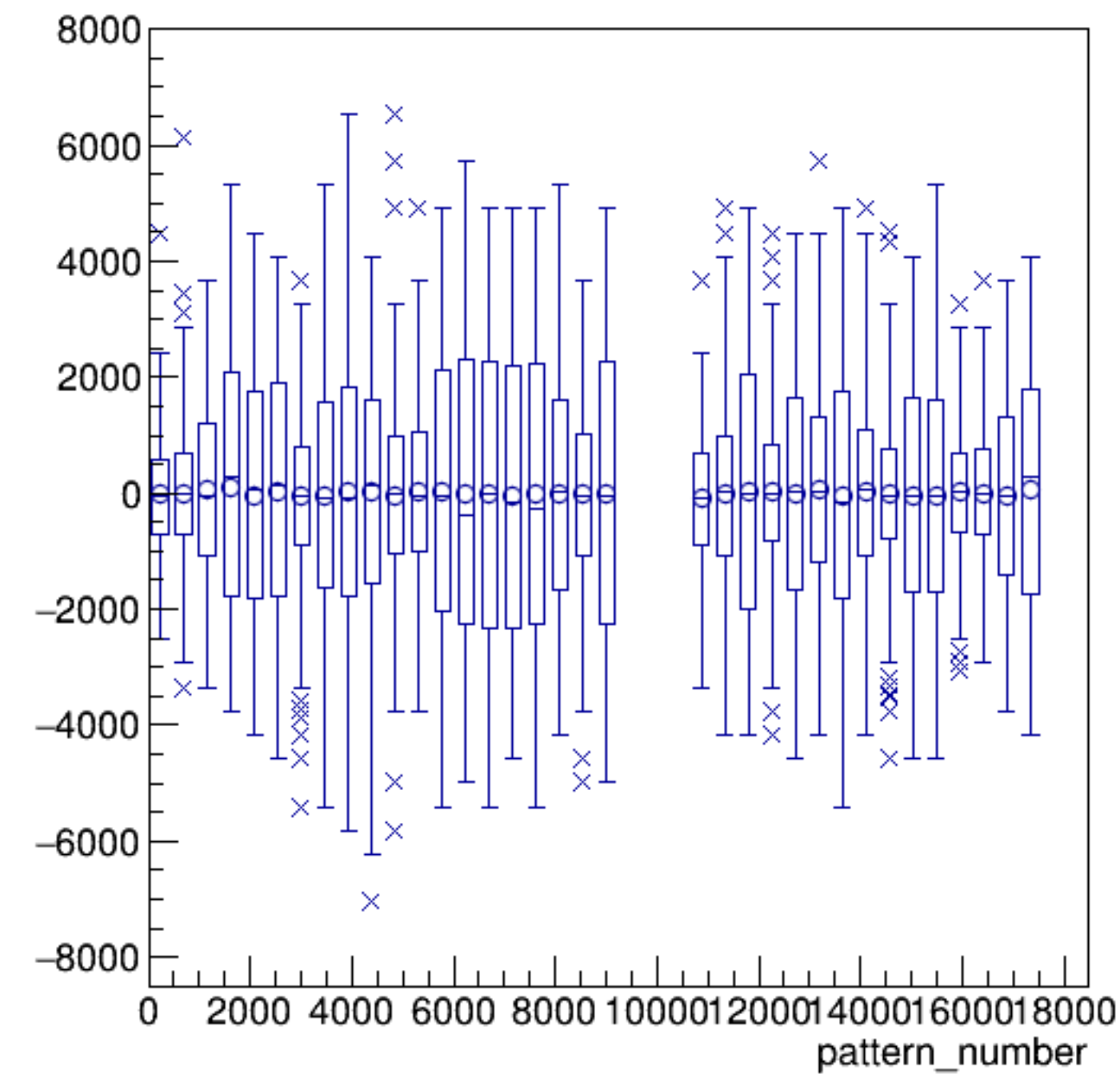
asym_sam5/ppm:pattern_number {ErrorFlag==0}
