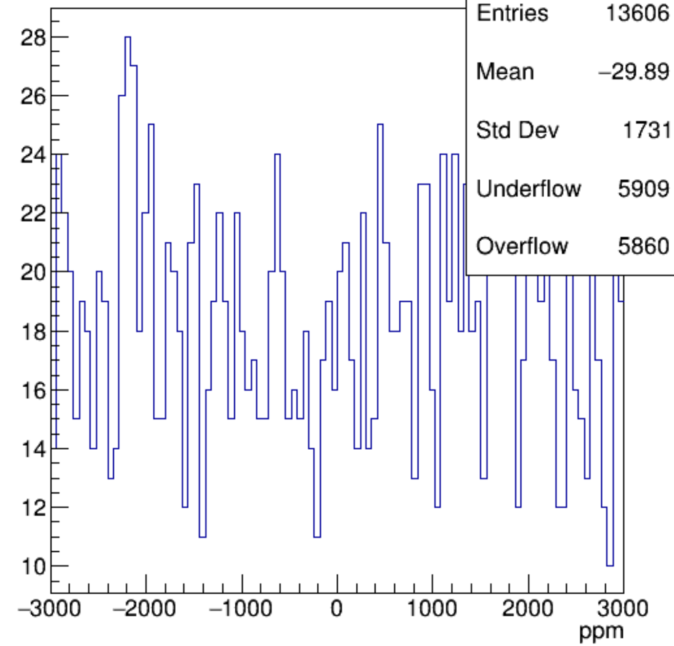
asym_sam3
