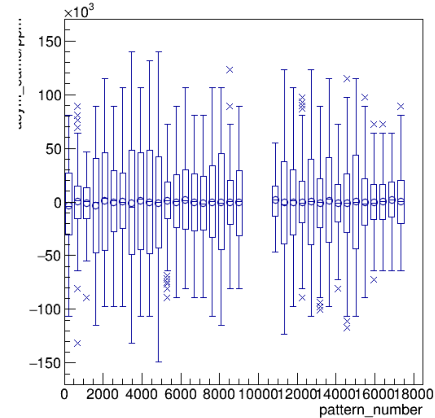
asym_sam3/ppm:pattern_number {ErrorFlag==0}
