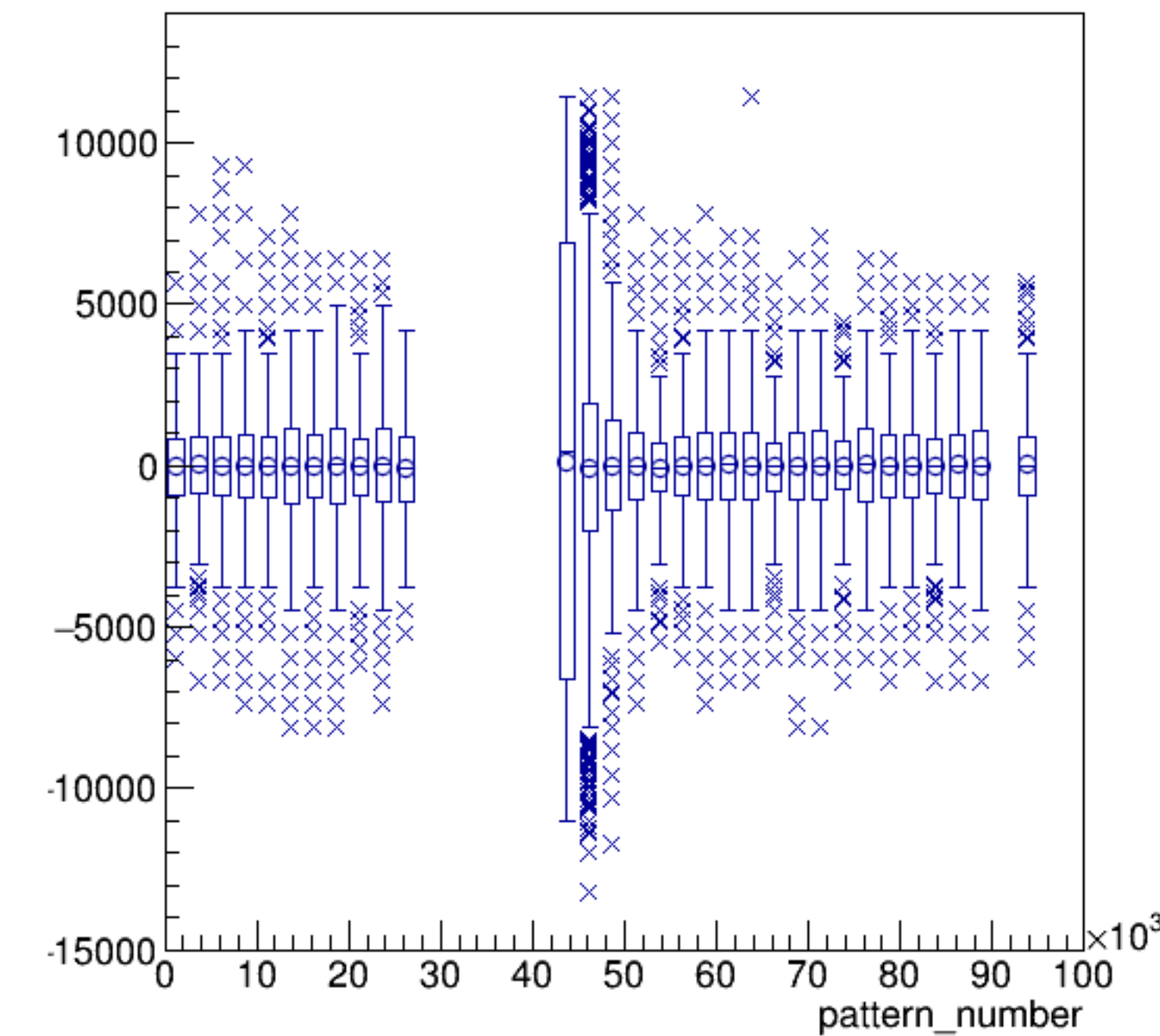
asym_sam1/ppm:pattern_number {ErrorFlag==0}
