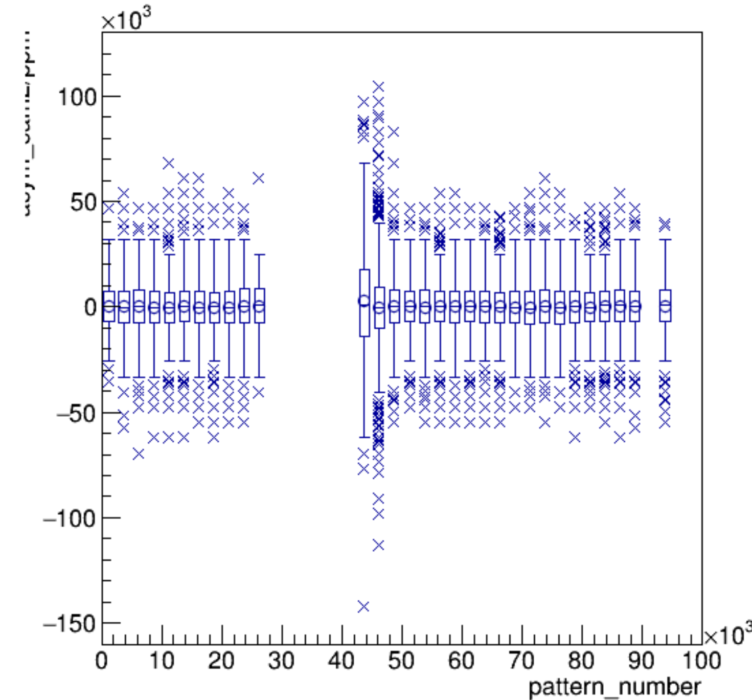
asym_sam2/ppm:pattern_number {ErrorFlag==0}
