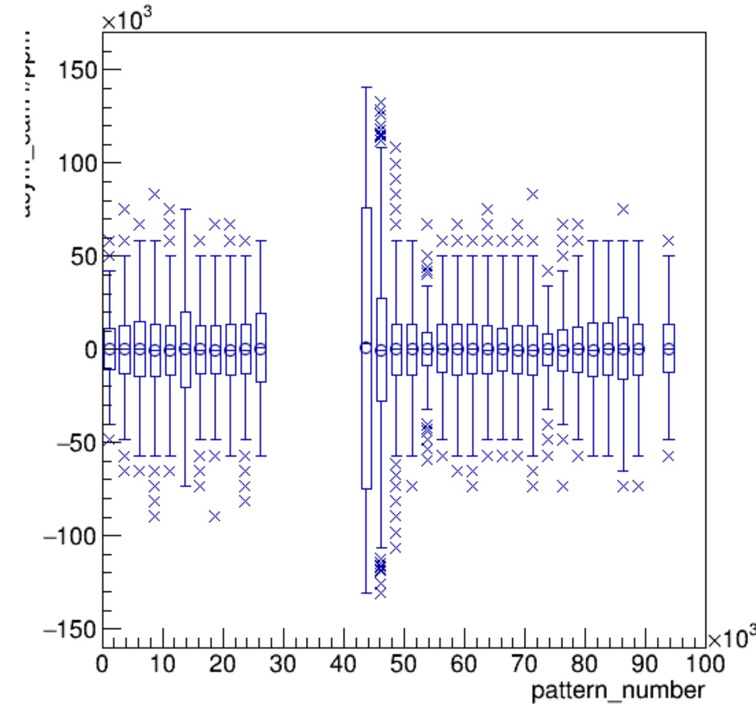
asym_sam4/ppm:pattern_number {ErrorFlag==0}
