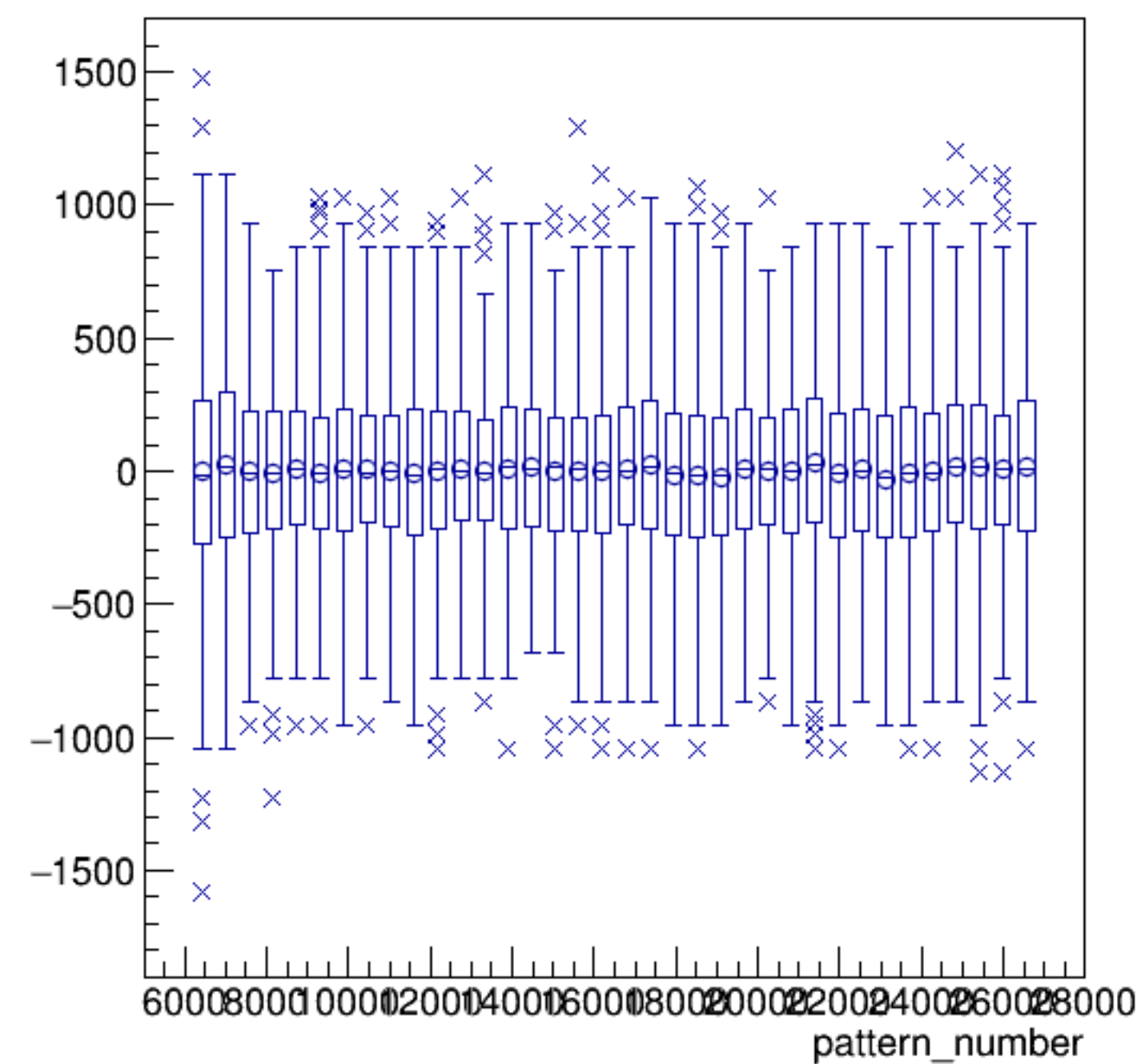
asym_sam8/ppm:pattern_number {ErrorFlag==0}
