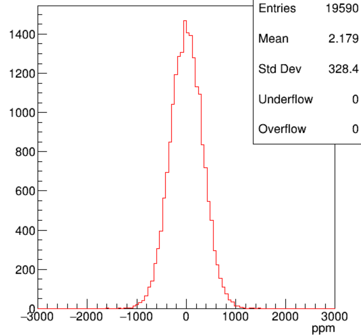
asym_sam8
