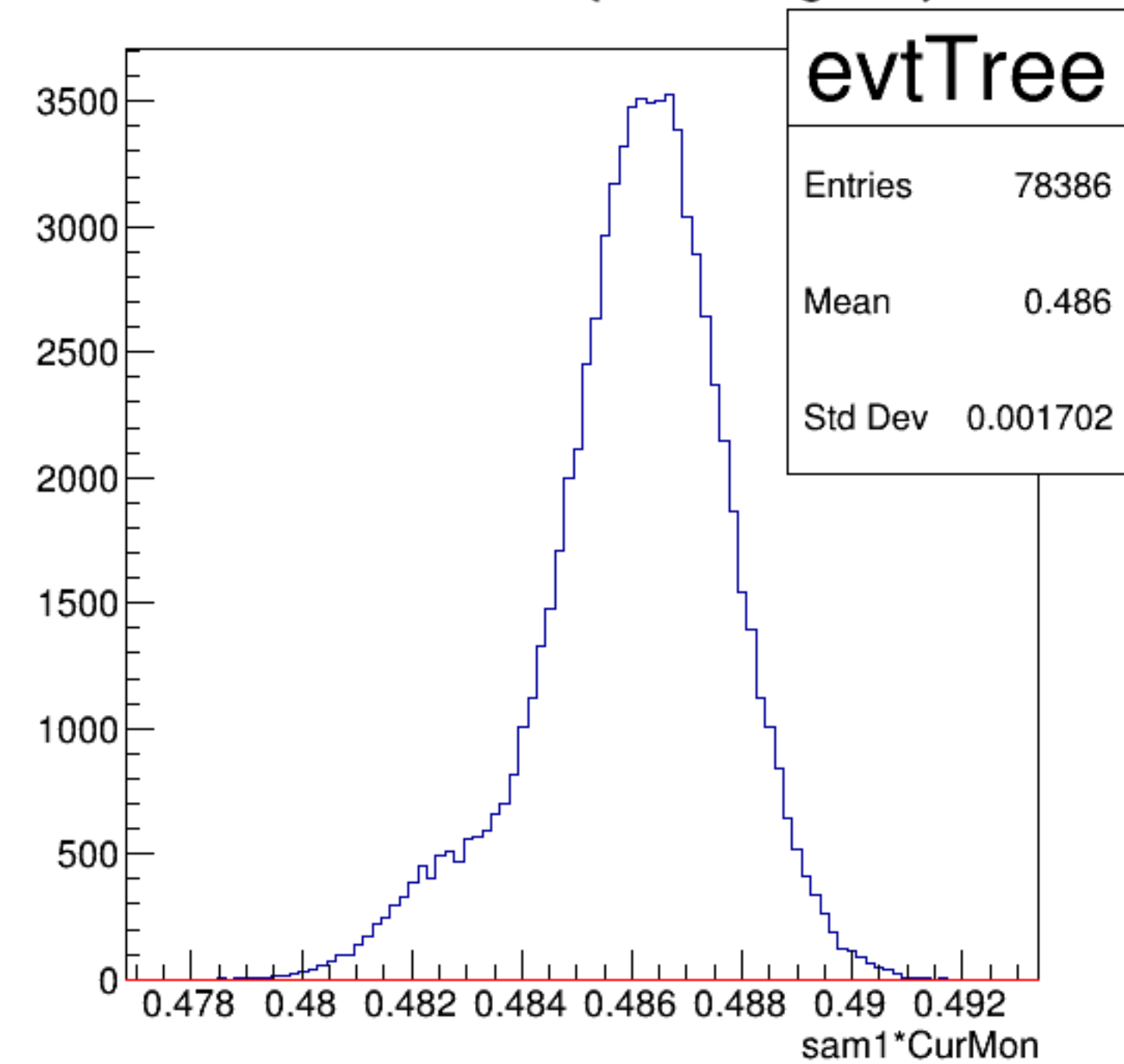
sam1*CurMon {ErrorFlag==0}
