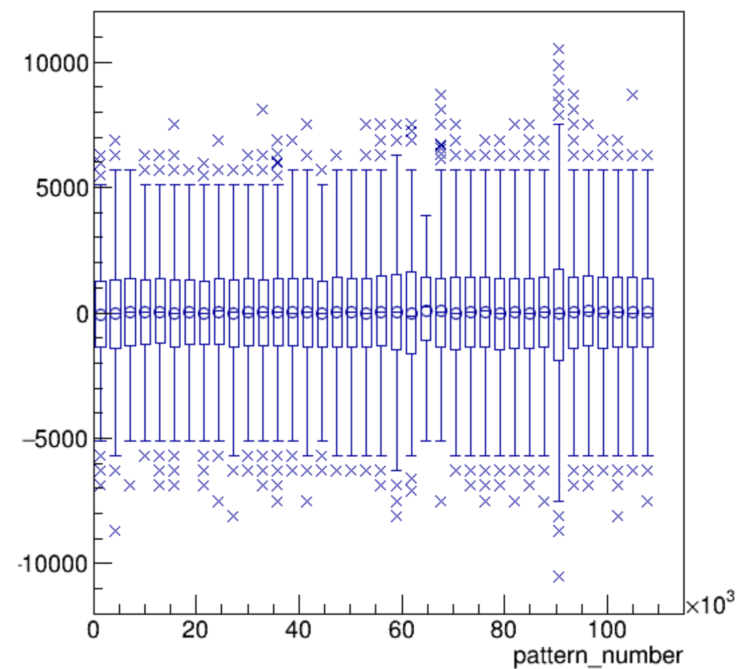
asym_sam6/ppm:pattern_number {ErrorFlag==0}
