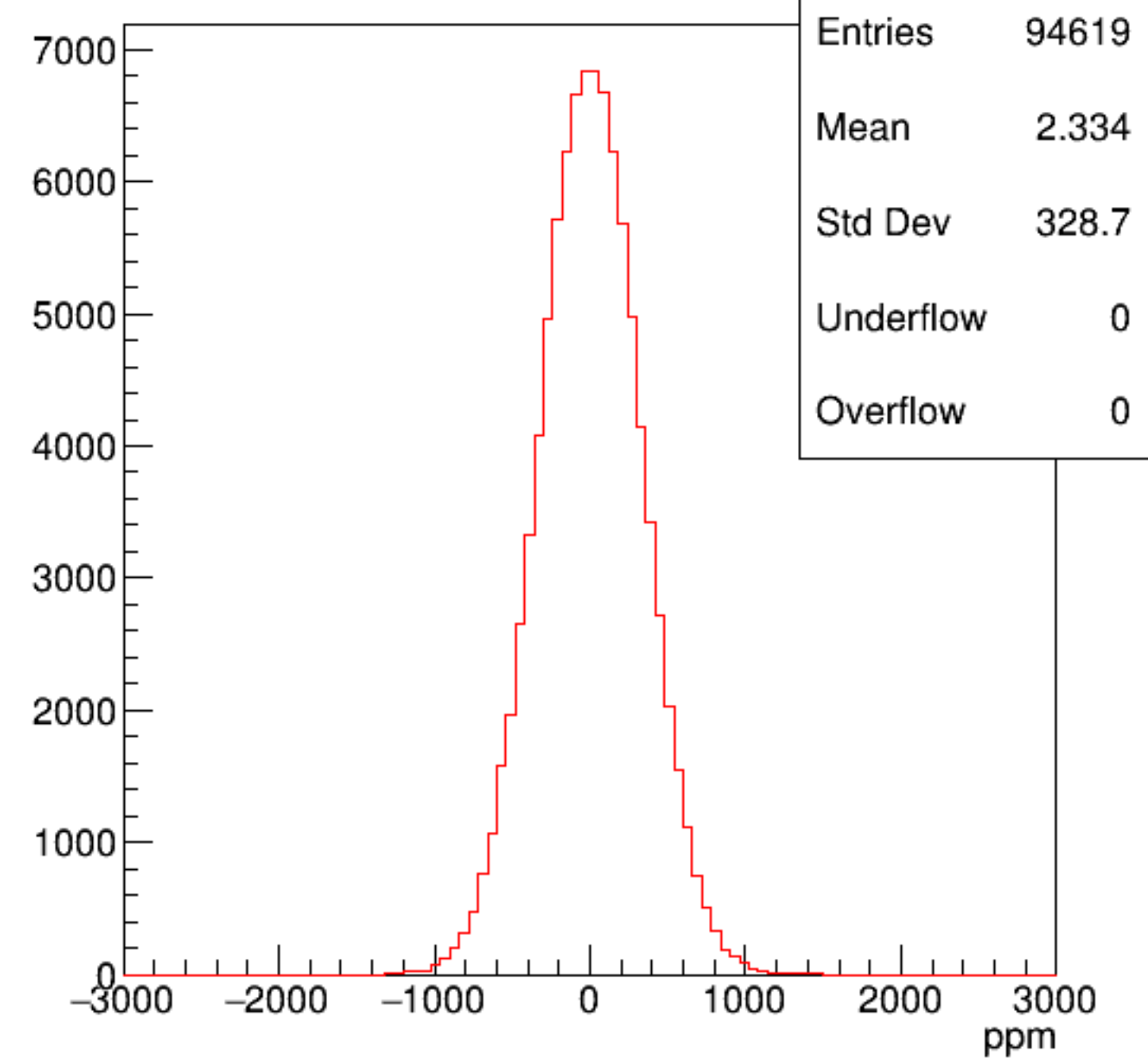
asym_sam8
