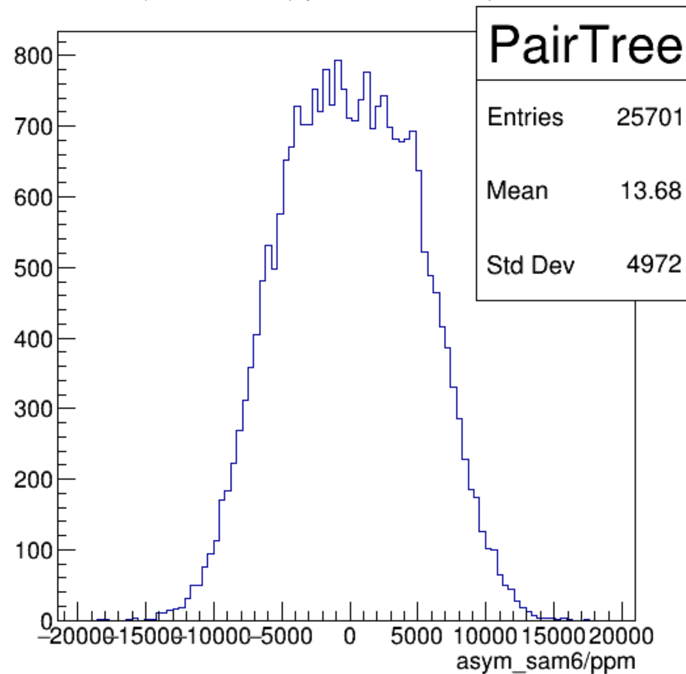
asym_sam6/ppm {ErrorFlag==0}
