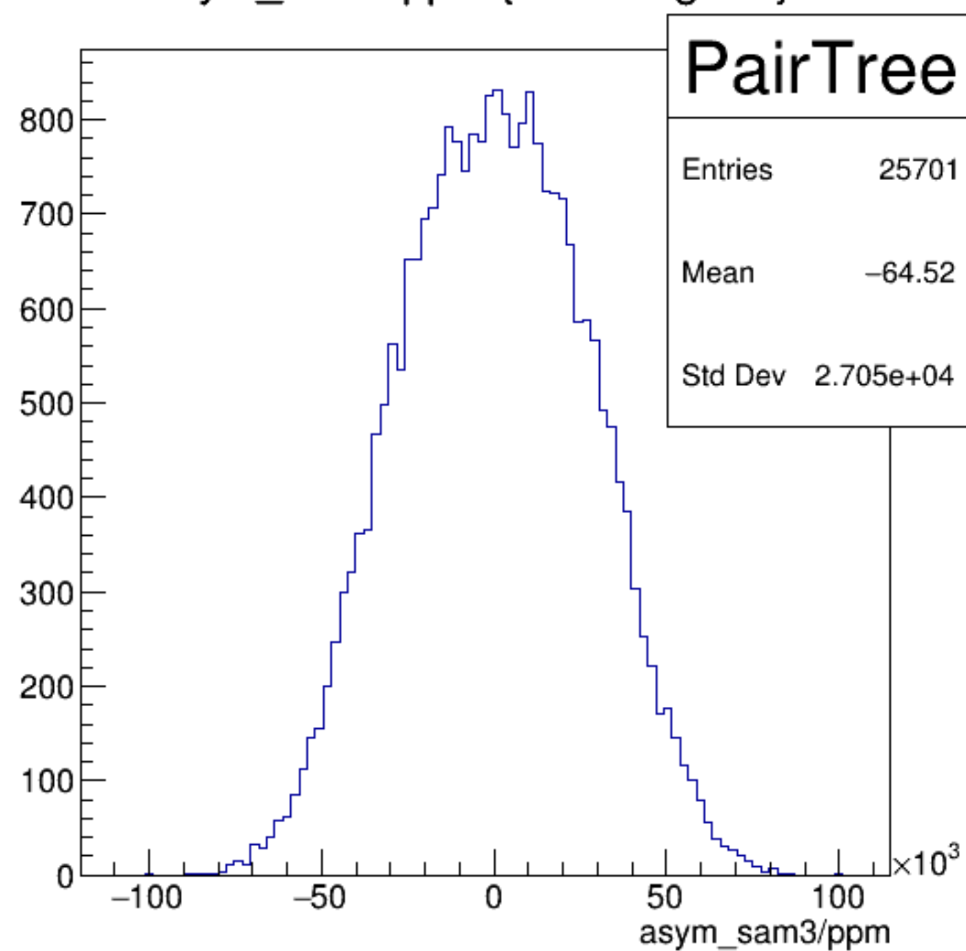
asym_sam3/ppm {ErrorFlag==0}
