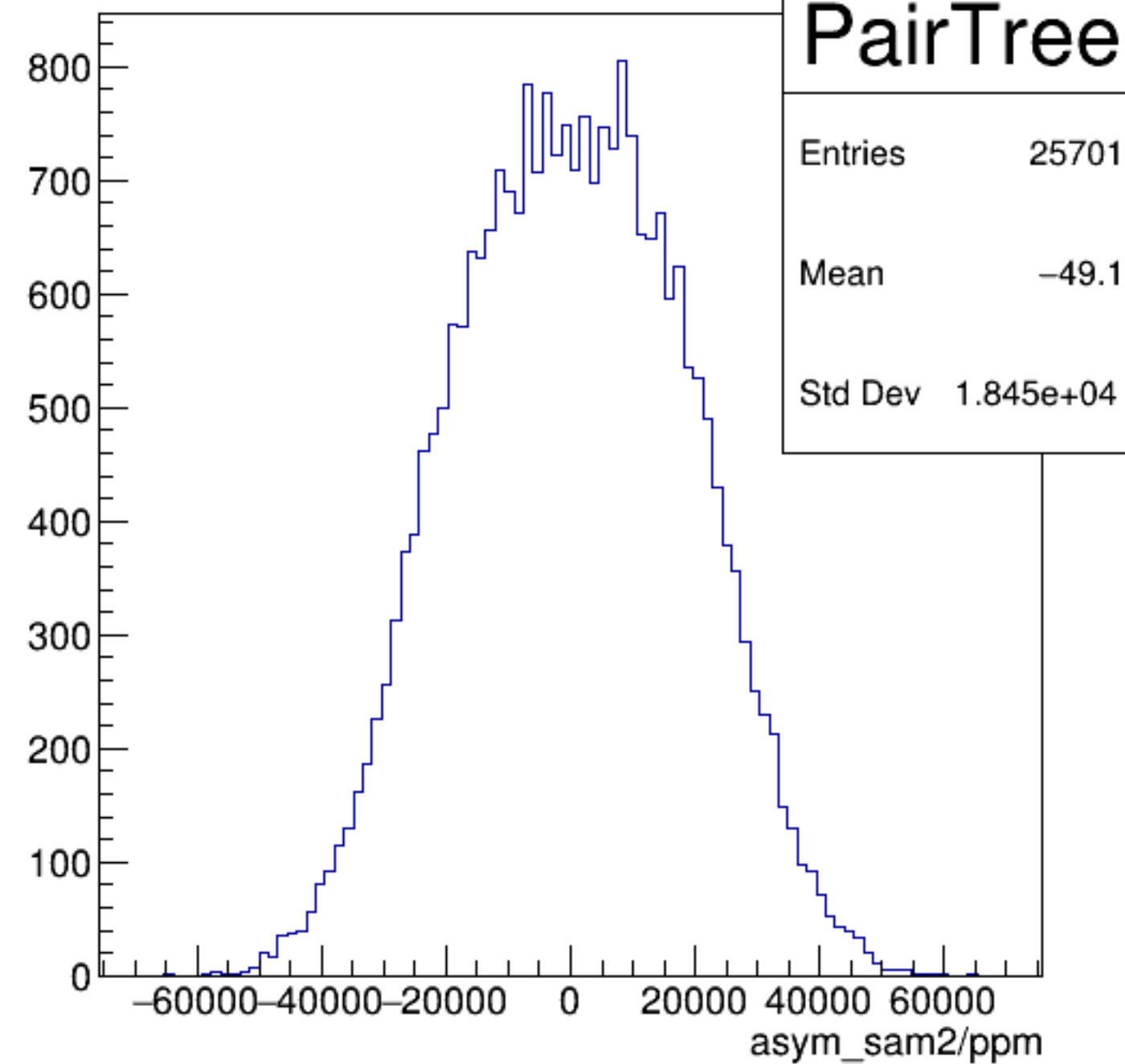
asym_sam2/ppm {ErrorFlag==0}
