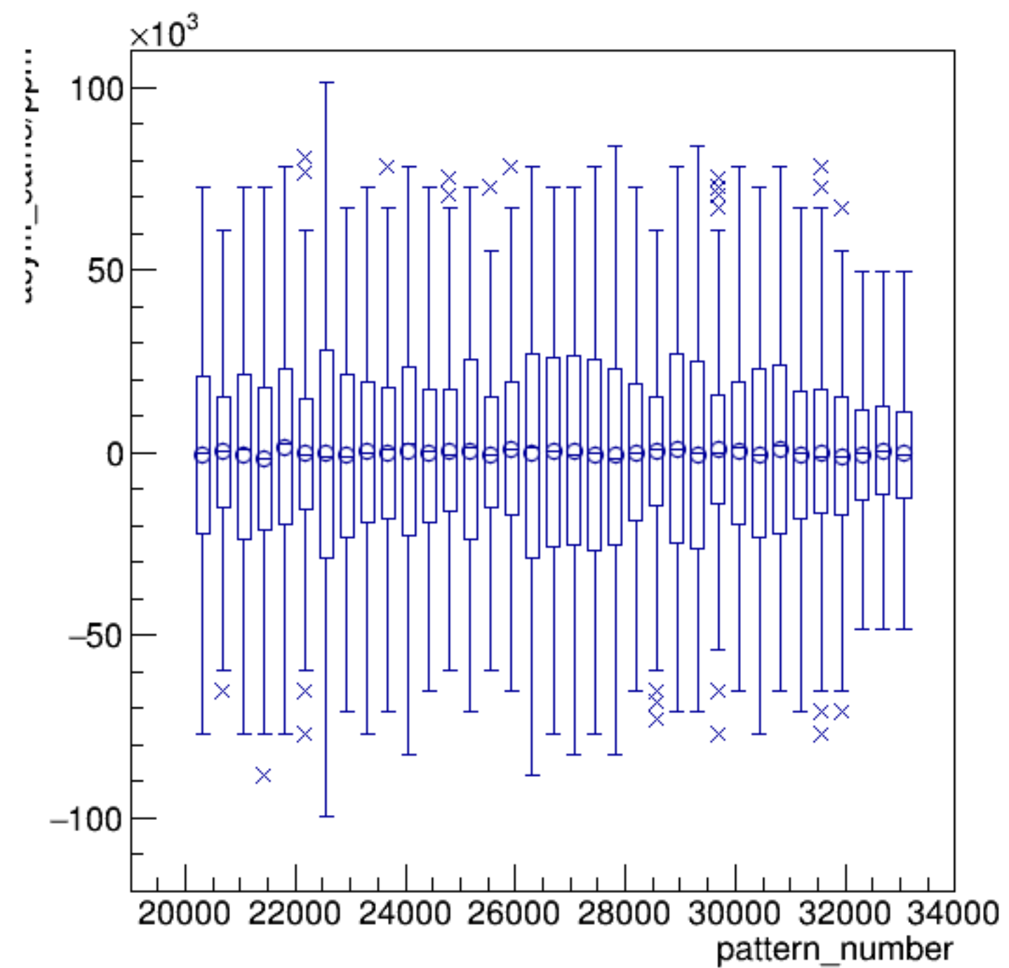
asym_sam3/ppm:pattern_number {ErrorFlag==0}
