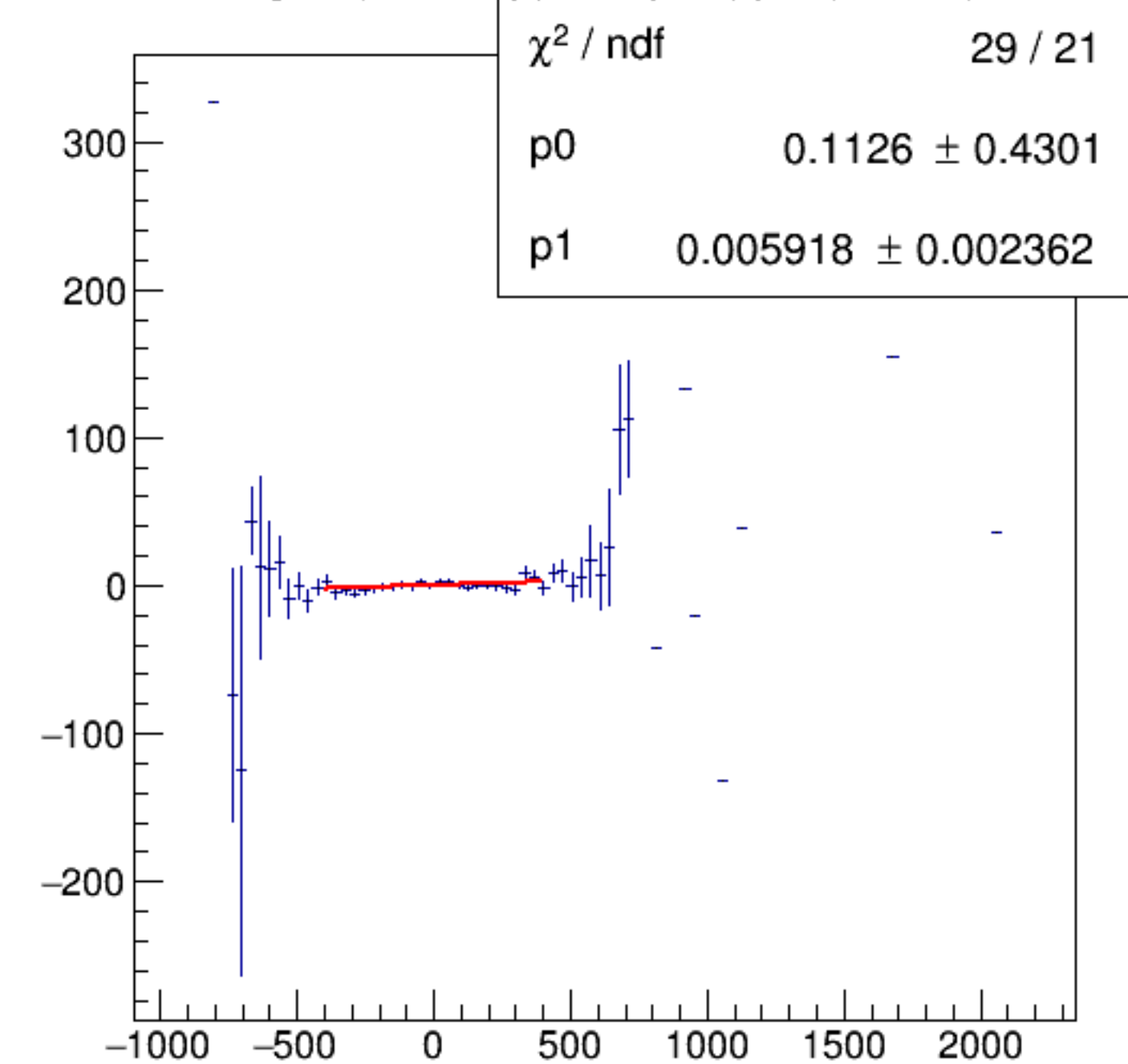
reg_asym_dsr/ppm:AqDS/ppm {ok_cut}
