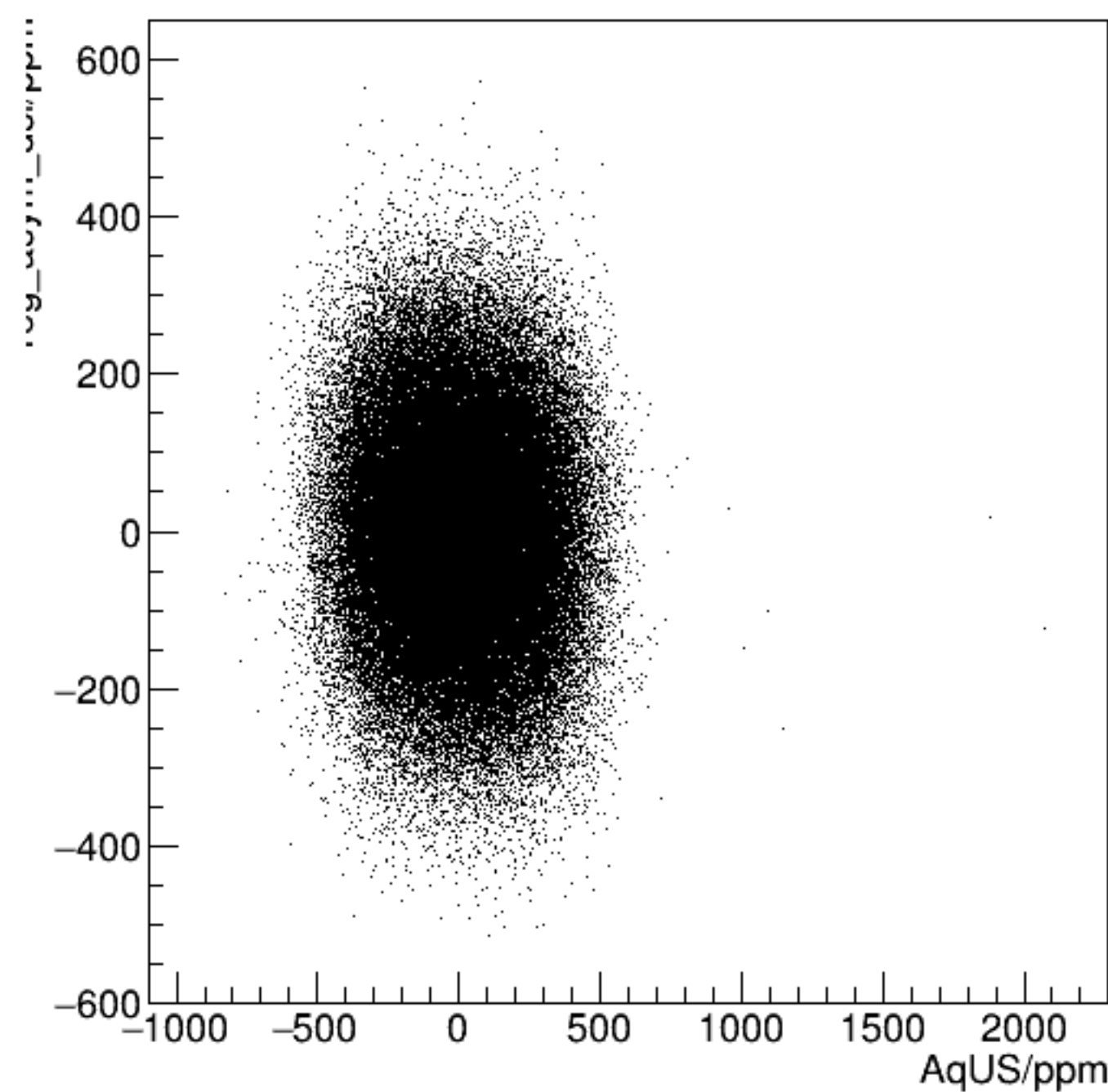
reg_asym_dsl/ppm:AqUS/ppm {ok_cut}
