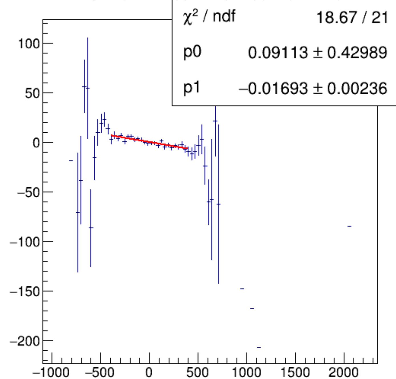
reg_asym_usl/ppm:AqDS/ppm {ok_cut}
