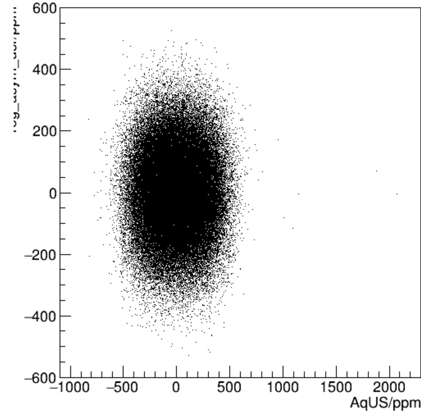
reg_asym_usr/ppm:AqUS/ppm {ok_cut}
