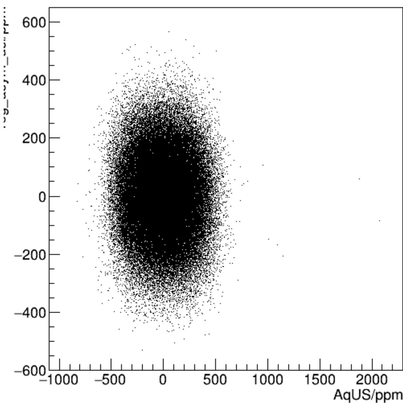
reg_asym_usl/ppm:AqUS/ppm {ok_cut}
