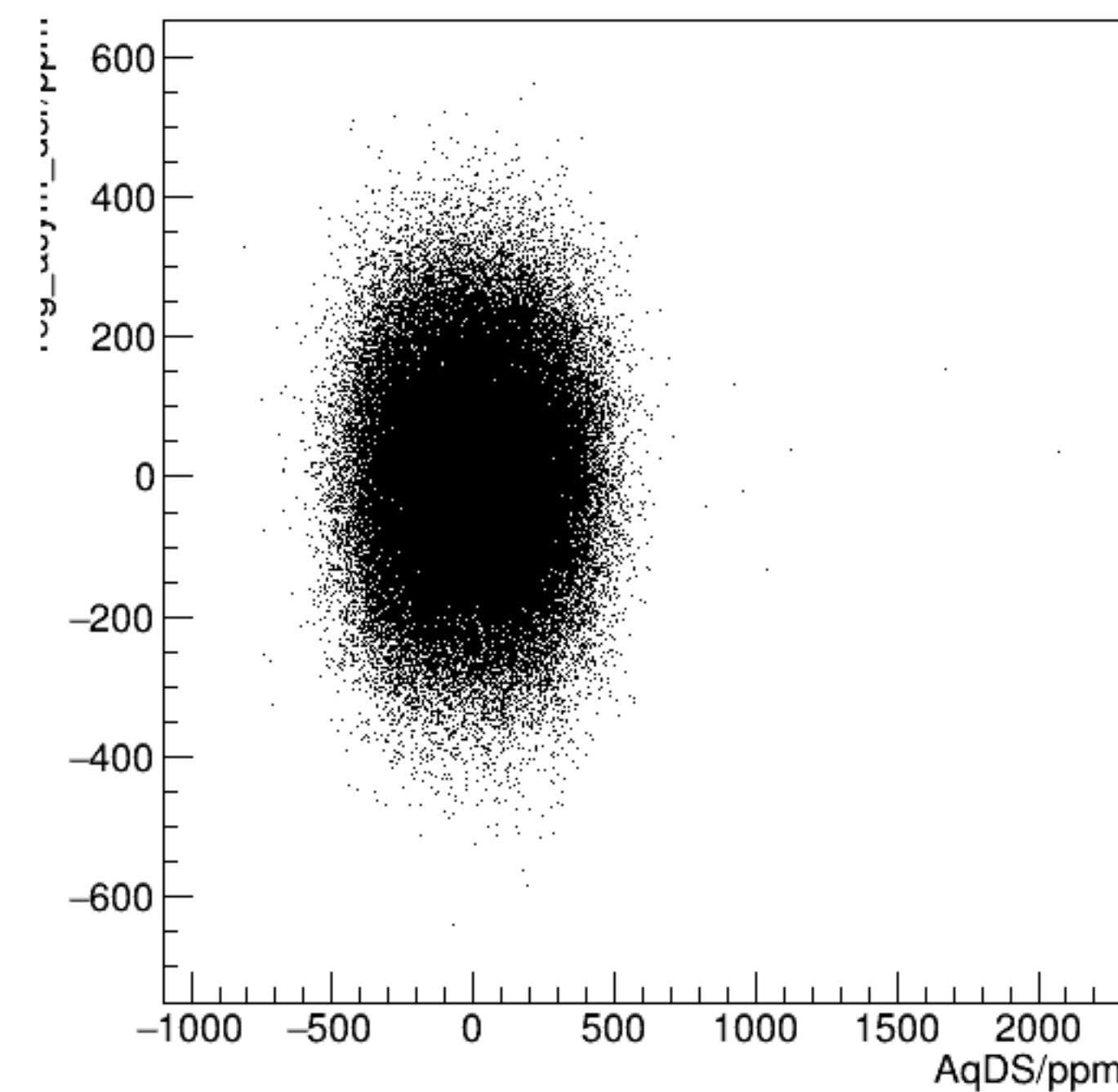
reg_asym_dsr/ppm:AqDS/ppm {ok_cut}
