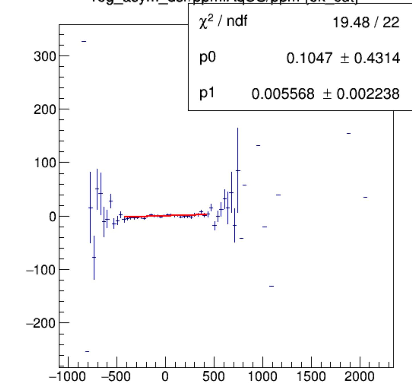
reg_asym_dsr/ppm:AqUS/ppm {ok_cut}
