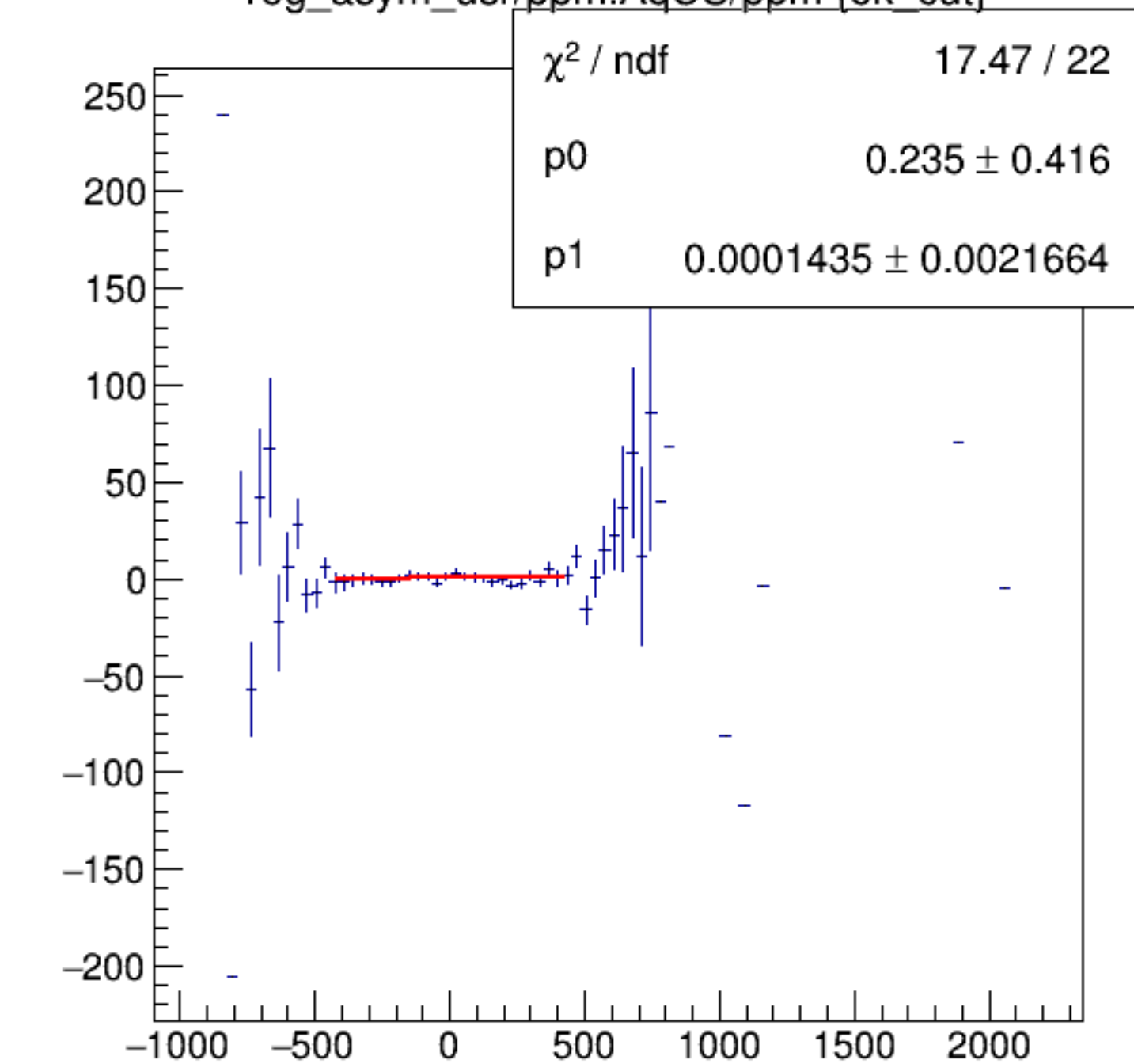
reg_asym_usr/ppm:AqUS/ppm {ok_cut}
