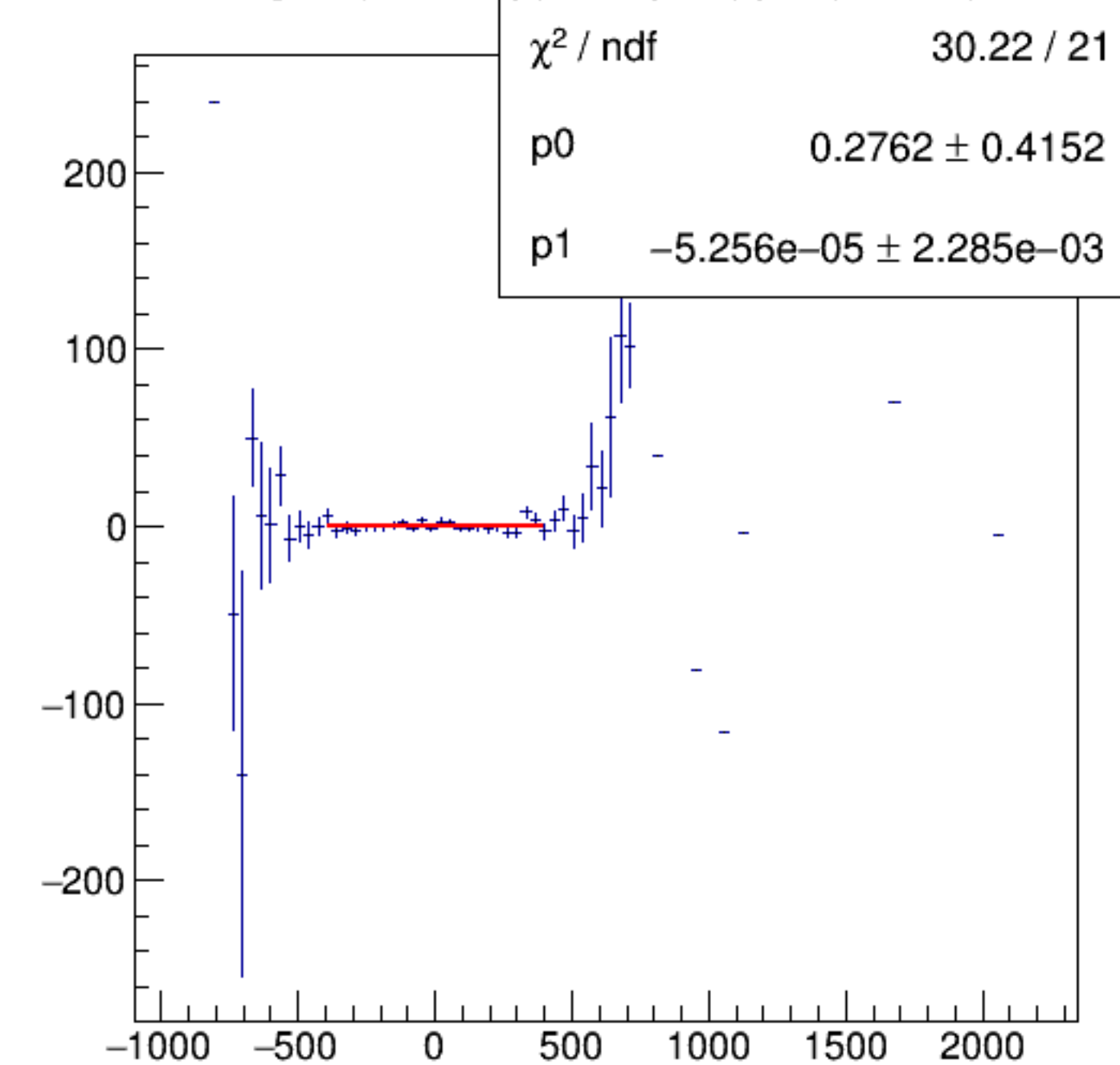
reg_asym_usr/ppm:AqDS/ppm {ok_cut}
