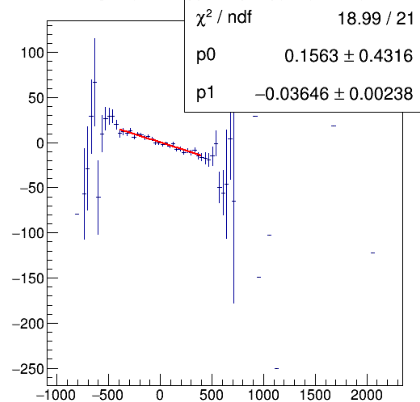
reg_asym_dsl/ppm:AqDS/ppm {ok_cut}
