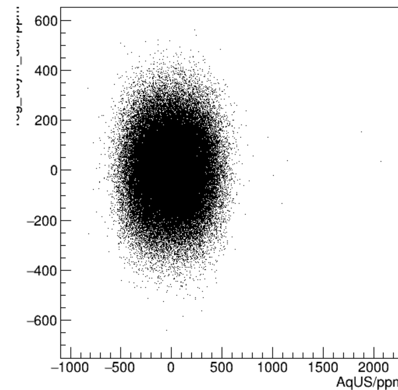
reg_asym_dsr/ppm:AqUS/ppm {ok_cut}
