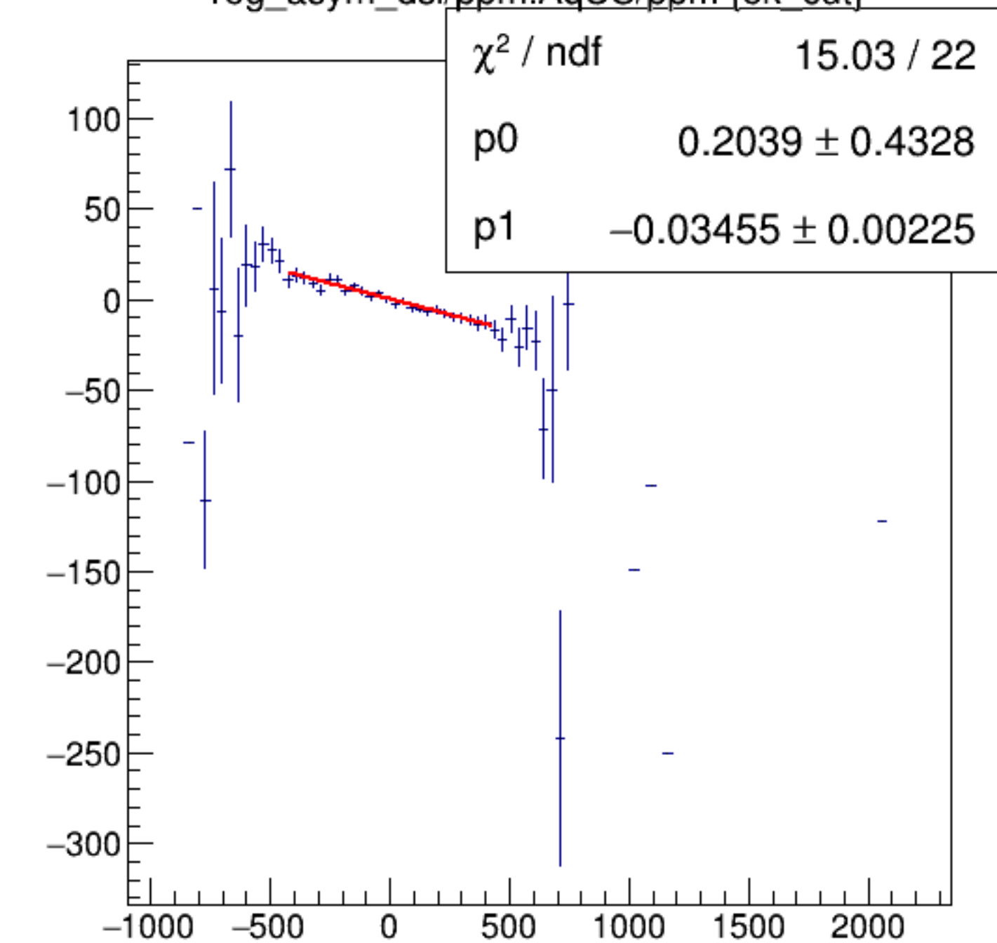
reg_asym_dsl/ppm:AqUS/ppm {ok_cut}
