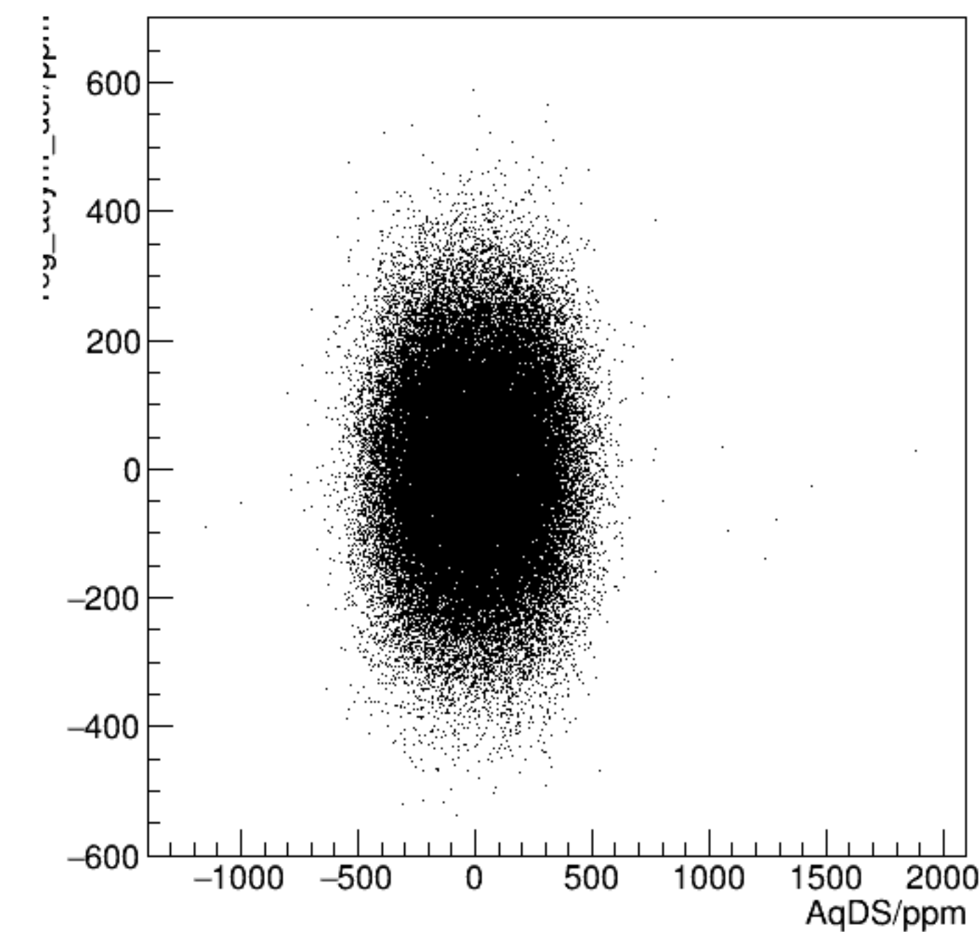
reg_asym_dsr/ppm:AqDS/ppm {ok_cut}
