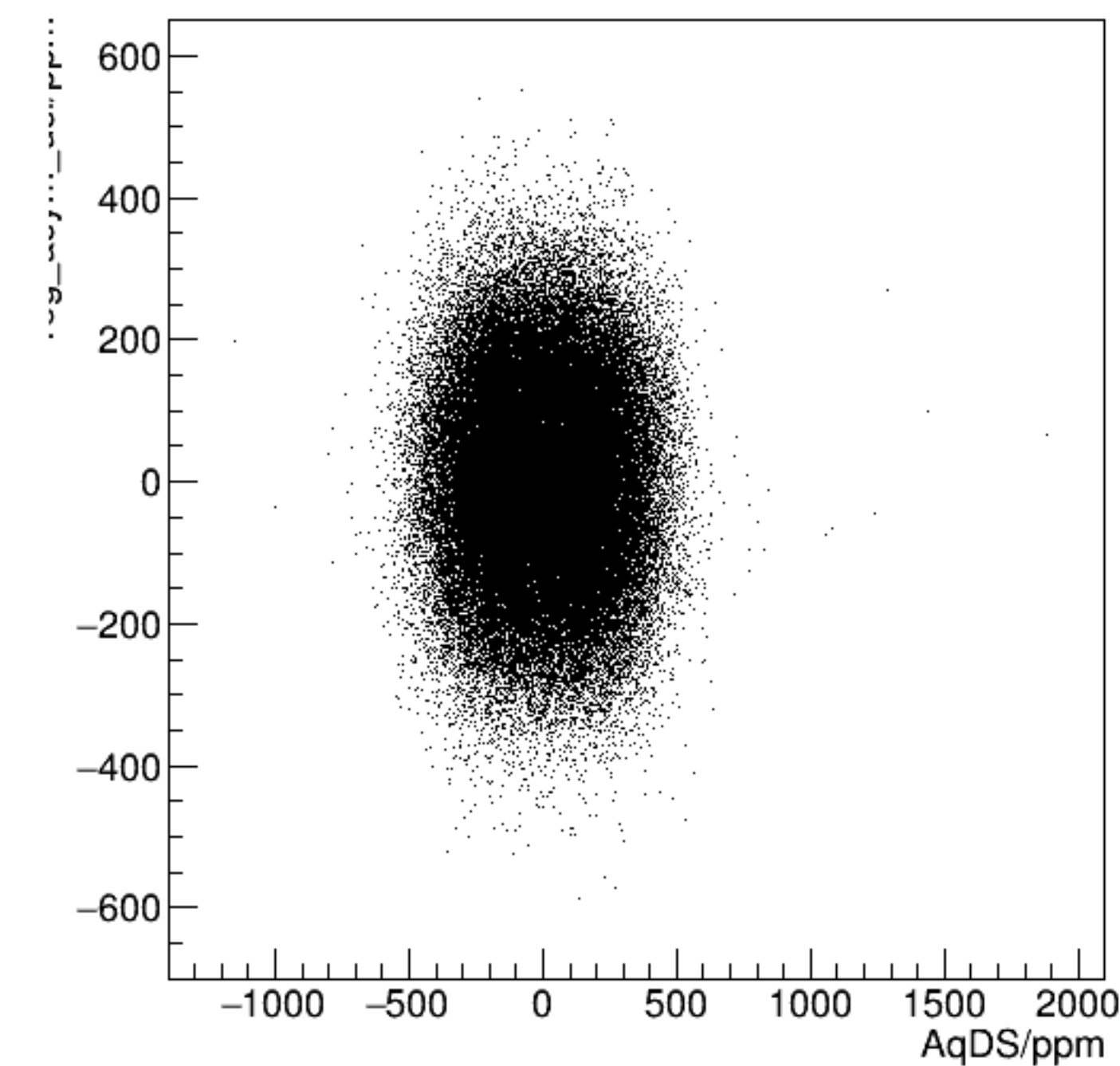
reg_asym_usl/ppm:AqDS/ppm {ok_cut}
