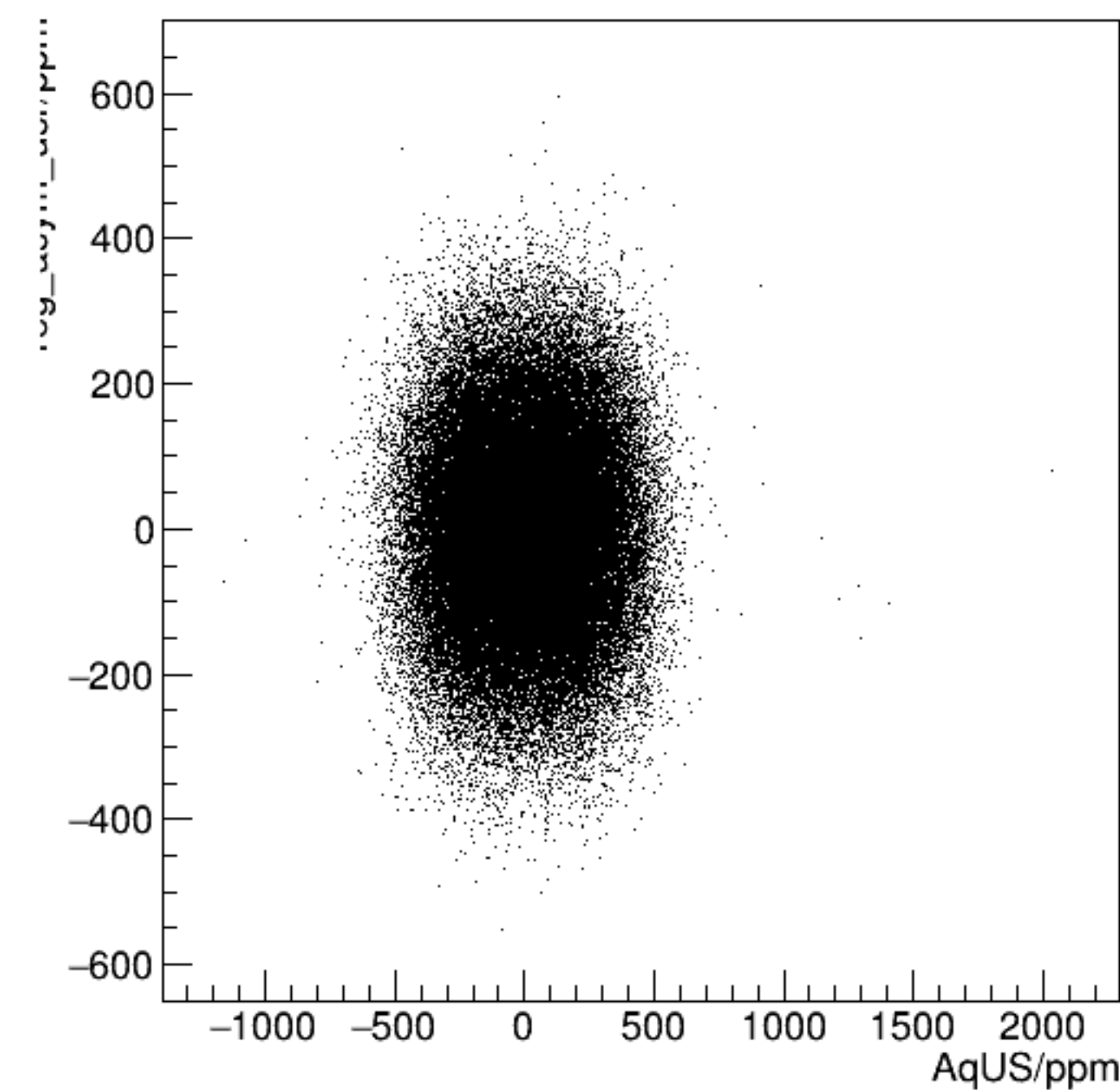
reg_asym_usr/ppm:AqUS/ppm {ok_cut}
