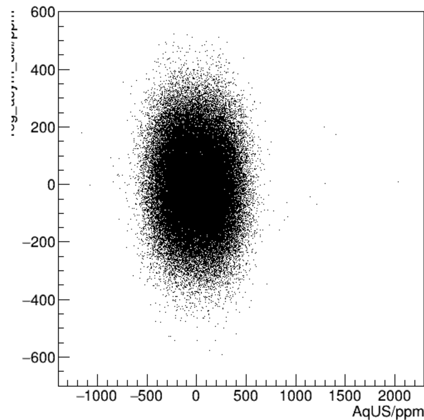
reg_asym_dsl/ppm:AqUS/ppm {ok_cut}
