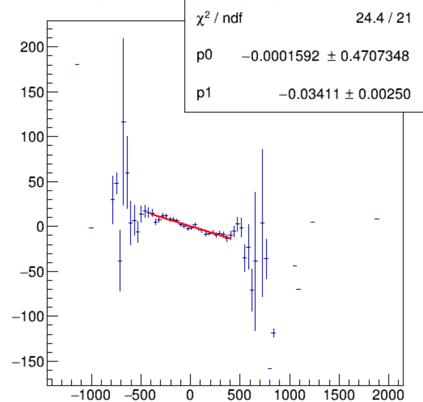
reg_asym_dsl/ppm:AqDS/ppm {ok_cut}
