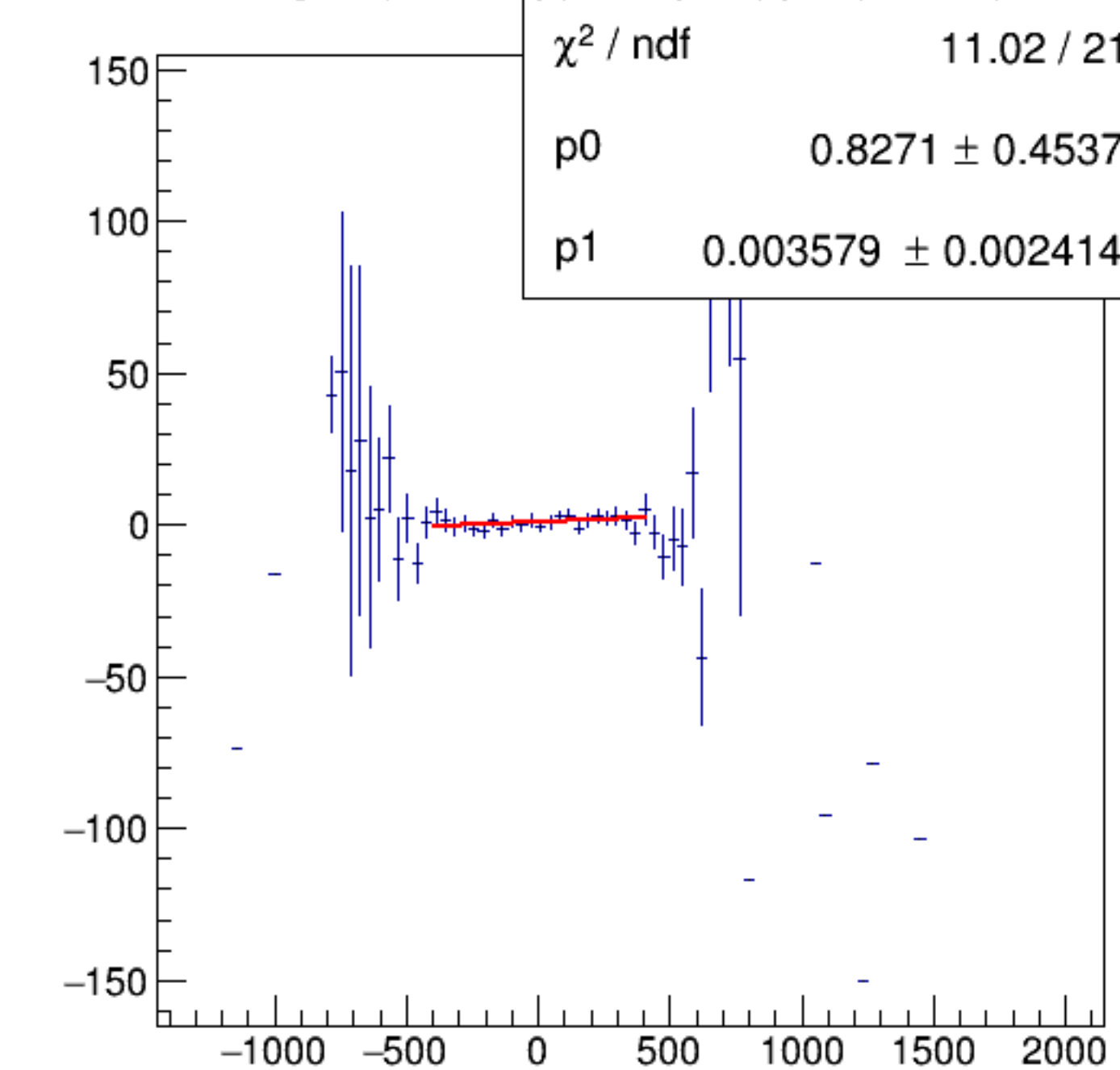
reg_asym_usr/ppm:AqDS/ppm {ok_cut}
