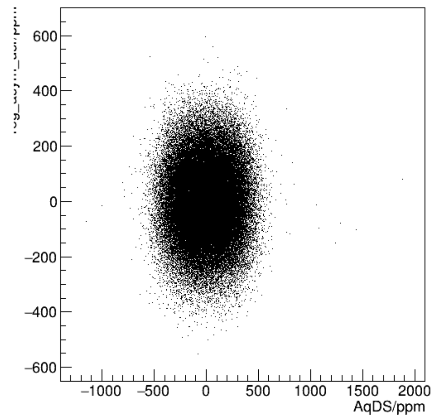
reg_asym_usr/ppm:AqDS/ppm {ok_cut}
