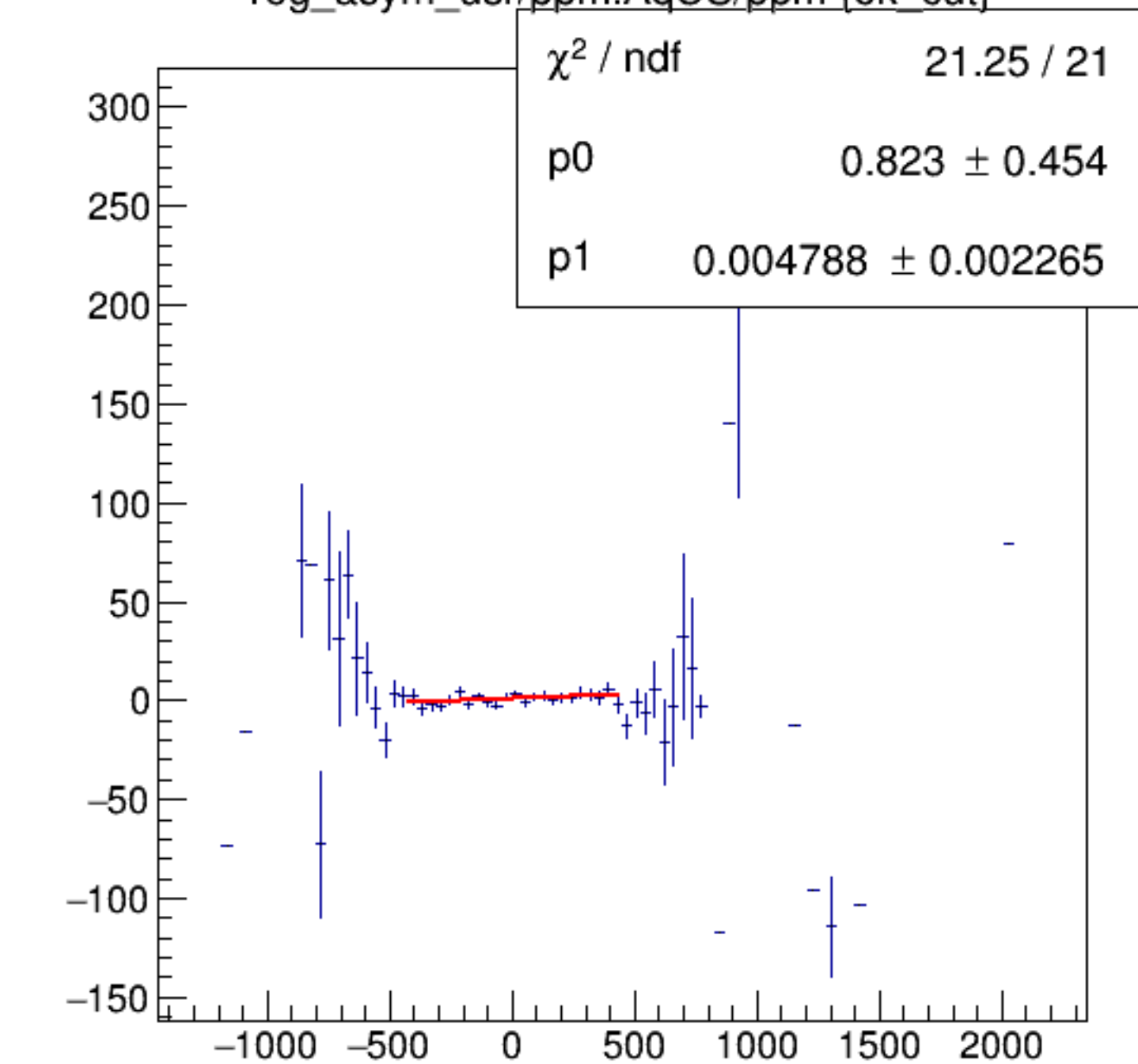
reg_asym_usr/ppm:AqUS/ppm {ok_cut}
