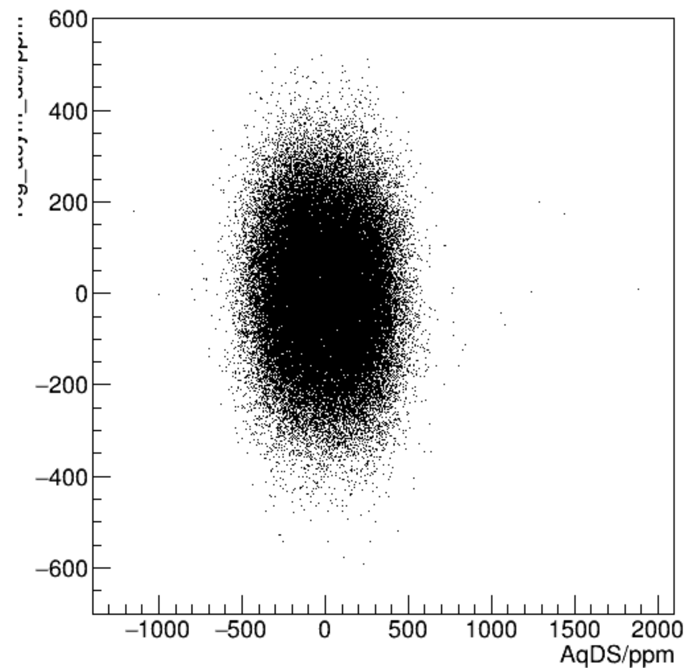
reg_asym_dsl/ppm:AqDS/ppm {ok_cut}
