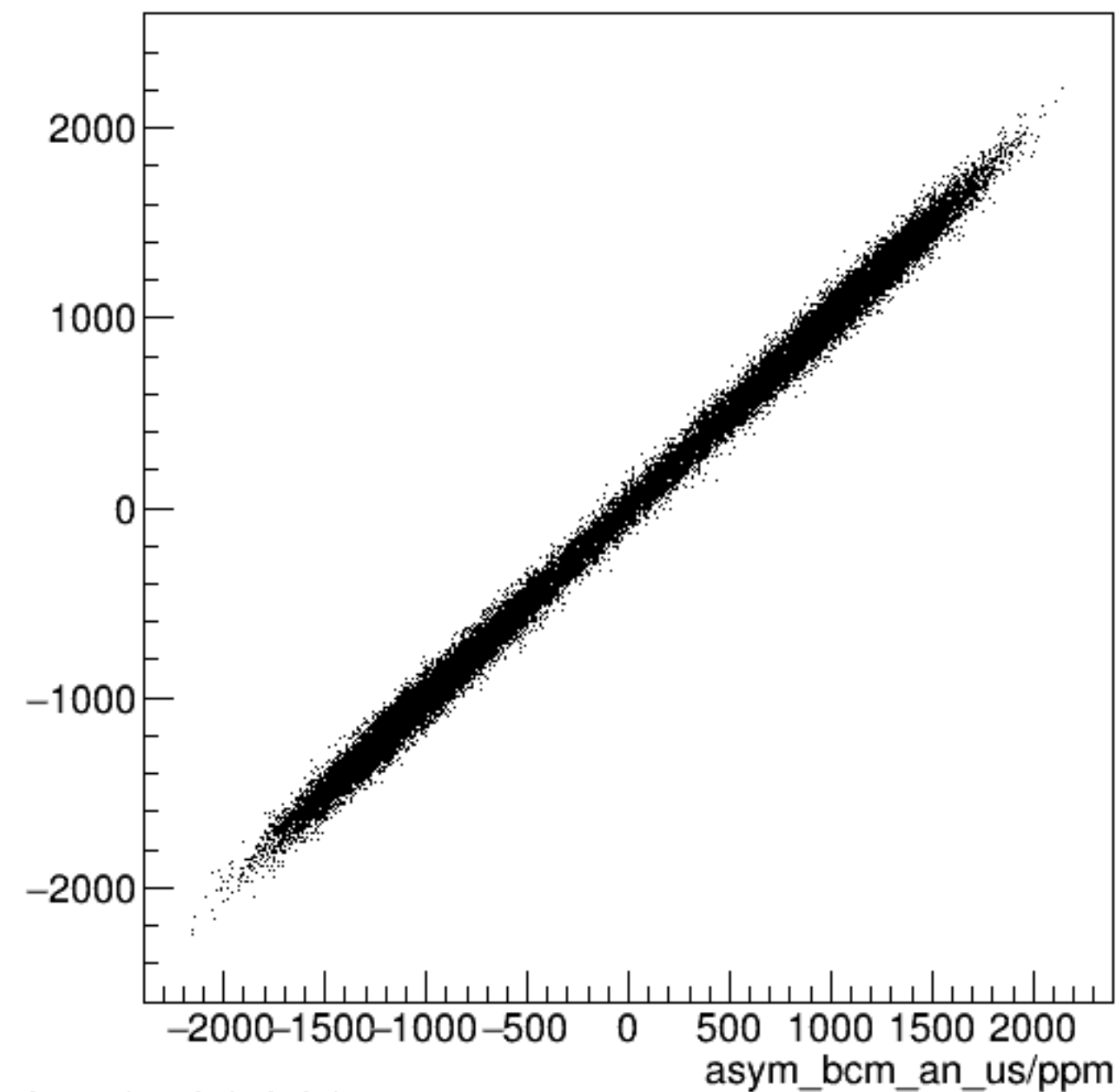
run3785_000_asym_bcm_dg_ds_vs_asym_bcm_an_us_pr.png
