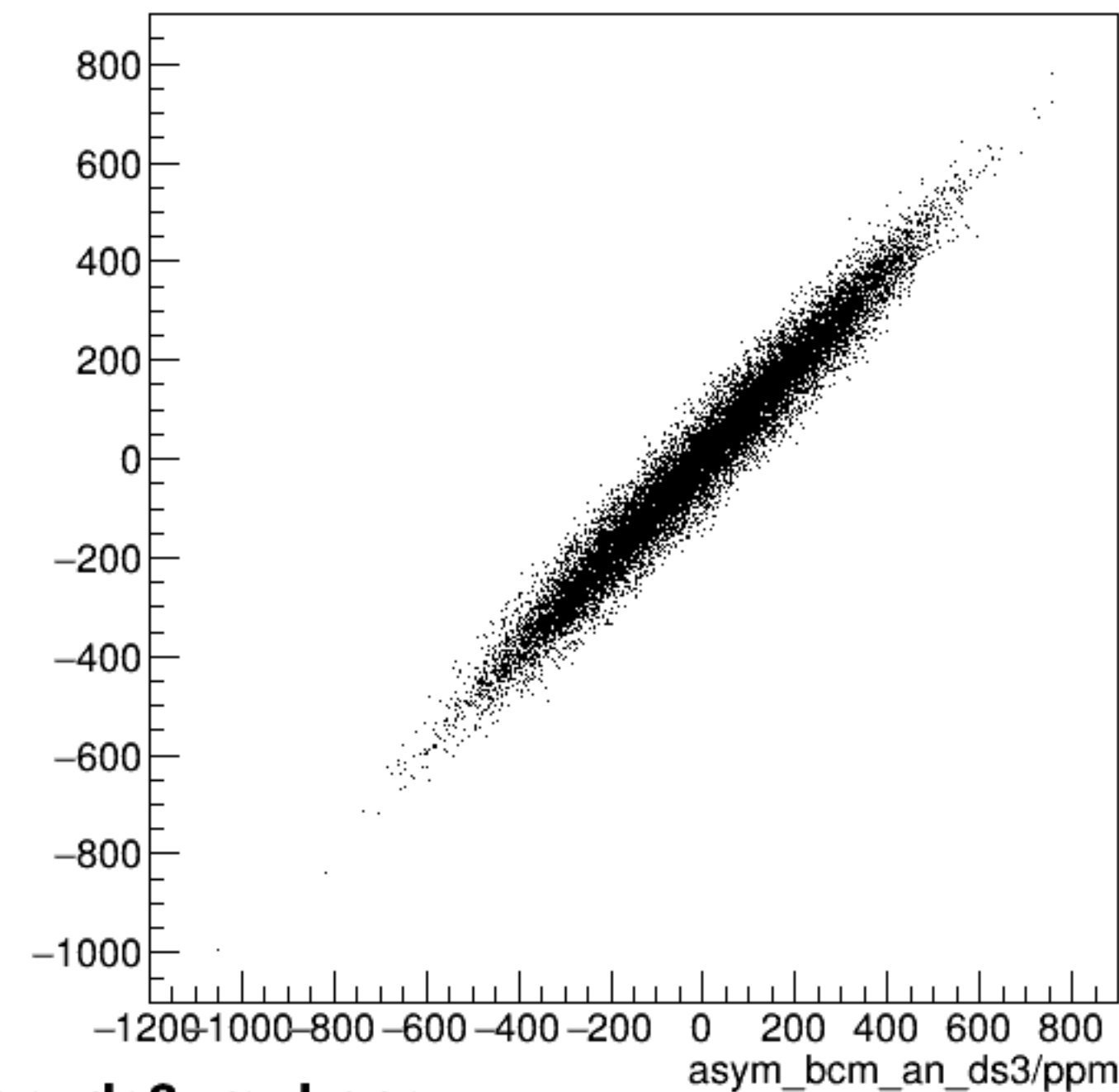
run3785_000_asym_bcm_an_us_vs_asym_bcm_an_ds3_mul.png
