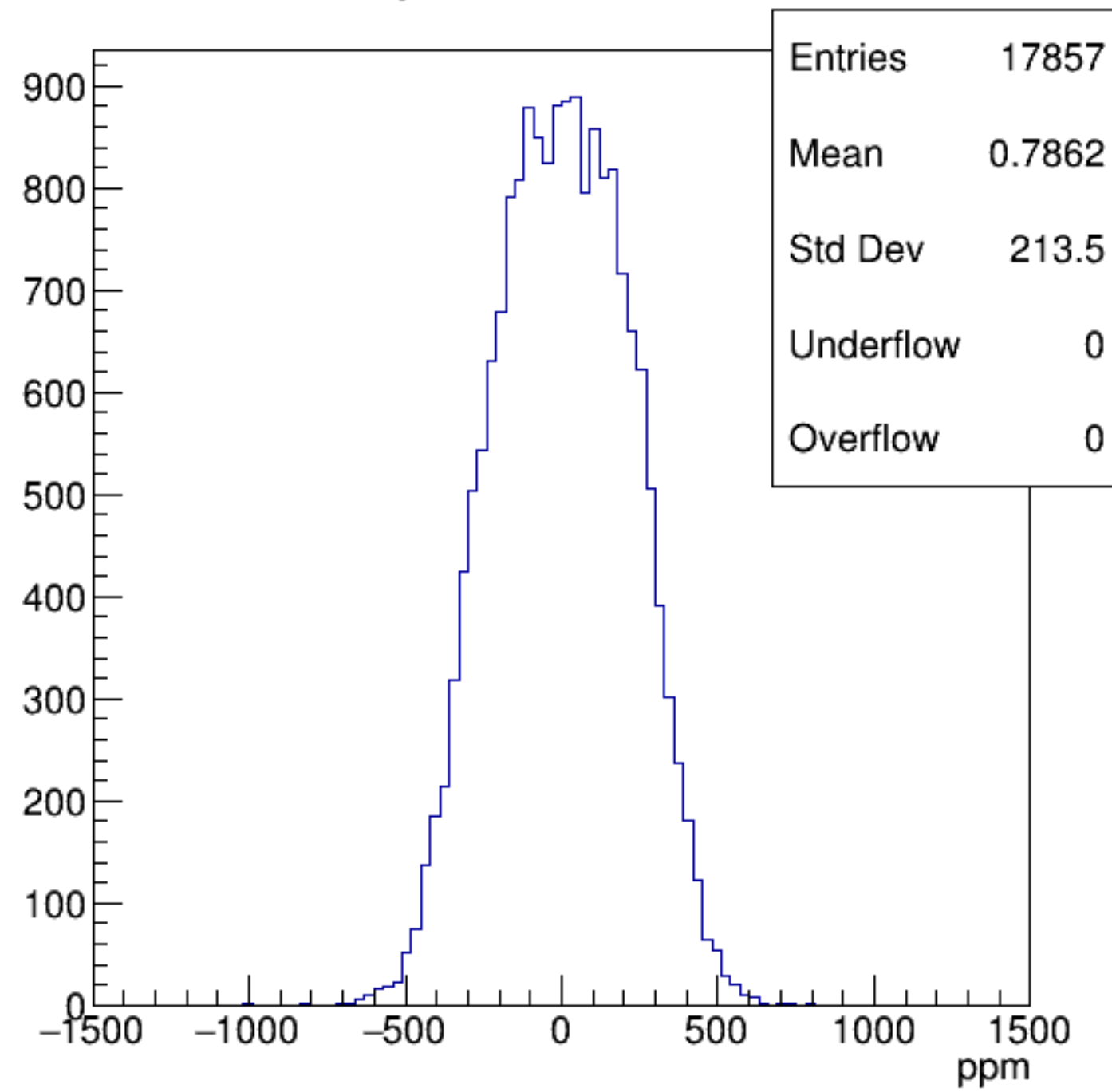
asym_bcm_an_us
