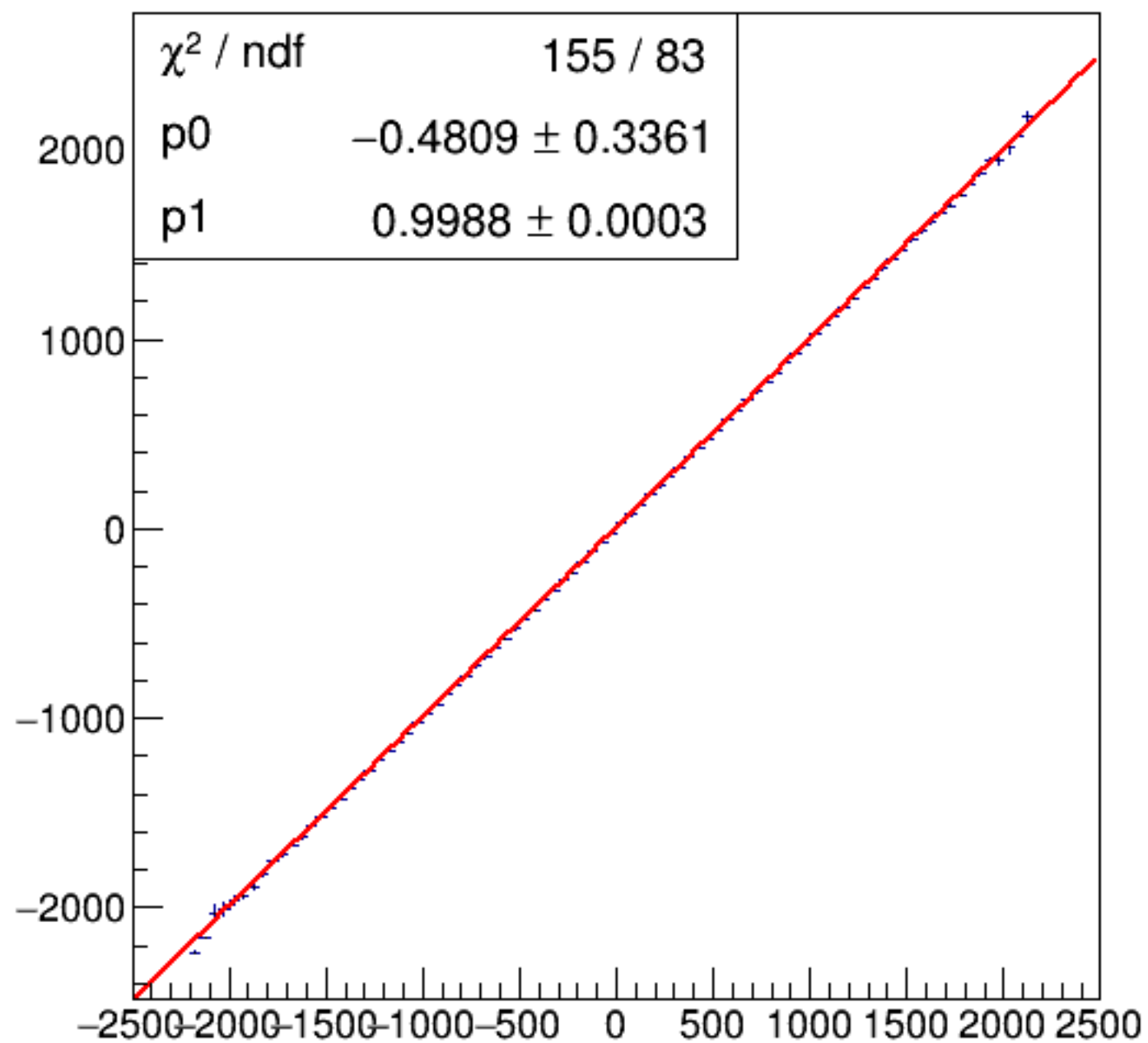
run3785_000_asym_bcm_dg_ds_vs_asym_bcm_an_us_pr.png
