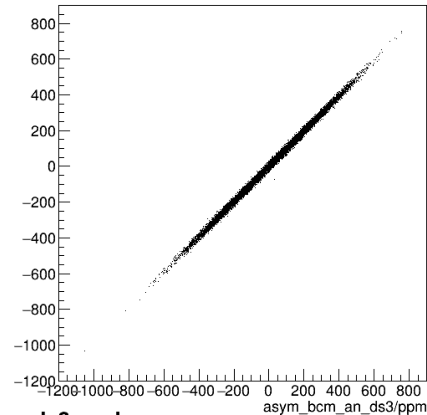
run3785_000_asym_bcm_an_ds_vs_asym_bcm_an_ds3_mul.png
