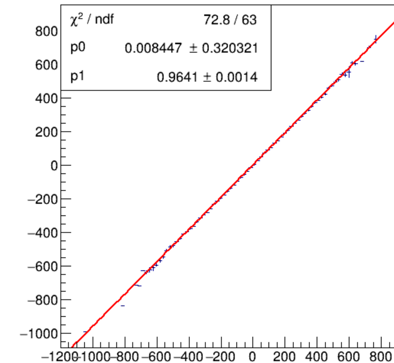
run3785_000_asym_bcm_an_us_vs_asym_bcm_an_ds3_mul.png
