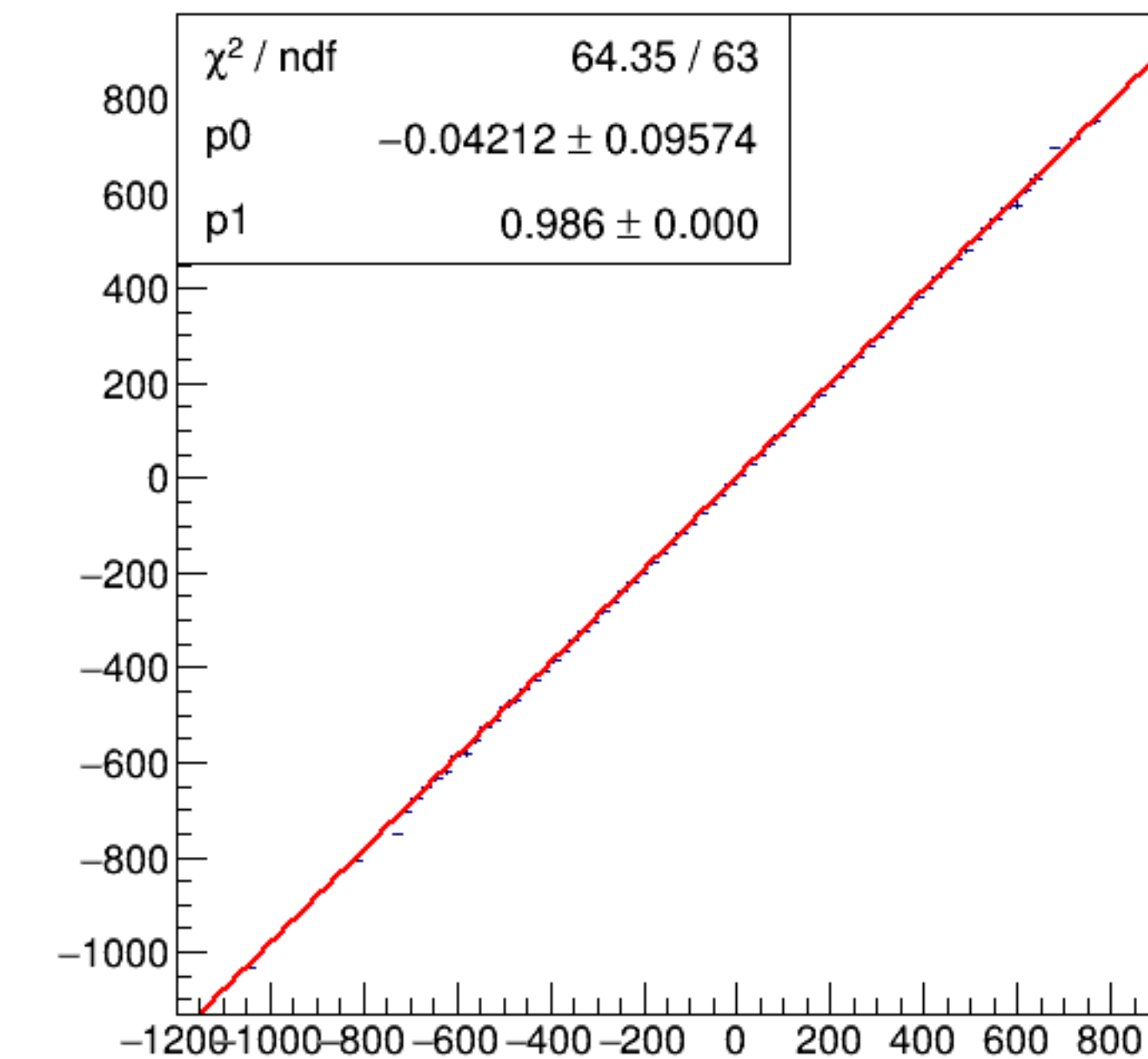
run3785_000_asym_bcm_an_ds_vs_asym_bcm_an_ds3_mul.png
