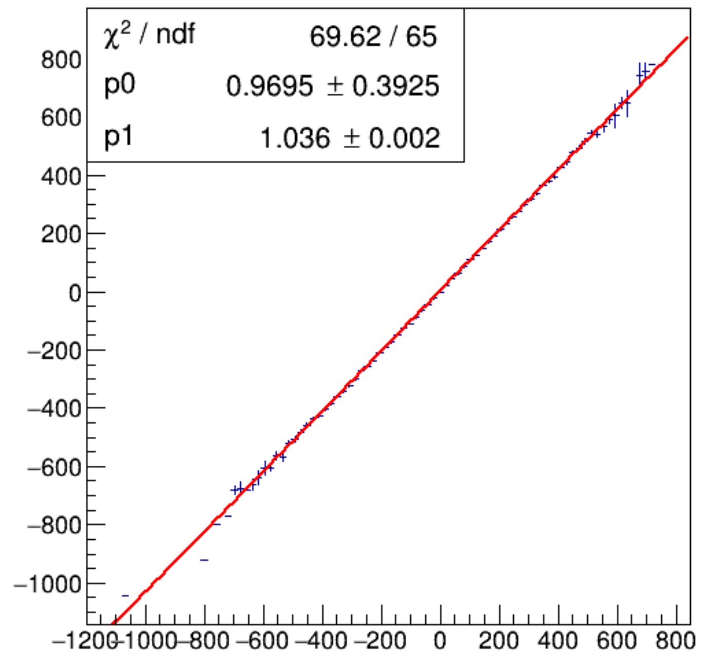
run3785_000_asym_bcm_dg_us_vs_asym_bcm_dg_ds_mul.png
