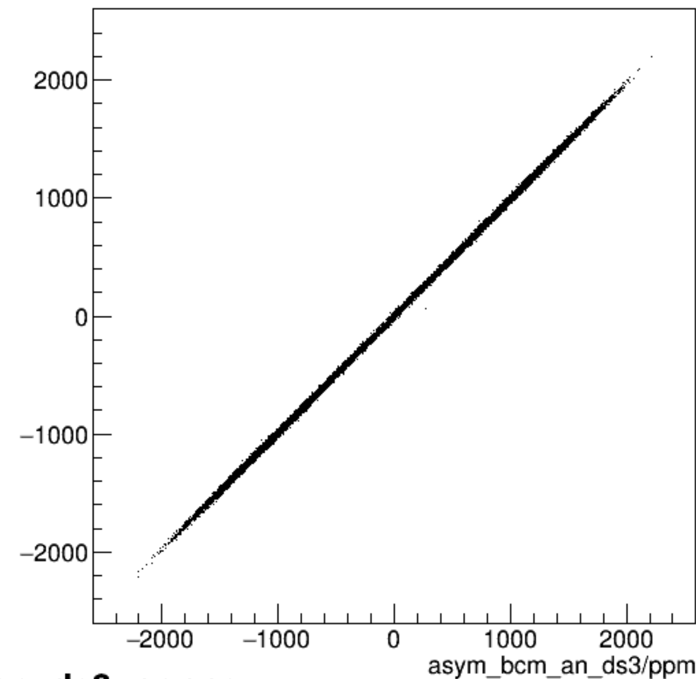
run3785_000_asym_bcm_an_ds_vs_asym_bcm_an_ds3_pr.png
