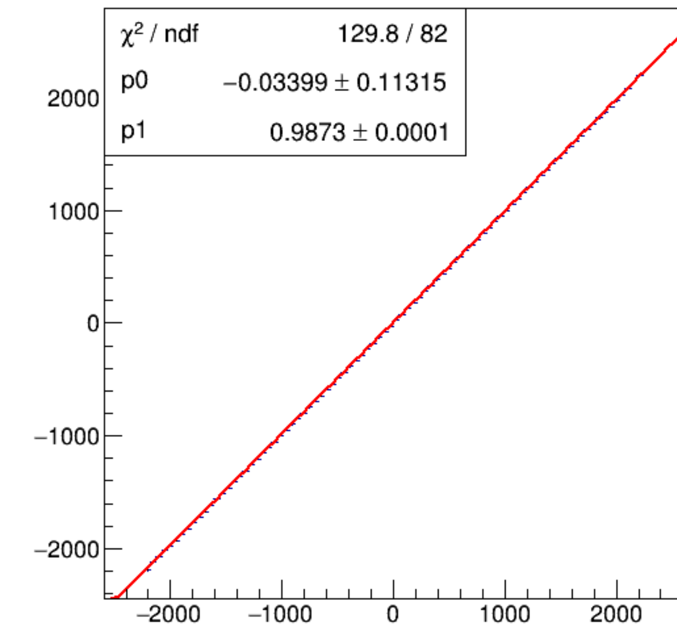
run3785_000_asym_bcm_an_ds_vs_asym_bcm_an_ds3_pr.png
