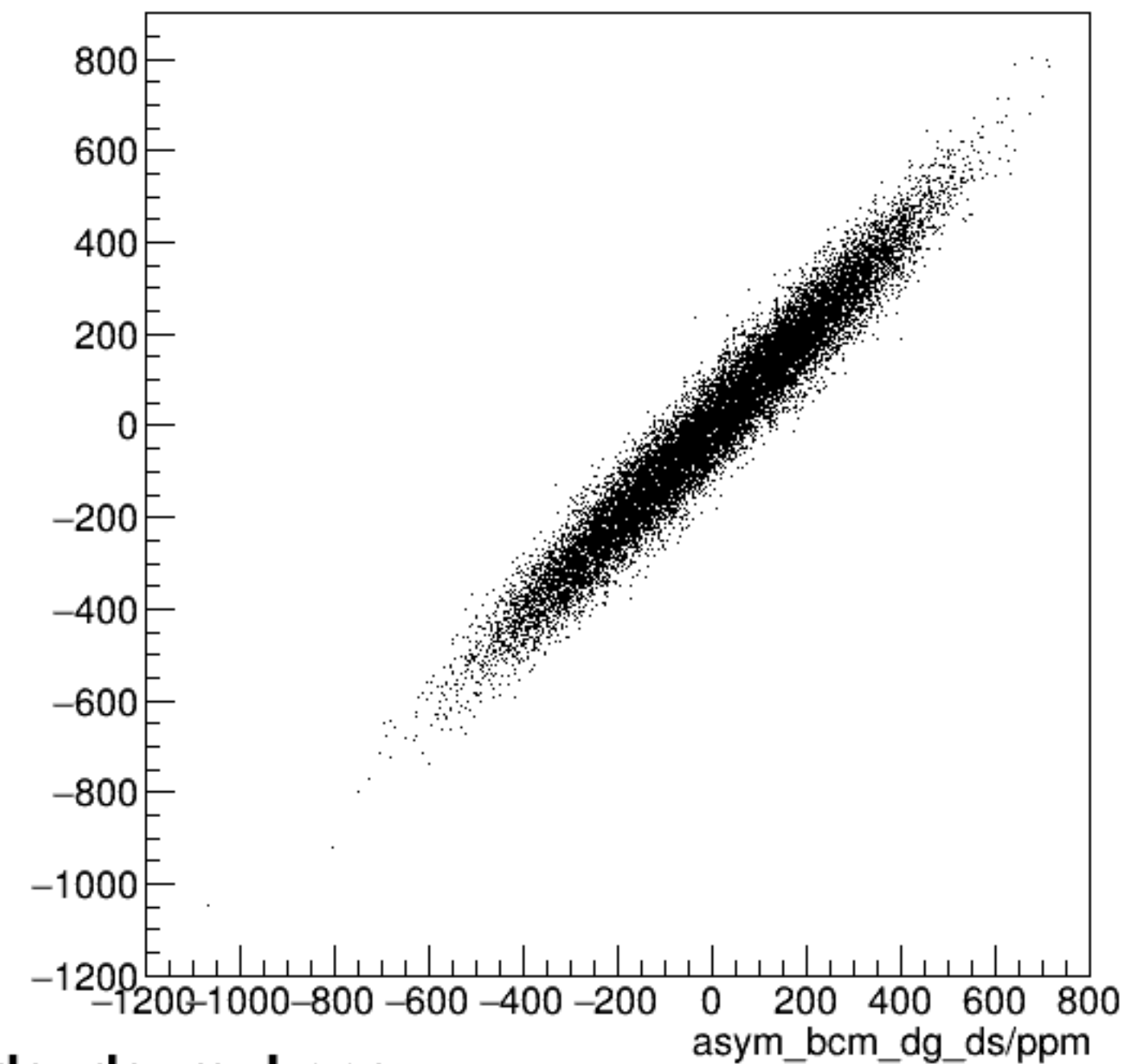
run3785_000_asym_bcm_dg_us_vs_asym_bcm_dg_ds_mul.png
