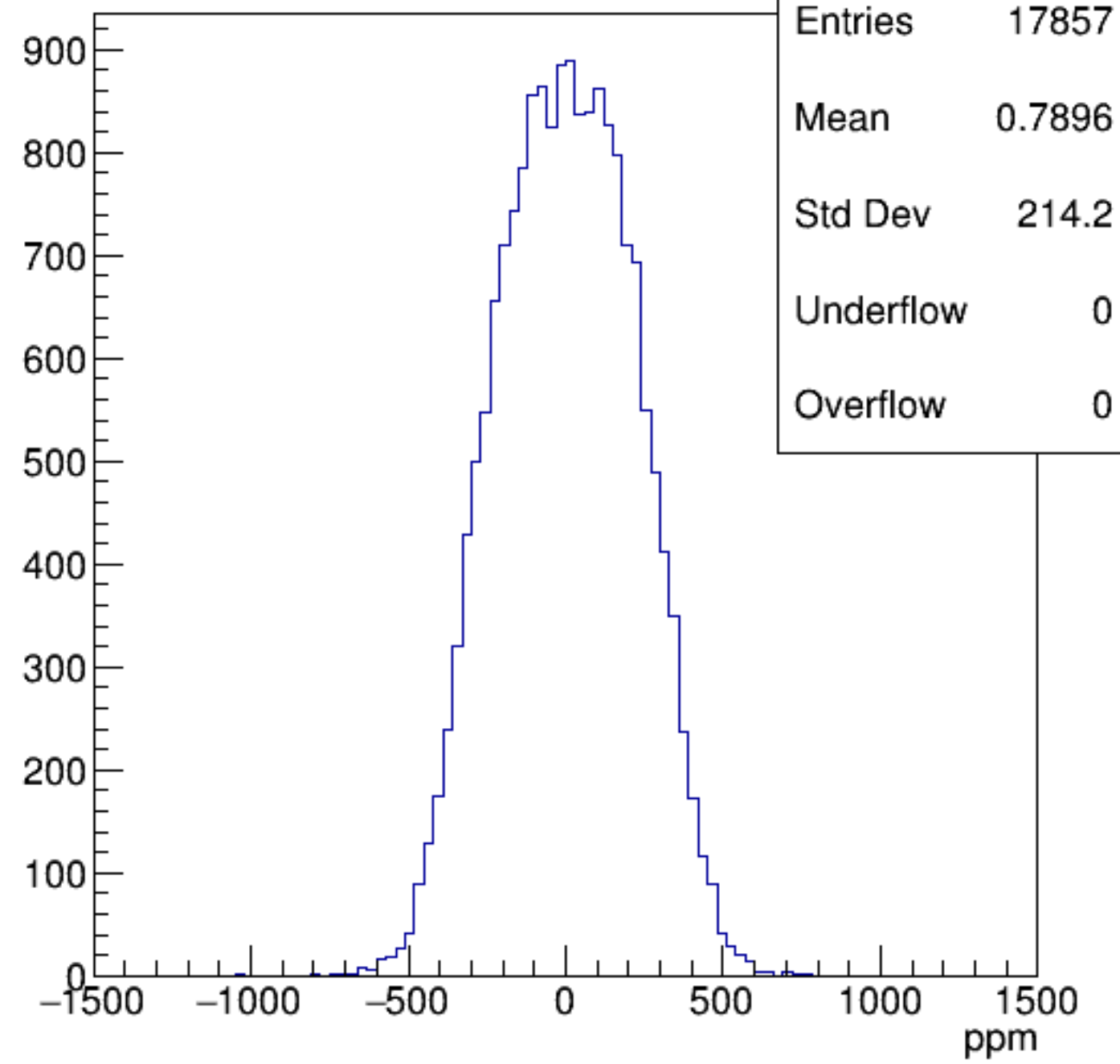
asym_bcm_an_ds
