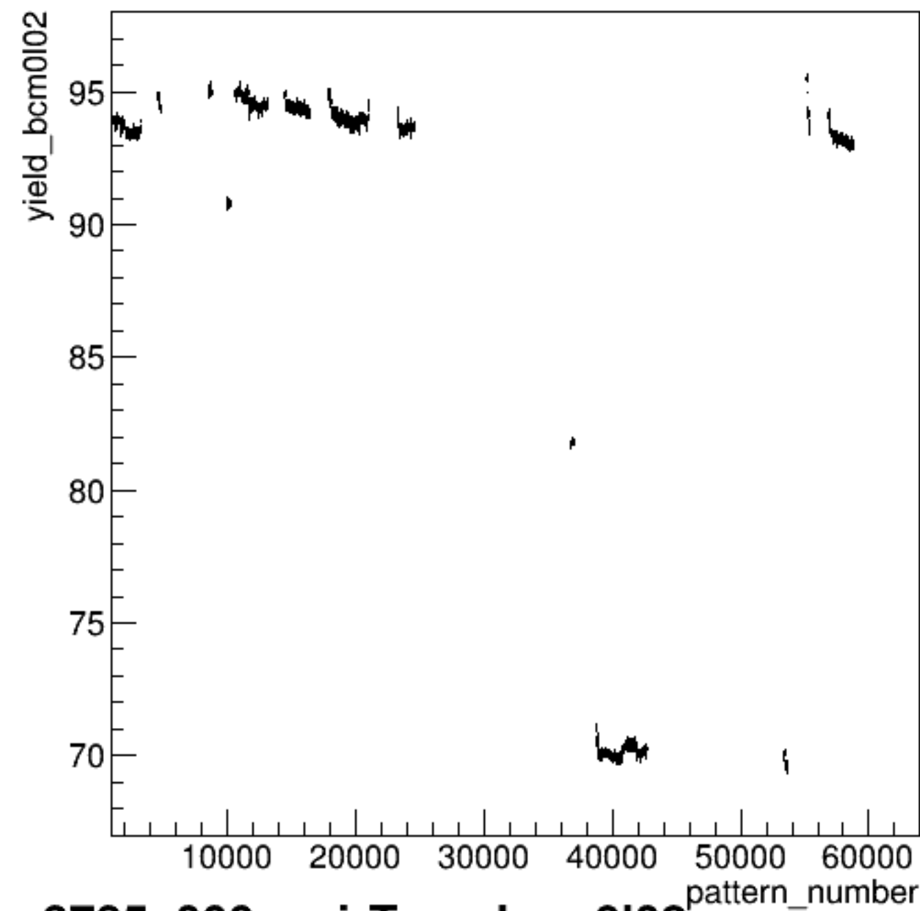
yield_bcm0l02:pattern_number {ErrorFlag==0}
