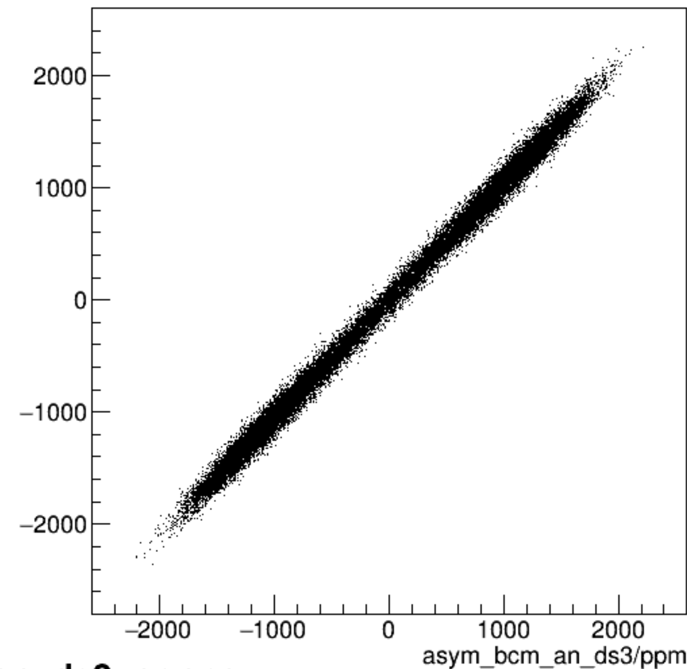
run3785_000_asym_bcm_dg_us_vs_asym_bcm_an_ds3_pr.png
