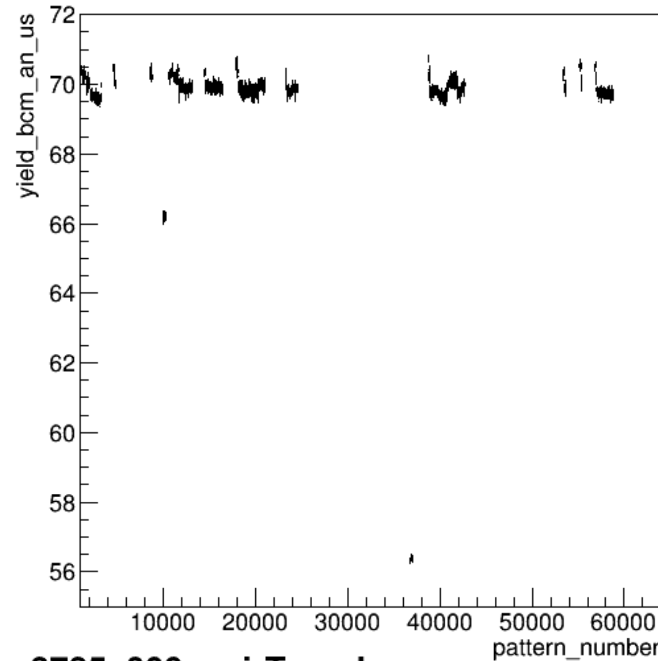
yield_bcm_an_us:pattern_number {ErrorFlag==0}
