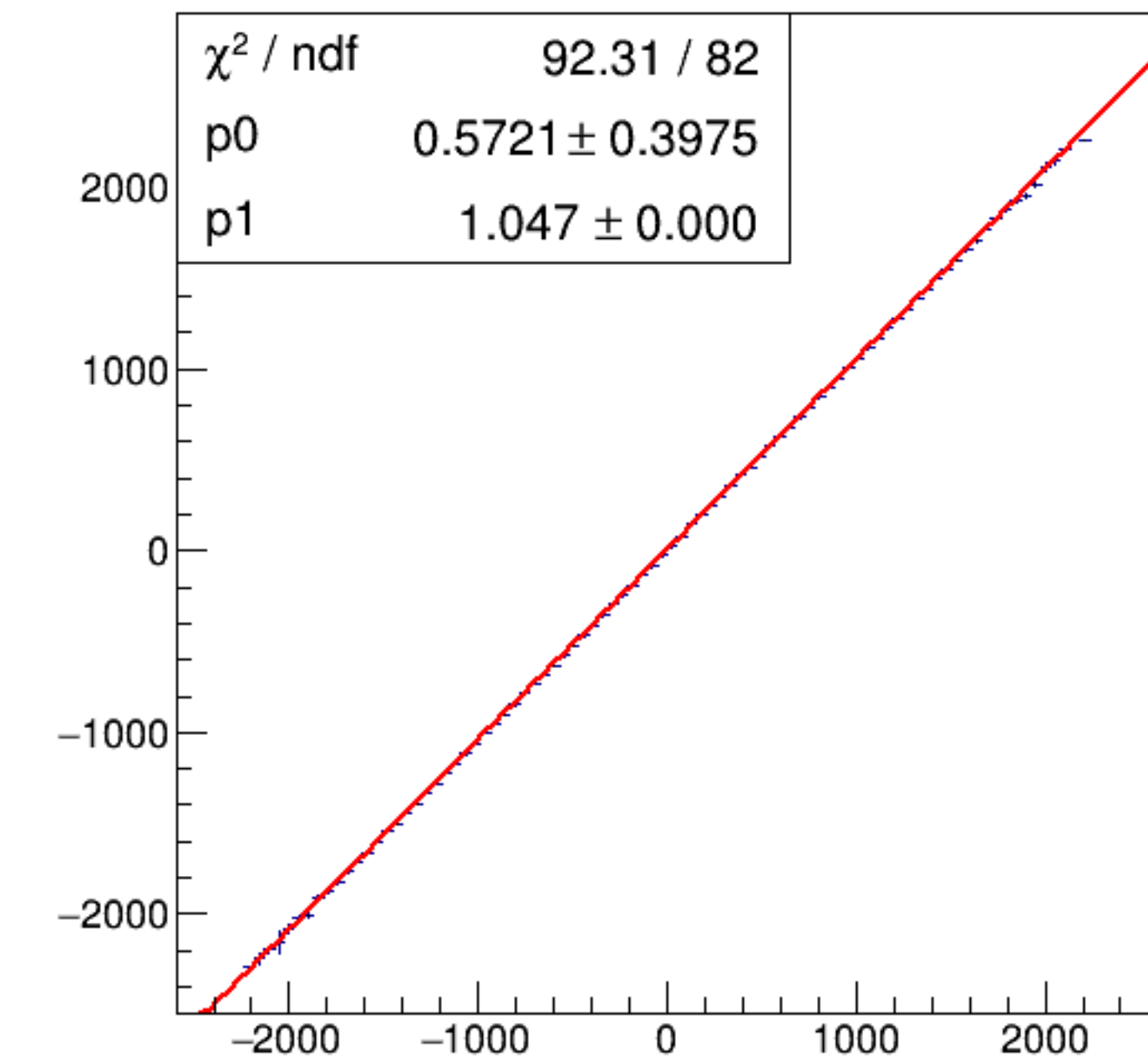
run3785_000_asym_bcm_dg_us_vs_asym_bcm_an_ds3_pr.png
