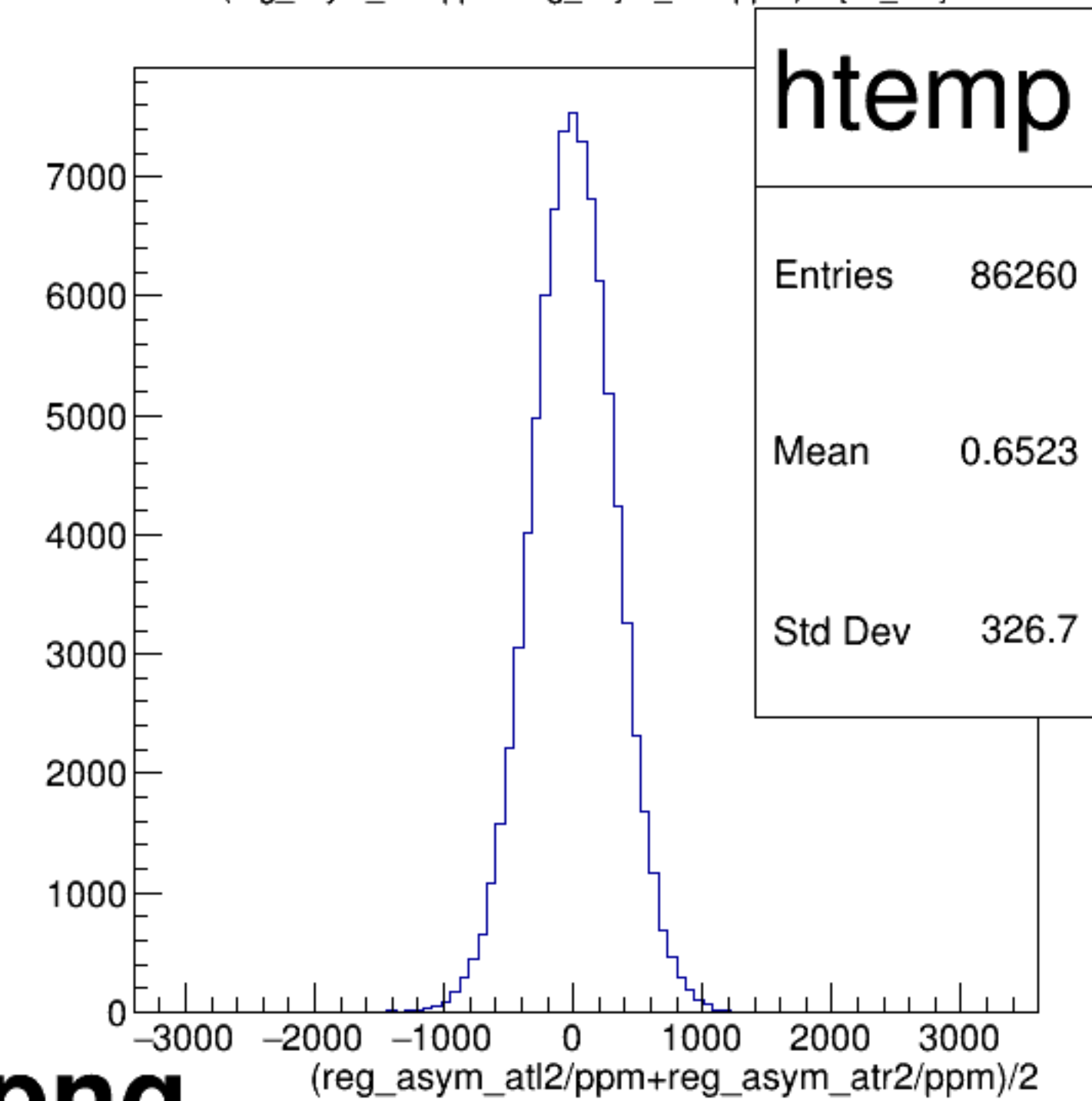
(reg_asym_atl2/ppm+reg_asym_atr2/ppm)/2 {ok_cut}
