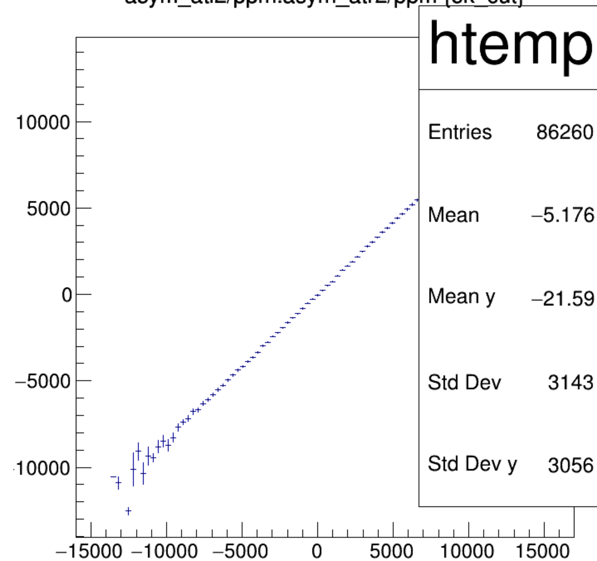
asym_atl2/ppm:asym_atr2/ppm {ok_cut}
