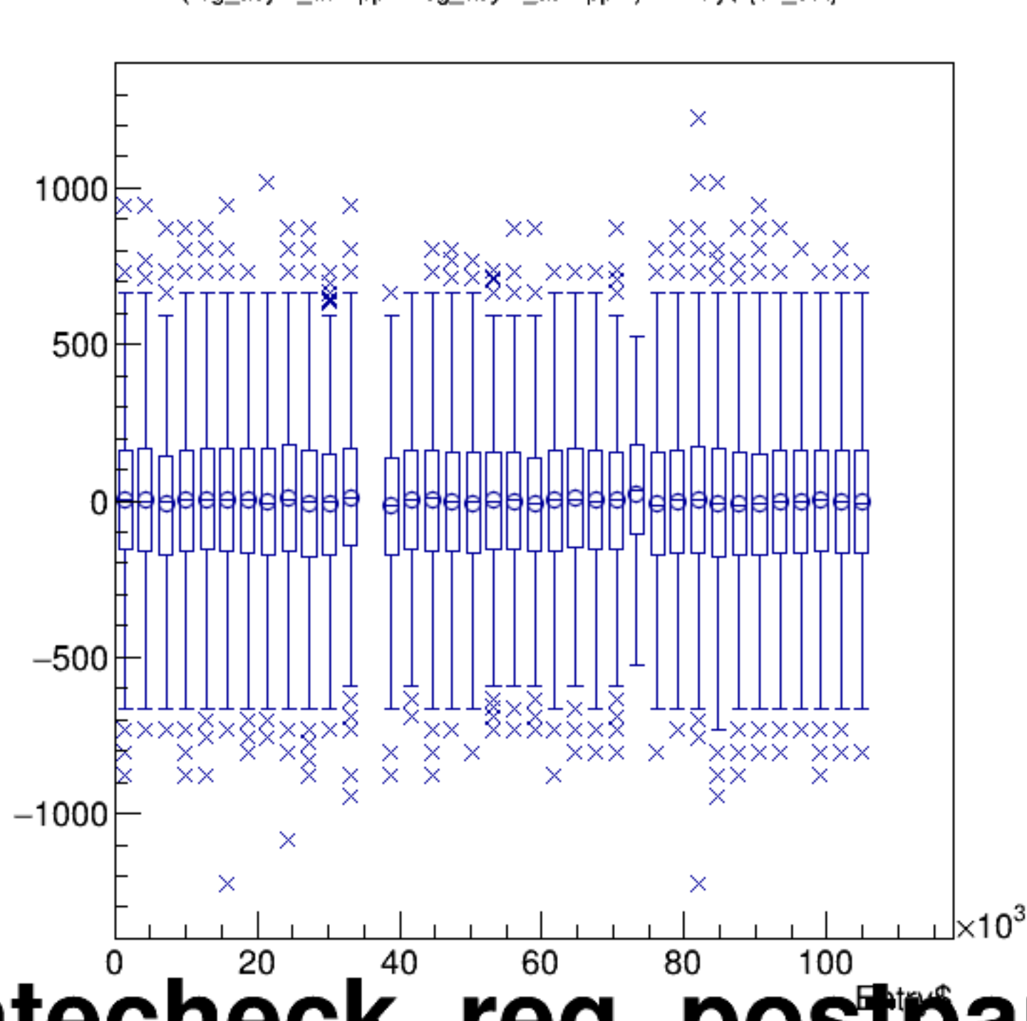
(reg_asym_atl2/ppm-reg_asym_atr2/ppm)/2:Entry$ {ok_cut}
