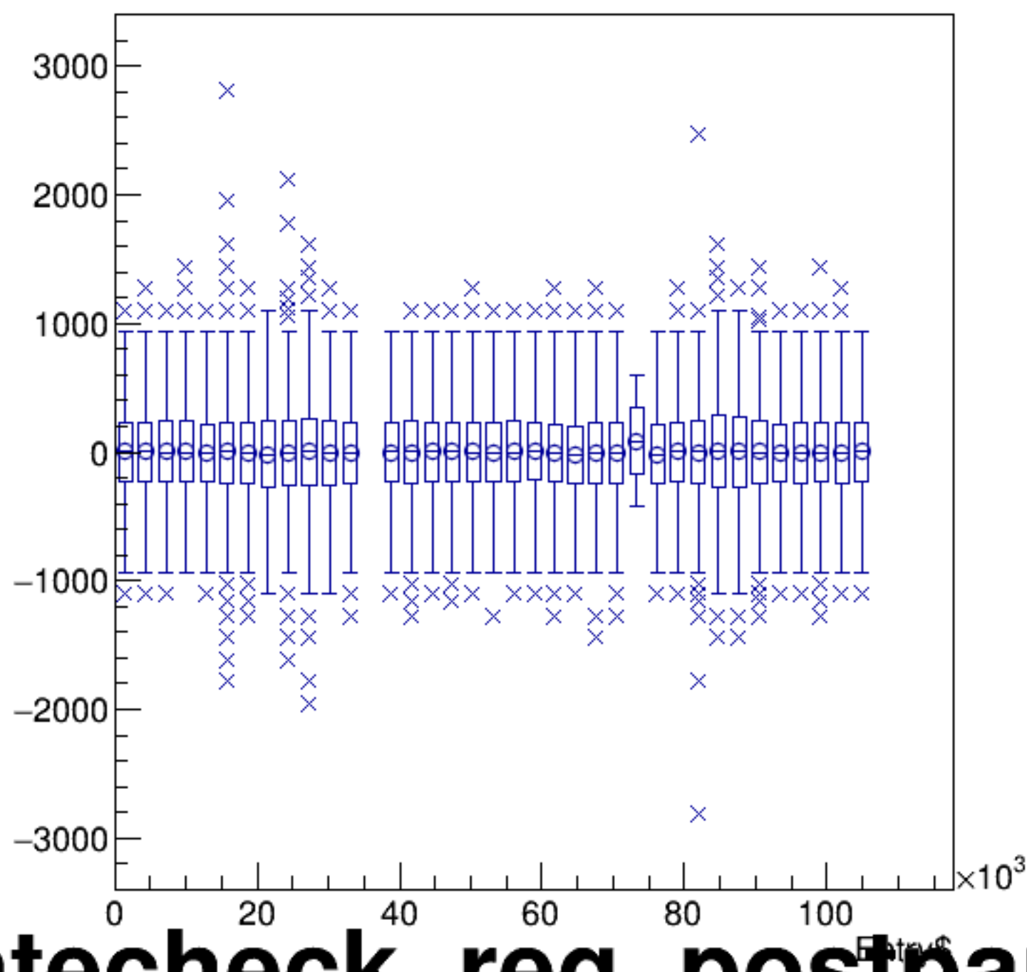
(reg_asym_atl1/ppm-reg_asym_atr1/ppm)/2:Entry$ {ok_cut}
