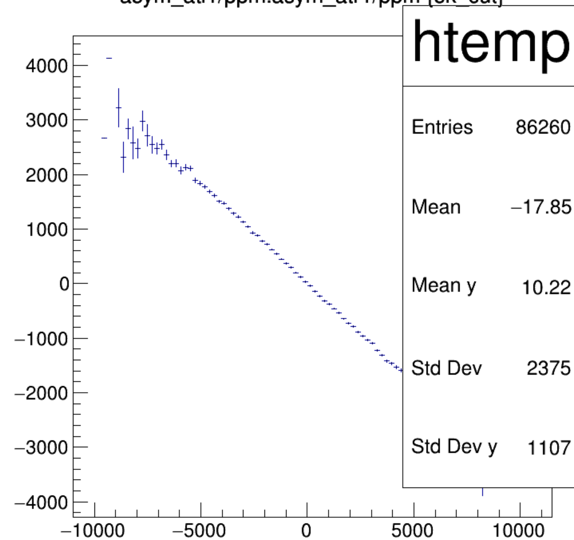
asym_atl1/ppm:asym_atr1/ppm {ok_cut}
