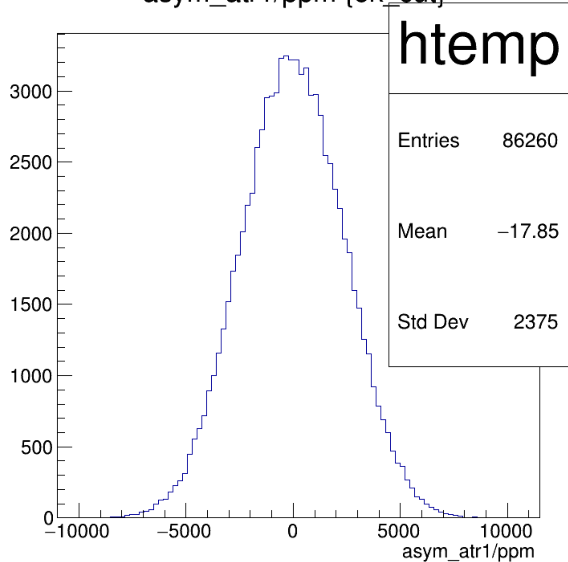
asym_atr1/ppm {ok_cut}
