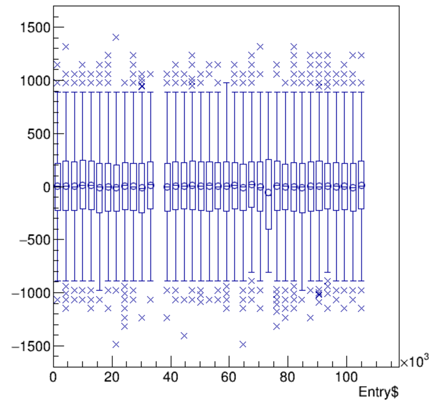
(reg_asym_atl1/ppm+reg_asym_atr1/ppm)/2:Entry$ {ok_cut}
