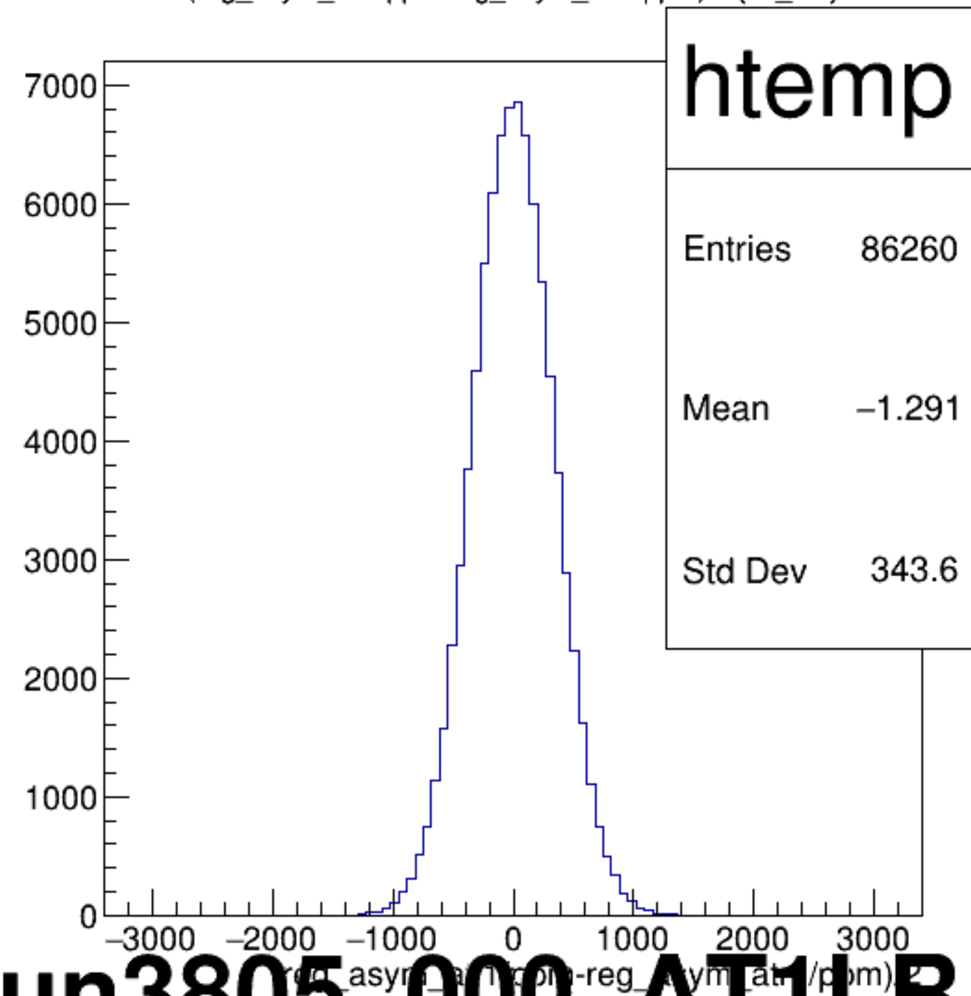
(reg_asym_atl1/ppm-reg_asym_atr1/ppm)/2 {ok_cut}
