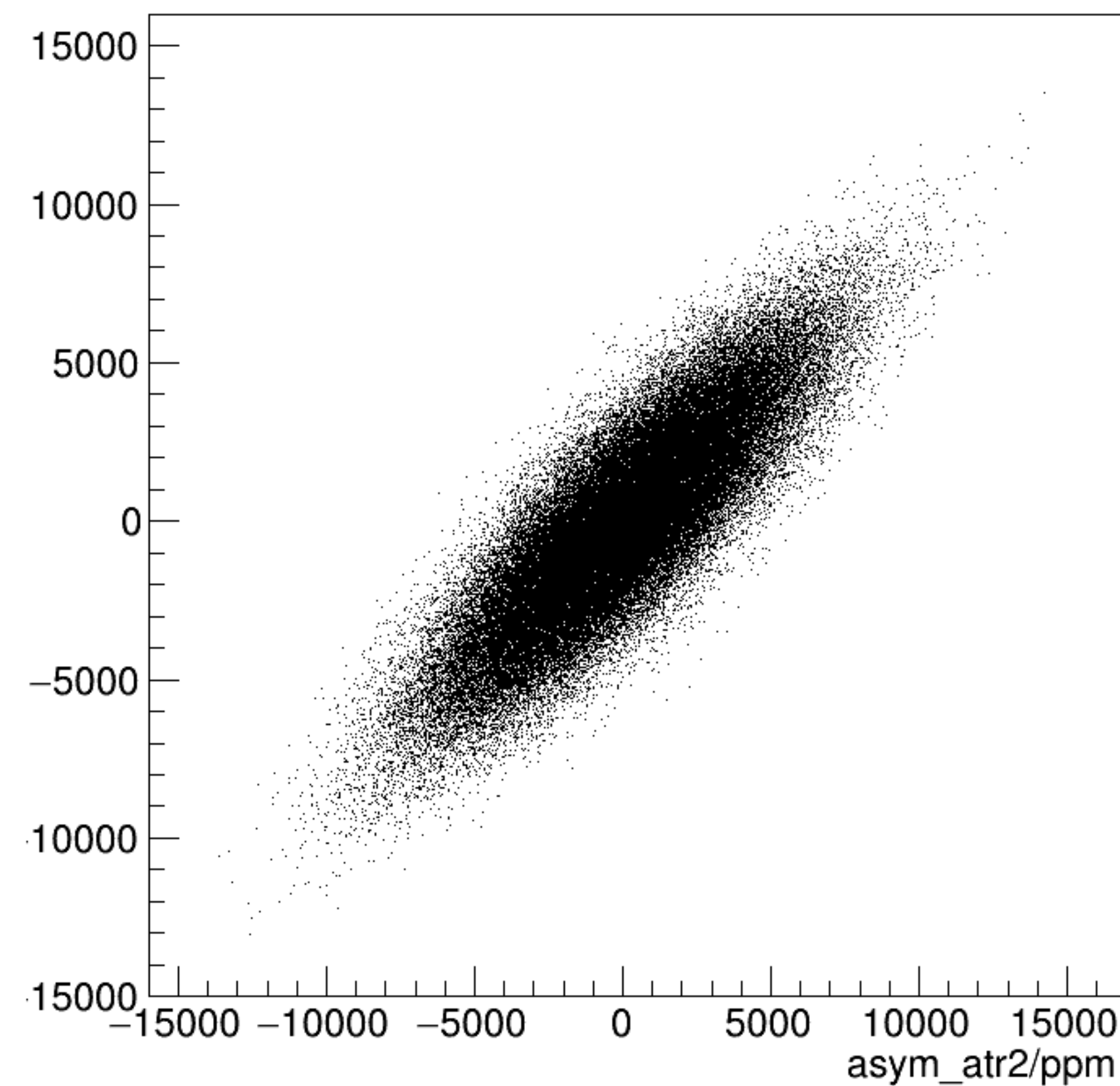
asym_atl2/ppm:asym_atr2/ppm {ok_cut}
