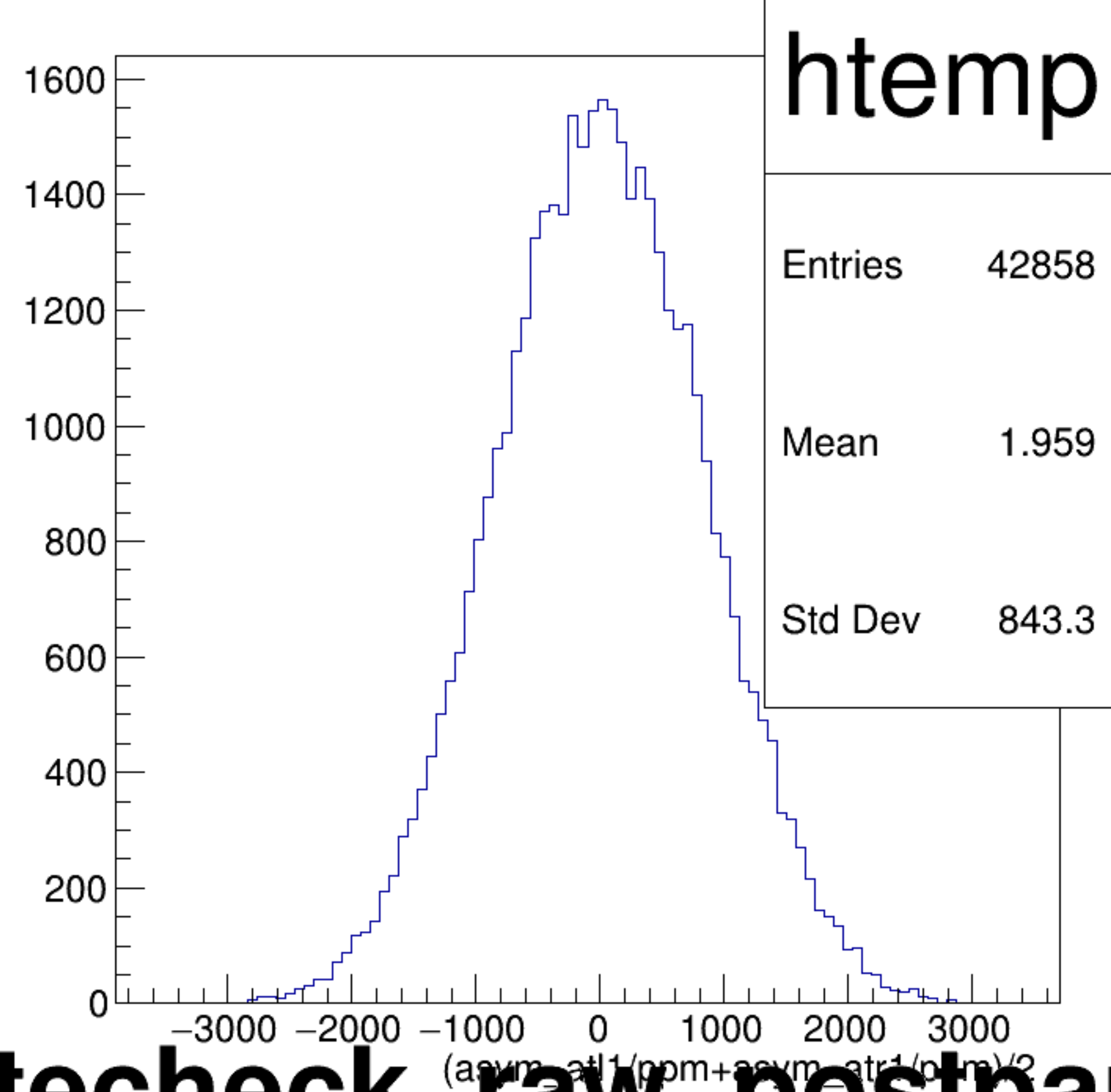
(asym_atl1/ppm+asym_atr1/ppm)/2 {ok_cut}
