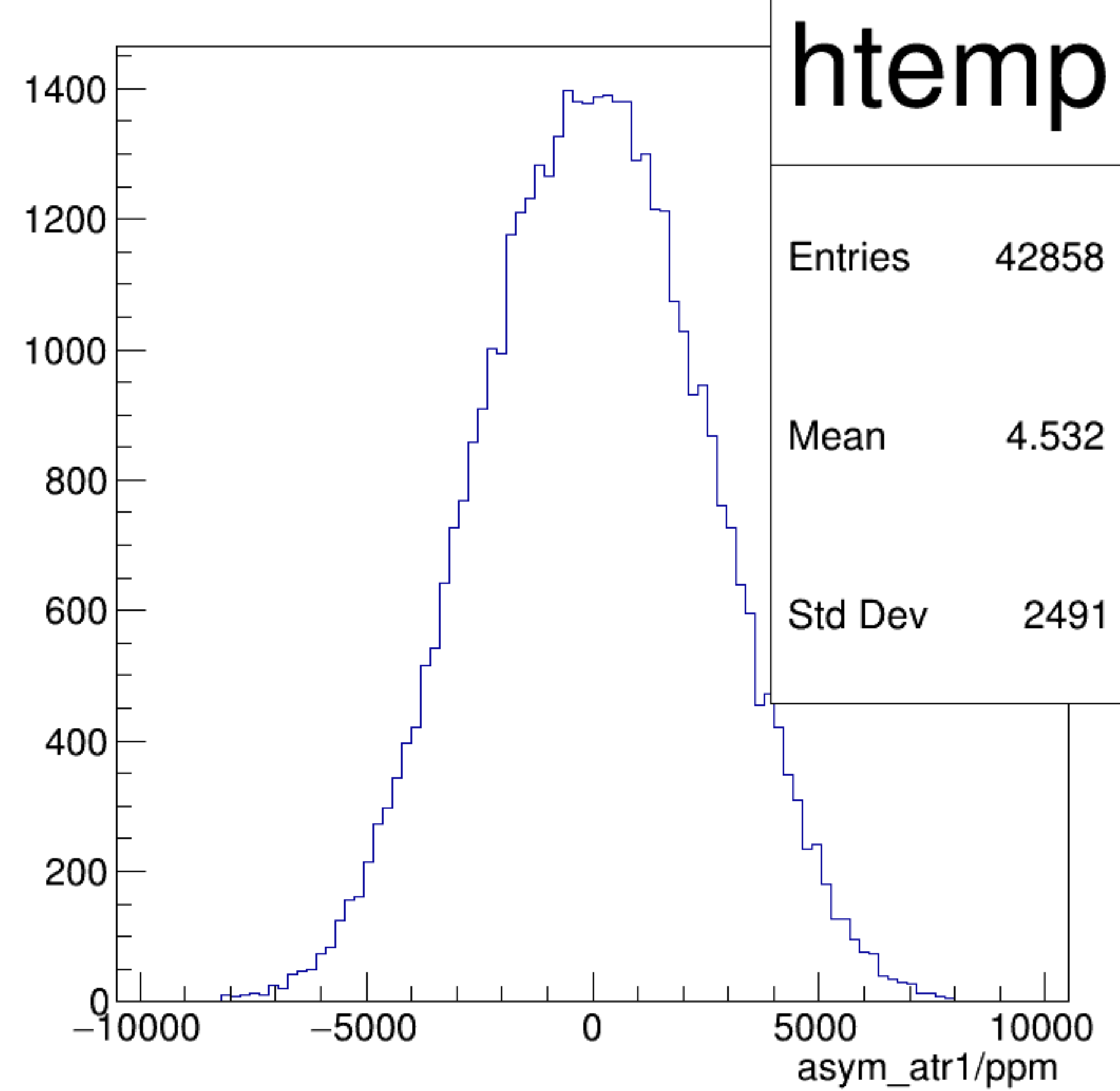
asym_atr1/ppm {ok_cut}
