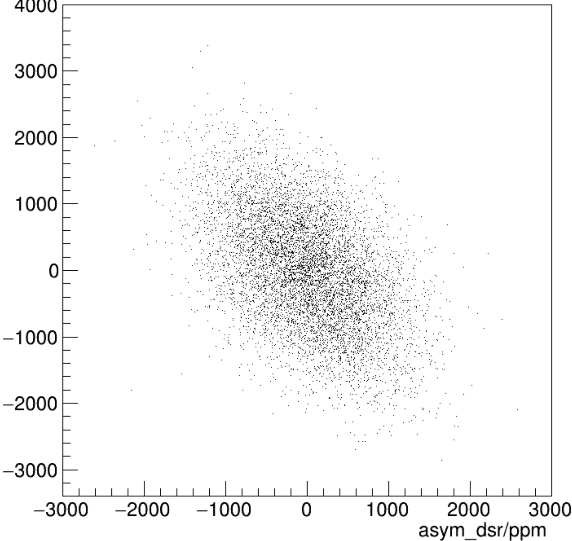
asym_dsl/ppm:asym_dsr/ppm {ok_cut}
