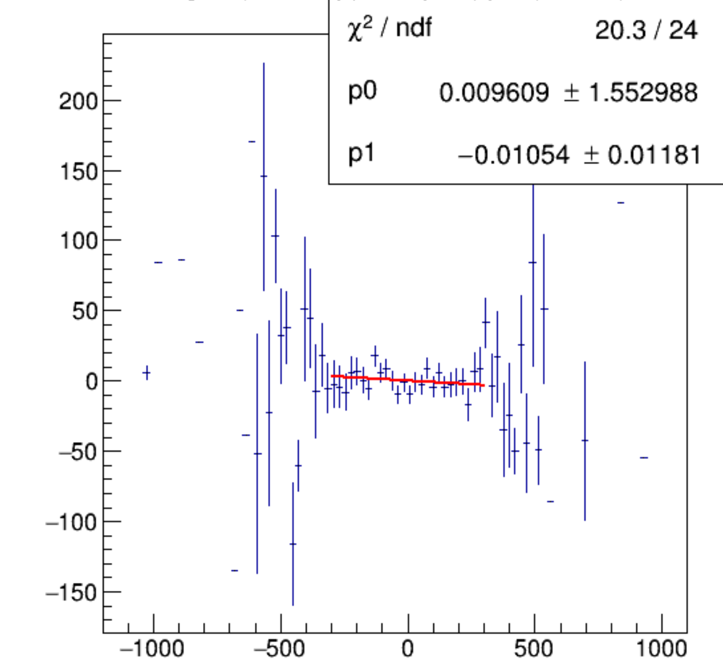
reg_asym_dsr/ppm:AqDS/ppm {ok_cut}
