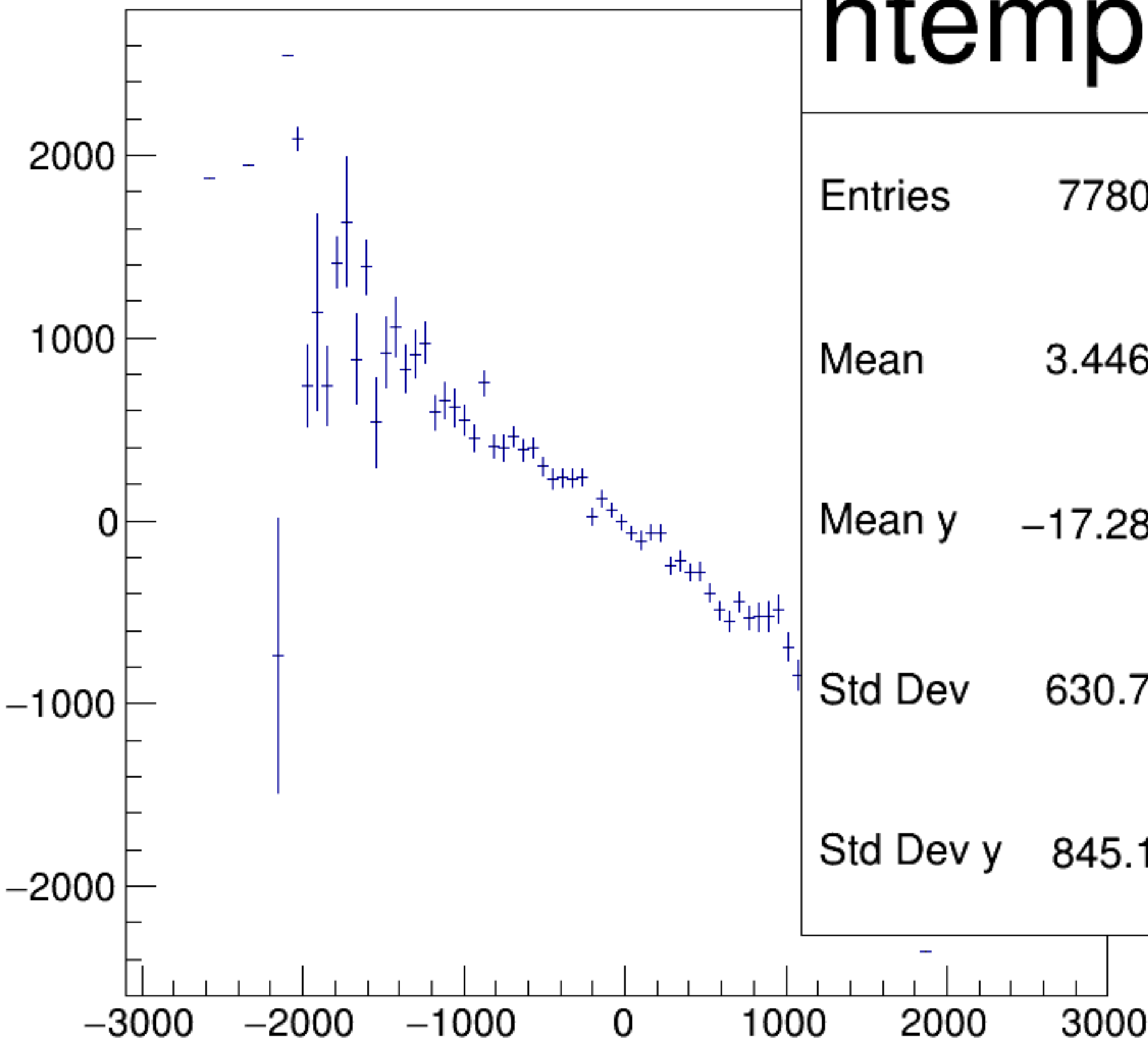
asym_dsl/ppm:asym_dsr/ppm {ok_cut}
