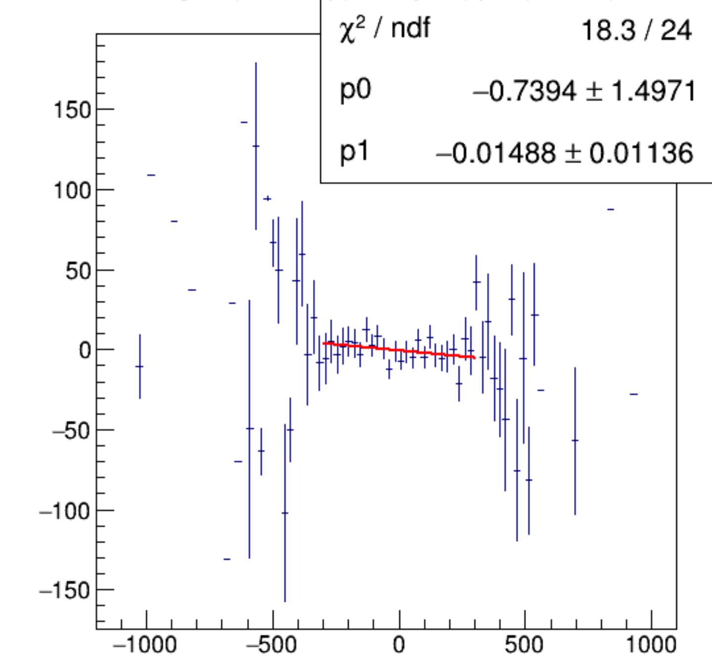
reg_asym_usr/ppm:AqDS/ppm {ok_cut}
