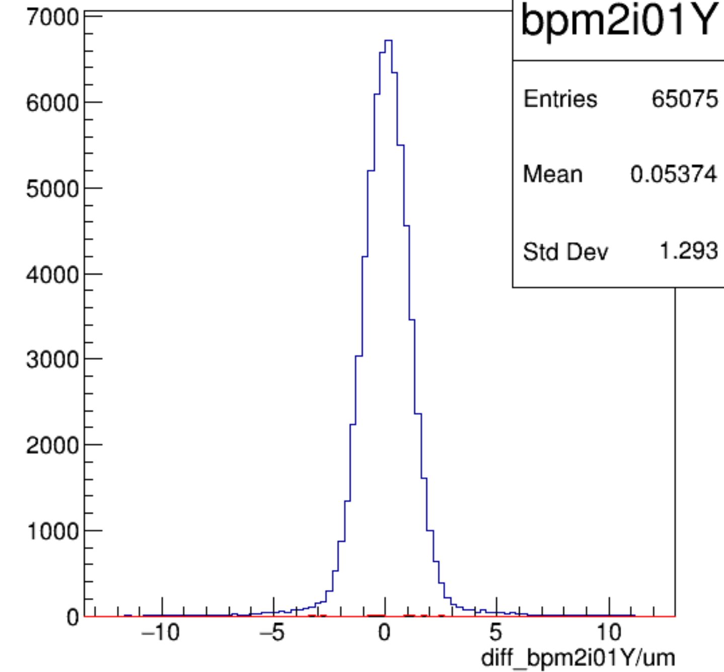
diff_bpm2i01Y/um {ErrorFlag==0}
