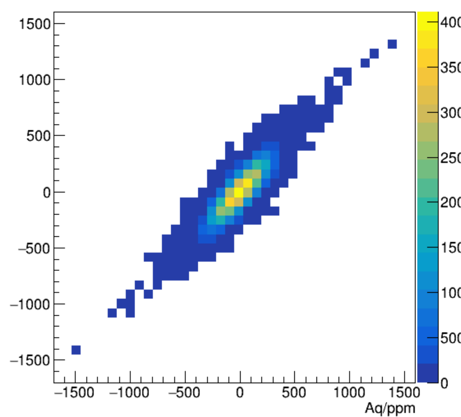
asym_bpm12WS/ppm:Aq/ppm {ErrorFlag==0}
