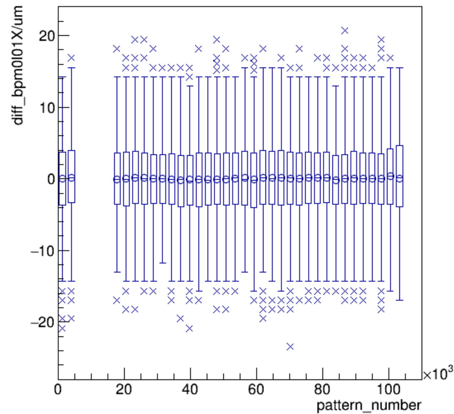
diff_bpm0l01X/um:pattern_number {ErrorFlag==0}
