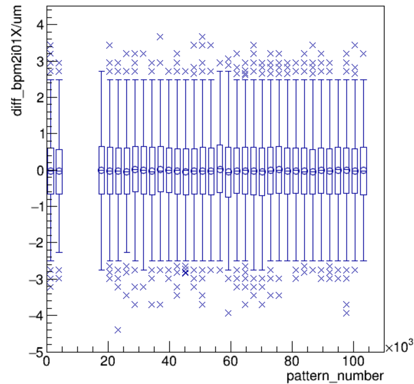
diff_bpm2i01X/um:pattern_number {ErrorFlag==0}
