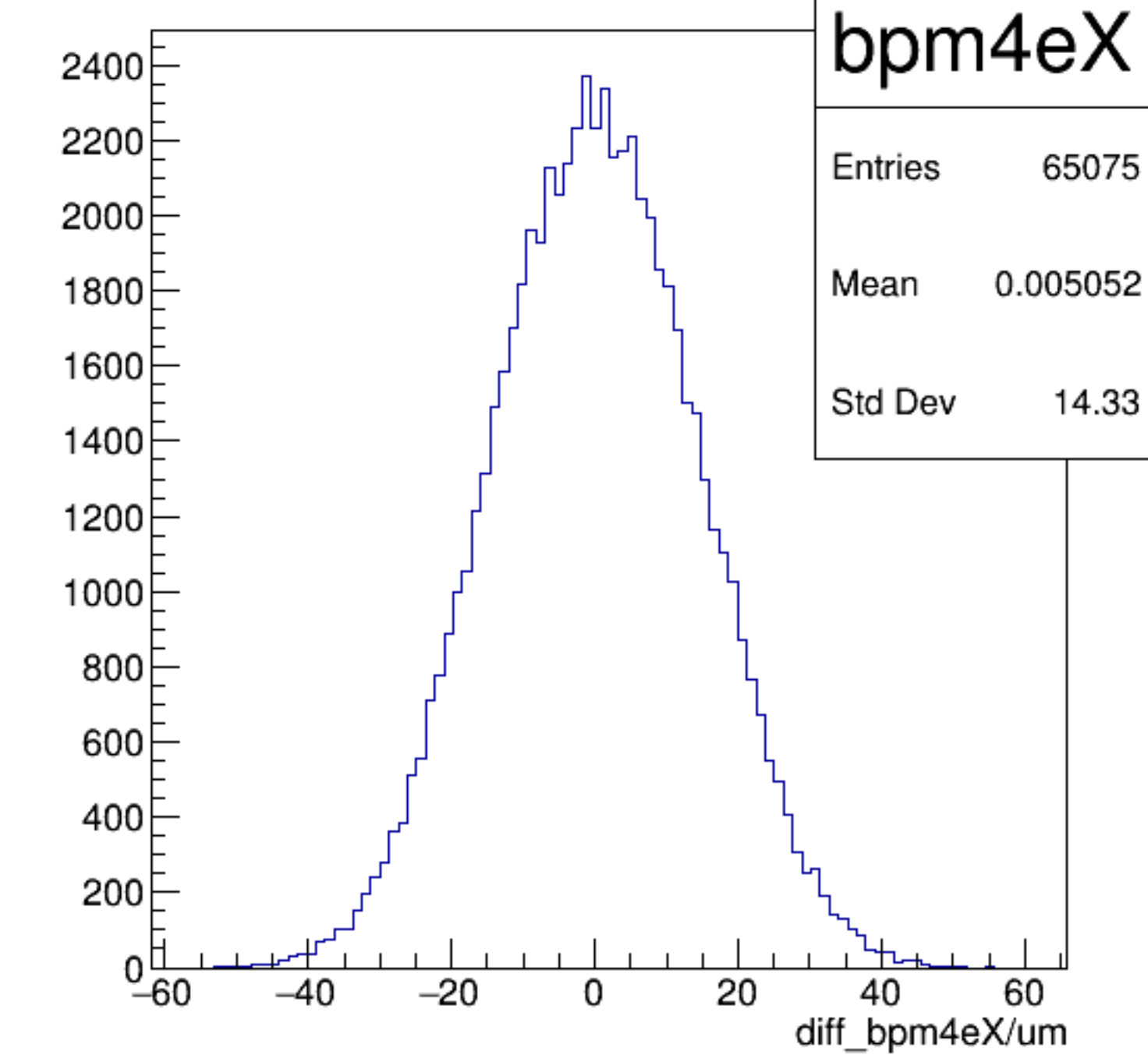
diff_bpm4eX/um {ErrorFlag==0}
