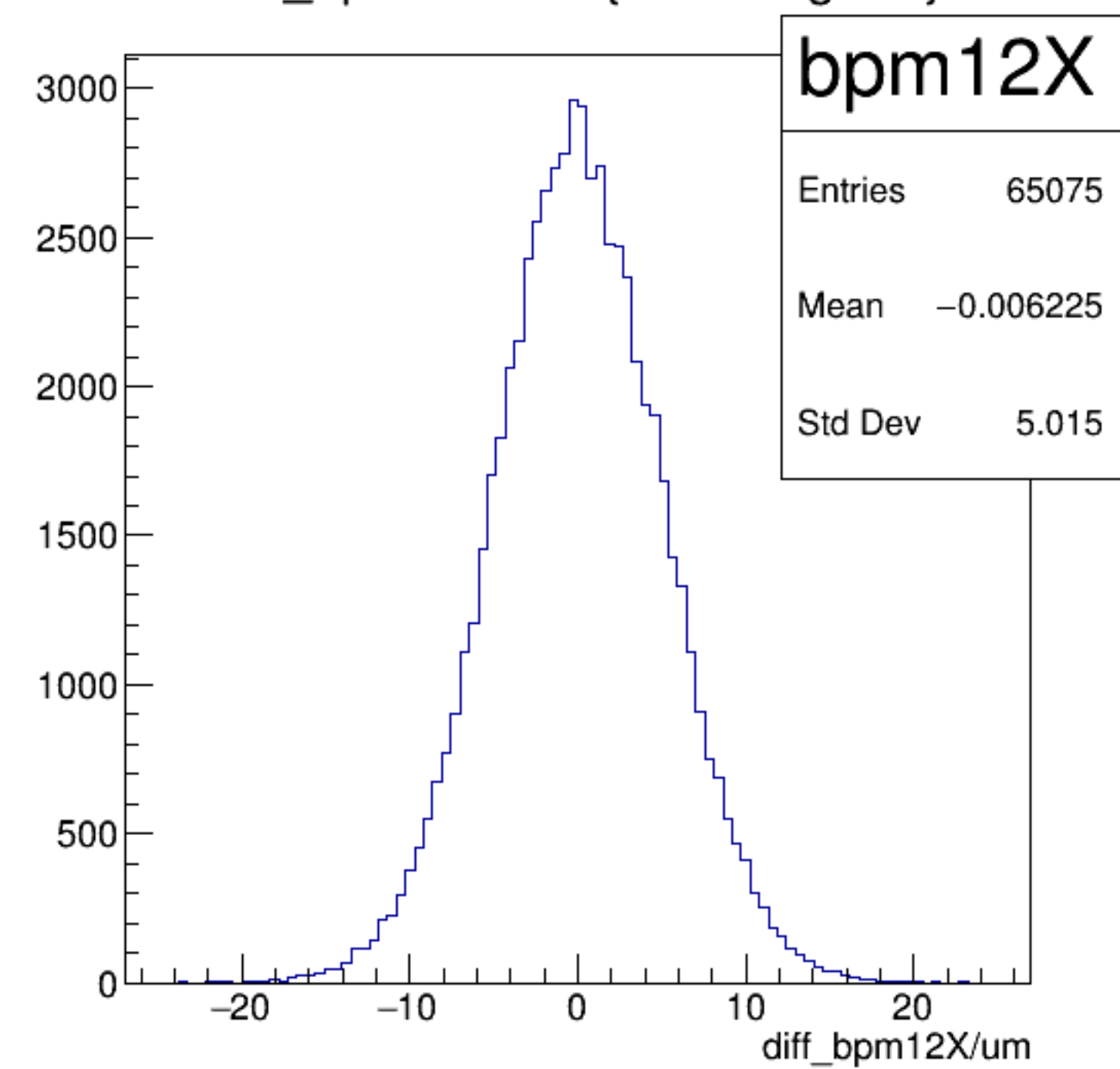
diff_bpm12X/um {ErrorFlag==0}
