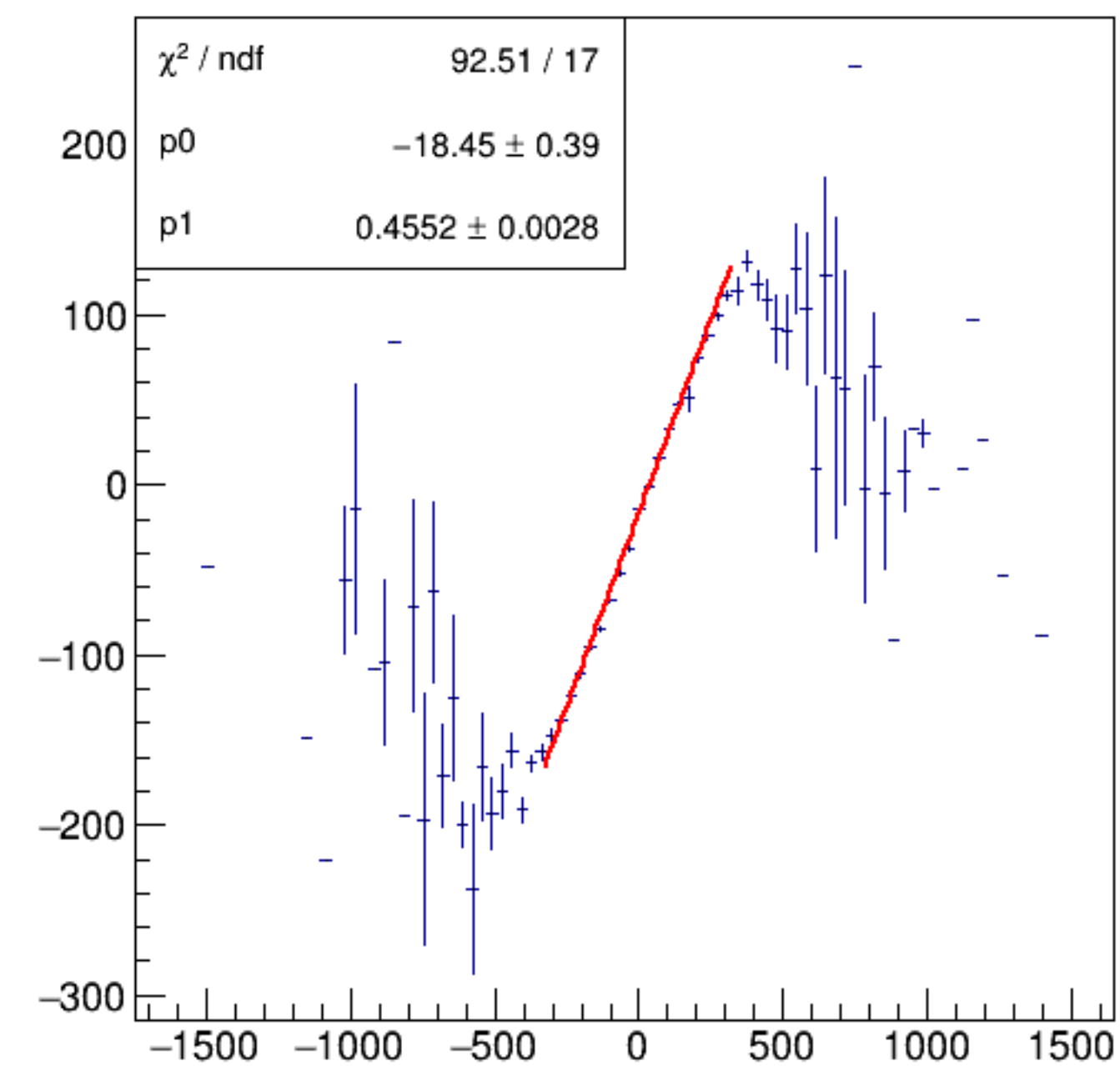
asym_bpm2i02WS/ppm:Aq/ppm {ErrorFlag==0}
