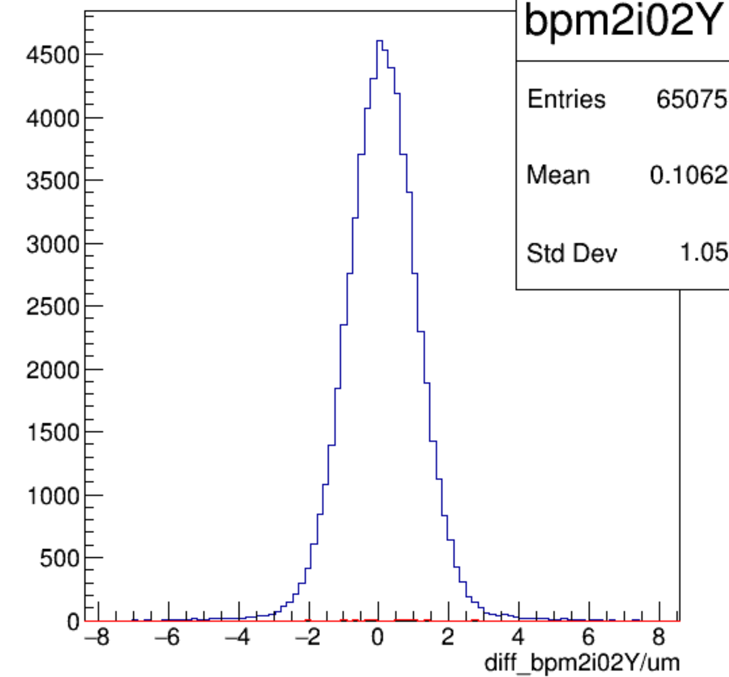
diff_bpm2i02Y/um {ErrorFlag==0}
