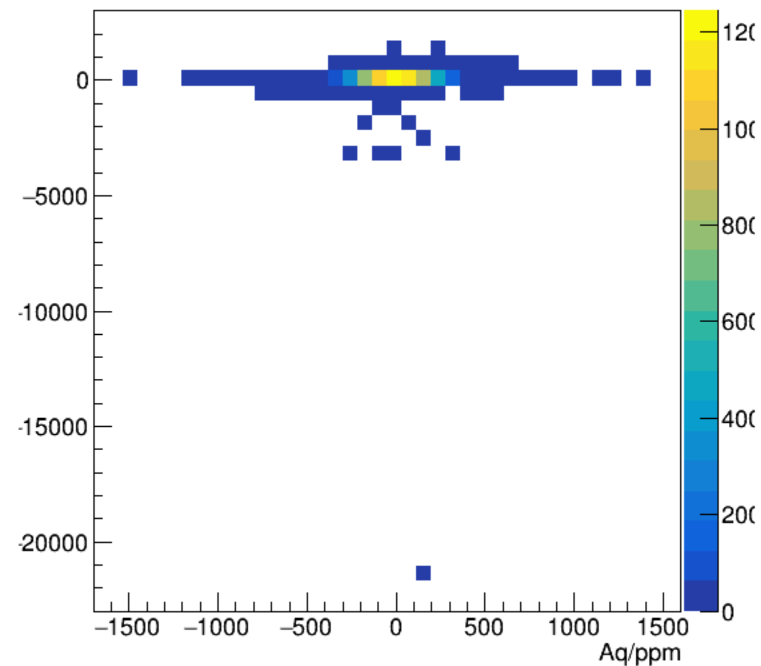
asym_bpm2i02WS/ppm:Aq/ppm {ErrorFlag==0}
