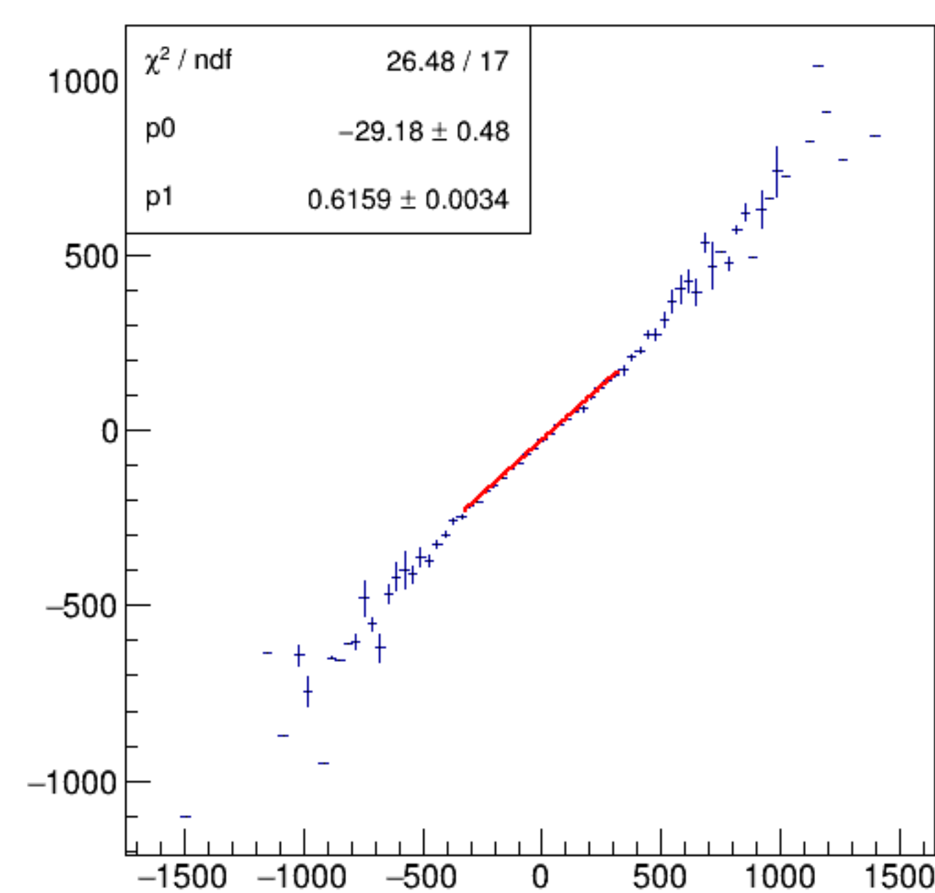
asym_bpm0i02WS/ppm:Aq/ppm {ErrorFlag==0}
