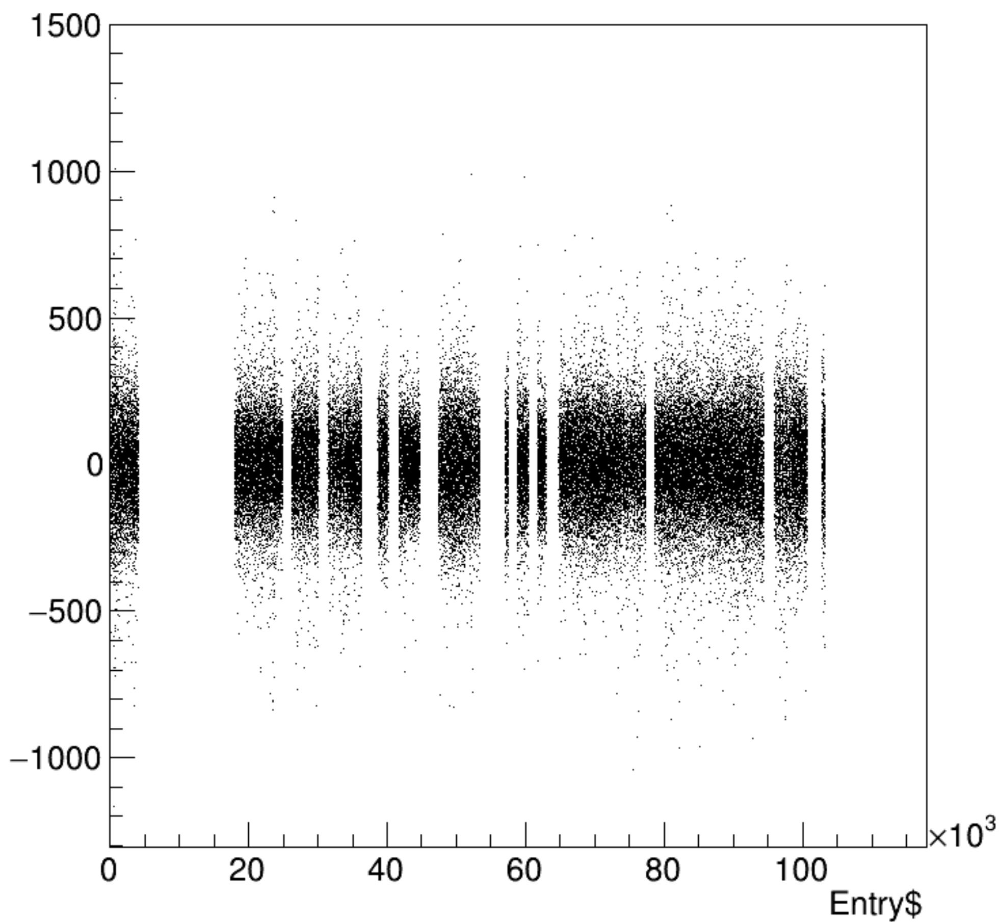
asym_bpm0l01WS/ppm:Entry$ {ErrorFlag==0}
