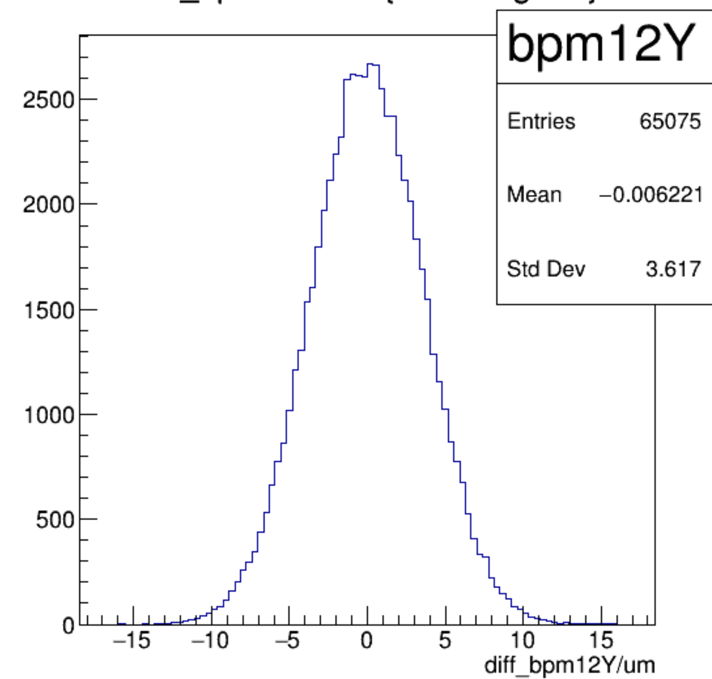
diff_bpm12Y/um {ErrorFlag==0}
