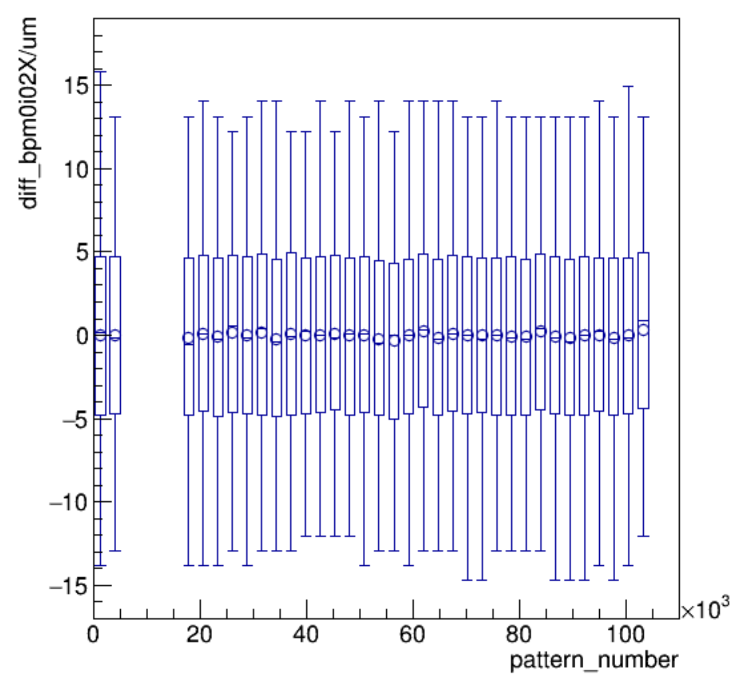
diff_bpm0i02X/um:pattern_number {ErrorFlag==0}
