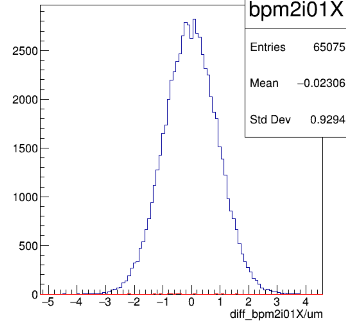
diff_bpm2i01X/um {ErrorFlag==0}
