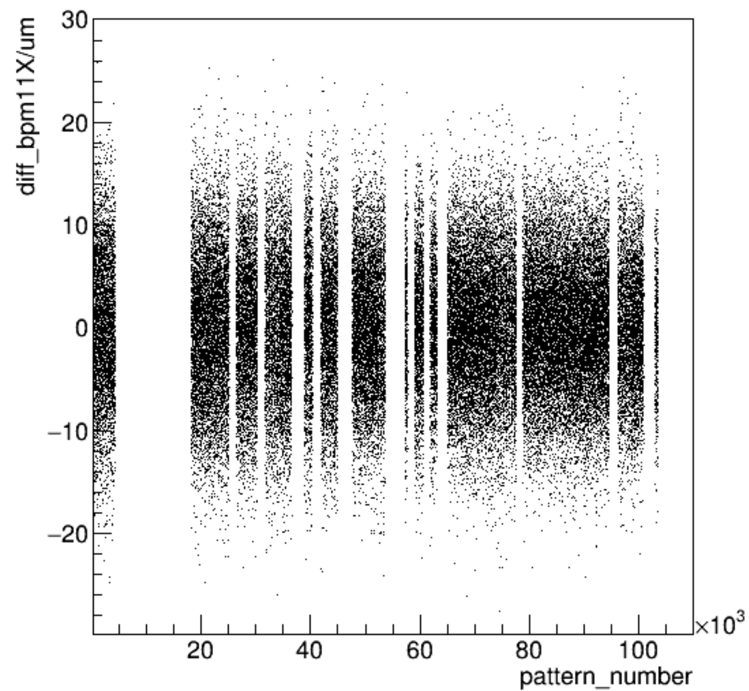
diff_bpm11X/um:pattern_number {ErrorFlag==0}
