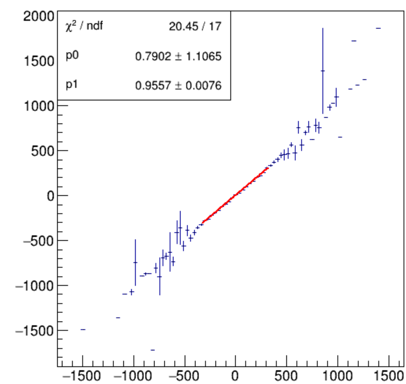
asym_bpm4acWS/ppm:Aq/ppm {ErrorFlag==0}
