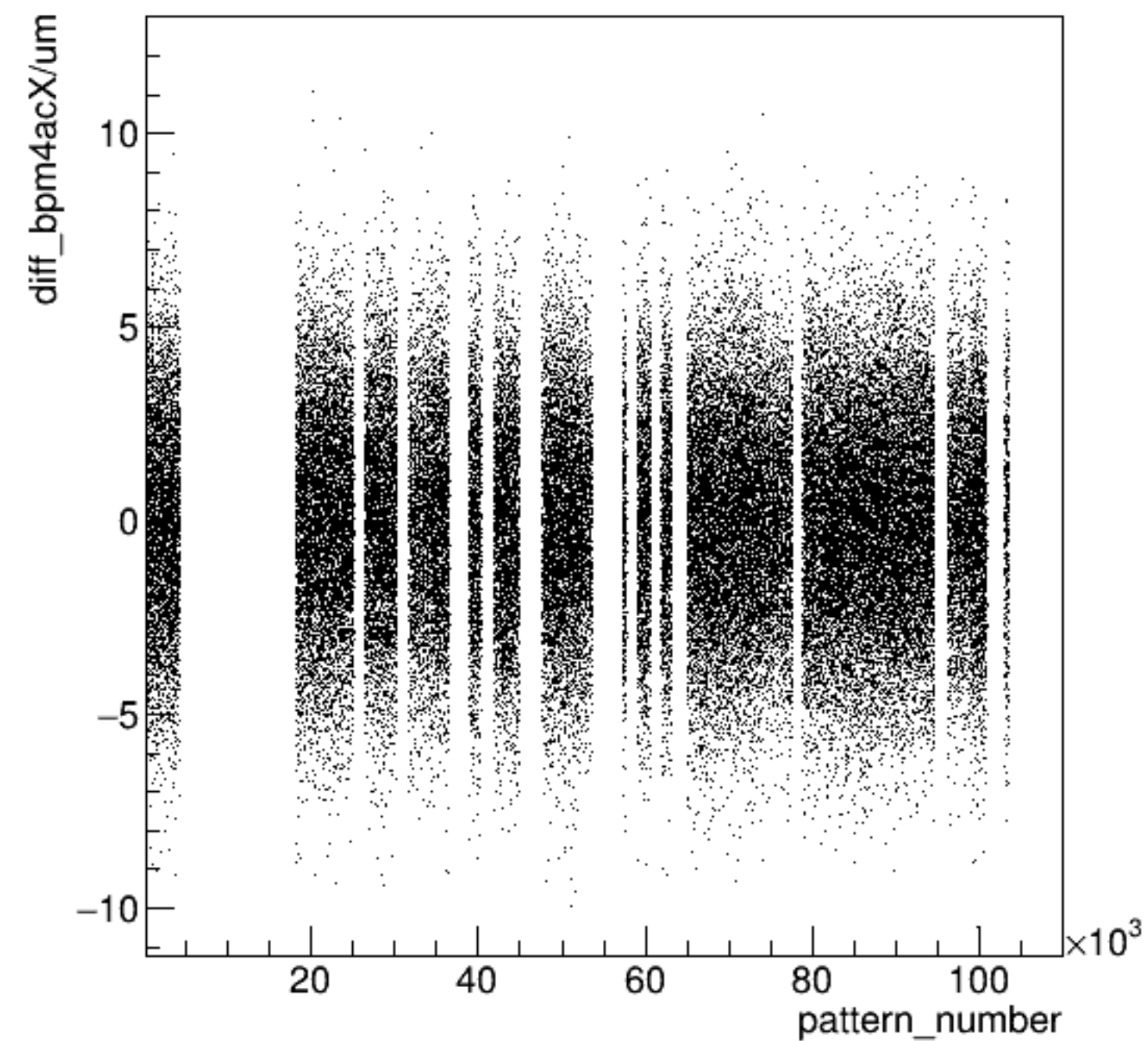
diff_bpm4acX/um:pattern_number {ErrorFlag==0}
