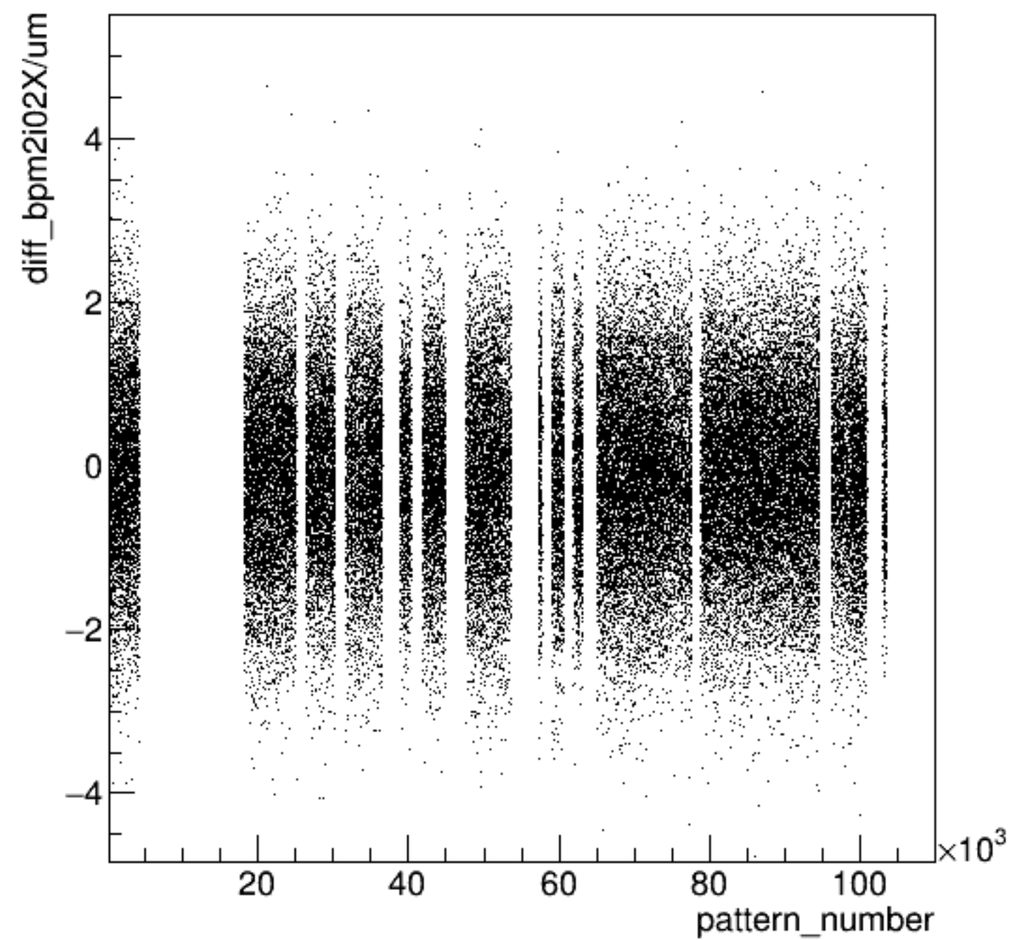
diff_bpm2i02X/um:pattern_number {ErrorFlag==0}
