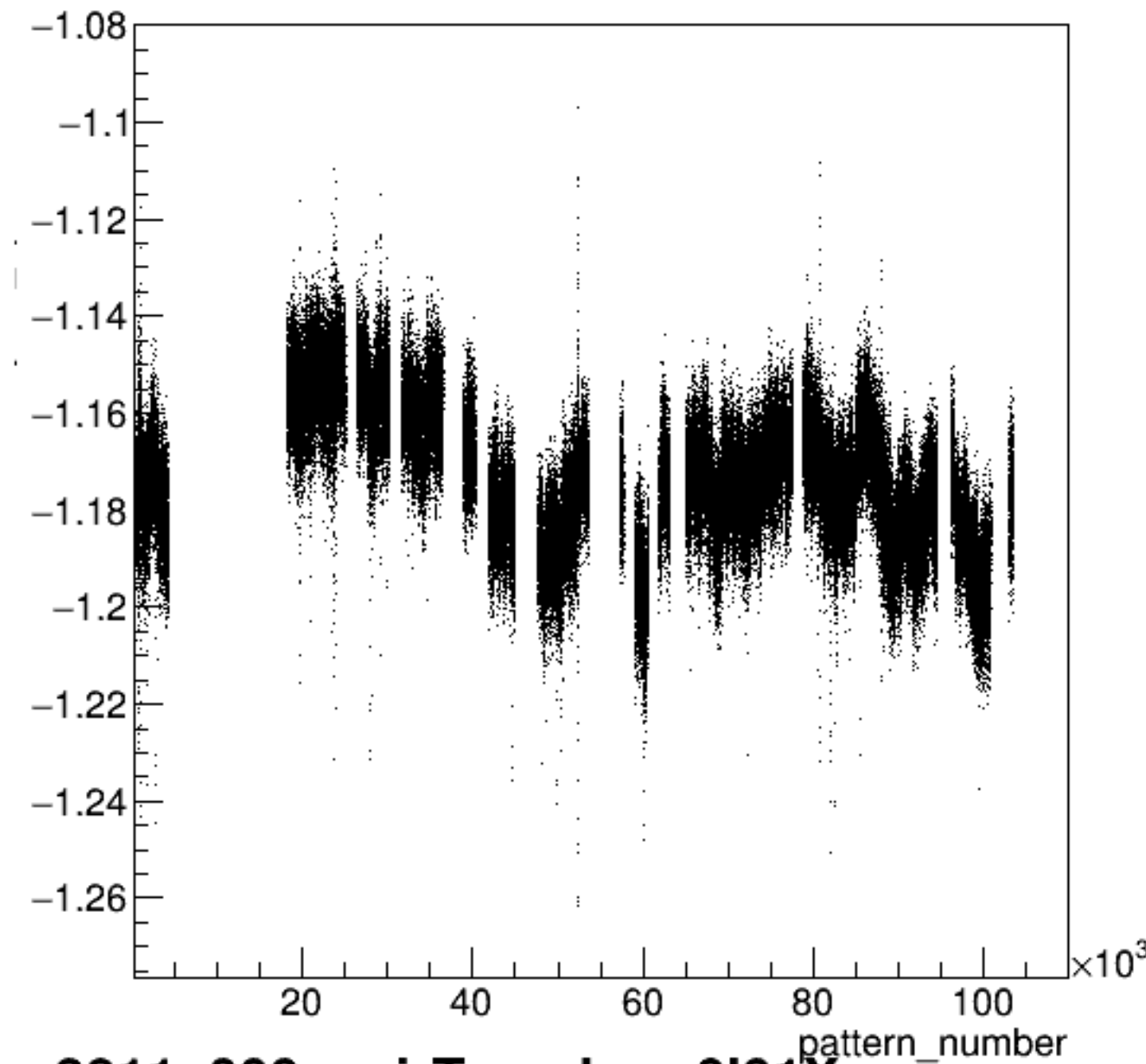
yield_bpm0l01X/mm:pattern_number {ErrorFlag==0}
