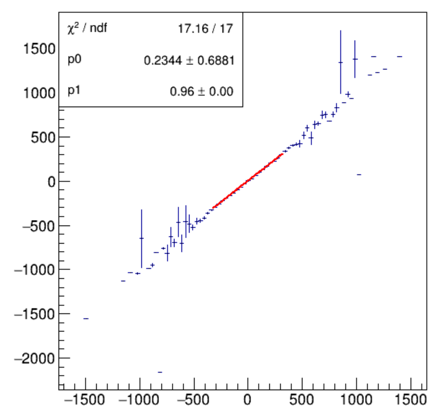
asym_bpm4eWS/ppm:Aq/ppm {ErrorFlag==0}
