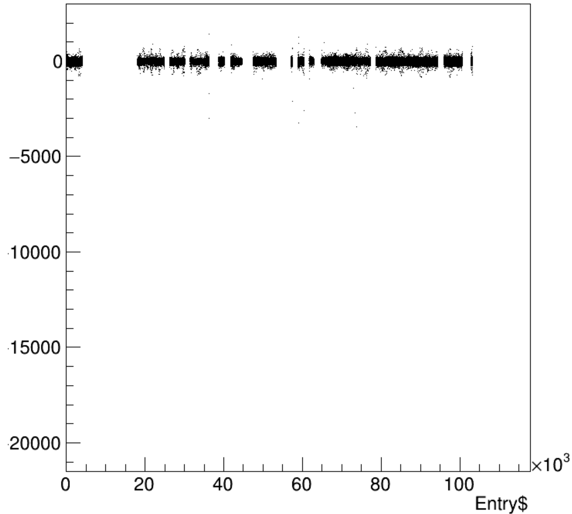
asym_bpm2i01WS/ppm:Entry$ {ErrorFlag==0}
