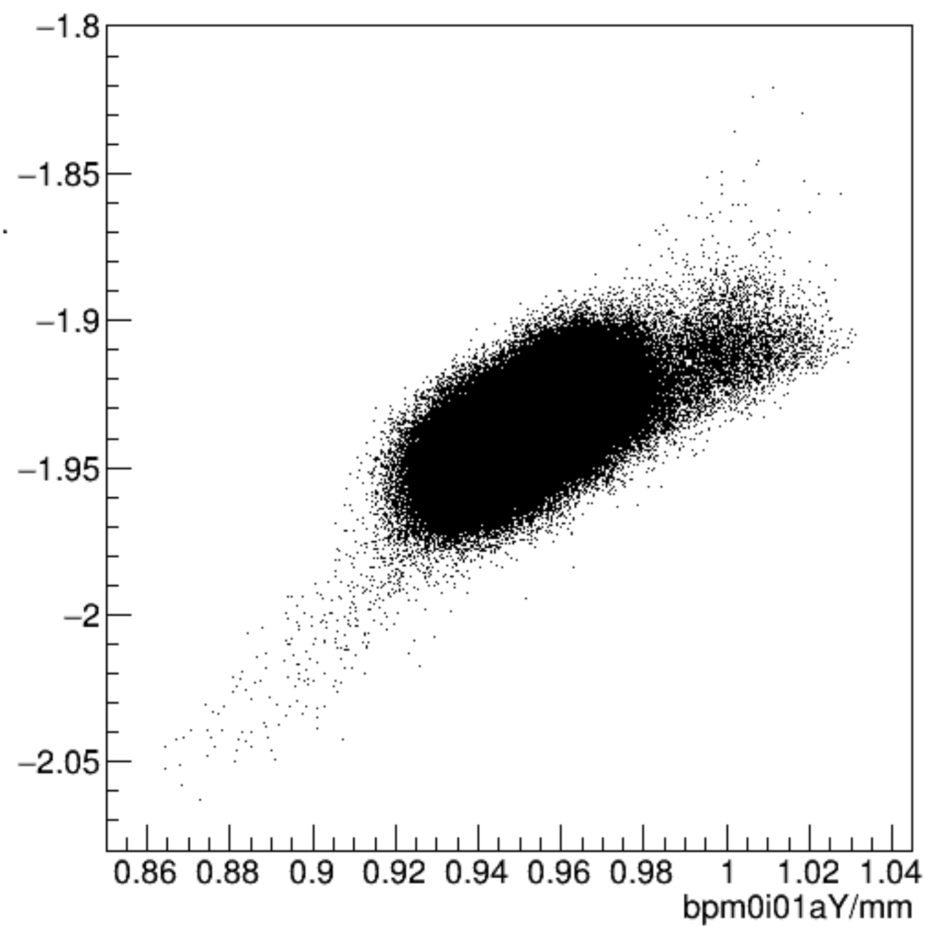
bpm0i01aX/mm:bpm0i01aY/mm {ErrorFlag==0}
