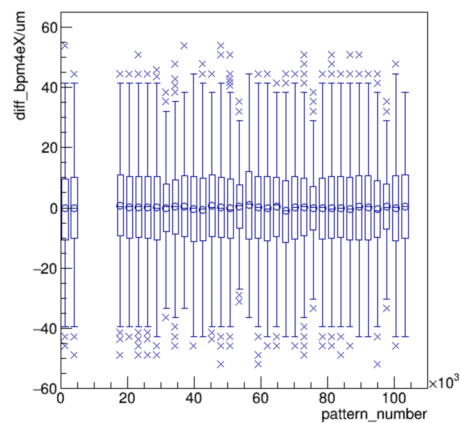
diff_bpm4eX/um:pattern_number {ErrorFlag==0}
