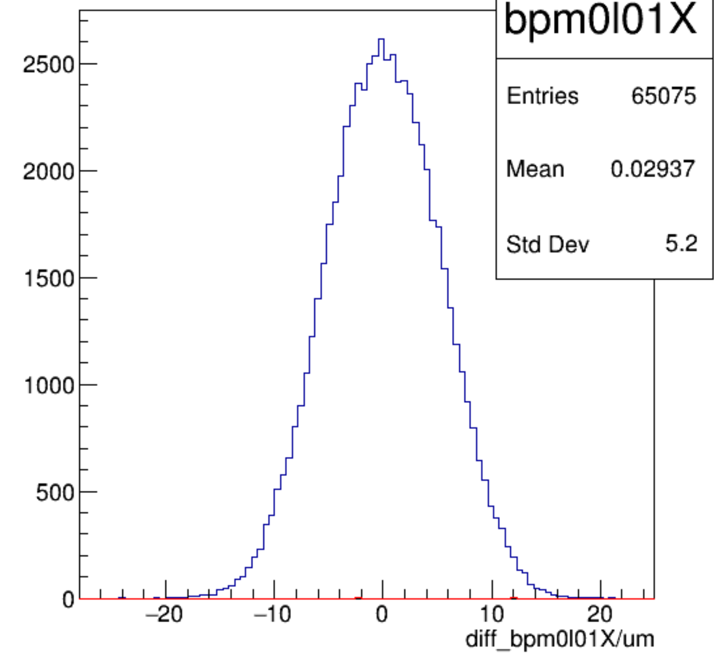
diff_bpm0l01X/um {ErrorFlag==0}
