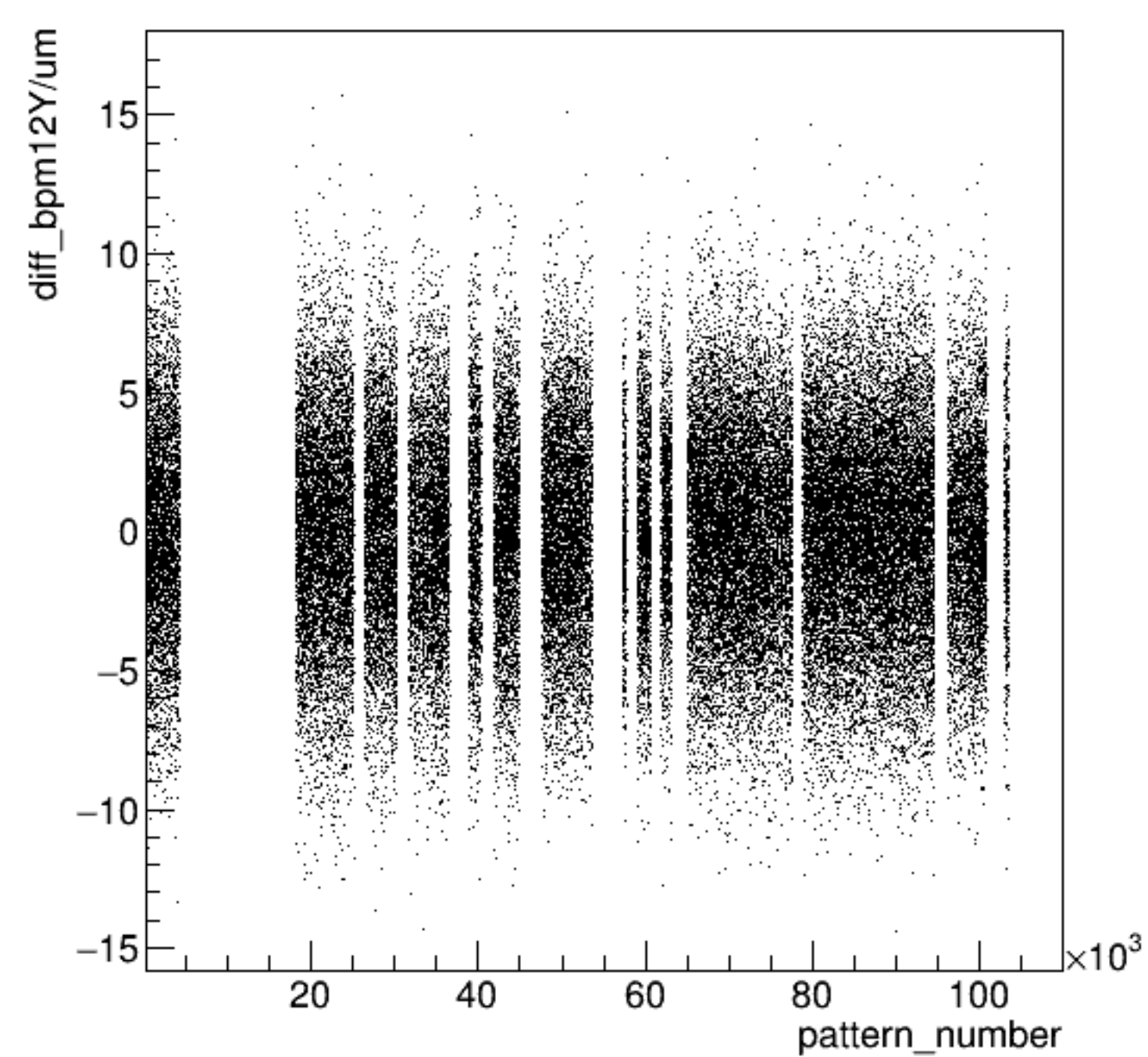
diff_bpm12Y/um:pattern_number {ErrorFlag==0}
