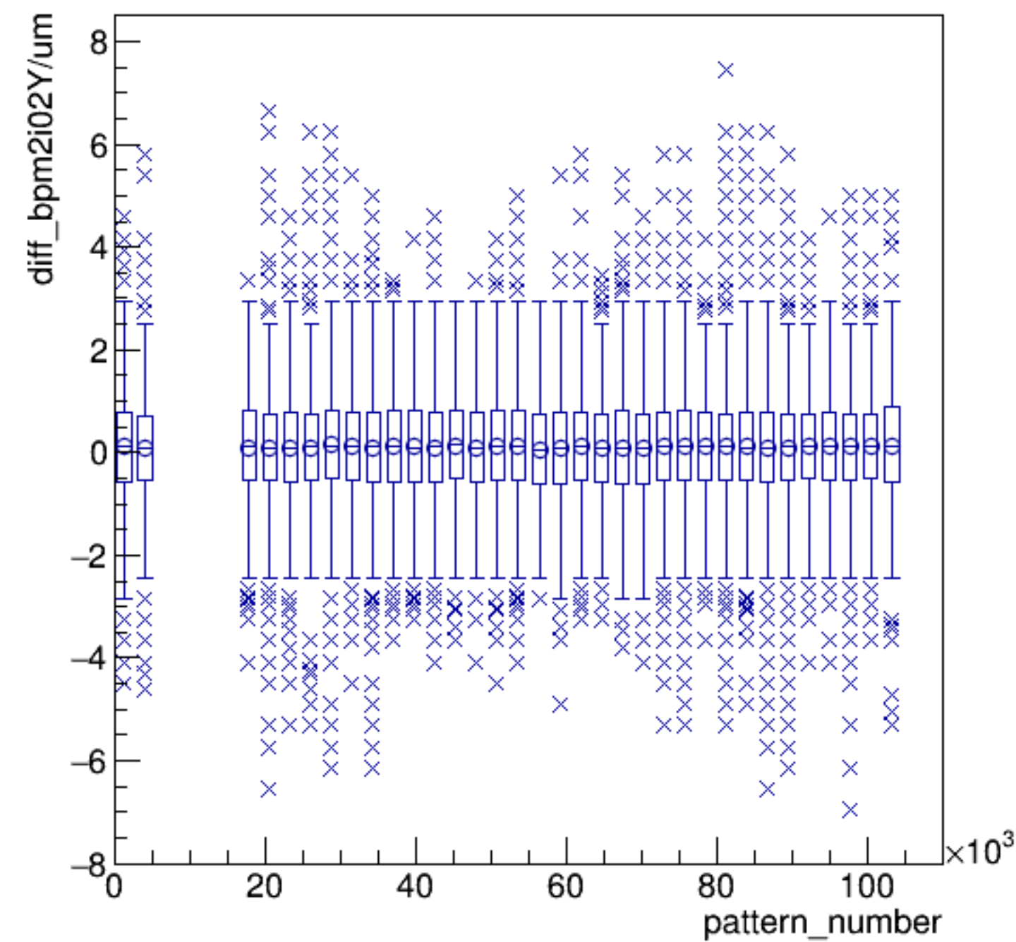
diff_bpm2i02Y/um:pattern_number {ErrorFlag==0}
