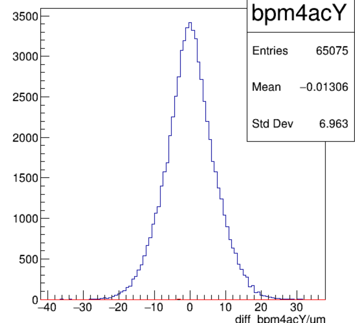
diff_bpm4acY/um {ErrorFlag==0}
