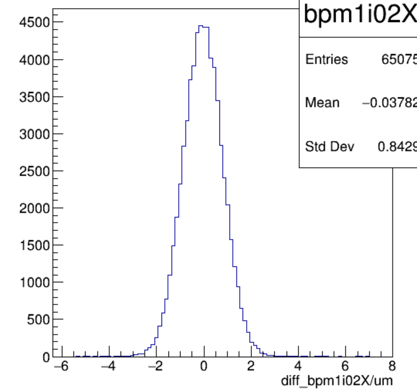
diff_bpm1i02X/um {ErrorFlag==0}
