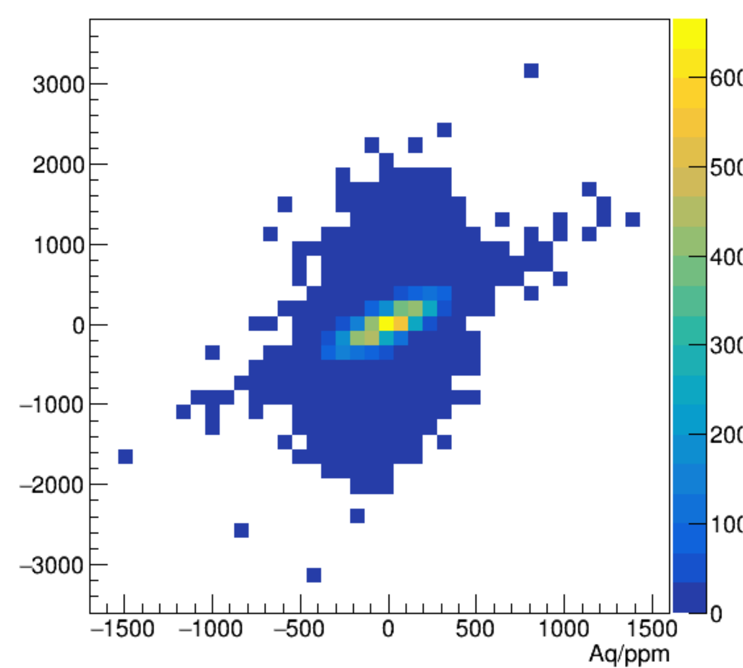
asym_bpm4aWS/ppm:Aq/ppm {ErrorFlag==0}
