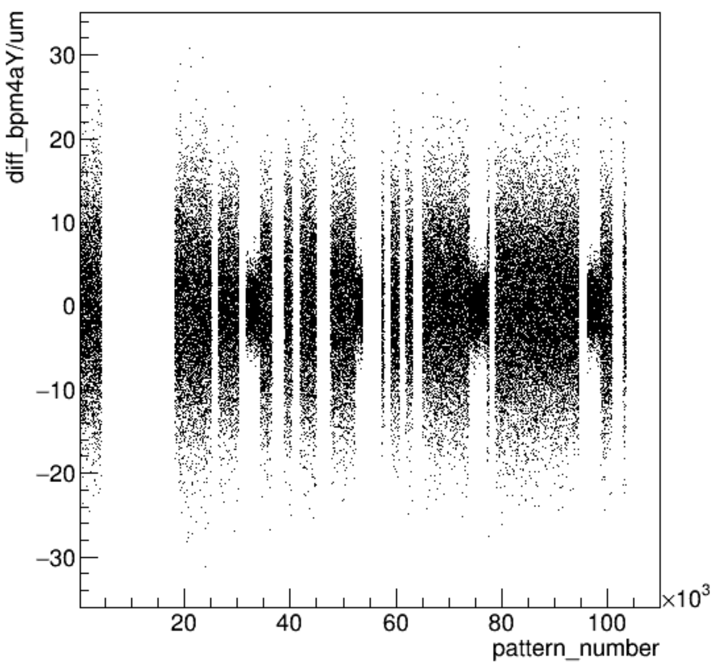
diff_bpm4aY/um:pattern_number {ErrorFlag==0}
