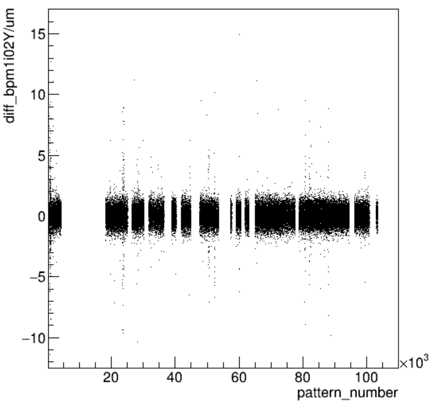
diff_bpm1i02Y/um:pattern_number {ErrorFlag==0}
