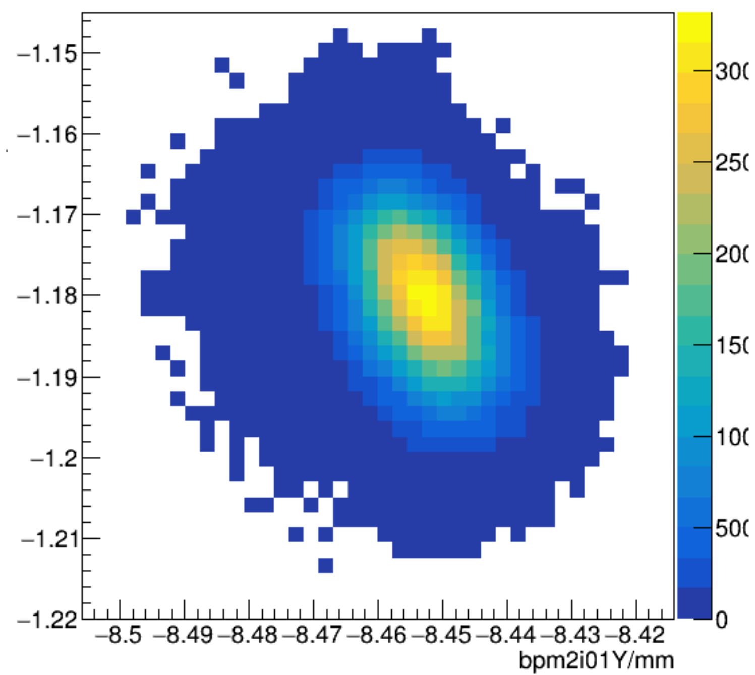
bpm2i01X/mm:bpm2i01Y/mm {ErrorFlag==0}
