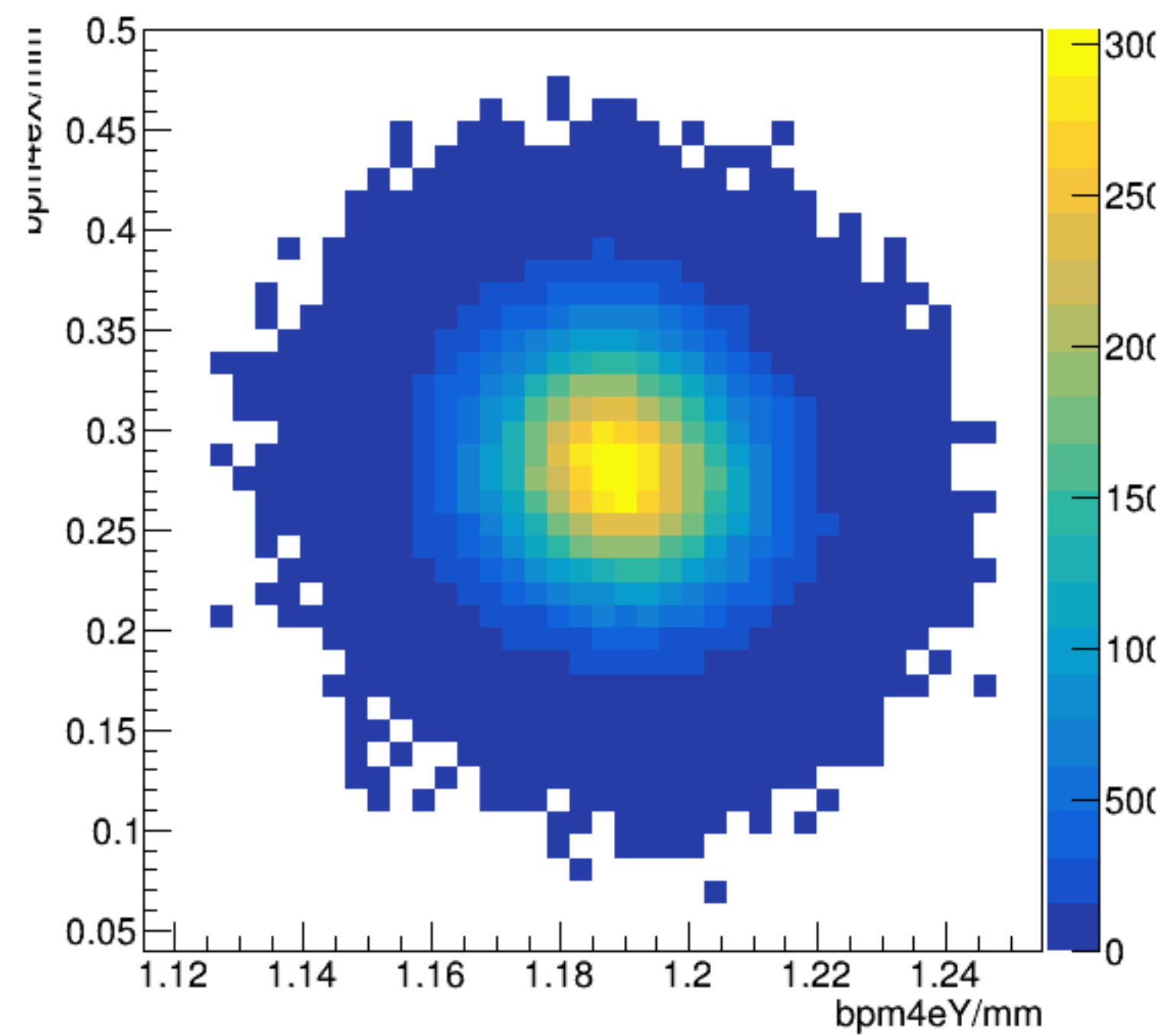
bpm4eX/mm:bpm4eY/mm {ErrorFlag==0}
