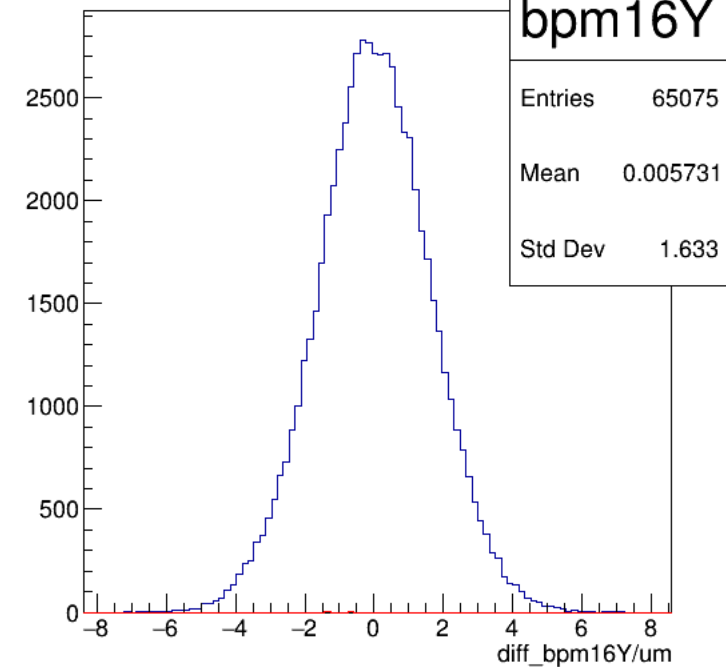
diff_bpm16Y/um {ErrorFlag==0}
