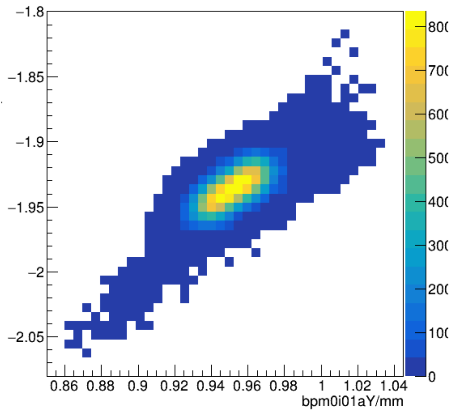
bpm0i01aX/mm:bpm0i01aY/mm {ErrorFlag==0}
