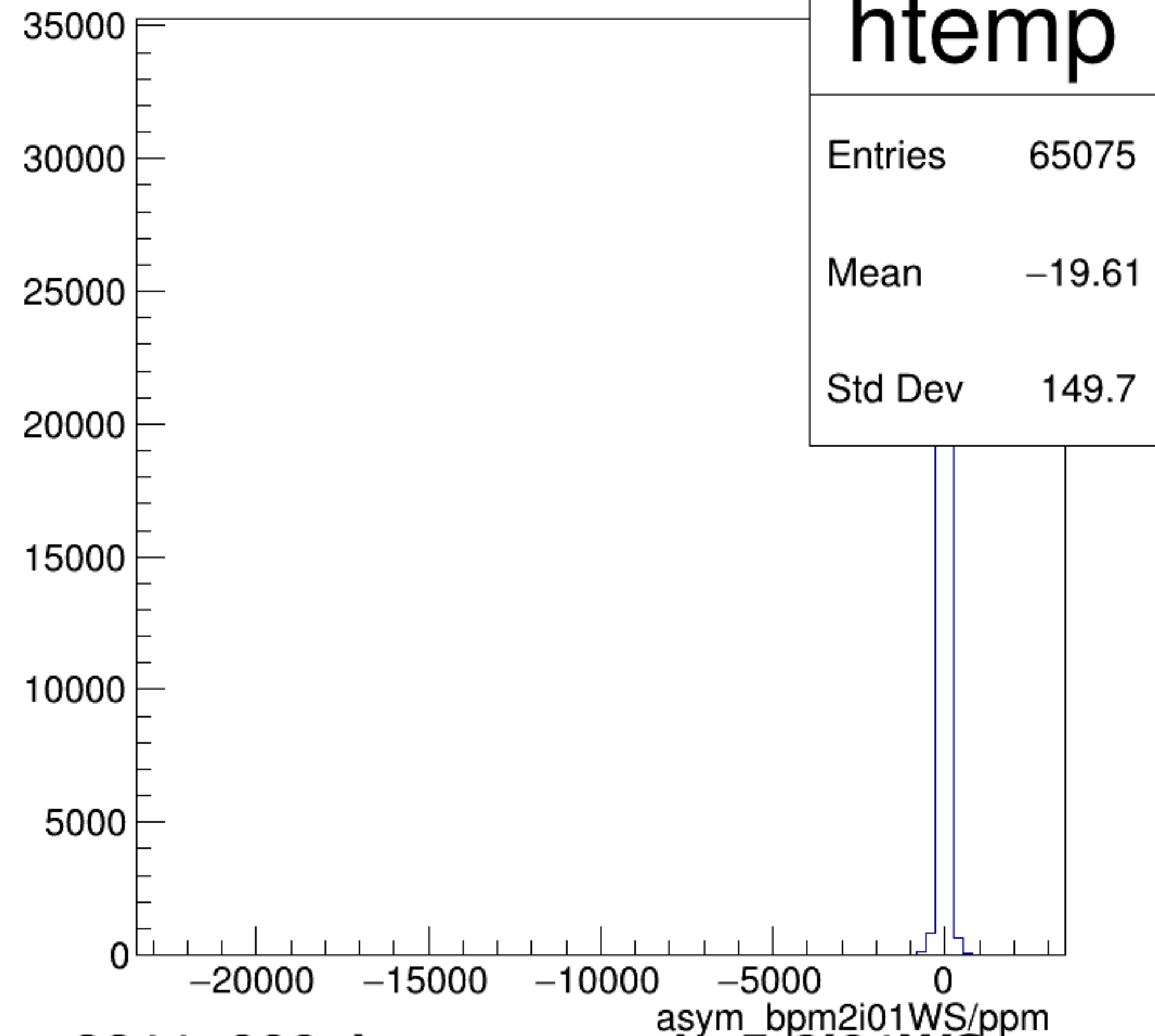
asym_bpm2i01WS/ppm {ErrorFlag==0}
