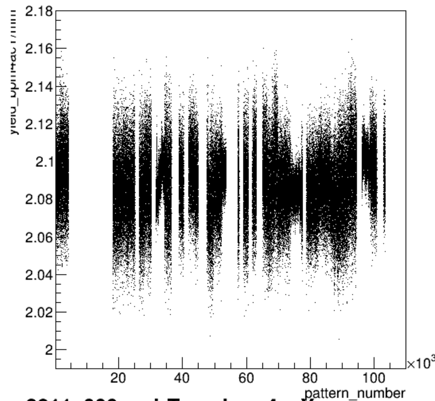
yield_bpm4acY/mm:pattern_number {ErrorFlag==0}
