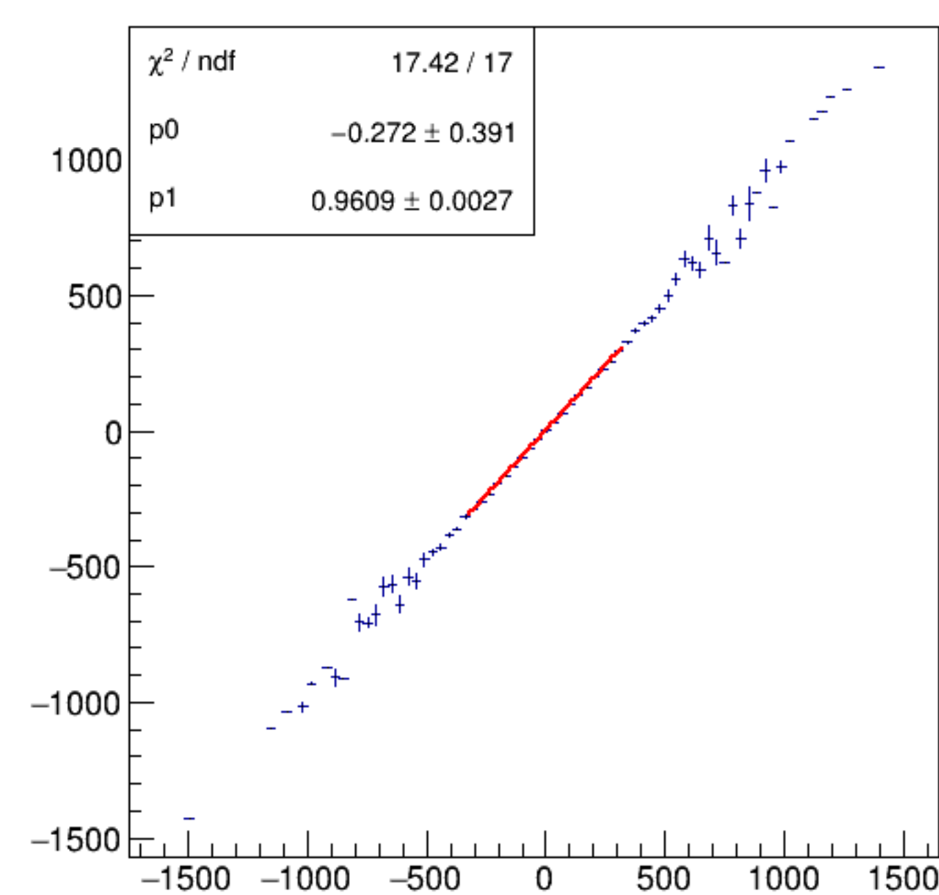
asym_bpm12WS/ppm:Aq/ppm {ErrorFlag==0}
