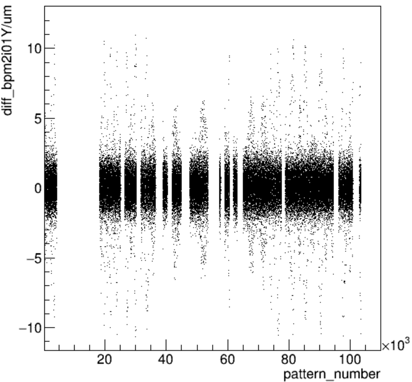
diff_bpm2i01Y/um:pattern_number {ErrorFlag==0}
