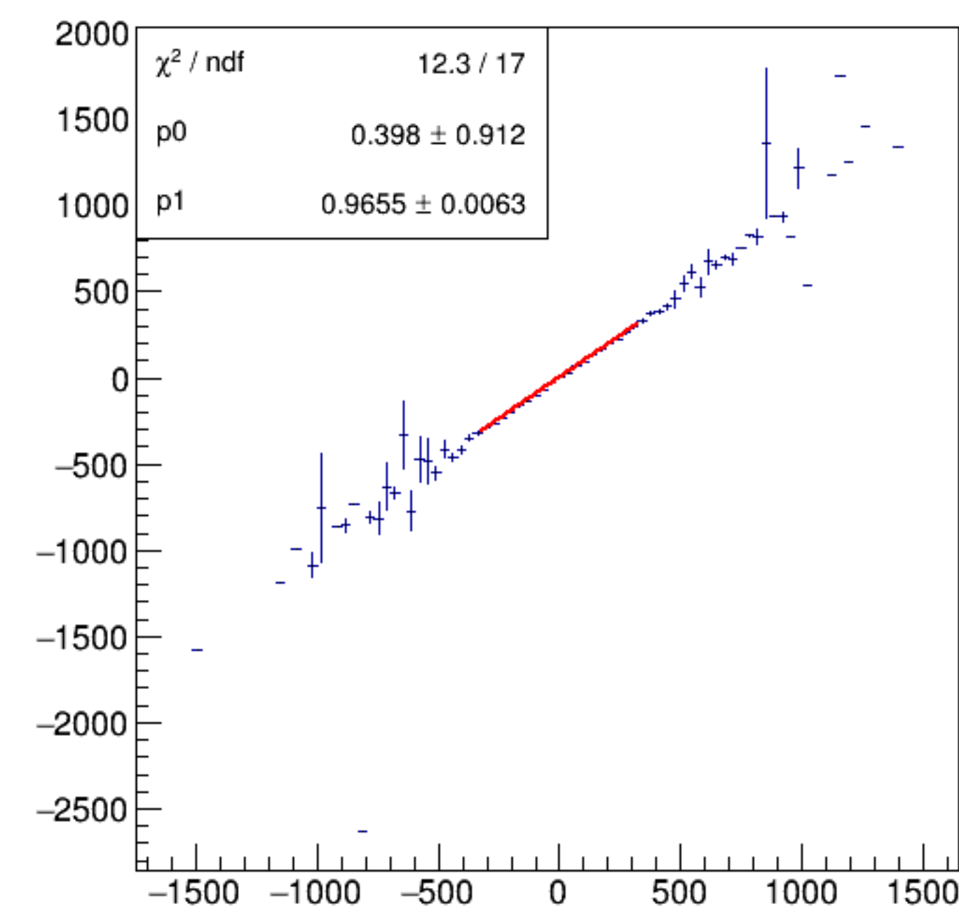
asym_bpm4aWS/ppm:Aq/ppm {ErrorFlag==0}
