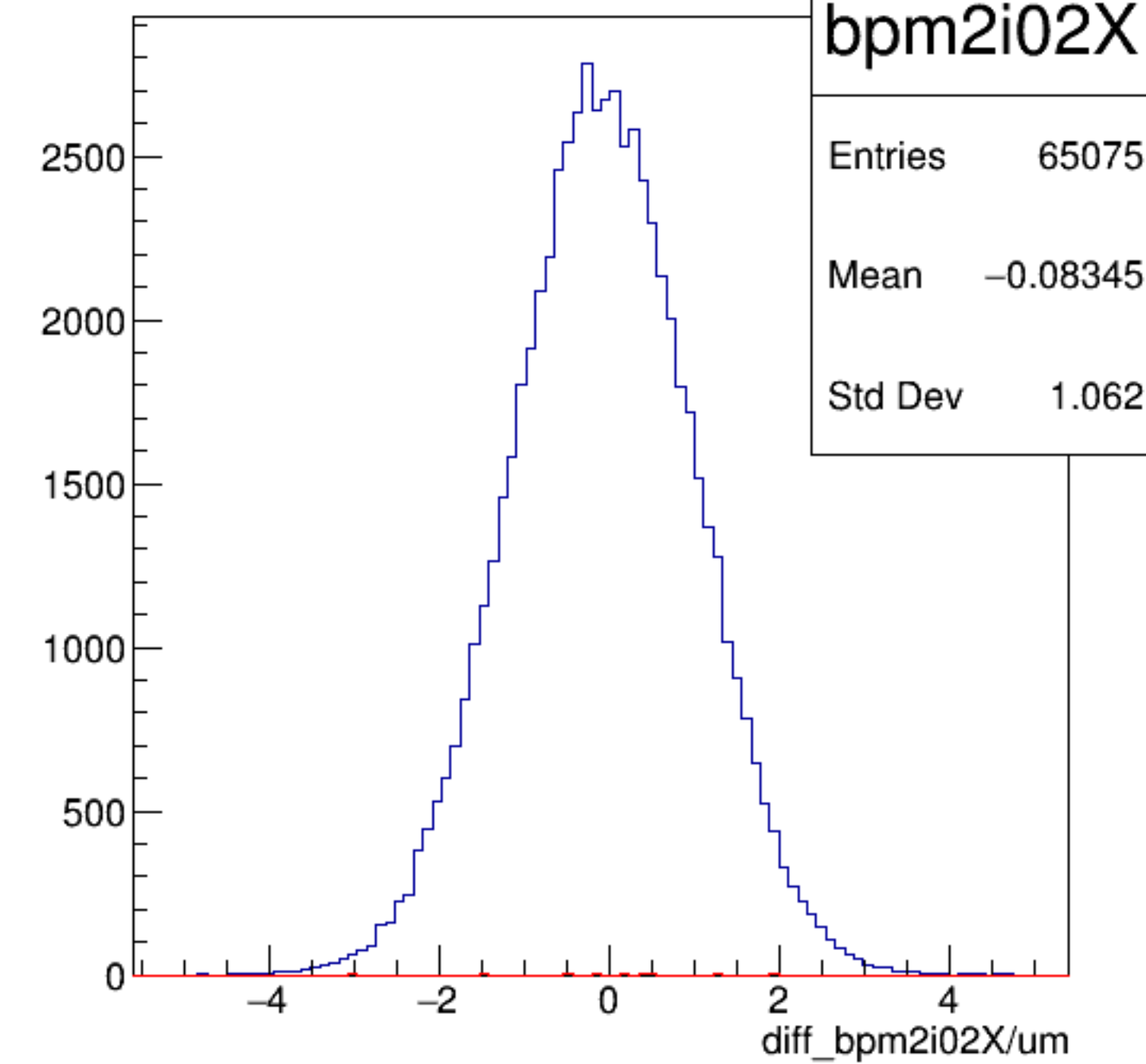
diff_bpm2i02X/um {ErrorFlag==0}
