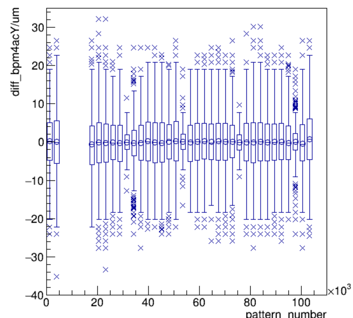
diff_bpm4acY/um:pattern_number {ErrorFlag==0}
