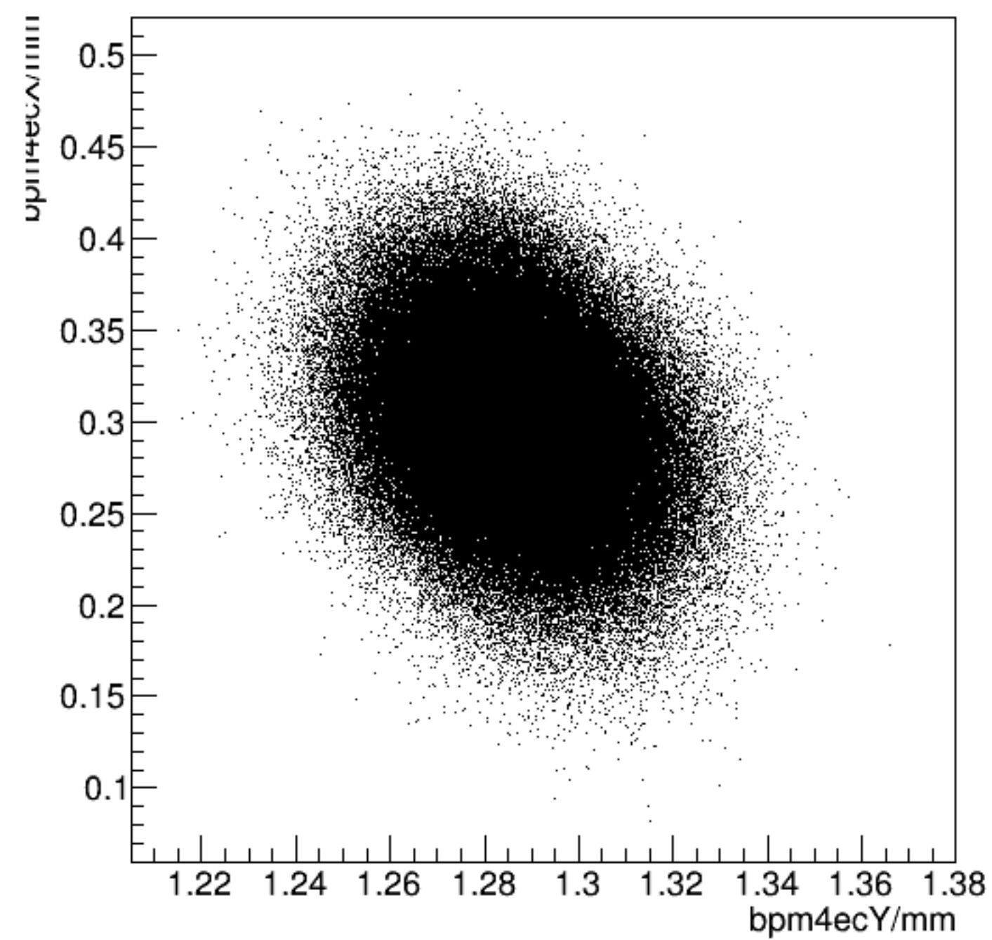
bpm4ecX/mm:bpm4ecY/mm {ErrorFlag==0}
