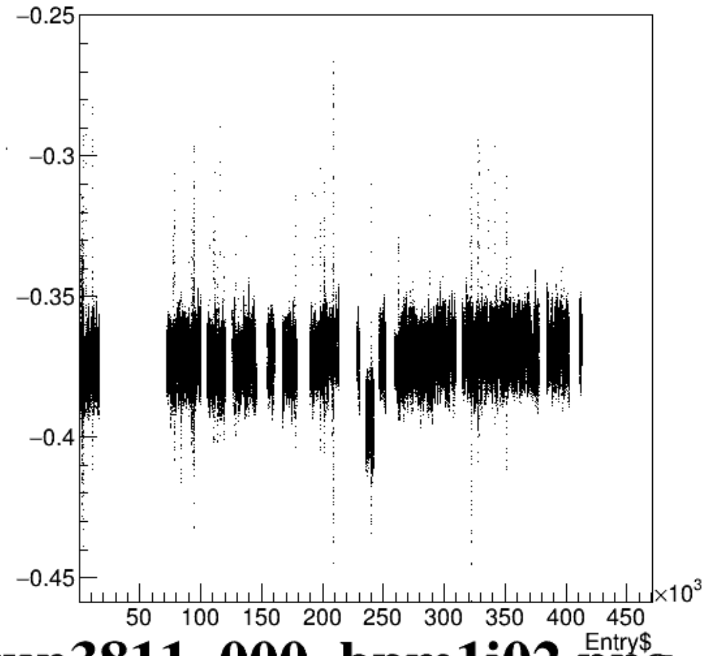
bpm1i02Y/mm:Entry$ {ErrorFlag==0}
