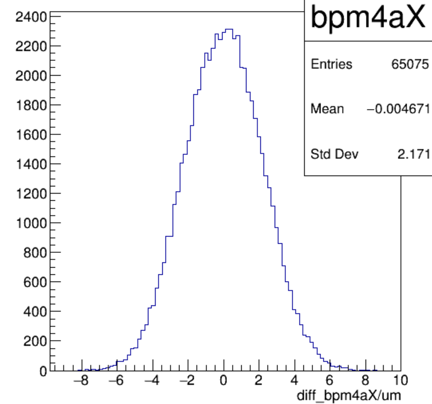
diff_bpm4aX/um {ErrorFlag==0}
