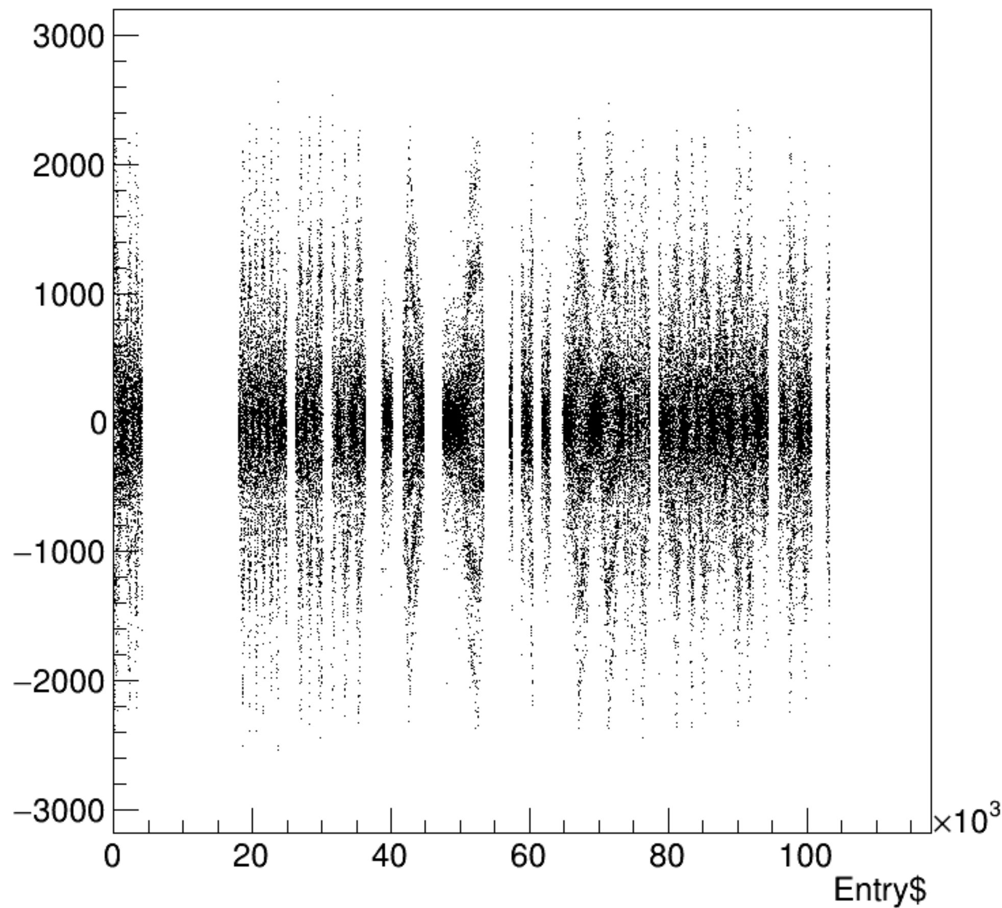
asym_bpm0i07WS/ppm:Entry$ {ErrorFlag==0}
