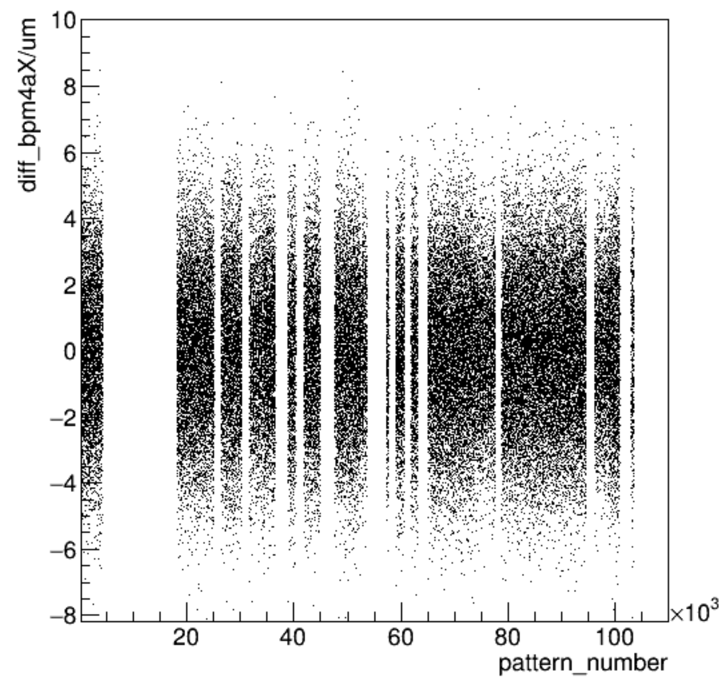
diff_bpm4aX/um:pattern_number {ErrorFlag==0}
