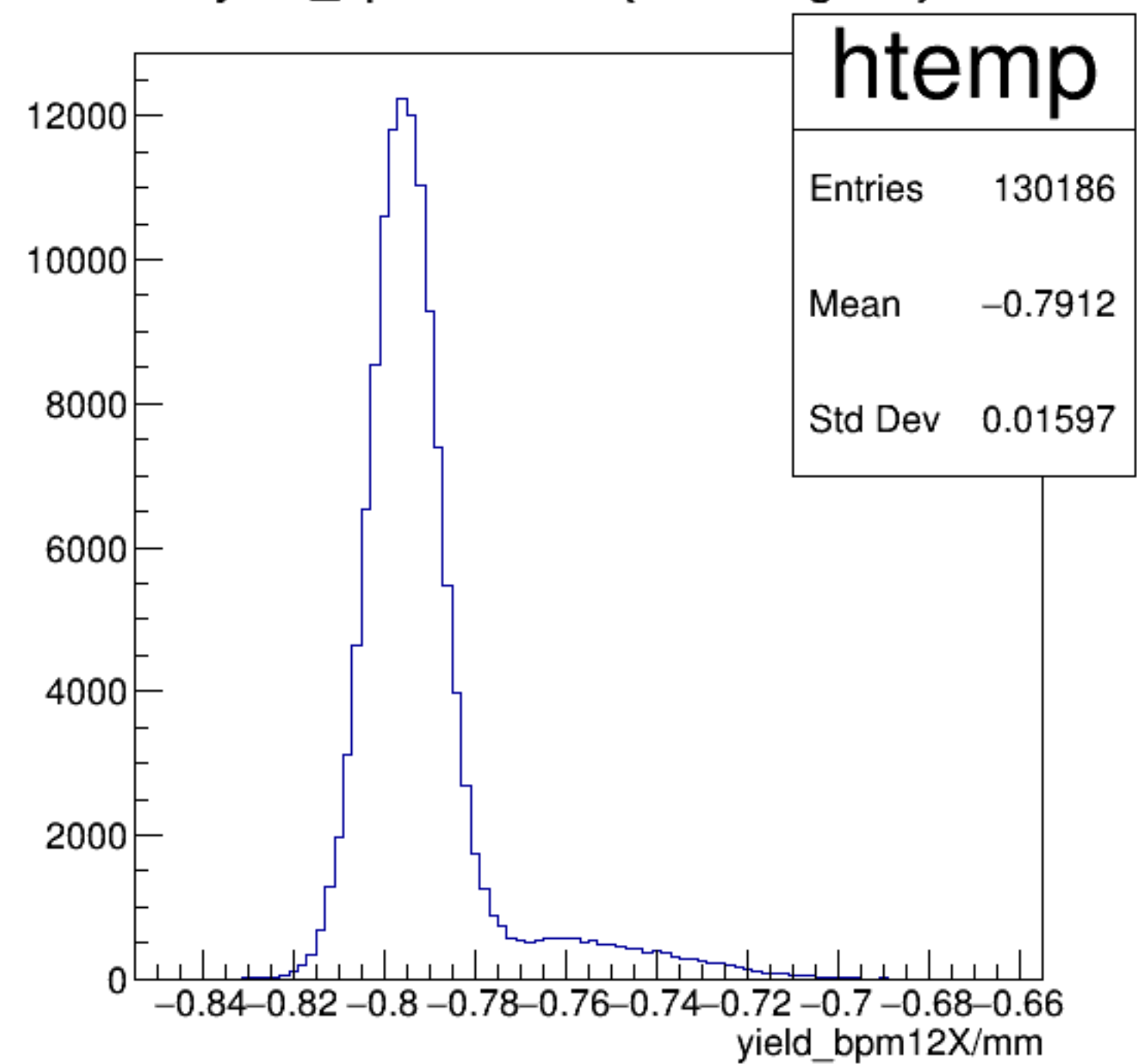
yield_bpm12X/mm {ErrorFlag==0}
