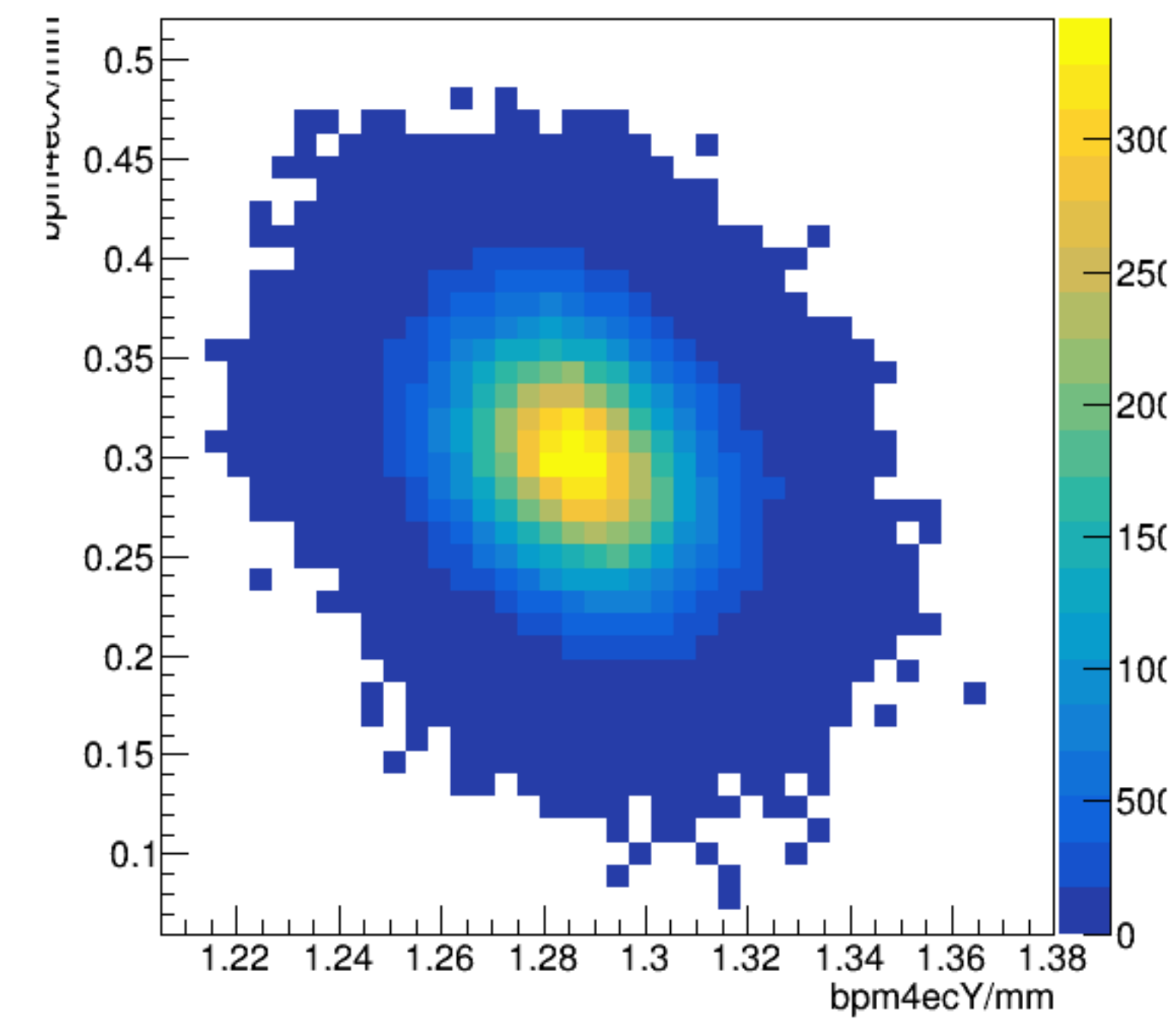
bpm4ecX/mm:bpm4ecY/mm {ErrorFlag==0}
