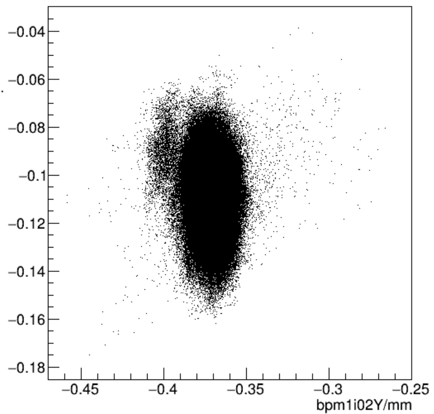
bpm1i02X/mm:bpm1i02Y/mm {ErrorFlag==0}
