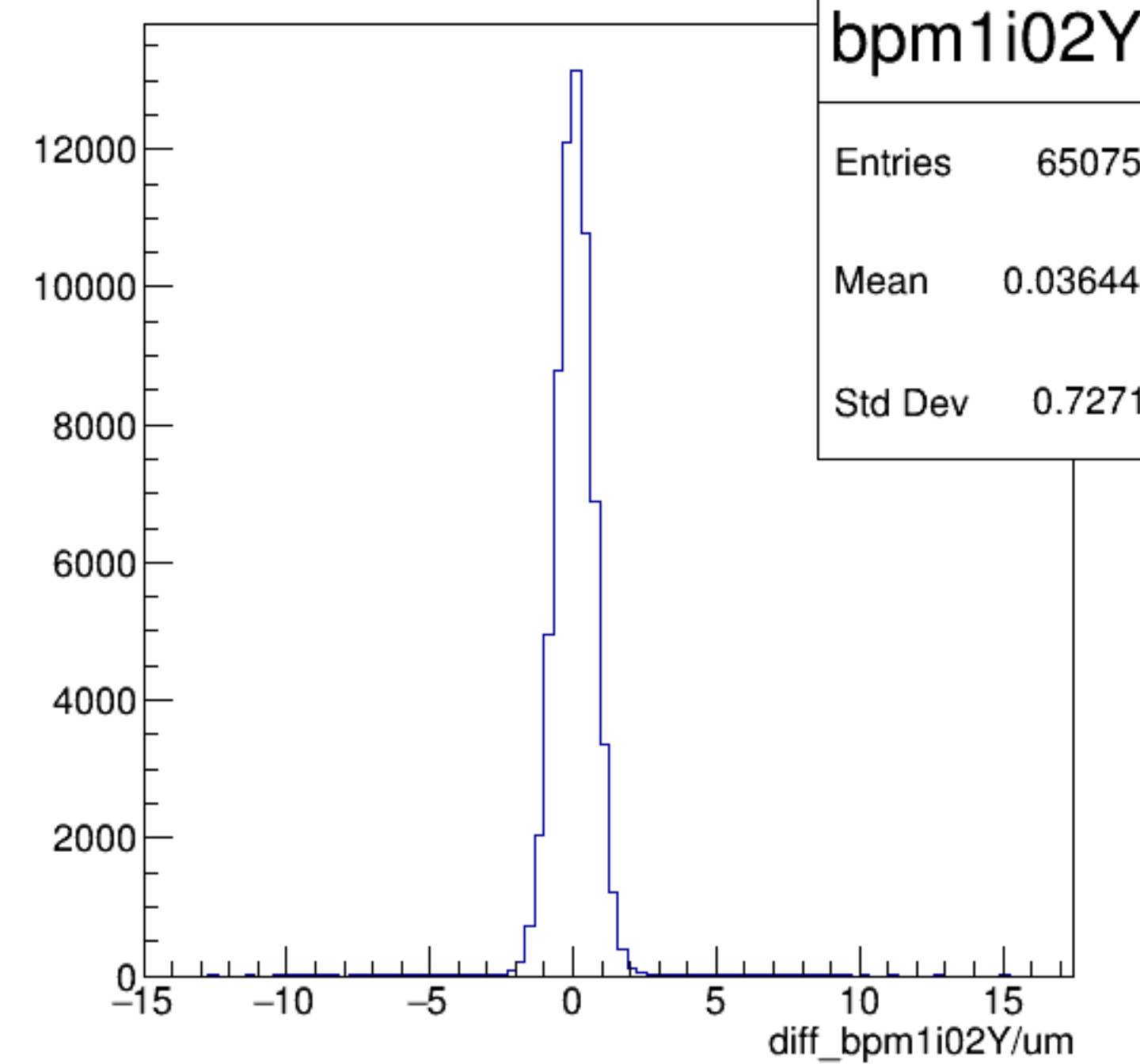
diff_bpm1i02Y/um {ErrorFlag==0}
