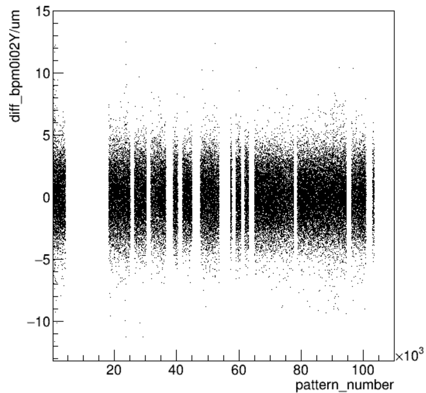
diff_bpm0i02Y/um:pattern_number {ErrorFlag==0}
