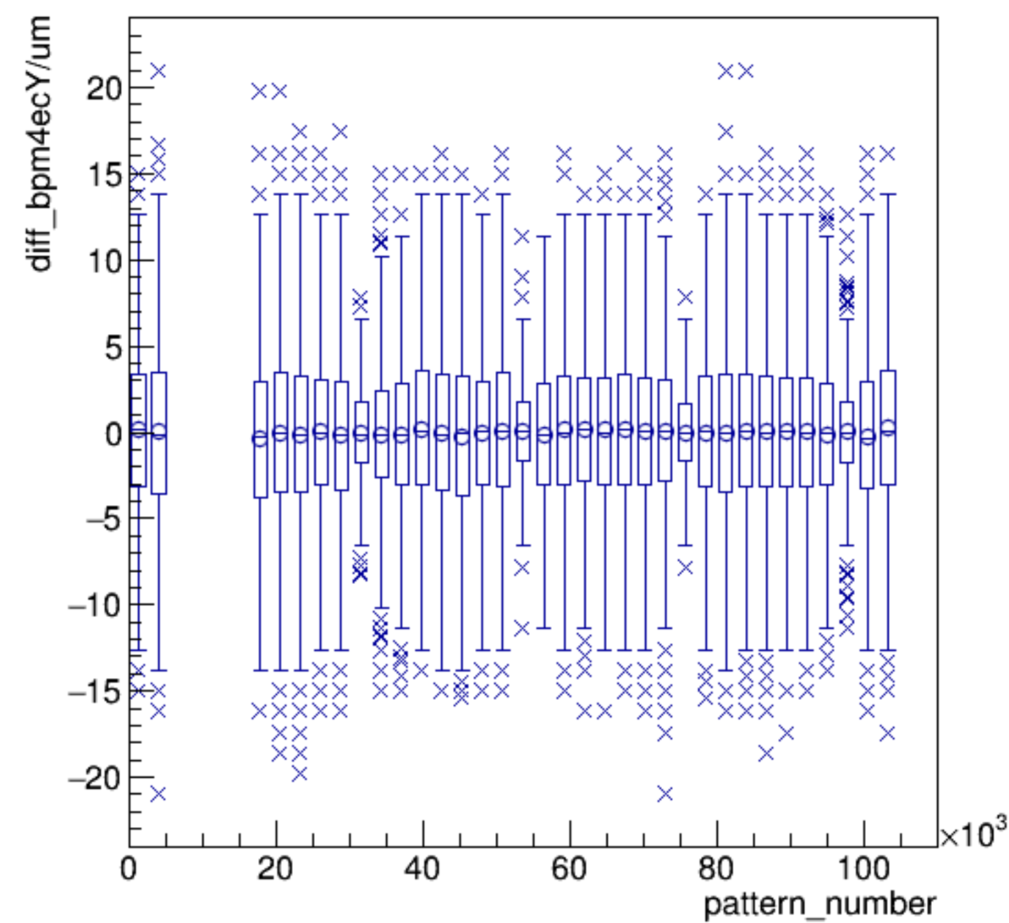
diff_bpm4ecY/um:pattern_number {ErrorFlag==0}
