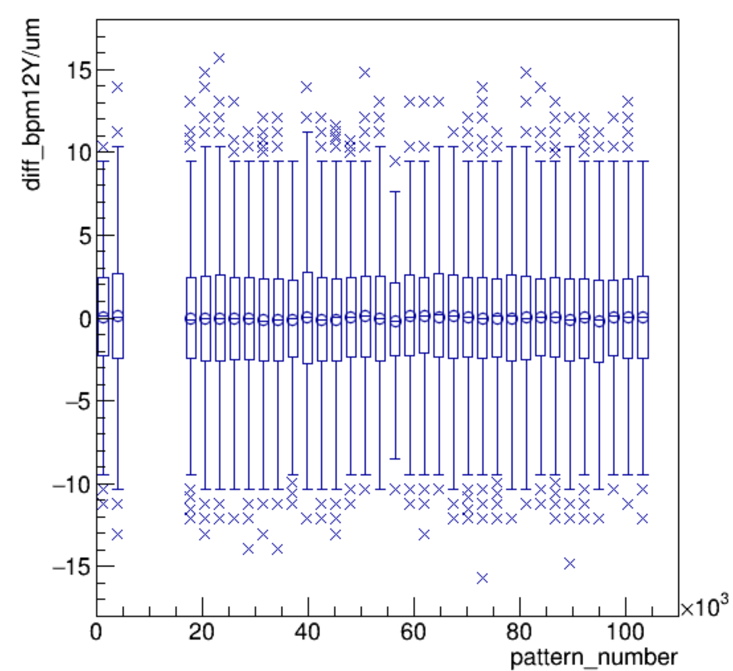
diff_bpm12Y/um:pattern_number {ErrorFlag==0}
