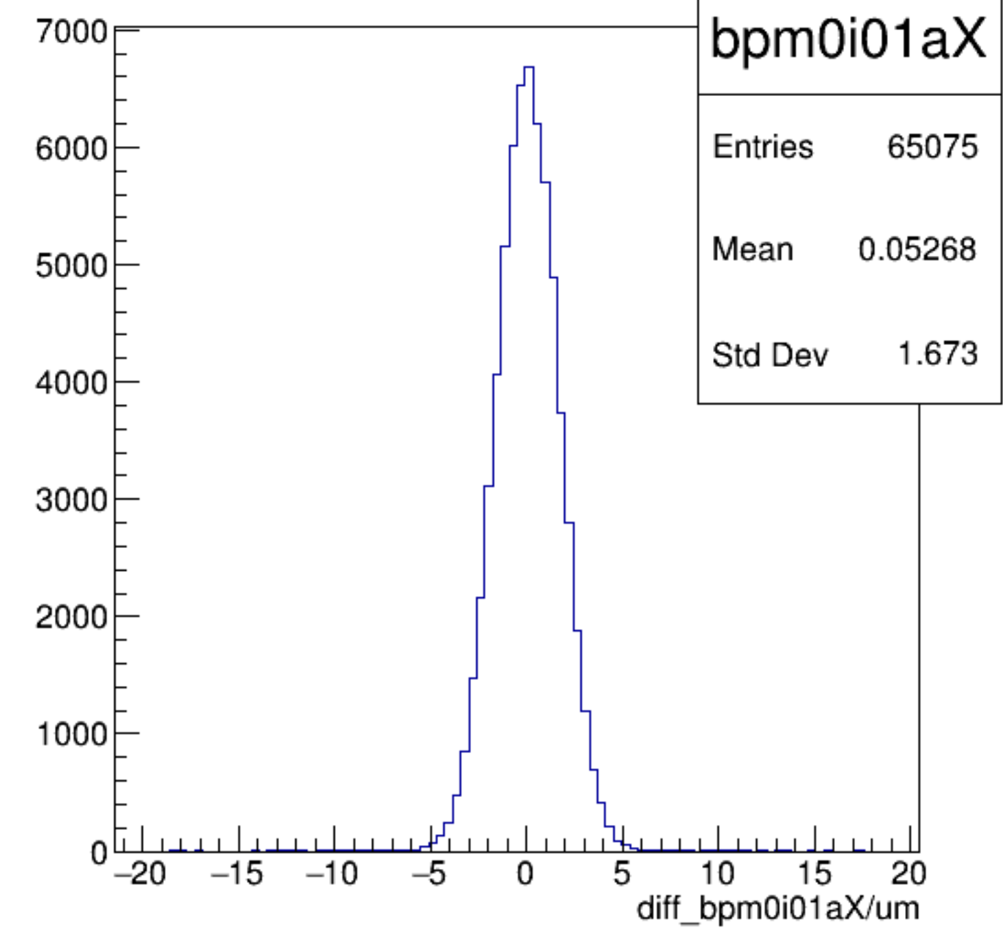
diff_bpm0i01aX/um {ErrorFlag==0}
