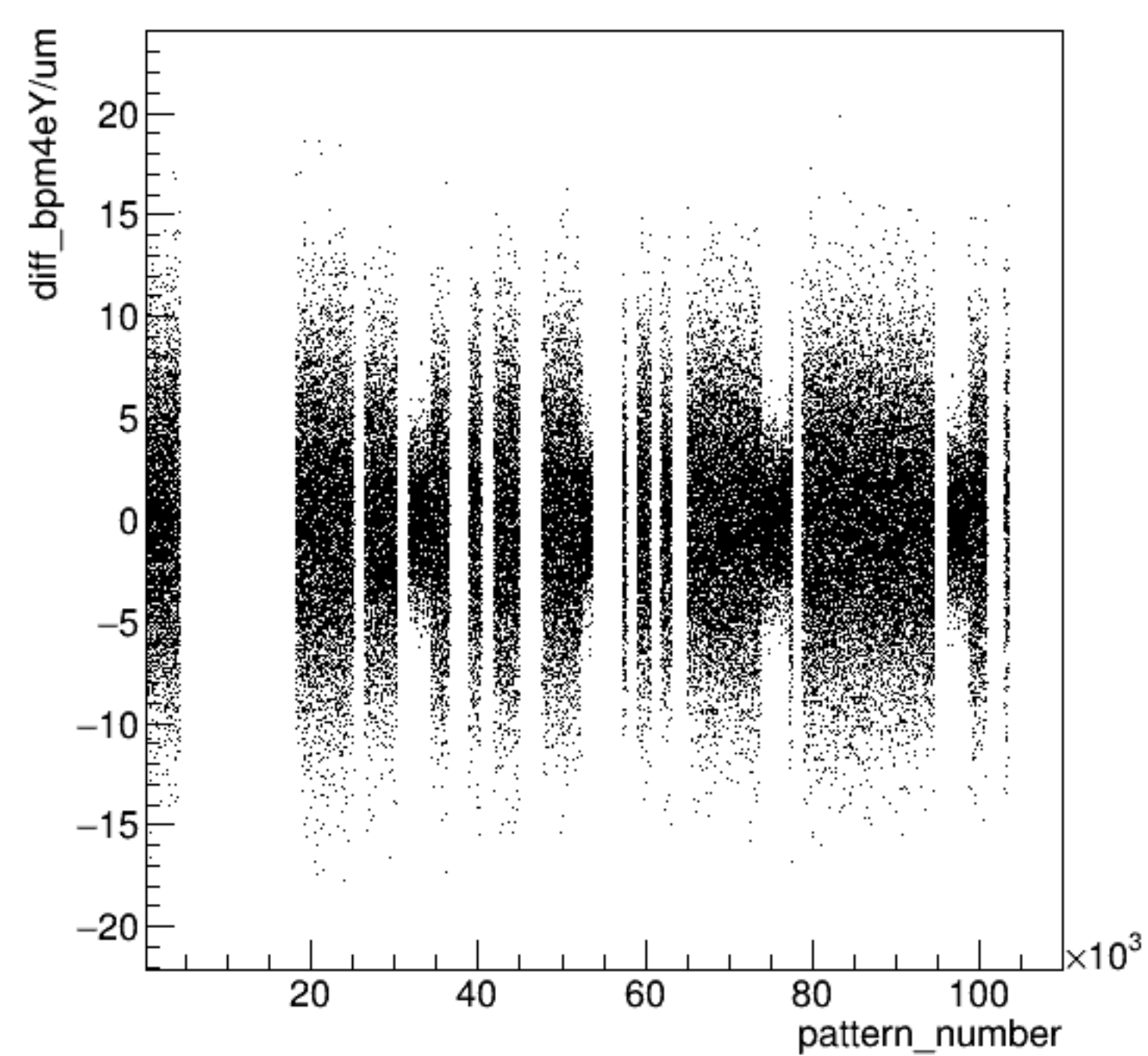
diff_bpm4eY/um:pattern_number {ErrorFlag==0}
