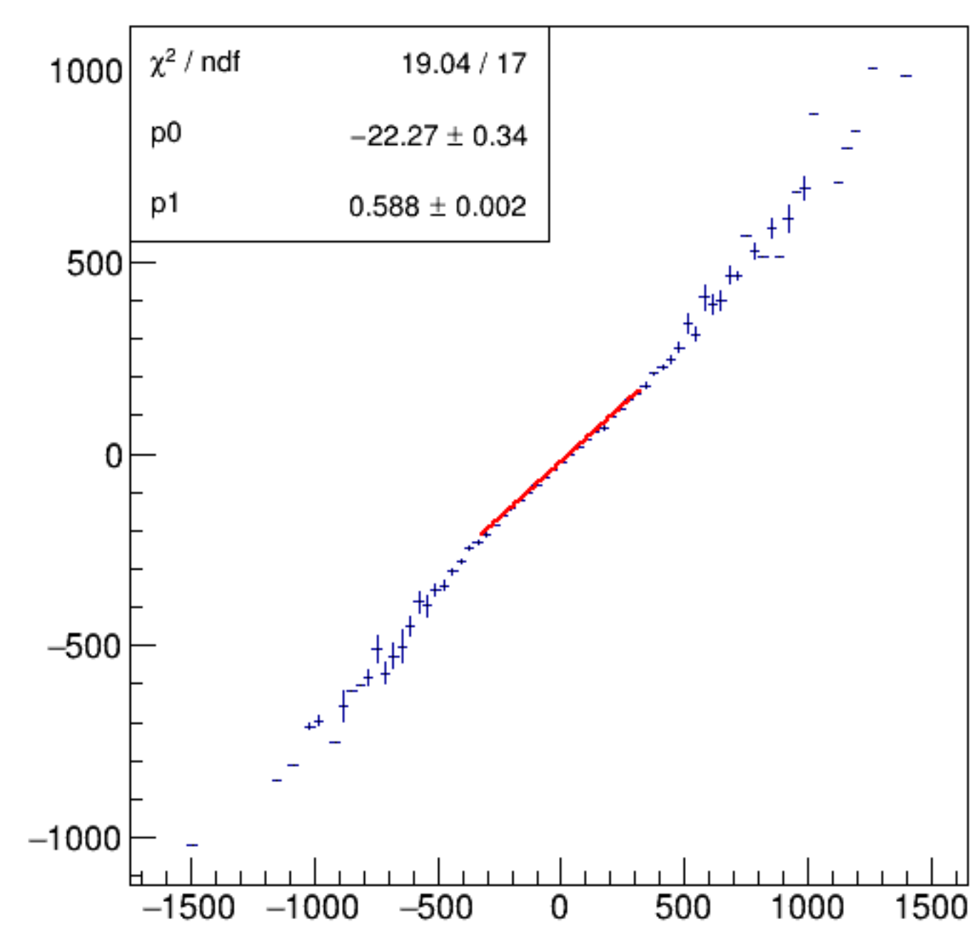
asym_bpm0i01aWS/ppm:Aq/ppm {ErrorFlag==0}
