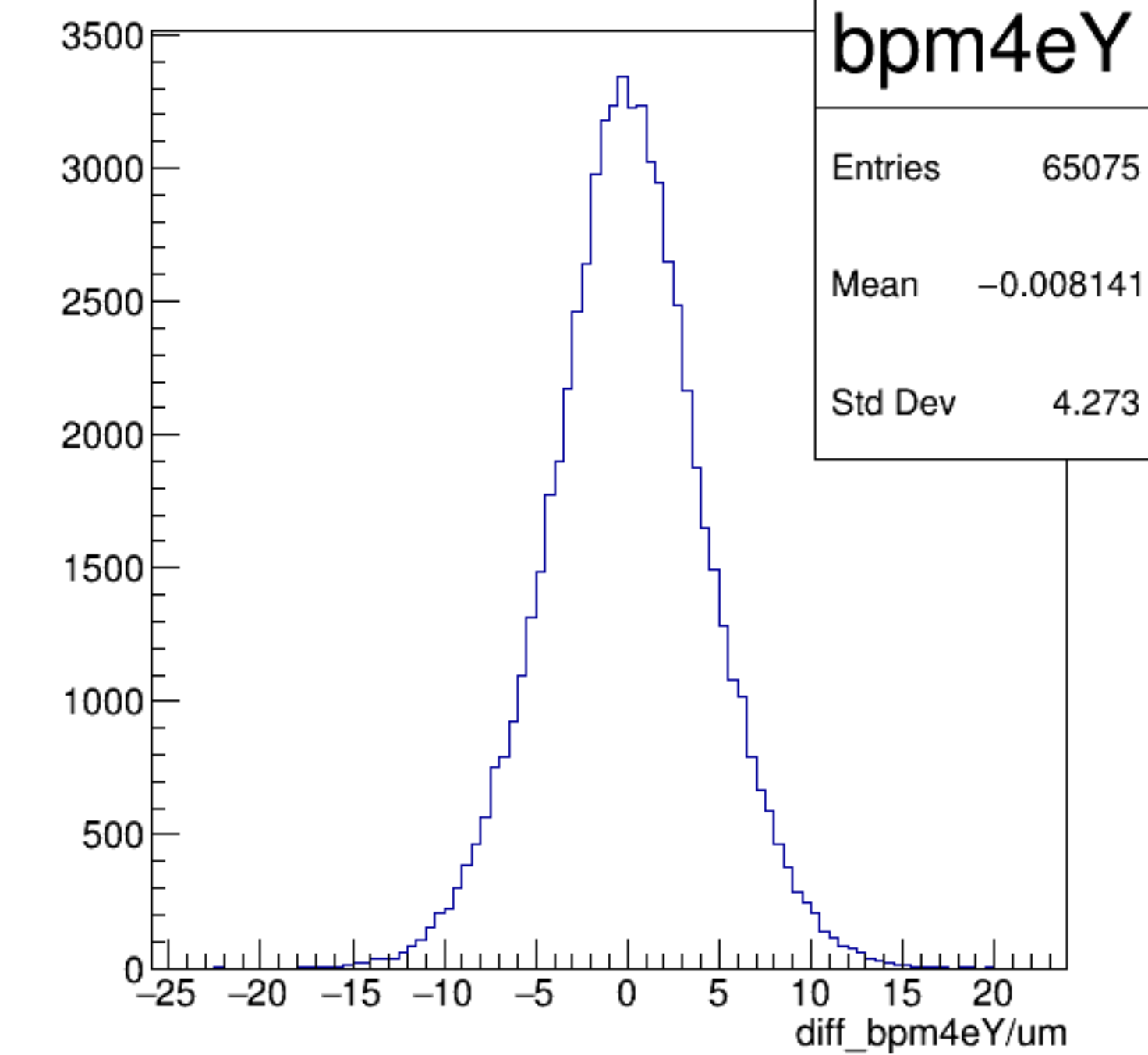
diff_bpm4eY/um {ErrorFlag==0}
