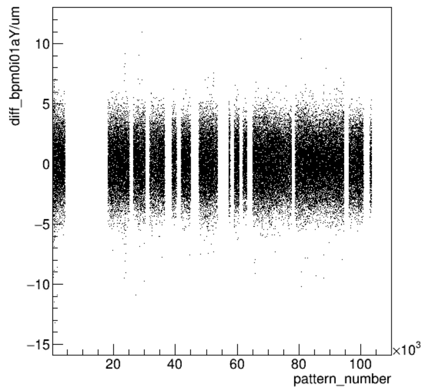
diff_bpm0i01aY/um:pattern_number {ErrorFlag==0}
