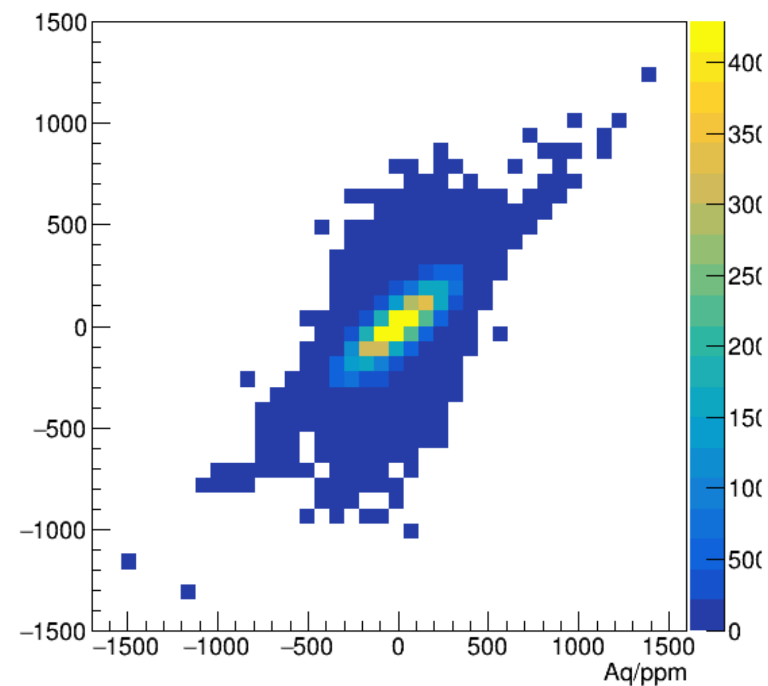
asym_bpm0l01WS/ppm:Aq/ppm {ErrorFlag==0}
