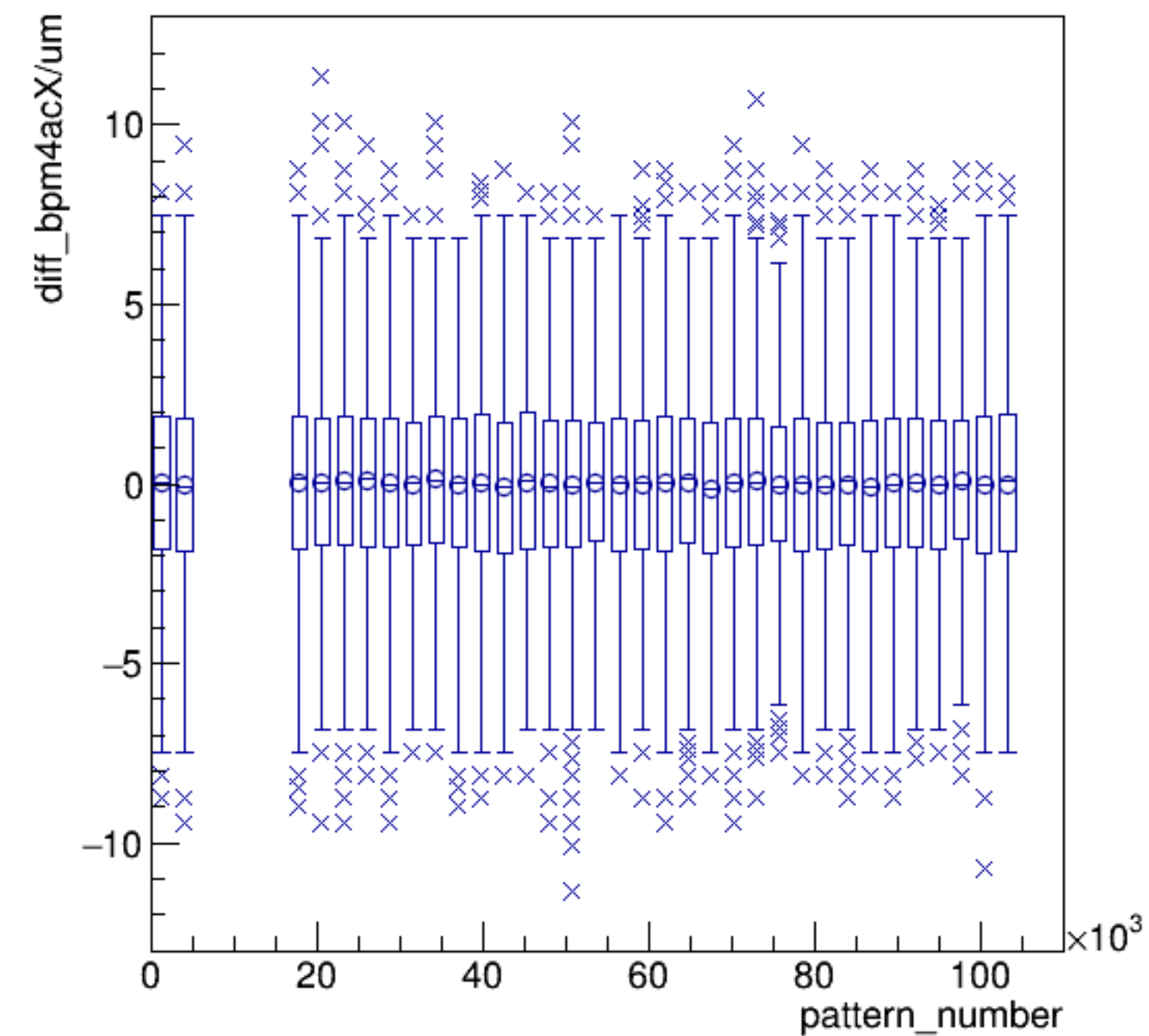
diff_bpm4acX/um:pattern_number {ErrorFlag==0}
