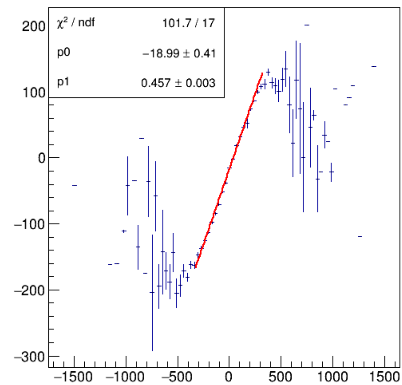
asym_bpm2i01WS/ppm:Aq/ppm {ErrorFlag==0}
