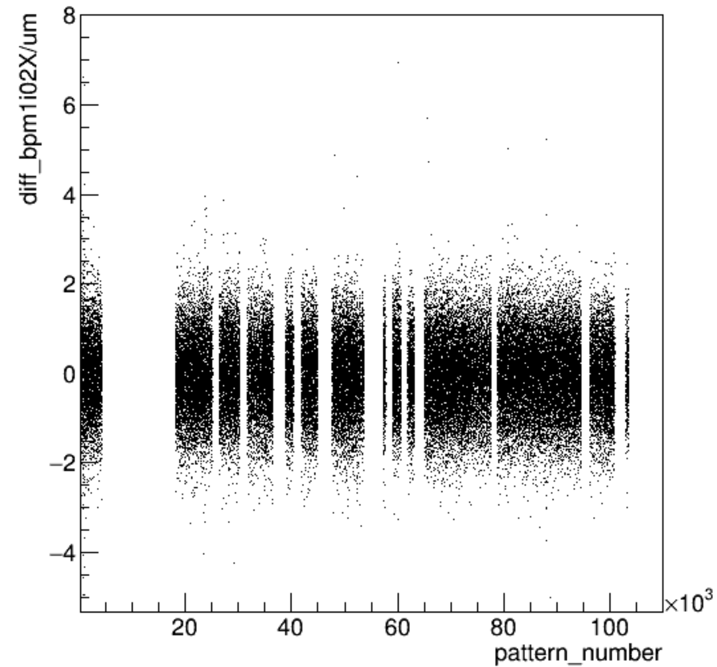
diff_bpm1i02X/um:pattern_number {ErrorFlag==0}
