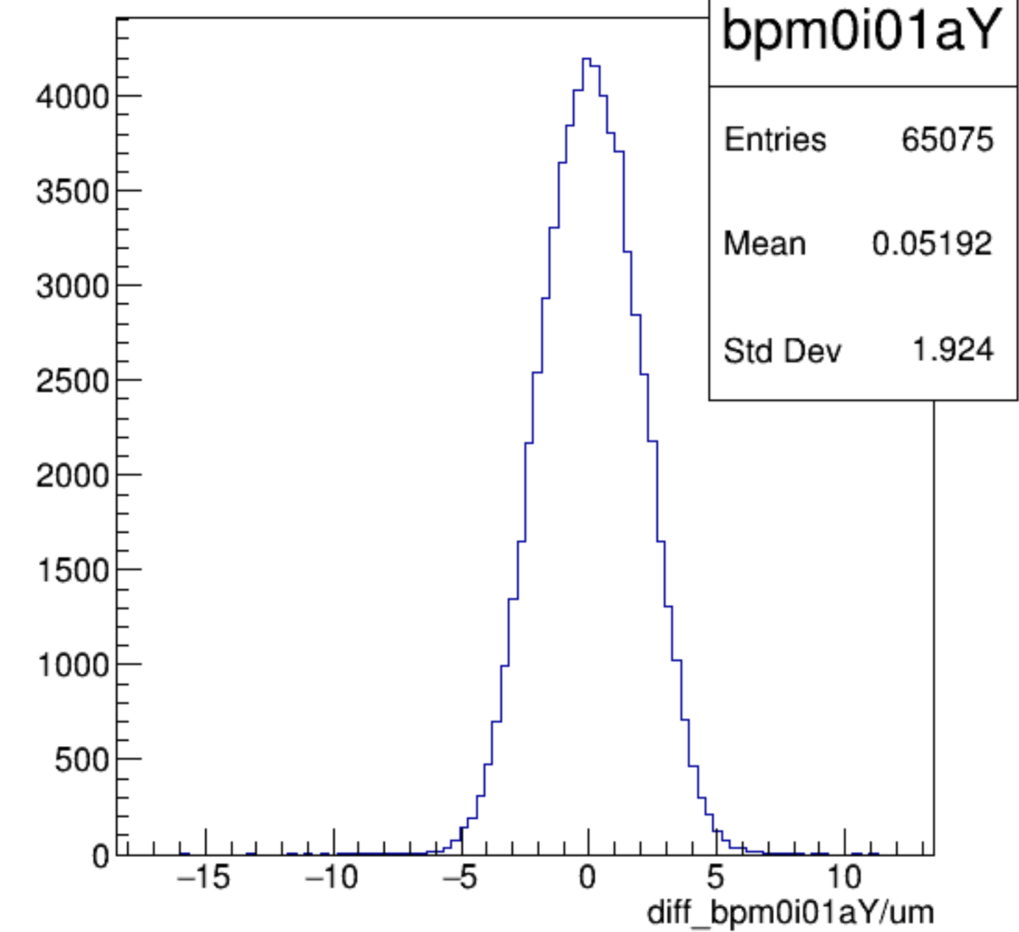
diff_bpm0i01aY/um {ErrorFlag==0}
