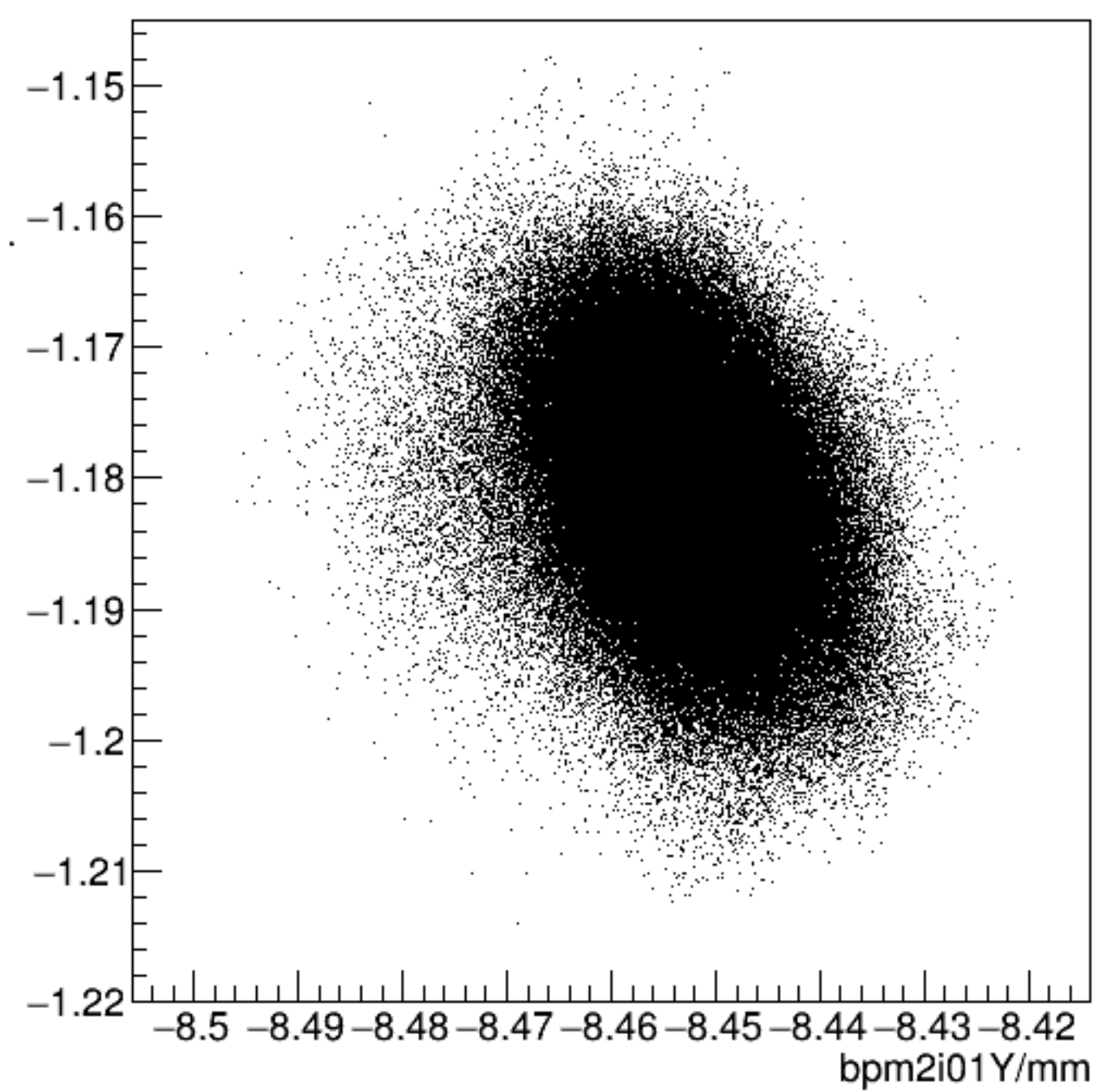
bpm2i01X/mm:bpm2i01Y/mm {ErrorFlag==0}
