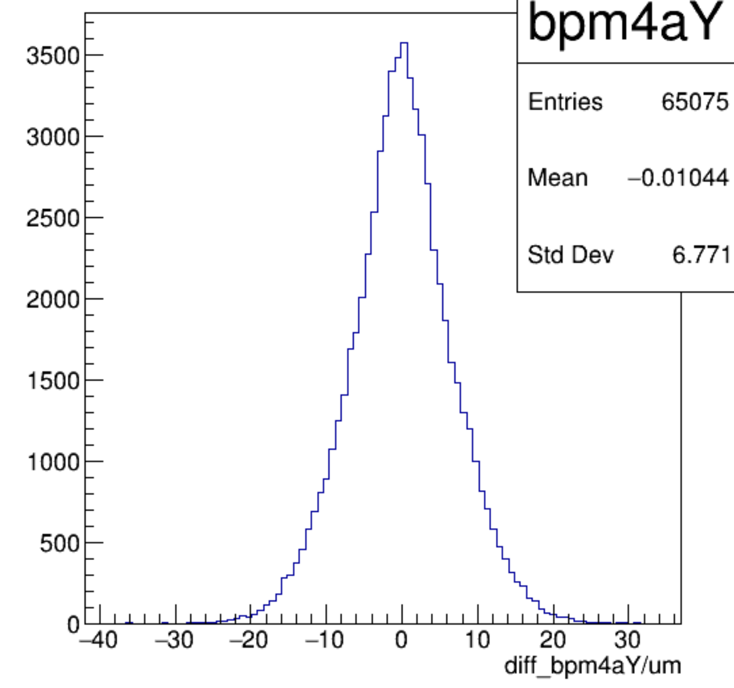
diff_bpm4aY/um {ErrorFlag==0}
