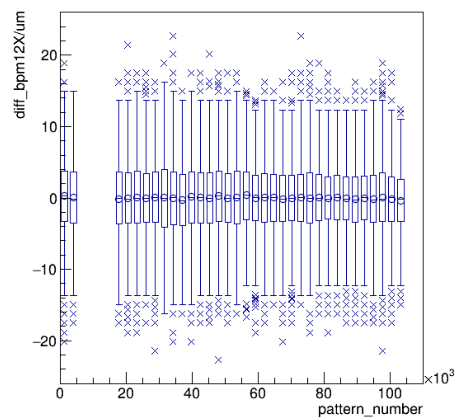
diff_bpm12X/um:pattern_number {ErrorFlag==0}
