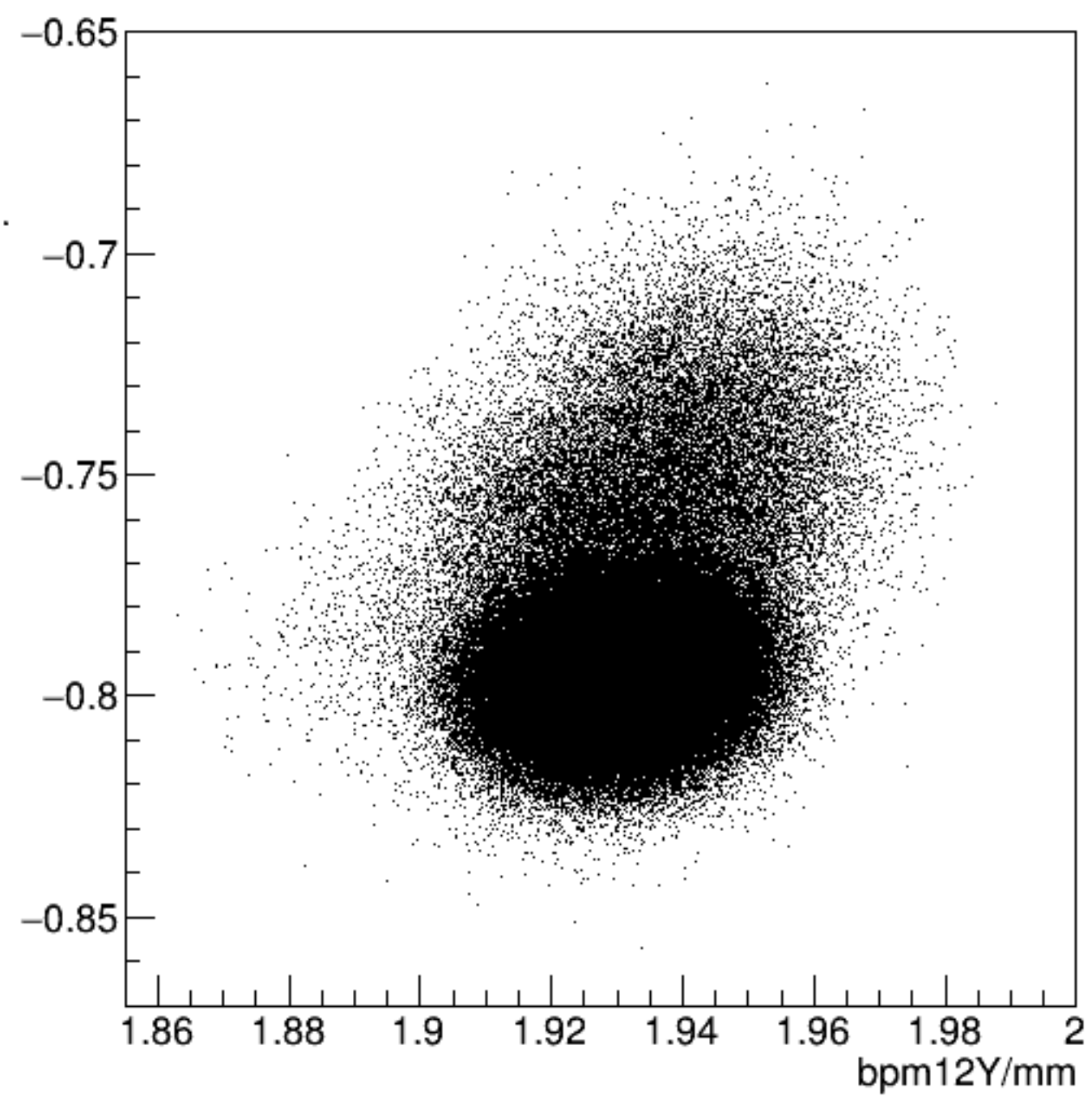
bpm12X/mm:bpm12Y/mm {ErrorFlag==0}
