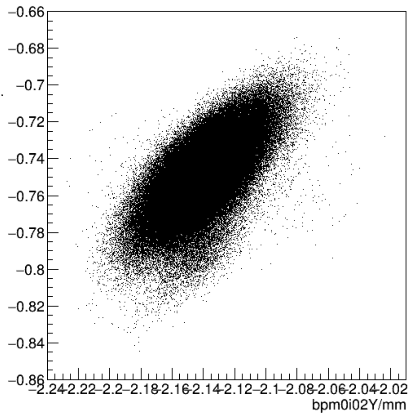
bpm0i02X/mm:bpm0i02Y/mm {ErrorFlag==0}
