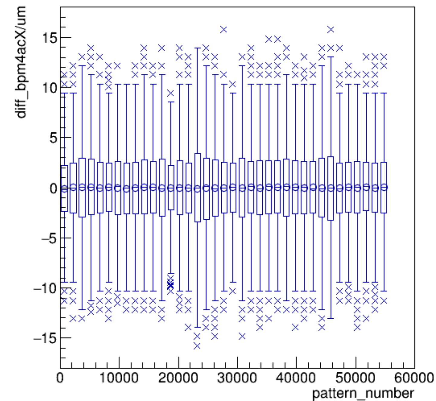
diff_bpm4acX/um:pattern_number {ErrorFlag==0}
