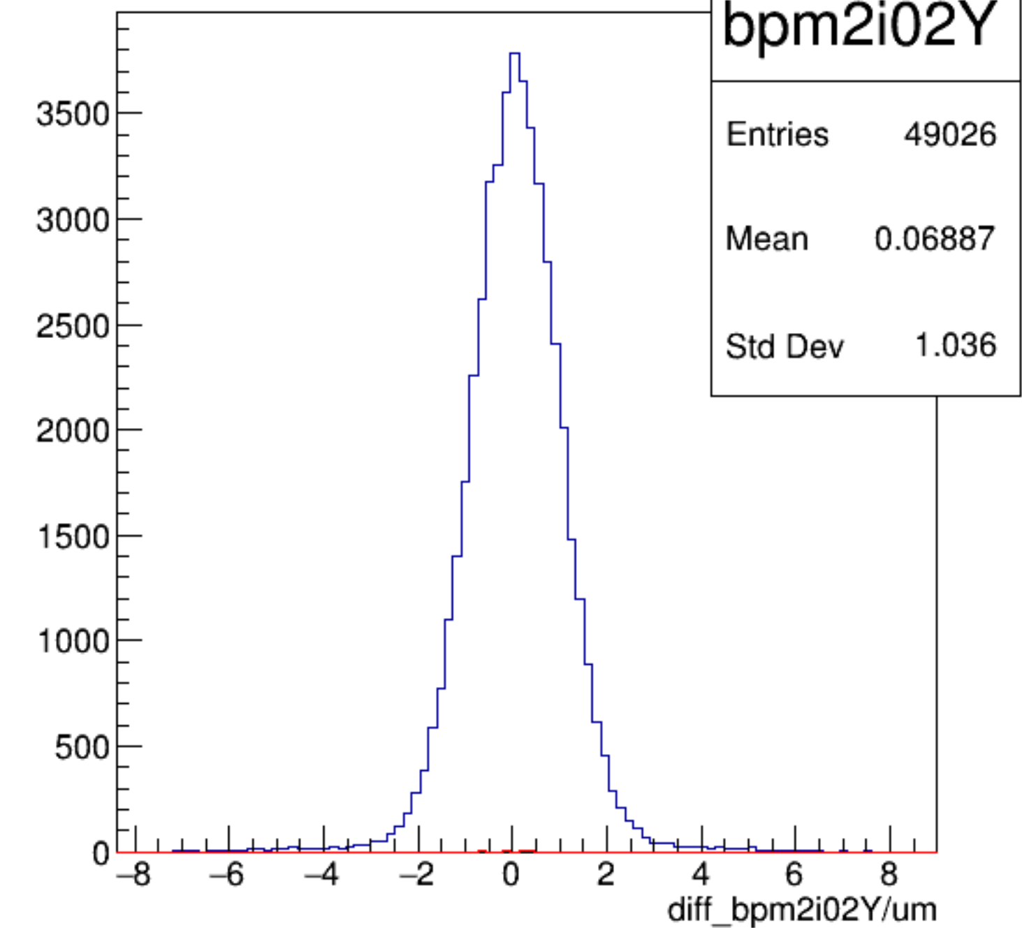
diff_bpm2i02Y/um {ErrorFlag==0}
