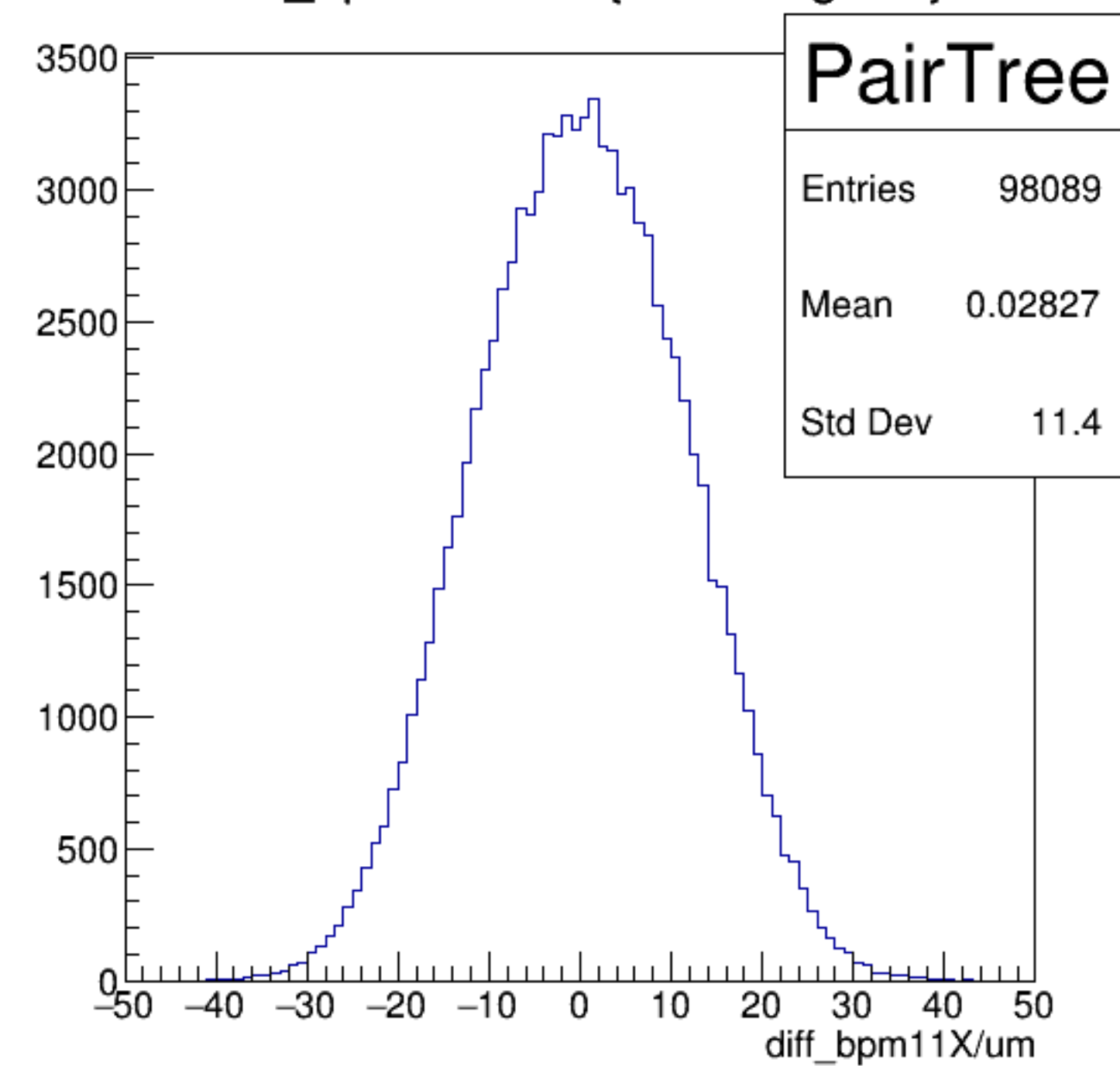
diff_bpm11X/um {ErrorFlag==0}
