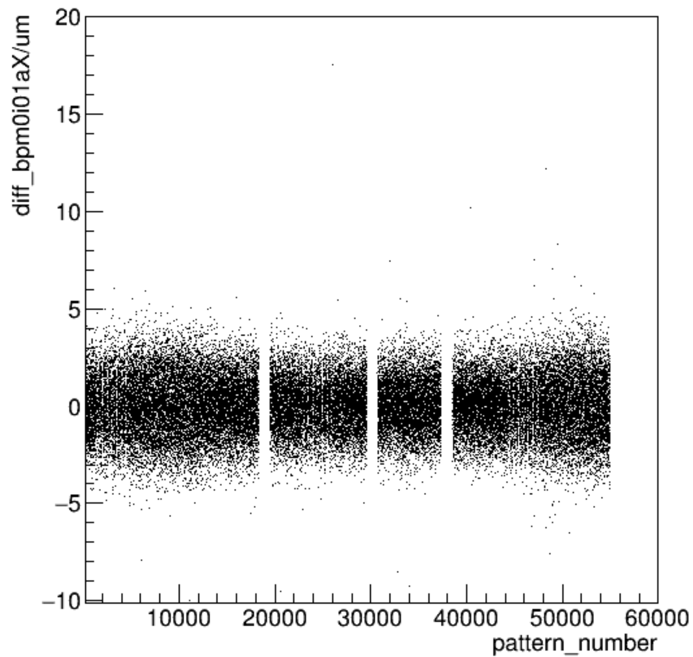
diff_bpm0i01aX/um:pattern_number {ErrorFlag==0}
