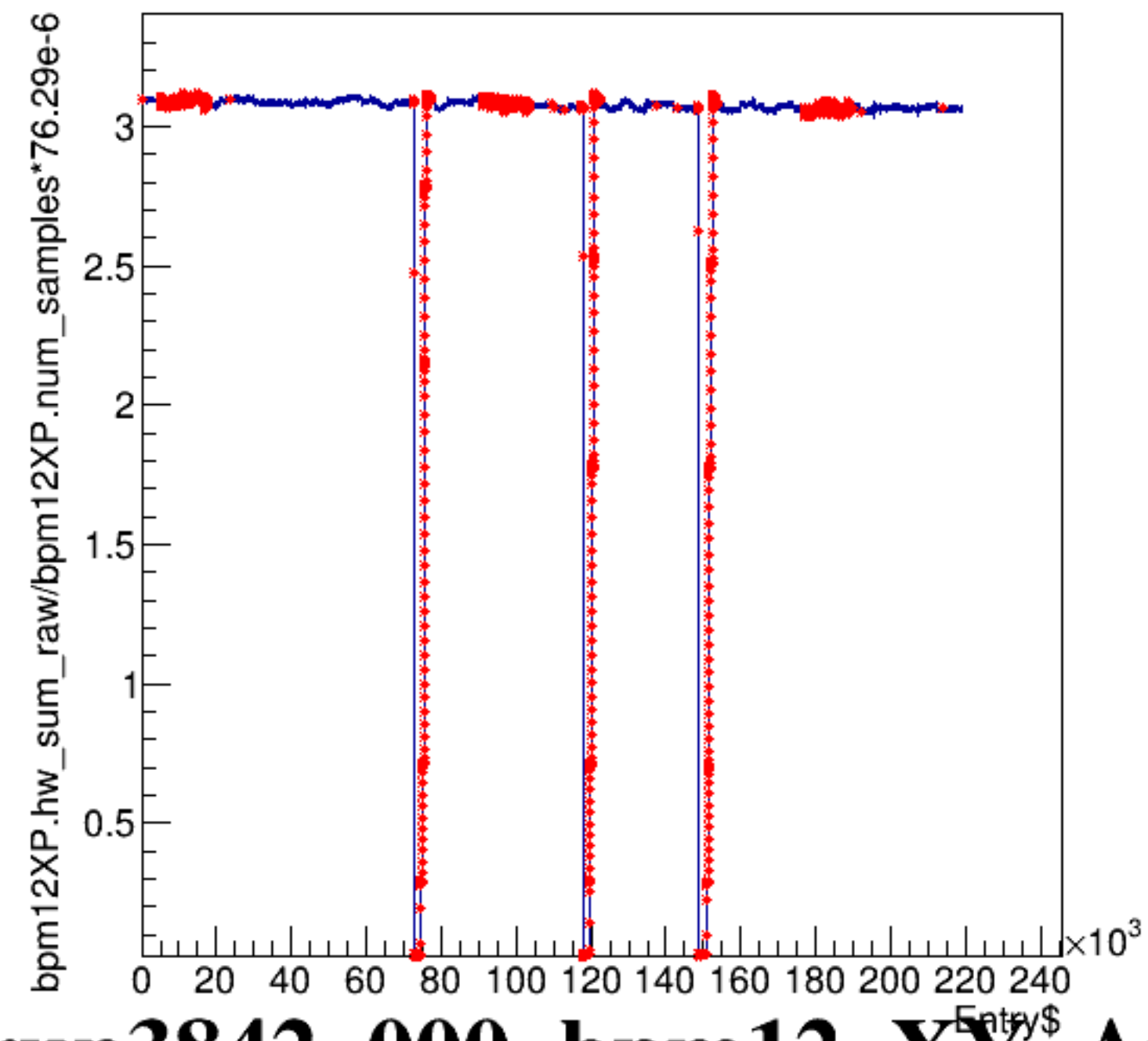
bpm12XP.hw_sum_raw/bpm12XP.num_samples*76.29e-6:Entry$
