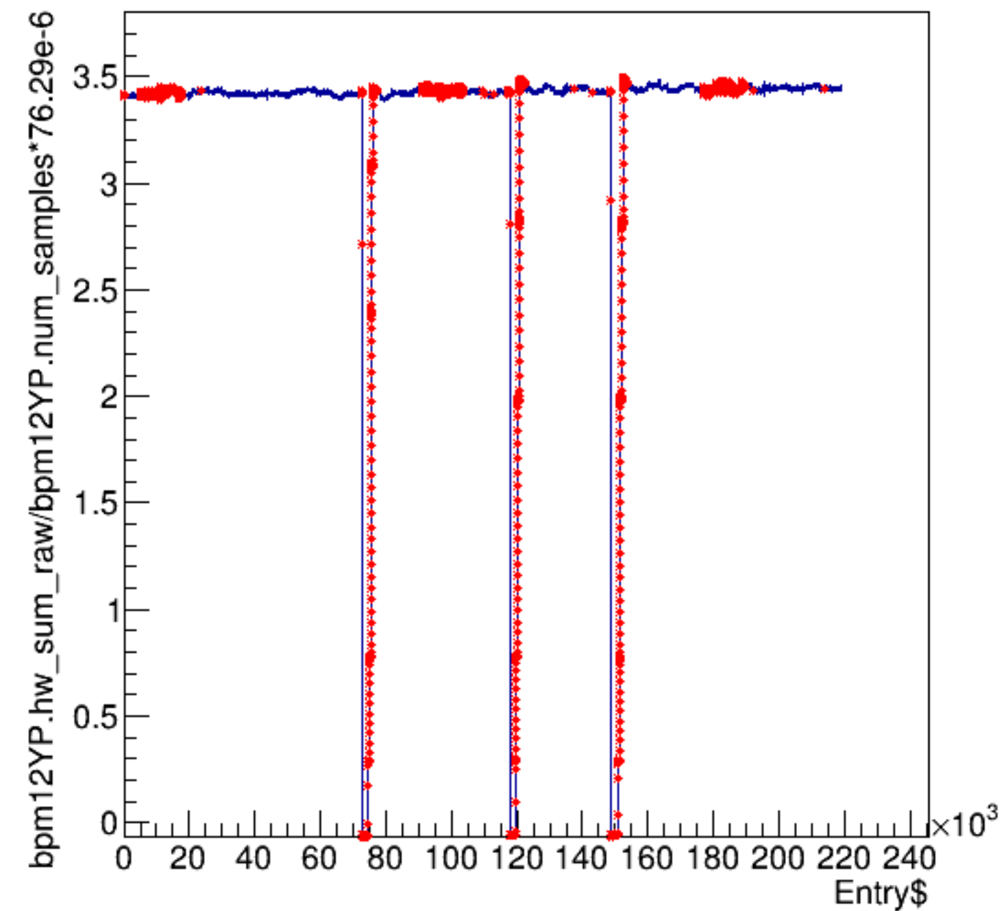
bpm12YP.hw_sum_raw/bpm12YP.num_samples*76.29e-6:Entry$
