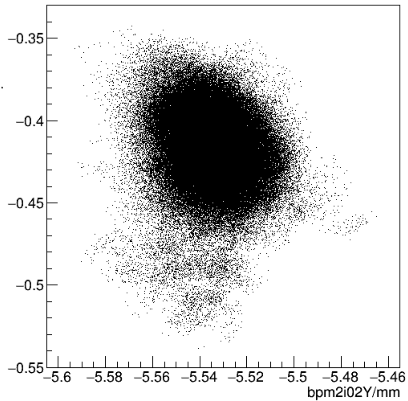
bpm2i02X/mm:bpm2i02Y/mm {ErrorFlag==0}
