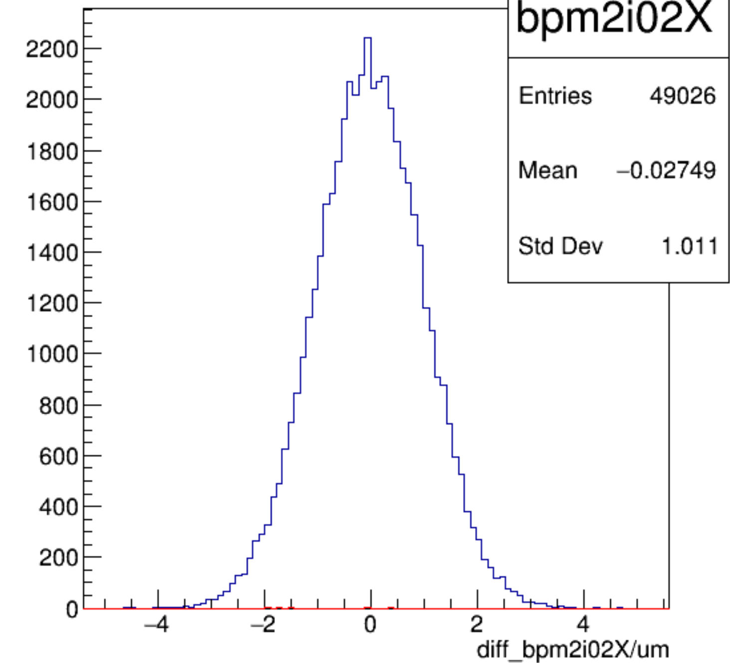
diff_bpm2i02X/um {ErrorFlag==0}
