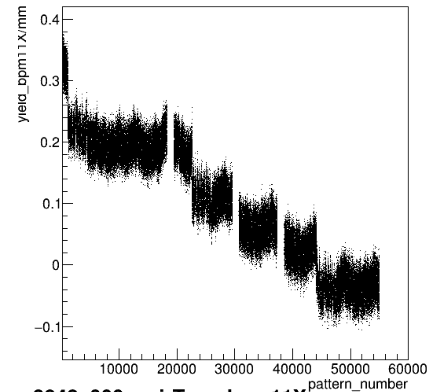
yield_bpm11X/mm:pattern_number {ErrorFlag==0}
