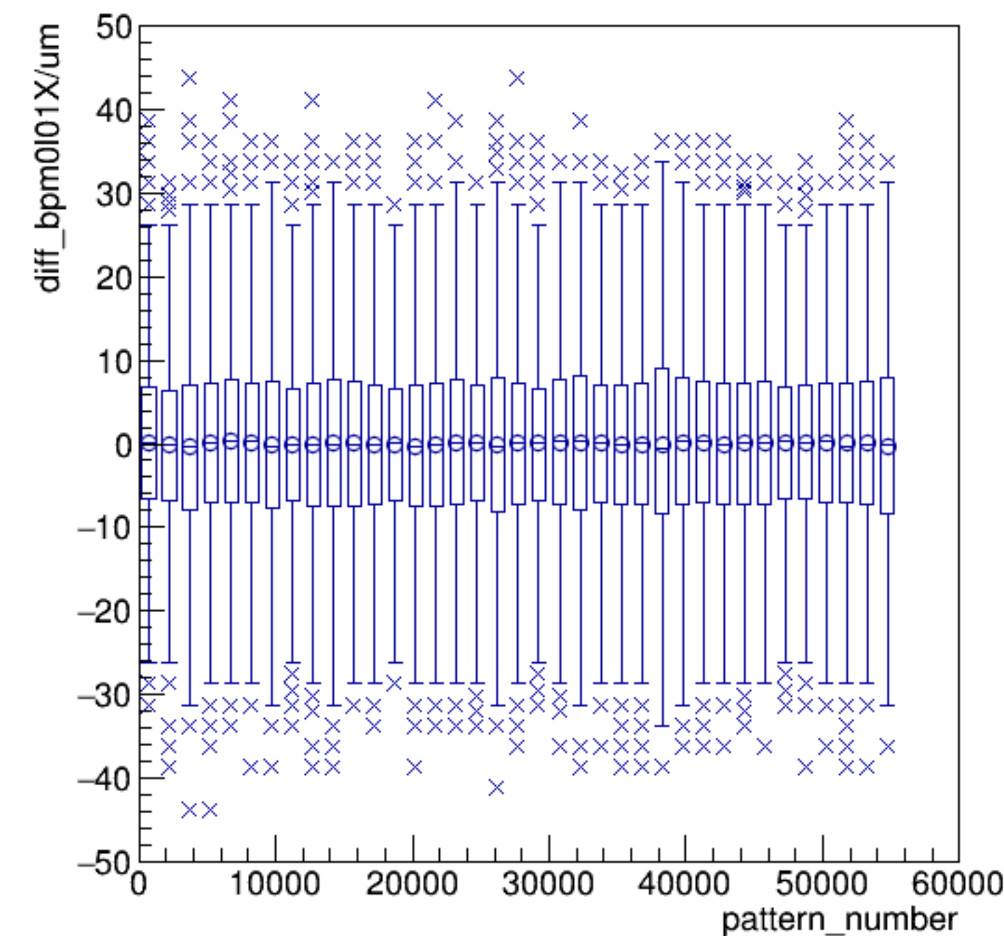
diff_bpm0l01X/um:pattern_number {ErrorFlag==0}
