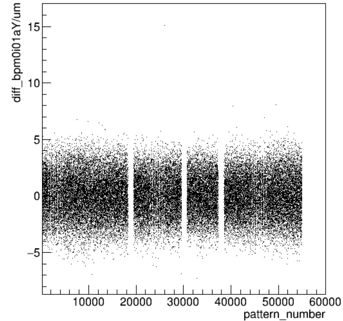
diff_bpm0i01aY/um:pattern_number {ErrorFlag==0}
