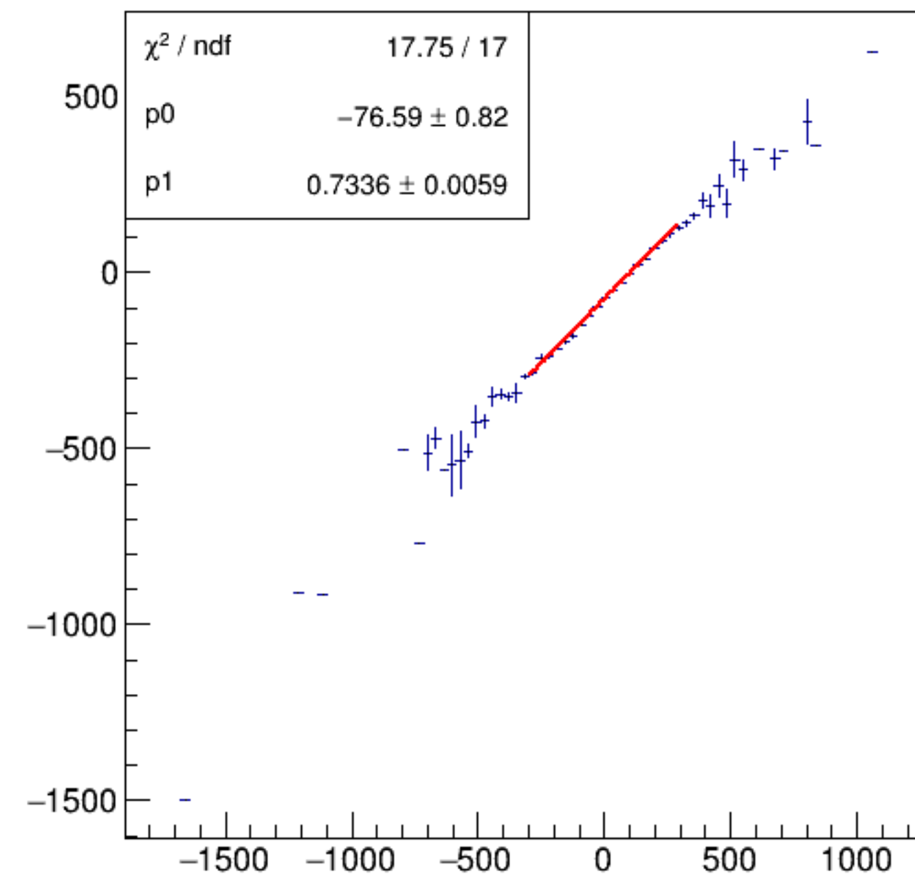
asym_bpm0i02WS/ppm:Aq/ppm {ErrorFlag==0}
