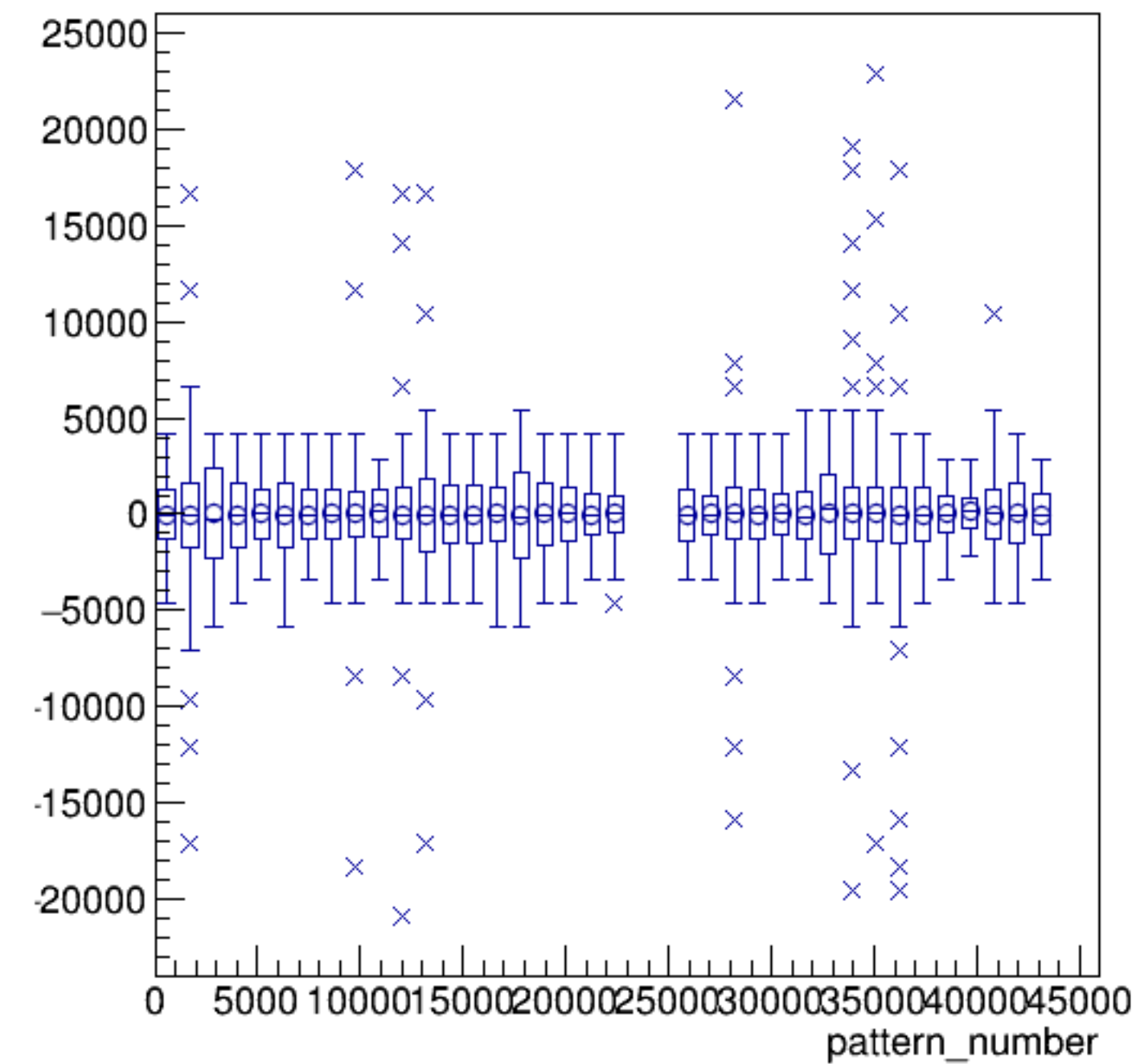
asym_usl/ppm:pattern_number {ErrorFlag==0}
