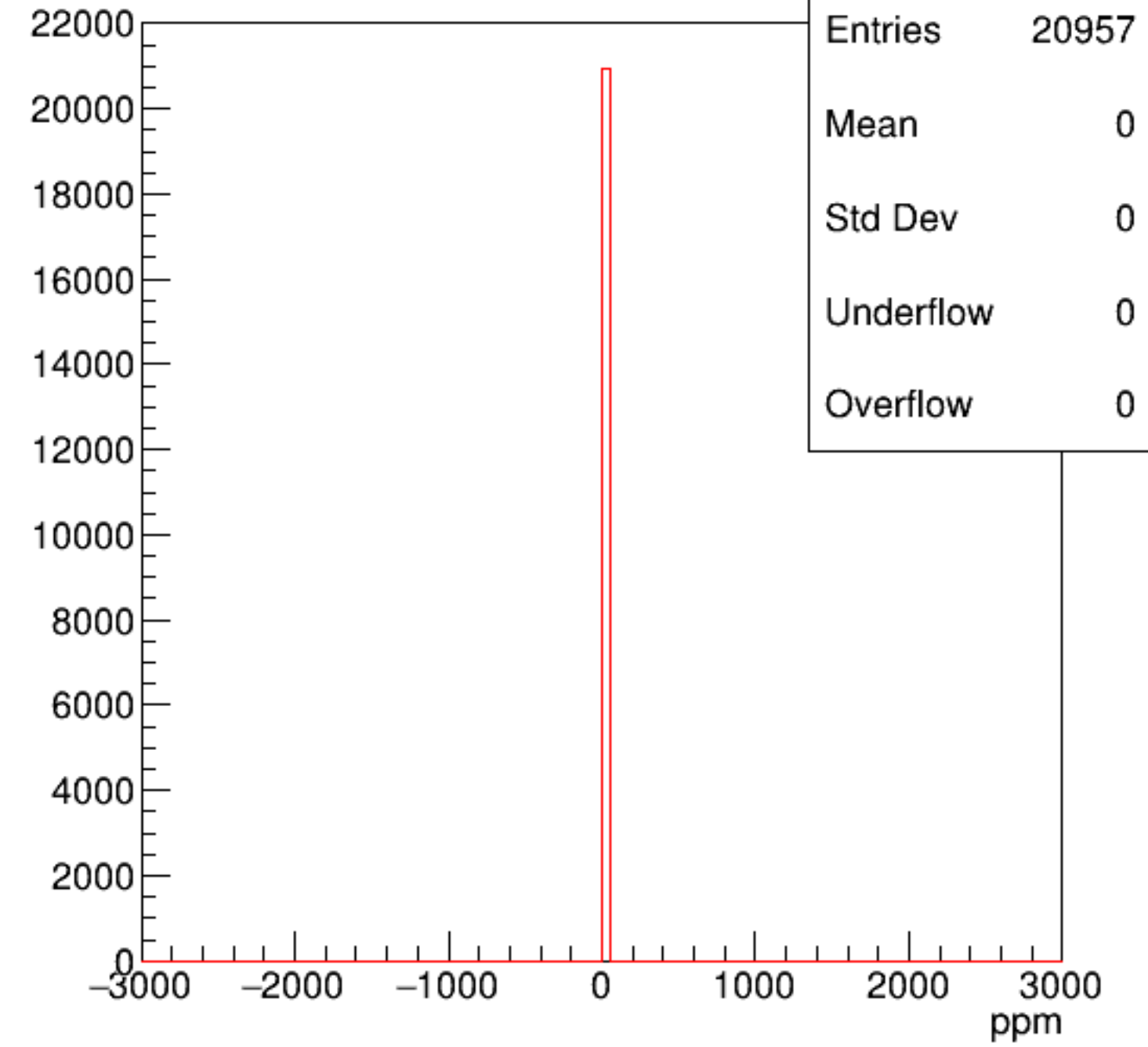
asym_usr
