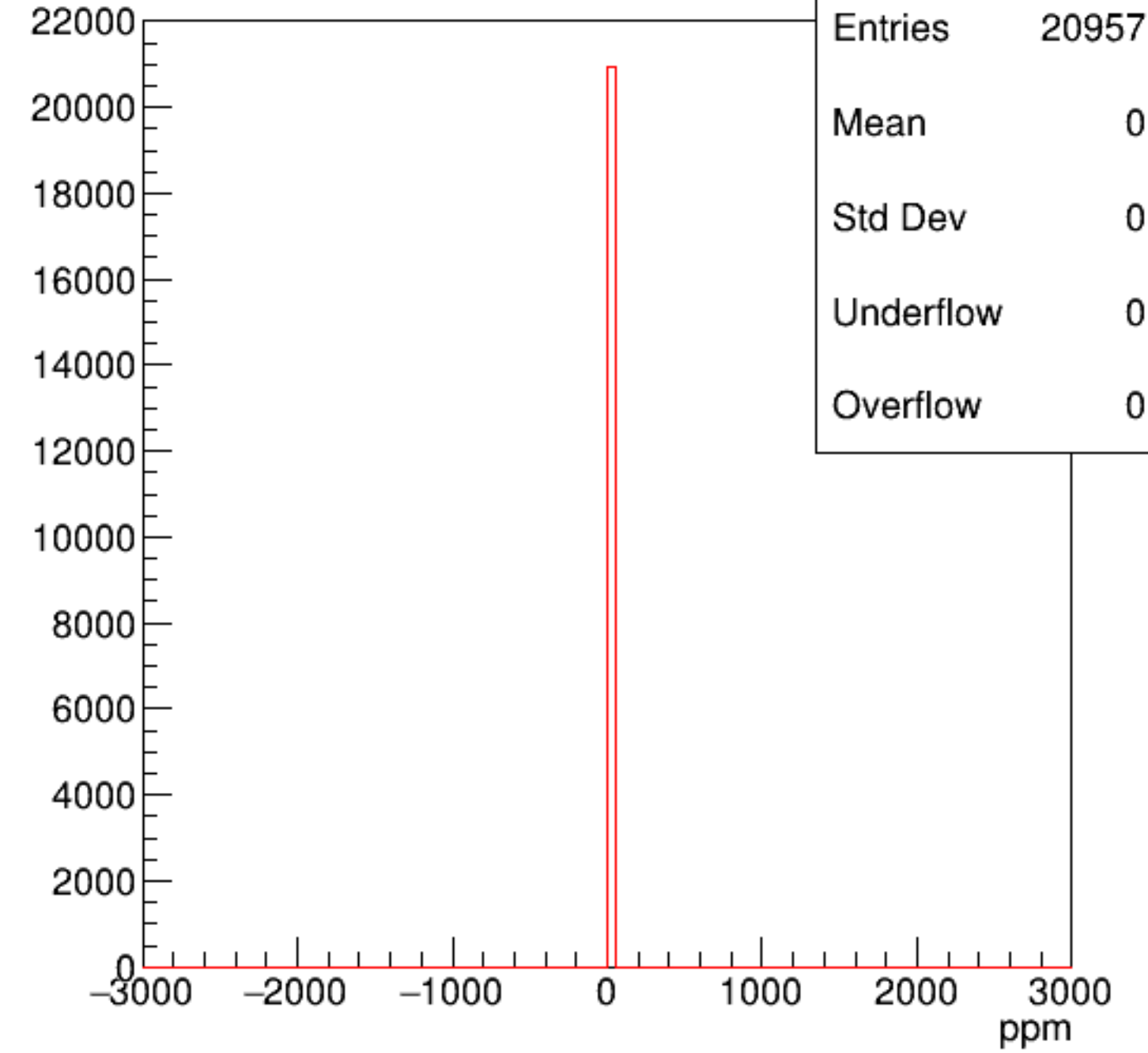
asym_dsr
