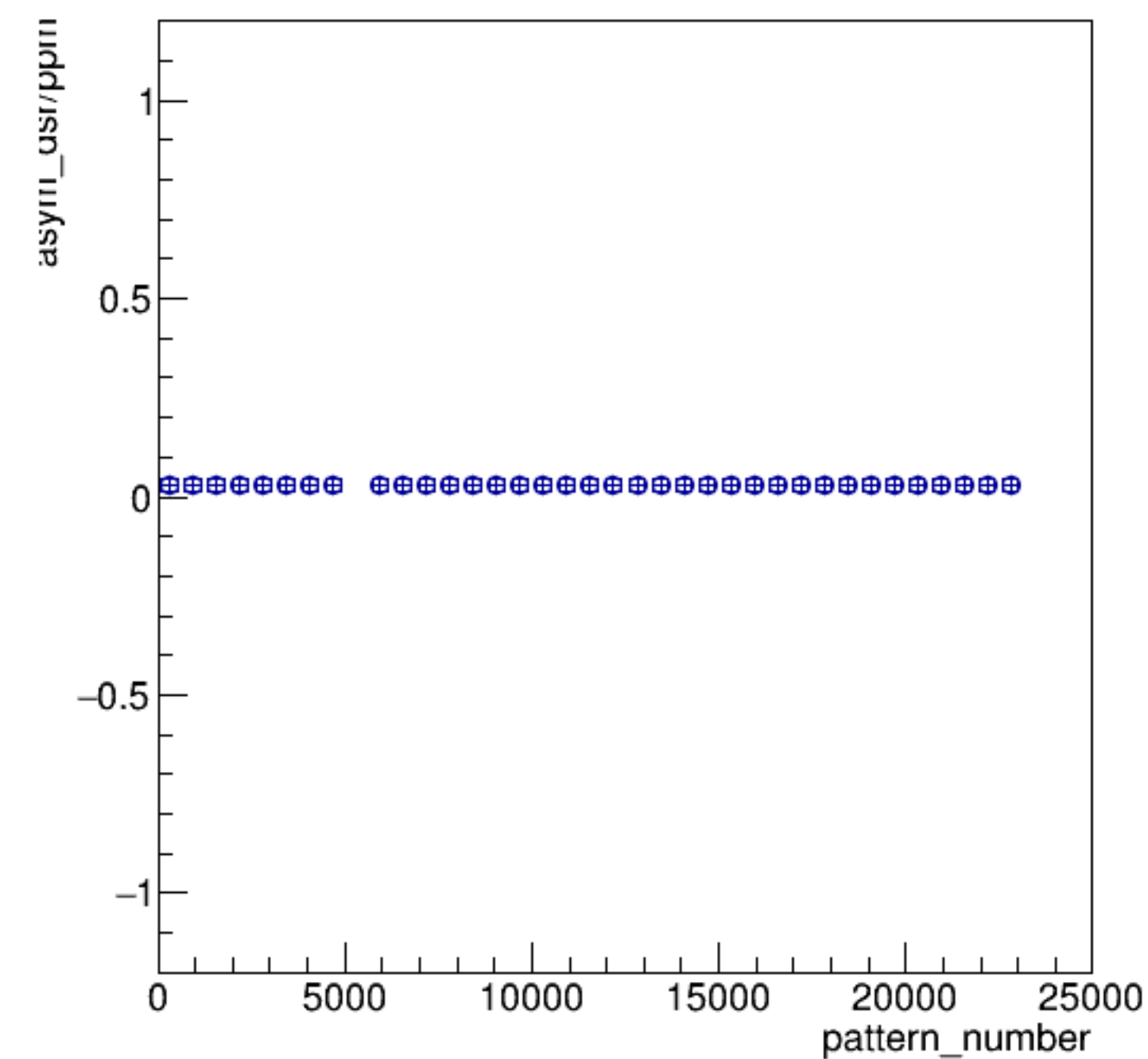
asym_dsr/ppm:pattern_number {ErrorFlag==0}
