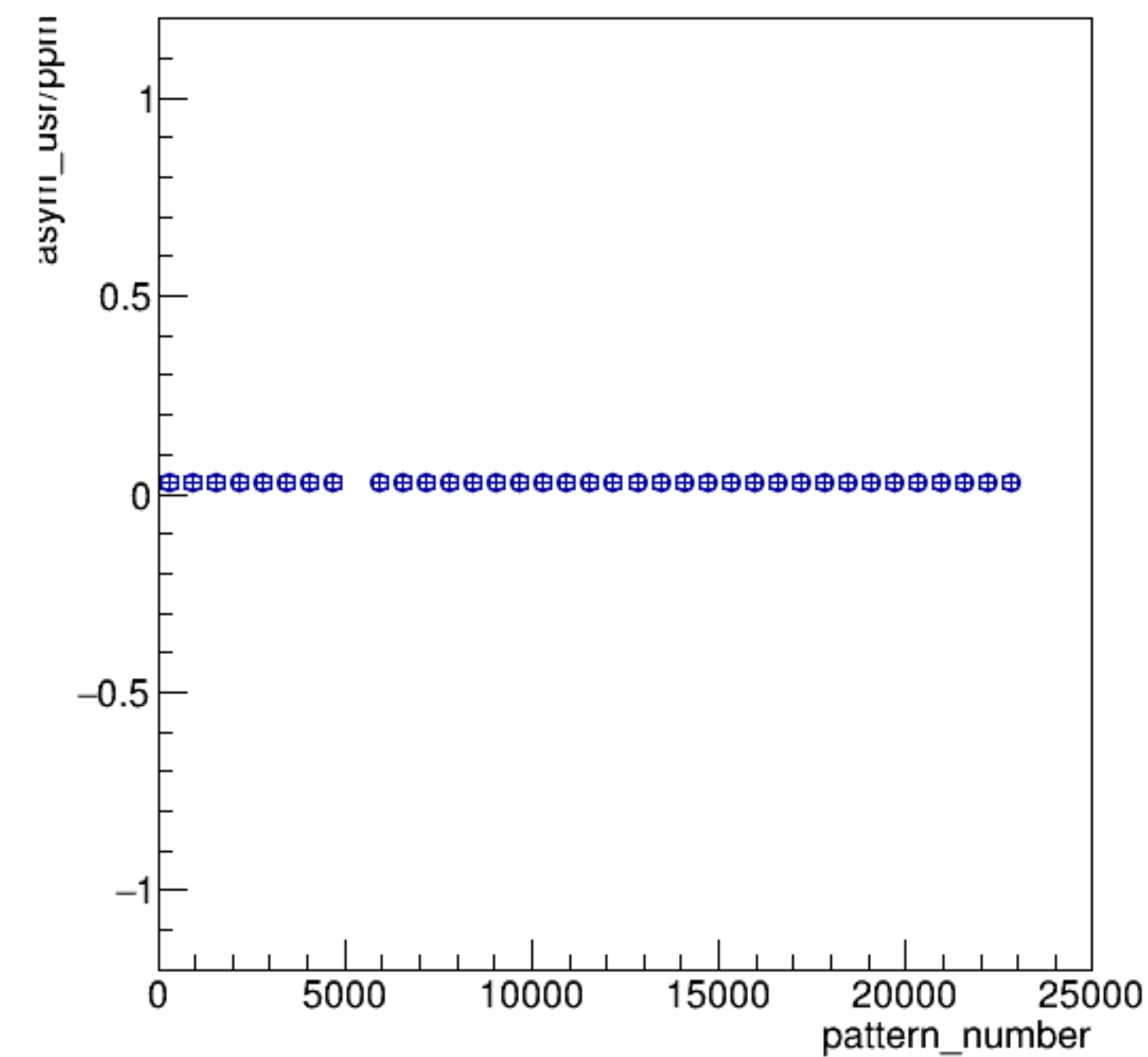
asym_usr/ppm:pattern_number {ErrorFlag==0}
