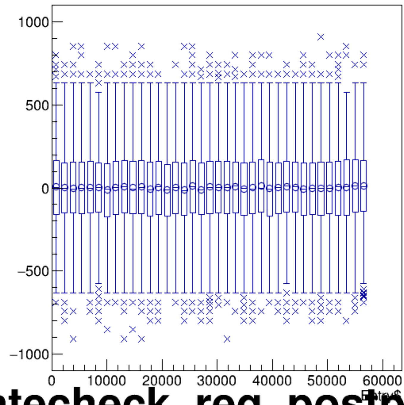
(reg_asym_atl1/ppm-reg_asym_atr1/ppm)/2:Entry$ {ok_cut}
