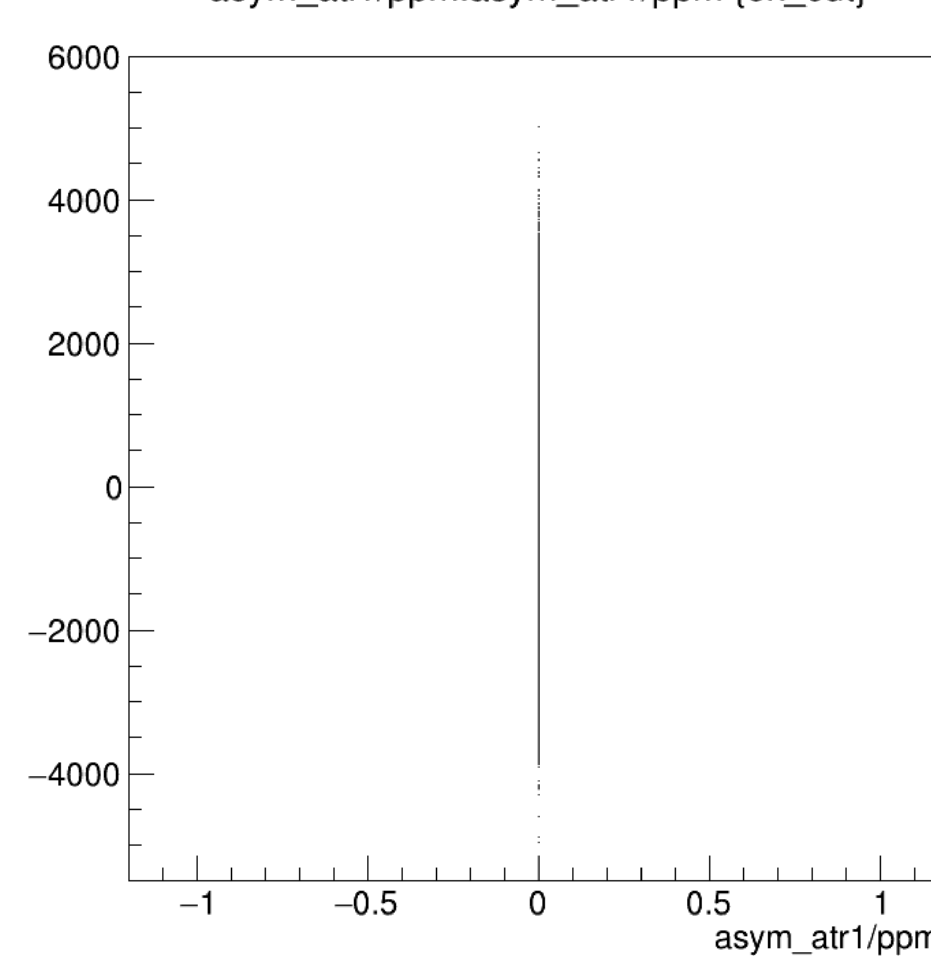
asym_atl1/ppm:asym_atr1/ppm {ok_cut}
