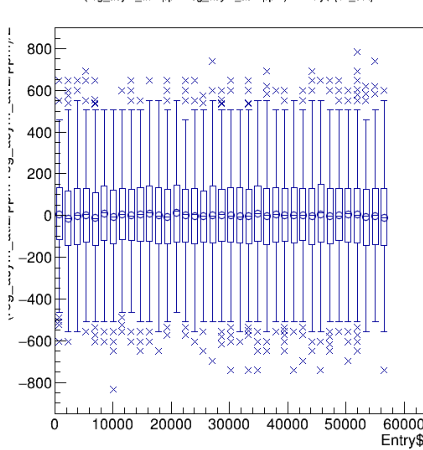
(reg_asym_atl2/ppm-reg_asym_atr2/ppm)/2:Entry$ {ok_cut}
