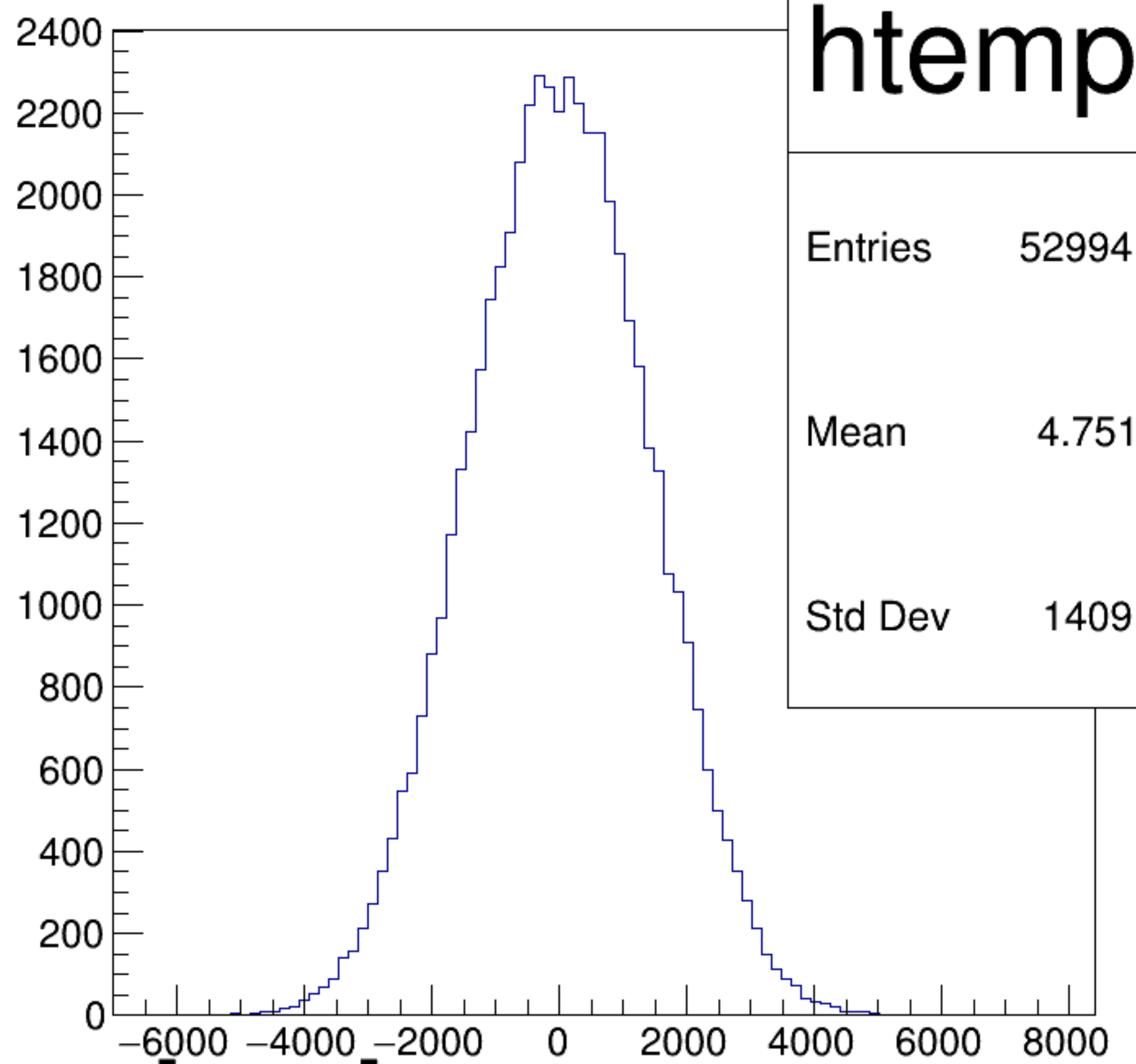
(asym_atl2/ppm+asym_atr2/ppm)/2 {ok_cut}
