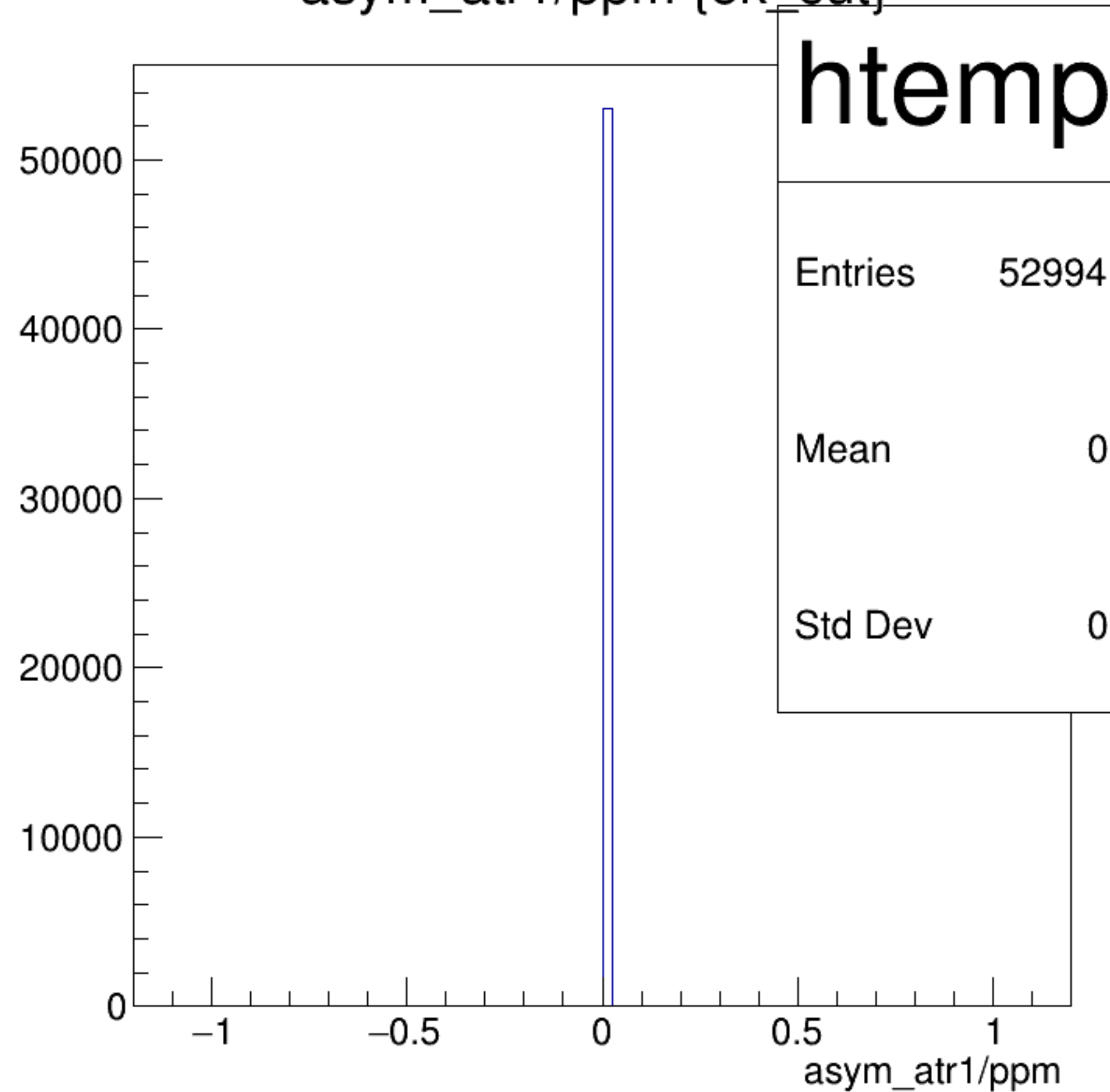
asym_atr1/ppm {ok_cut}
