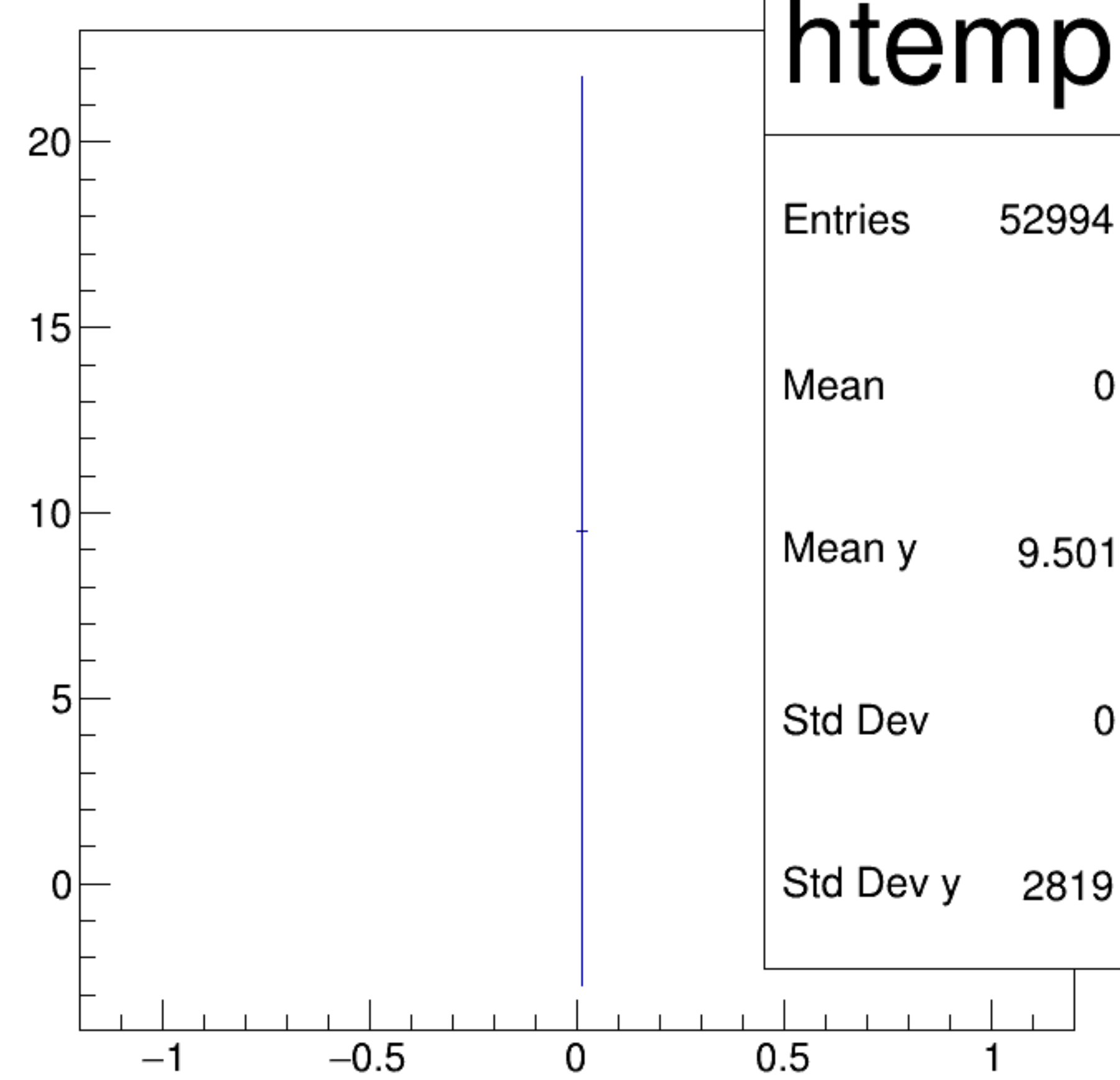
asym_atl2/ppm:asym_atr2/ppm {ok_cut}
