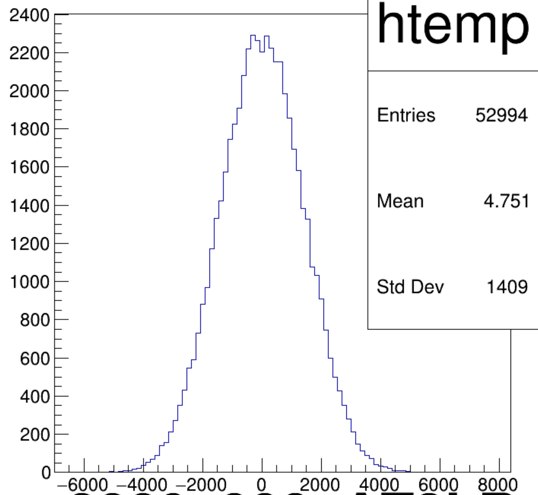
(asym_atl2/ppm-asym_atr2/ppm)/2 {ok_cut}
