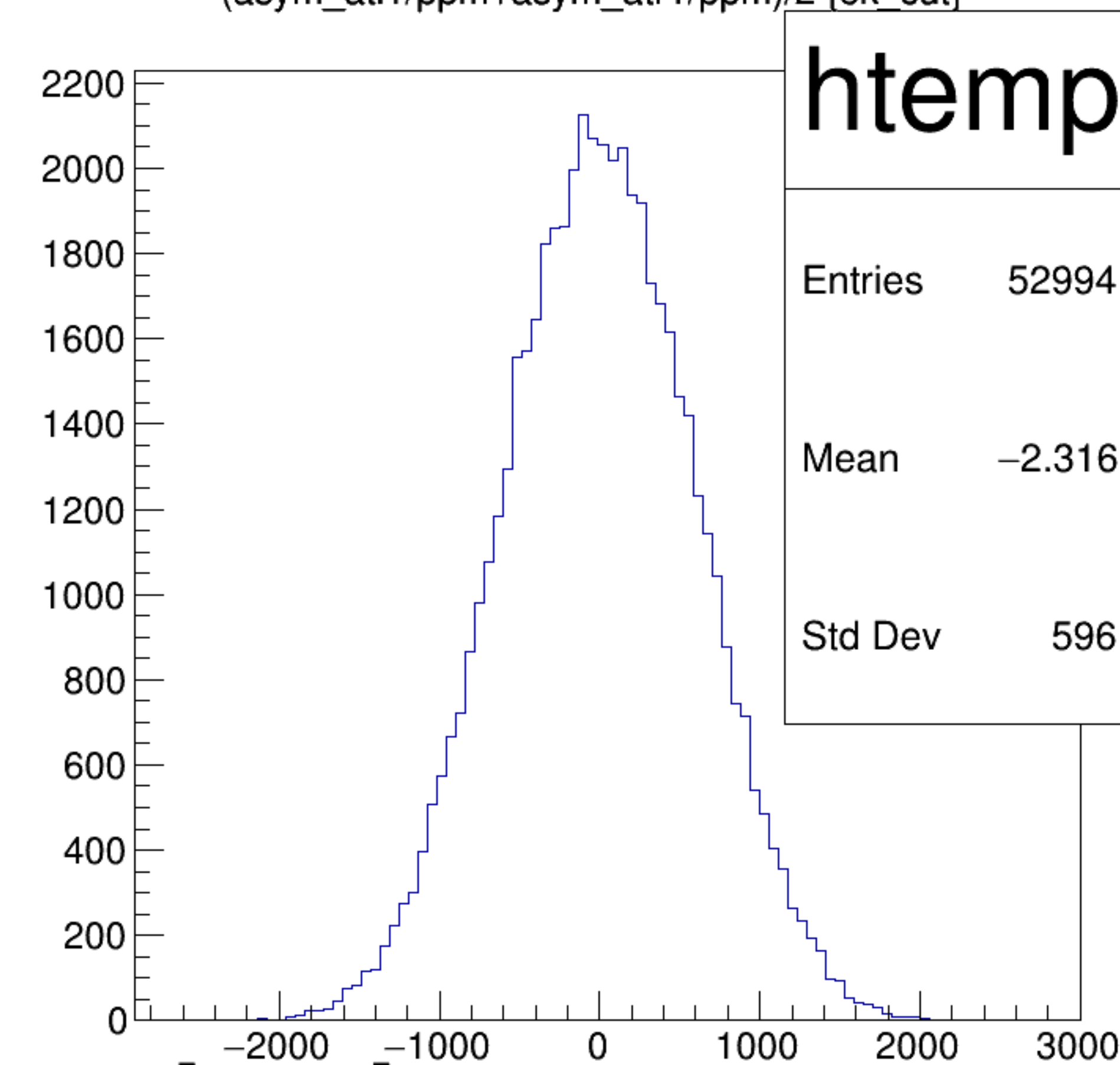
(asym_atl1/ppm+asym_atr1/ppm)/2 {ok_cut}
