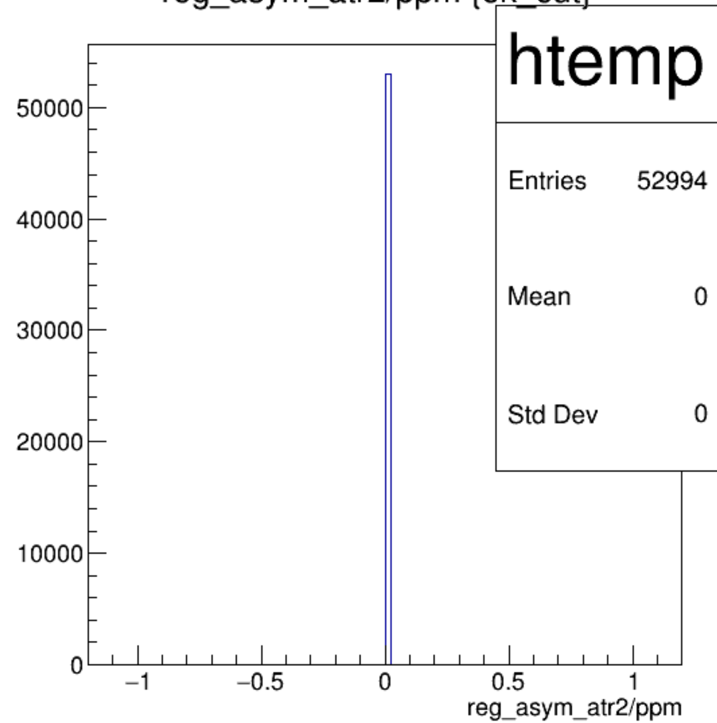
reg_asym_atr2/ppm {ok_cut}
