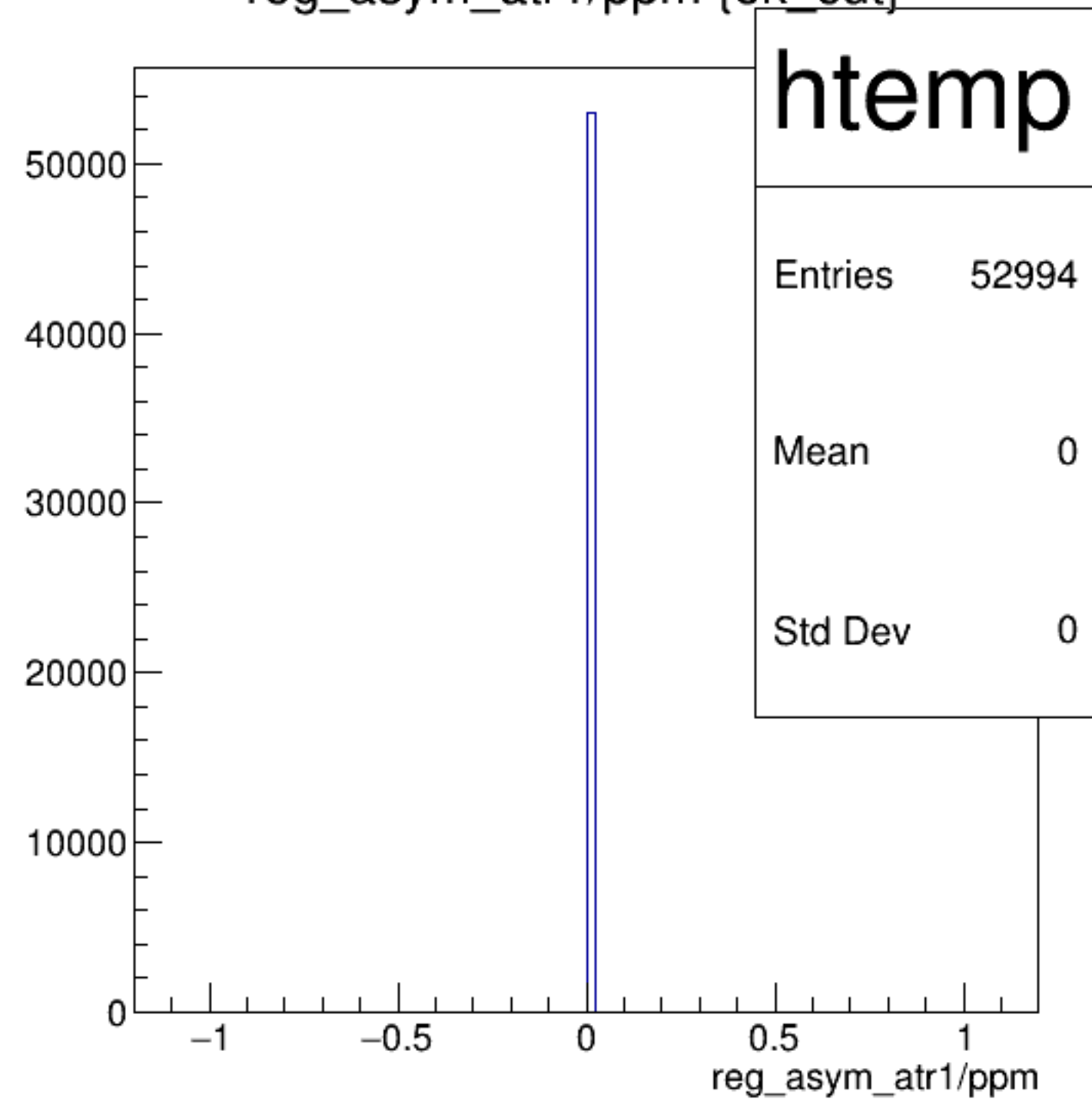
reg_asym_atr1/ppm {ok_cut}
