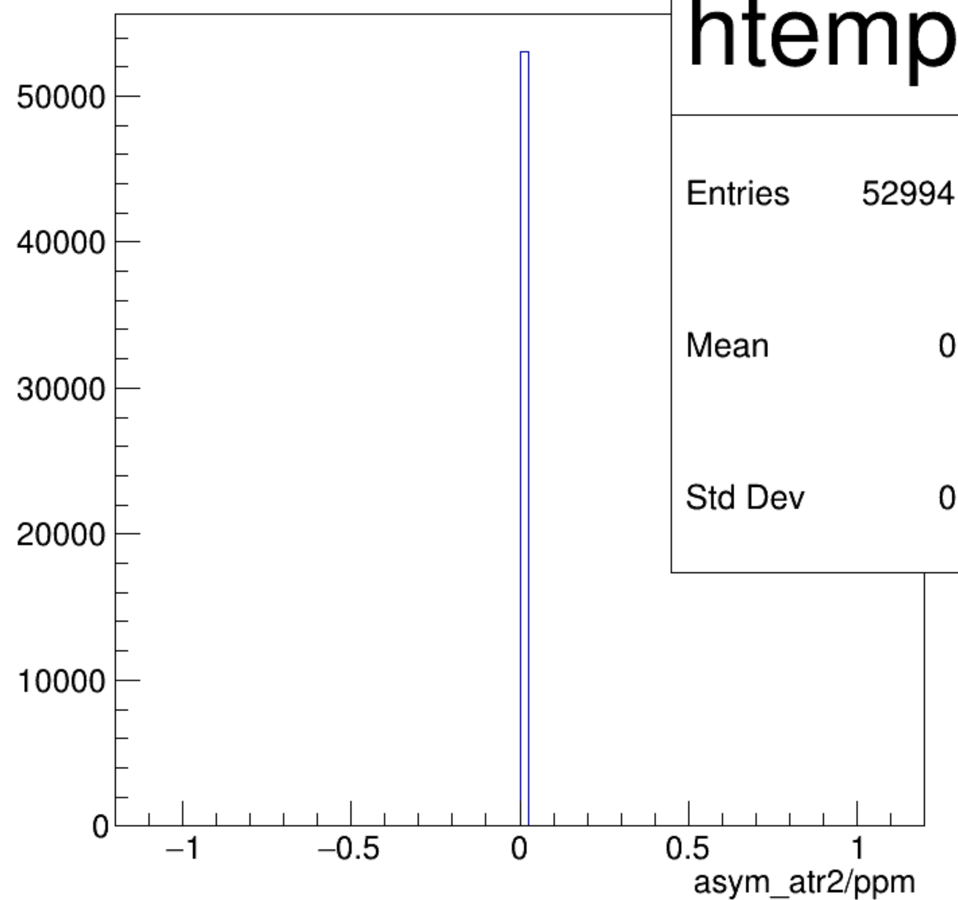
asym_atr2/ppm {ok_cut}
