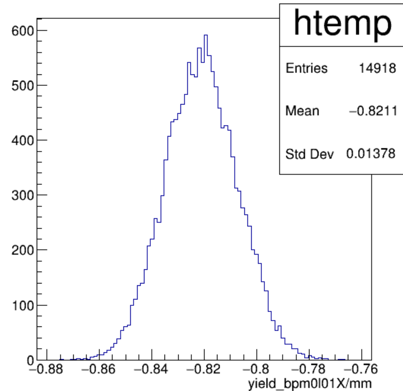
yield_bpm0l01X/mm {ErrorFlag==0}
