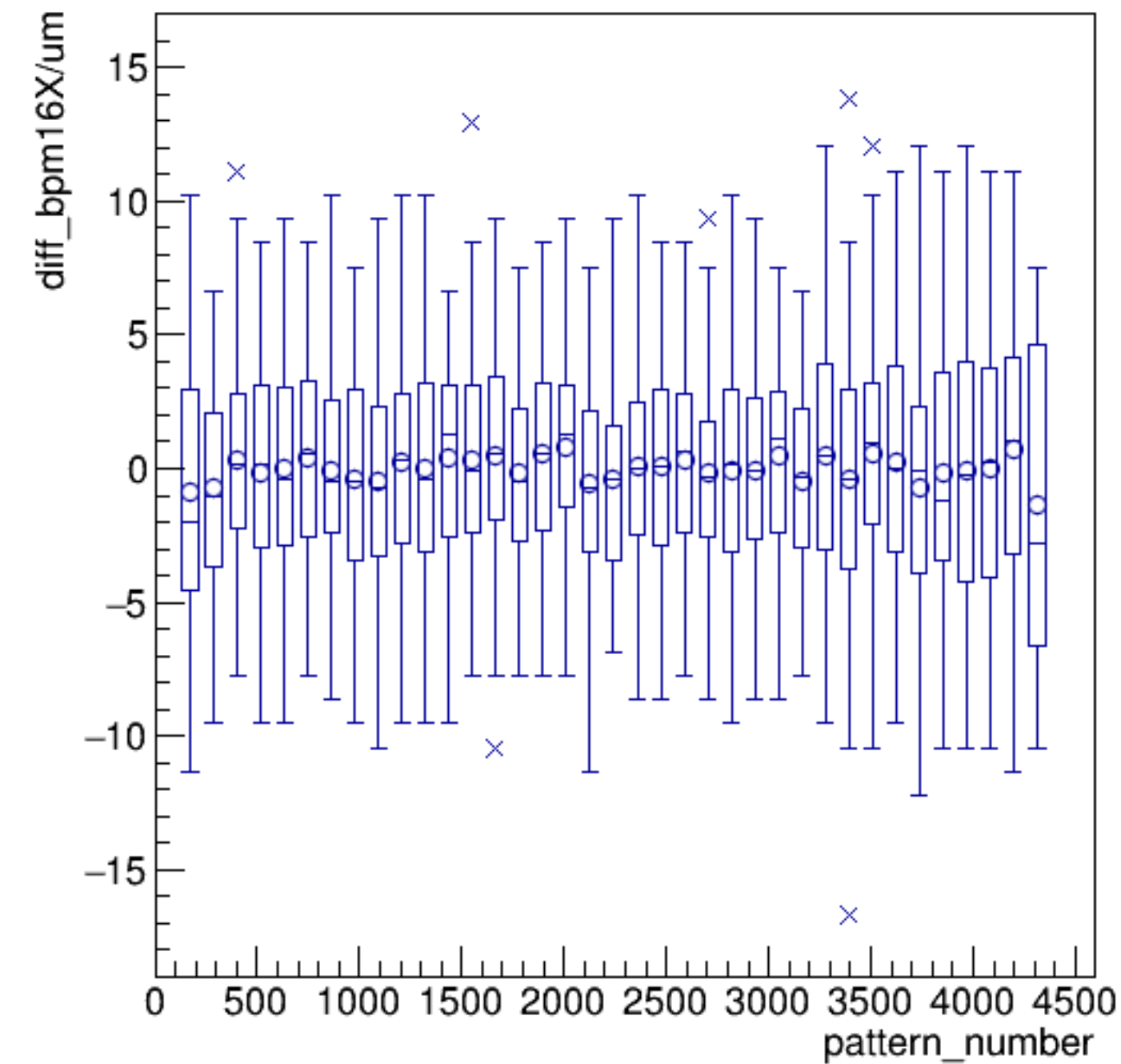
diff_bpm16X/um:pattern_number {ErrorFlag==0}
