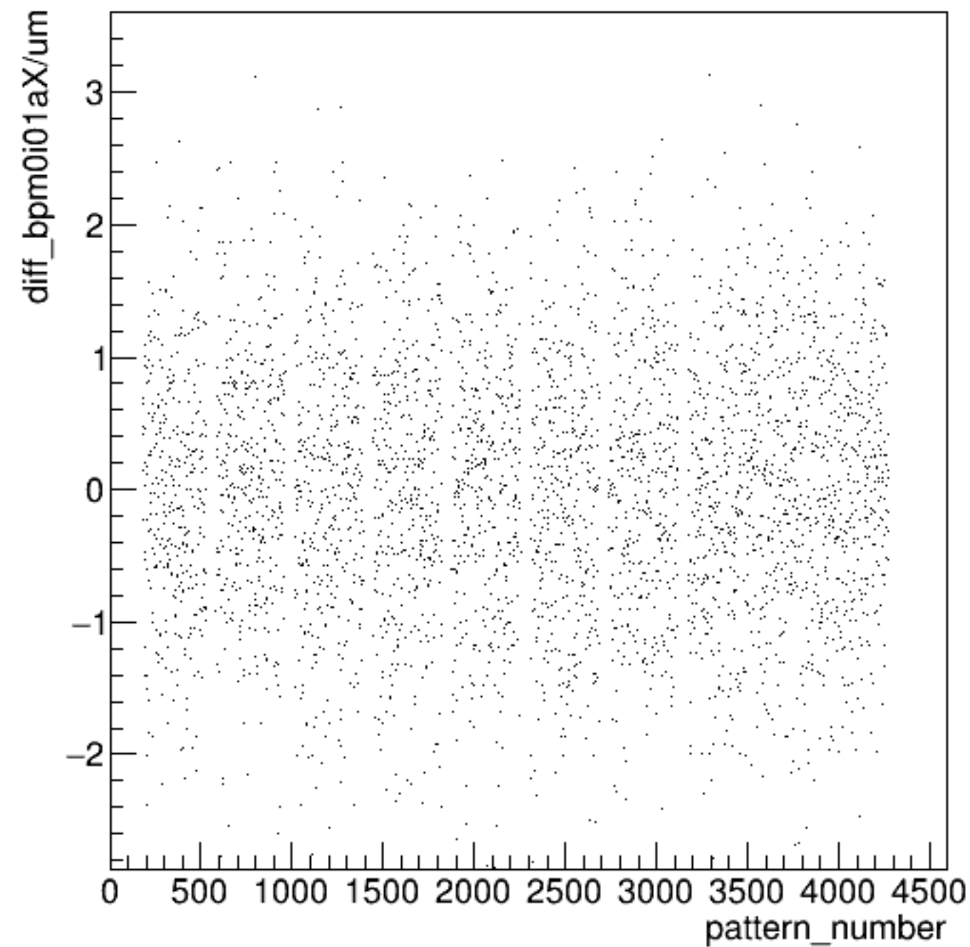
diff_bpm0i01aX/um:pattern_number {ErrorFlag==0}
