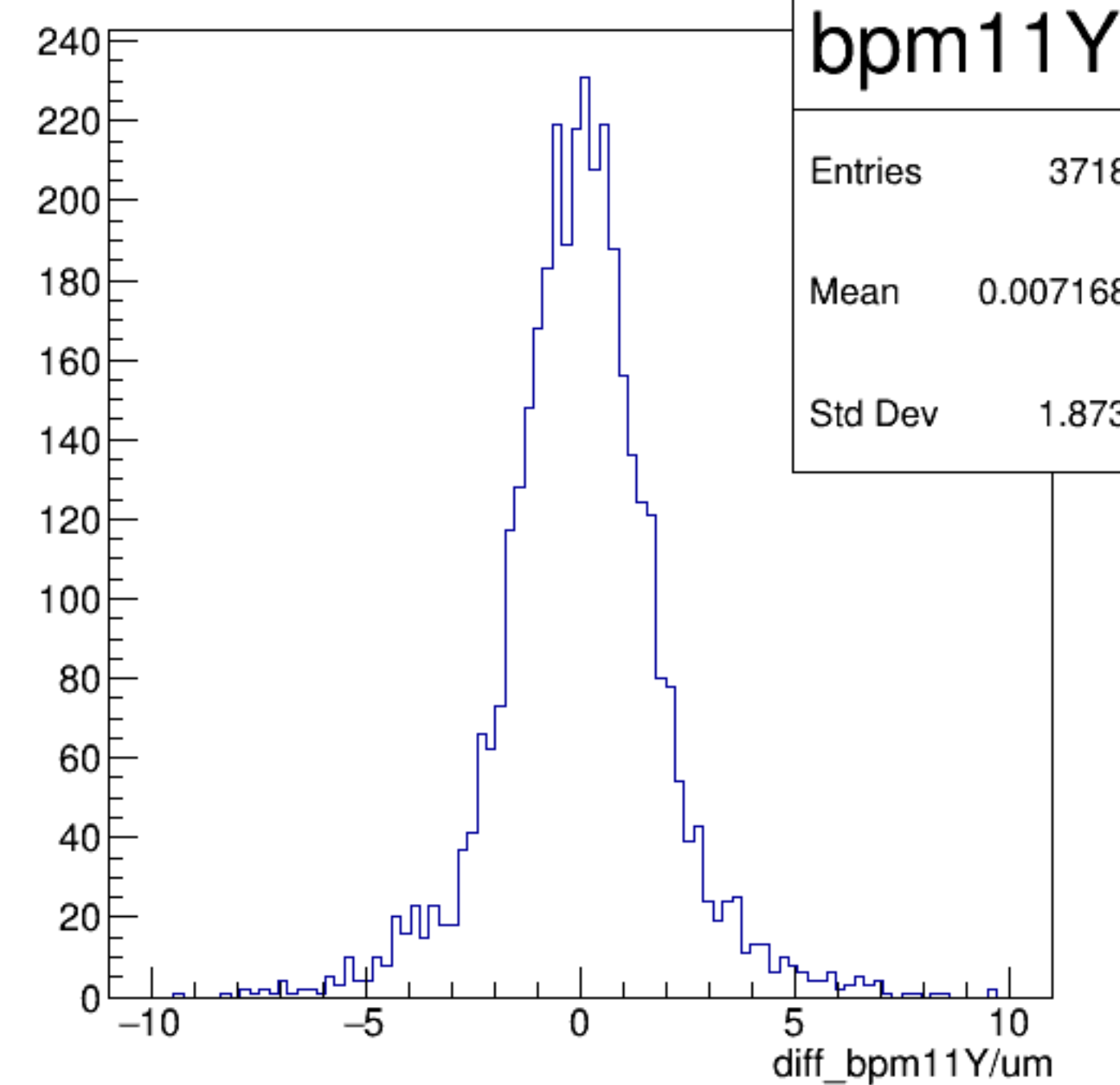
diff_bpm11Y/um {ErrorFlag==0}
