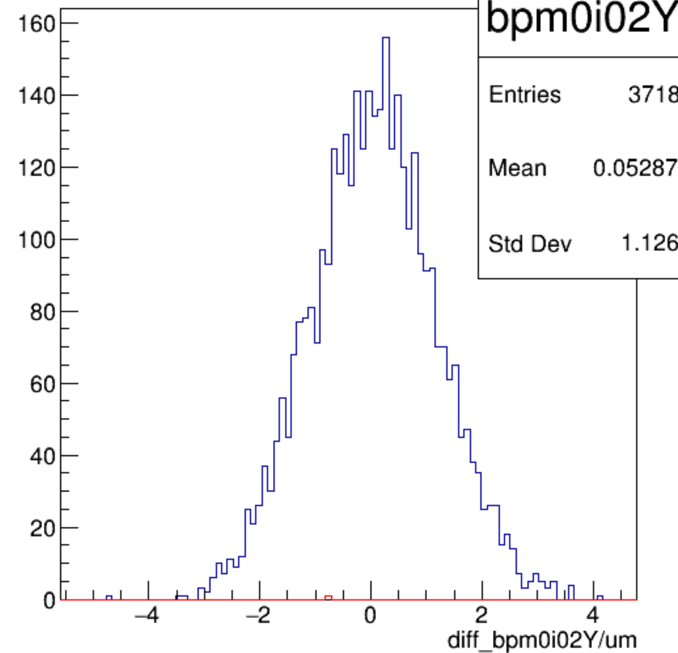
diff_bpm0i02Y/um {ErrorFlag==0}
