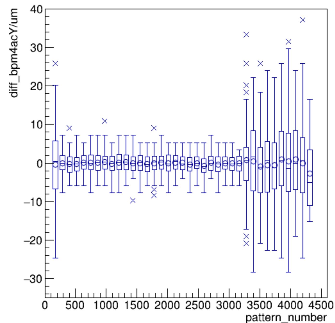
diff_bpm4acY/um:pattern_number {ErrorFlag==0}
