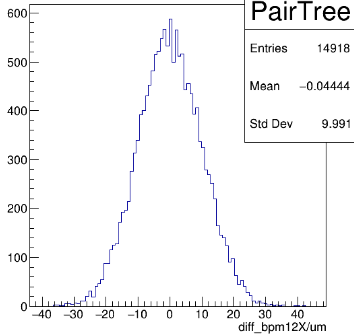
diff_bpm12X/um {ErrorFlag==0}
