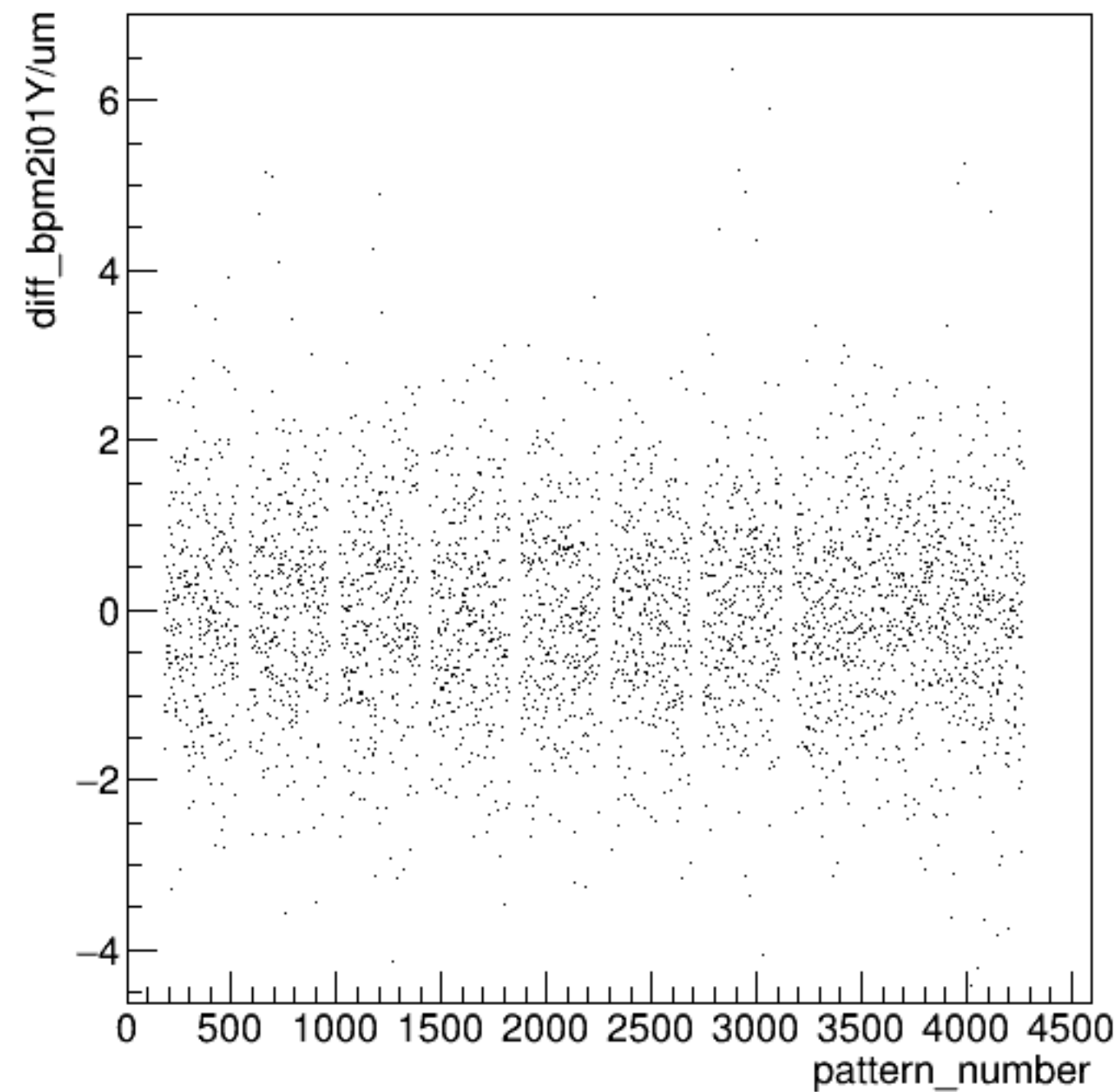
diff_bpm2i01Y/um:pattern_number {ErrorFlag==0}
