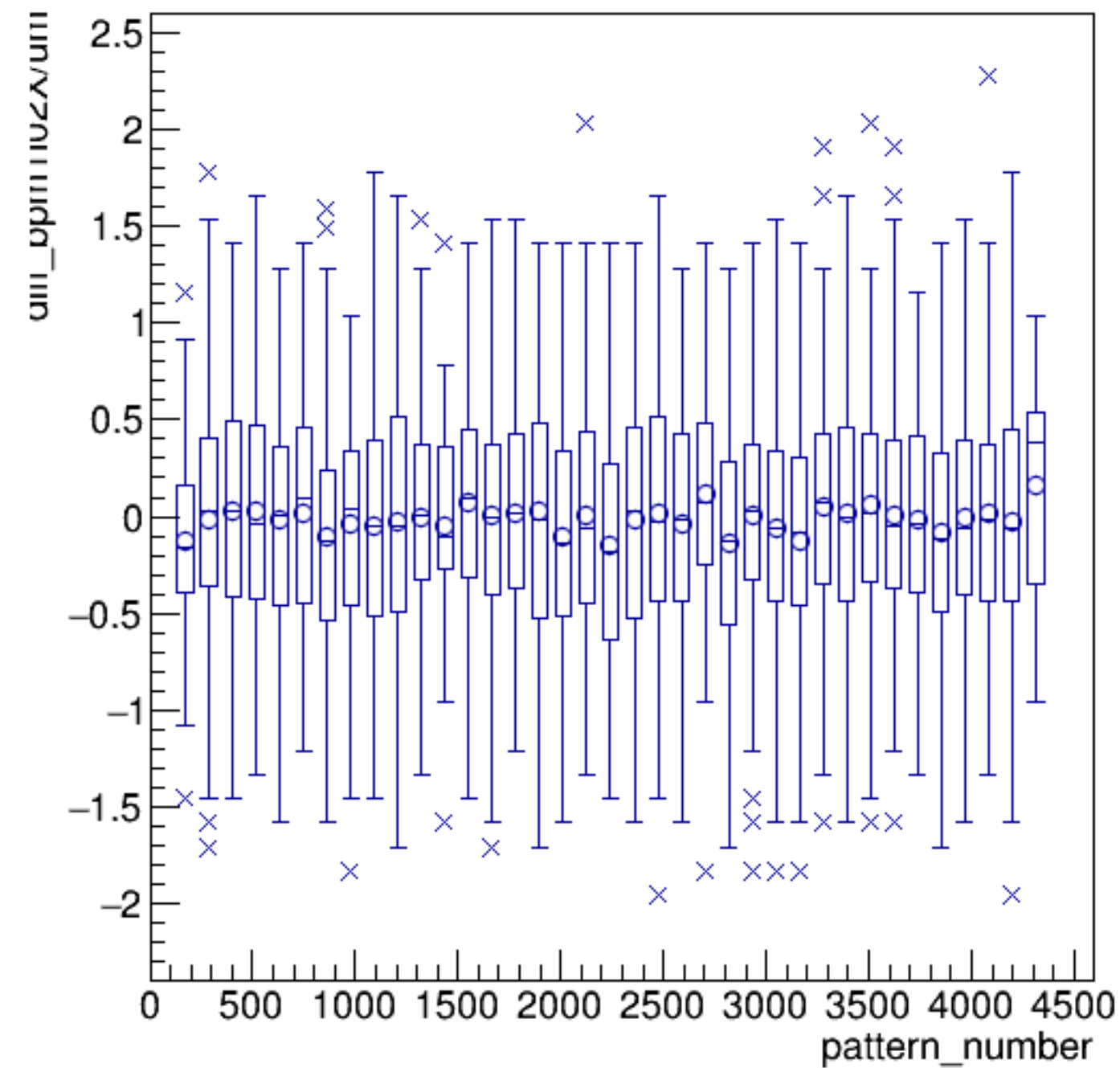
diff_bpm1i02X/um:pattern_number {ErrorFlag==0}
