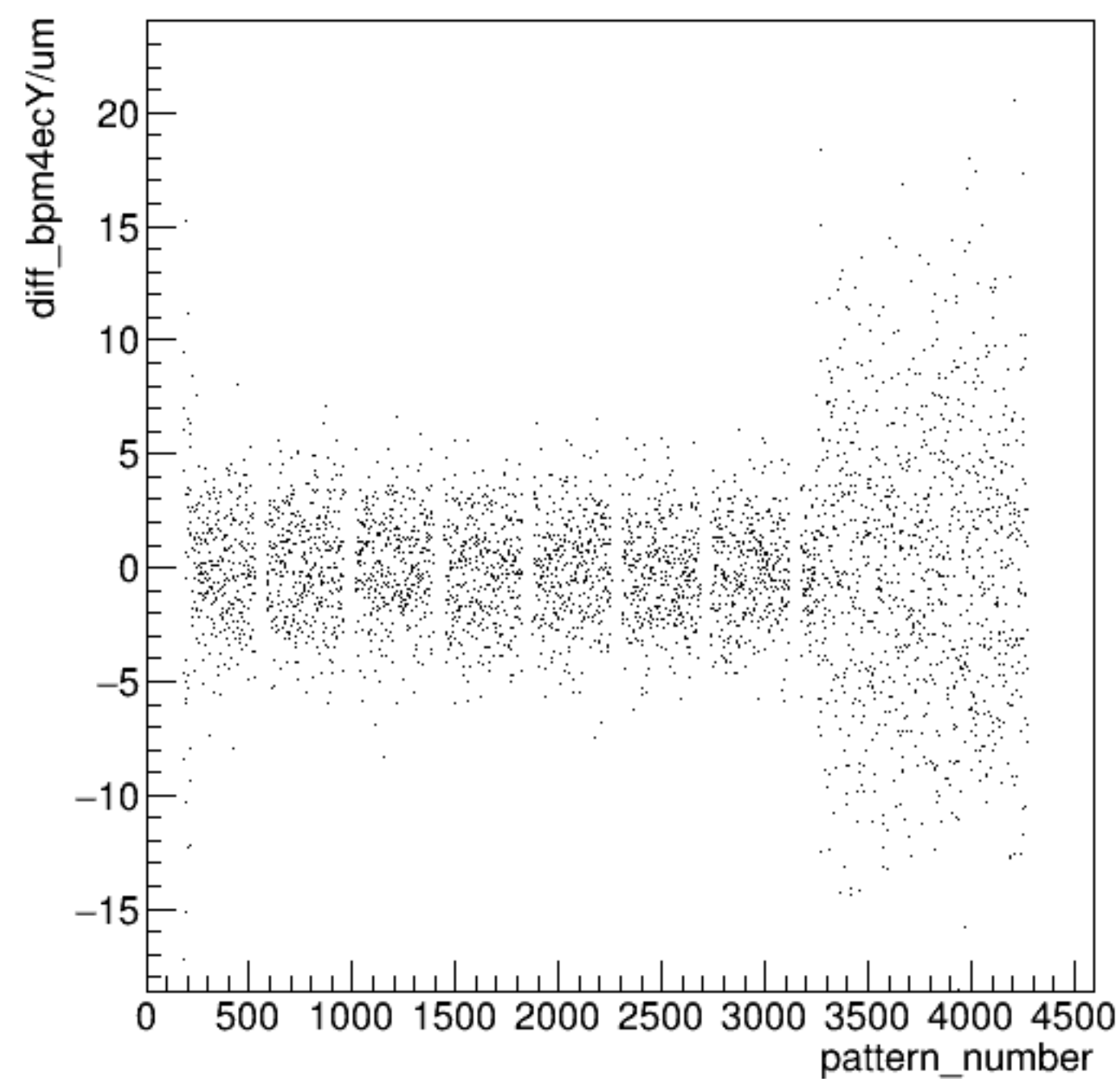
diff_bpm4ecY/um:pattern_number {ErrorFlag==0}
