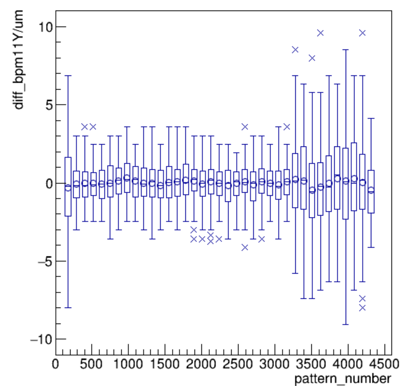
diff_bpm11Y/um:pattern_number {ErrorFlag==0}
