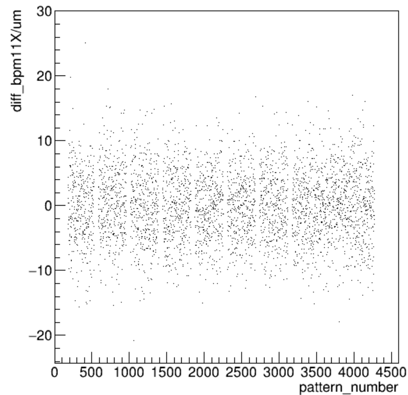
diff_bpm11X/um:pattern_number {ErrorFlag==0}
