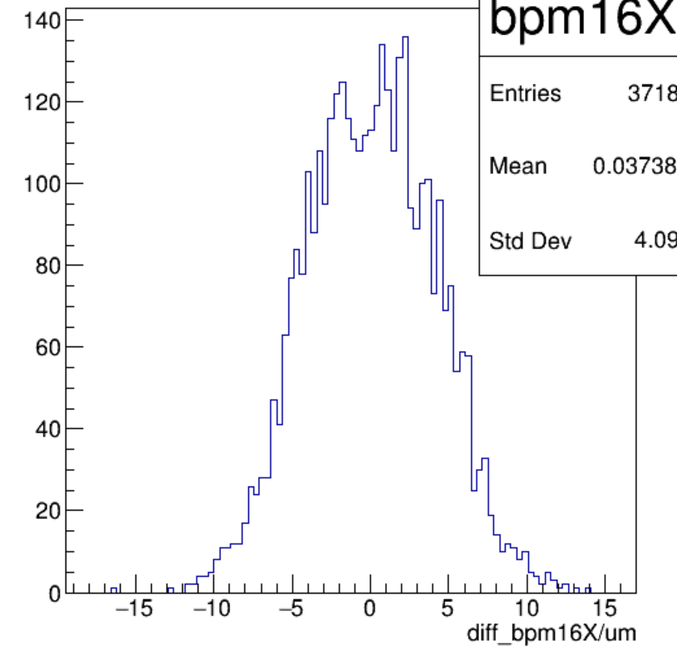
diff_bpm16X/um {ErrorFlag==0}
