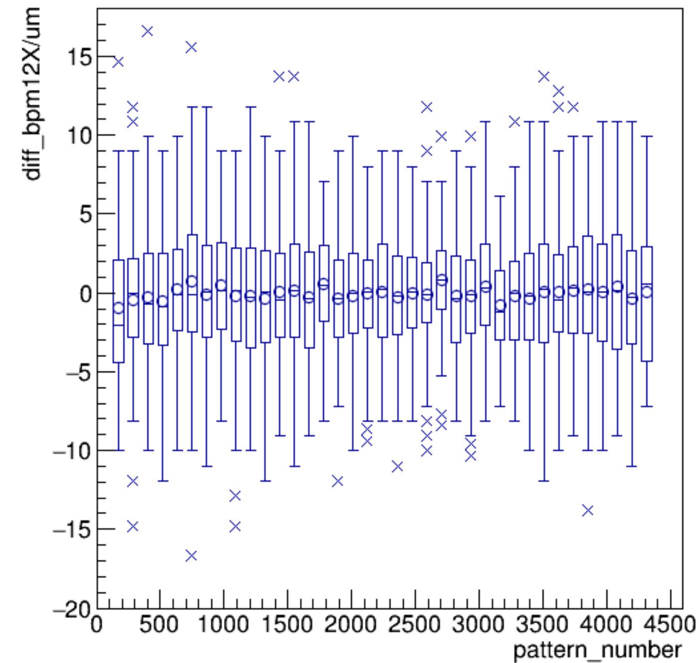
diff_bpm12X/um:pattern_number {ErrorFlag==0}
