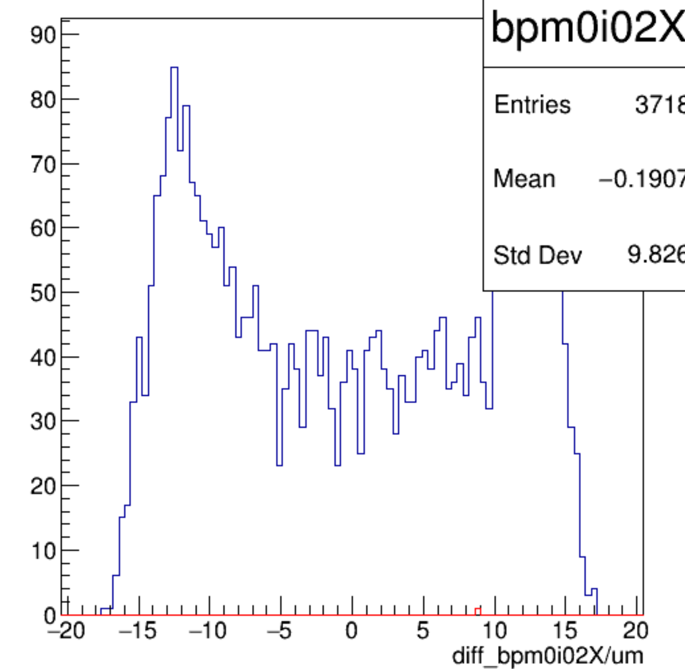
diff_bpm0i02X/um {ErrorFlag==0}
