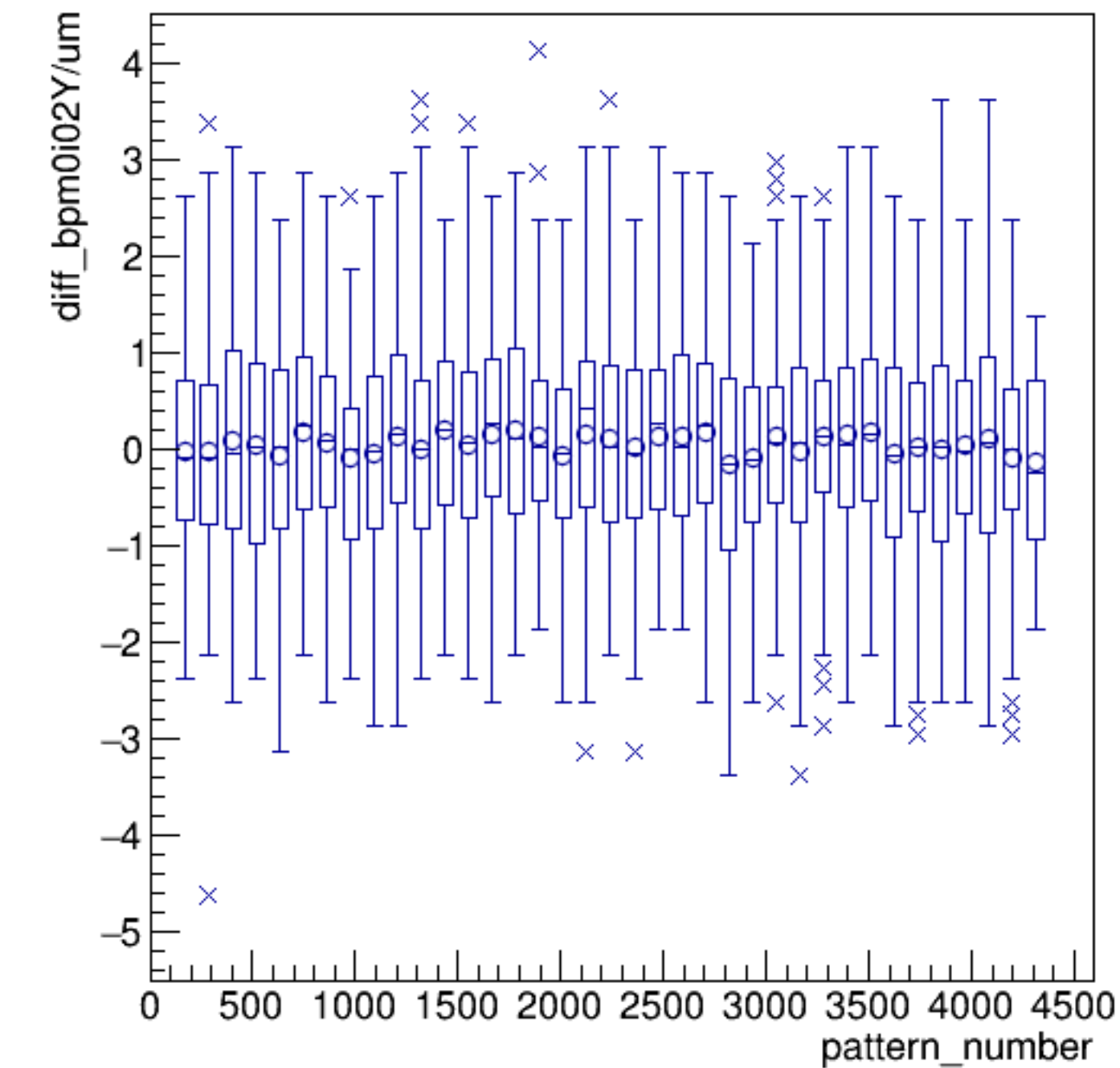
diff_bpm0i02Y/um:pattern_number {ErrorFlag==0}
