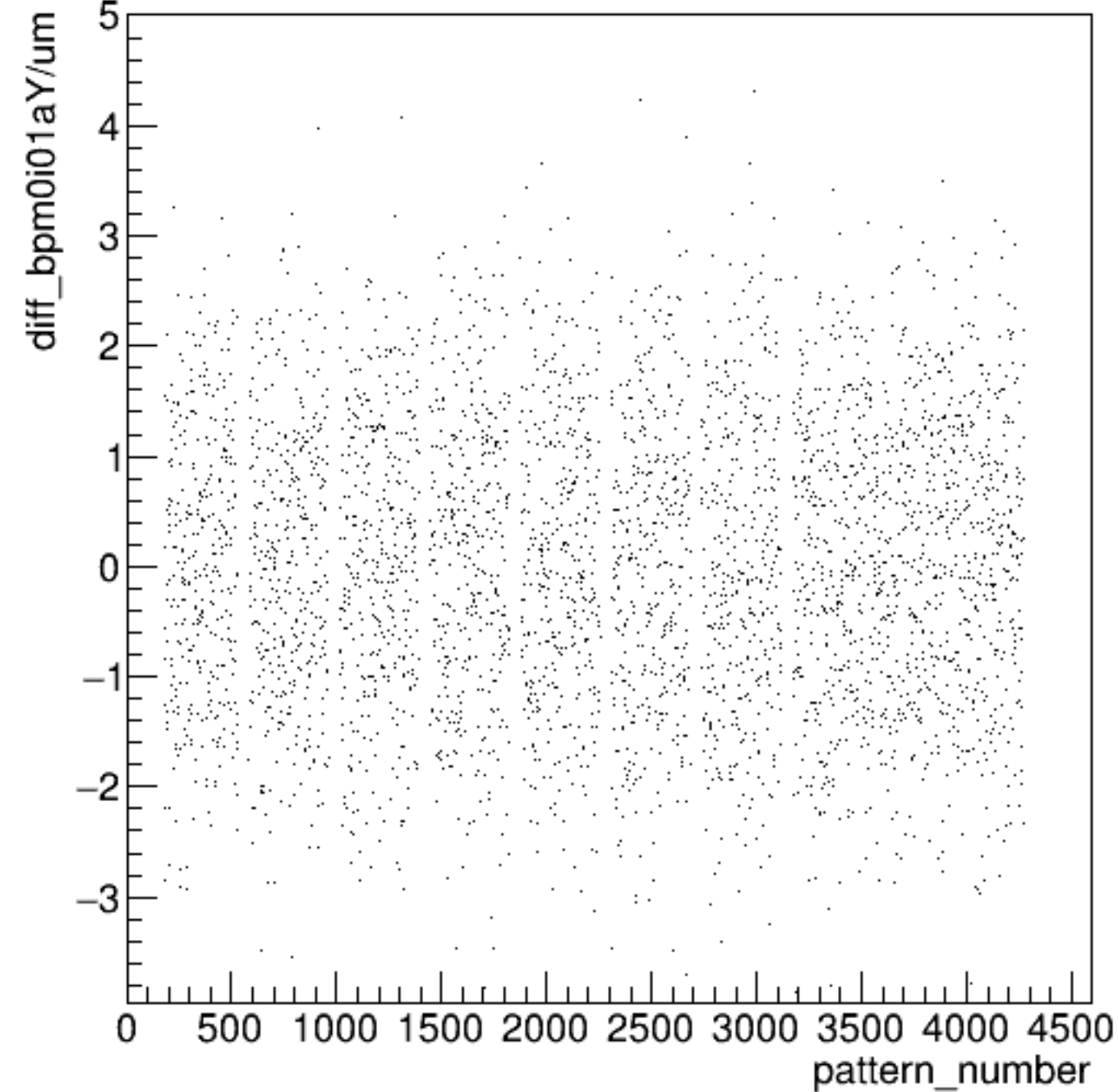
diff_bpm0i01aY/um:pattern_number {ErrorFlag==0}
