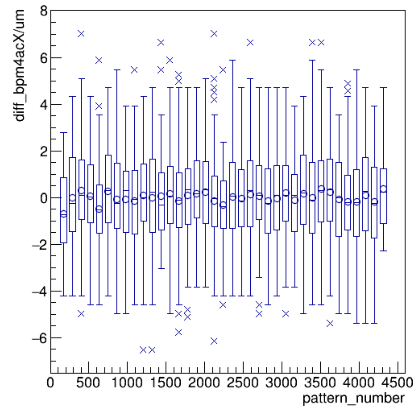
diff_bpm4acX/um:pattern_number {ErrorFlag==0}
