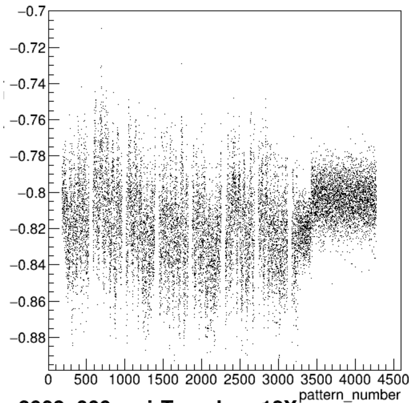
yield_bpm12X/mm:pattern_number {ErrorFlag==0}
