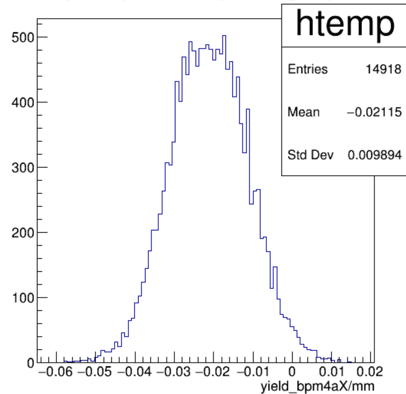
yield_bpm4aX/mm {ErrorFlag==0}
