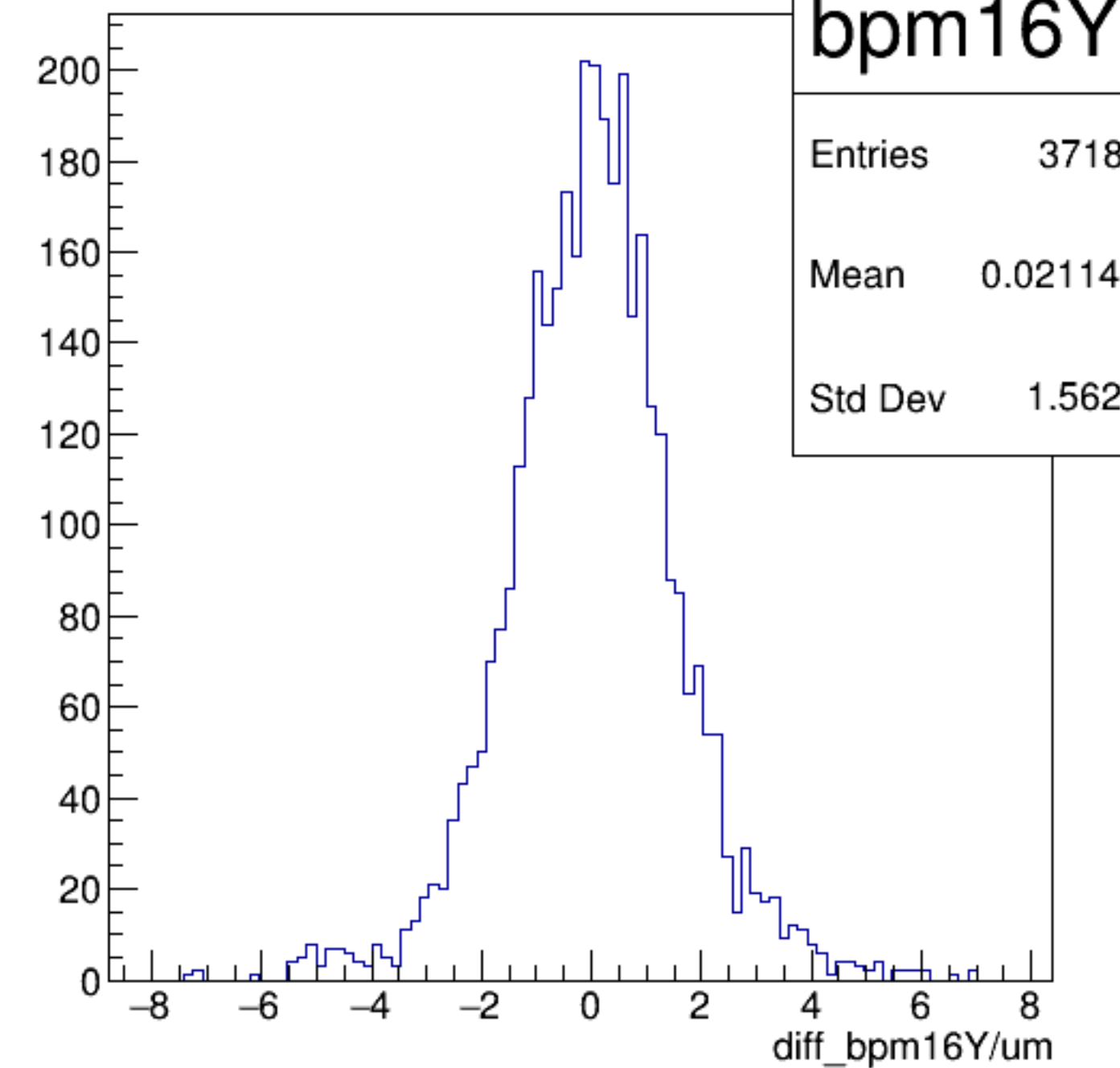
diff_bpm16Y/um {ErrorFlag==0}
