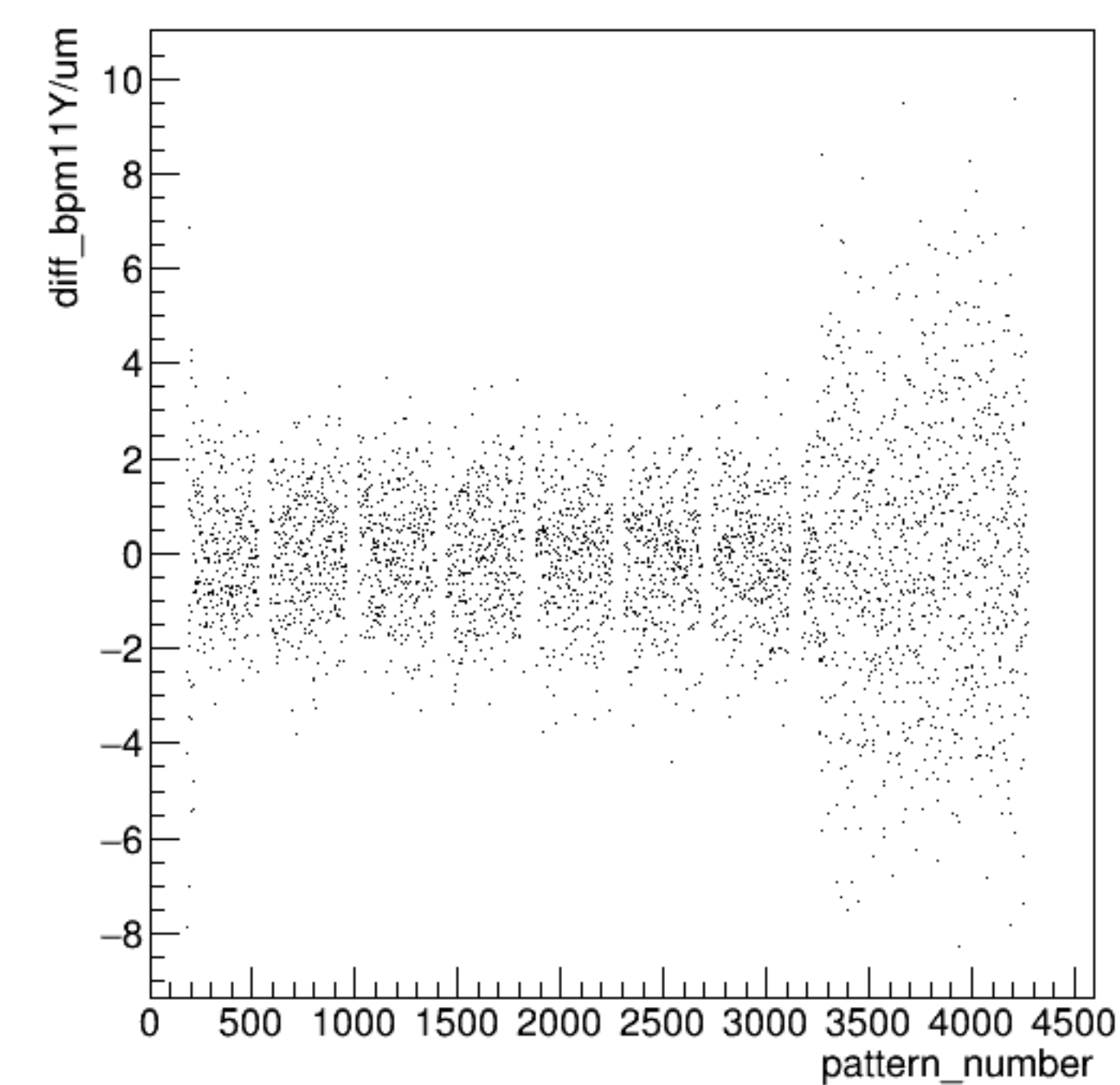
diff_bpm11Y/um:pattern_number {ErrorFlag==0}
