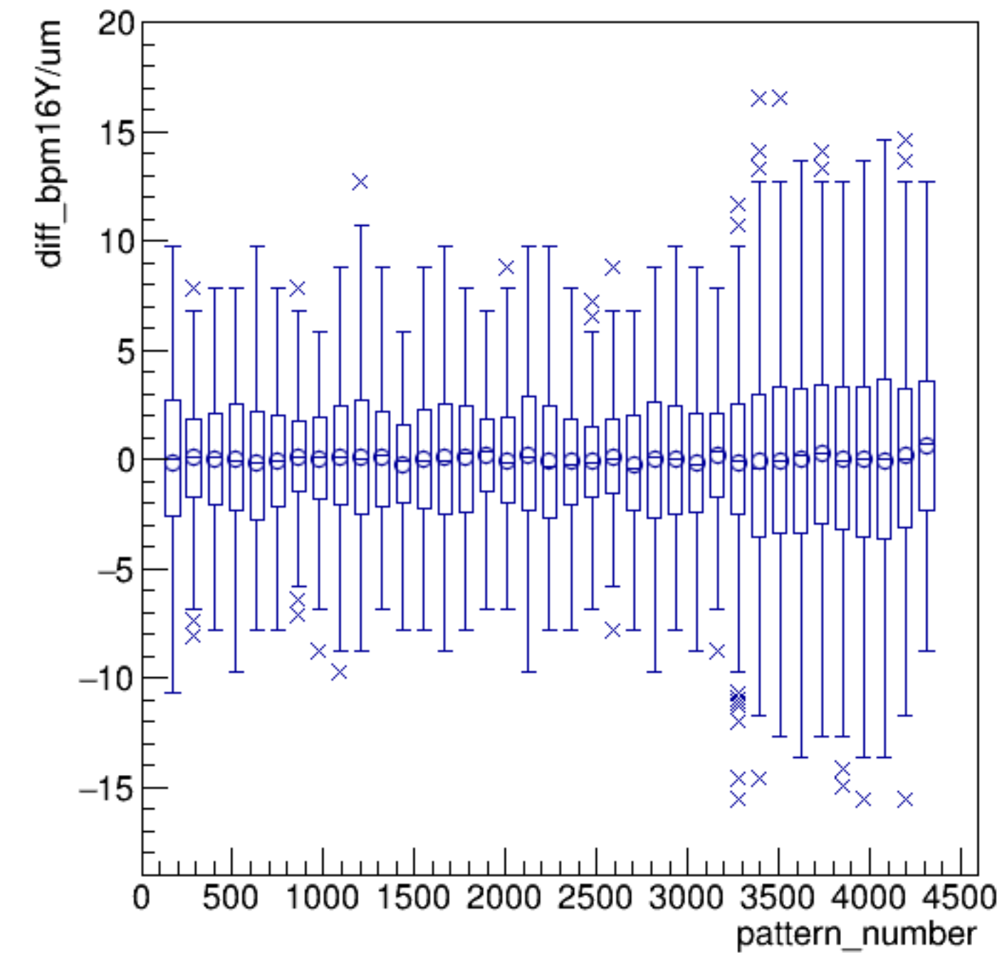
diff_bpm16Y/um:pattern_number {ErrorFlag==0}
