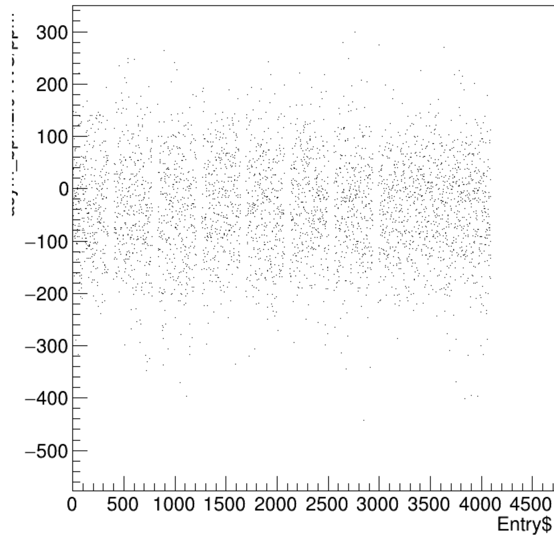
asym_bpm2i01WS/ppm:Entry$ {ErrorFlag==0}
