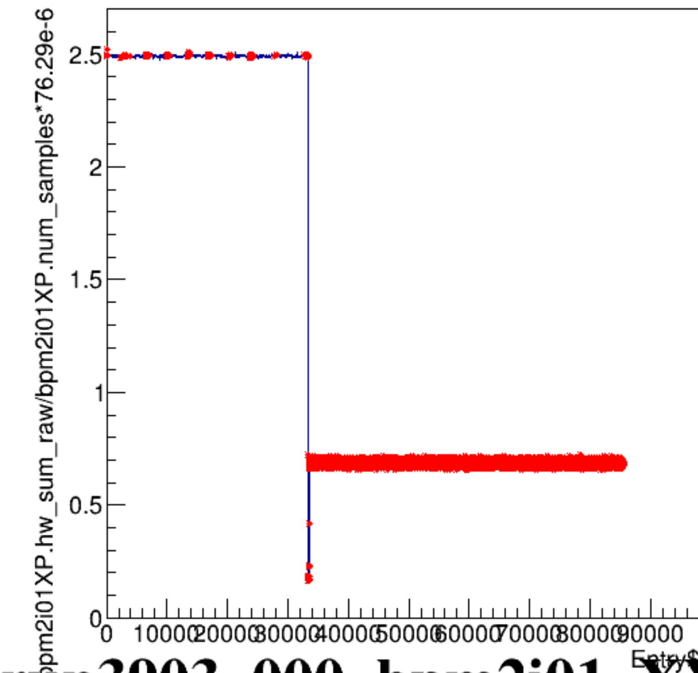
bpm2i01XP.hw_sum_raw/bpm2i01XP.num_samples*76.29e-6:Entry$
