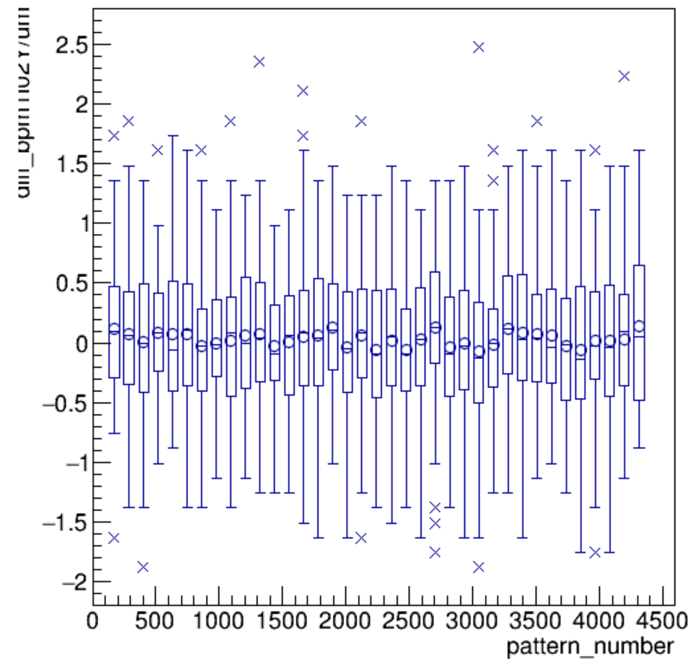
diff_bpm1i02Y/um:pattern_number {ErrorFlag==0}
