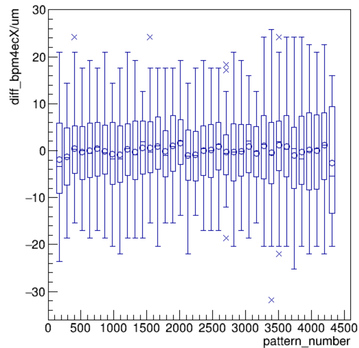
diff_bpm4ecX/um:pattern_number {ErrorFlag==0}
