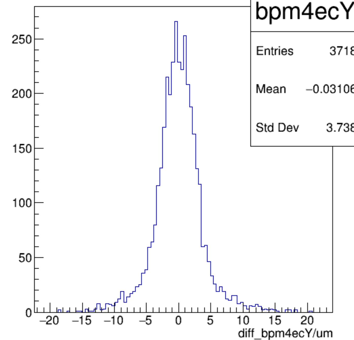
diff_bpm4ecY/um {ErrorFlag==0}
