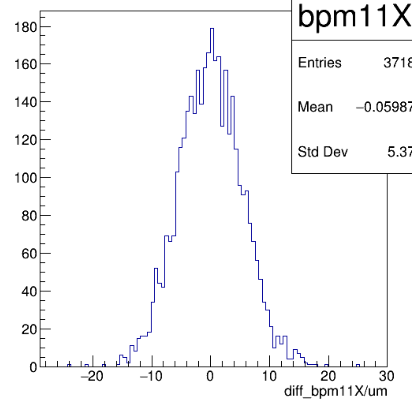
diff_bpm11X/um {ErrorFlag==0}
