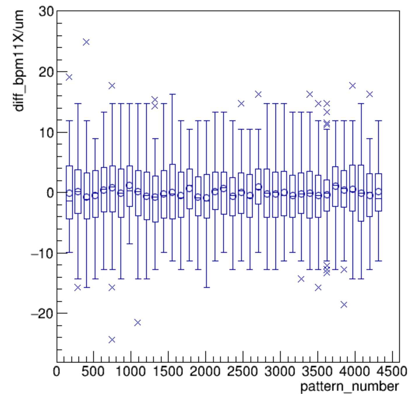
diff_bpm11X/um:pattern_number {ErrorFlag==0}
