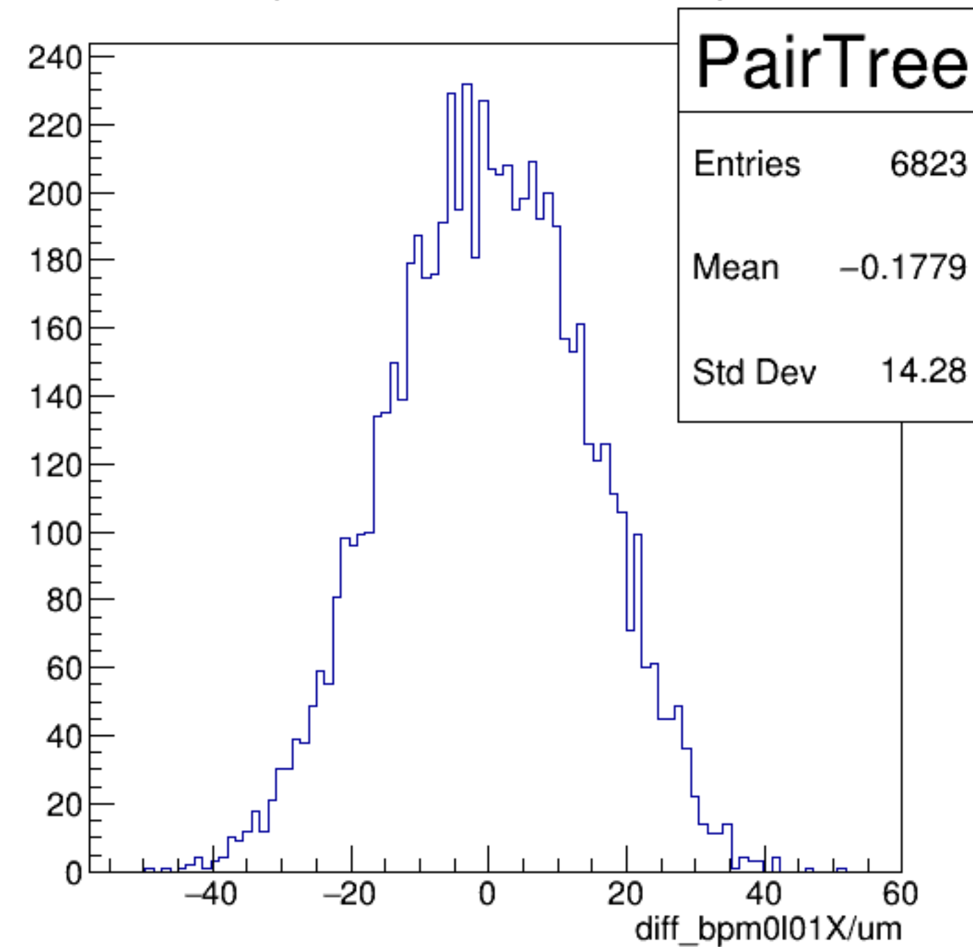
diff_bpm0l01X/um {ErrorFlag==0}
