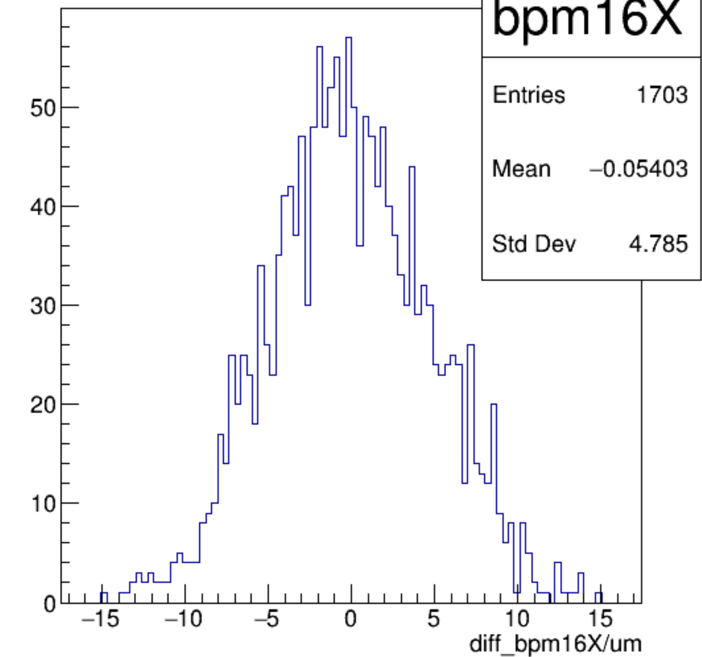
diff_bpm16X/um {ErrorFlag==0}
