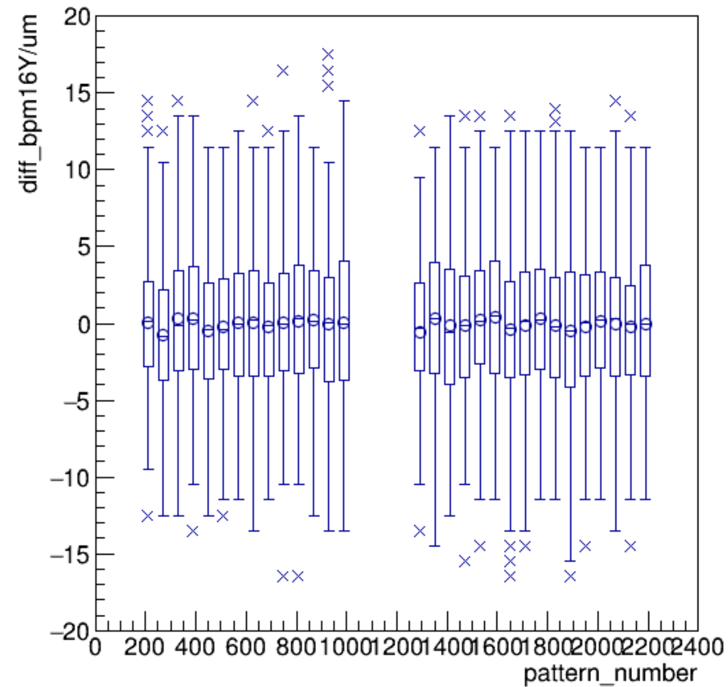
diff_bpm16Y/um:pattern_number {ErrorFlag==0}
