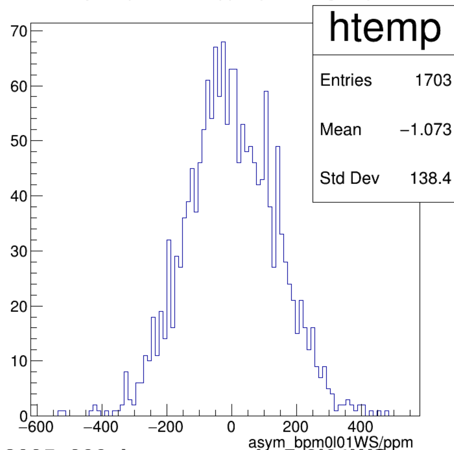
asym_bpm0l01WS/ppm {ErrorFlag==0}
