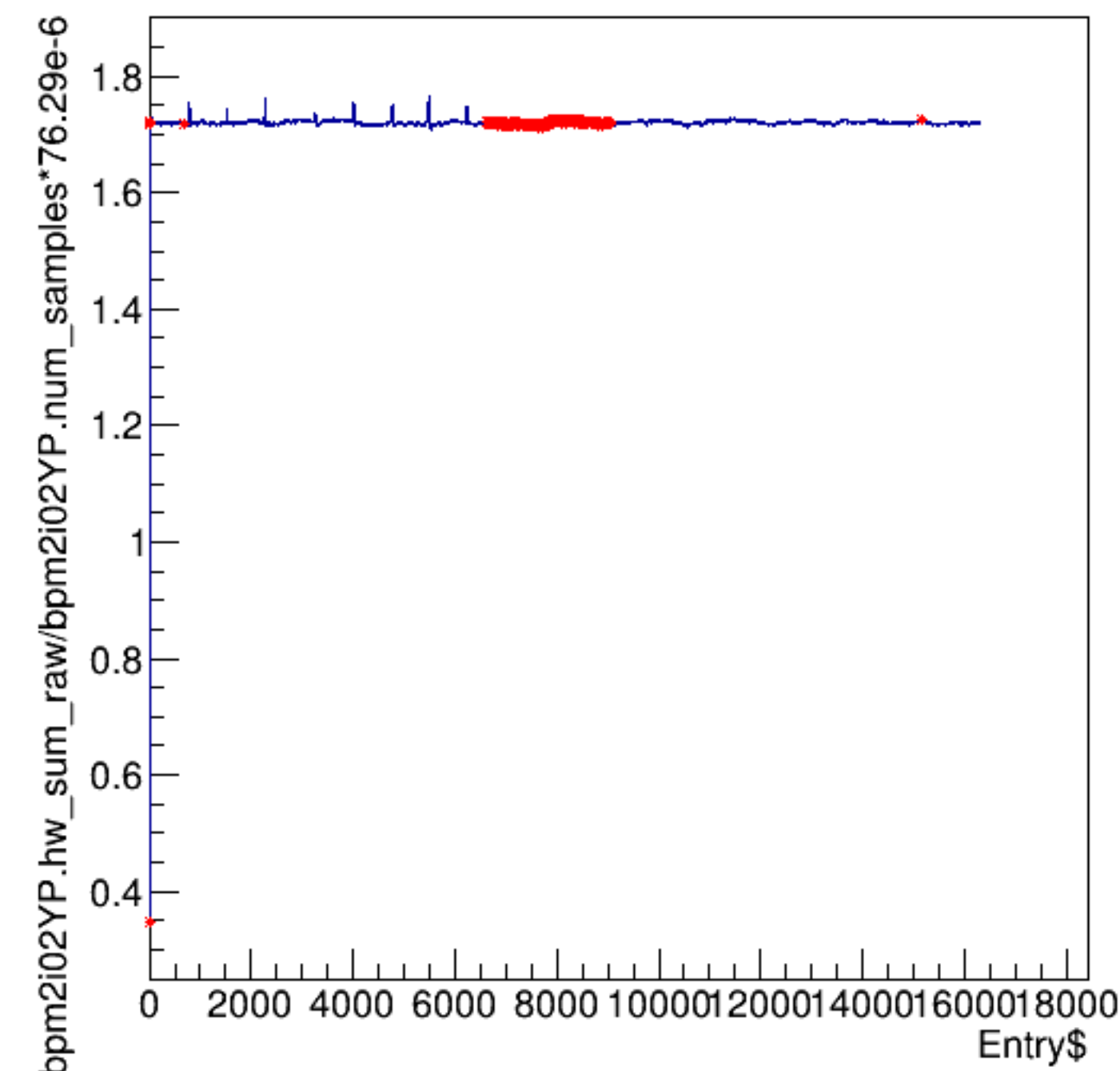
bpm2i02YP.hw_sum_raw/bpm2i02YP.num_samples*76.29e-6:Entry$
