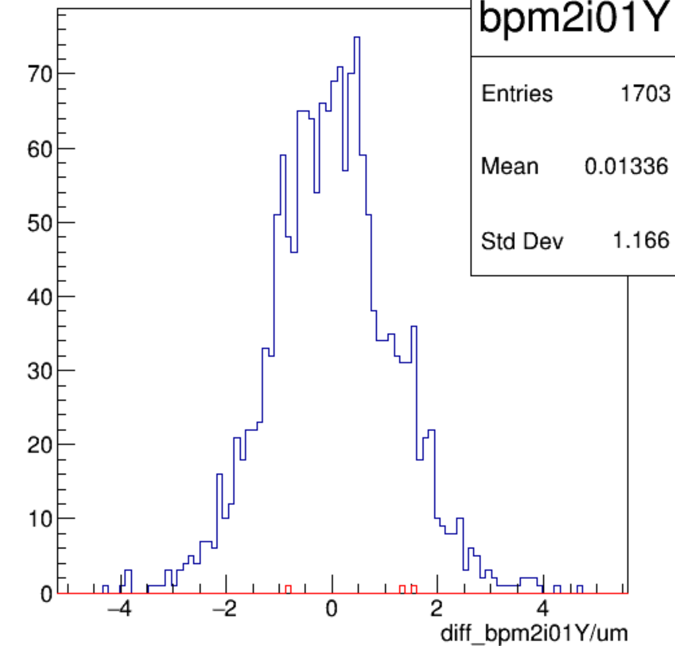
diff_bpm2i01Y/um {ErrorFlag==0}
