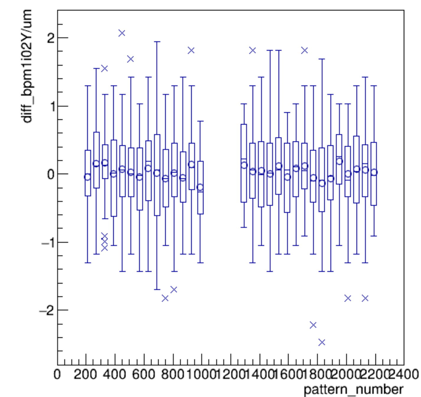
diff_bpm1i02Y/um:pattern_number {ErrorFlag==0}
