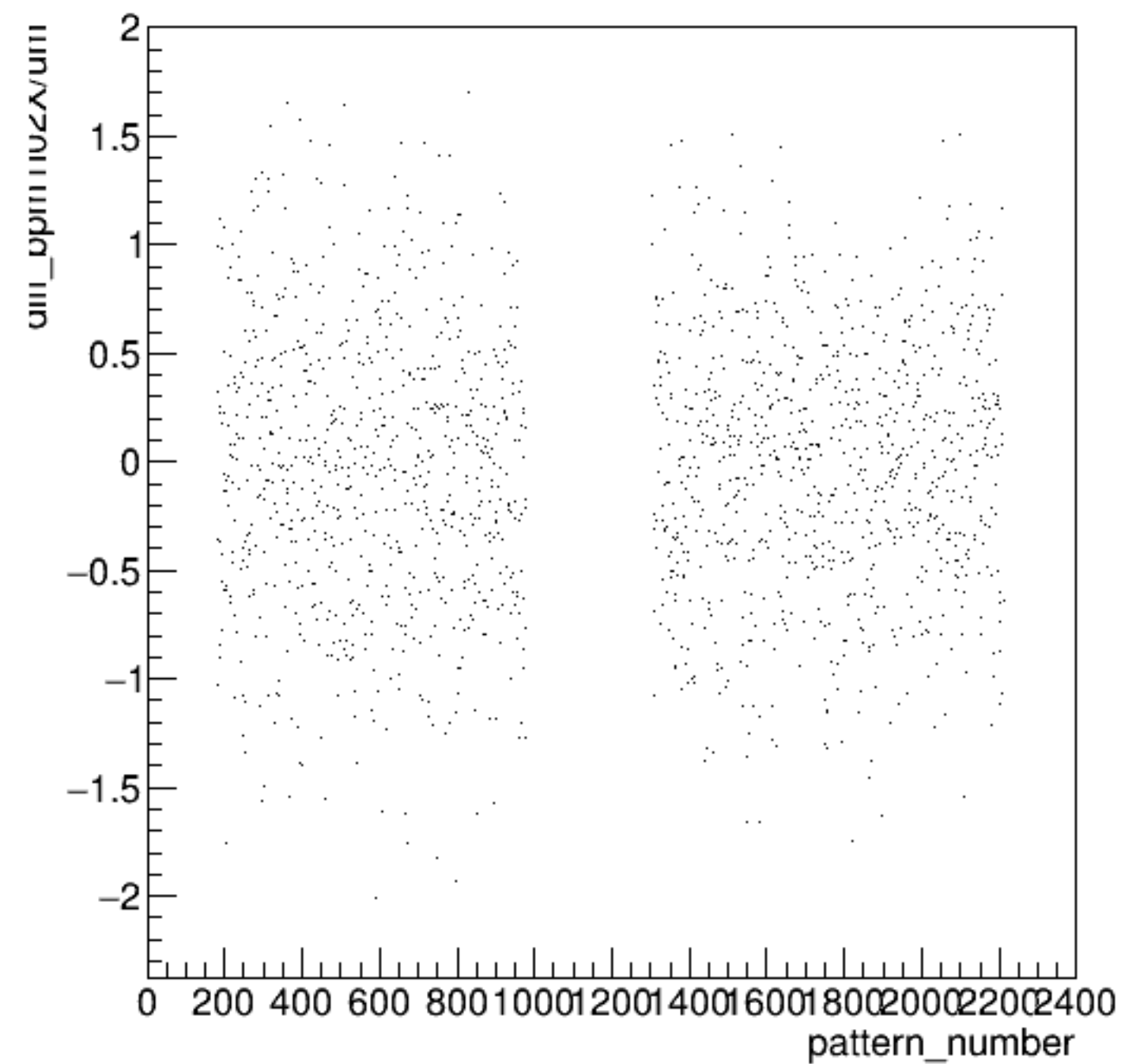
diff_bpm1i02X/um:pattern_number {ErrorFlag==0}
