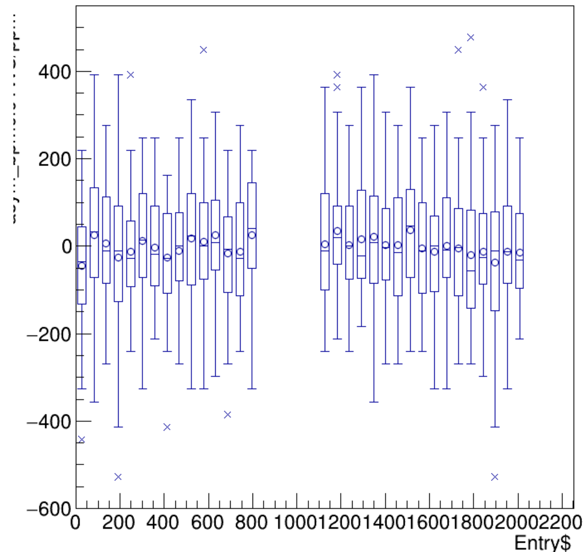
asym_bpm0l01WS/ppm:Entry$ {ErrorFlag==0}
