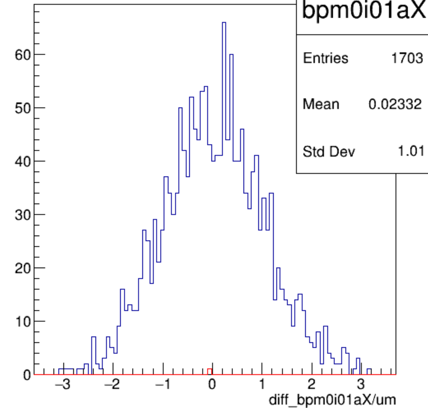
diff_bpm0i01aX/um {ErrorFlag==0}
