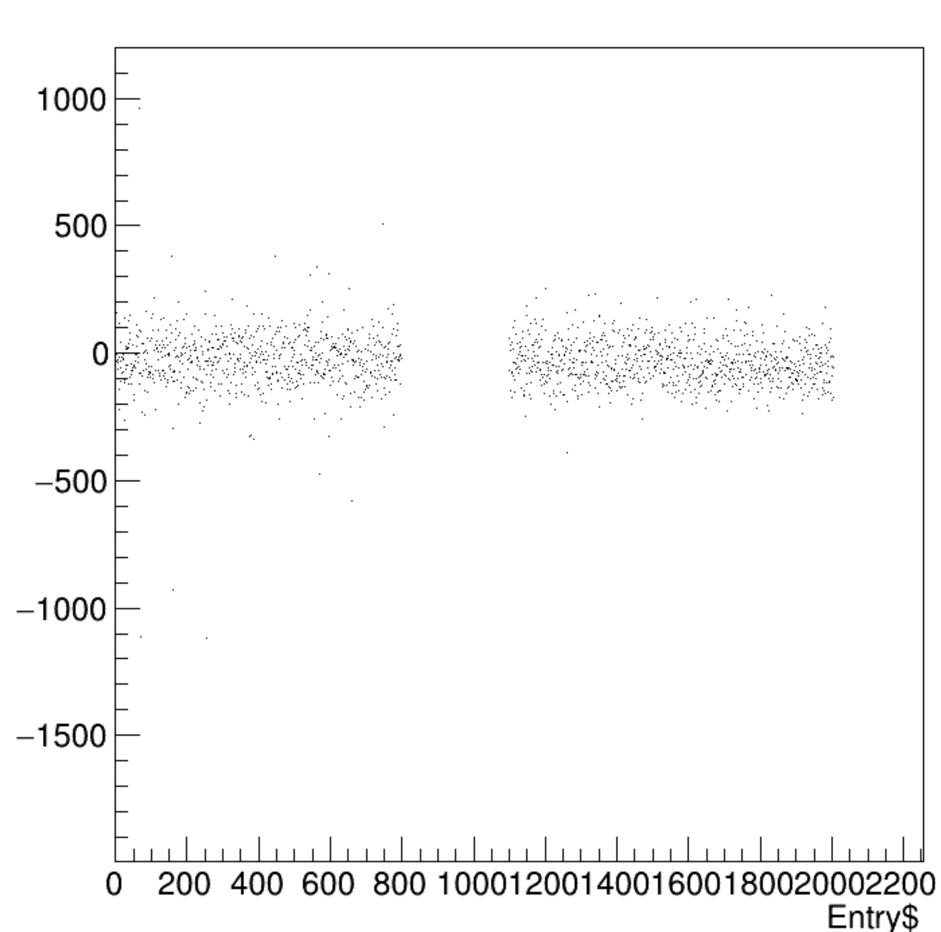
asym_bpm2i01WS/ppm:Entry$ {ErrorFlag==0}
