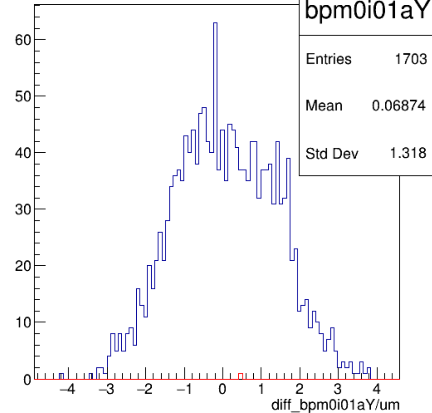
diff_bpm0i01aY/um {ErrorFlag==0}
