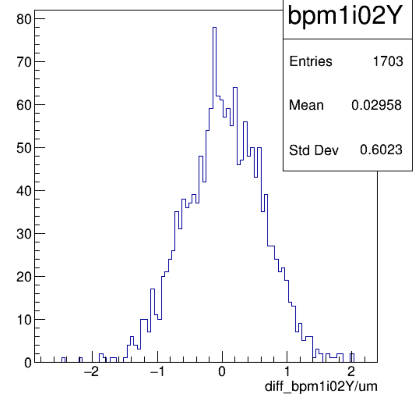
diff_bpm1i02Y/um {ErrorFlag==0}
