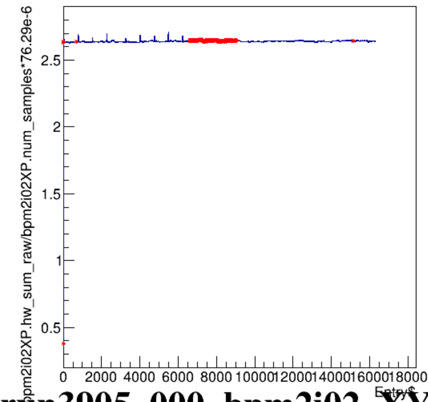
bpm2i02XP.hw_sum_raw/bpm2i02XP.num_samples*76.29e-6:Entry$
