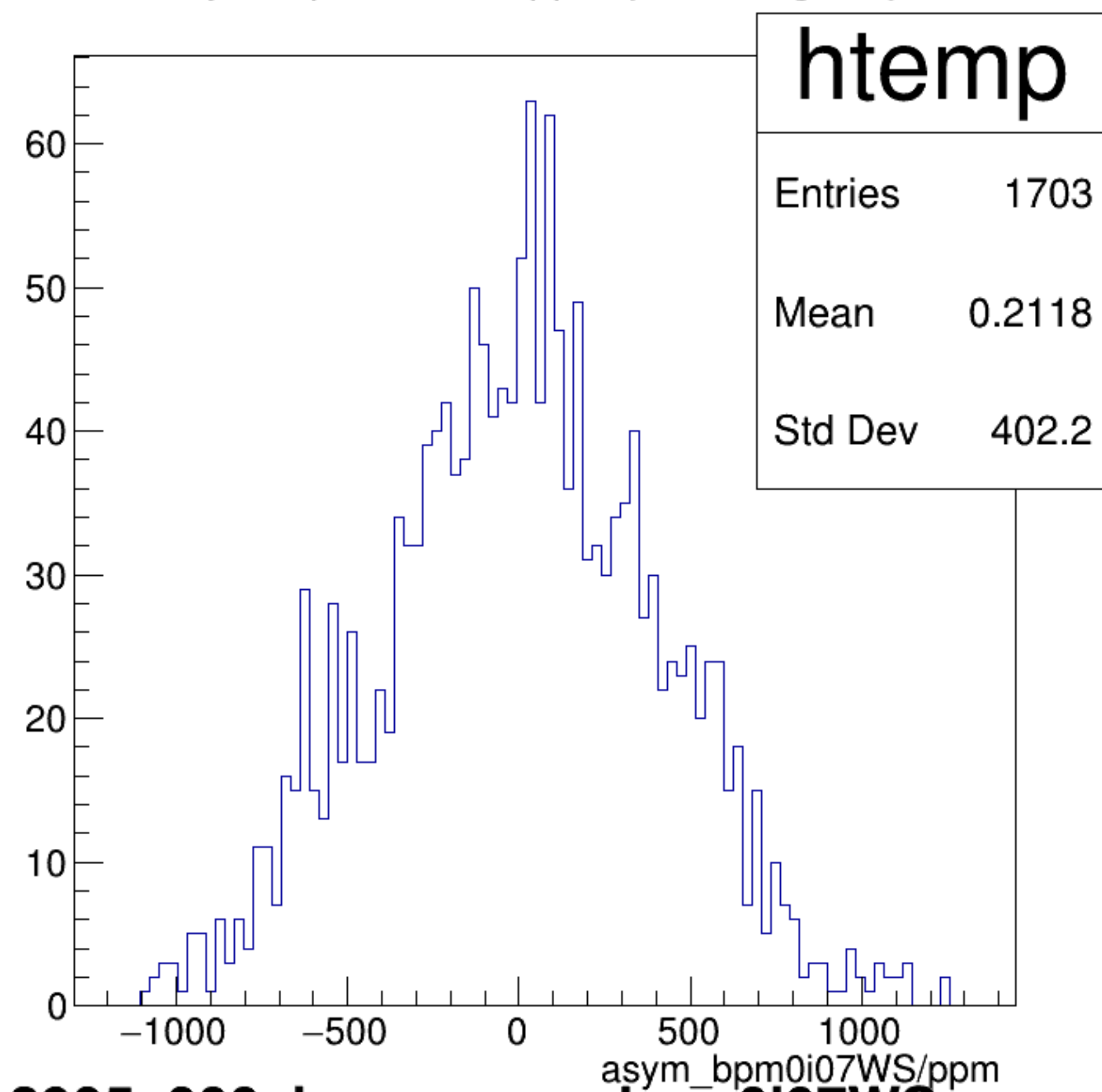
asym_bpm0i07WS/ppm {ErrorFlag==0}
