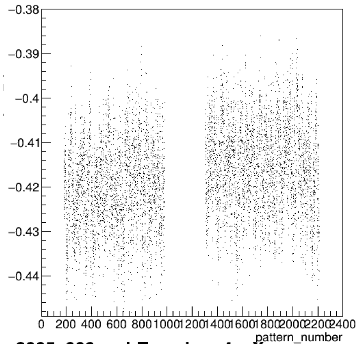
yield_bpm4acX/mm:pattern_number {ErrorFlag==0}
