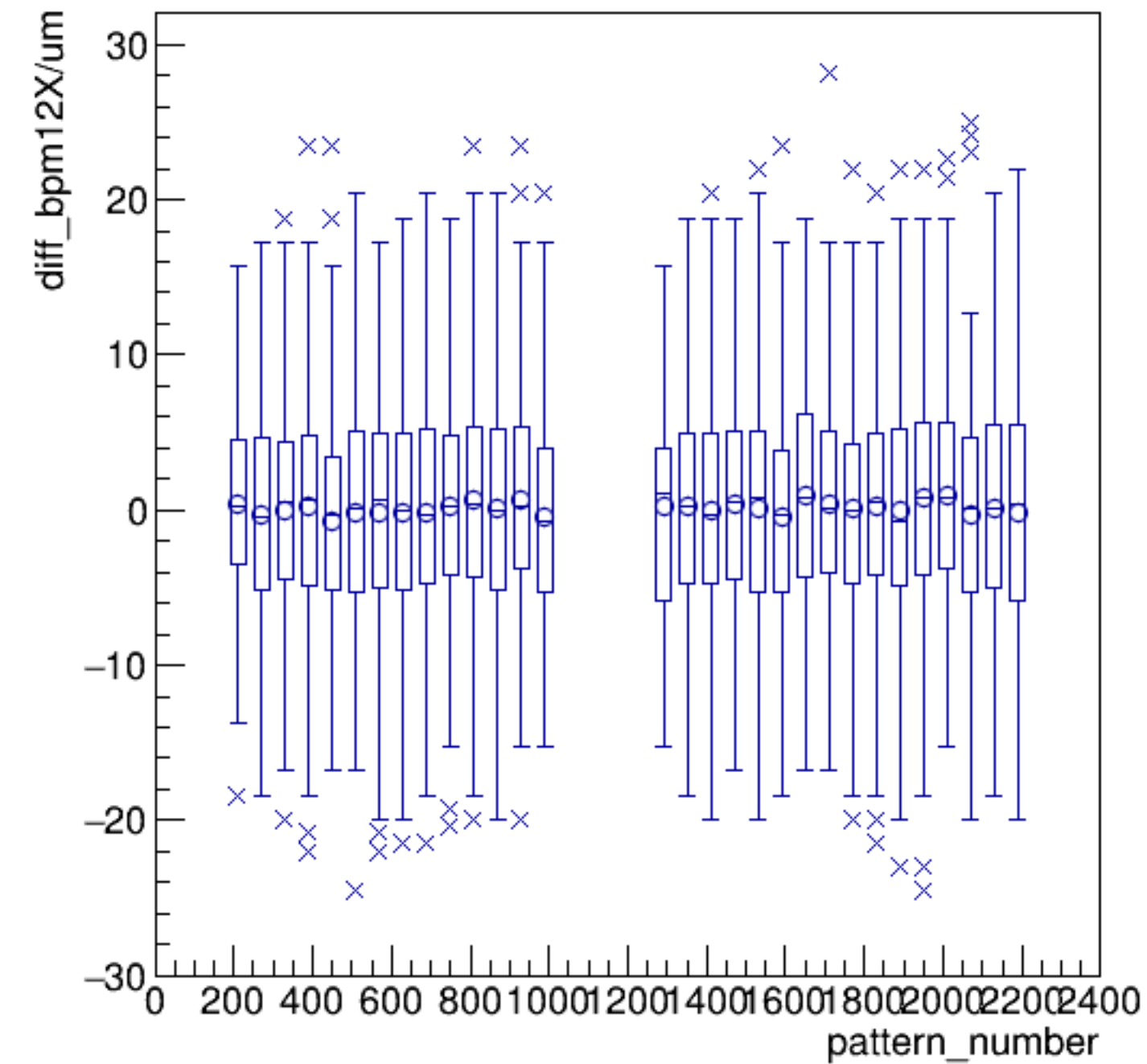
diff_bpm12X/um:pattern_number {ErrorFlag==0}
