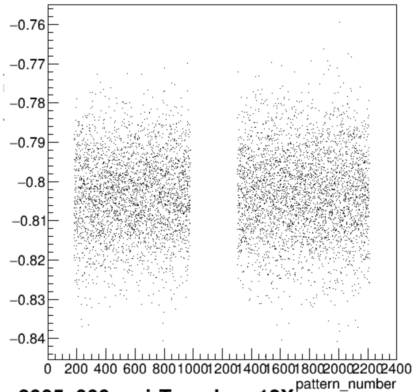
yield_bpm12X/mm:pattern_number {ErrorFlag==0}
