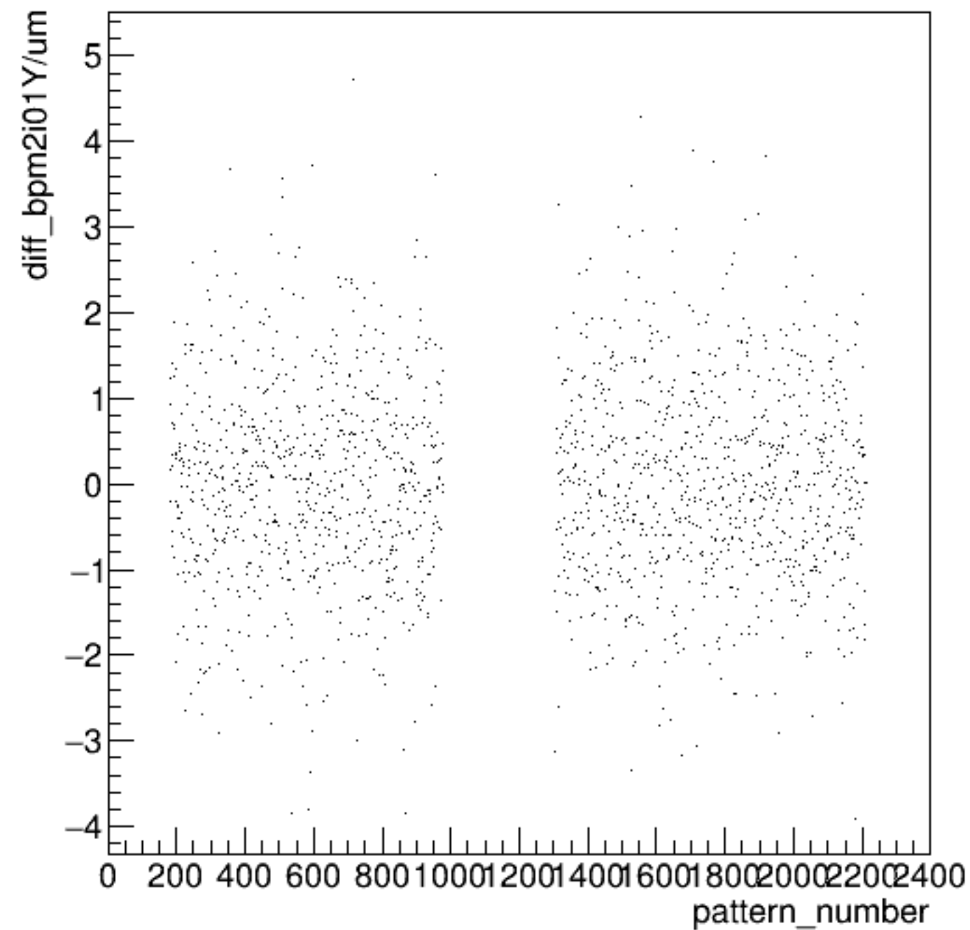
diff_bpm2i01Y/um:pattern_number {ErrorFlag==0}
