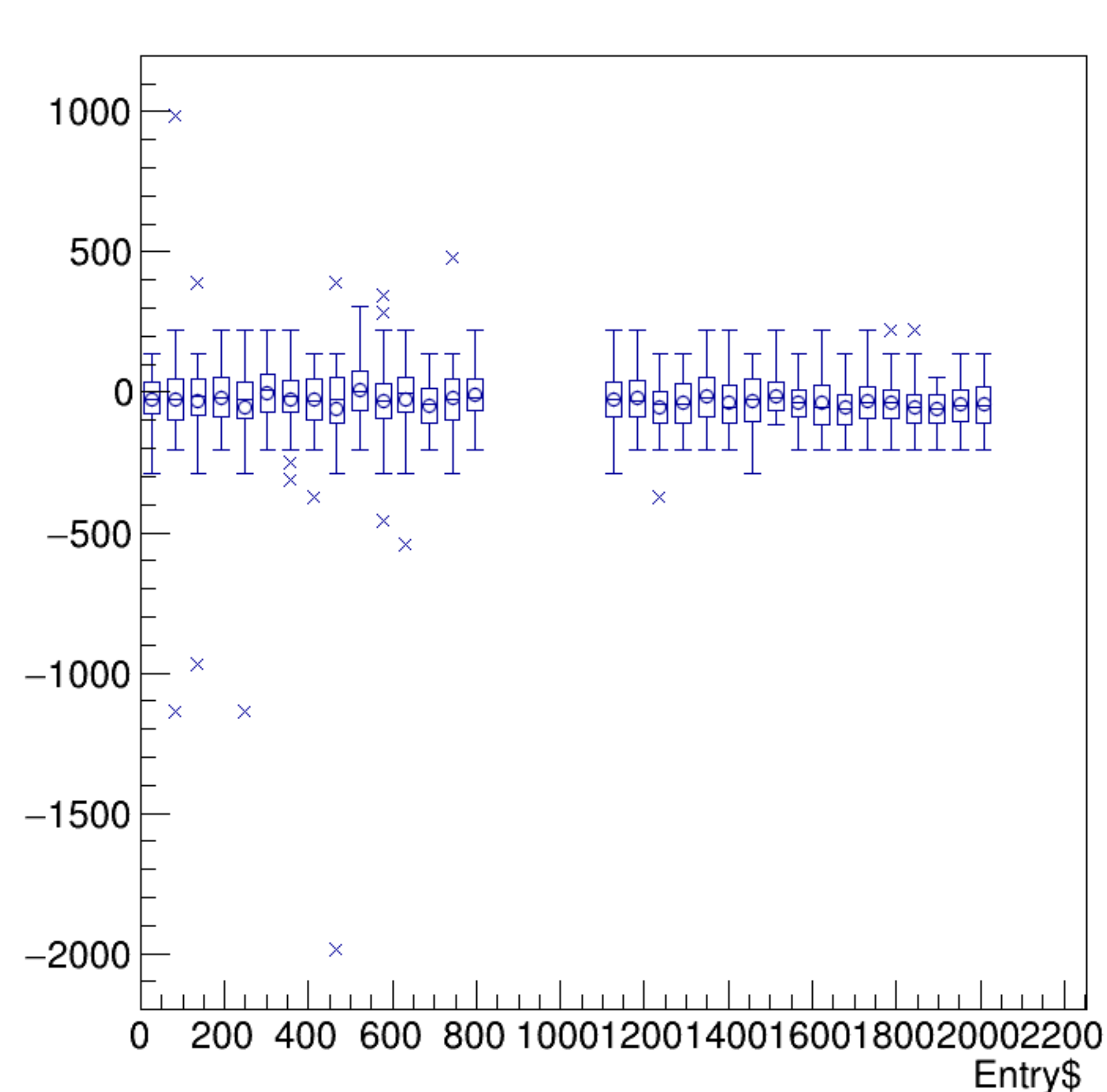
asym_bpm2i01WS/ppm:Entry$ {ErrorFlag==0}
