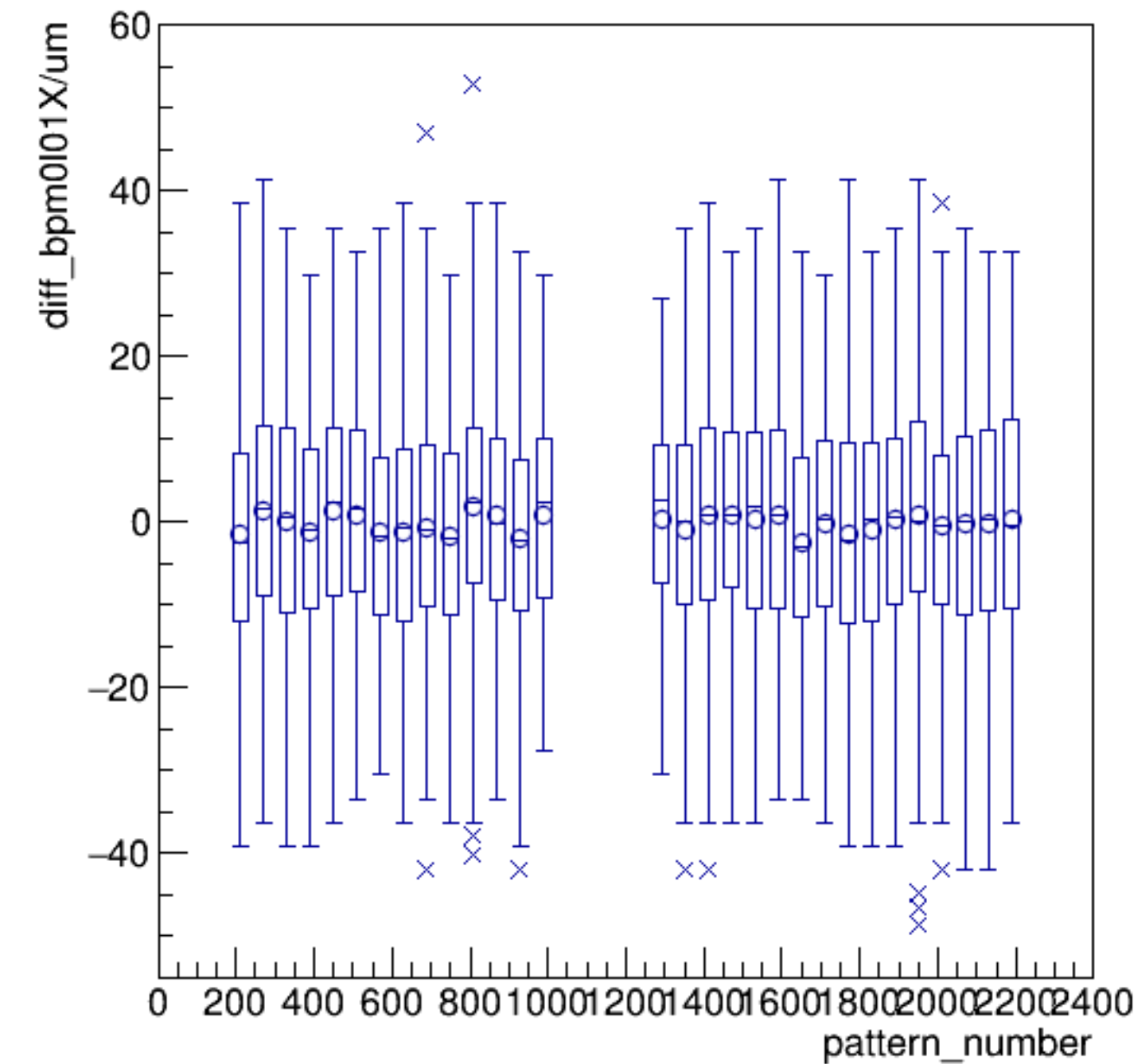
diff_bpm0l01X/um:pattern_number {ErrorFlag==0}
