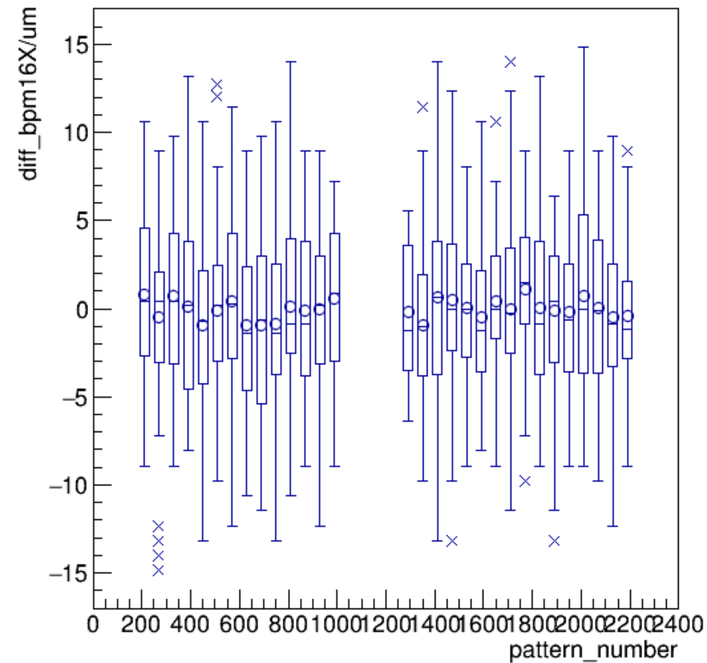
diff_bpm16X/um:pattern_number {ErrorFlag==0}
