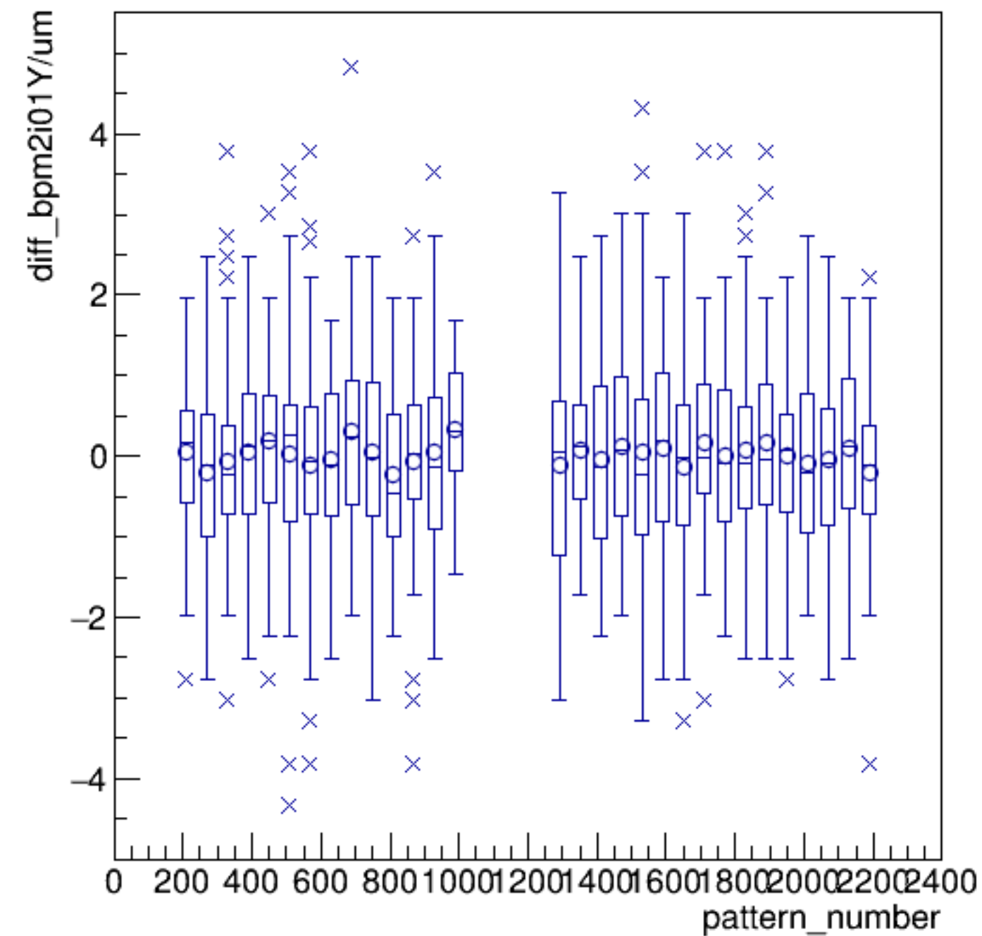
diff_bpm2i01Y/um:pattern_number {ErrorFlag==0}
