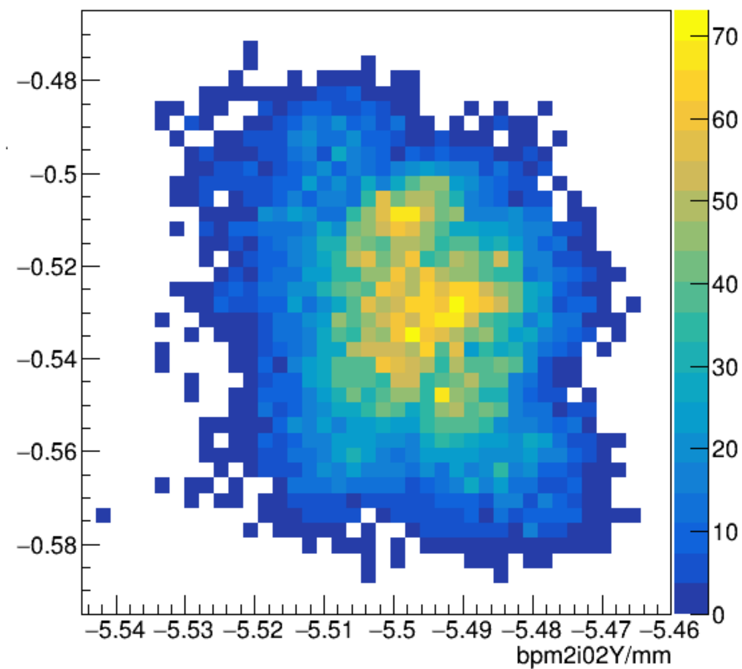
bpm2i02X/mm:bpm2i02Y/mm {ErrorFlag==0}
