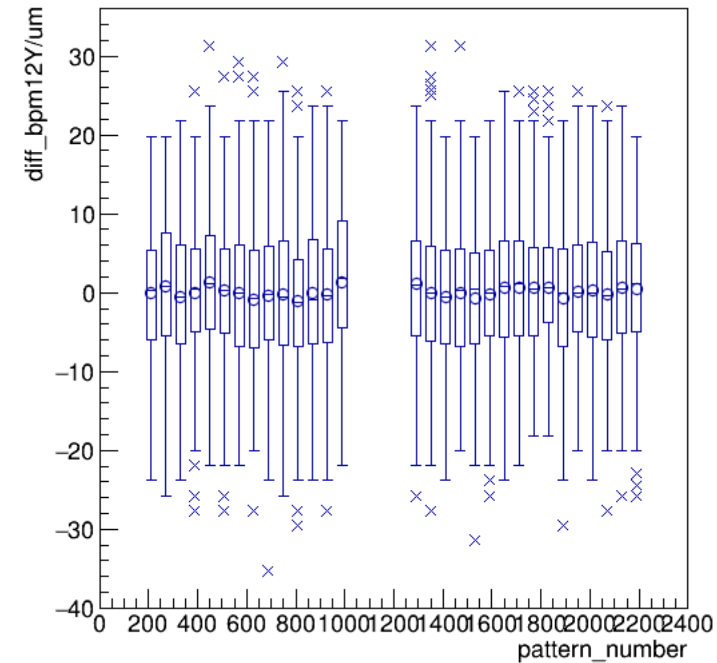
diff_bpm12Y/um:pattern_number {ErrorFlag==0}
