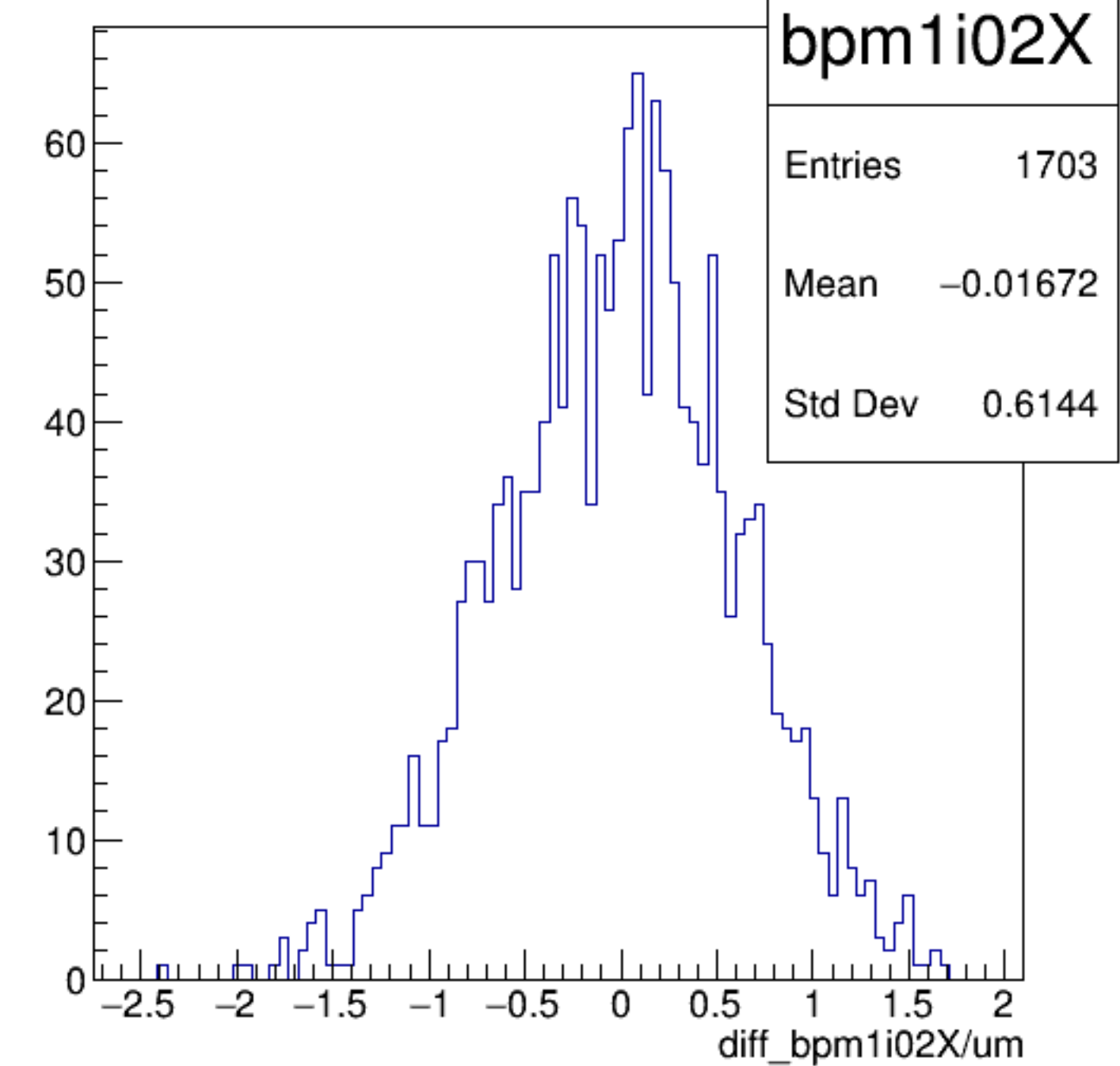
diff_bpm1i02X/um {ErrorFlag==0}
