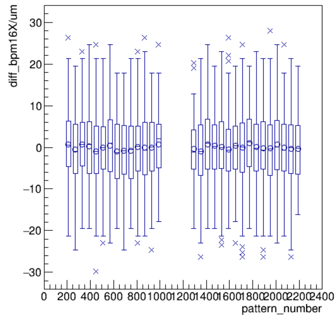
diff_bpm16X/um:pattern_number {ErrorFlag==0}
