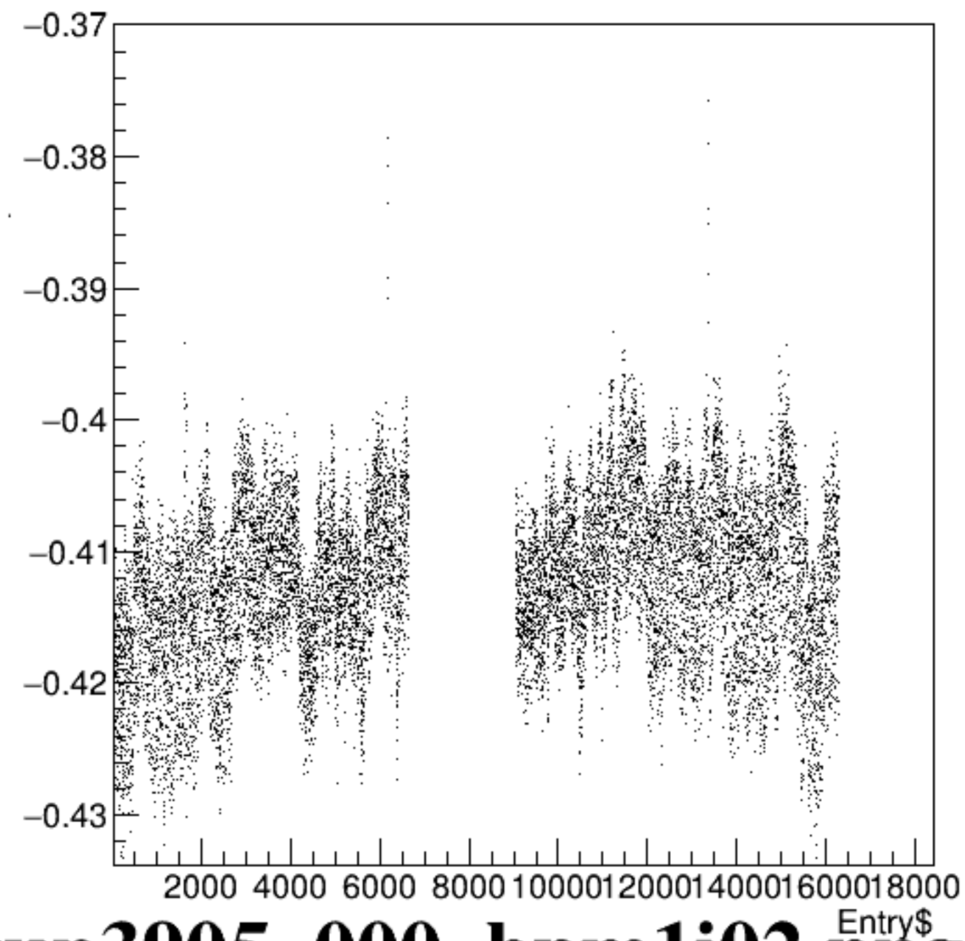
bpm1i02Y/mm:Entry$ {ErrorFlag==0}
