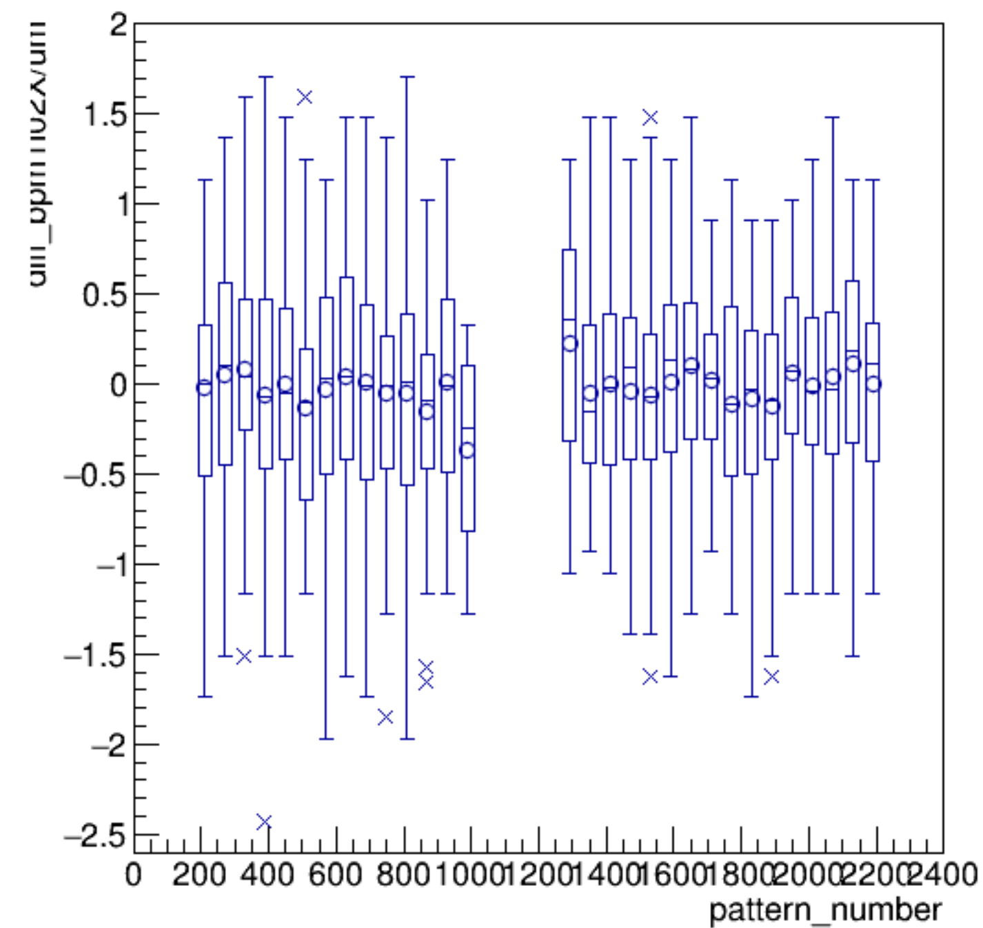
diff_bpm1i02X/um:pattern_number {ErrorFlag==0}
