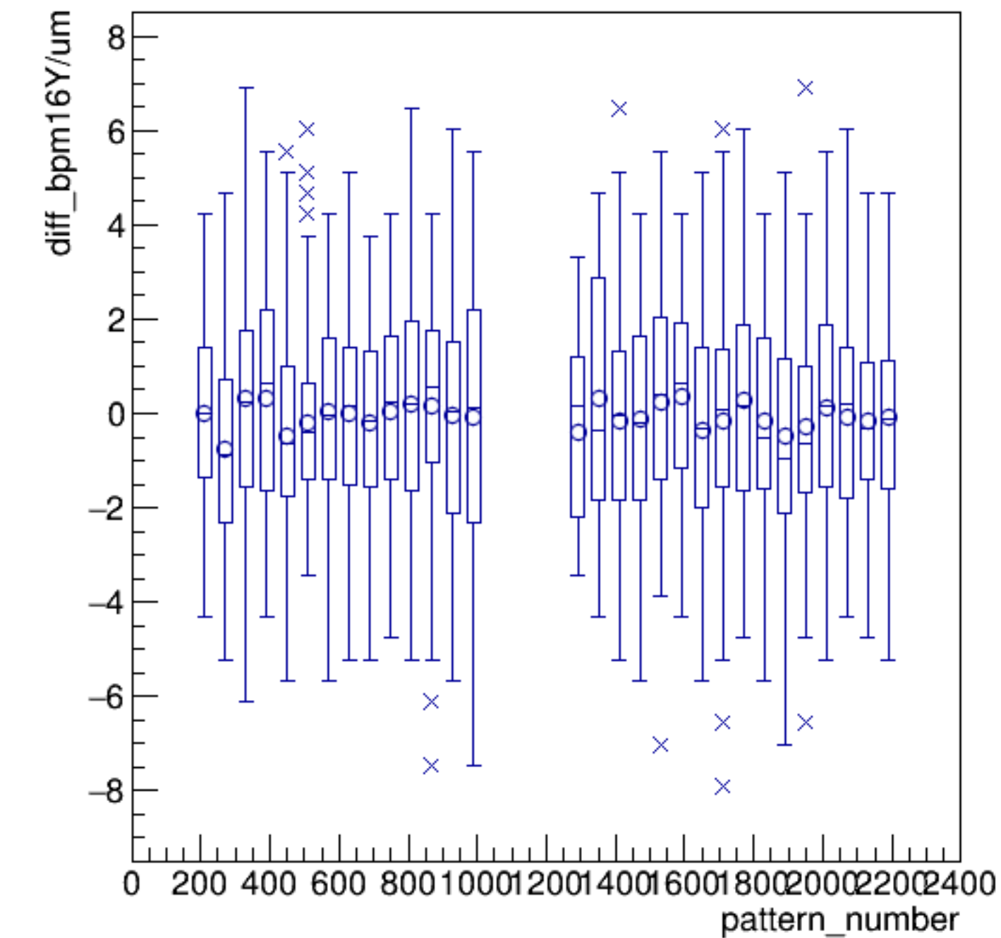
diff_bpm16Y/um:pattern_number {ErrorFlag==0}
