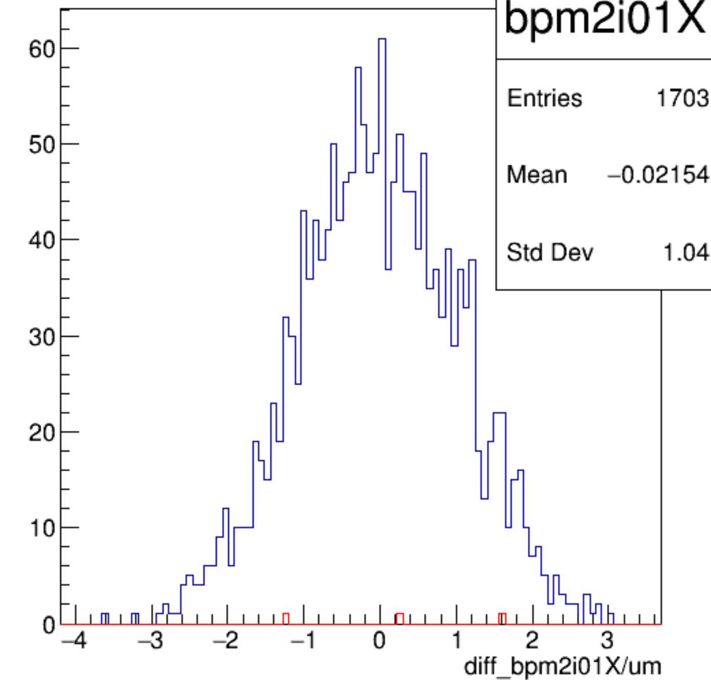
diff_bpm2i01X/um {ErrorFlag==0}
