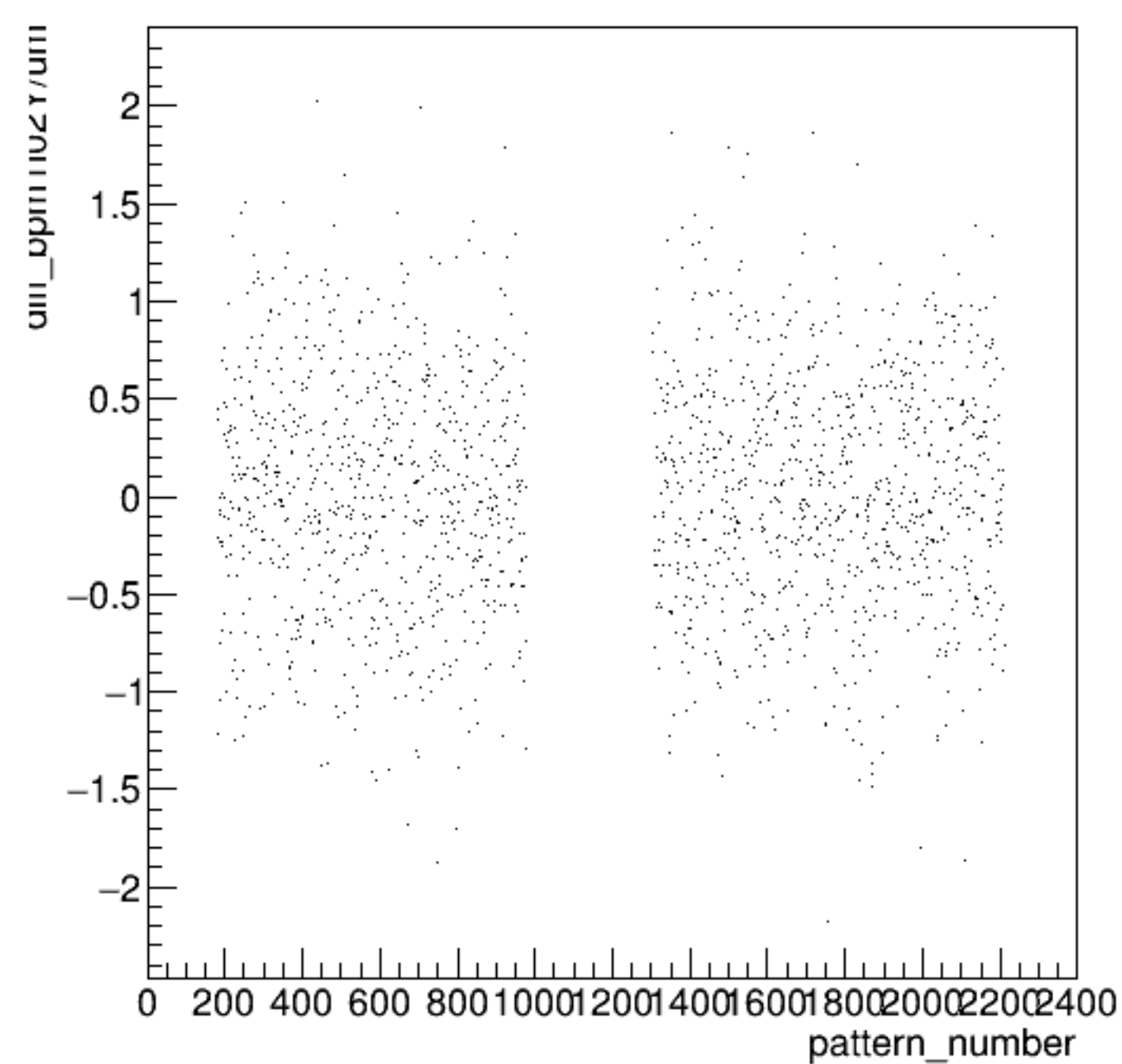
diff_bpm1i02Y/um:pattern_number {ErrorFlag==0}
