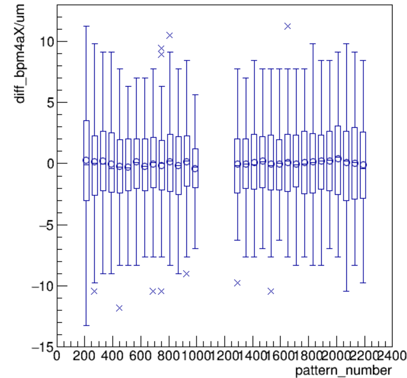
diff_bpm4aX/um:pattern_number {ErrorFlag==0}
