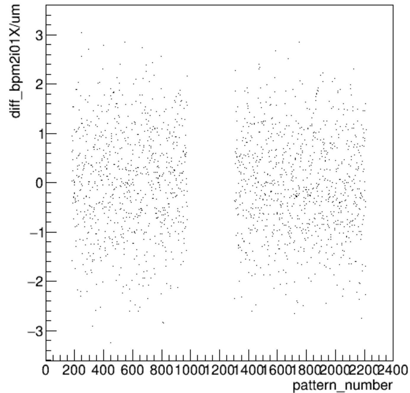
diff_bpm2i01X/um:pattern_number {ErrorFlag==0}
