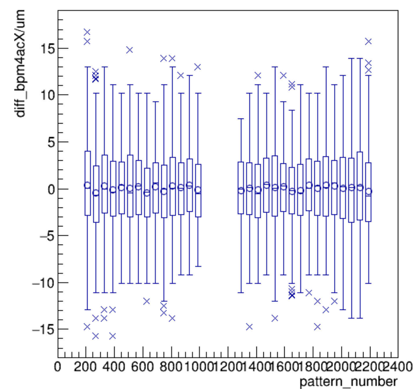
diff_bpm4acX/um:pattern_number {ErrorFlag==0}
