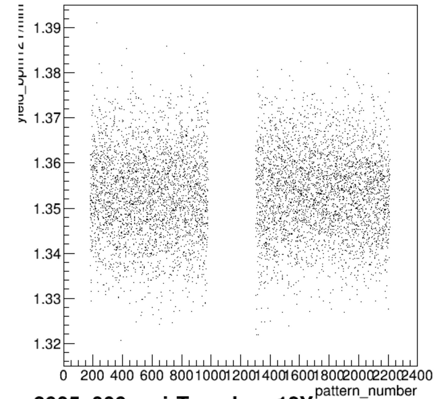
yield_bpm12Y/mm:pattern_number {ErrorFlag==0}
