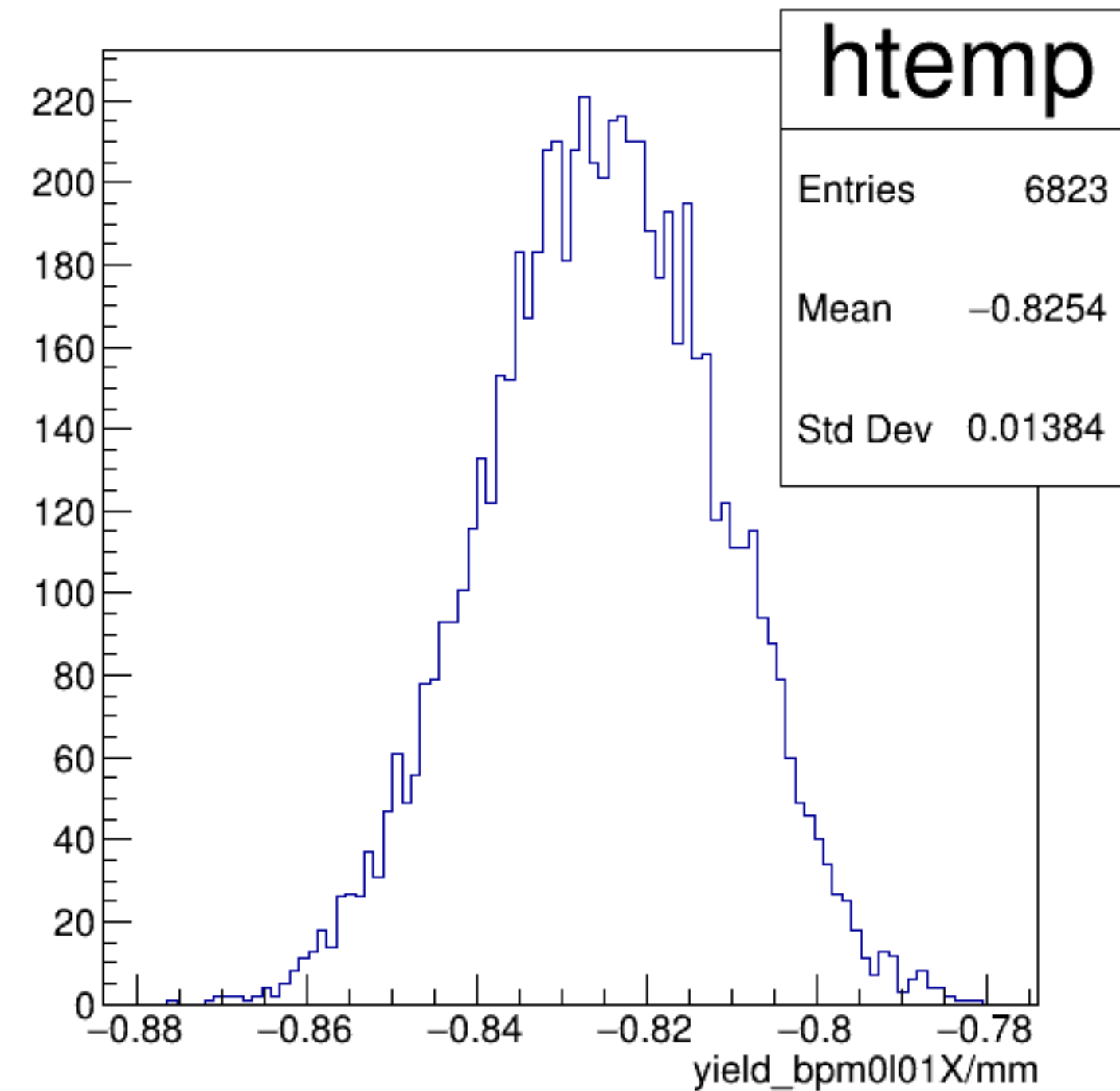
yield_bpm0l01X/mm {ErrorFlag==0}
