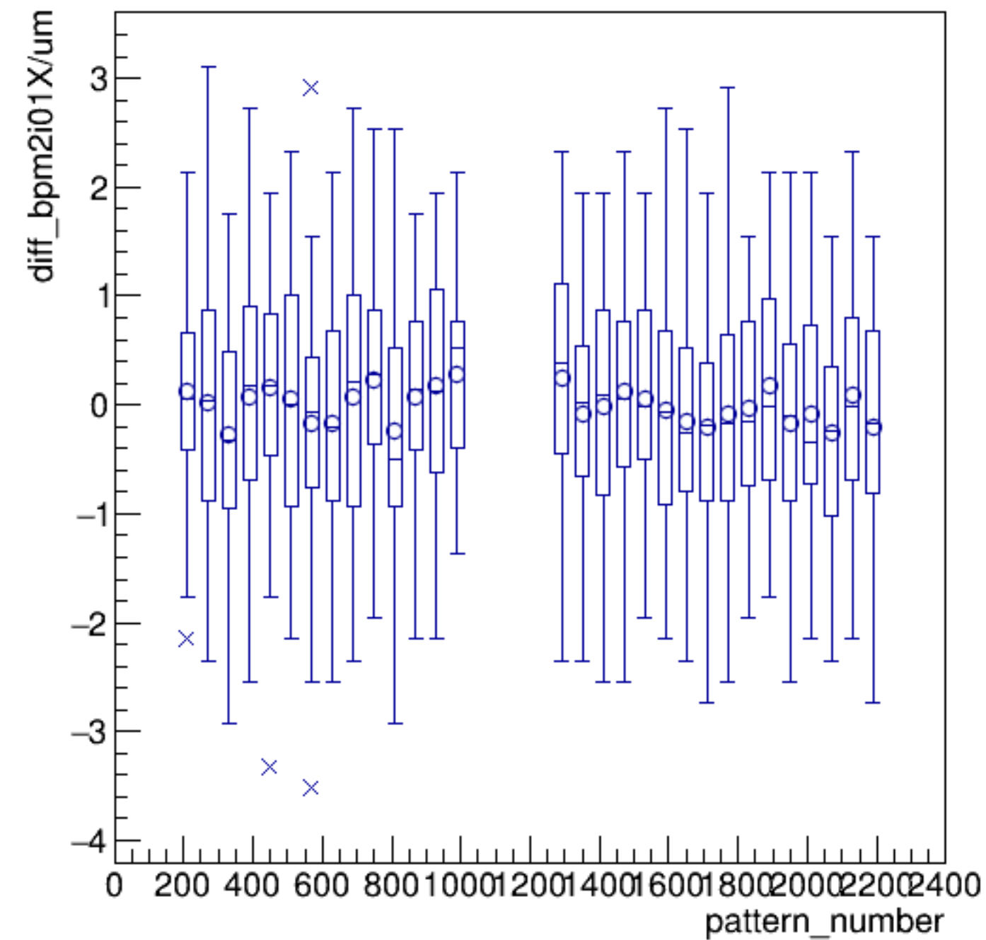
diff_bpm2i01X/um:pattern_number {ErrorFlag==0}
