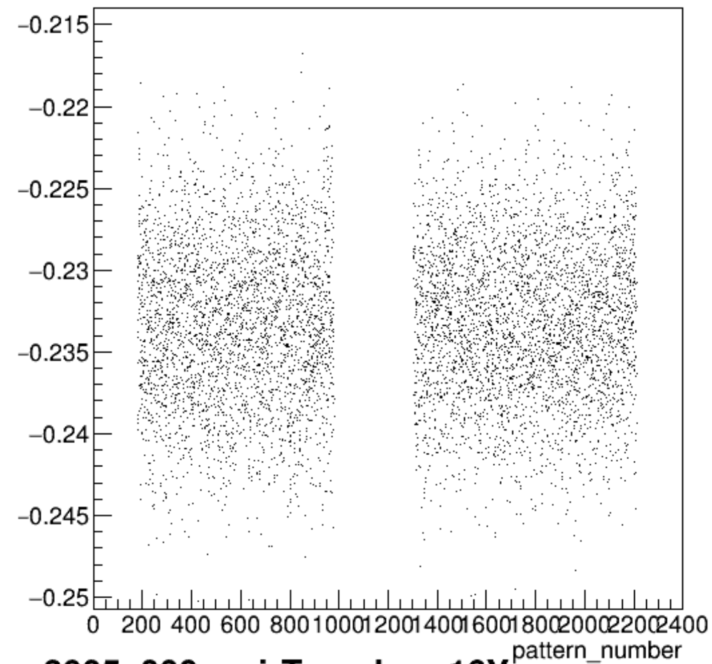
yield_bpm16Y/mm:pattern_number {ErrorFlag==0}
