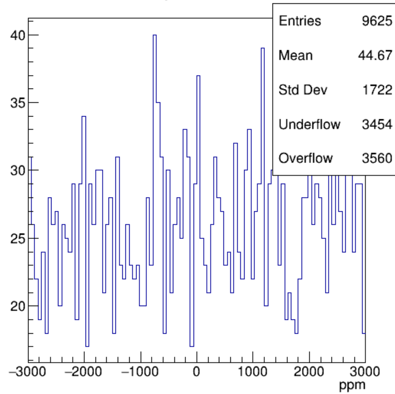
asym_sam3
