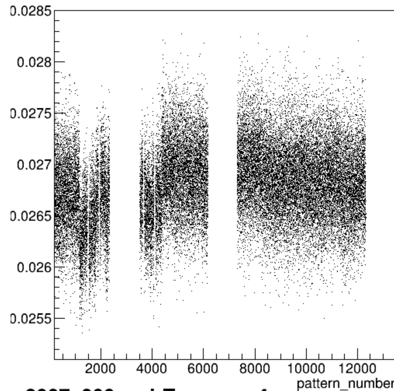
yield_sam4:pattern_number {ErrorFlag==0}
