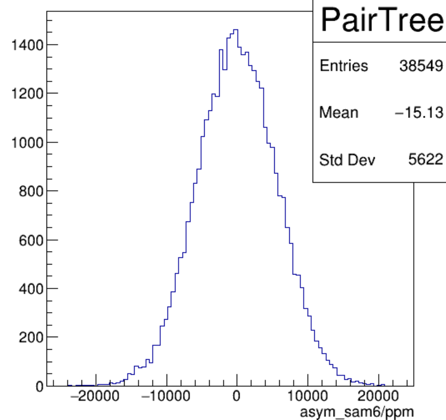
asym_sam6/ppm {ErrorFlag==0}
