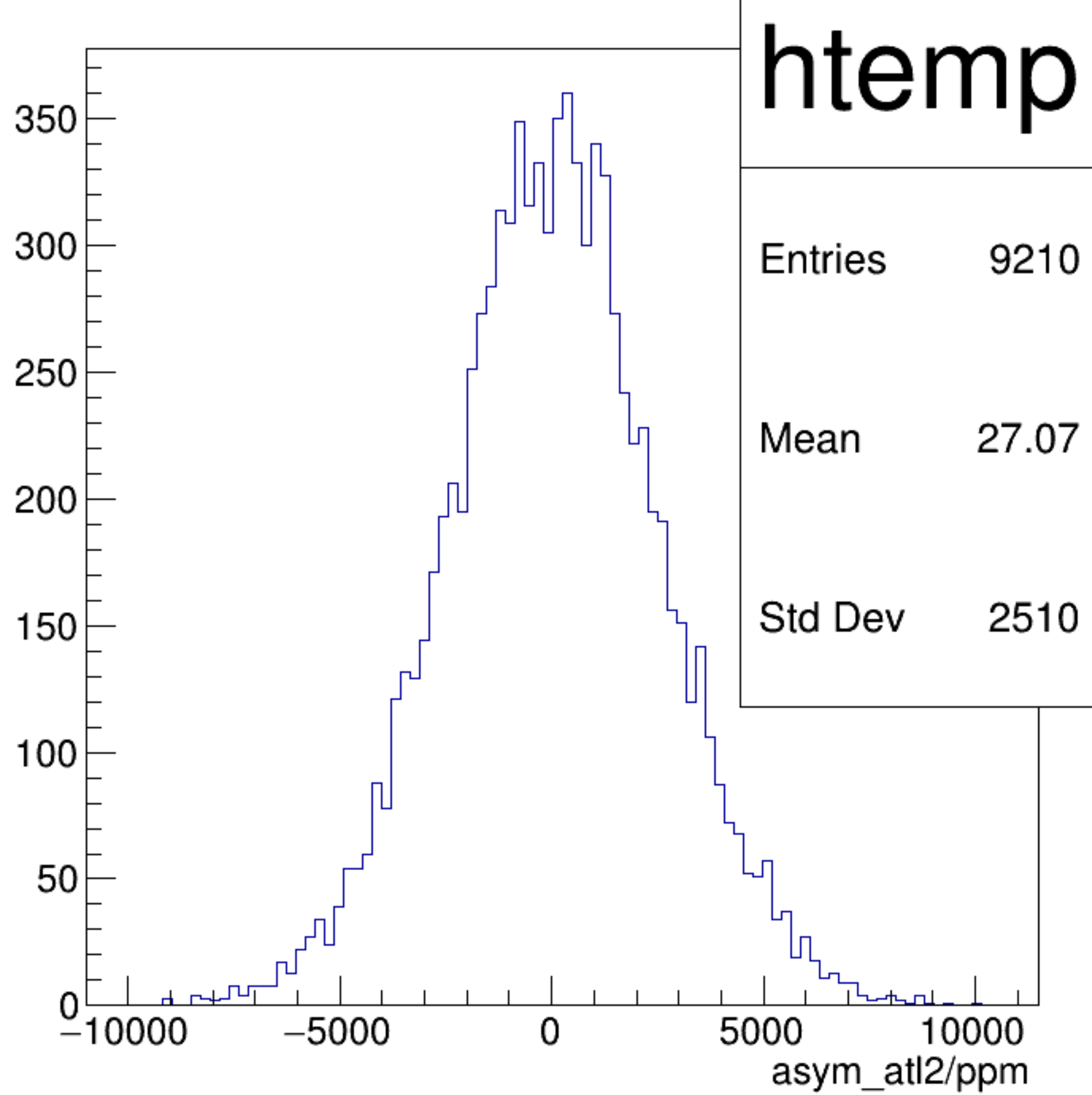
asym_atl2/ppm {ok_cut}
