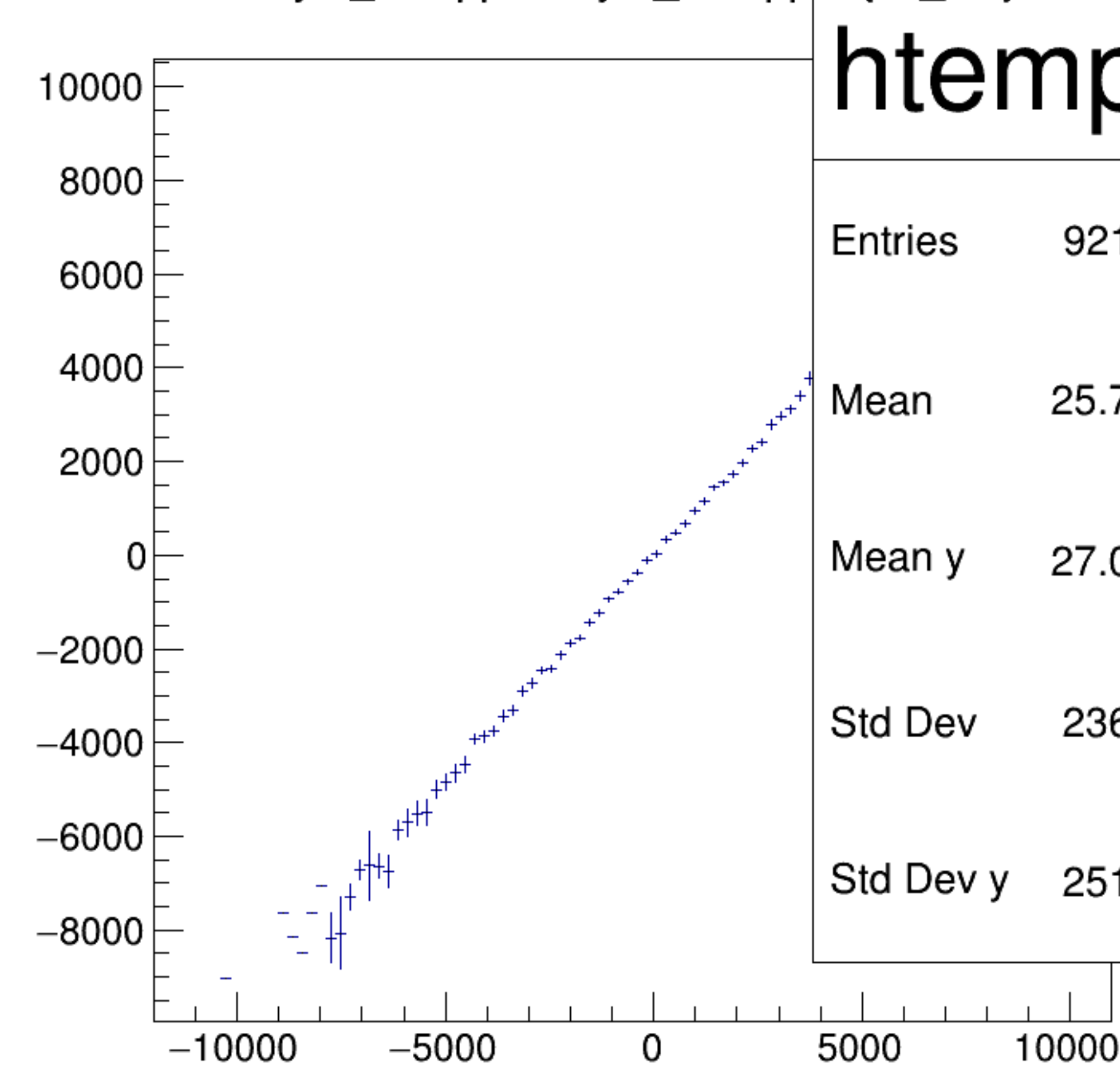
asym_atl2/ppm:asym_atr2/ppm {ok_cut}
