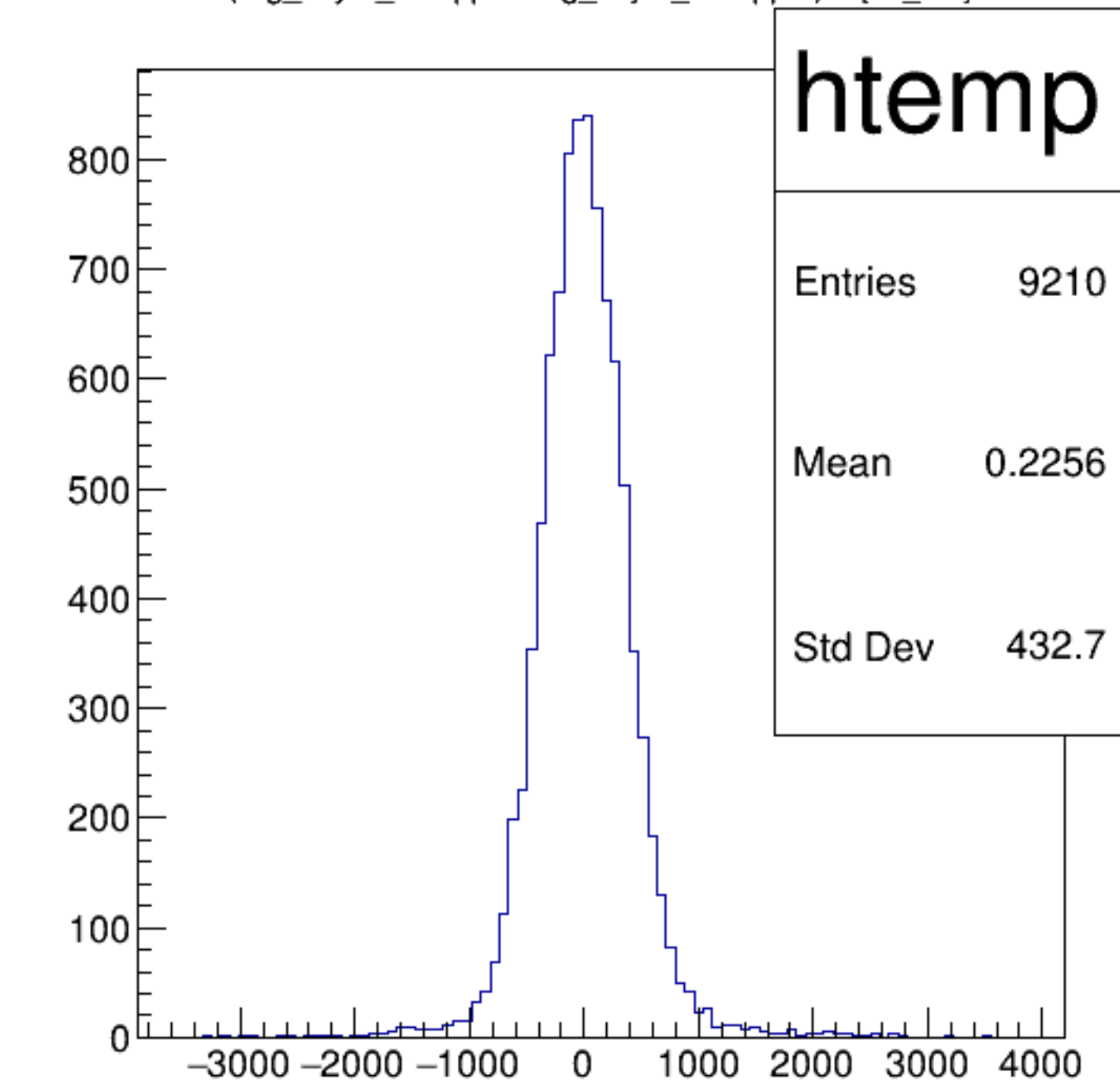
(reg_asym_atl1/ppm+reg_asym_atr1/ppm)/2 {ok_cut}
