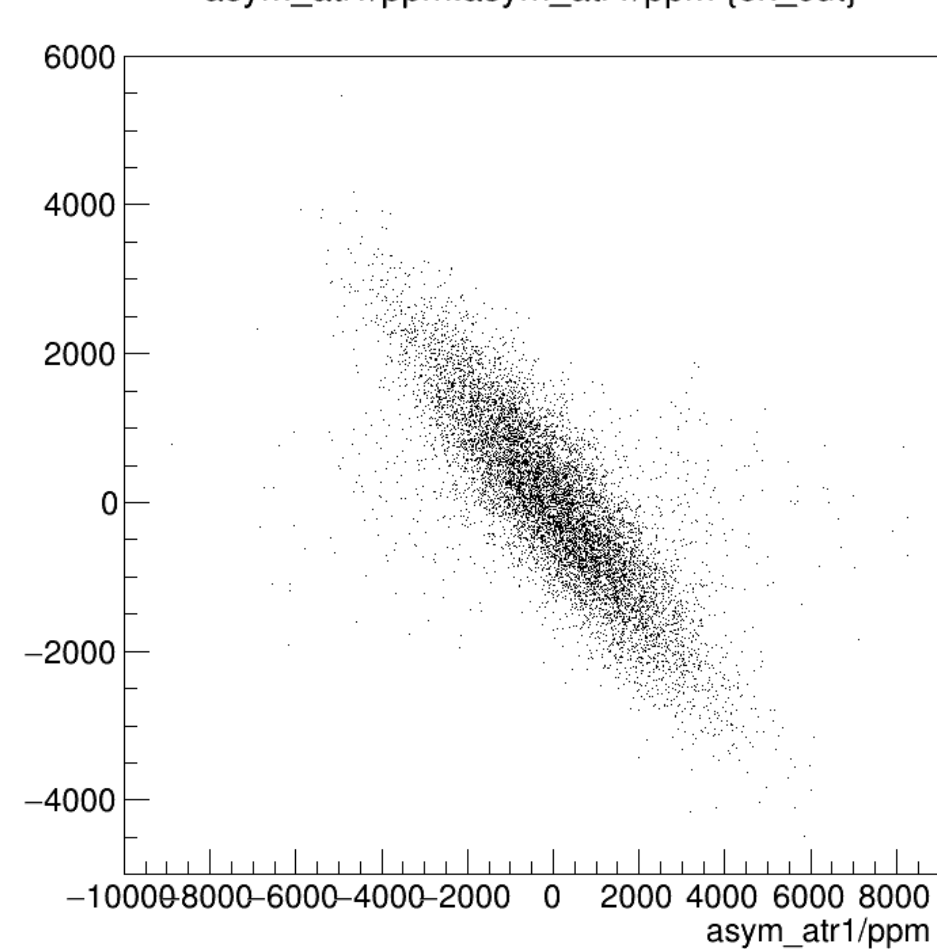
asym_atl1/ppm:asym_atr1/ppm {ok_cut}
