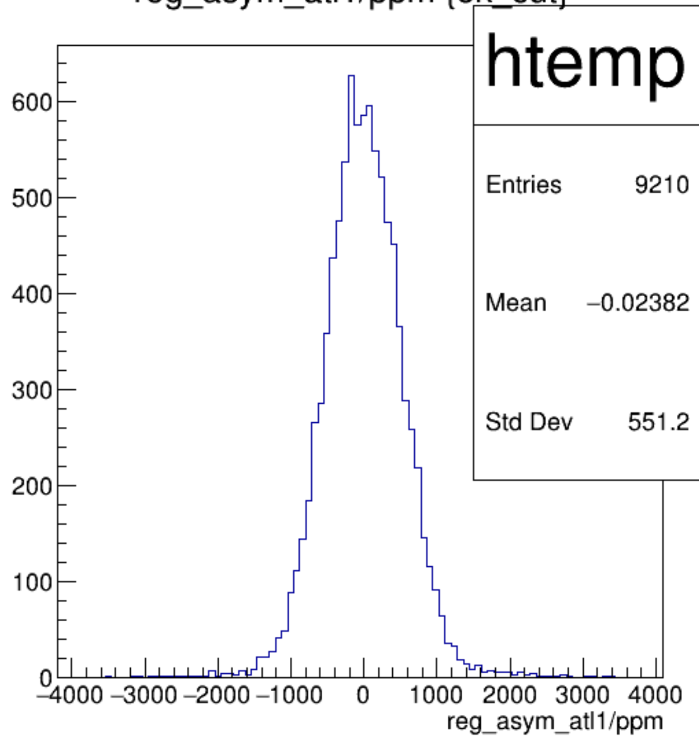
reg_asym_atl1/ppm {ok_cut}
