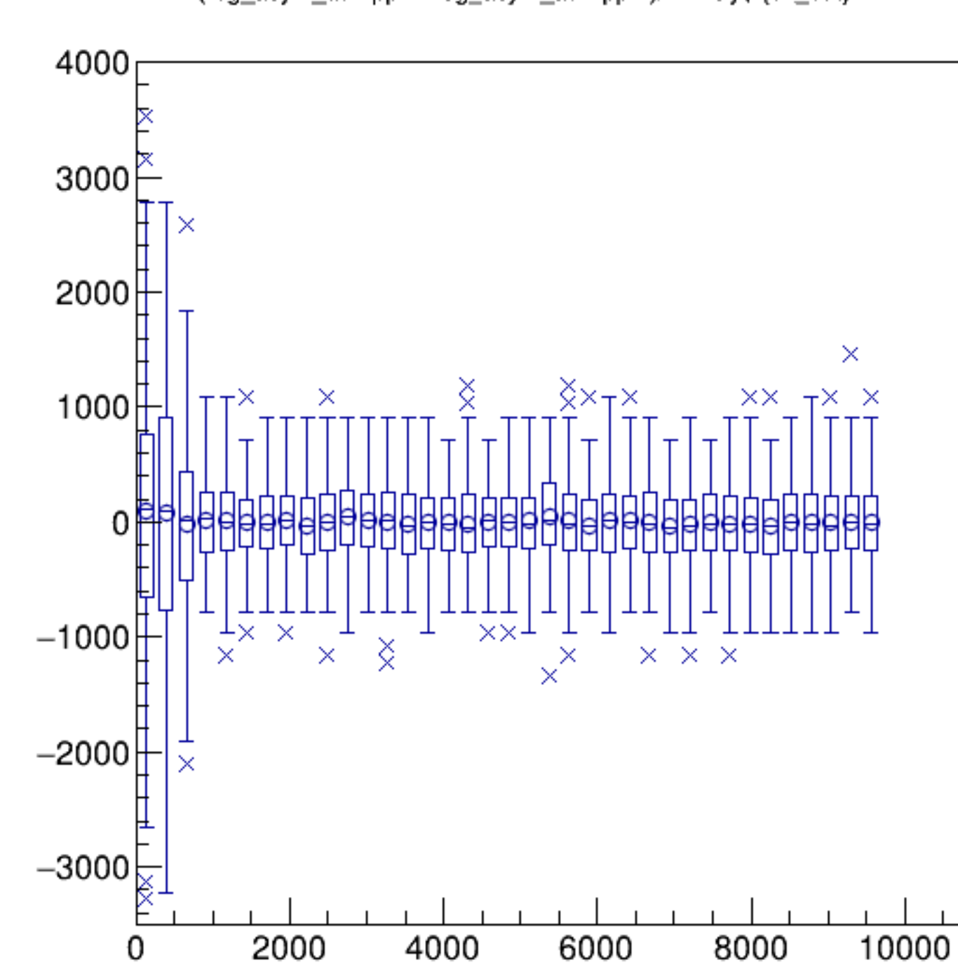
(reg_asym_atl1/ppm+reg_asym_atr1/ppm)/2:Entry$ {ok_cut}
