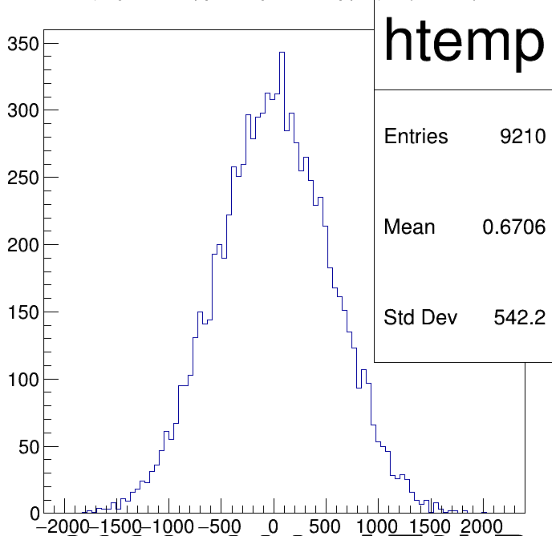
(asym_atl2/ppm-asym_atr2/ppm)/2 {ok_cut}
