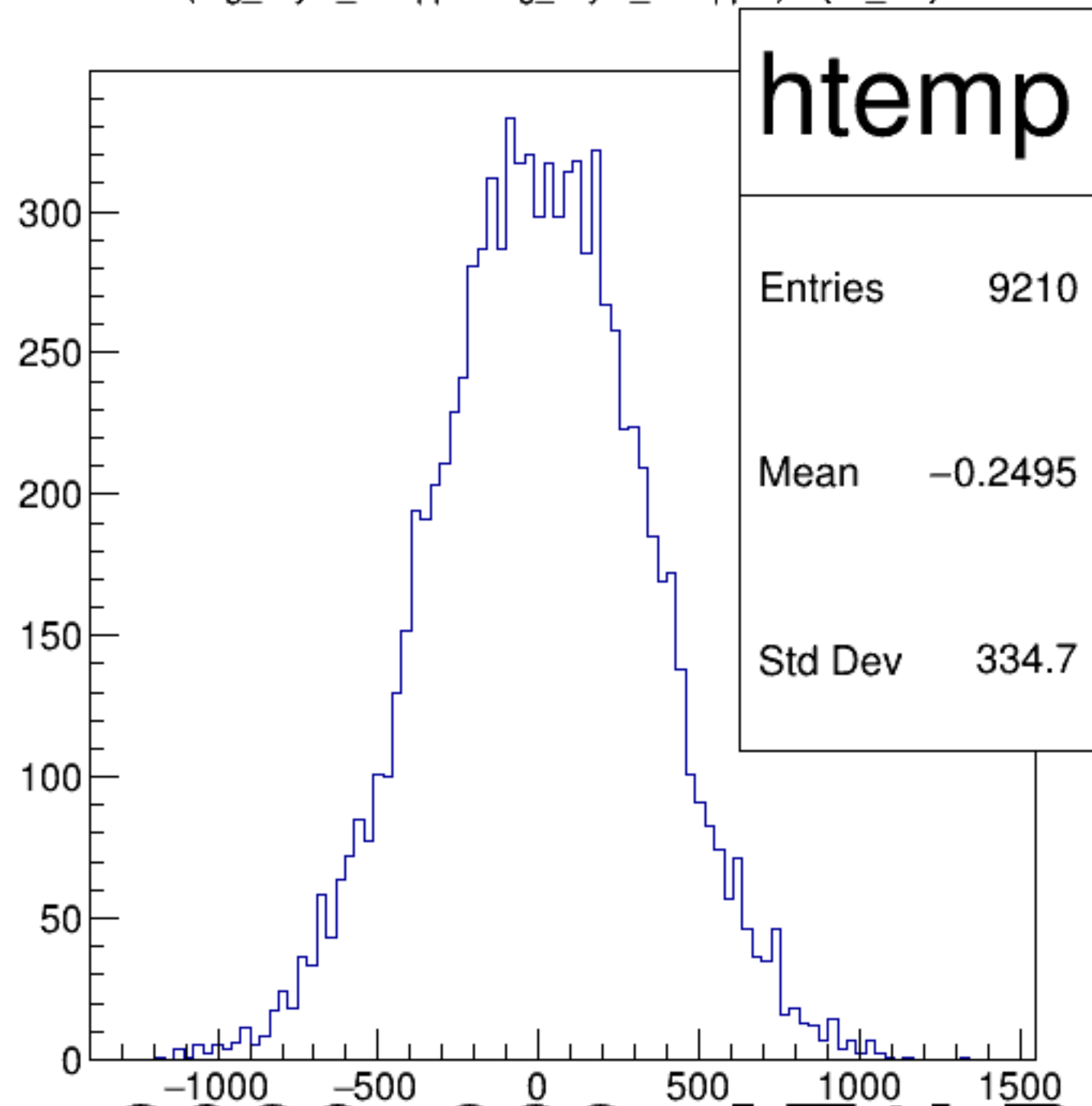
(reg_asym_atl1/ppm-reg_asym_atr1/ppm)/2 {ok_cut}
