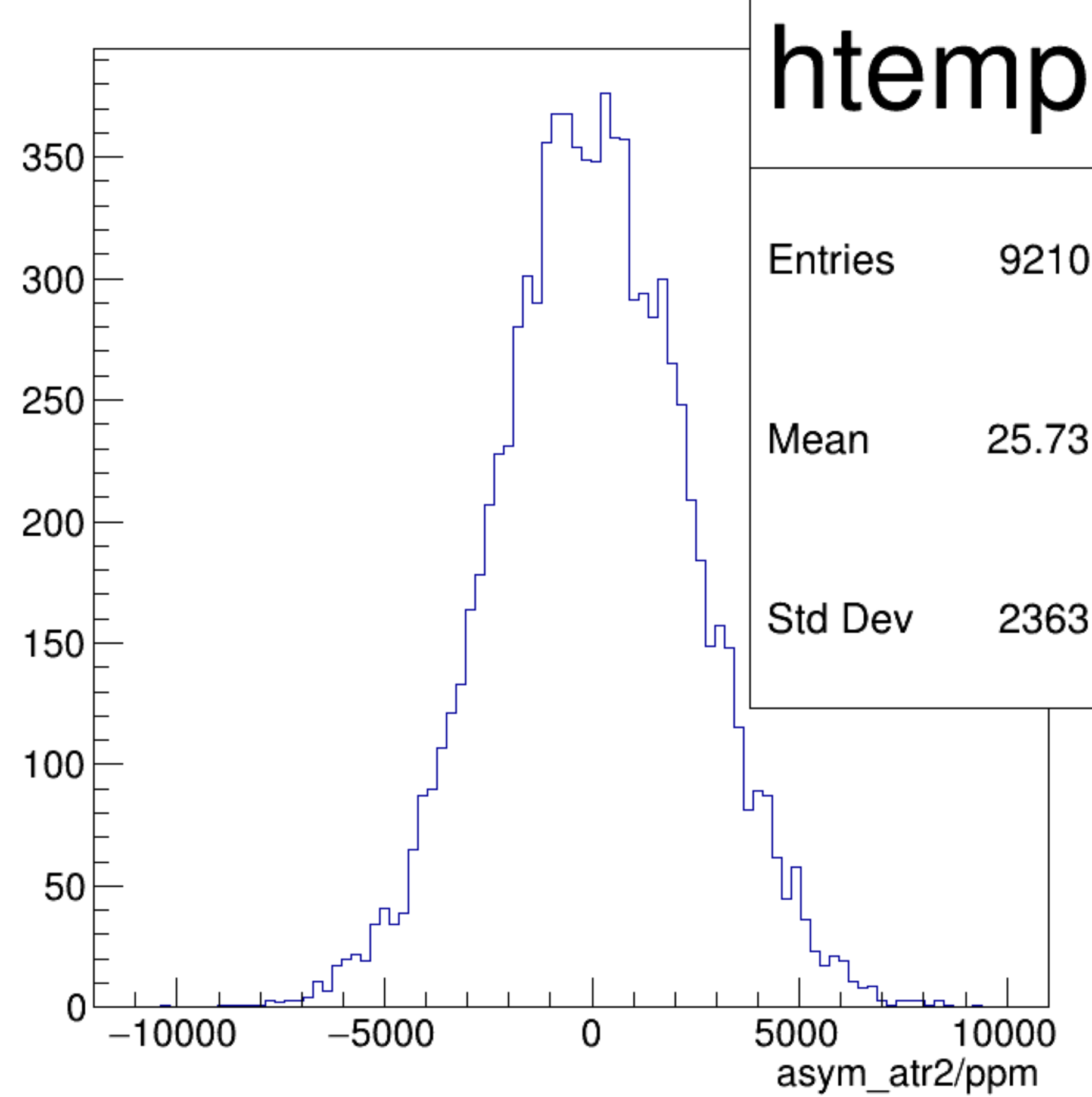
asym_atr2/ppm {ok_cut}
