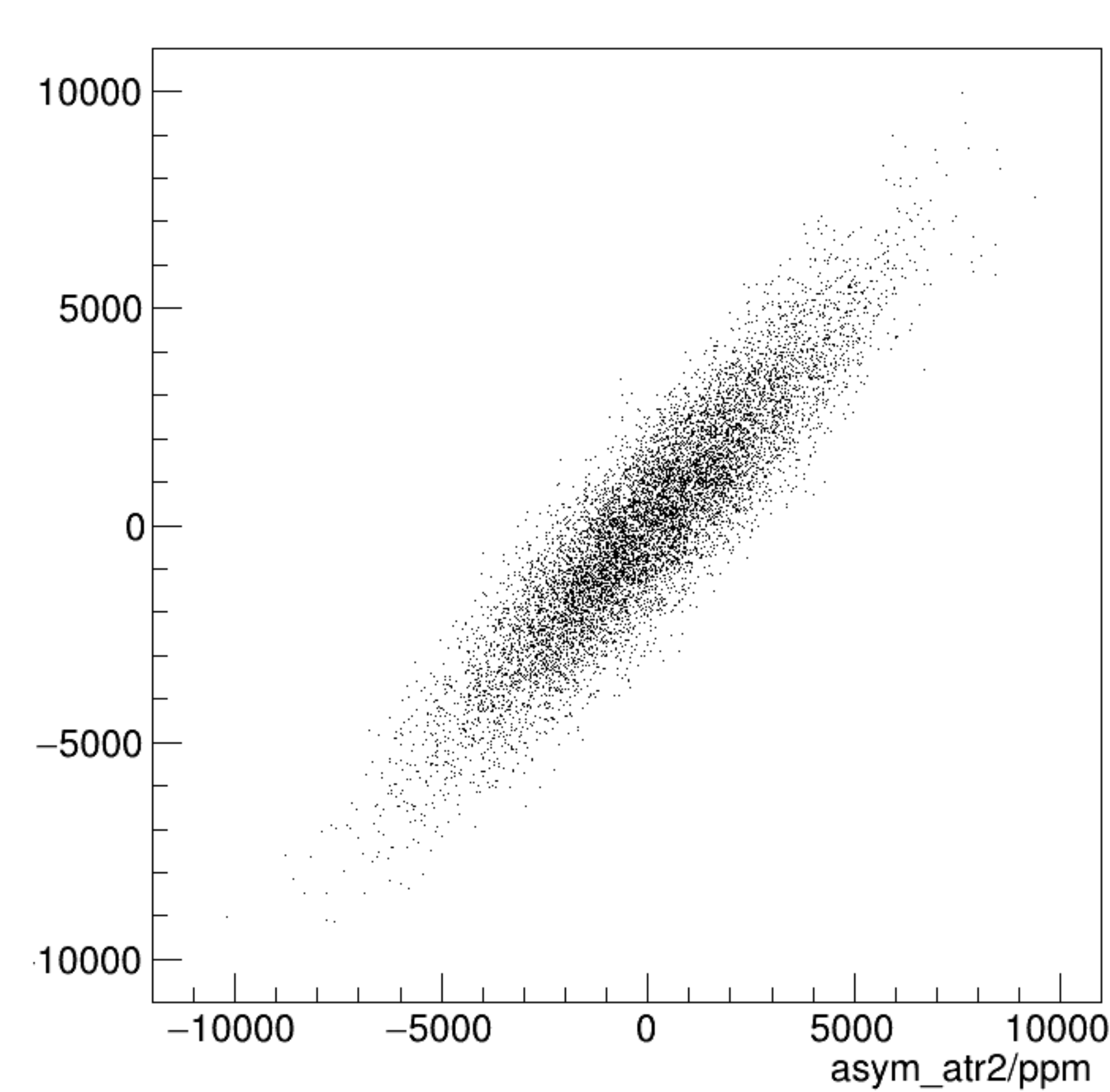
asym_atl2/ppm:asym_atr2/ppm {ok_cut}
