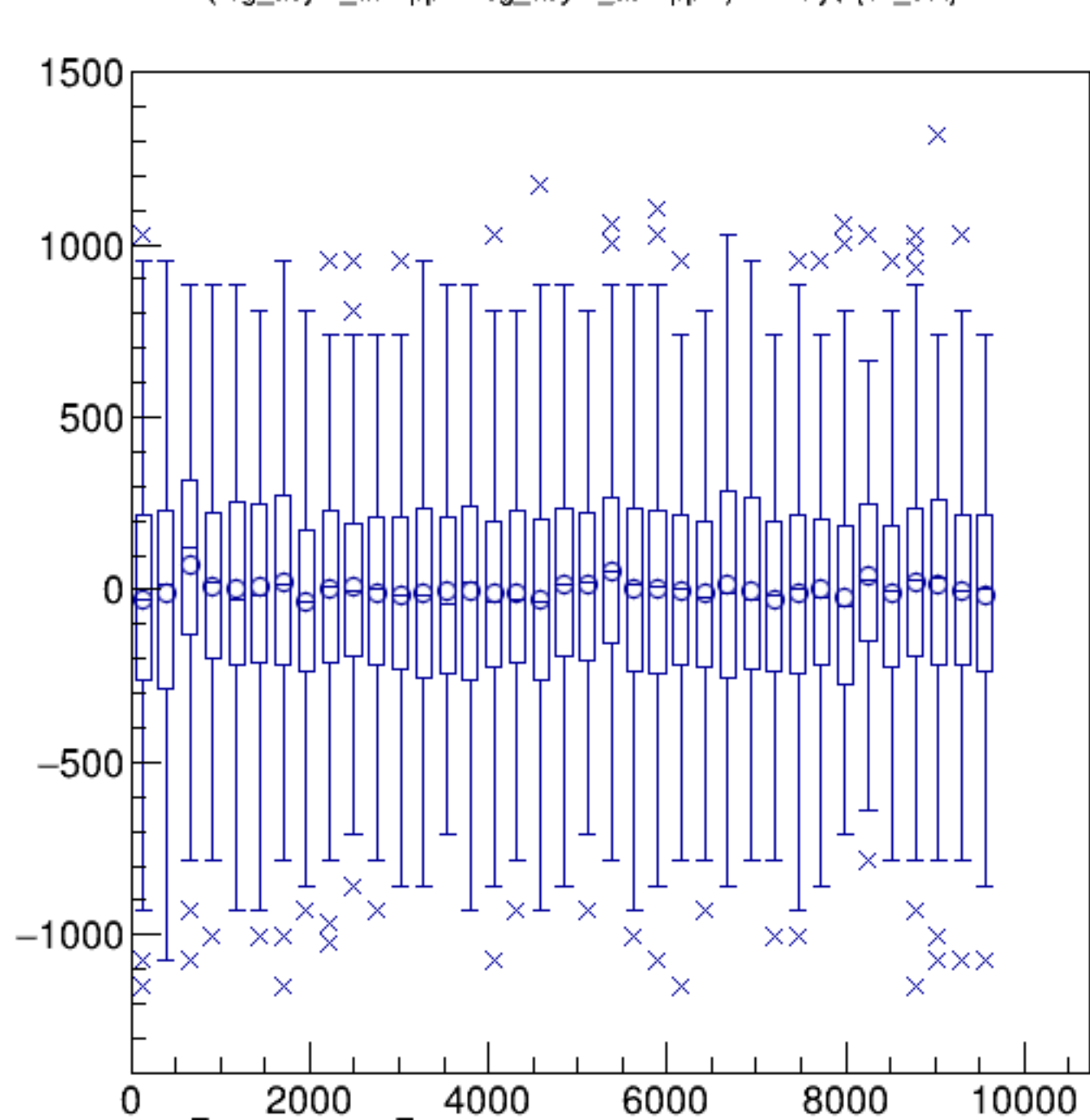
(reg_asym_atl1/ppm-reg_asym_atr1/ppm)/2:Entry$ {ok_cut}
