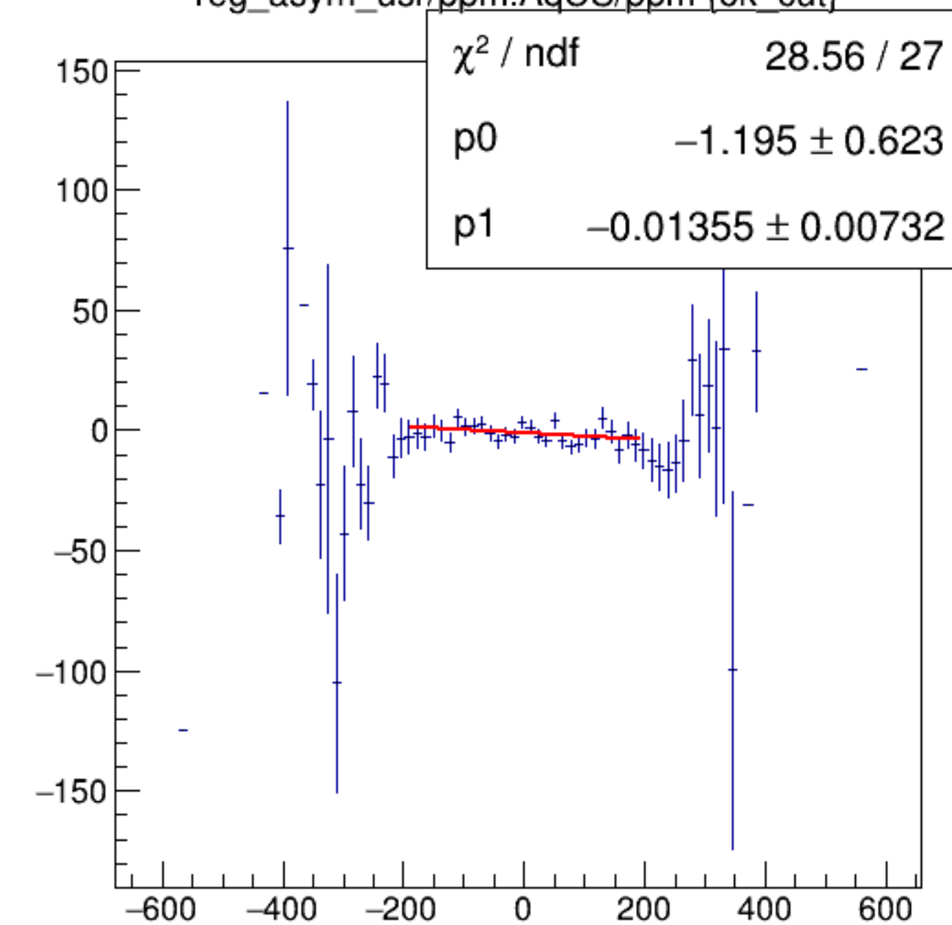
reg_asym_usr/ppm:AqUS/ppm {ok_cut}
