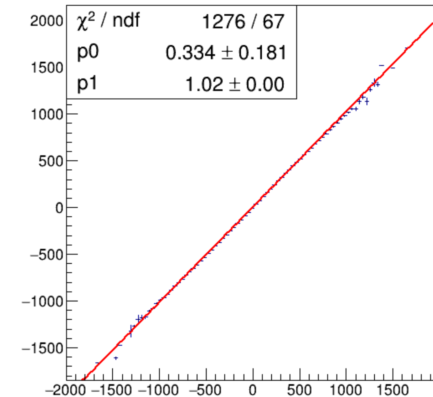
run3944_000_asym_bcm_dg_us_vs_asym_bcm_dg_ds_pr.png
