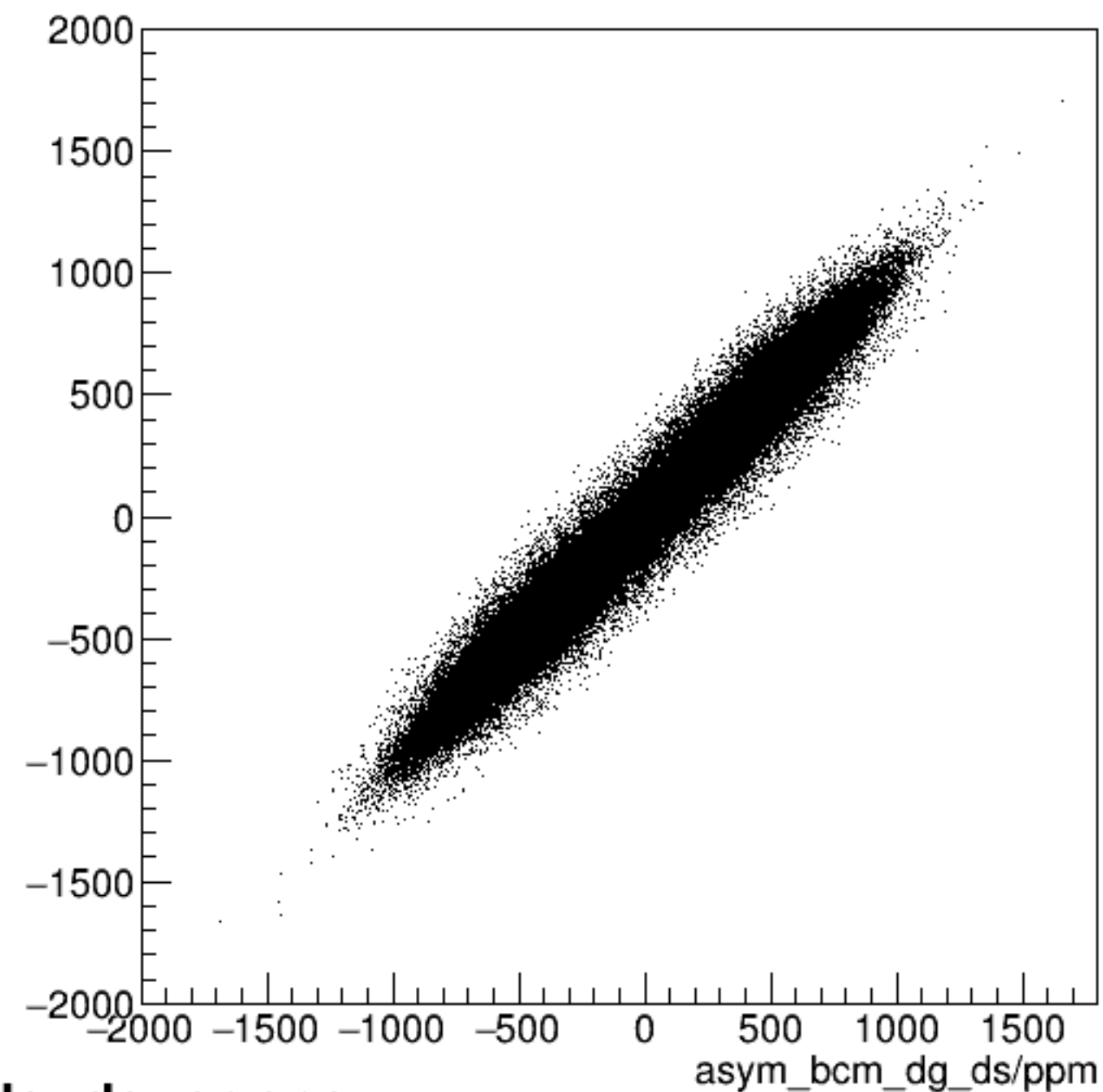
run3944_000_asym_bcm_dg_us_vs_asym_bcm_dg_ds_pr.png
