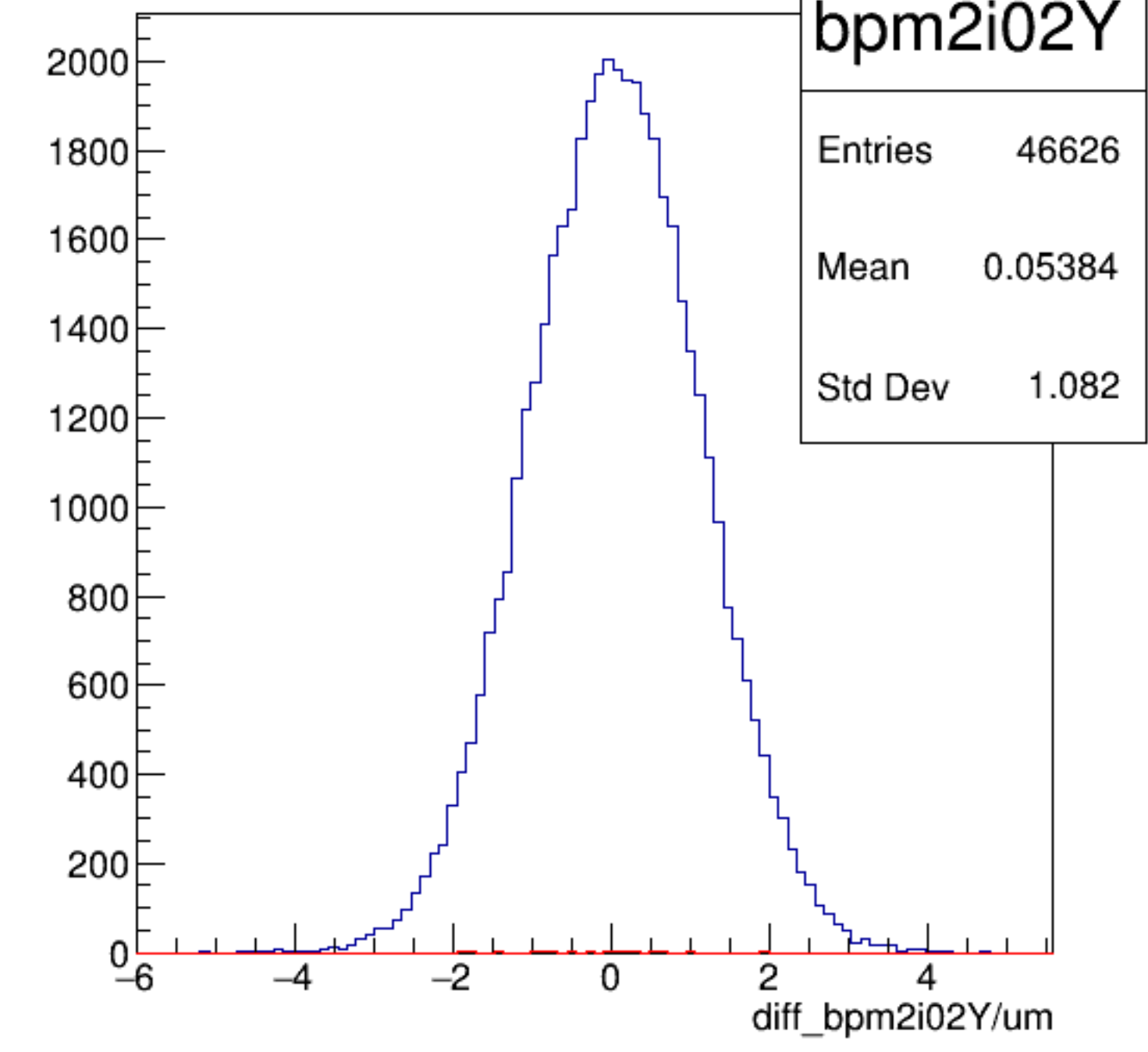
diff_bpm2i02Y/um {ErrorFlag==0}
