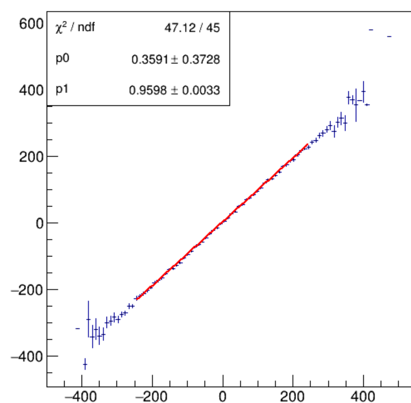
asym_bpm16WS/ppm:Aq/ppm {ErrorFlag==0}
