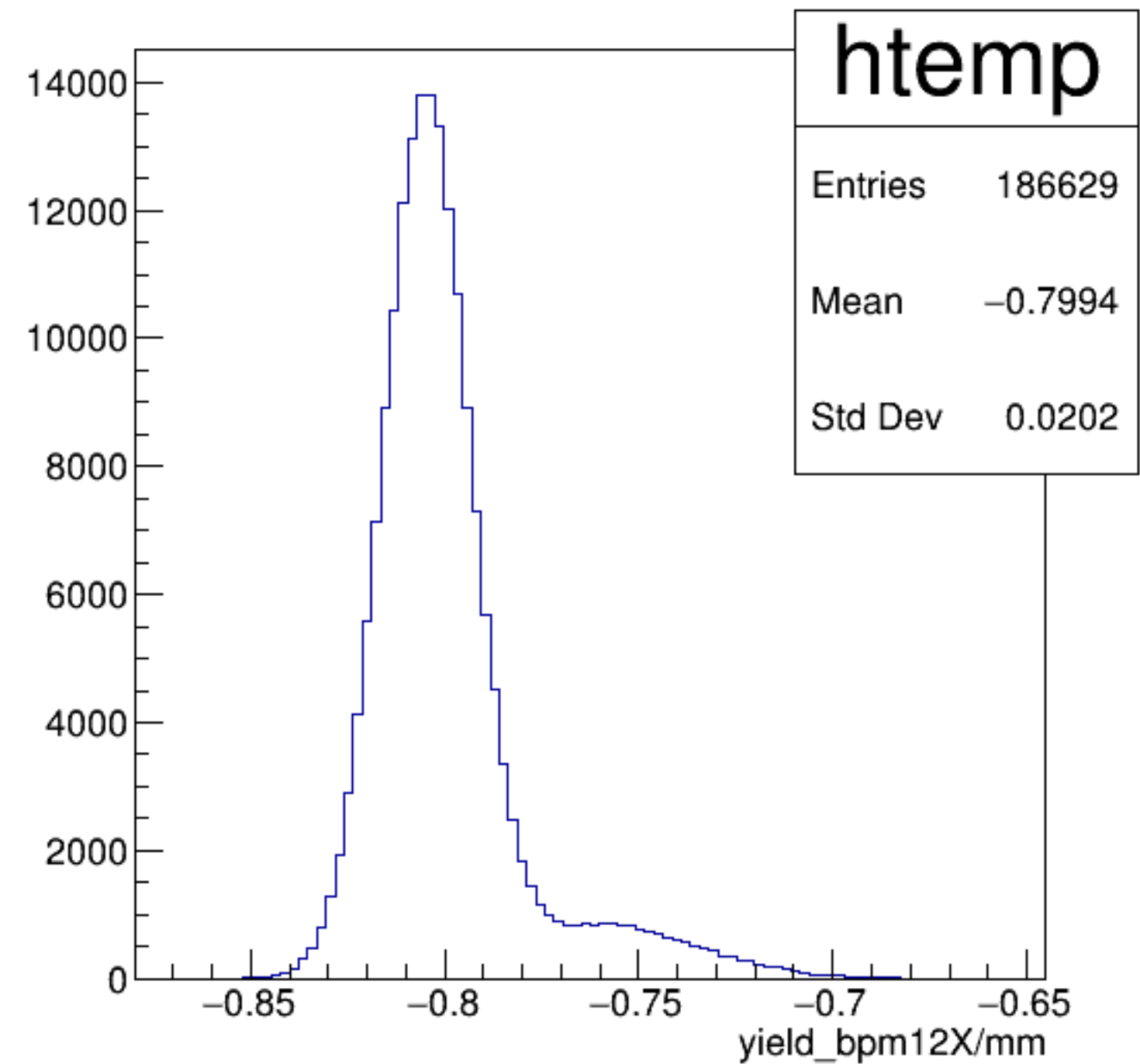
yield_bpm12X/mm {ErrorFlag==0}
