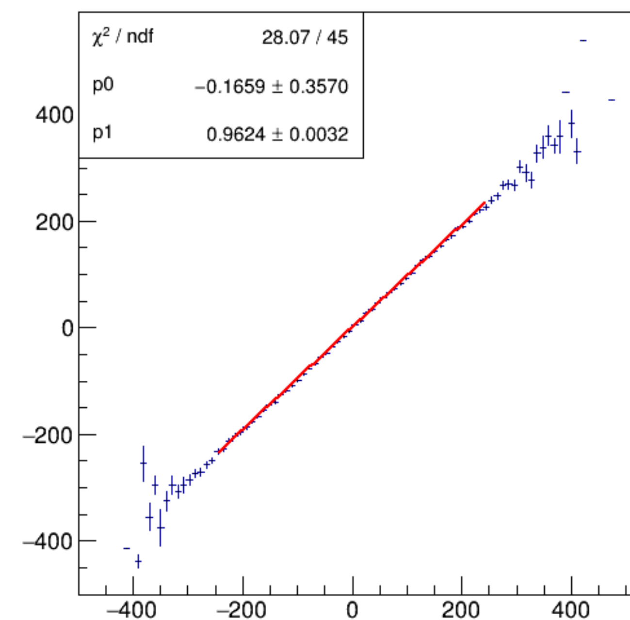
asym_bpm11WS/ppm:Aq/ppm {ErrorFlag==0}
