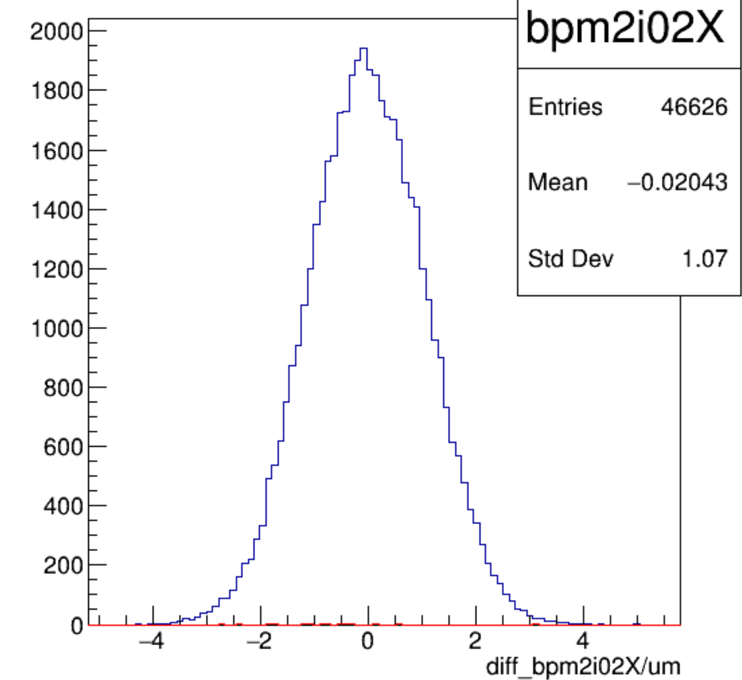
diff_bpm2i02X/um {ErrorFlag==0}
