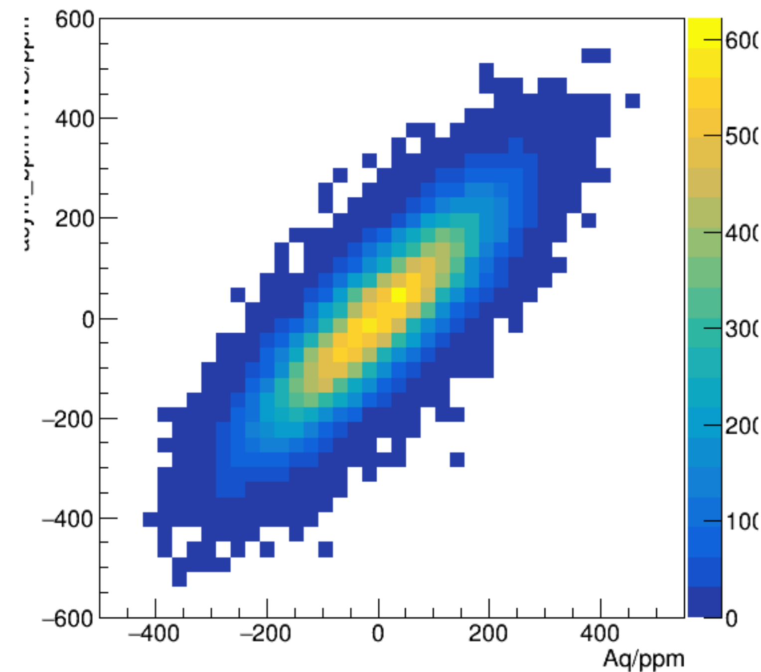
asym_bpm11WS/ppm:Aq/ppm {ErrorFlag==0}
