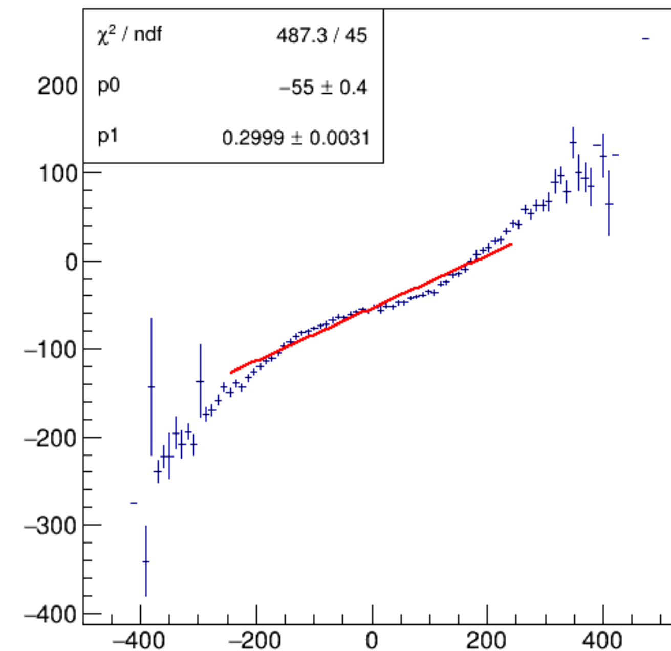
asym_bpm2i01WS/ppm:Aq/ppm {ErrorFlag==0}
