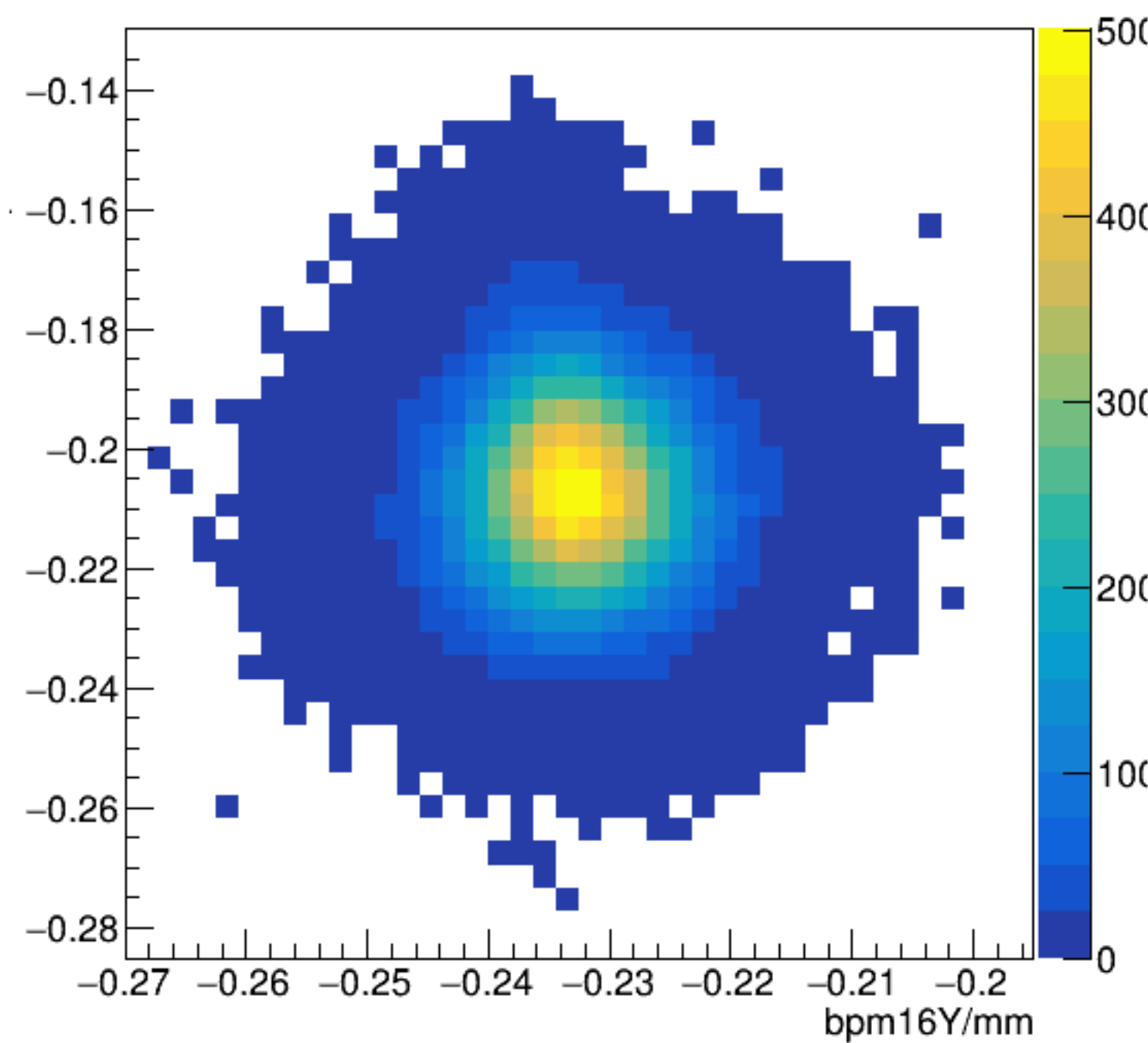
bpm16X/mm:bpm16Y/mm {ErrorFlag==0}
