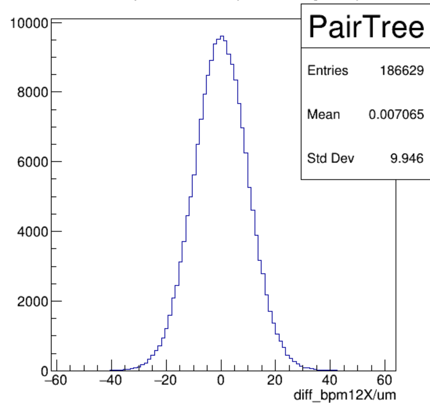
diff_bpm12X/um {ErrorFlag==0}
