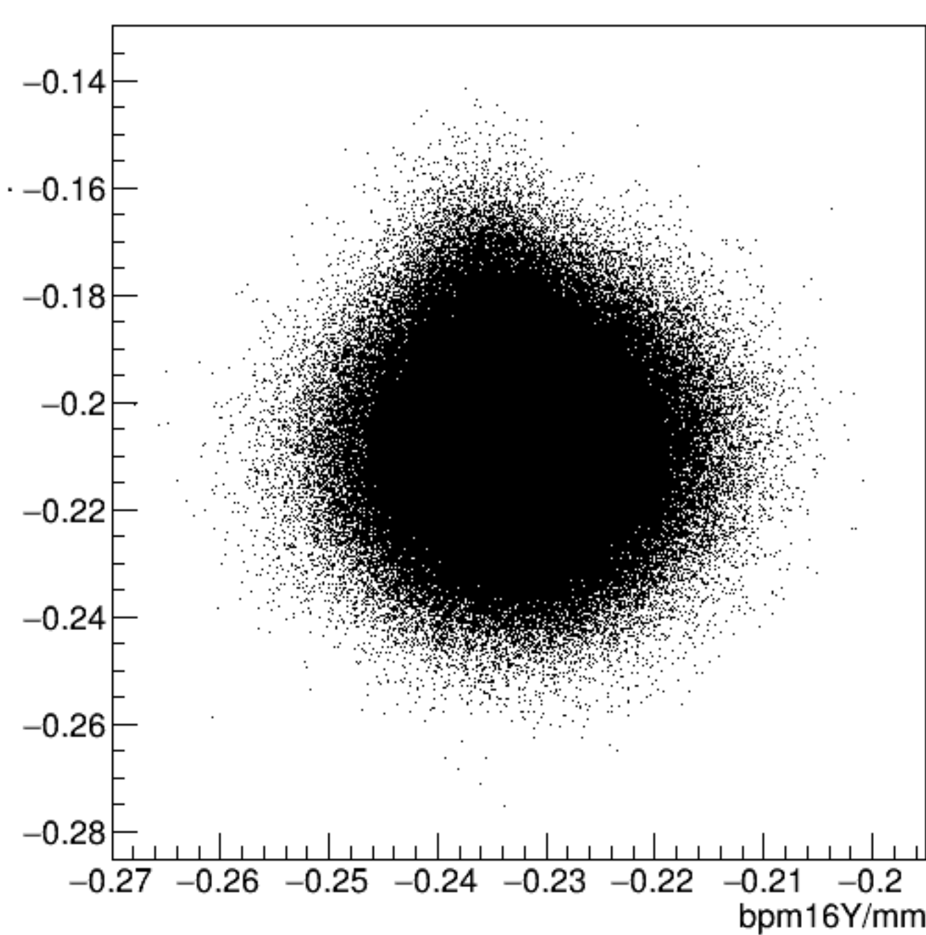
bpm16X/mm:bpm16Y/mm {ErrorFlag==0}
