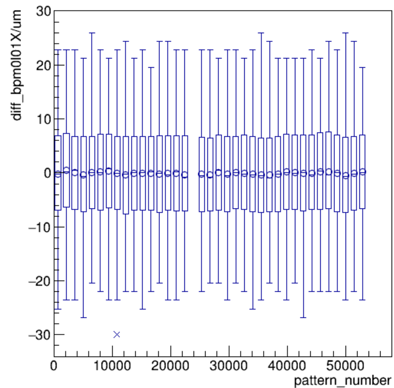
diff_bpm0l01X/um:pattern_number {ErrorFlag==0}
