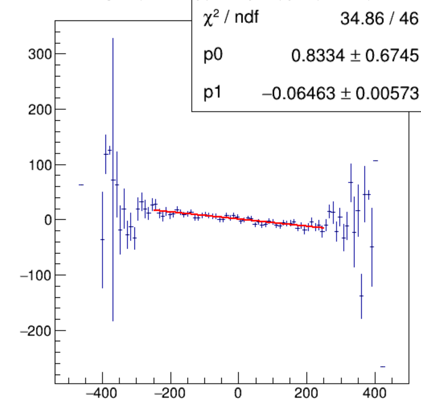
reg_asym_dsr/ppm:AqDS/ppm {ok_cut}
