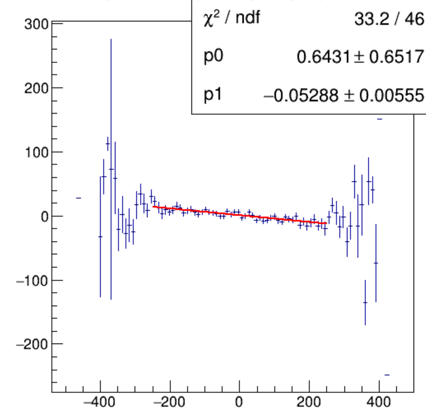
reg_asym_usr/ppm:AqDS/ppm {ok_cut}
