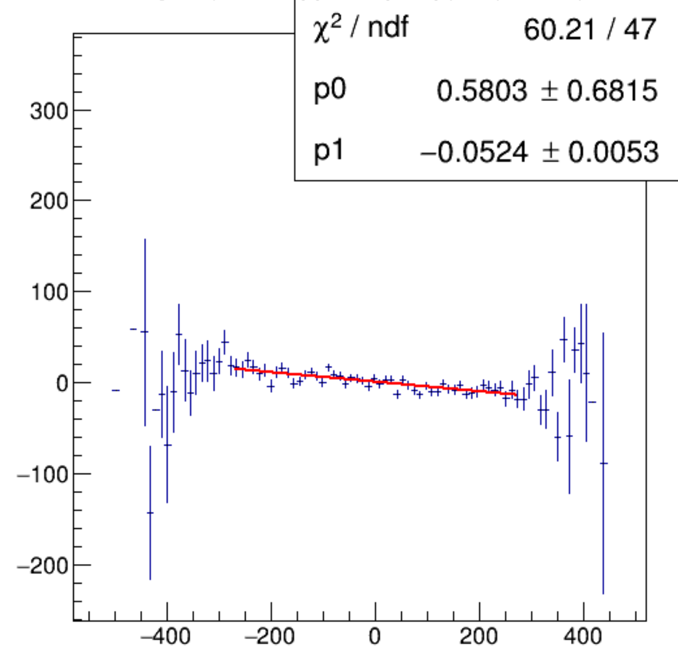
reg_asym_dsl/ppm:AqUS/ppm {ok_cut}
