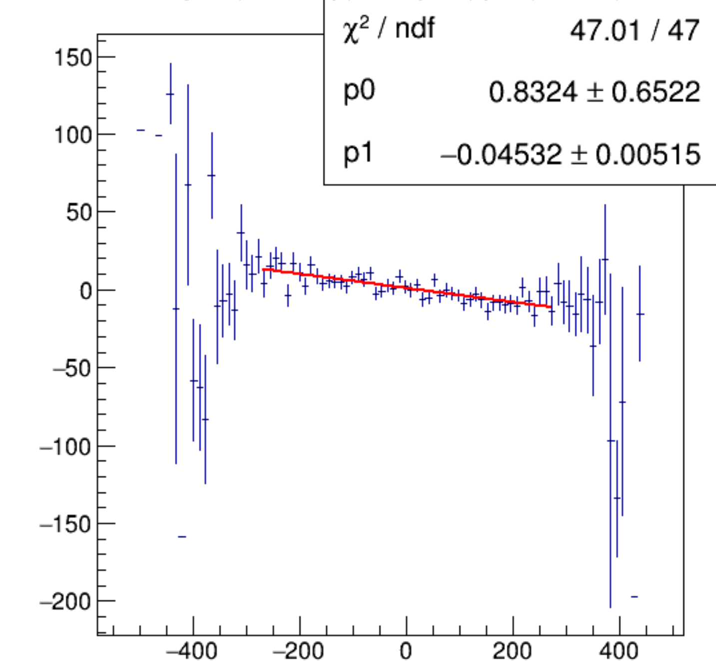
reg_asym_usr/ppm:AqUS/ppm {ok_cut}
