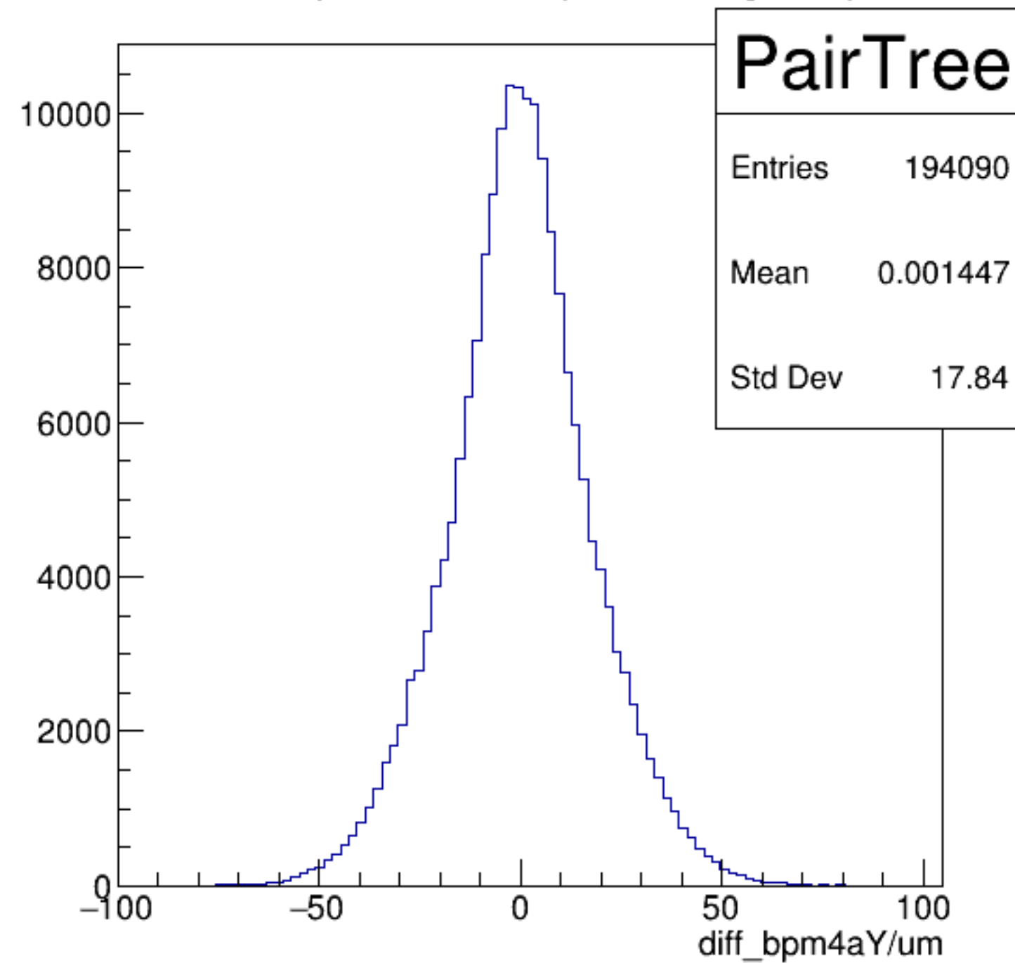
diff_bpm4aY/um {ErrorFlag==0}
