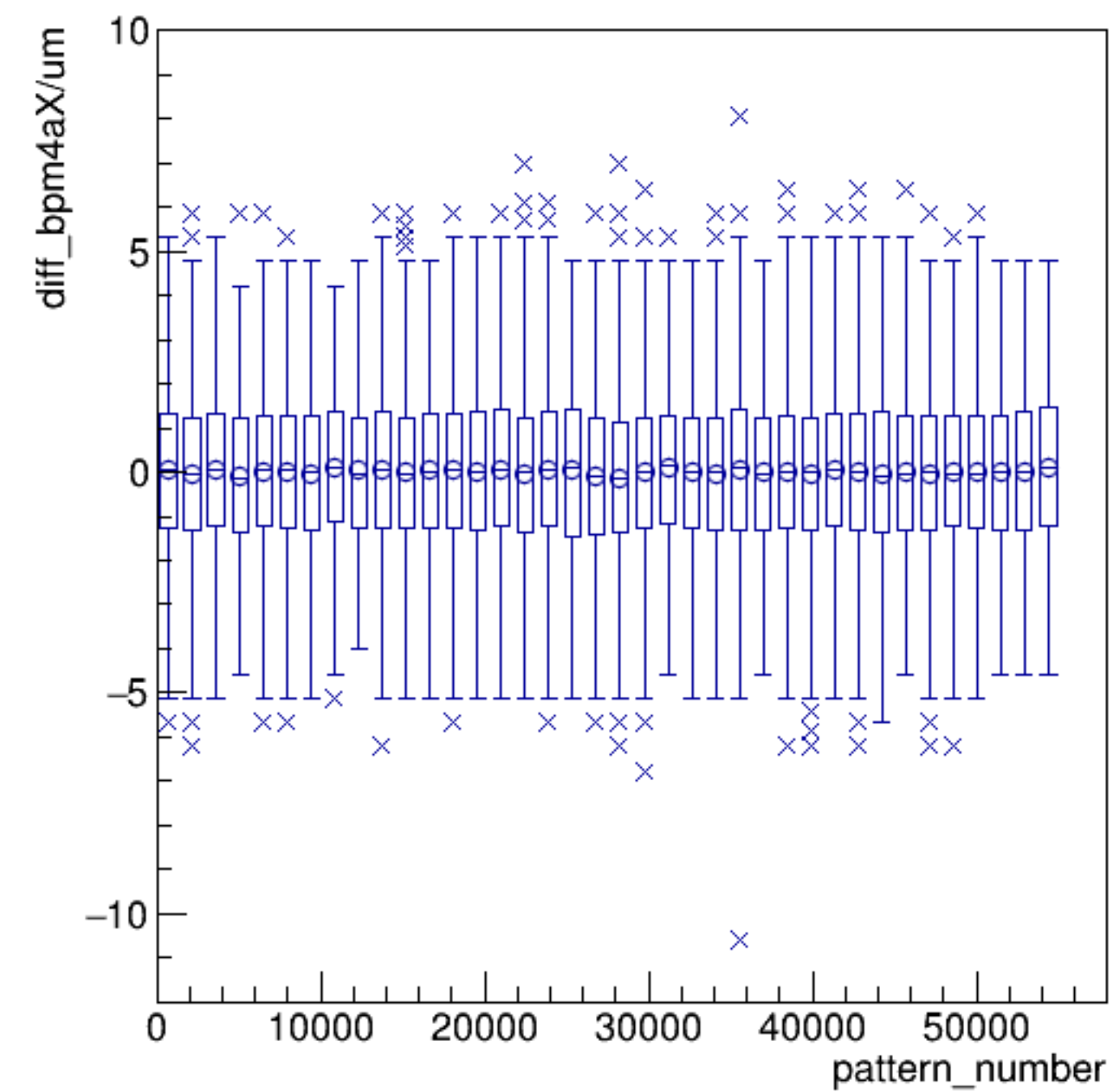
diff_bpm4aX/um:pattern_number {ErrorFlag==0}
