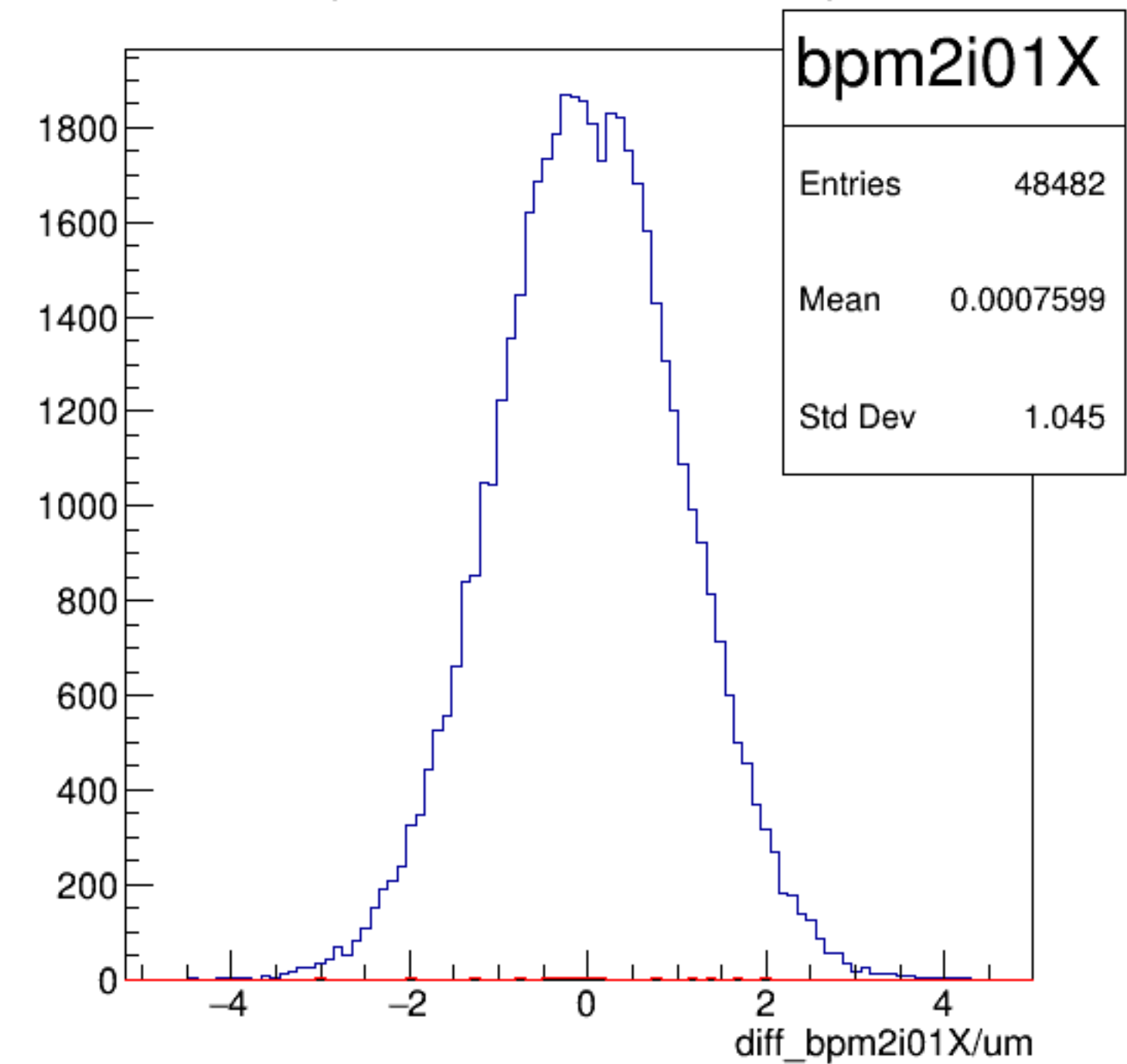
diff_bpm2i01X/um {ErrorFlag==0}
