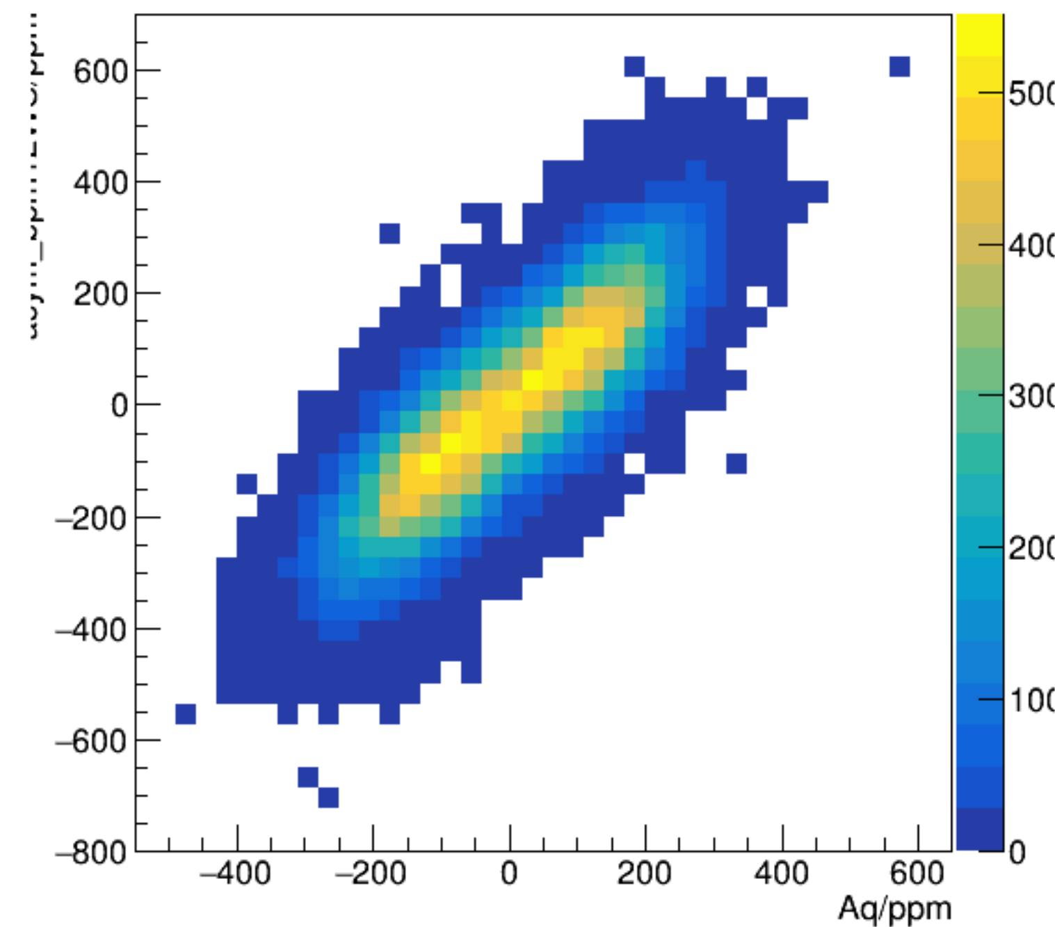
asym_bpm12WS/ppm:Aq/ppm {ErrorFlag==0}
