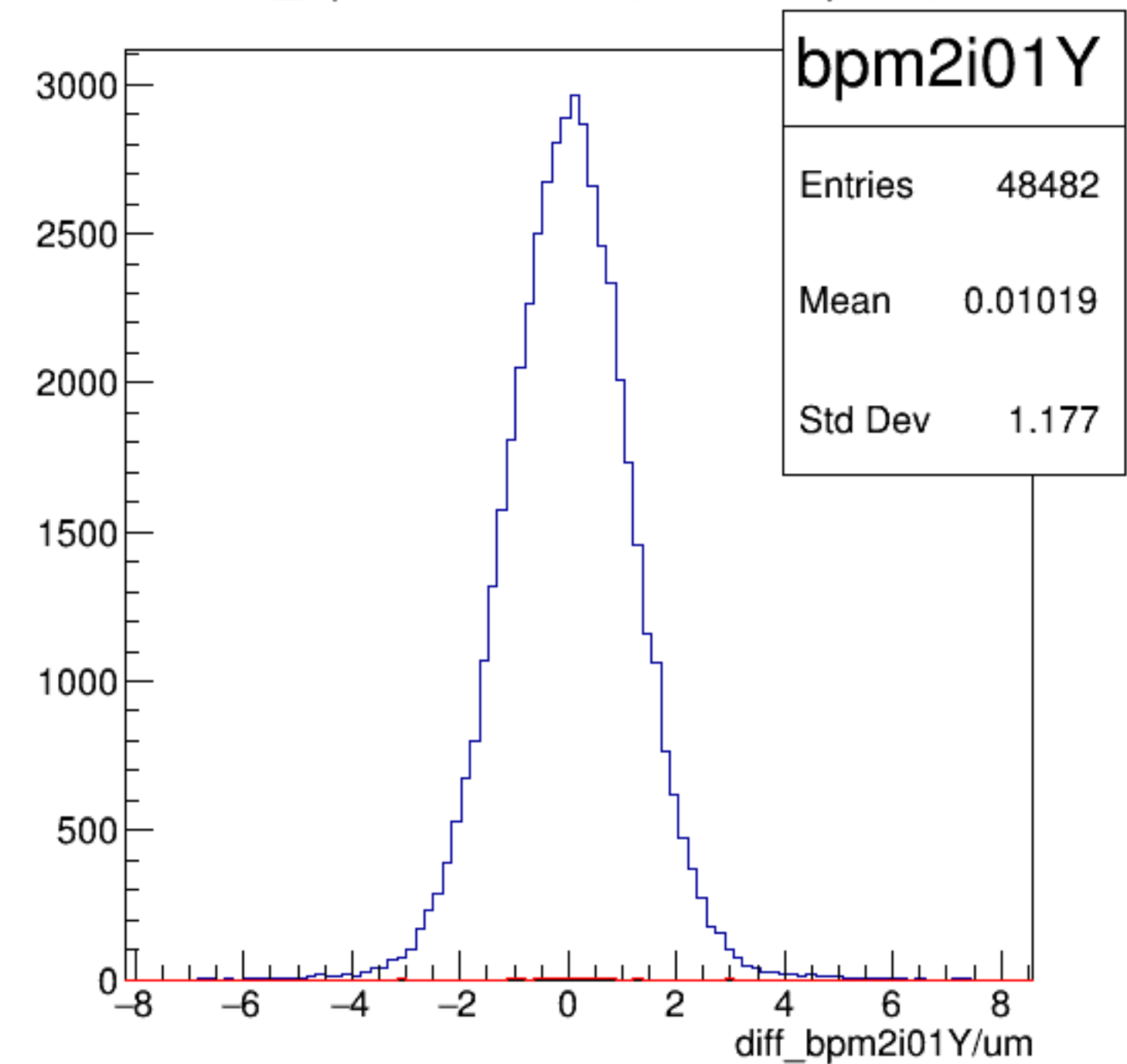
diff_bpm2i01Y/um {ErrorFlag==0}
