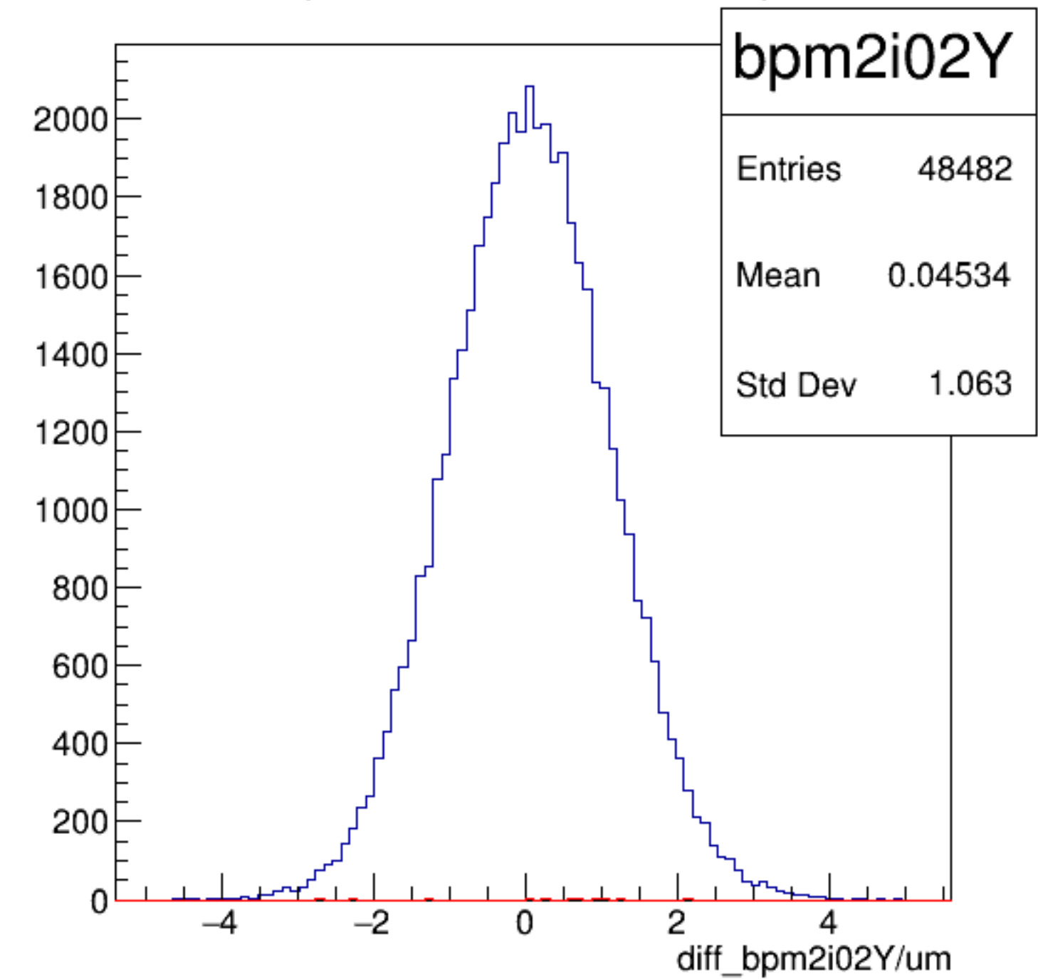
diff_bpm2i02Y/um {ErrorFlag==0}
