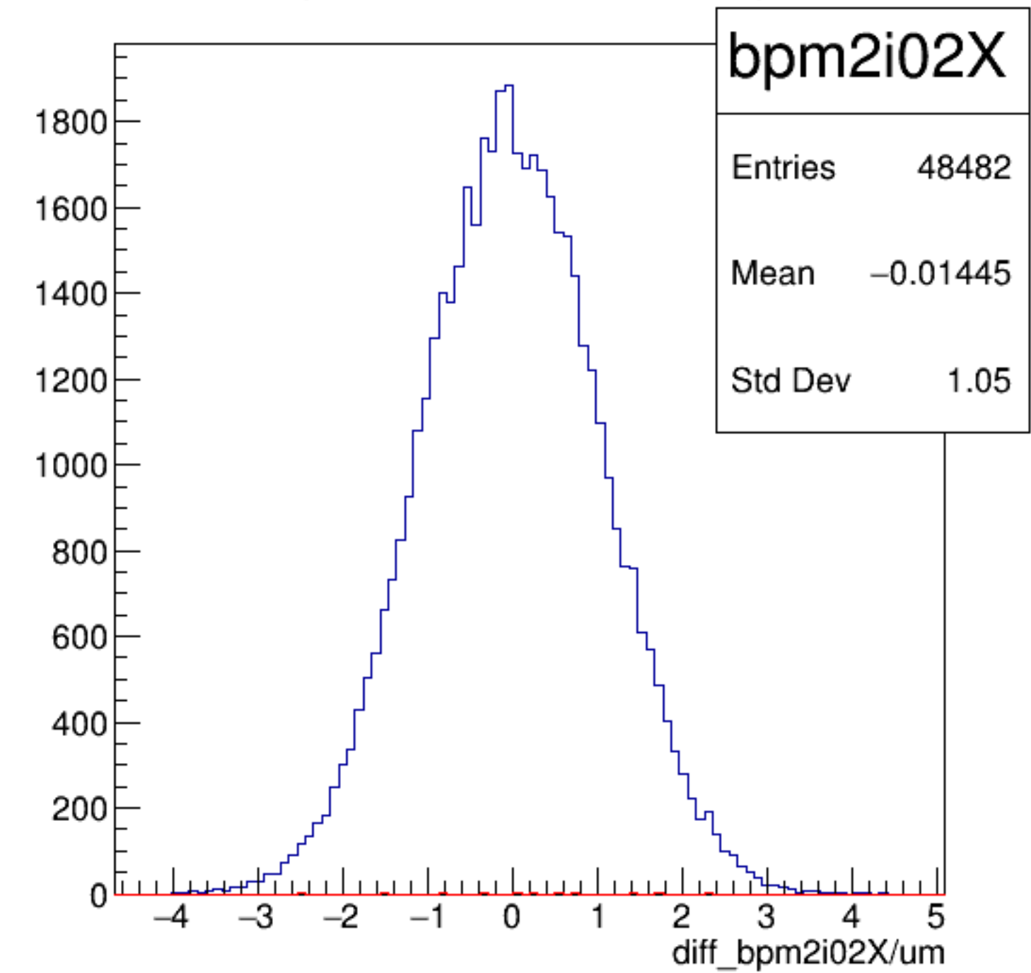
diff_bpm2i02X/um {ErrorFlag==0}
