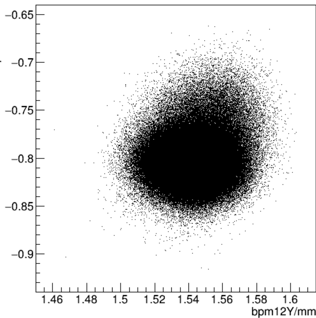
bpm12X/mm:bpm12Y/mm {ErrorFlag==0}
