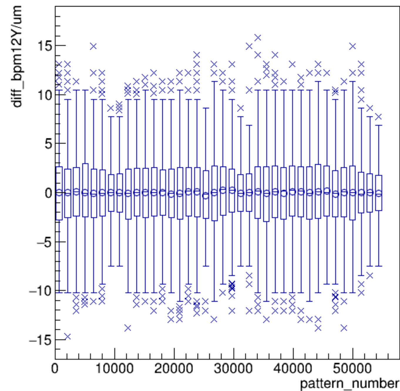
diff_bpm12Y/um:pattern_number {ErrorFlag==0}
