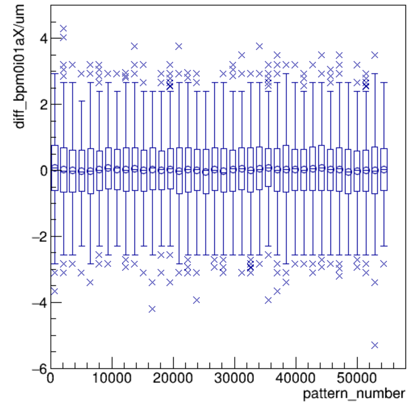
diff_bpm0i01aX/um:pattern_number {ErrorFlag==0}
