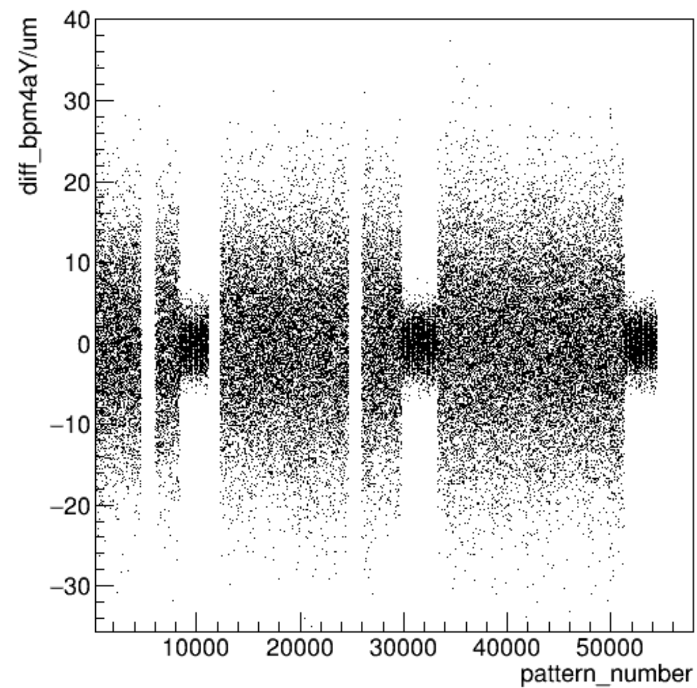
diff_bpm4aY/um:pattern_number {ErrorFlag==0}
