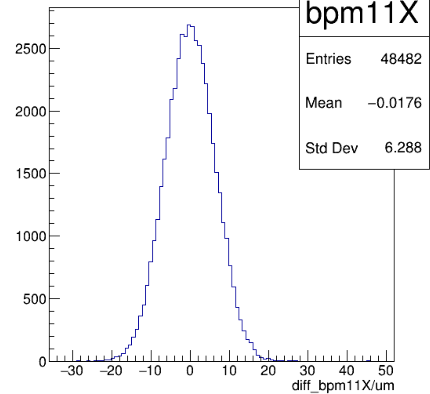
diff_bpm11X/um {ErrorFlag==0}
