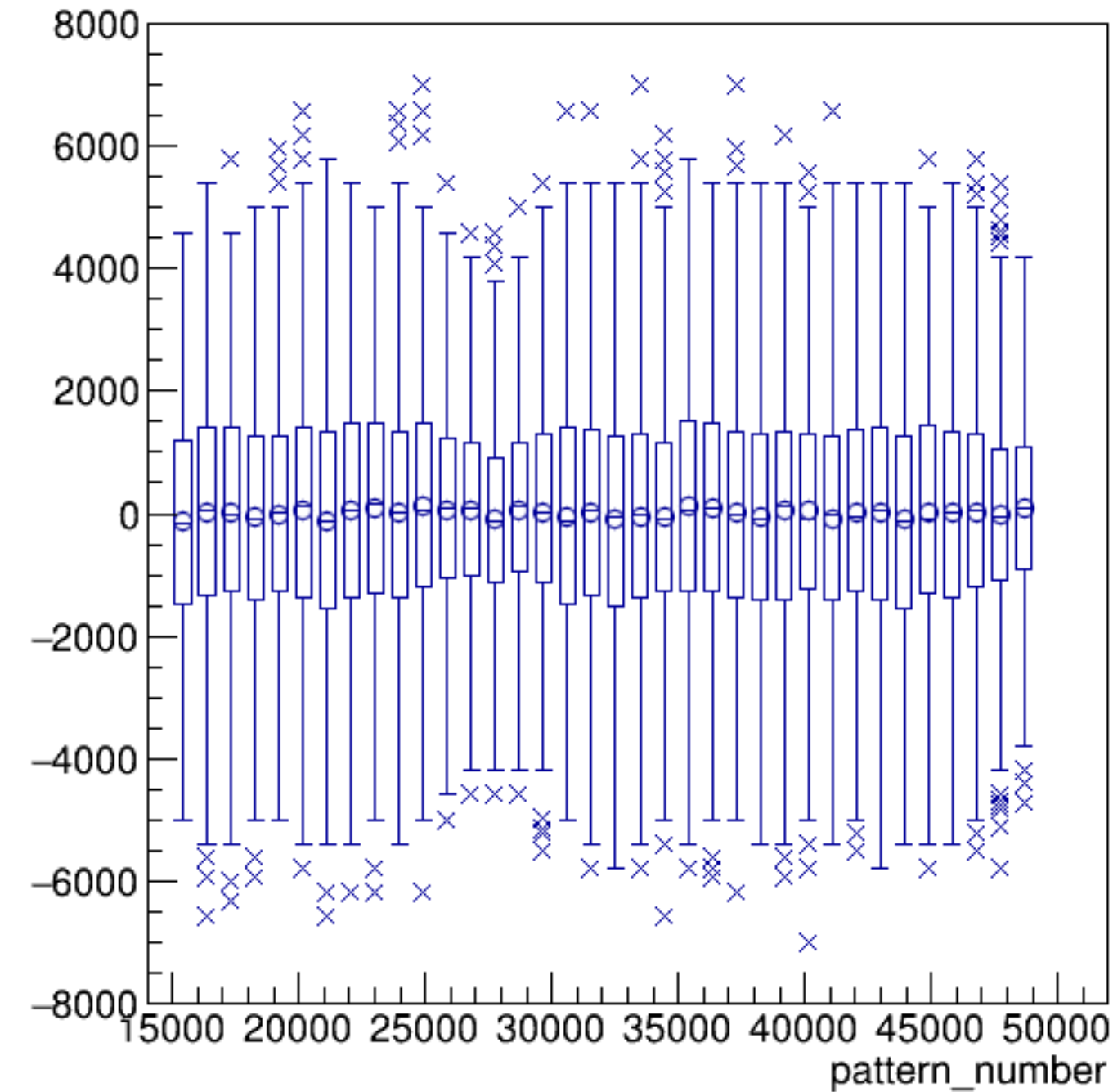
asym_atr1/ppm:pattern_number {ErrorFlag==0}
