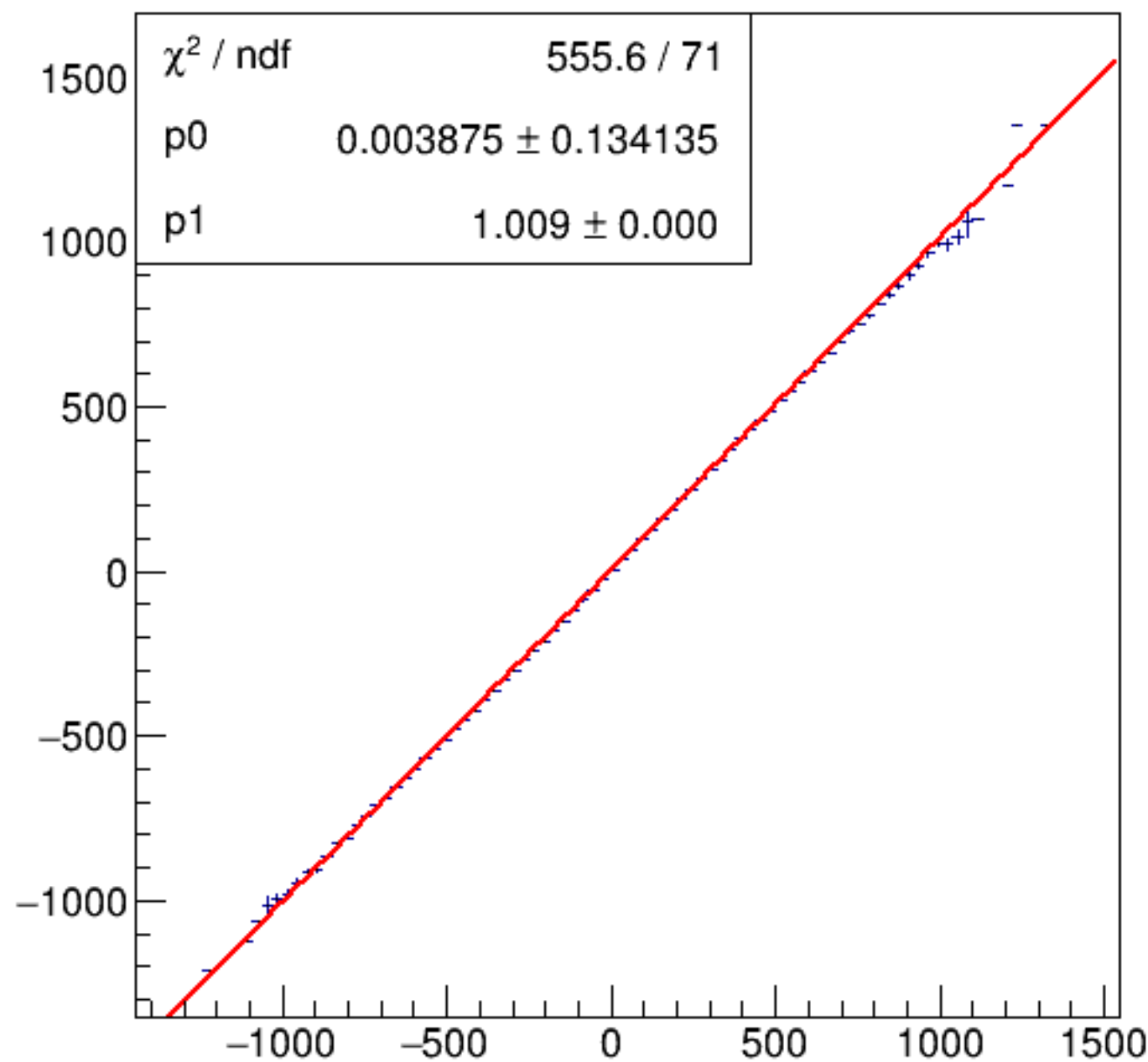
run3982_000_asym_bcm_dg_ds_vs_asym_bcm_an_us_pr.png
