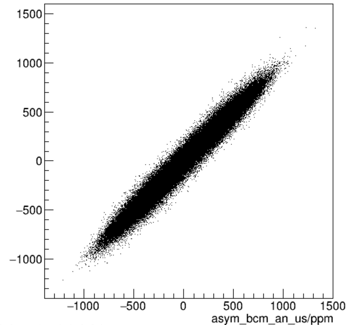
run3982_000_asym_bcm_dg_ds_vs_asym_bcm_an_us_pr.png
