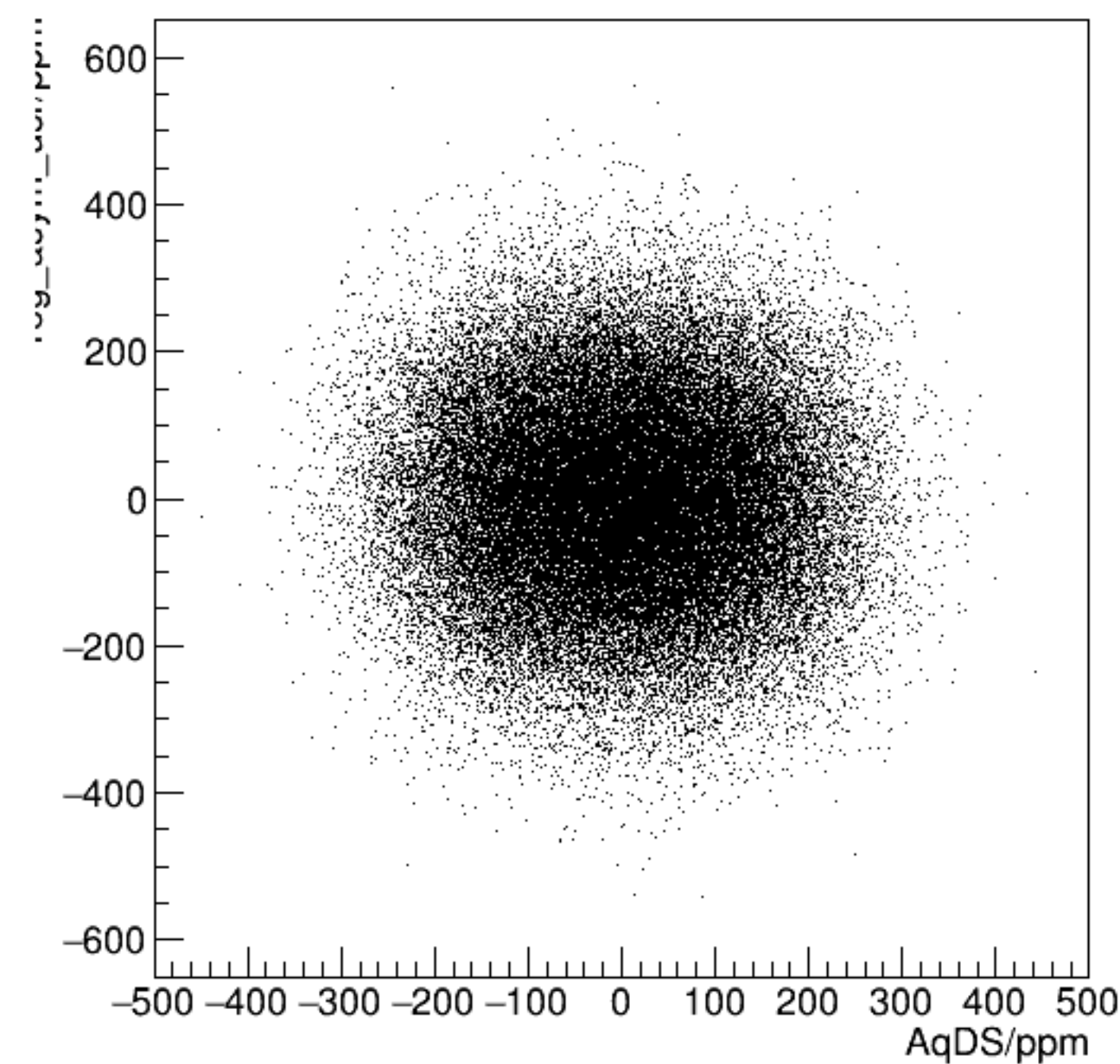
reg_asym_usr/ppm:AqDS/ppm {ok_cut}
