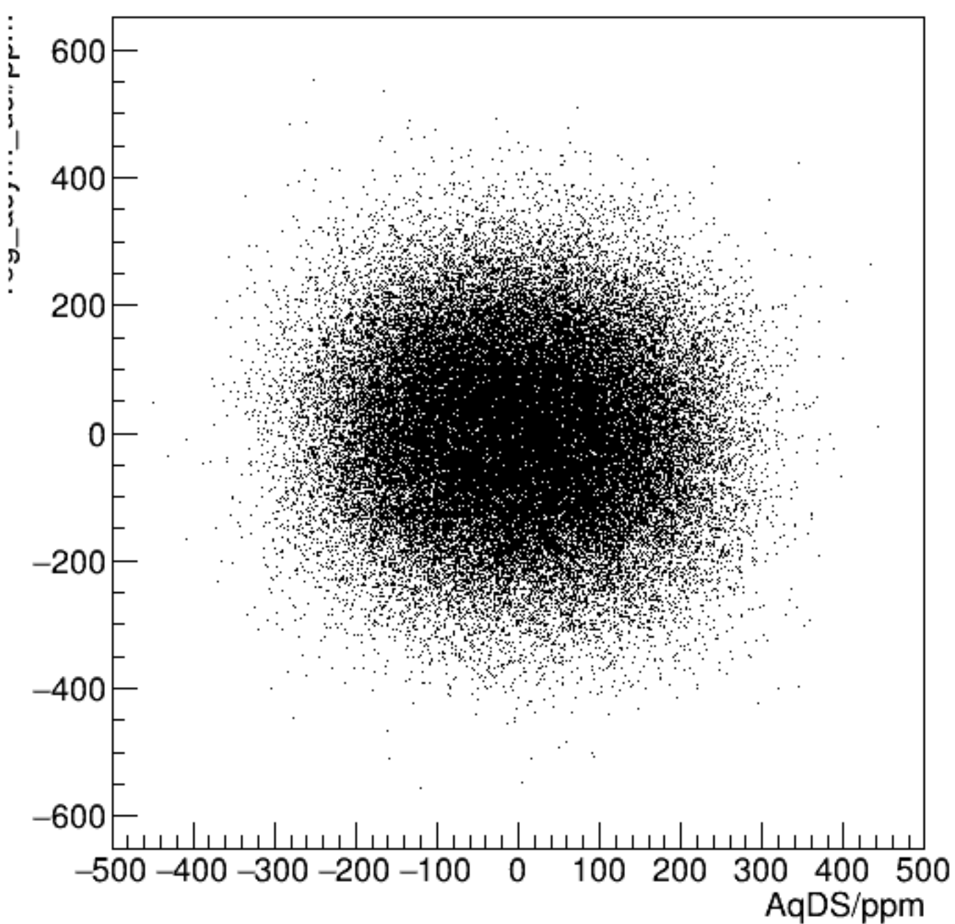
reg_asym_usl/ppm:AqDS/ppm {ok_cut}
