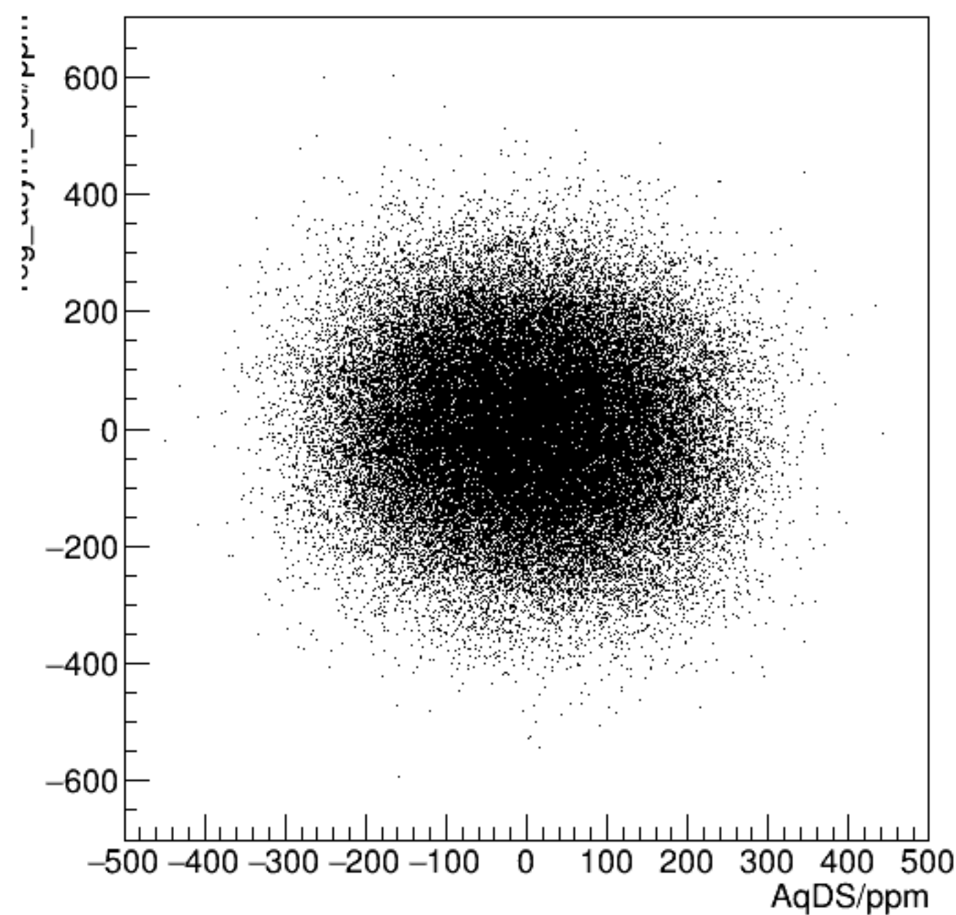
reg_asym_dsl/ppm:AqDS/ppm {ok_cut}
