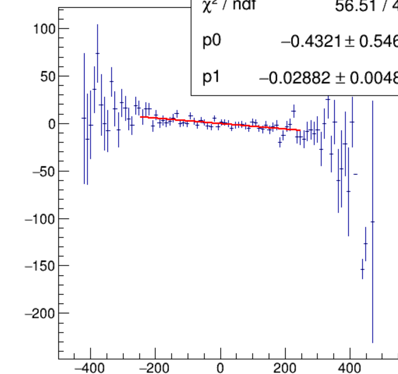
reg_asym_dsr/ppm:AqUS/ppm {ok_cut}
