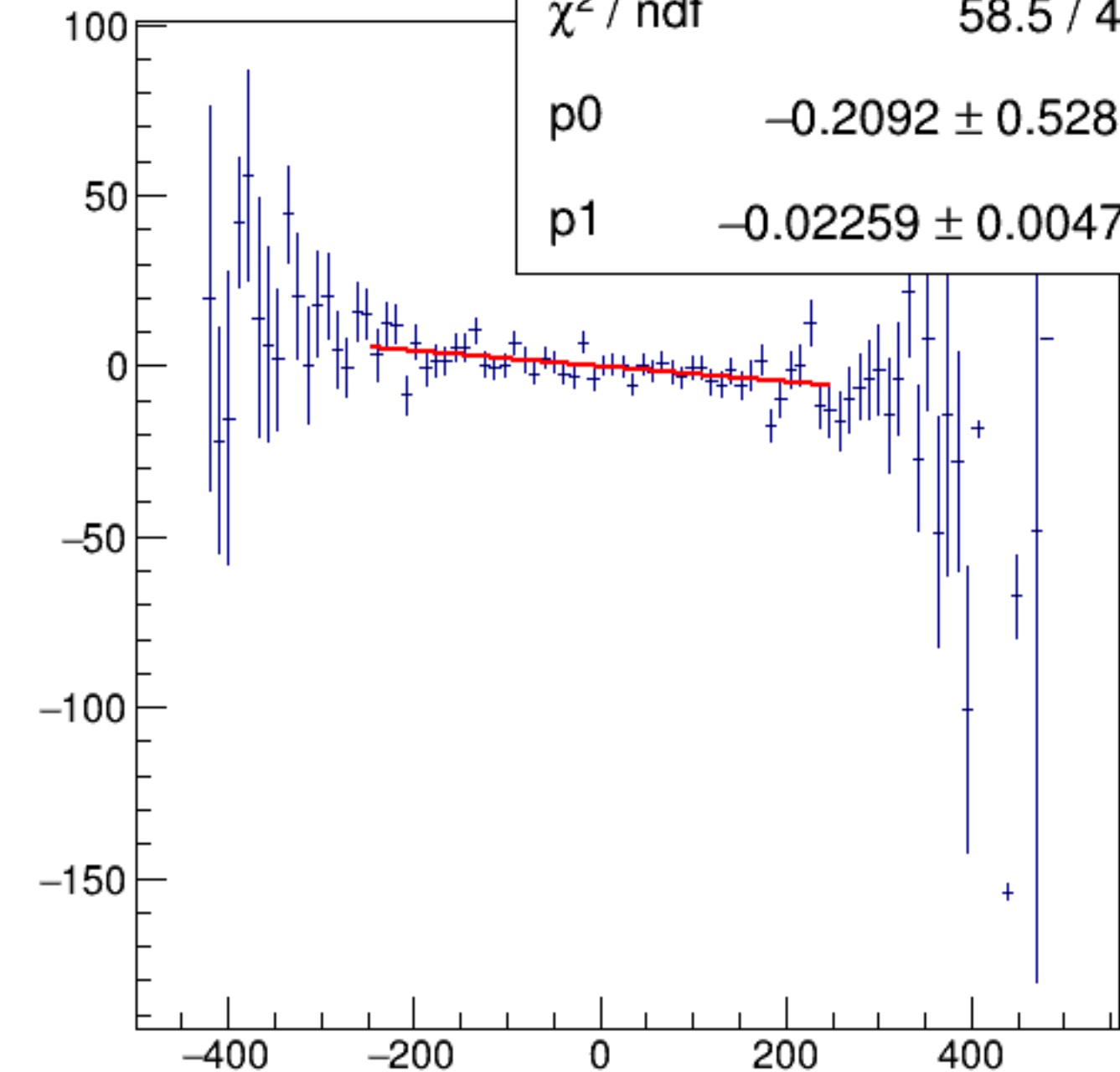
reg_asym_usr/ppm:AqUS/ppm {ok_cut}
