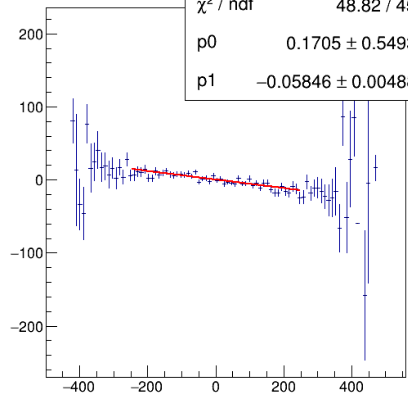
reg_asym_dsl/ppm:AqUS/ppm {ok_cut}
