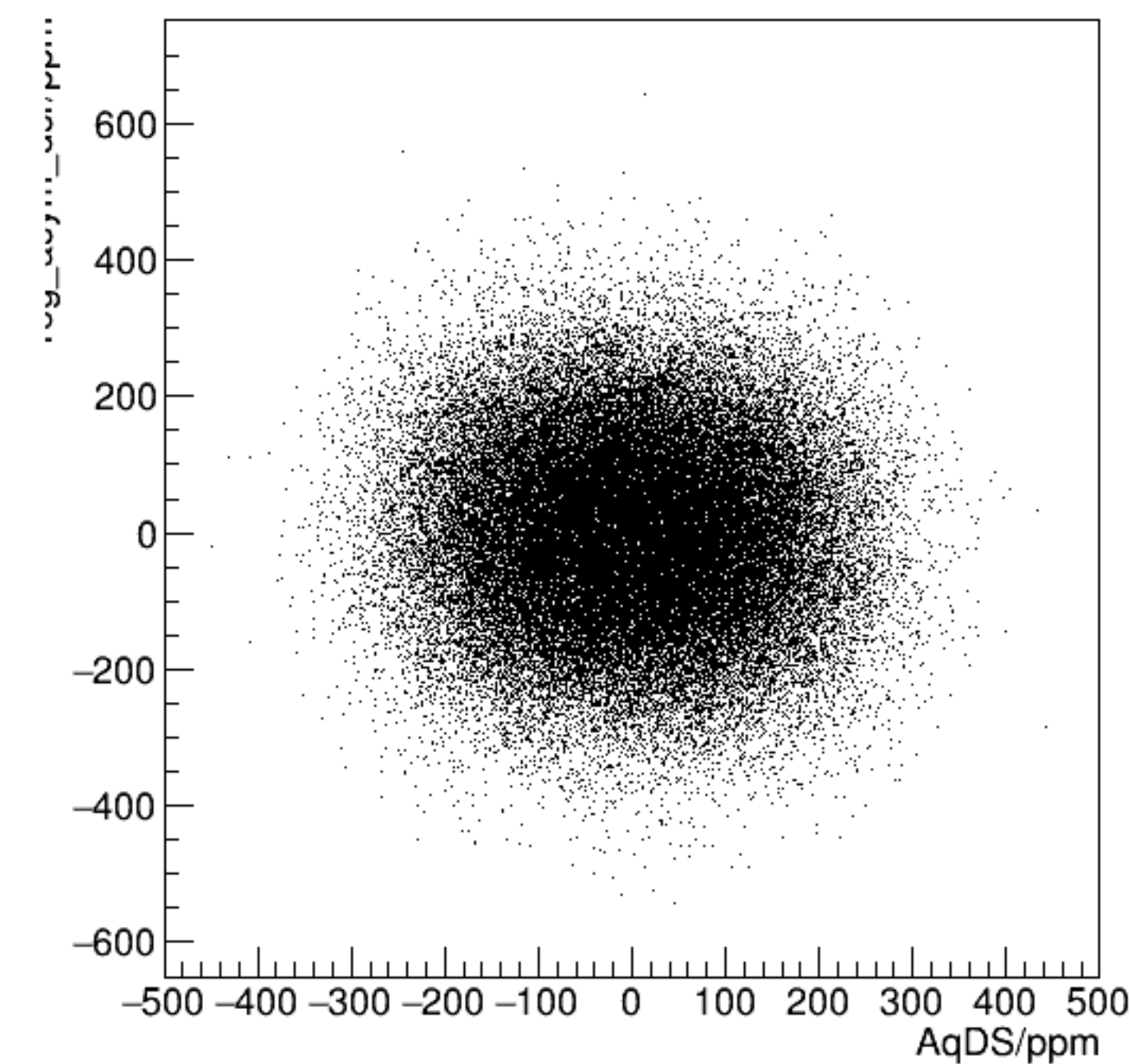
reg_asym_dsr/ppm:AqDS/ppm {ok_cut}
