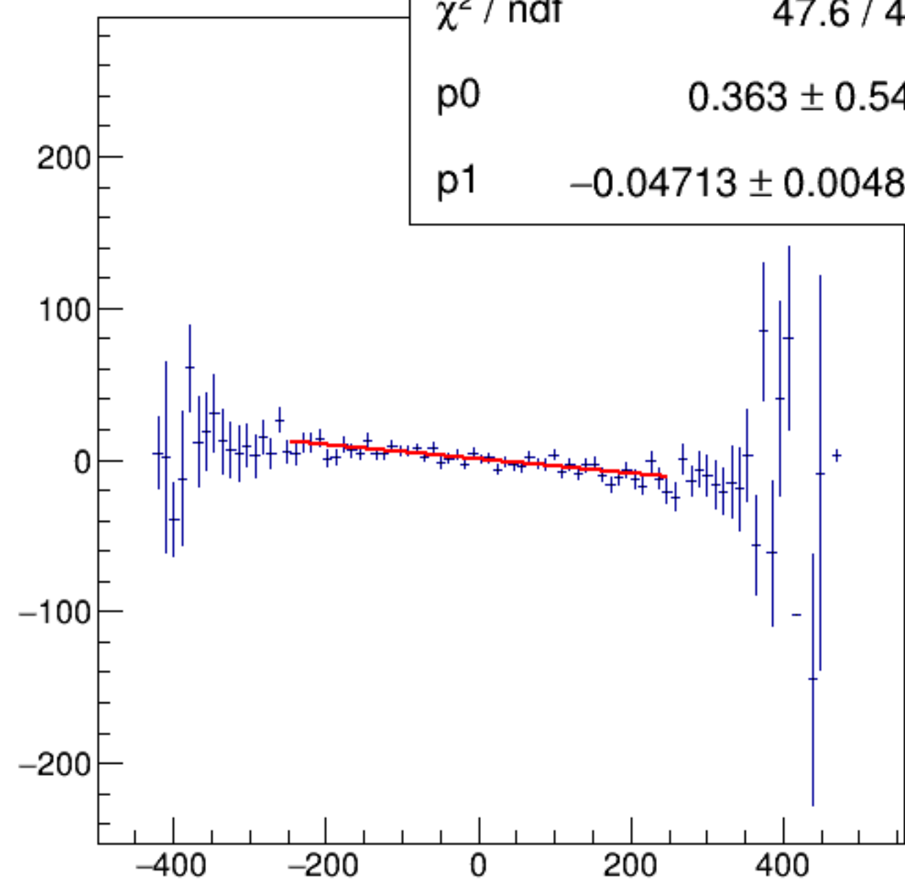
reg_asym_usl/ppm:AqUS/ppm {ok_cut}
