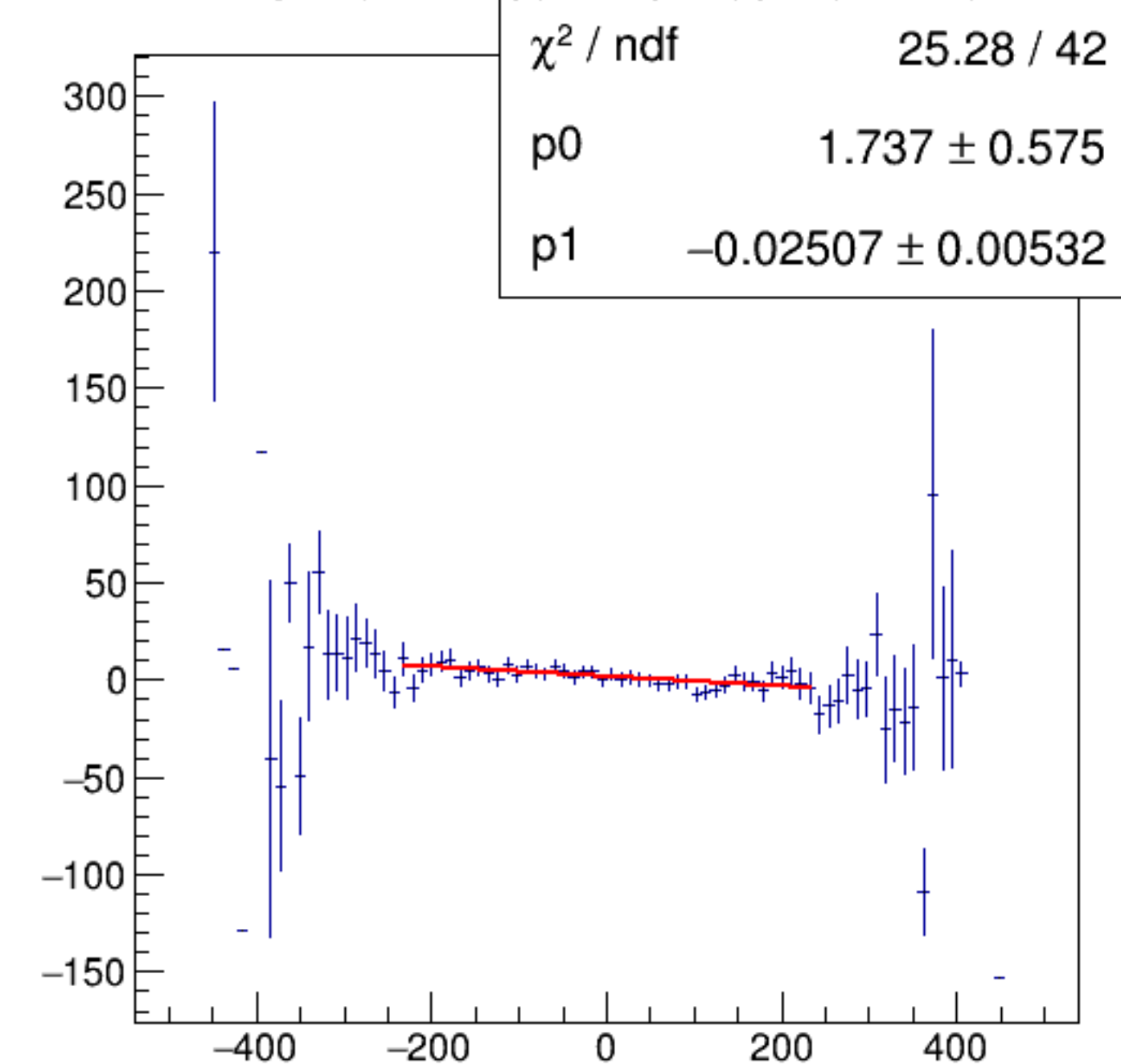
reg_asym_usr/ppm:AqUS/ppm {ok_cut}
