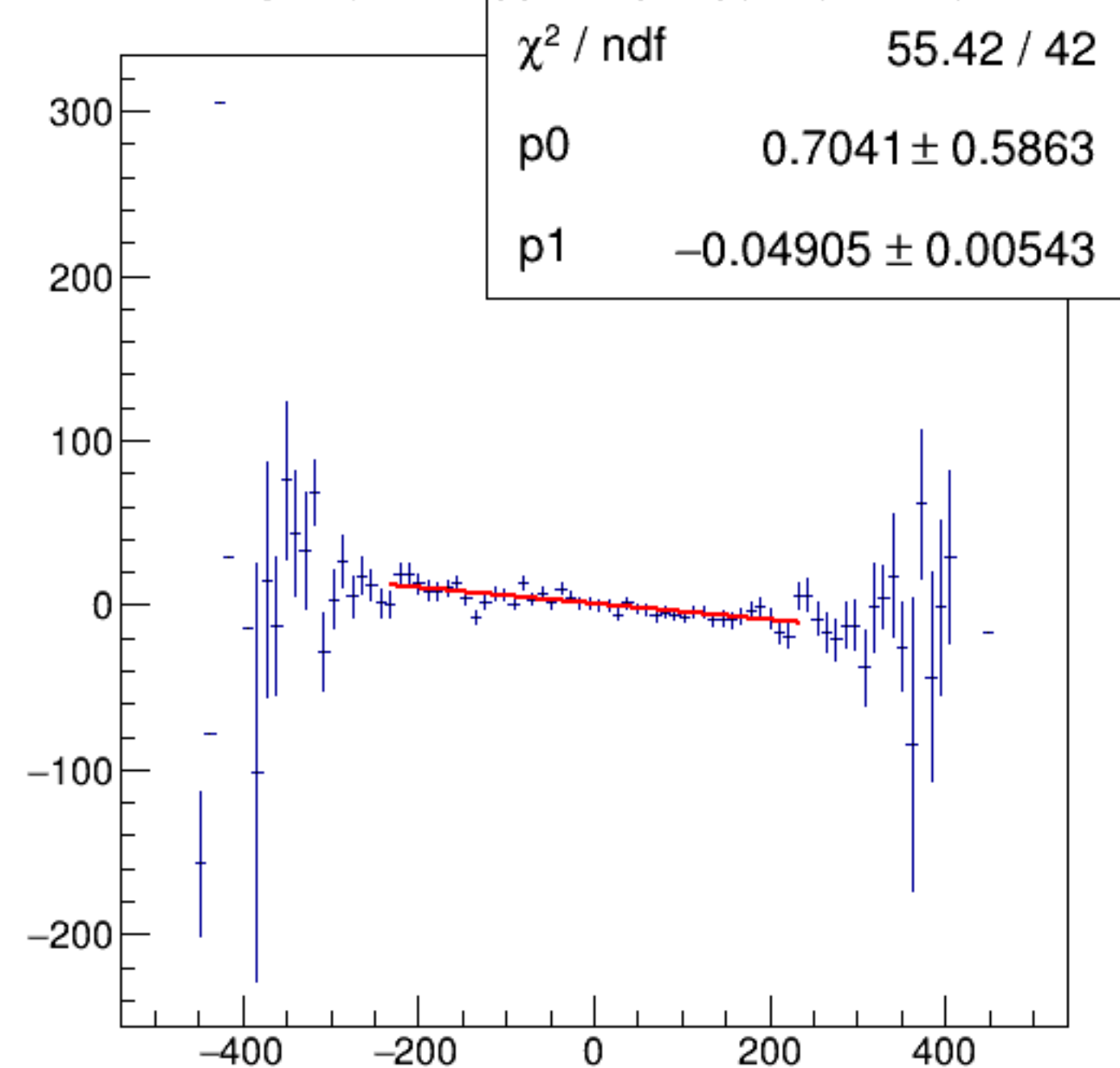
reg_asym_usl/ppm:AqUS/ppm {ok_cut}
