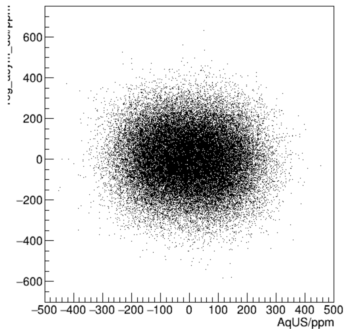
reg_asym_dsl/ppm:AqUS/ppm {ok_cut}
