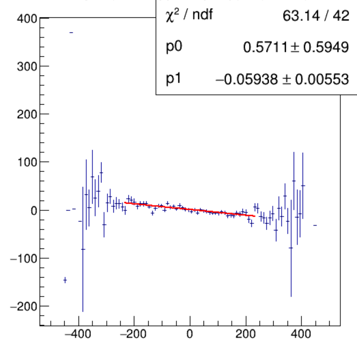
reg_asym_dsl/ppm:AqUS/ppm {ok_cut}
