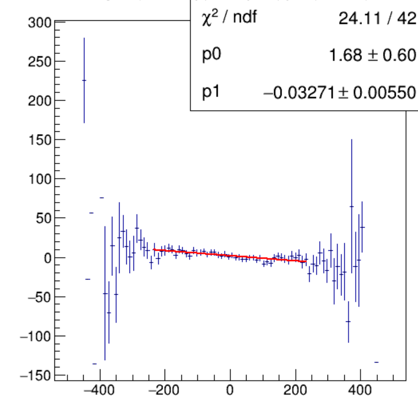
reg_asym_dsr/ppm:AqUS/ppm {ok_cut}
