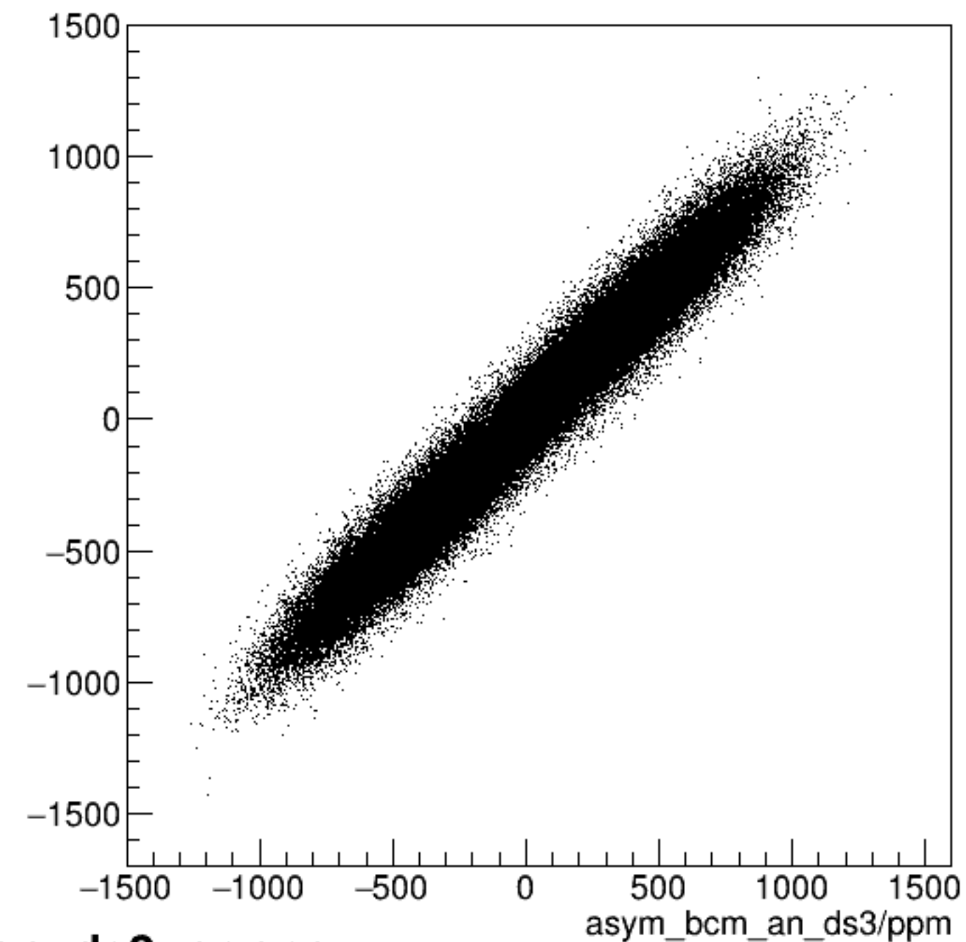
run3994_000_asym_bcm_dg_us_vs_asym_bcm_an_ds3_pr.png
