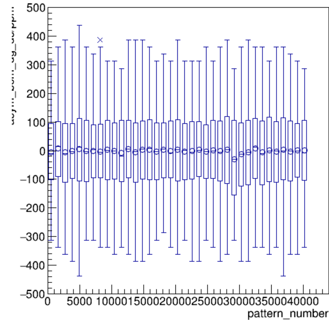
asym_bcm_dg_ds/ppm:pattern_number {ErrorFlag==0}
