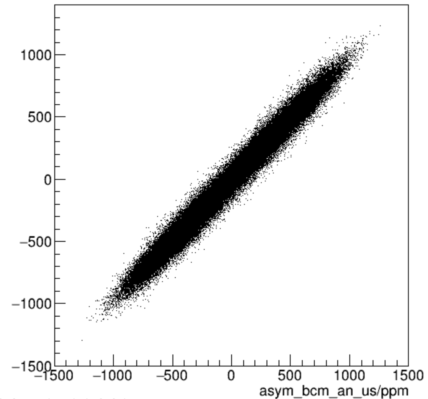
run3994_000_asym_bcm_dg_ds_vs_asym_bcm_an_us_pr.png
