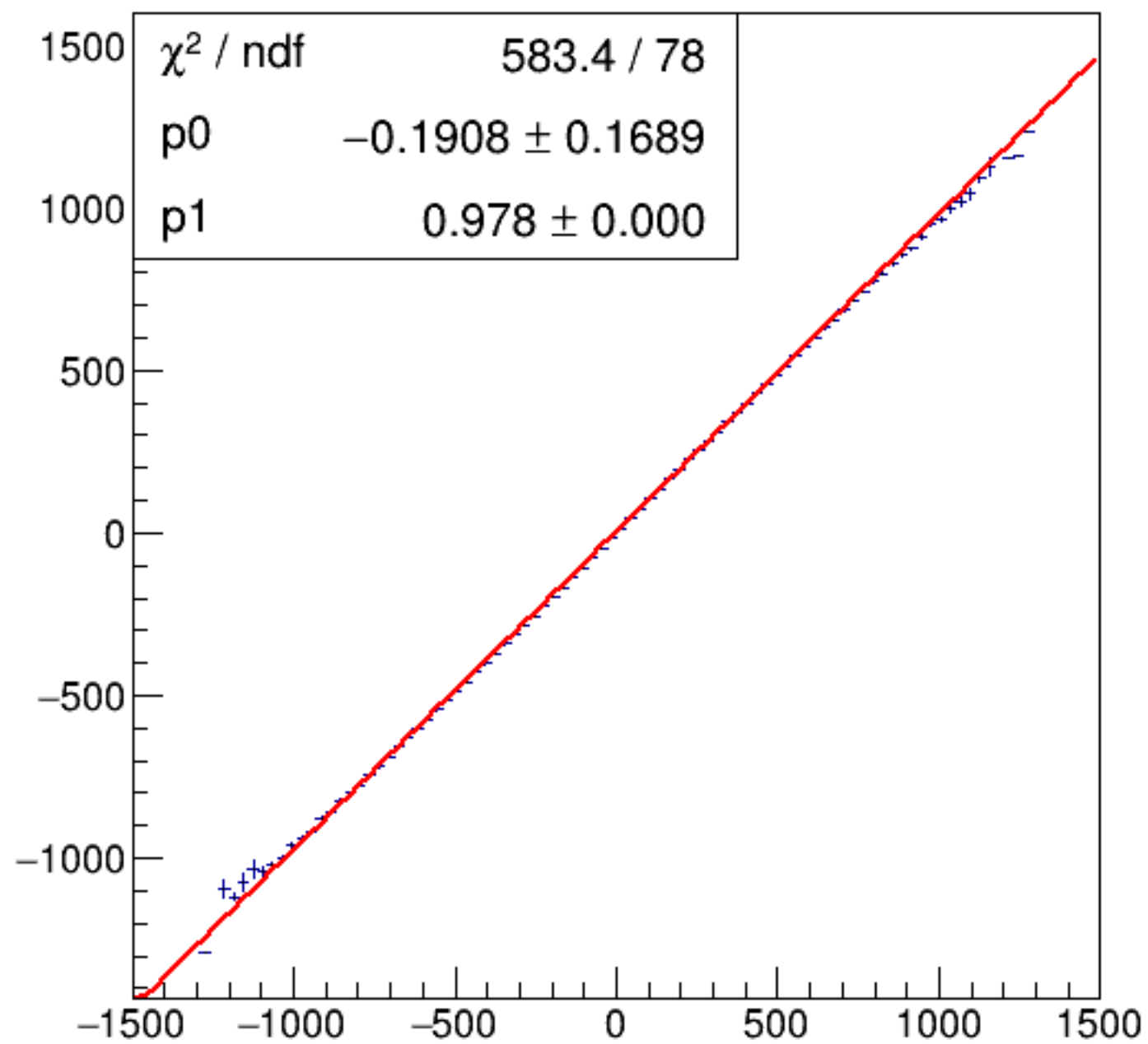
run3994_000_asym_bcm_dg_ds_vs_asym_bcm_an_us_pr.png
