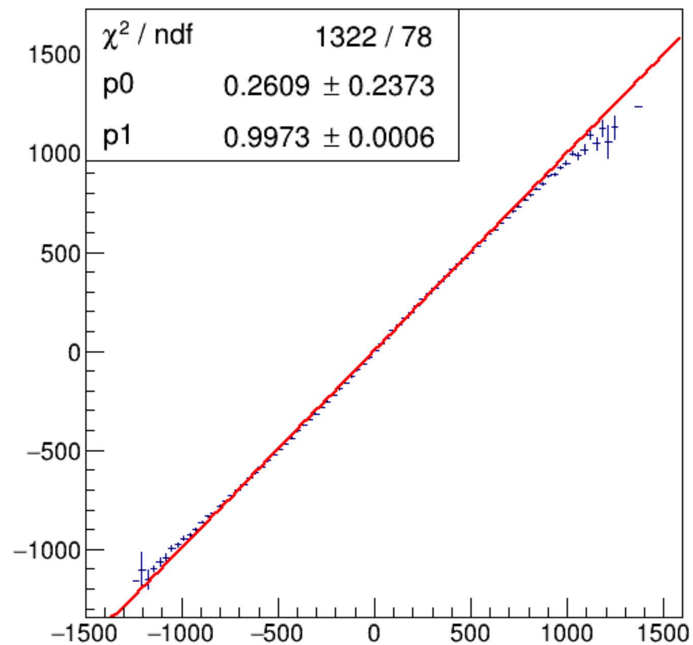
run3994_000_asym_bcm_dg_us_vs_asym_bcm_an_ds_pr.png
