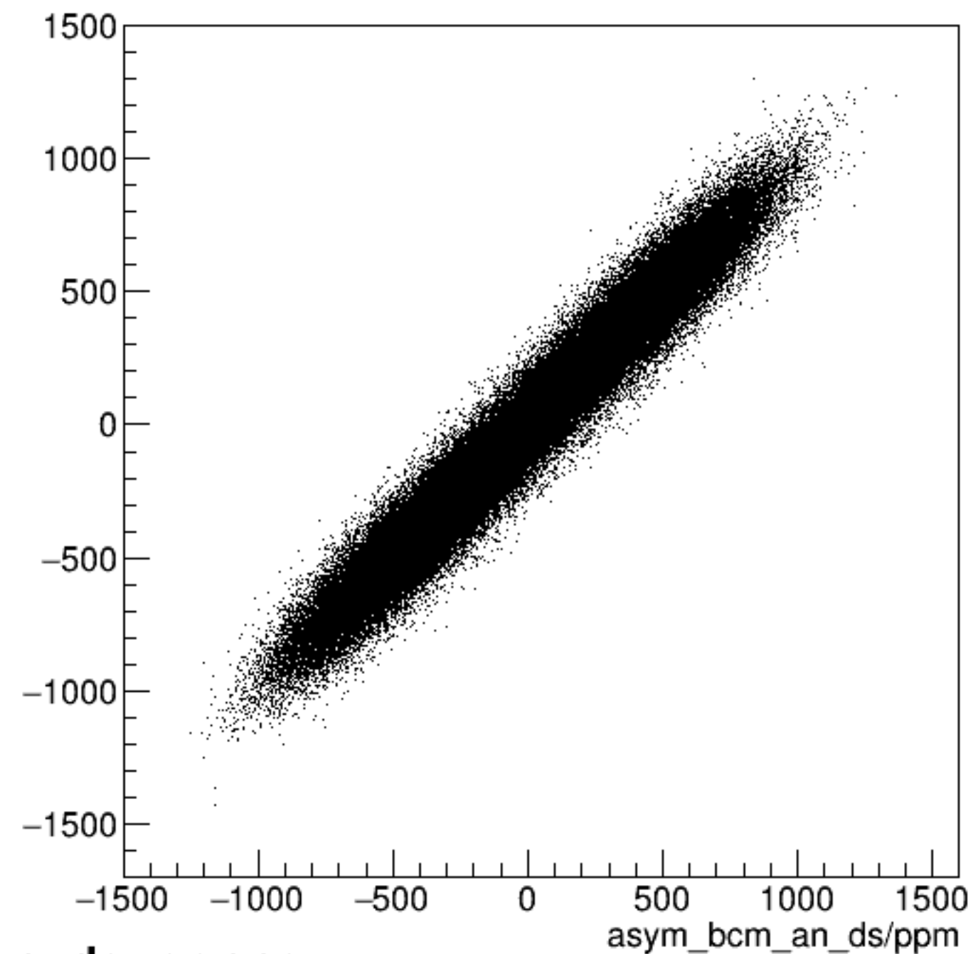
run3994_000_asym_bcm_dg_us_vs_asym_bcm_an_ds_pr.png
