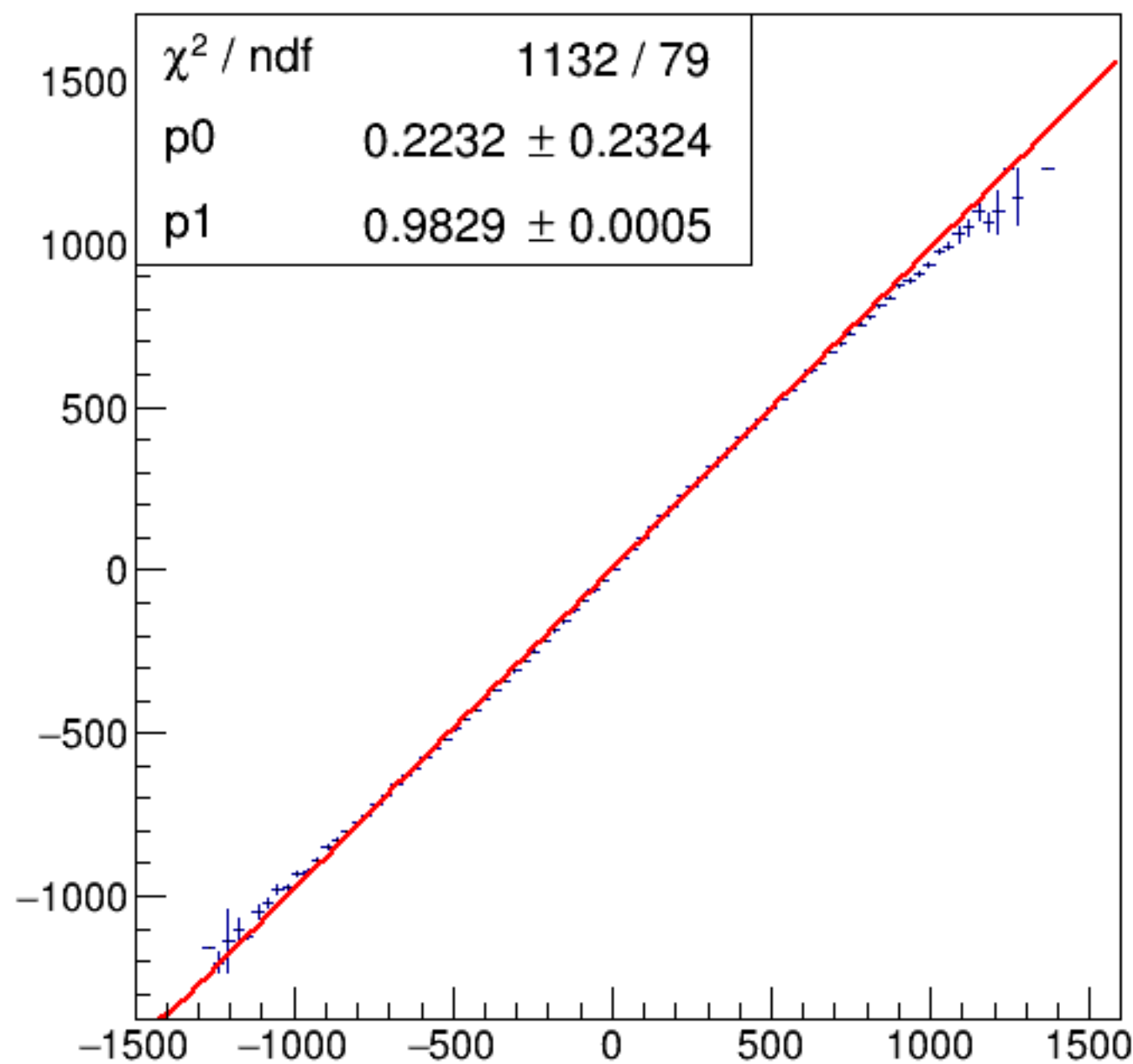
run3994_000_asym_bcm_dg_us_vs_asym_bcm_an_ds3_pr.png
