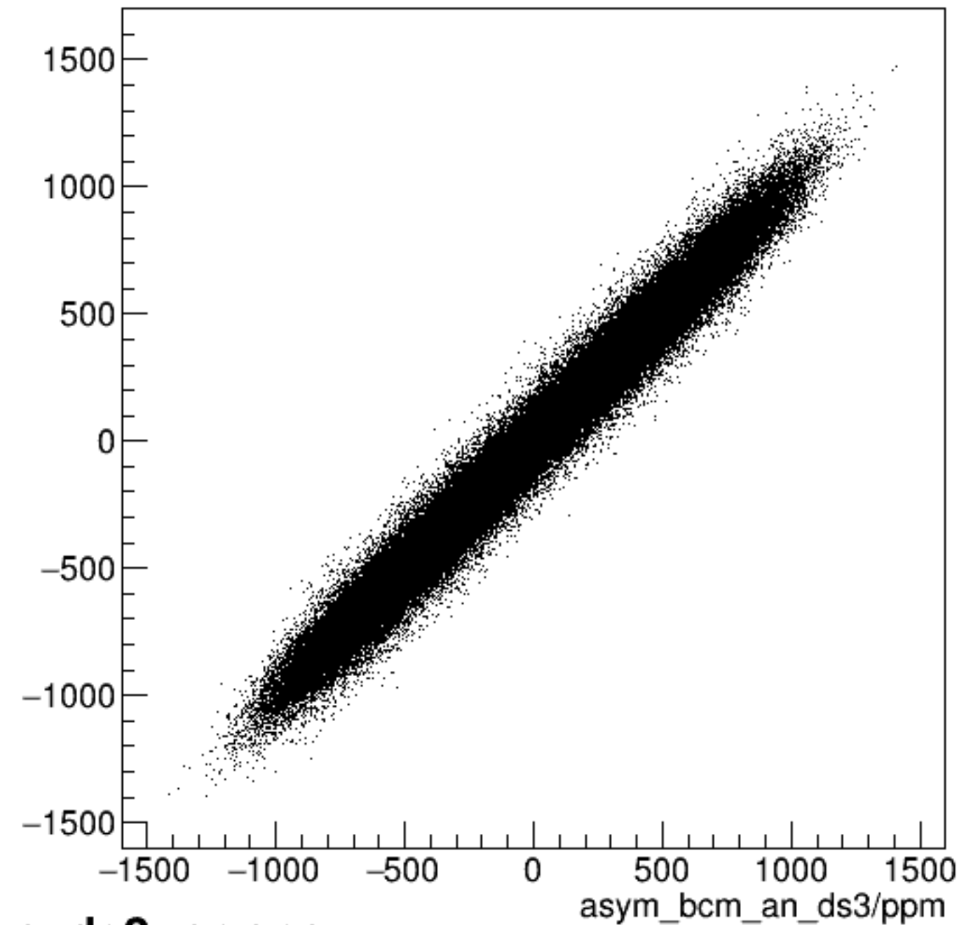
run3996_000_asym_bcm_dg_us_vs_asym_bcm_an_ds3_pr.png
