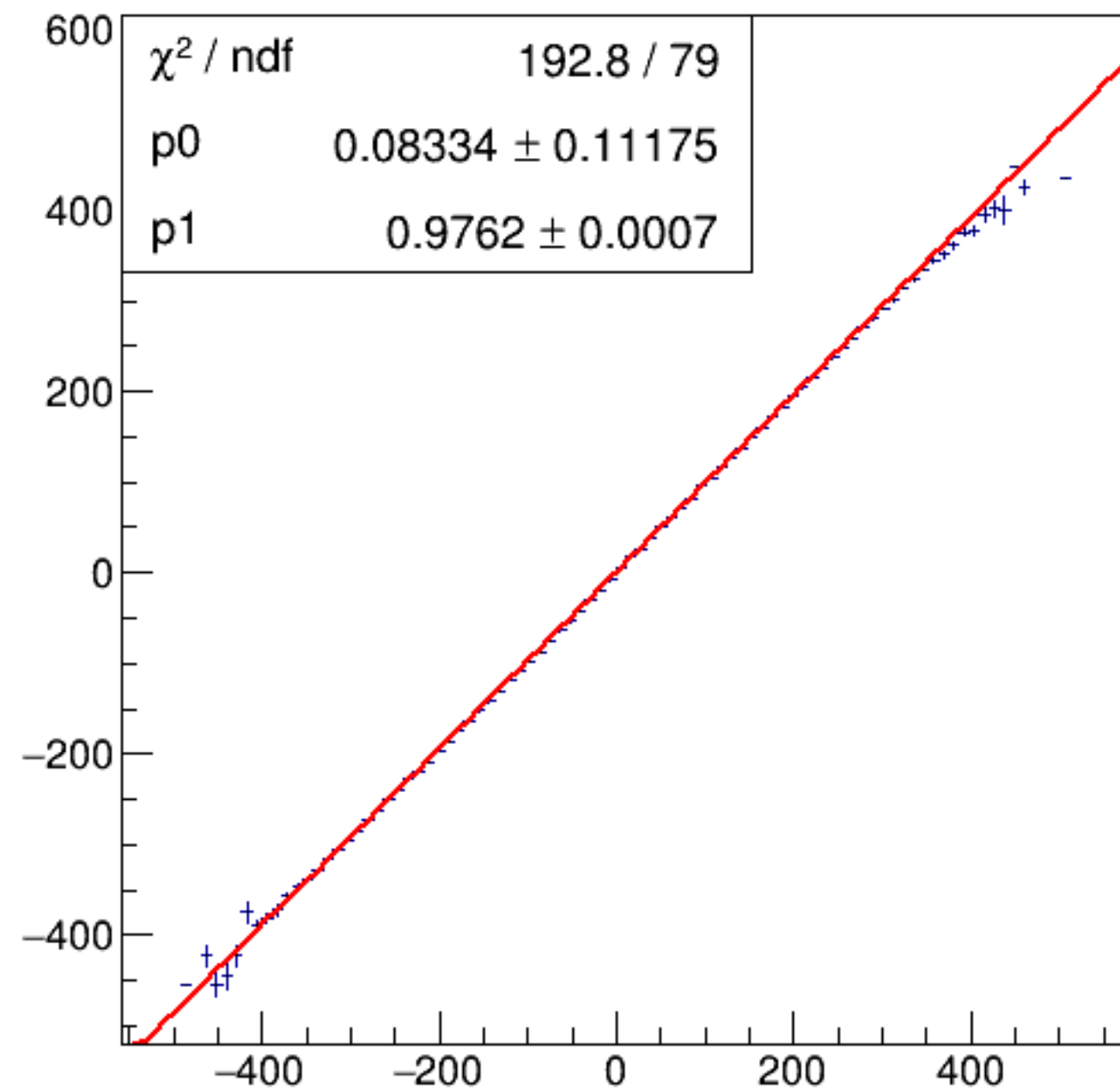
run3996_000_asym_bcm_an_us_vs_asym_bcm_an_ds3_mul.png
