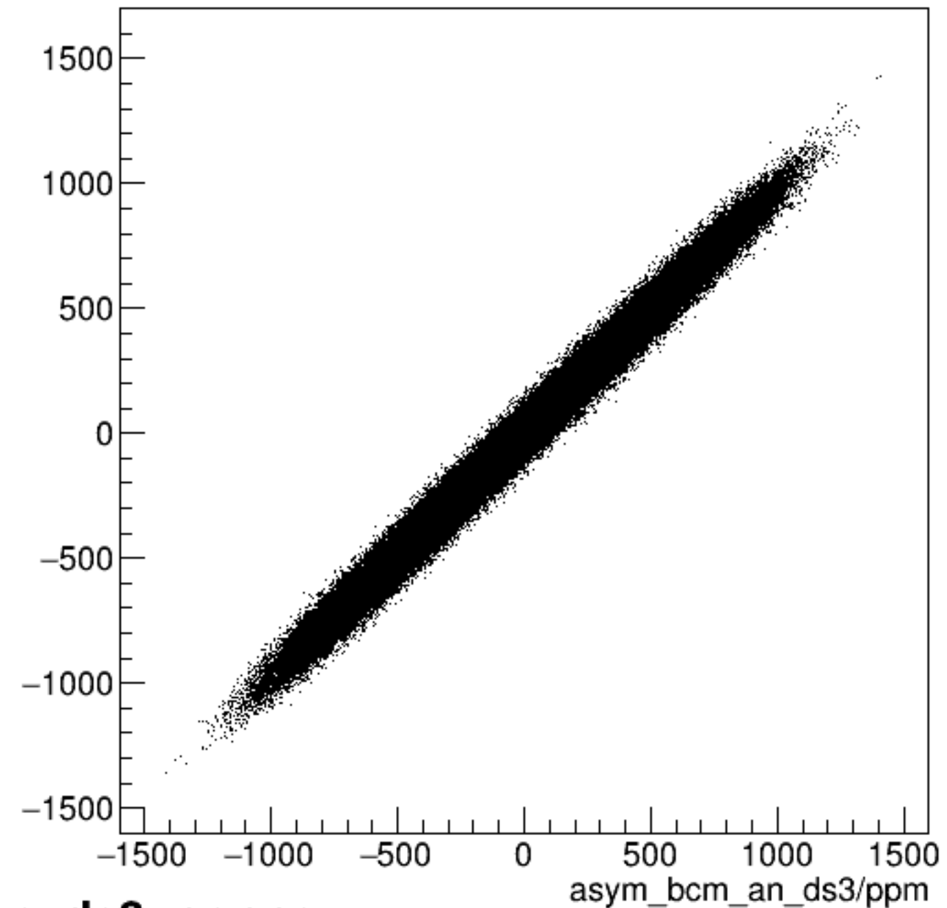
run3996_000_asym_bcm_an_us_vs_asym_bcm_an_ds3_pr.png
