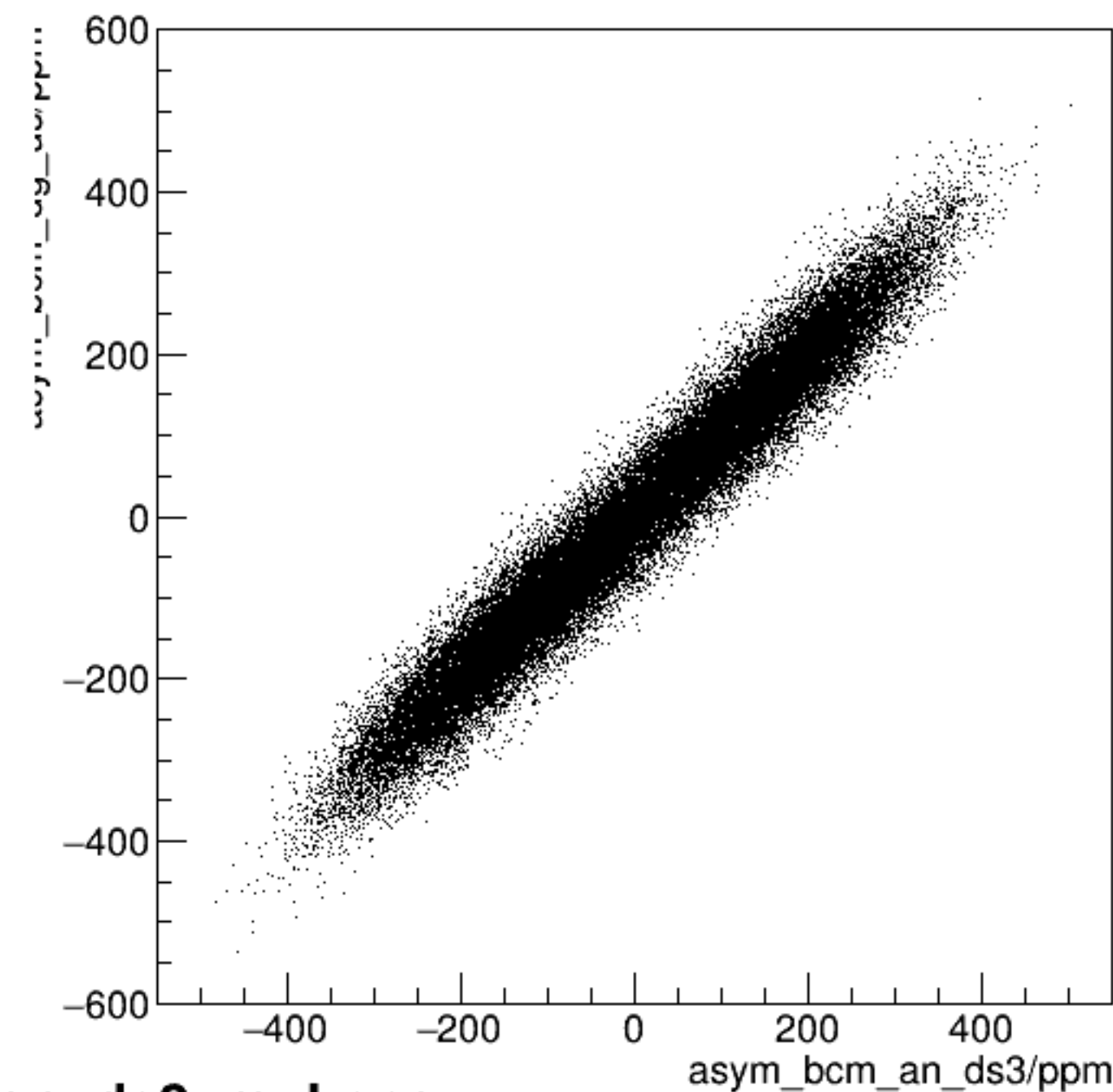
run3996_000_asym_bcm_dg_us_vs_asym_bcm_an_ds3_mul.png
