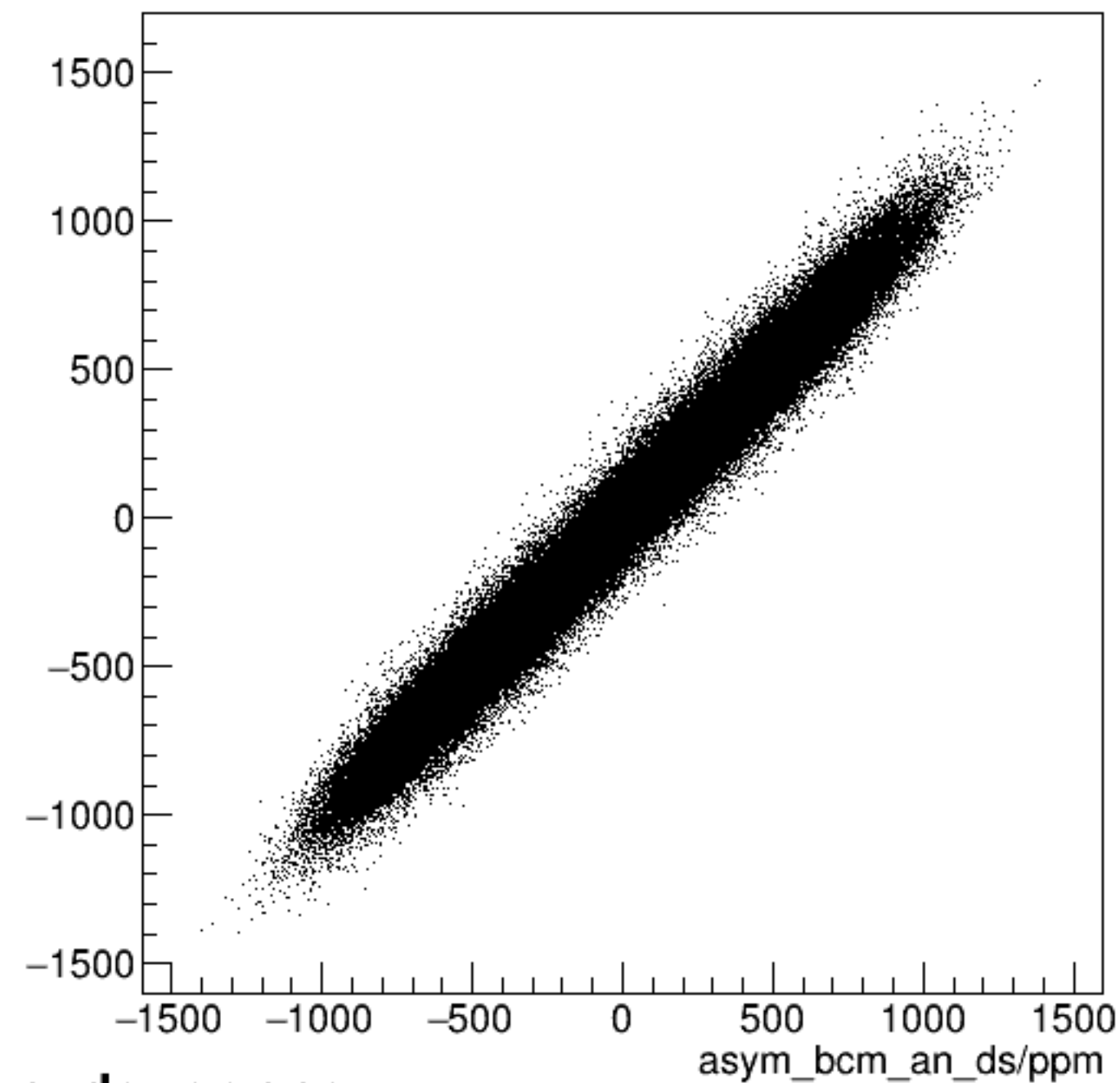
run3996_000_asym_bcm_dg_us_vs_asym_bcm_an_ds_pr.png
