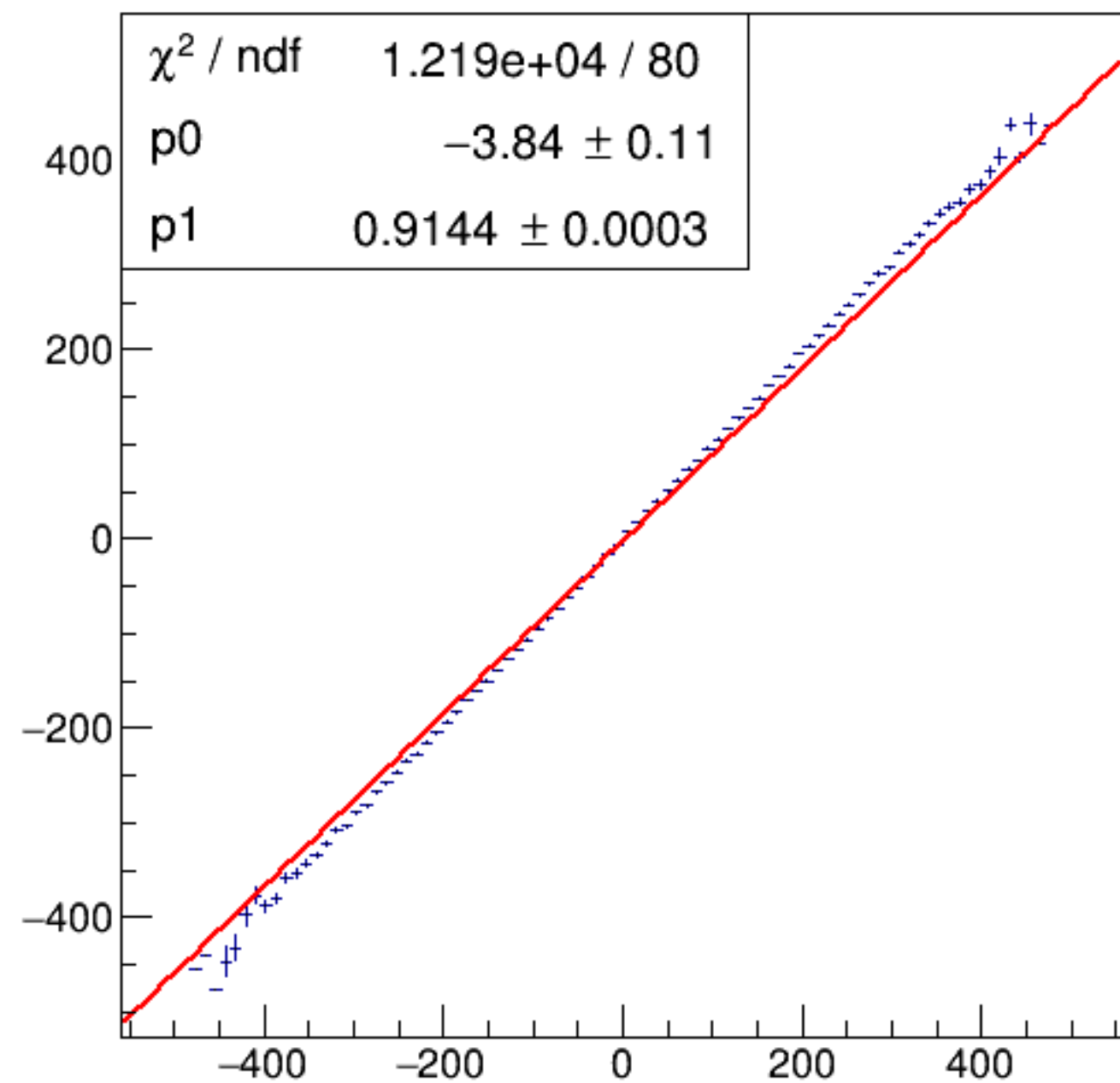
run3996_000_asym_bcm_an_us_vs_asym_bcm_an_ds_mul.png
